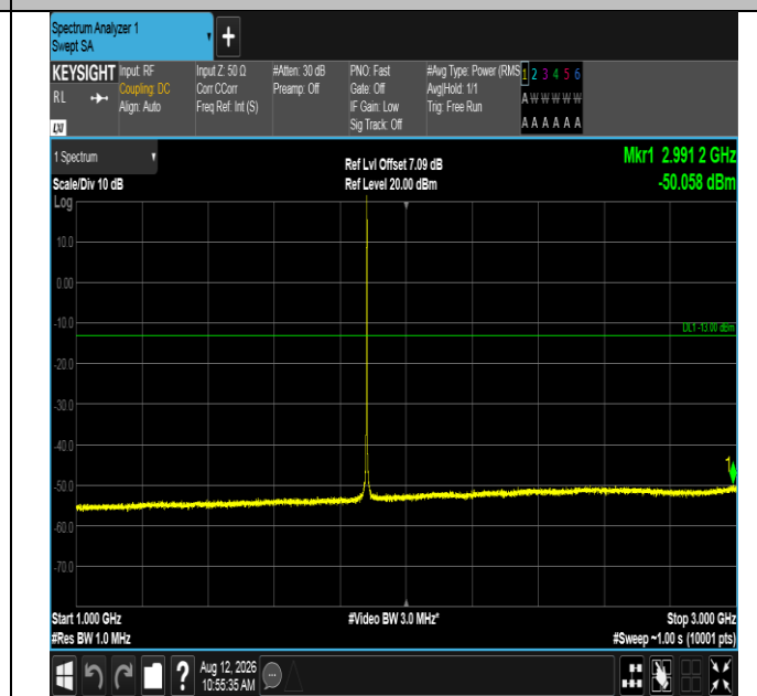
Band2-1.4MHz-16QAM-18900-1RB#5-1000~3000-PASS
