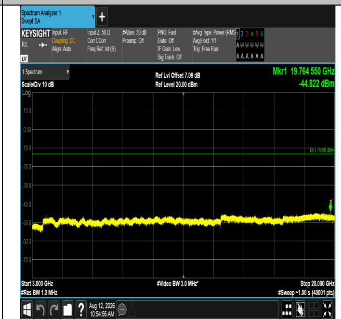
Band2-1.4MHz-QPSK-18900-1RB#5-3000~20000-PASS
