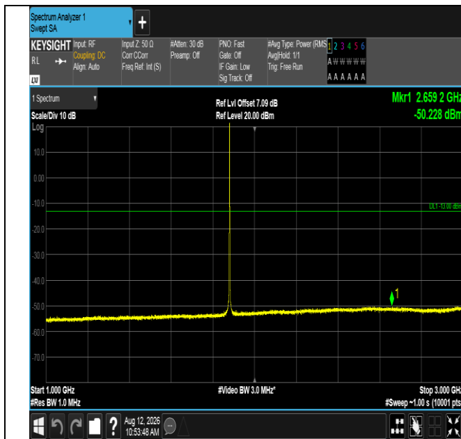
Band2-1.4MHz-16QAM-18900-1RB#0-1000~3000-PASS
