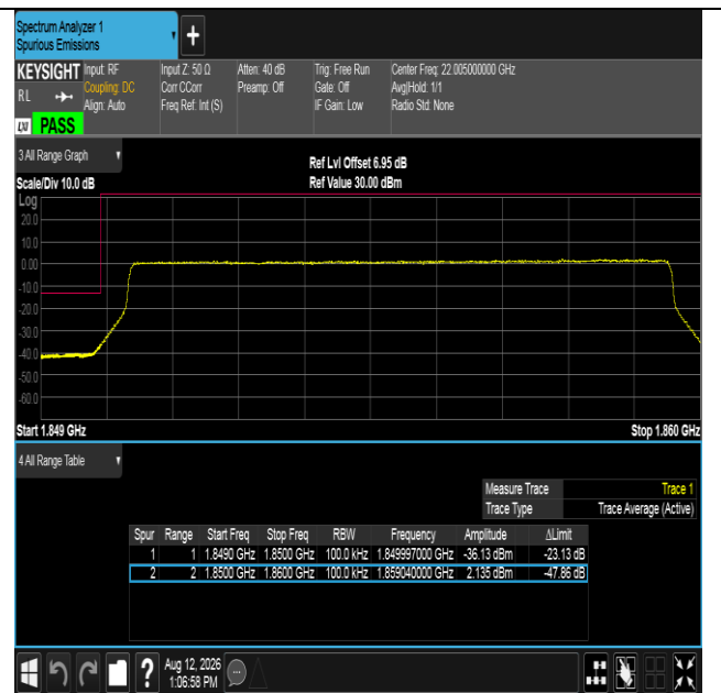
Band2-10MHz-16QAM-18650-50RB#0-PASS
