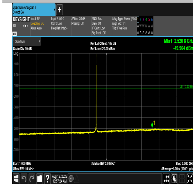
Band2-1.4MHz-16QAM-18900-6RB#0-1000~3000-PASS
