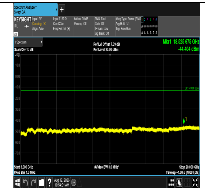
Band2-1.4MHz-16QAM-18900-1RB#0-3000~20000-PASS
