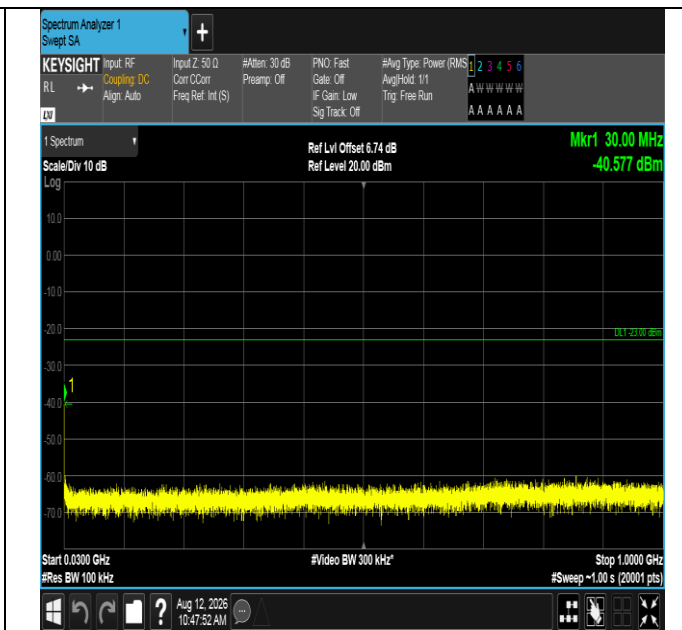
Band2-1.4MHz-16QAM-18607-1RB#0-30~1000-PASS
