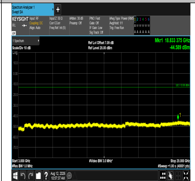
Band2-1.4MHz-16QAM-18900-6RB#0-3000~20000-PASS
