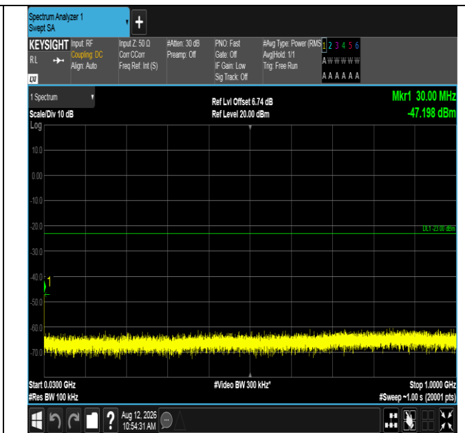
Band2-1.4MHz-QPSK-18900-1RB#5-30~1000-PASS
