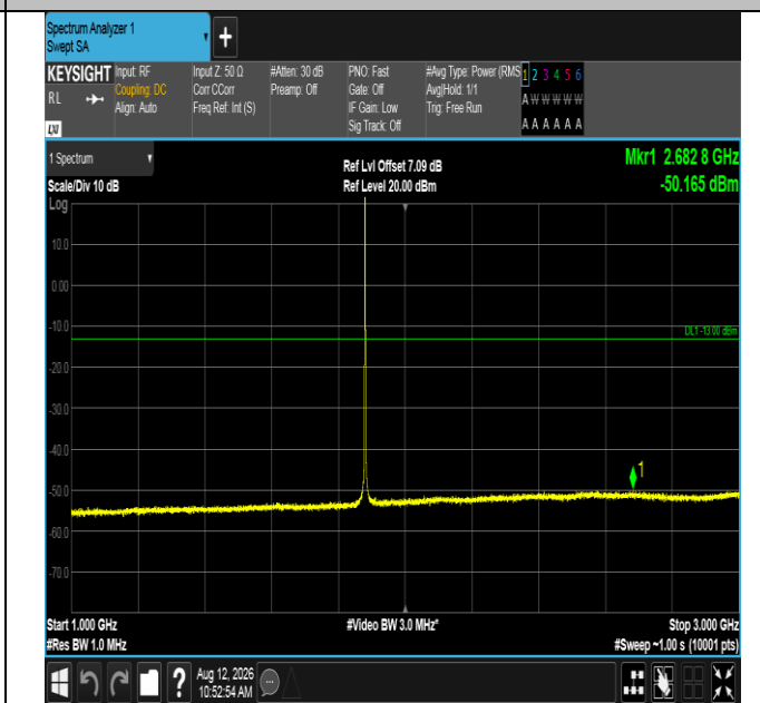
Band2-1.4MHz-QPSK-18900-1RB#0-1000~3000-PASS
