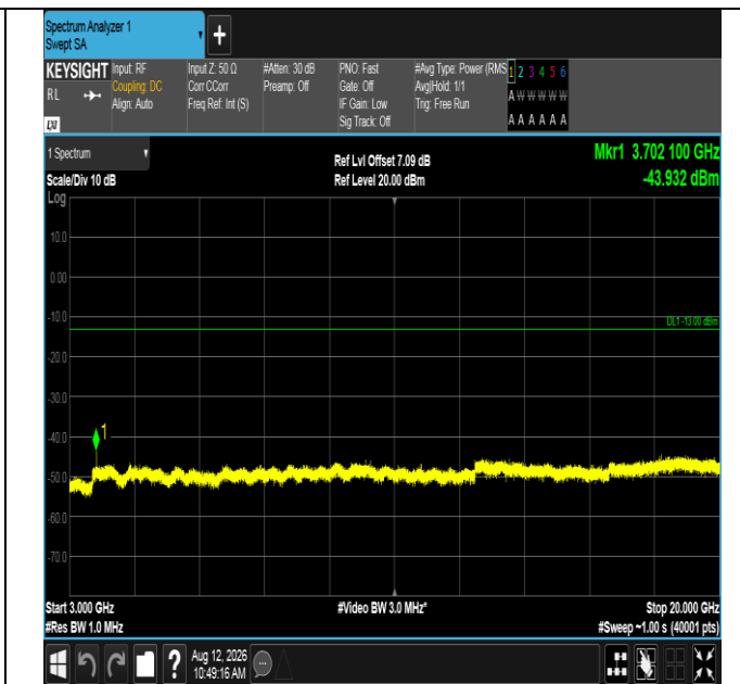
Band2-1.4MHz-QPSK-18607-1RB#5-3000~20000-PASS
