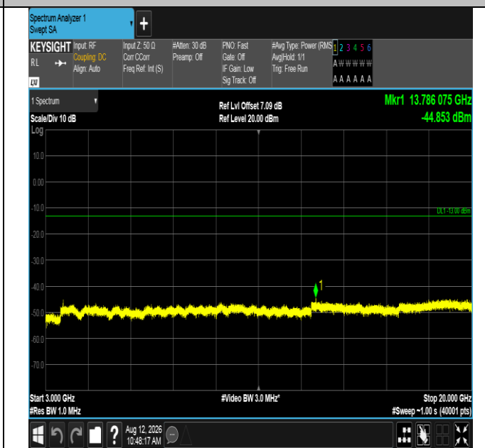
Band2-1.4MHz-16QAM-18607-1RB#0-3000~20000-PASS
