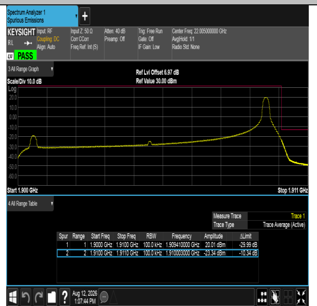
Band2-10MHz-QPSK-19150-1RB#49-PASS
