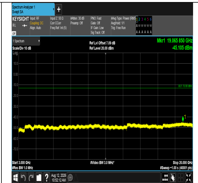
Band2-1.4MHz-16QAM-18607-6RB#0-3000~20000-PASS
