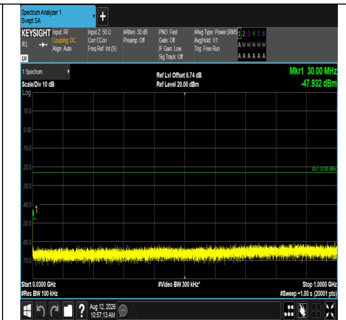
Band2-1.4MHz-16QAM-18900-6RB#0-30~1000-PASS
