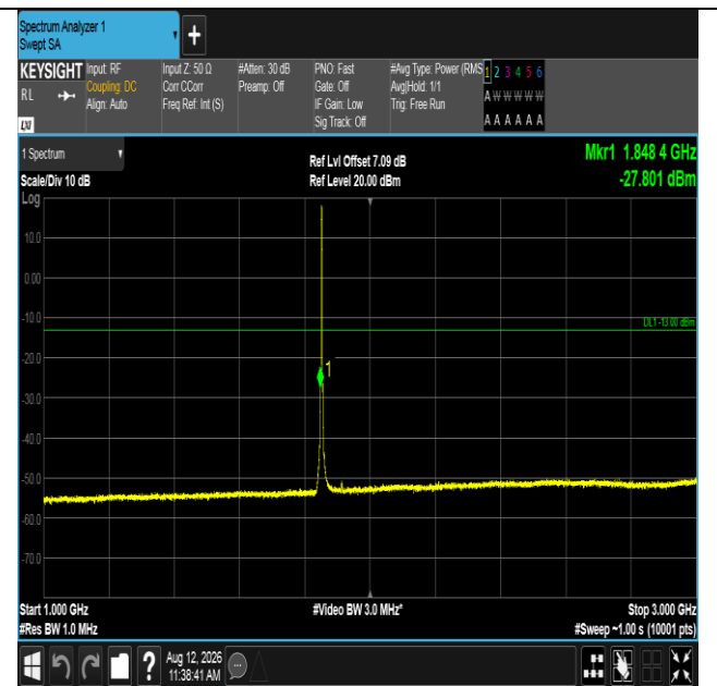
Band2-3MHz-QPSK-18615-15RB#0-1000~3000-PASS
