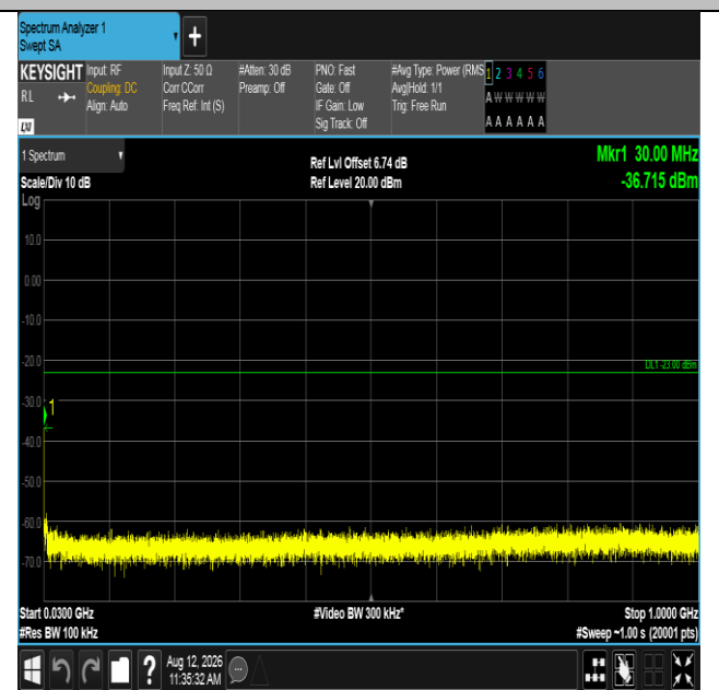
Band2-3MHz-16QAM-18615-1RB#0-30~1000-PASS
