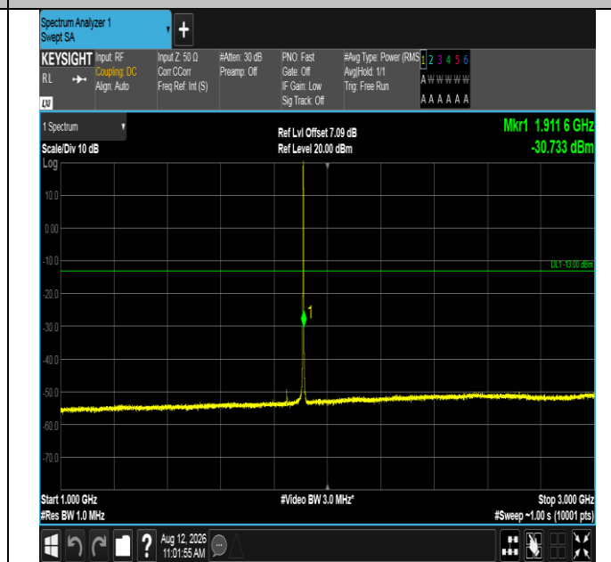
Band2-1.4MHz-QPSK-19193-6RB#0-1000~3000-PASS
