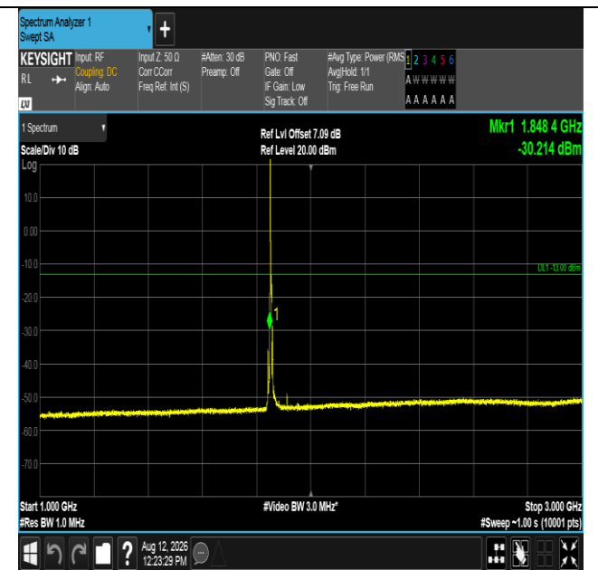
Band2-5MHz-QPSK-18625-1RB#0-1000~3000-PASS
