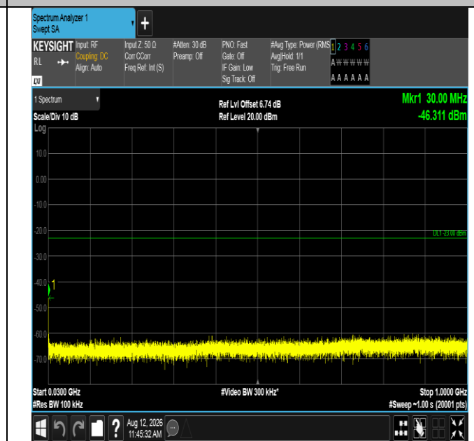
Band2-3MHz-16QAM-18900-15RB#0-30~1000-PASS
