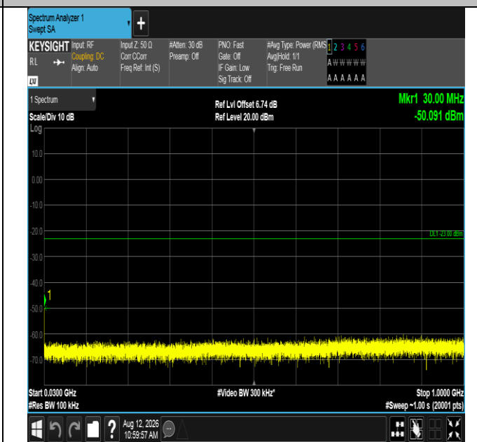
Band2-1.4MHz-QPSK-19193-1RB#5-30~1000-PASS
