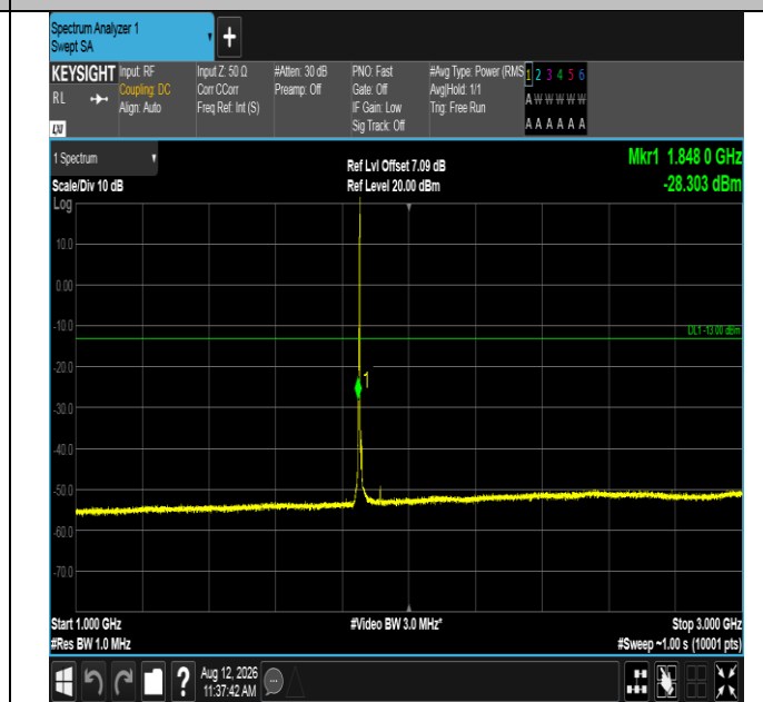
Band2-3MHz-16QAM-18615-1RB#14-1000~3000-PASS
