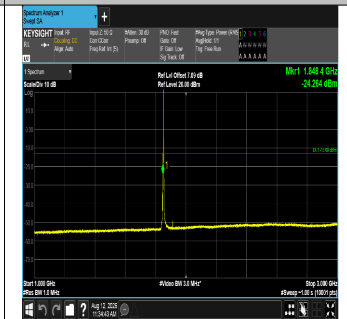
Band2-3MHz-QPSK-18615-1RB#0-1000~3000-PASS
