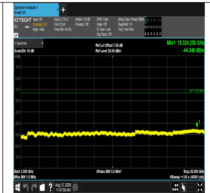
Band2-3MHz-16QAM-19185-1RB#0-3000~20000-PASS
