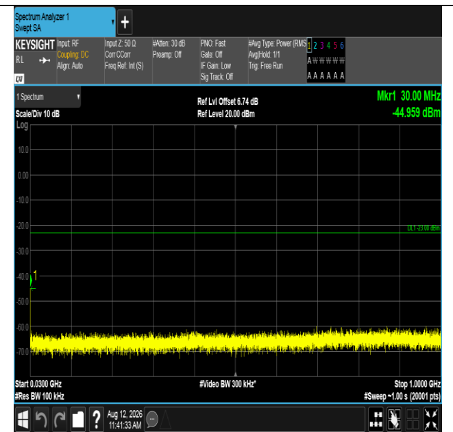
Band2-3MHz-16QAM-18900-1RB#0-30~1000-PASS
