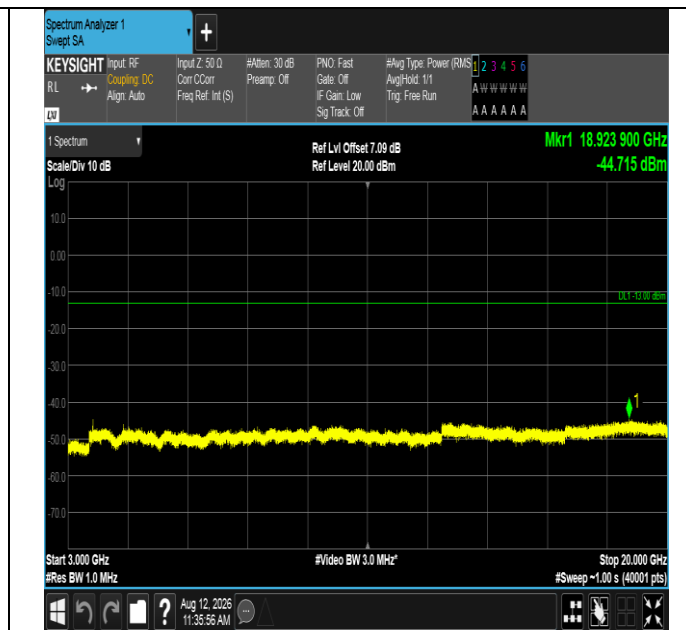
Band2-3MHz-16QAM-18615-1RB#0-3000~20000-PASS
