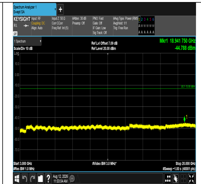
Band2-1.4MHz-16QAM-19193-6RB#0-3000~20000-PASS
