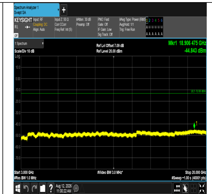
Band2-1.4MHz-QPSK-19193-1RB#5-3000~20000-PASS
