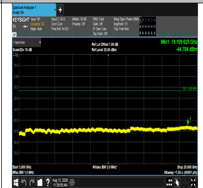
Band2-3MHz-16QAM-18615-15RB#0-3000~20000-PASS
