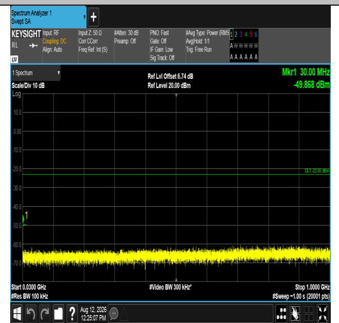
Band2-5MHz-QPSK-18625-1RB#24-30~1000-PASS
