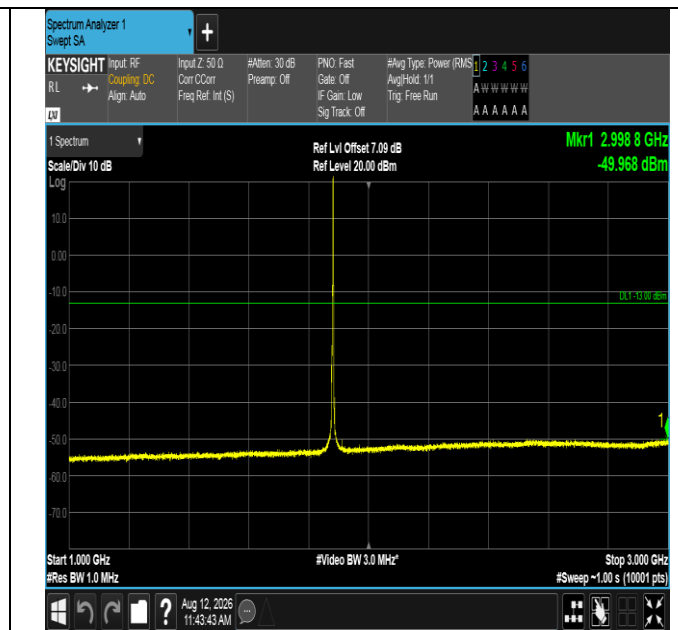
Band2-3MHz-16QAM-18900-1RB#14-1000~3000-PASS
