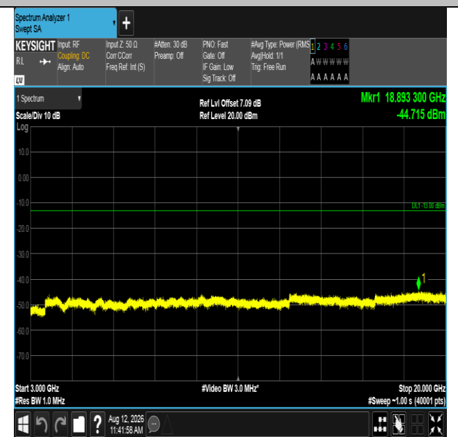
Band2-3MHz-16QAM-18900-1RB#0-3000~20000-PASS
