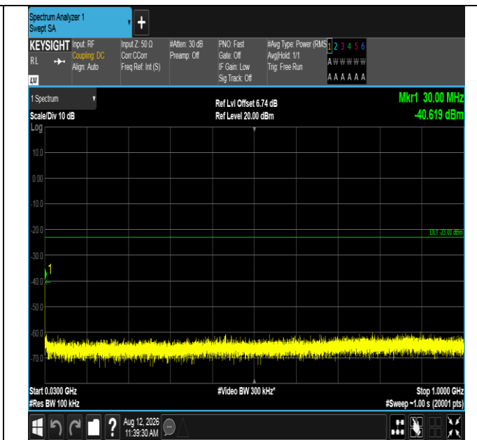
Band2-3MHz-16QAM-18615-15RB#0-30~1000-PASS
