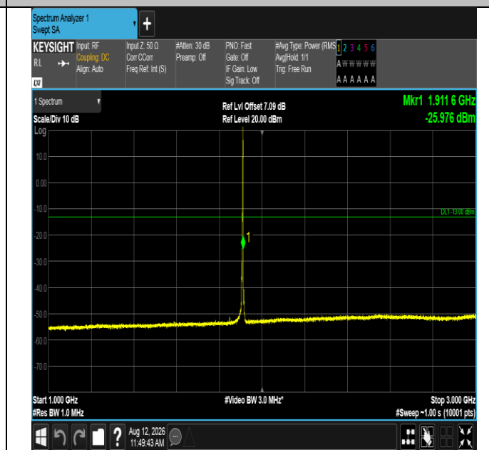
Band2-3MHz-16QAM-19185-1RB#14-1000~3000-PASS
