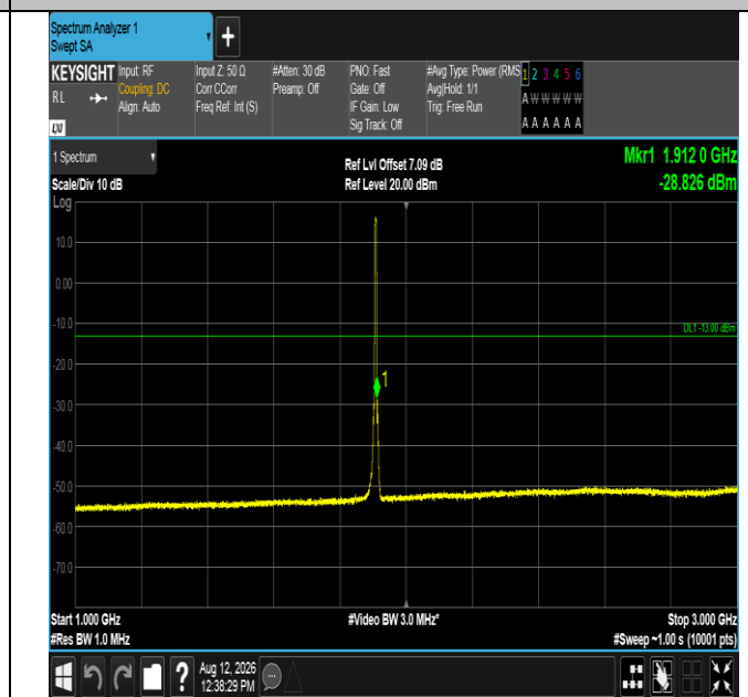
Band2-5MHz-QPSK-19175-25RB#0-1000~3000-PASS
