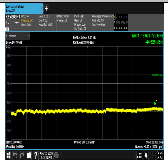
Band2-10MHz-QPSK-18650-1RB#49-3000~20000-PASS
