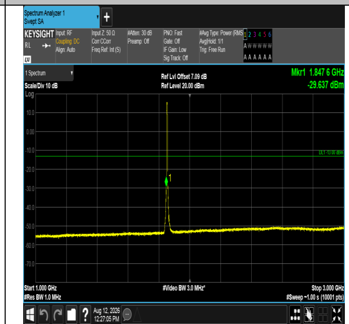
Band2-5MHz-QPSK-18625-25RB#0-1000~3000-PASS
