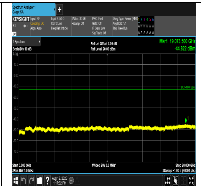
Band2-10MHz-QPSK-18900-1RB#49-3000~20000-PASS
