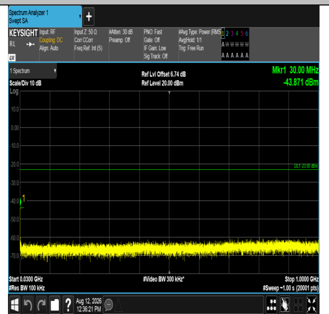
Band2-5MHz-QPSK-19175-1RB#24-30~1000-PASS
