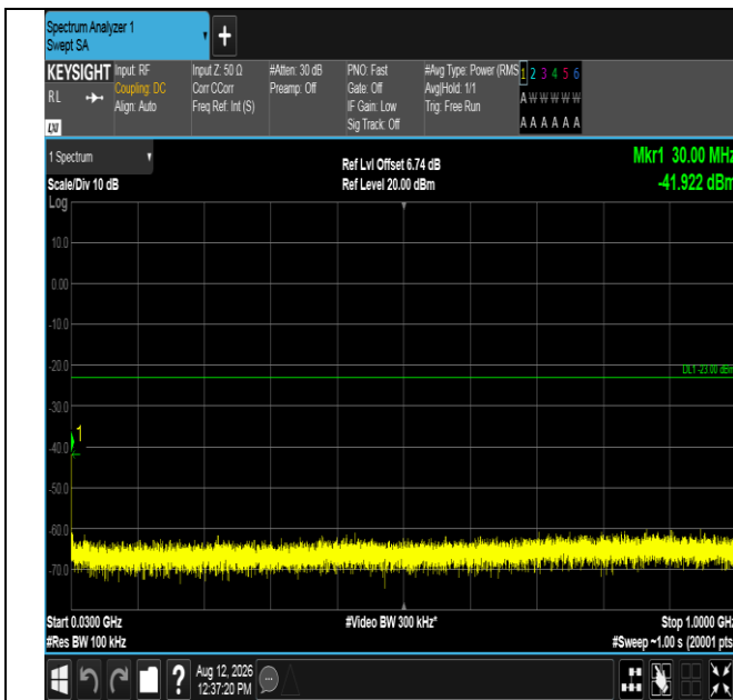
Band2-5MHz-16QAM-19175-1RB#24-30~1000-PASS
