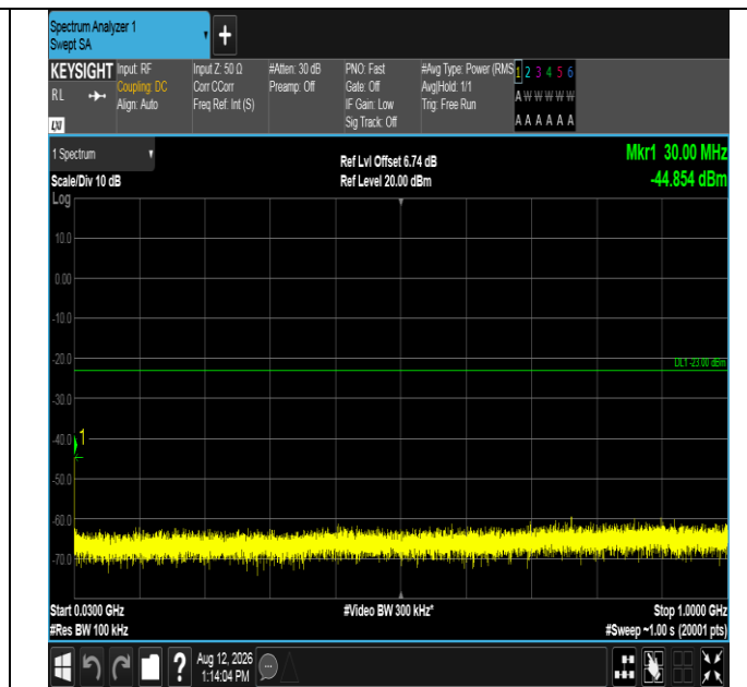
Band2-10MHz-16QAM-18650-50RB#0-30~1000-PASS
