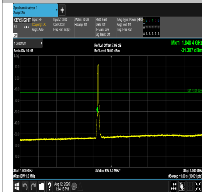
Band2-10MHz-16QAM-18650-50RB#0-1000~3000-PASS
