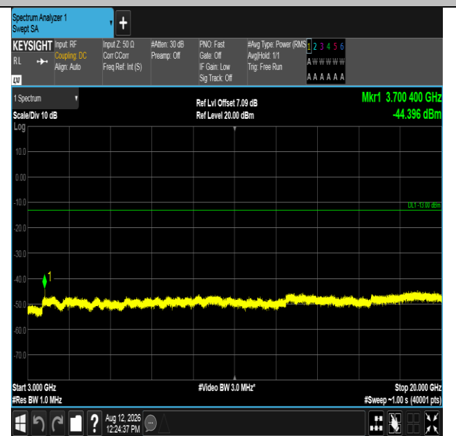
Band2-5MHz-16QAM-18625-1RB#0-3000~20000-PASS
