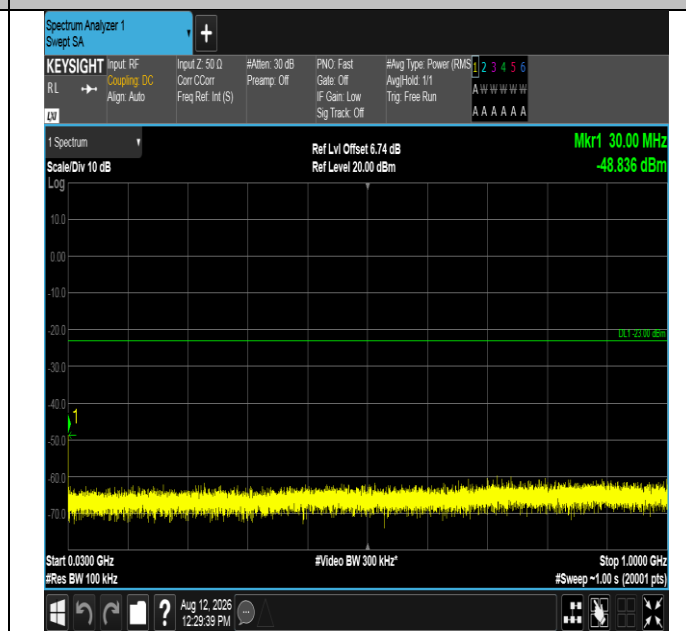
Band2-5MHz-16QAM-18900-1RB#0-30~1000-PASS
