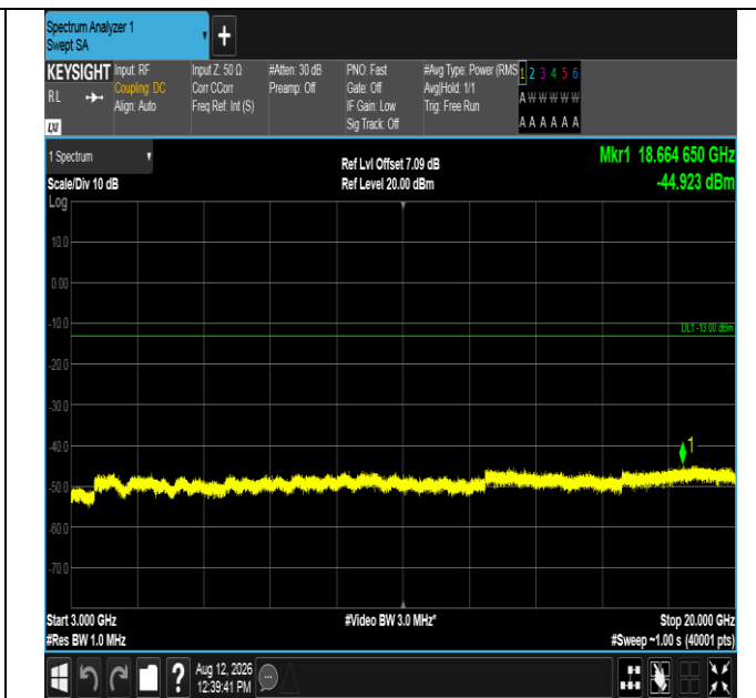
Band2-5MHz-16QAM-19175-25RB#0-3000~20000-PASS
