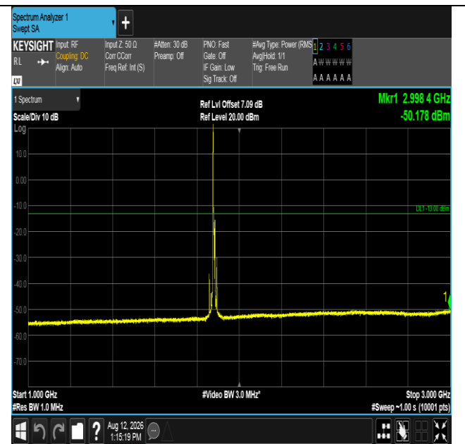
Band2-10MHz-QPSK-18900-1RB#0-1000~3000-PASS
