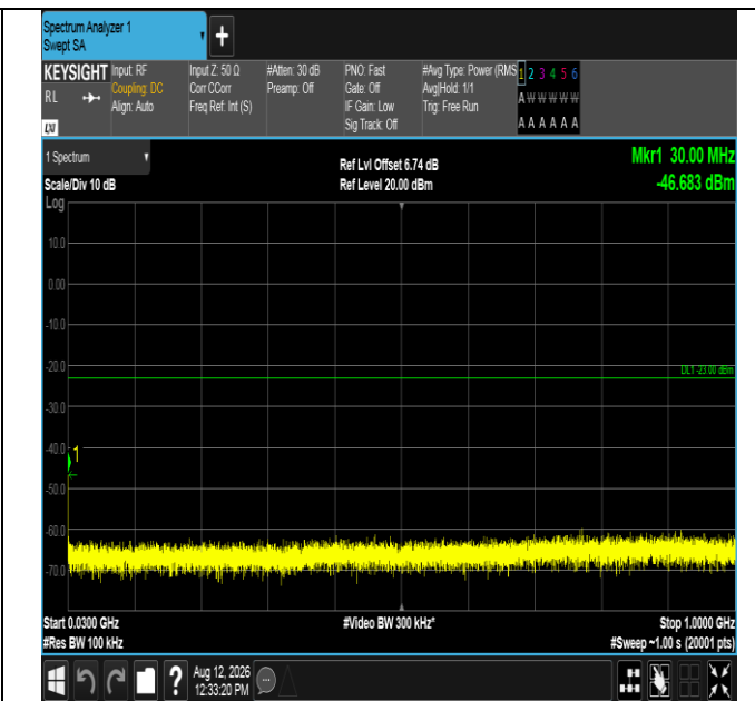
Band2-5MHz-16QAM-18900-25RB#0-30~1000-PASS
