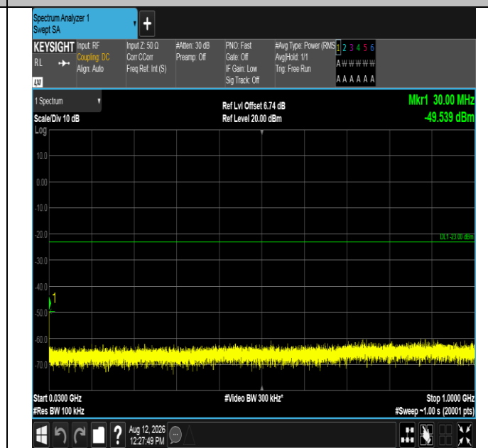
Band2-5MHz-16QAM-18625-25RB#0-30~1000-PASS
