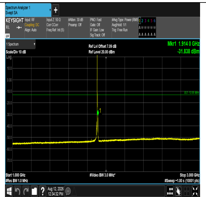
Band2-5MHz-QPSK-19175-1RB#0-1000~3000-PASS
