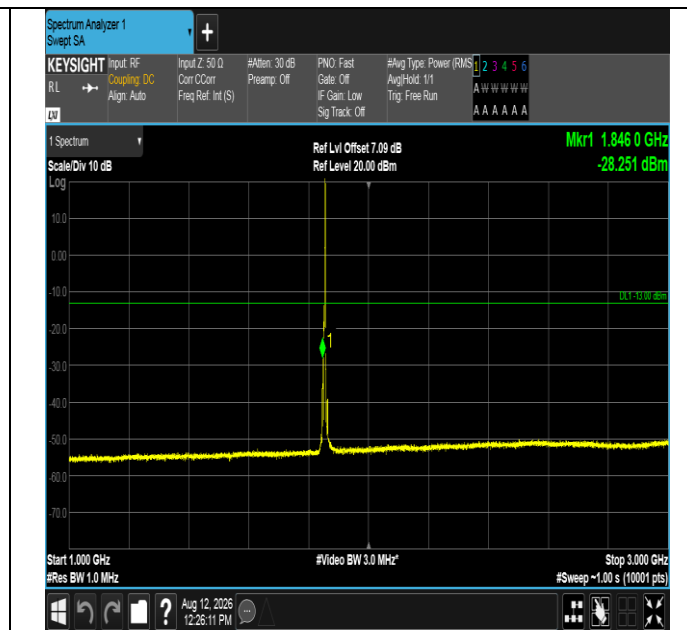
Band2-5MHz-16QAM-18625-1RB#24-1000~3000-PASS
