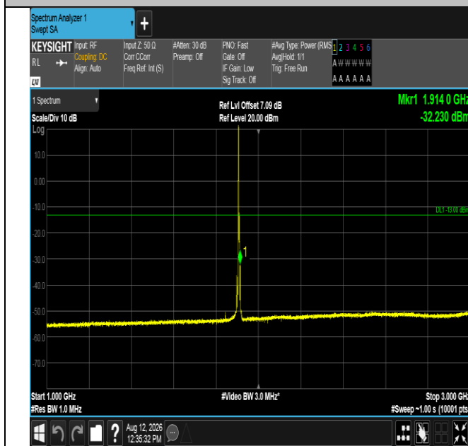
Band2-5MHz-16QAM-19175-1RB#0-1000~3000-PASS
