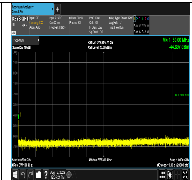
Band2-5MHz-16QAM-19175-1RB#0-30~1000-PASS
