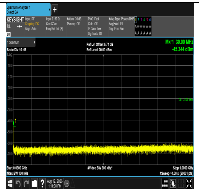
Band2-10MHz-QPSK-18650-1RB#49-30~1000-PASS
