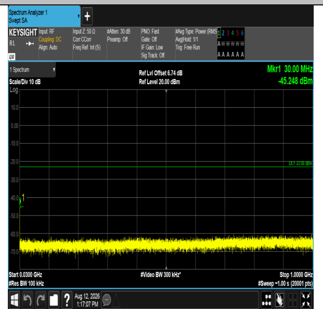
Band2-10MHz-QPSK-18900-1RB#49-30~1000-PASS
