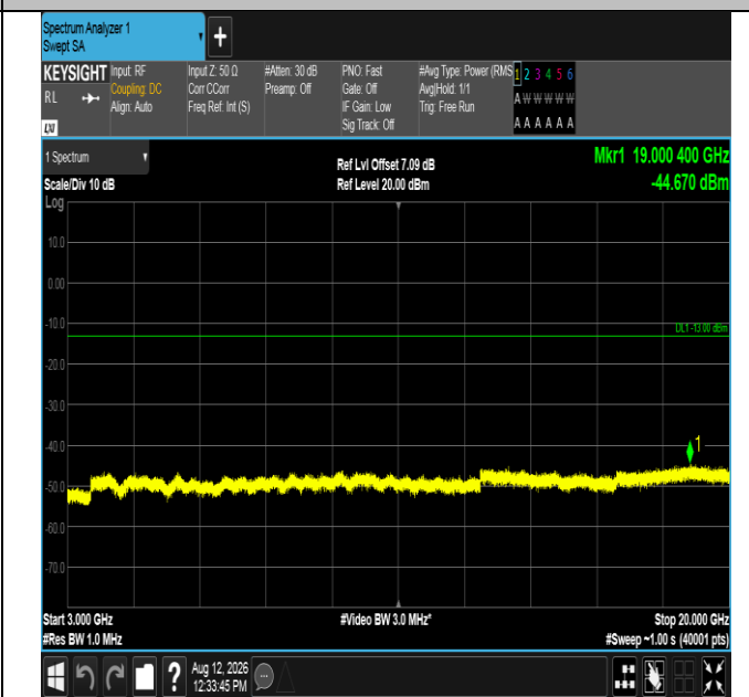
Band2-5MHz-16QAM-18900-25RB#0-3000~20000-PASS
