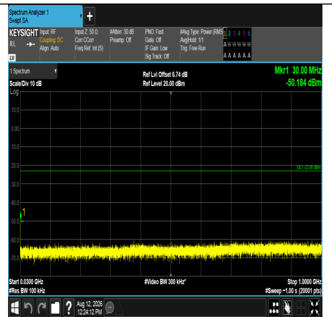
Band2-5MHz-16QAM-18625-1RB#0-30~1000-PASS
