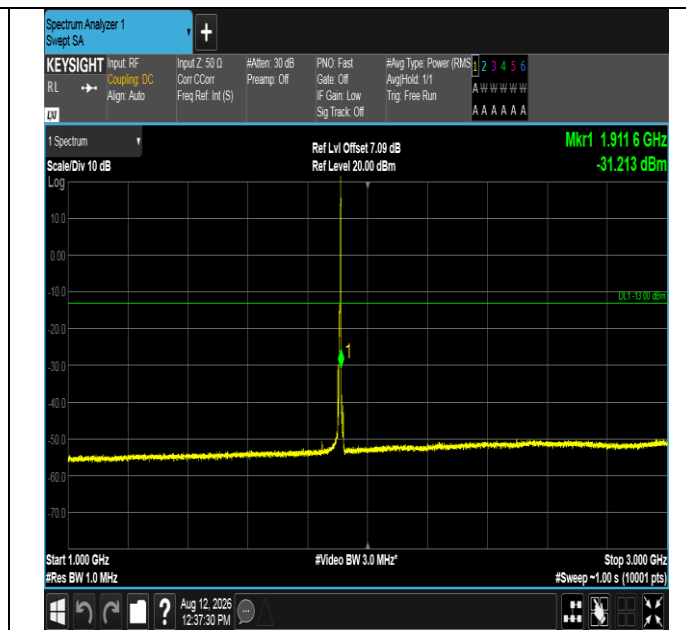
Band2-5MHz-16QAM-19175-1RB#24-1000~3000-PASS
