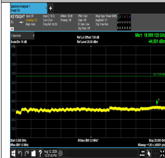
Band2-5MHz-16QAM-19175-1RB#24-3000~20000-PASS
