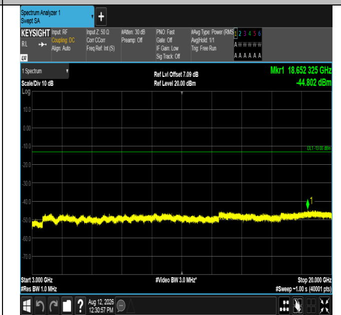
Band2-5MHz-QPSK-18900-1RB#24-3000~20000-PASS
