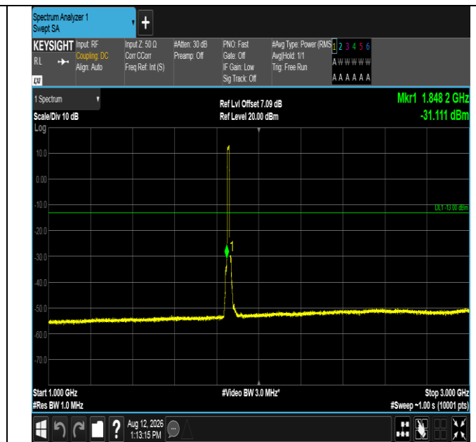
Band2-10MHz-QPSK-18650-50RB#0-1000~3000-PASS
