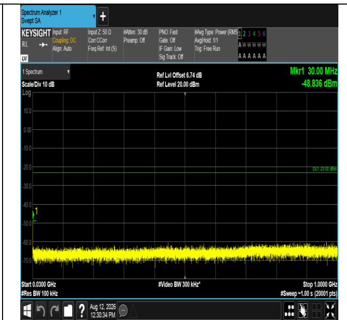
Band2-5MHz-QPSK-18900-1RB#24-30~1000-PASS
