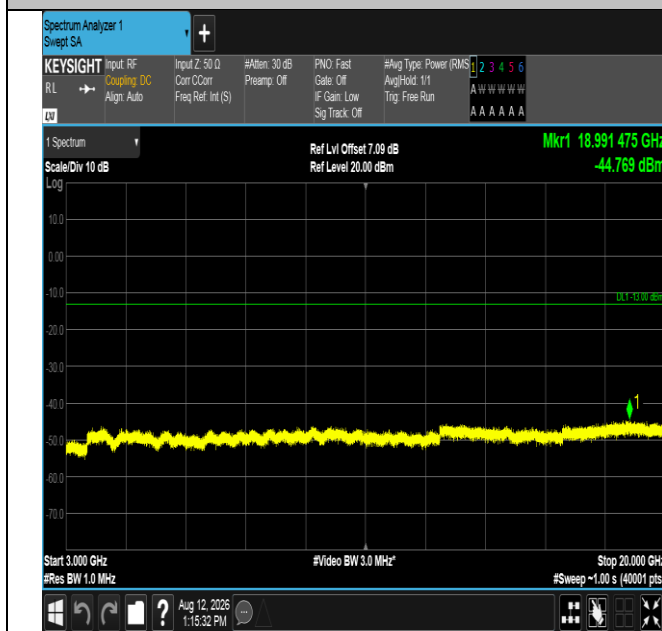
Band2-10MHz-QPSK-18900-1RB#0-3000~20000-PASS
