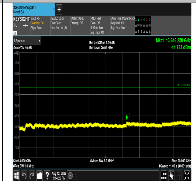
Band2-10MHz-16QAM-18650-50RB#0-3000~20000-PASS
