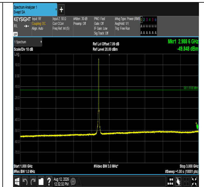
Band2-5MHz-QPSK-18900-25RB#0-1000~3000-PASS
