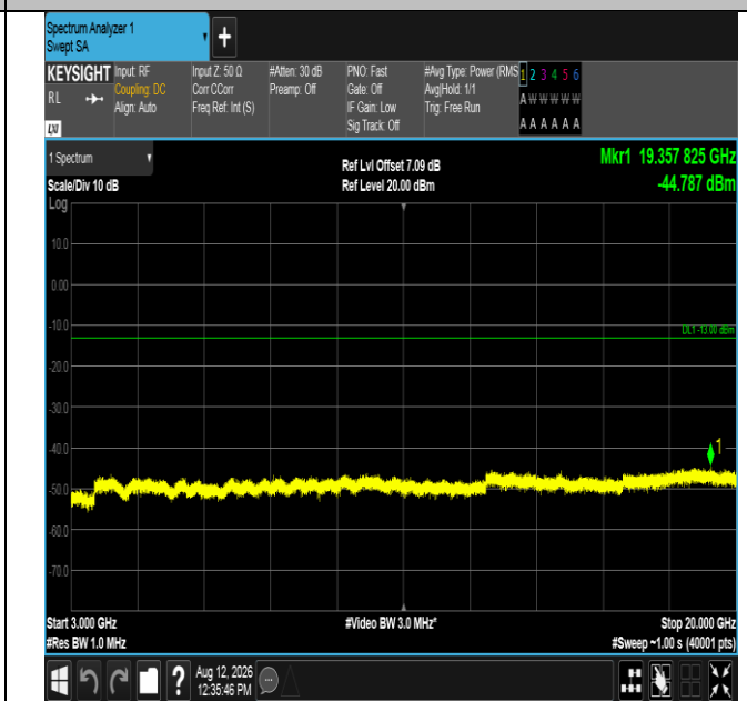
Band2-5MHz-16QAM-19175-1RB#0-3000~20000-PASS
