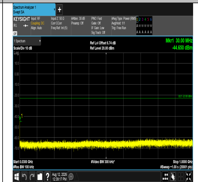
Band2-5MHz-16QAM-19175-25RB#0-30~1000-PASS
