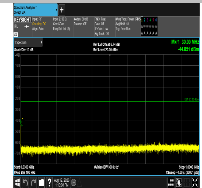
Band2-10MHz-16QAM-18650-1RB#0-30~1000-PASS
