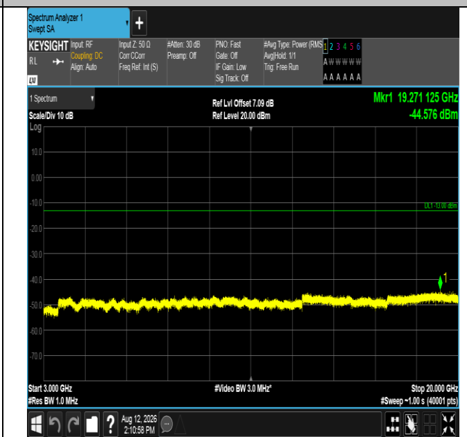
Band2-15MHz-16QAM-19125-1RB#0-3000~20000-PASS
