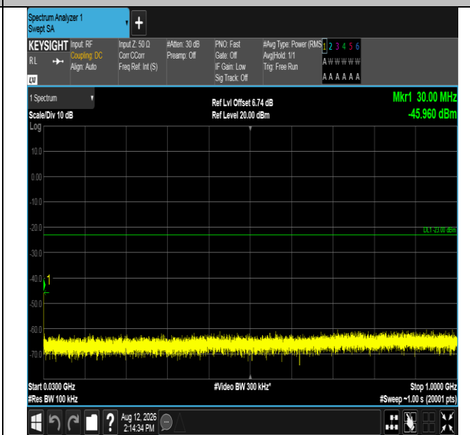
Band2-15MHz-16QAM-19125-75RB#0-30~1000-PASS
