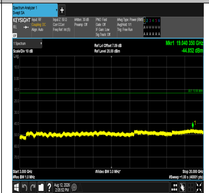
Band2-15MHz-QPSK-18900-1RB#74-3000~20000-PASS
