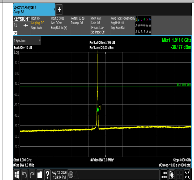
Band2-10MHz-16QAM-19150-1RB#49-1000~3000-PASS
