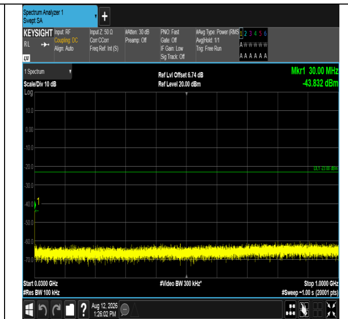
Band2-10MHz-16QAM-19150-50RB#0-30~1000-PASS
