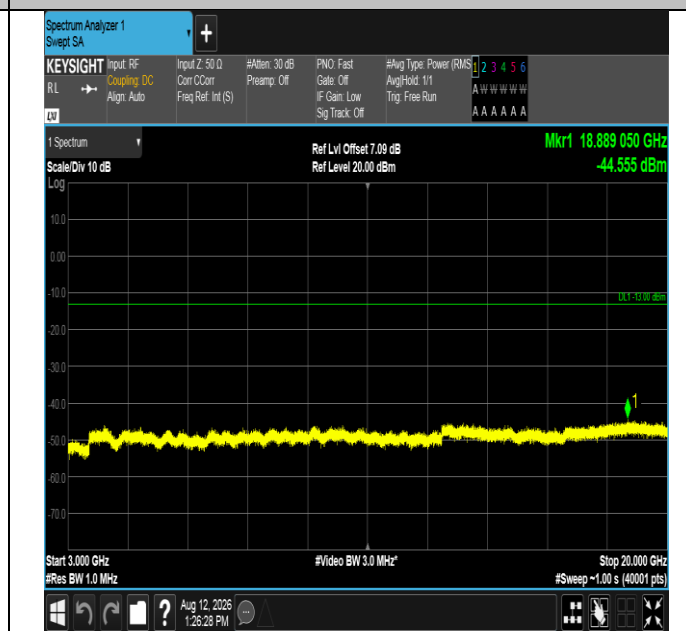
Band2-10MHz-16QAM-19150-50RB#0-3000~20000-PASS
