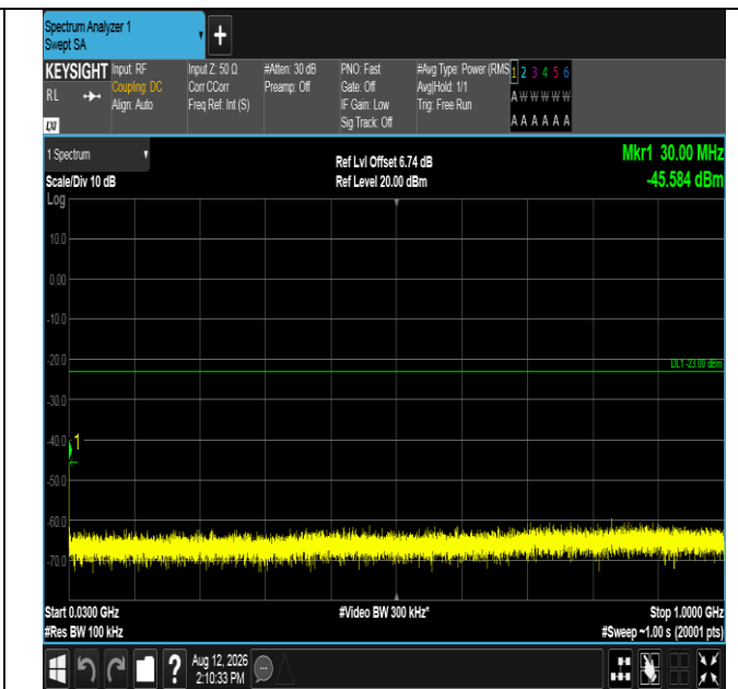
Band2-15MHz-16QAM-19125-1RB#0-30~1000-PASS
