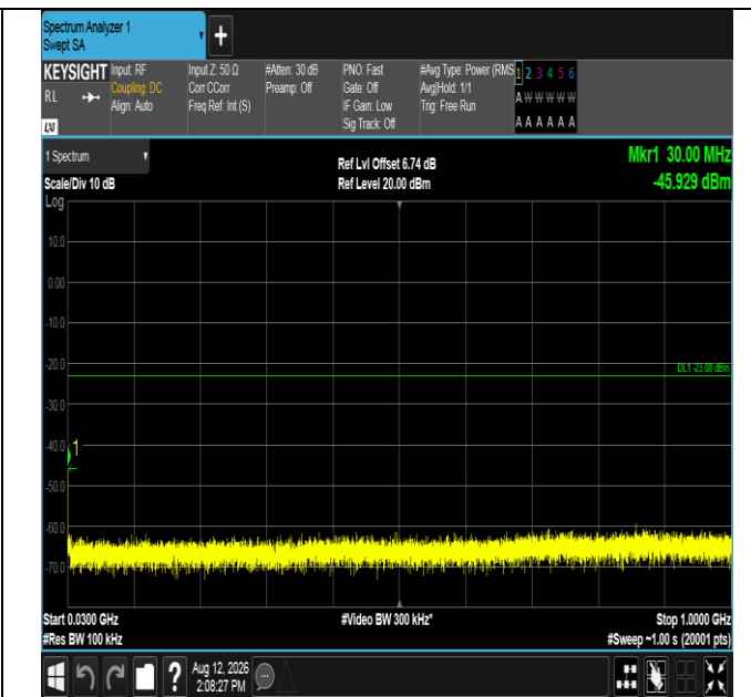
Band2-15MHz-16QAM-18900-75RB#0-30~1000-PASS
