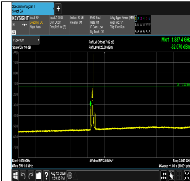
Band2-15MHz-QPSK-18675-1RB#74-1000~3000-PASS
