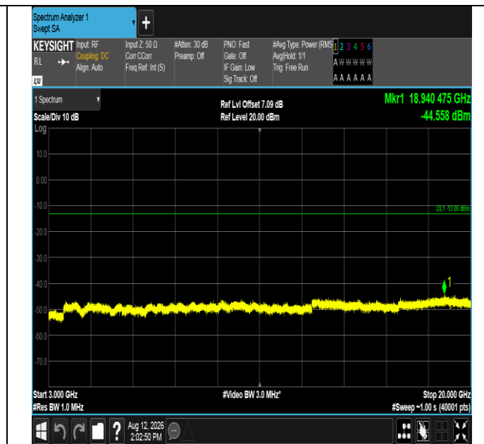
Band2-15MHz-16QAM-18675-75RB#0-3000~20000-PASS
