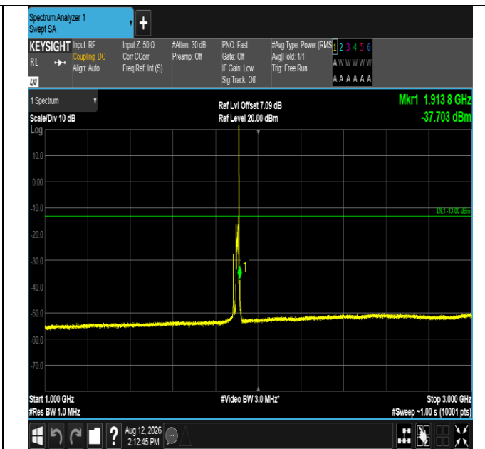
Band2-15MHz-16QAM-19125-1RB#74-1000~3000-PASS
