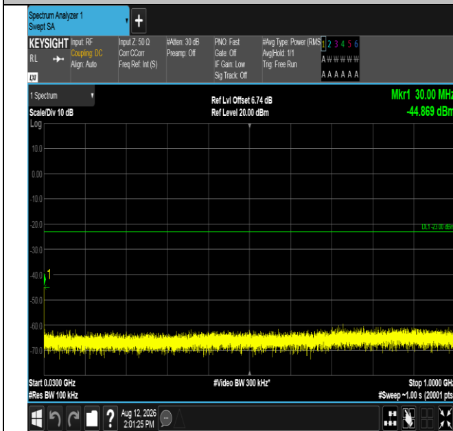
Band2-15MHz-QPSK-18675-75RB#0-30~1000-PASS
