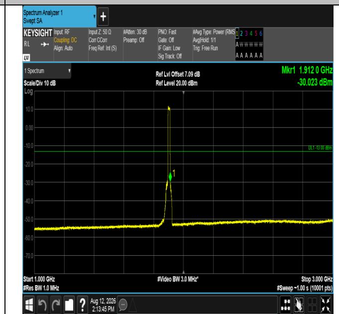
Band2-15MHz-QPSK-19125-75RB#0-1000~3000-PASS
