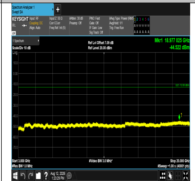
Band2-10MHz-QPSK-19150-1RB#49-3000~20000-PASS
