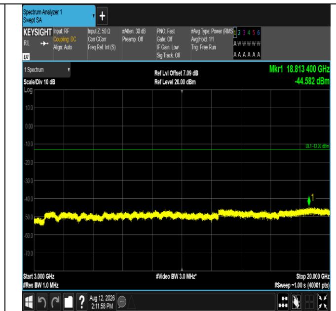
Band2-15MHz-QPSK-19125-1RB#74-3000~20000-PASS
