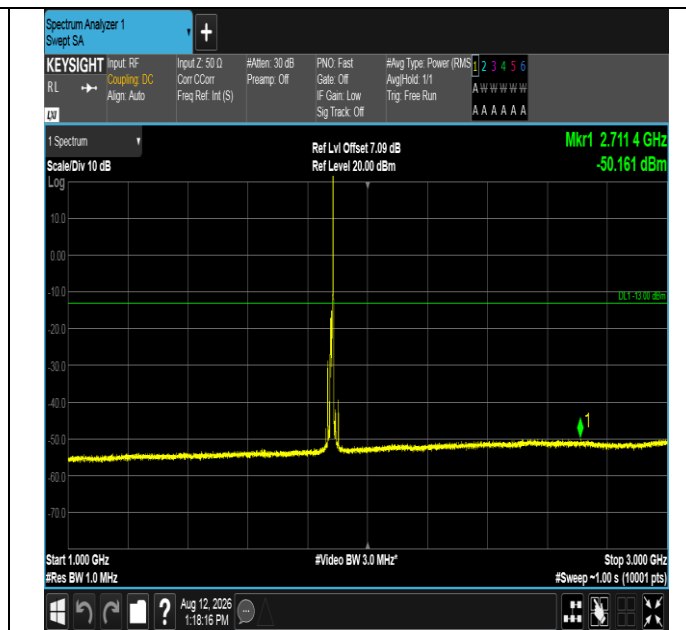
Band2-10MHz-16QAM-18900-1RB#49-1000~3000-PASS
