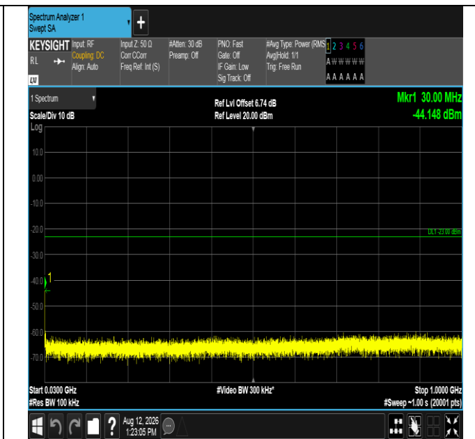
Band2-10MHz-QPSK-19150-1RB#49-30~1000-PASS
