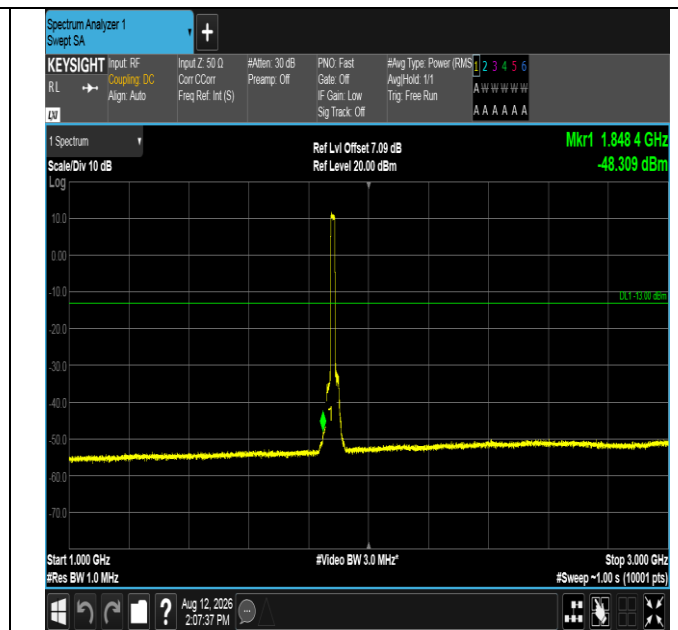
Band2-15MHz-QPSK-18900-75RB#0-1000~3000-PASS
