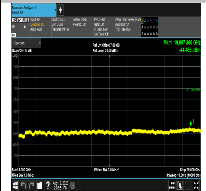
Band2-15MHz-16QAM-18900-75RB#0-3000~20000-PASS
