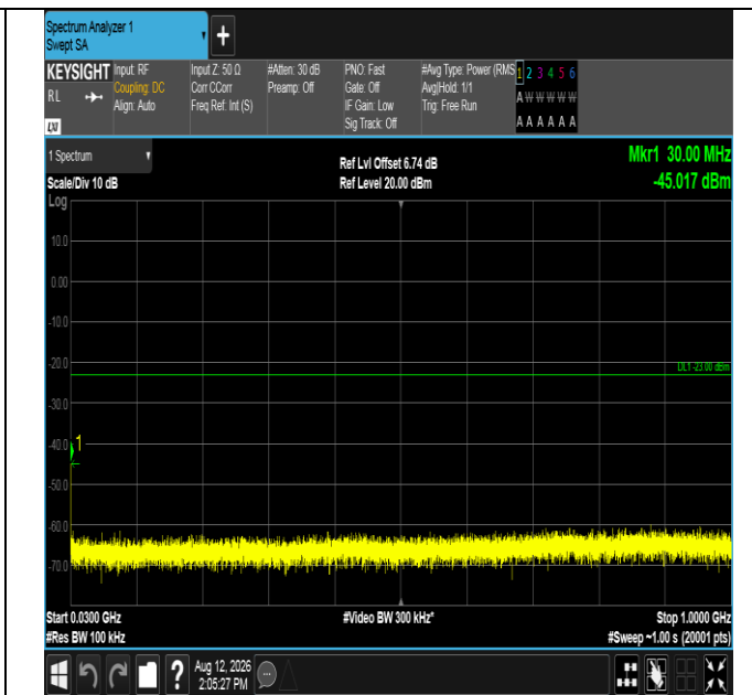
Band2-15MHz-QPSK-18900-1RB#74-30~1000-PASS
