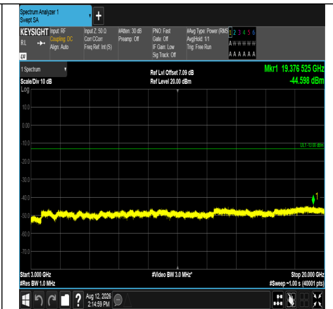
Band2-15MHz-16QAM-19125-75RB#0-3000~20000-PASS
