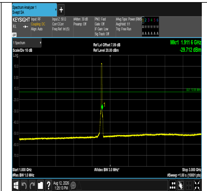
Band2-10MHz-QPSK-19150-50RB#0-1000~3000-PASS
