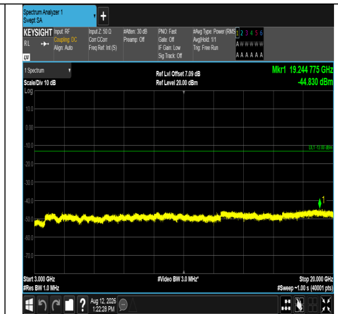
Band2-10MHz-16QAM-19150-1RB#0-3000~20000-PASS
