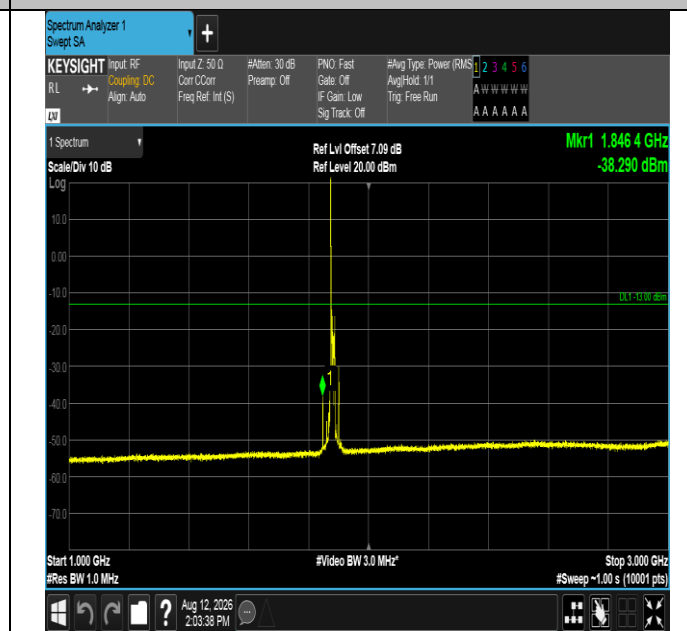
Band2-15MHz-QPSK-18900-1RB#0-1000~3000-PASS
