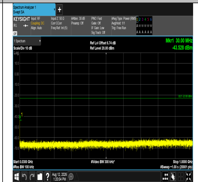
Band2-10MHz-16QAM-18900-50RB#0-30~1000-PASS
