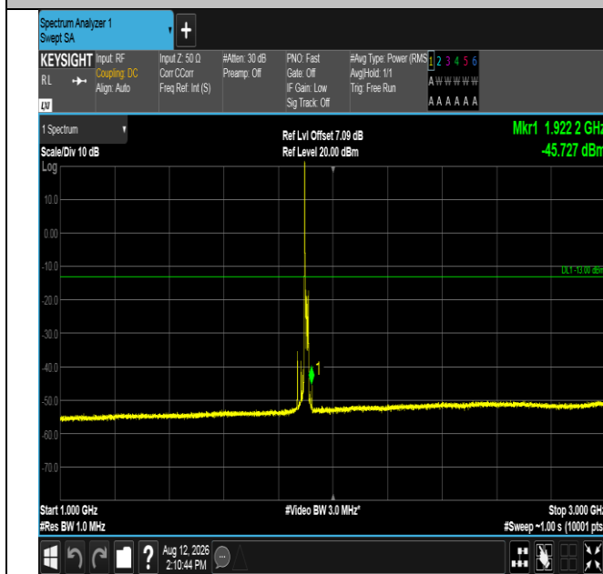
Band2-15MHz-16QAM-19125-1RB#0-1000~3000-PASS
