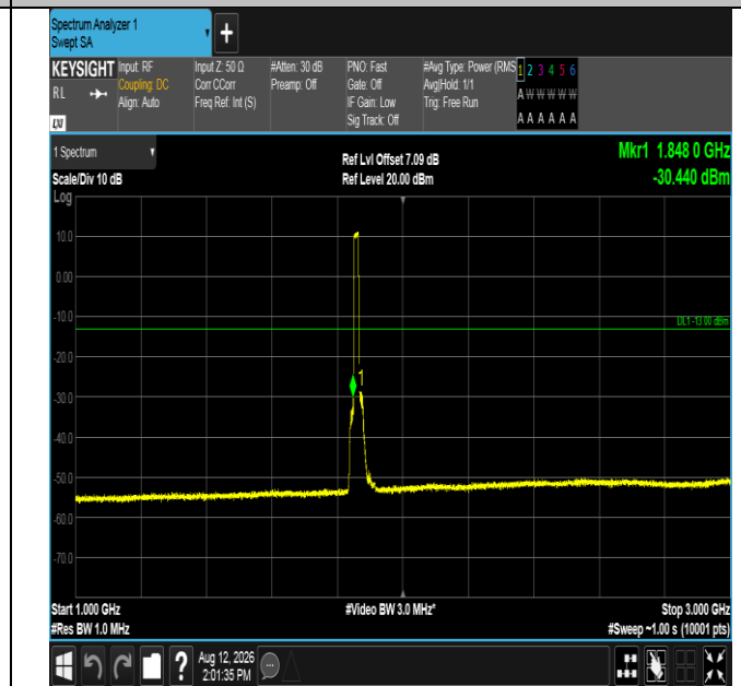
Band2-15MHz-QPSK-18675-75RB#0-1000~3000-PASS
