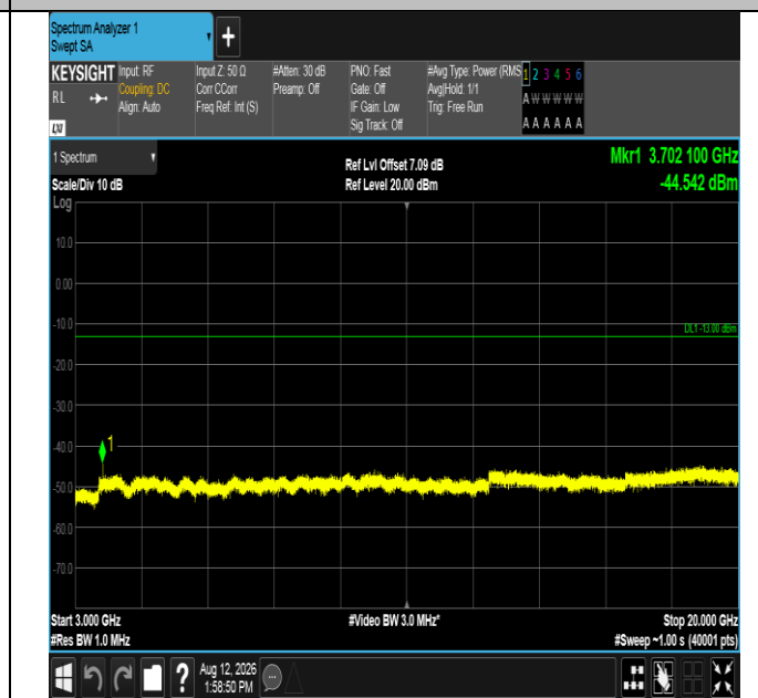
Band2-15MHz-16QAM-18675-1RB#0-3000~20000-PASS
