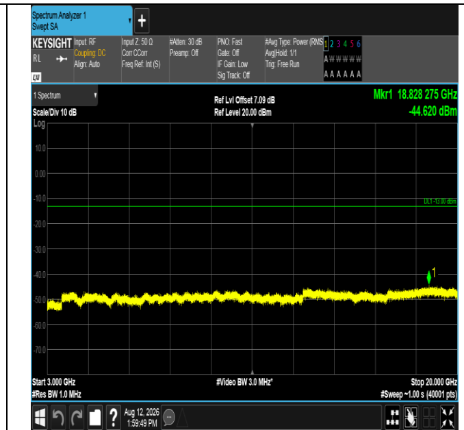
Band2-15MHz-QPSK-18675-1RB#74-3000~20000-PASS
