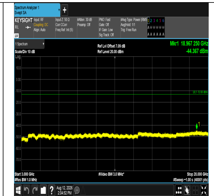
Band2-15MHz-16QAM-18900-1RB#0-3000~20000-PASS
