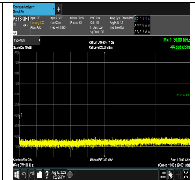
Band2-15MHz-16QAM-18675-1RB#0-30~1000-PASS
