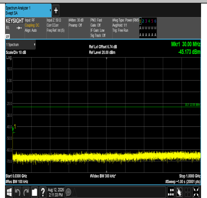
Band2-15MHz-QPSK-19125-1RB#74-30~1000-PASS
