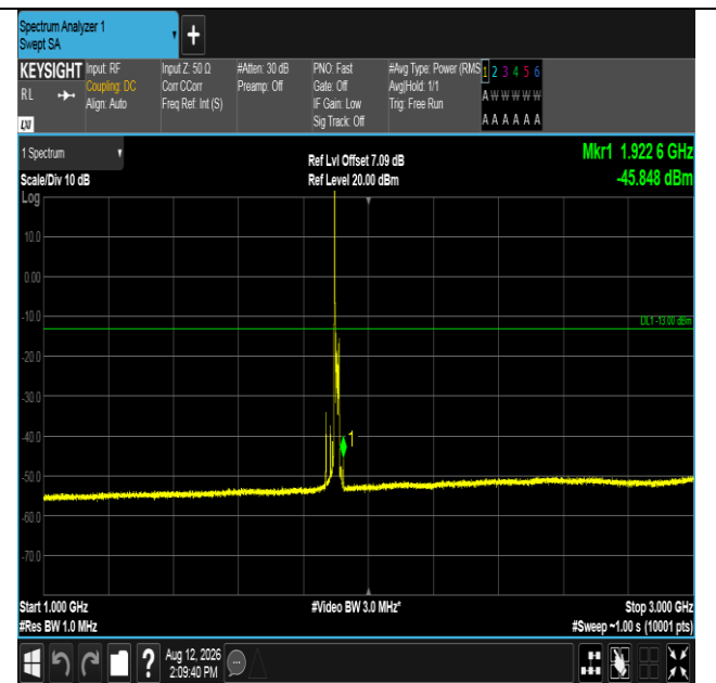
Band2-15MHz-QPSK-19125-1RB#0-1000~3000-PASS
