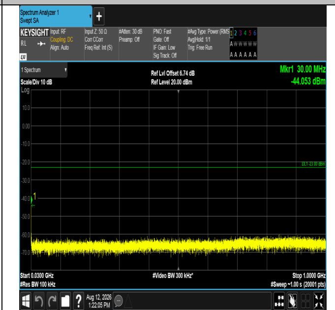
Band2-10MHz-16QAM-19150-1RB#0-30~1000-PASS
