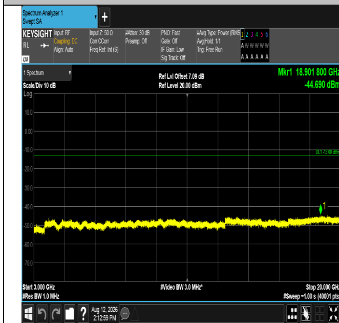
Band2-15MHz-16QAM-19125-1RB#74-3000~20000-PASS
