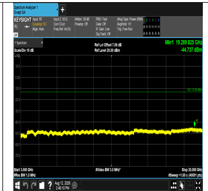
Band2-20MHz-16QAM-18700-1RB#0-3000~20000-PASS
