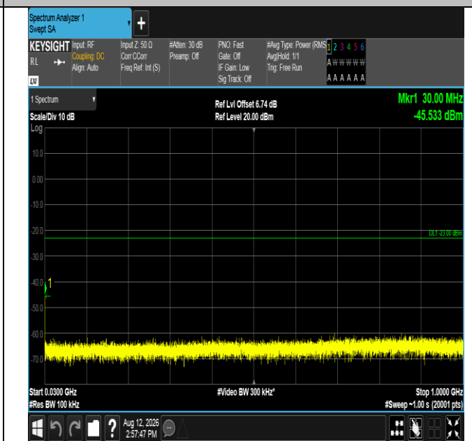
Band2-20MHz-16QAM-19100-1RB#0-30~1000-PASS
