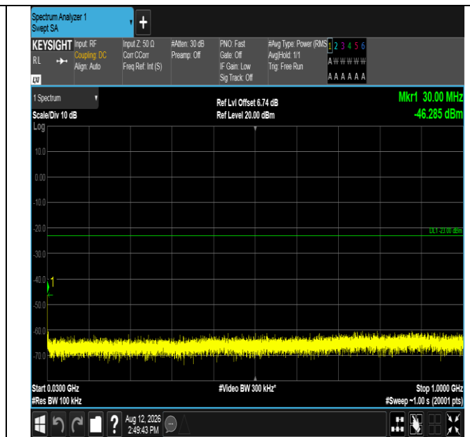
Band2-20MHz-16QAM-18700-100RB#0-30~1000-PASS
