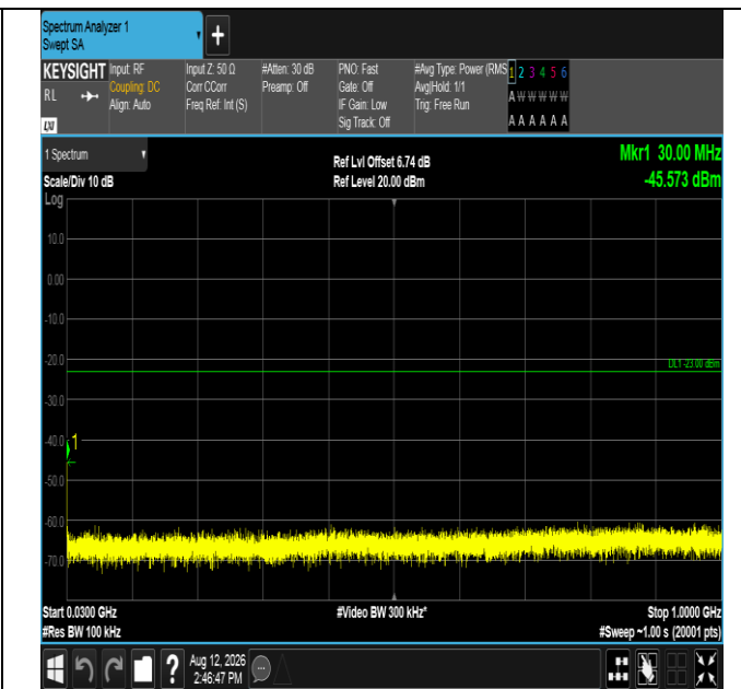
Band2-20MHz-QPSK-18700-1RB#99-30~1000-PASS
