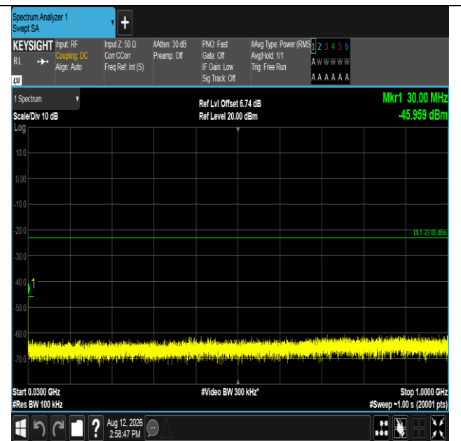
Band2-20MHz-QPSK-19100-1RB#99-30~1000-PASS
