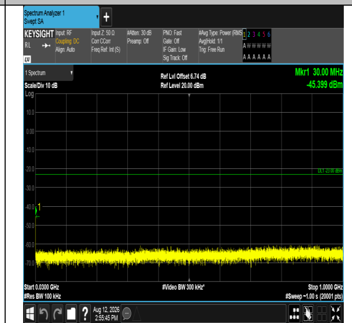
Band2-20MHz-16QAM-18900-100RB#0-30~1000-PASS
