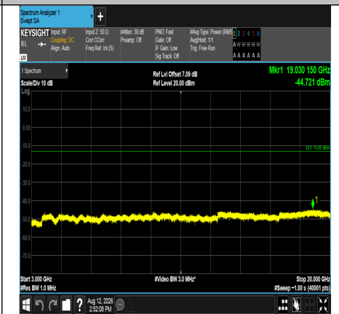
Band2-20MHz-16QAM-18900-1RB#0-3000~20000-PASS
