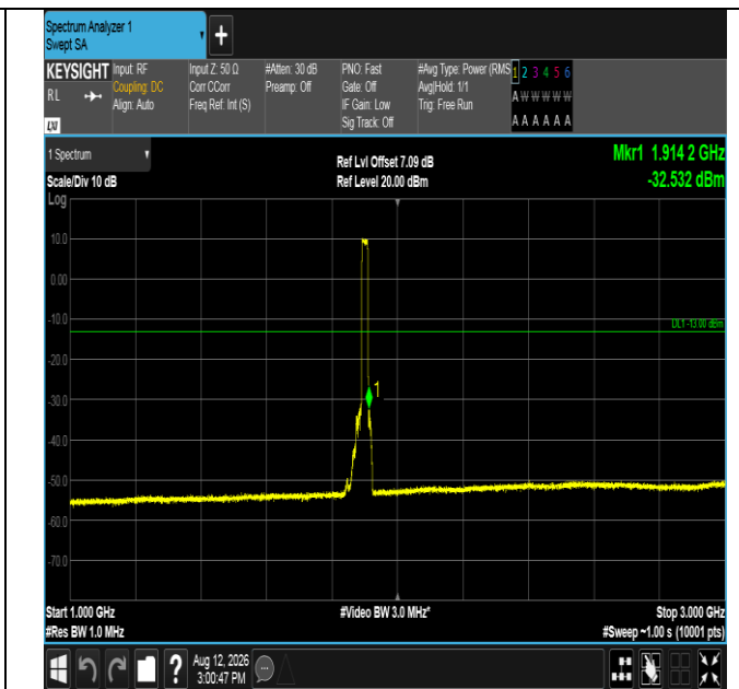
Band2-20MHz-QPSK-19100-100RB#0-1000~3000-PASS
