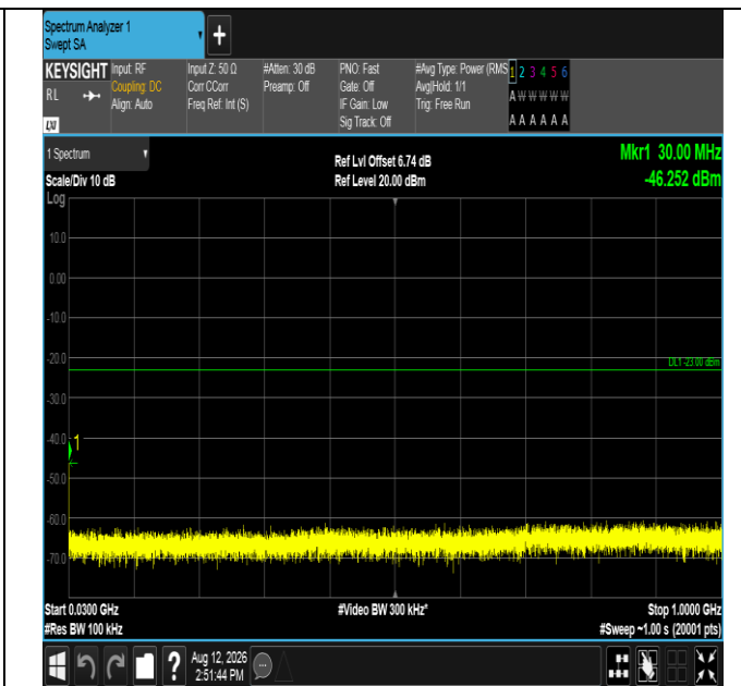
Band2-20MHz-16QAM-18900-1RB#0-30~1000-PASS
