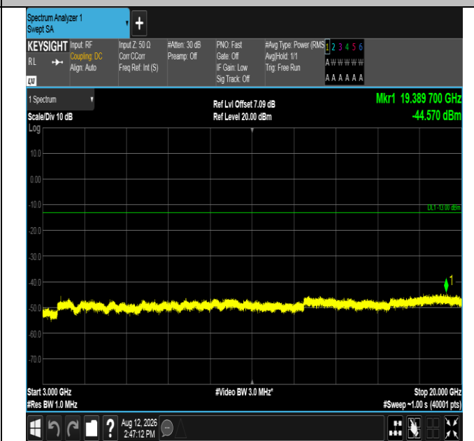
Band2-20MHz-QPSK-18700-1RB#99-3000~20000-PASS
