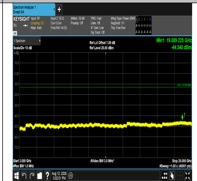
Band2-20MHz-16QAM-19100-100RB#0-3000~20000-PASS
