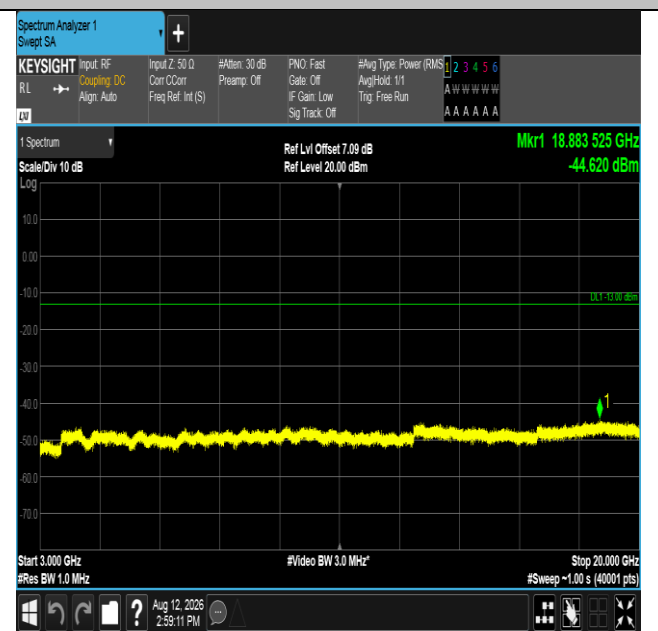
Band2-20MHz-QPSK-19100-1RB#99-3000~20000-PASS
