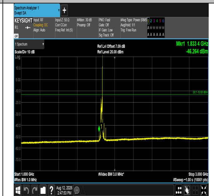
Band2-20MHz-16QAM-18700-1RB#99-1000~3000-PASS
