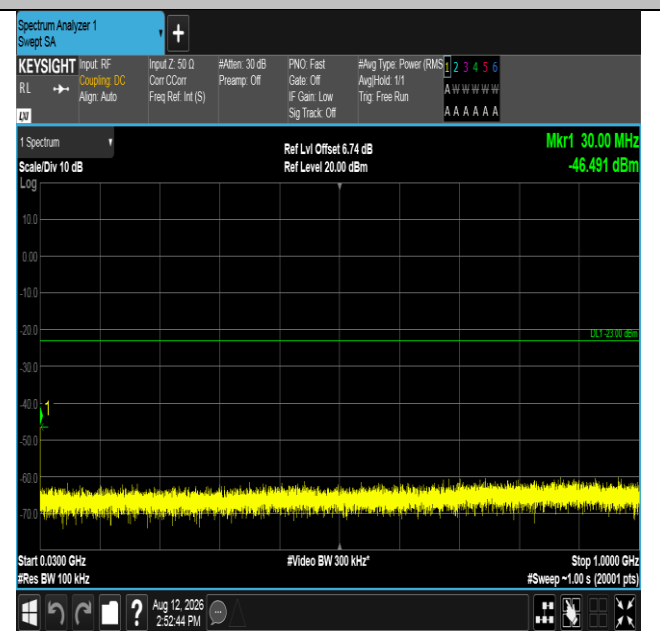
Band2-20MHz-QPSK-18900-1RB#99-30~1000-PASS
