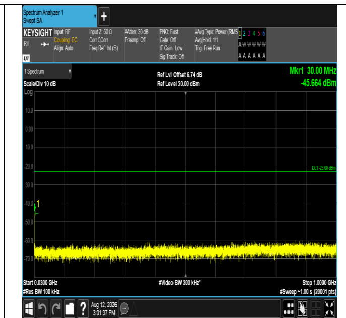
Band2-20MHz-16QAM-19100-100RB#0-30~1000-PASS
