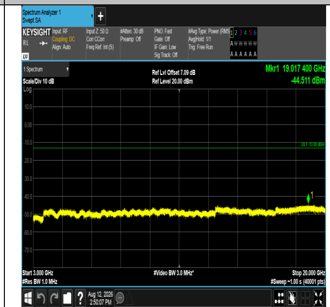
Band2-20MHz-16QAM-18700-100RB#0-3000~20000-PASS
