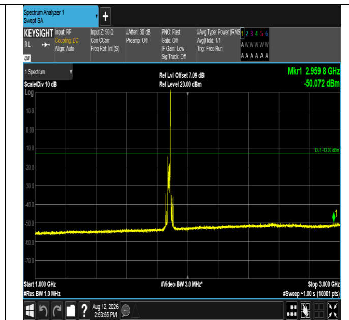
Band2-20MHz-16QAM-18900-1RB#99-1000~3000-PASS
