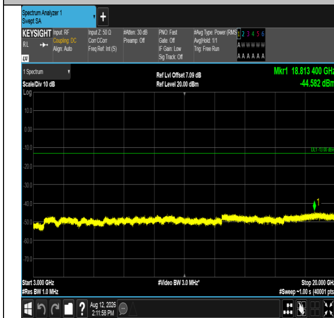
Band2-15MHz-QPSK-19125-1RB#74-3000~20000-PASS
