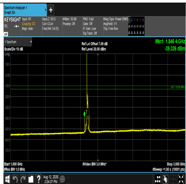
Band2-15MHz-16QAM-18900-1RB#0-1000~3000-PASS
