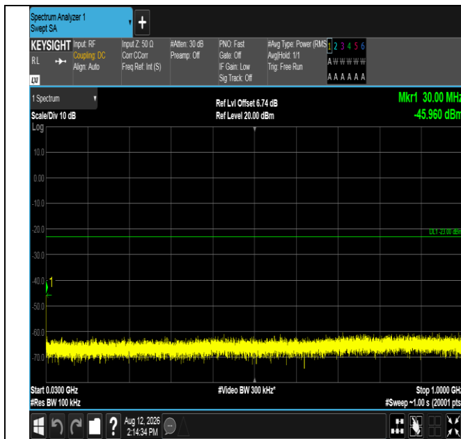
Band2-15MHz-16QAM-19125-75RB#0-30~1000-PASS
