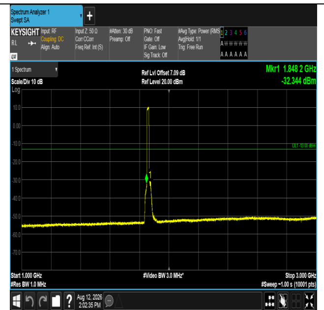
Band2-15MHz-16QAM-18675-75RB#0-1000~3000-PASS
