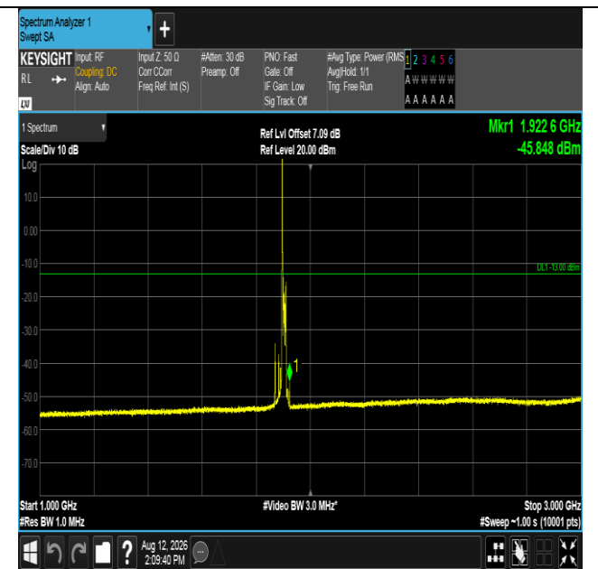
Band2-15MHz-QPSK-19125-1RB#0-1000~3000-PASS
