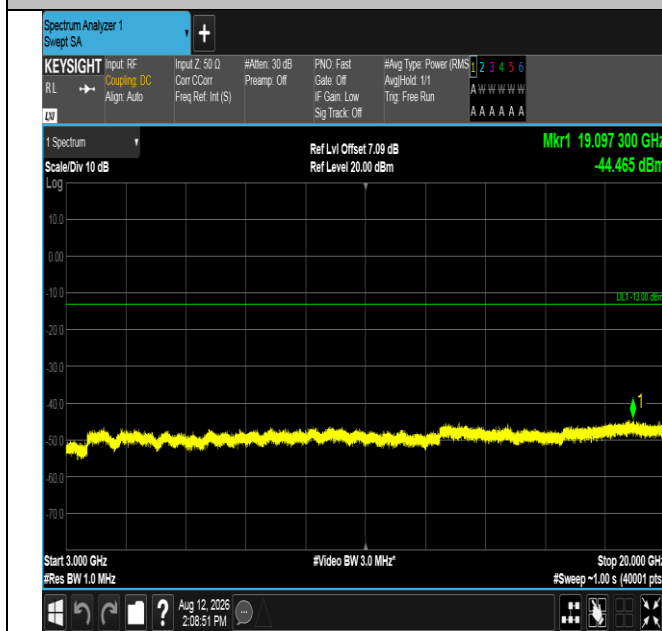
Band2-15MHz-16QAM-18900-75RB#0-3000~20000-PASS
