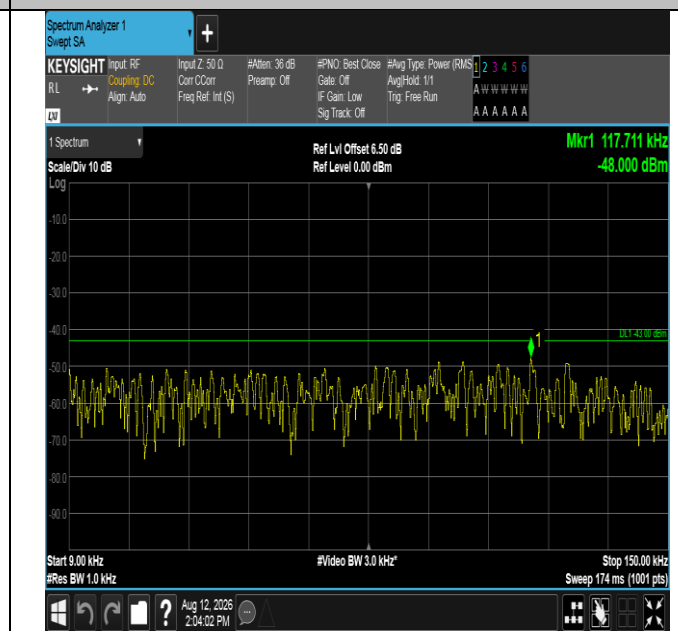
Band2-15MHz-16QAM-18900-1RB#0-0.009~0.15-PASS
