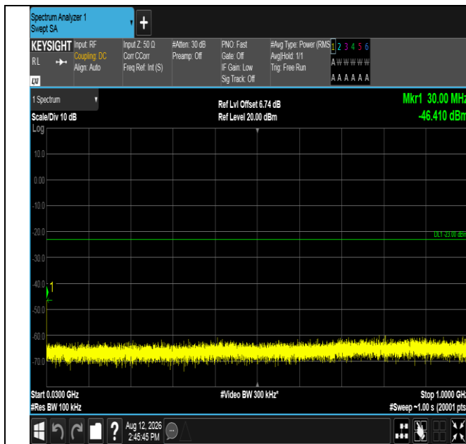
Band2-20MHz-16QAM-18700-1RB#0-30~1000-PASS
