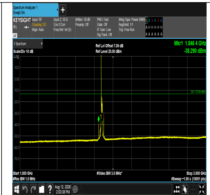
Band2-15MHz-QPSK-18900-1RB#0-1000~3000-PASS
