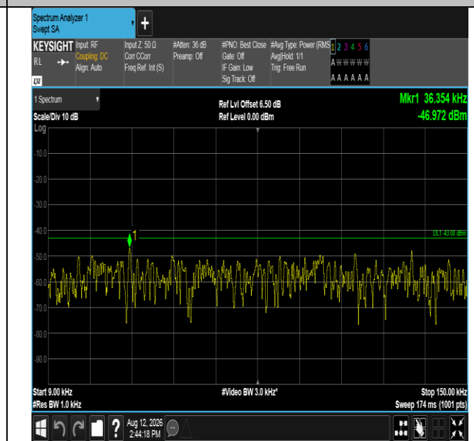
Band2-20MHz-QPSK-18700-1RB#0-0.009~0.15-PASS
