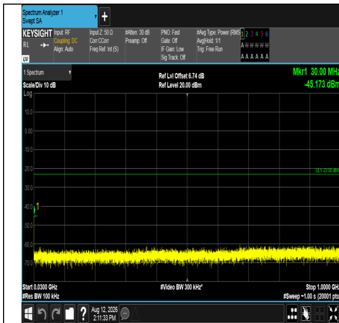
Band2-15MHz-QPSK-19125-1RB#74-30~1000-PASS
