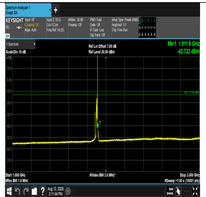
Band2-15MHz-QPSK-19125-1RB#74-1000~3000-PASS
