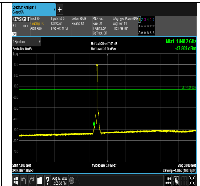
Band2-15MHz-16QAM-18900-75RB#0-1000~3000-PASS
