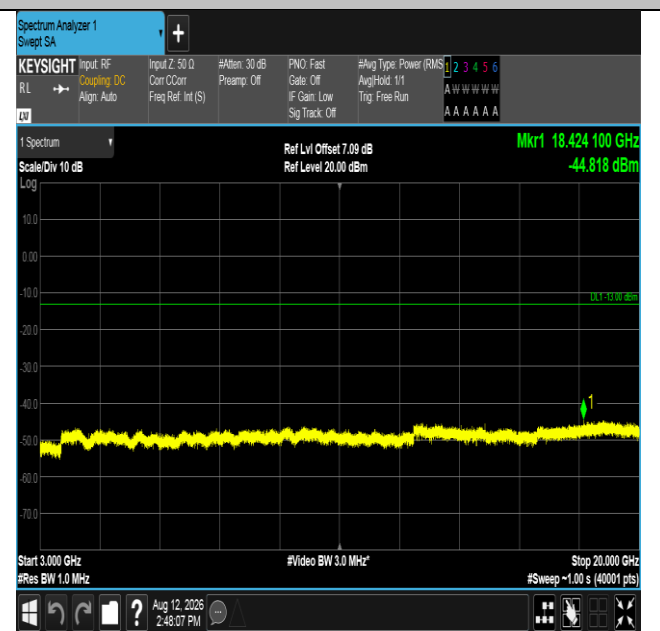
Band2-20MHz-16QAM-18700-1RB#99-3000~20000-PASS
