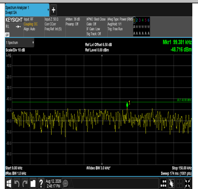
Band2-20MHz-QPSK-18700-100RB#0-0.009~0.15-PASS
