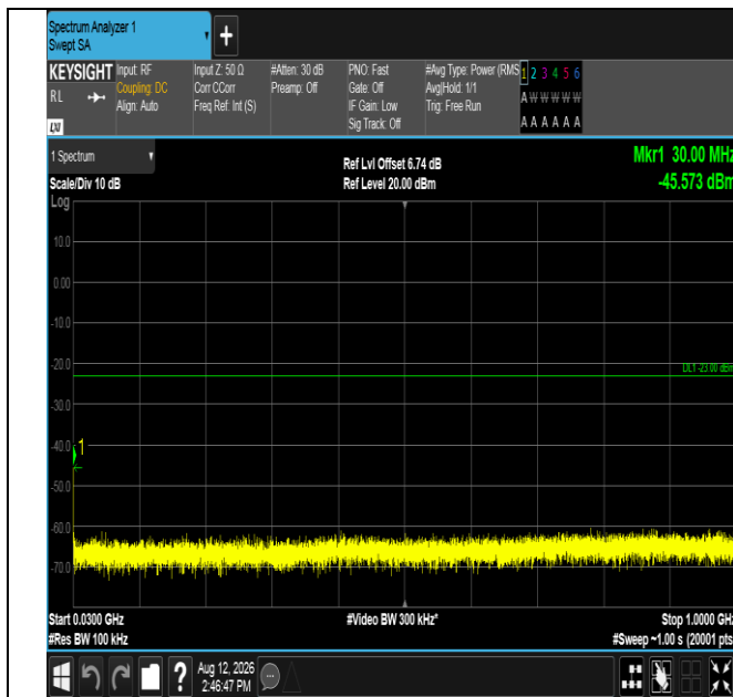
Band2-20MHz-QPSK-18700-1RB#99-30~1000-PASS
