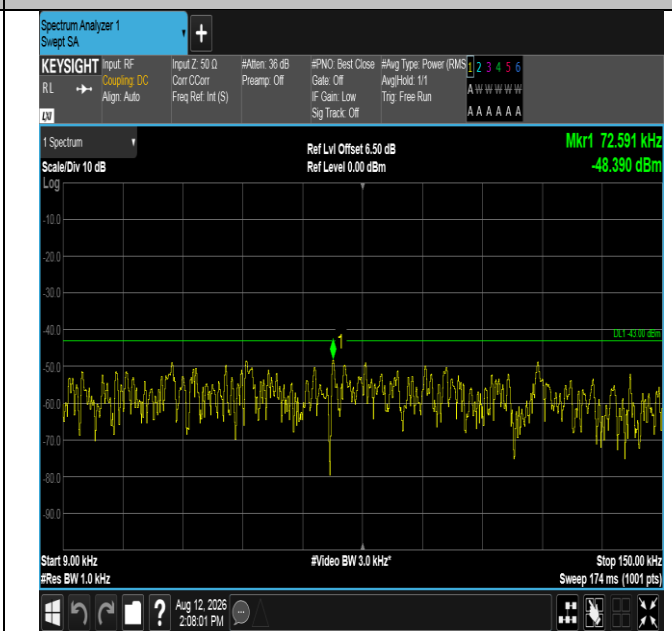
Band2-15MHz-16QAM-18900-75RB#0-0.009~0.15-PASS
