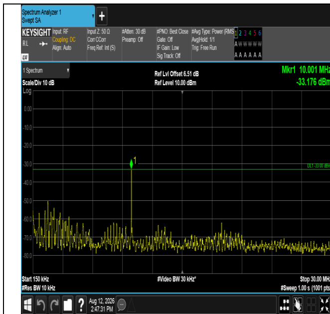
Band2-20MHz-16QAM-18700-1RB#99-0.15~30-PASS
