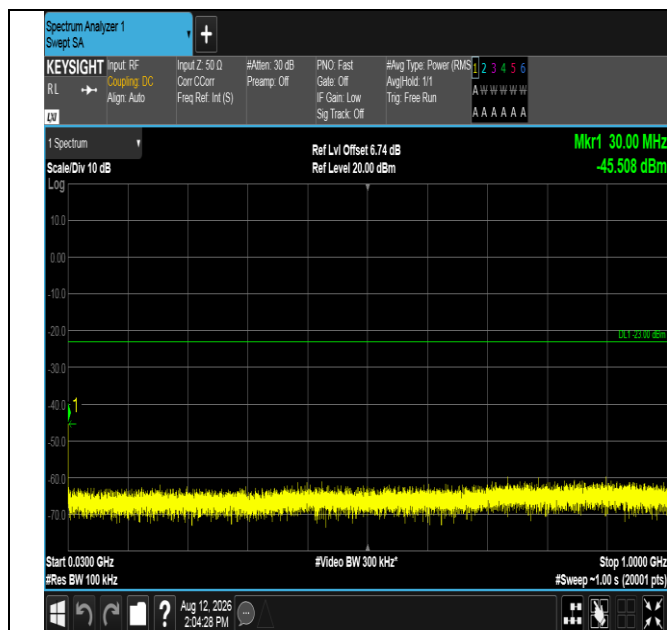
Band2-15MHz-16QAM-18900-1RB#0-30~1000-PASS
