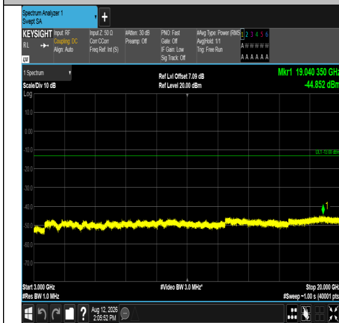
Band2-15MHz-QPSK-18900-1RB#74-3000~20000-PASS
