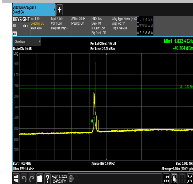
Band2-20MHz-16QAM-18700-1RB#99-1000~3000-PASS
