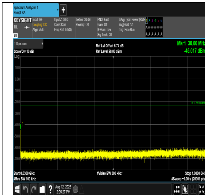
Band2-15MHz-QPSK-18900-1RB#74-30~1000-PASS
