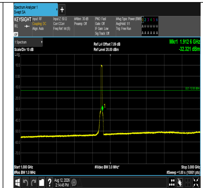
Band2-15MHz-16QAM-19125-75RB#0-1000~3000-PASS
