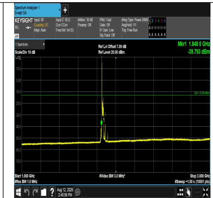
Band2-20MHz-16QAM-18700-1RB#0-1000~3000-PASS
