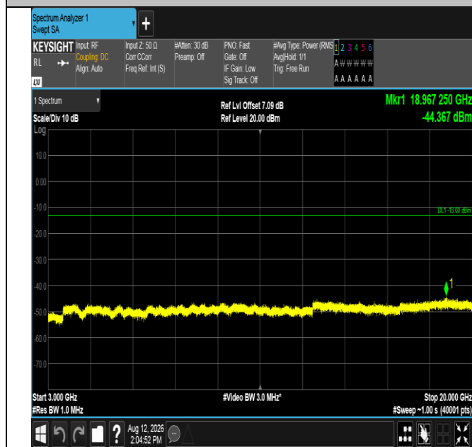
Band2-15MHz-16QAM-18900-1RB#0-3000~20000-PASS
