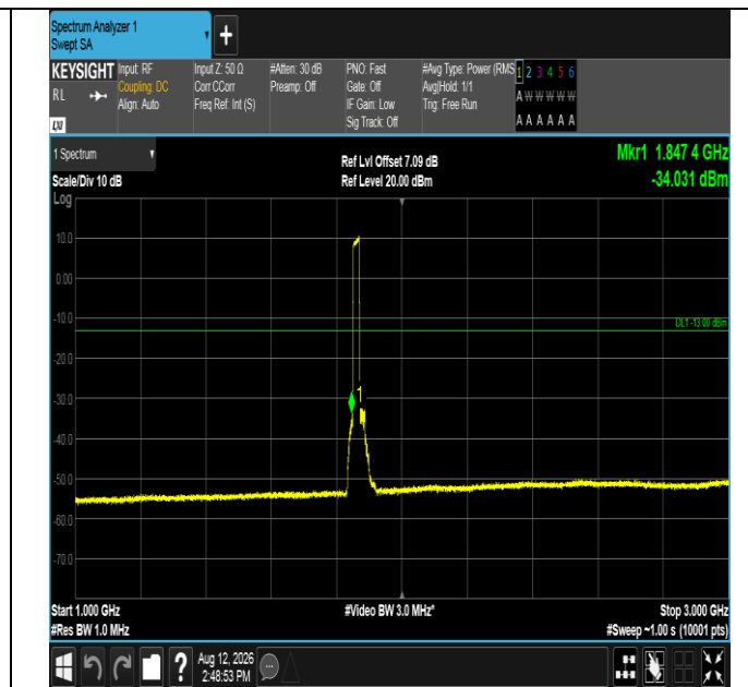
Band2-20MHz-QPSK-18700-100RB#0-1000~3000-PASS
