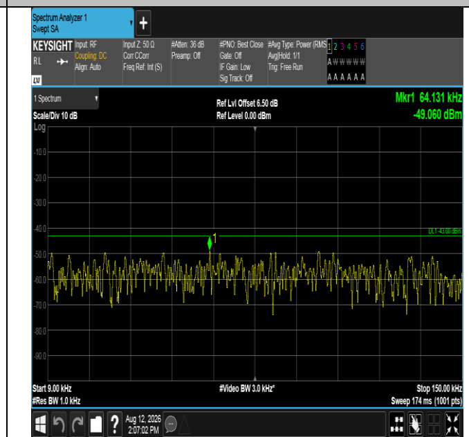
Band2-15MHz-QPSK-18900-75RB#0-0.009~0.15-PASS
