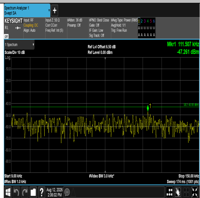
Band2-15MHz-16QAM-18900-1RB#74-0.009~0.15-PASS
