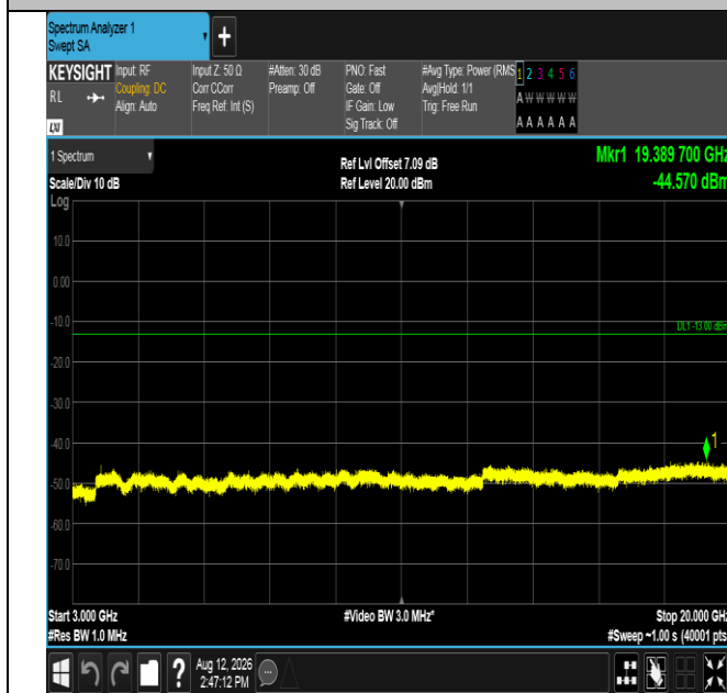
Band2-20MHz-QPSK-18700-1RB#99-3000~20000-PASS
