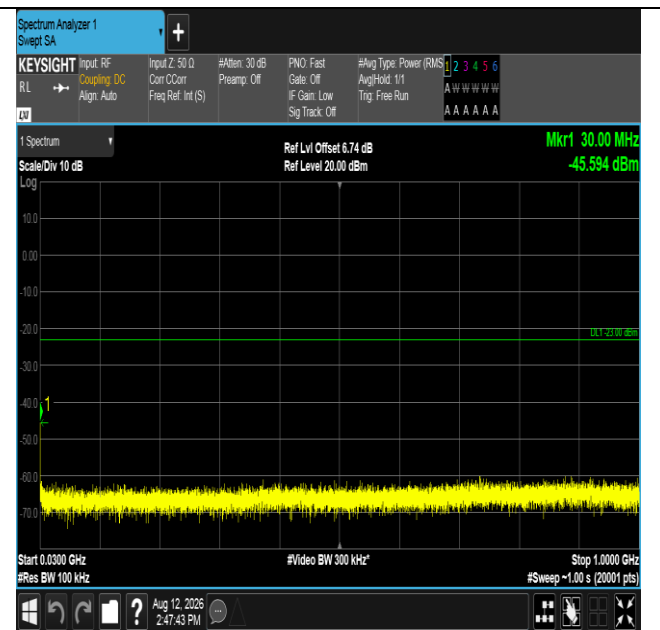
Band2-20MHz-16QAM-18700-1RB#99-30~1000-PASS
