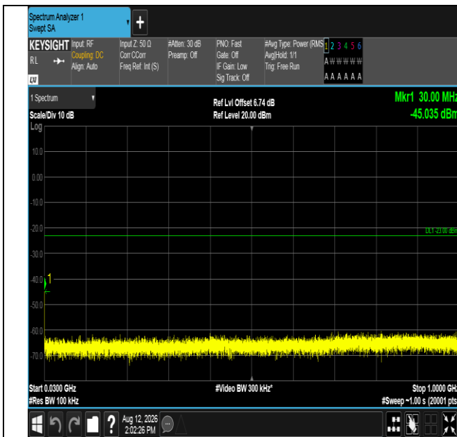
Band2-15MHz-16QAM-18675-75RB#0-30~1000-PASS
