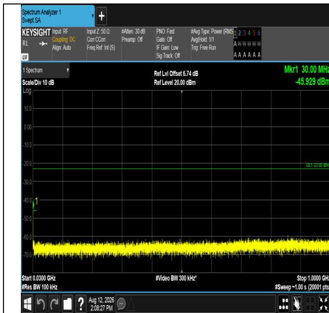
Band2-15MHz-16QAM-18900-75RB#0-30~1000-PASS
