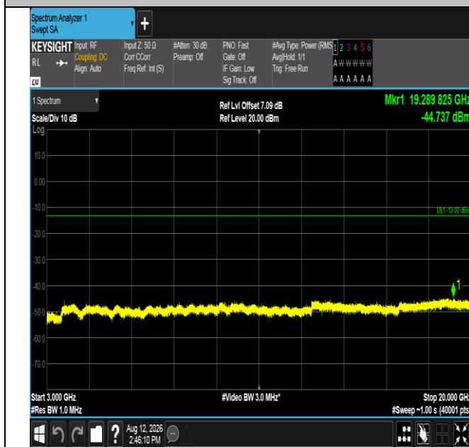
Band2-20MHz-16QAM-18700-1RB#0-3000~20000-PASS
