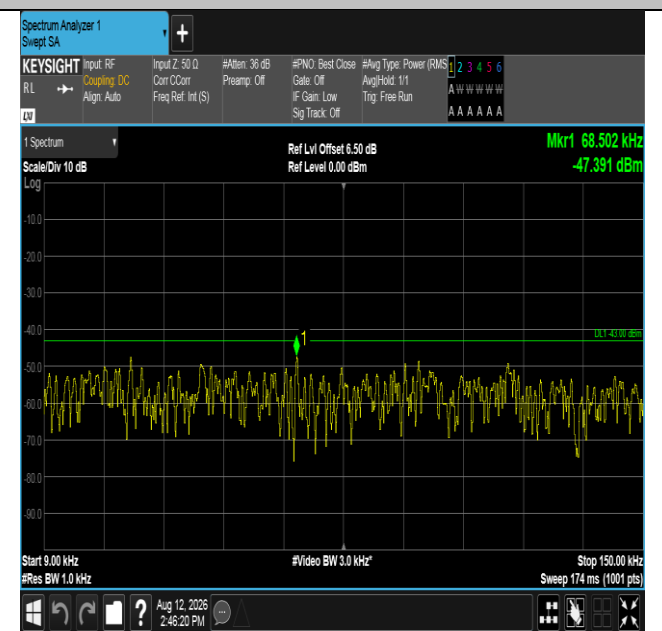
Band2-20MHz-QPSK-18700-1RB#99-0.009~0.15-PASS
