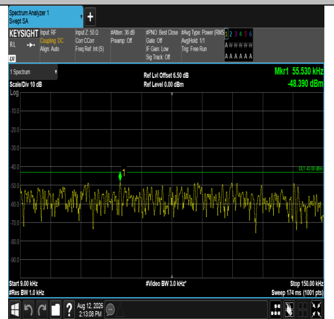
Band2-15MHz-QPSK-19125-75RB#0-0.009~0.15-PASS
