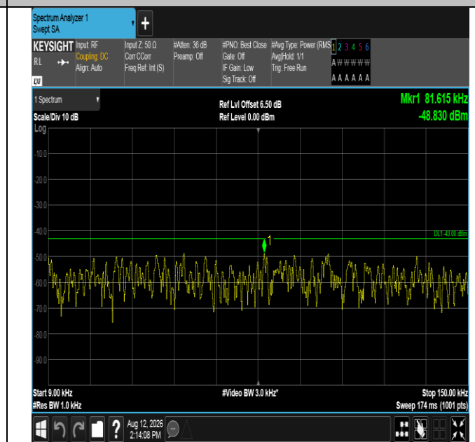
Band2-15MHz-16QAM-19125-75RB#0-0.009~0.15-PASS
