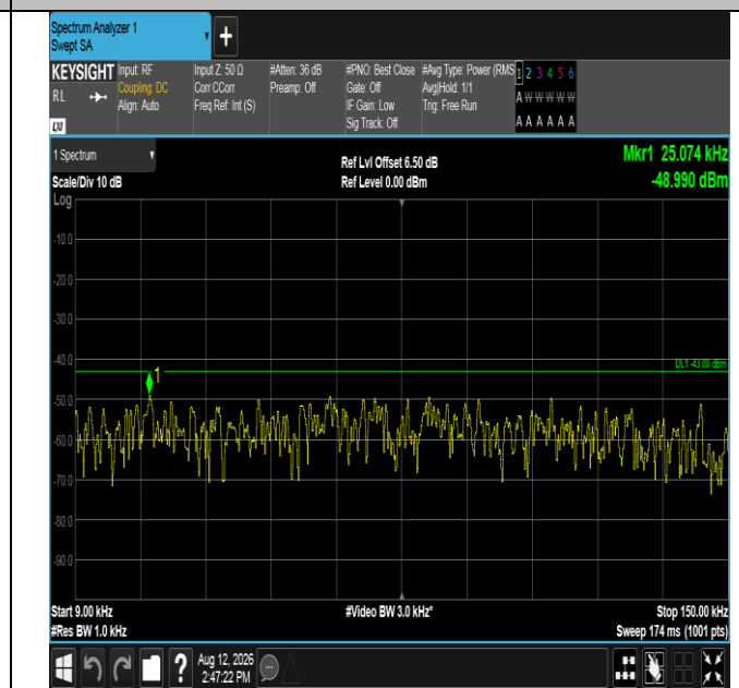
Band2-20MHz-16QAM-18700-1RB#99-0.009~0.15-PASS
