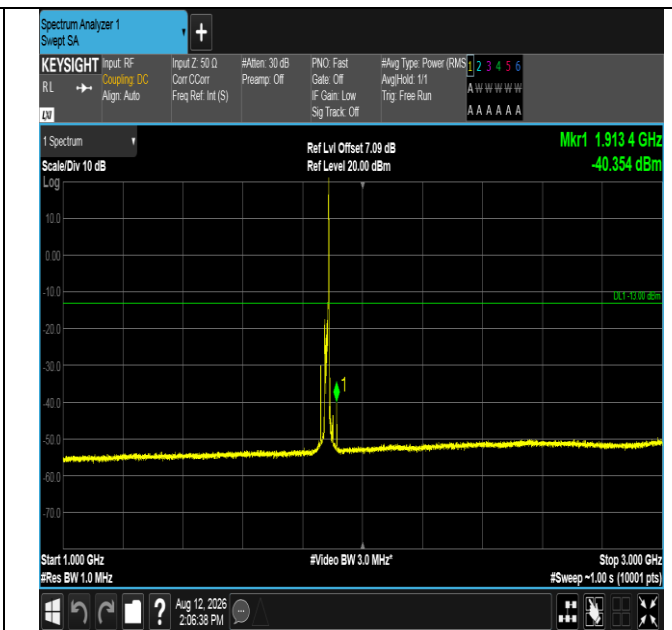
Band2-15MHz-16QAM-18900-1RB#74-1000~3000-PASS
