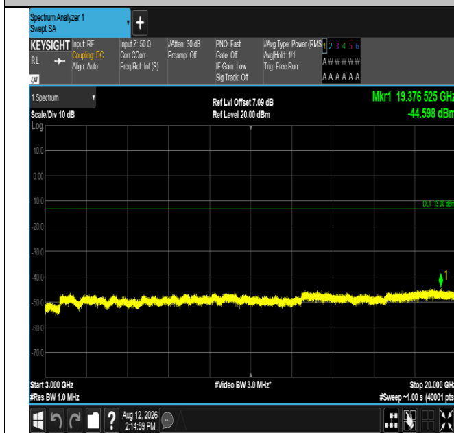
Band2-15MHz-16QAM-19125-75RB#0-3000~20000-PASS
