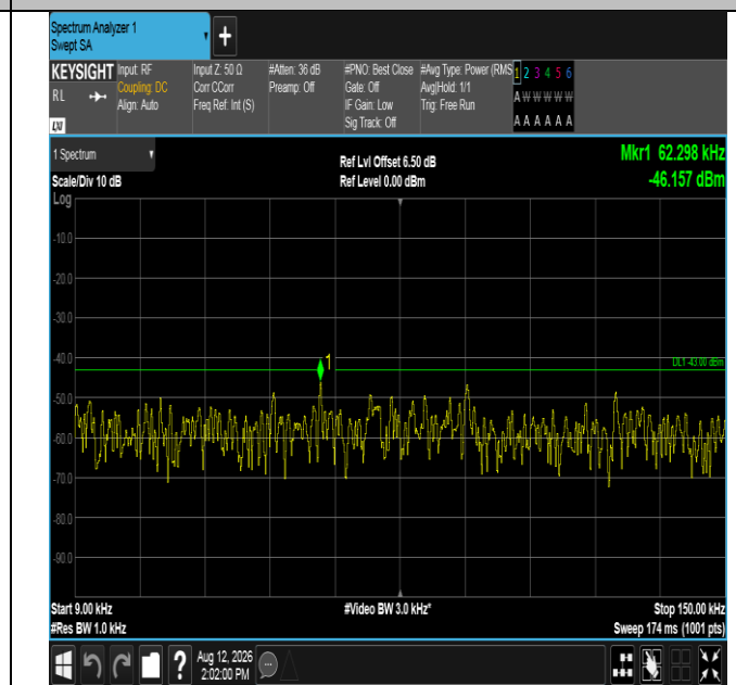
Band2-15MHz-16QAM-18675-75RB#0-0.009~0.15-PASS
