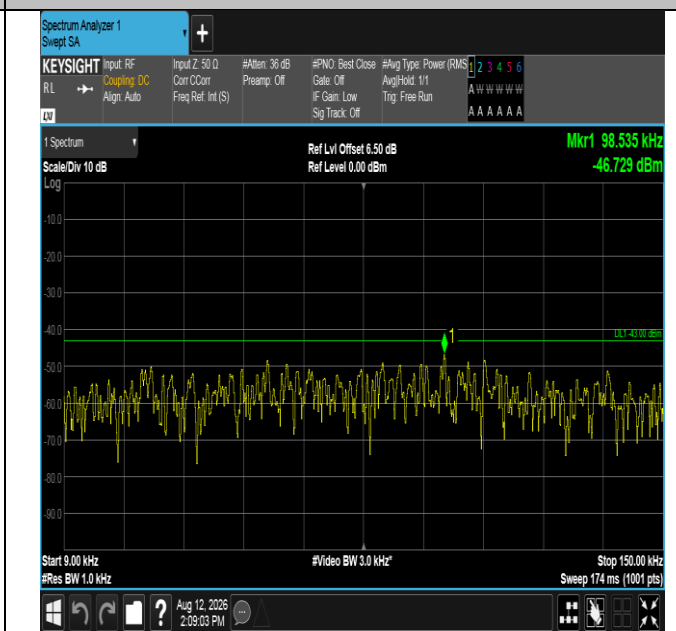
Band2-15MHz-QPSK-19125-1RB#0-0.009~0.15-PASS
