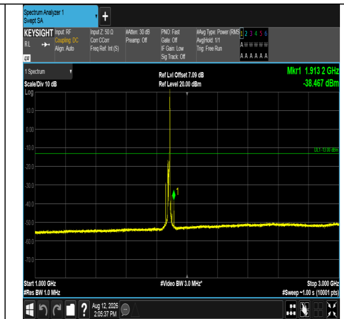
Band2-15MHz-QPSK-18900-1RB#74-1000~3000-PASS
