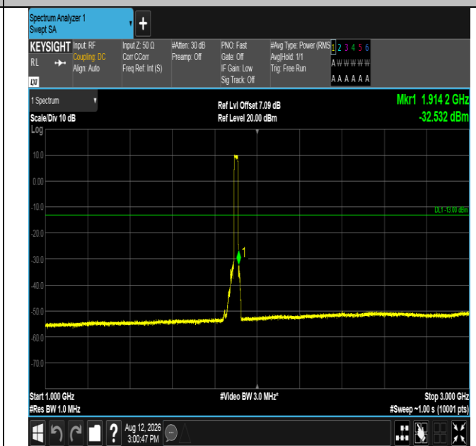
Band2-20MHz-QPSK-19100-100RB#0-1000~3000-PASS
