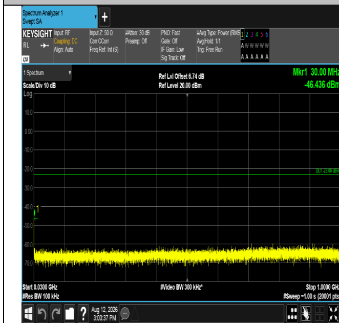
Band2-20MHz-QPSK-19100-100RB#0-30~1000-PASS
