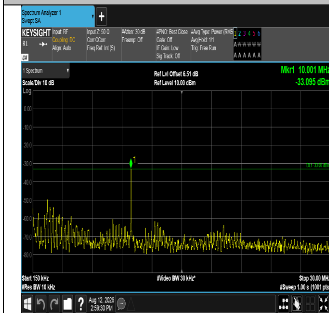
Band2-20MHz-16QAM-19100-1RB#99-0.15~30-PASS
