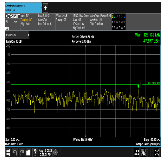
Band2-20MHz-16QAM-19100-1RB#99-0.009~0.15-PASS
