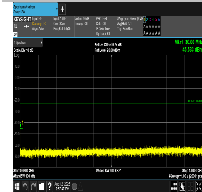
Band2-20MHz-16QAM-19100-1RB#0-30~1000-PASS
