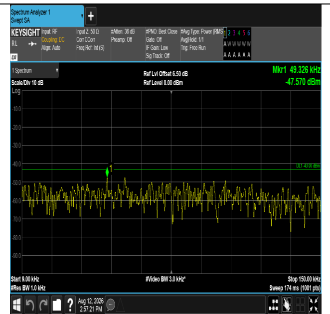
Band2-20MHz-16QAM-19100-1RB#0-0.009~0.15-PASS
