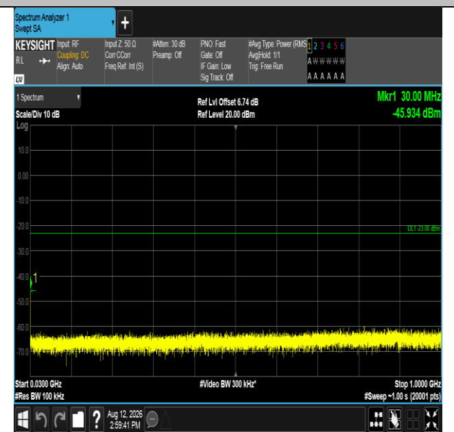
Band2-20MHz-16QAM-19100-1RB#99-30~1000-PASS
