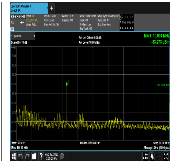
Band2-20MHz-QPSK-19100-100RB#0-0.15~30-PASS
