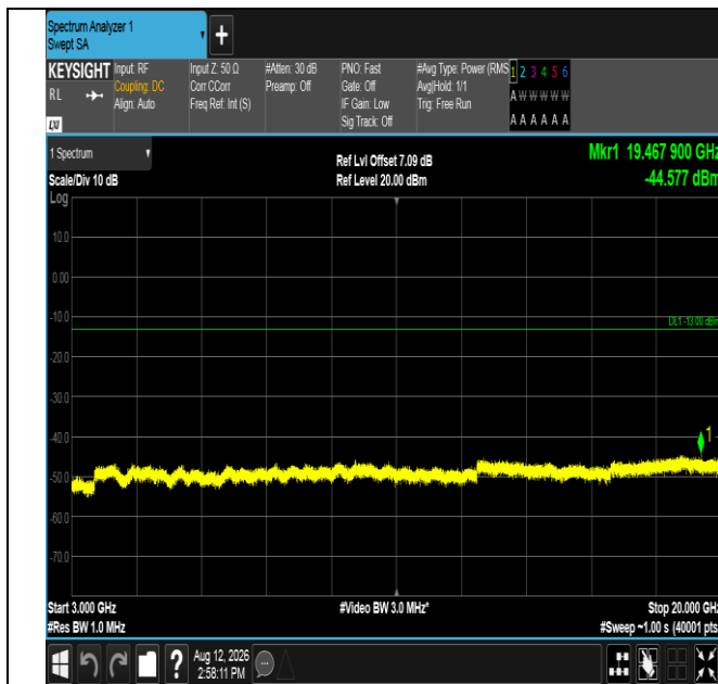
Band2-20MHz-16QAM-19100-1RB#0-3000~20000-PASS
