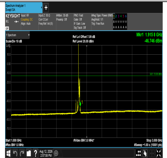
Band2-20MHz-16QAM-19100-1RB#0-1000~3000-PASS
