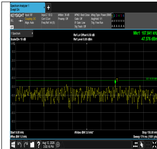
Band2-20MHz-QPSK-19100-100RB#0-0.009~0.15-PASS
