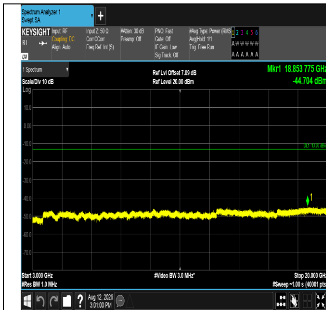
Band2-20MHz-QPSK-19100-100RB#0-3000~20000-PASS
