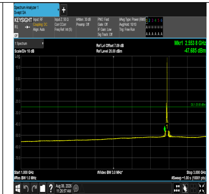
Band38-10MHz-QPSK-37800-1RB#49-1000~3000-PASS
