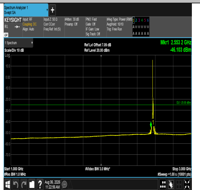
Band38-10MHz-QPSK-37800-1RB#0-1000~3000-PASS
