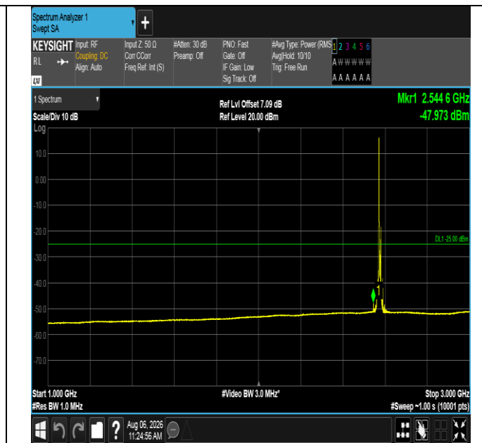
Band38-10MHz-16QAM-37800-1RB#0-1000~3000-PASS
