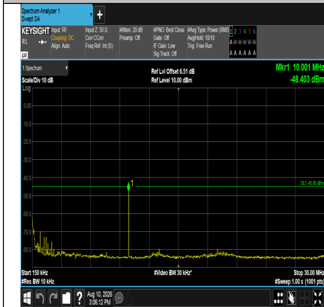
Band38-10MHz-QPSK-38000-50RB#0-0.15~30-PASS
