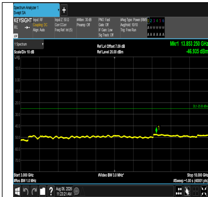
Band38-10MHz-QPSK-37800-1RB#0-3000~18000-PASS
