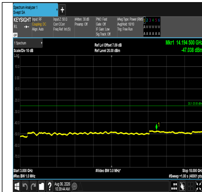
Band38-5MHz-16QAM-38225-1RB#24-3000~18000-PASS
