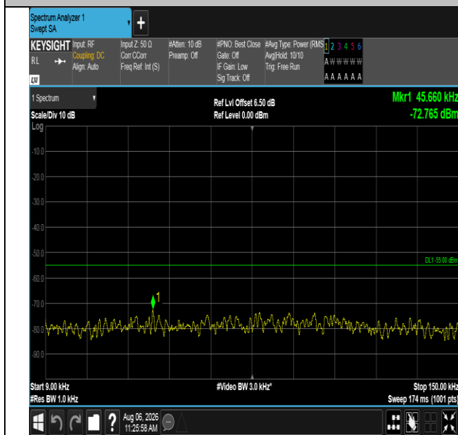
Band38-10MHz-QPSK-37800-1RB#49-0.009~0.15-PASS
