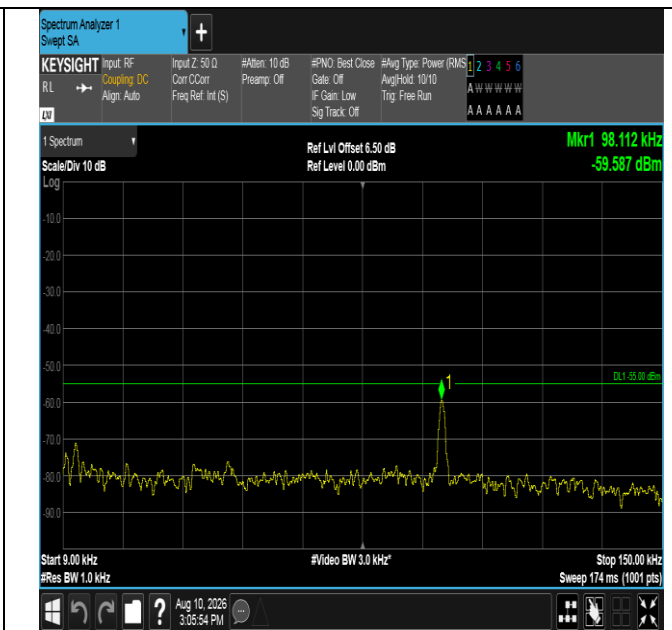
Band38-10MHz-QPSK-38000-50RB#0-0.009~0.15-PASS
