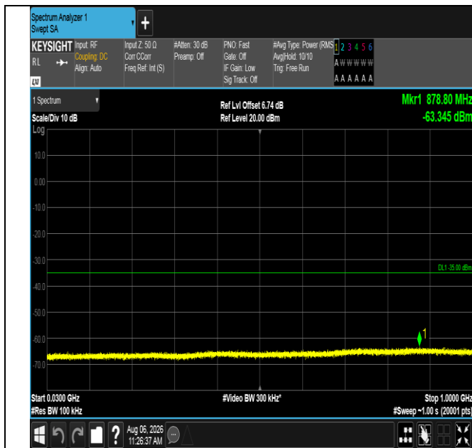
Band38-10MHz-QPSK-37800-1RB#49-30~1000-PASS
