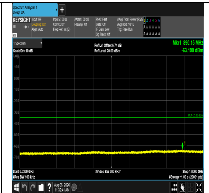
Band38-10MHz-16QAM-38000-1RB#0-30~1000-PASS
