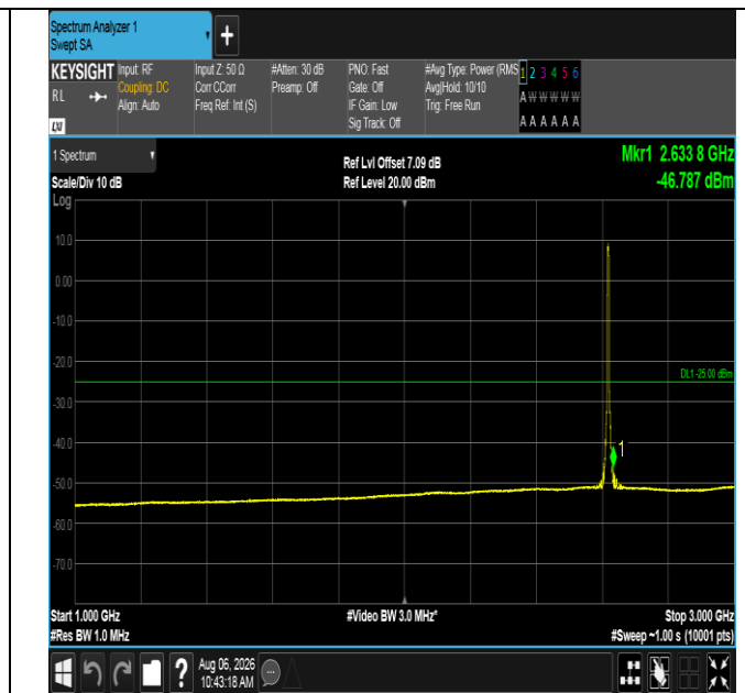
Band38-5MHz-16QAM-38225-25RB#0-1000~3000-PASS
