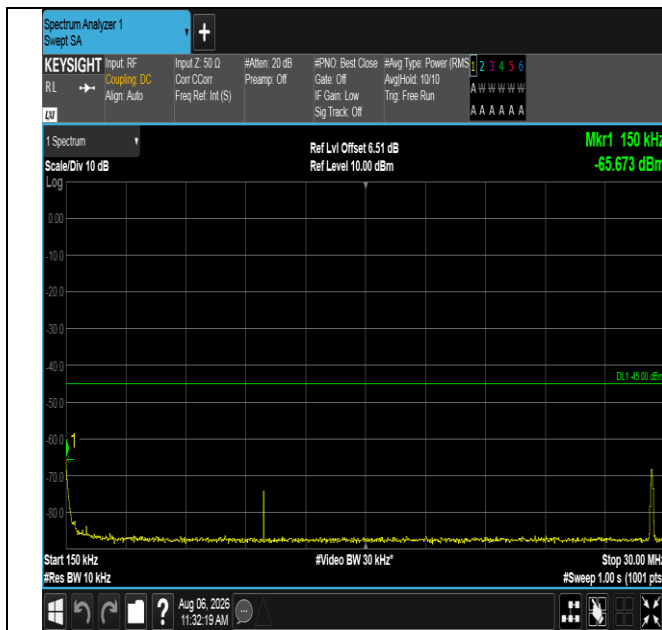
Band38-10MHz-16QAM-38000-1RB#0-0.15~30-PASS
