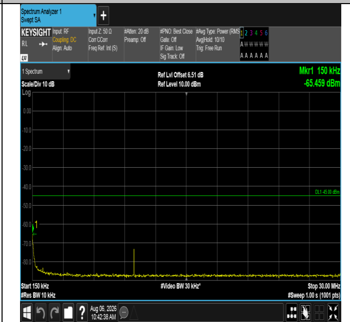
Band38-5MHz-16QAM-38225-25RB#0-0.15~30-PASS
