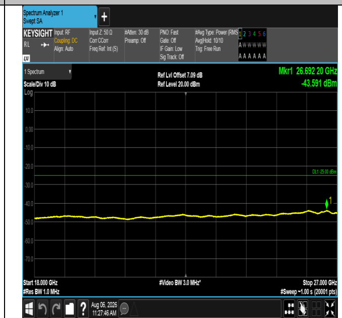
Band38-10MHz-QPSK-37800-1RB#49-18000~27000-PASS
