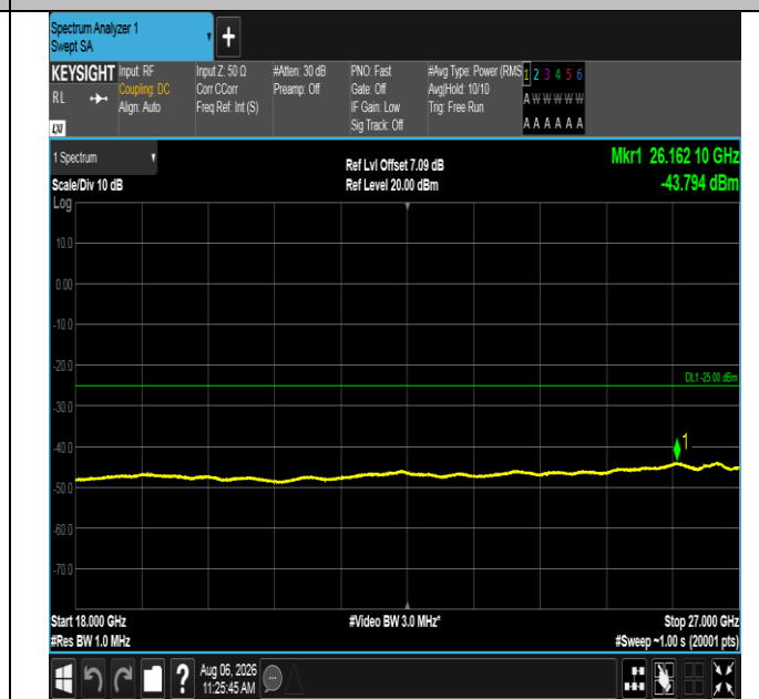
Band38-10MHz-16QAM-37800-1RB#0-18000~27000-PASS
