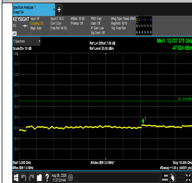
Band38-10MHz-QPSK-37800-1RB#49-3000~18000-PASS
