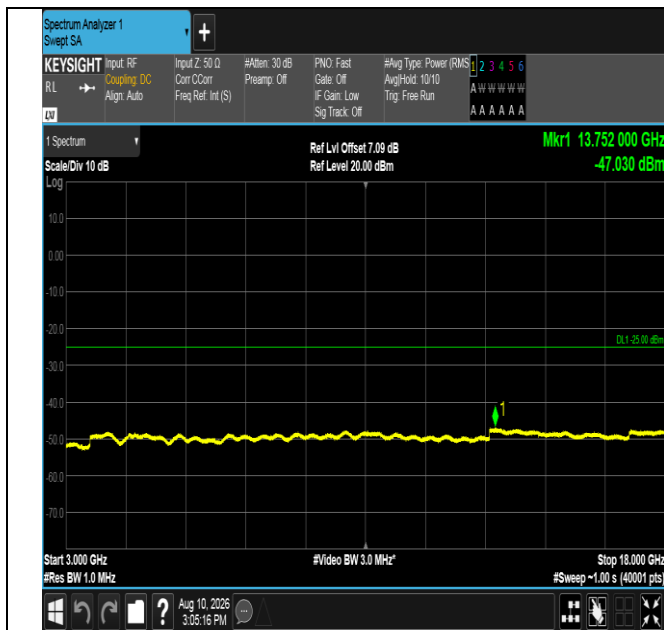
Band38-10MHz-QPSK-37800-50RB#0-3000~18000-PASS
