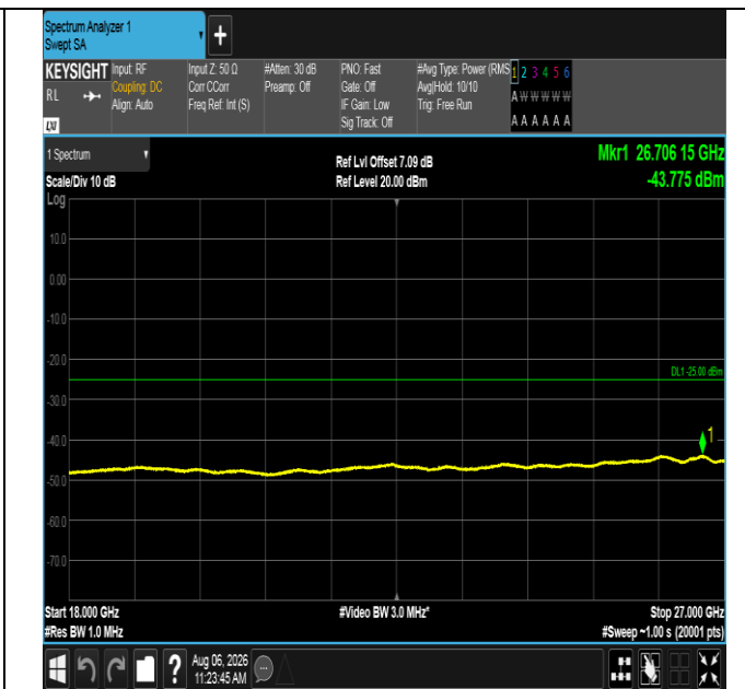
Band38-10MHz-QPSK-37800-1RB#0-18000~27000-PASS
