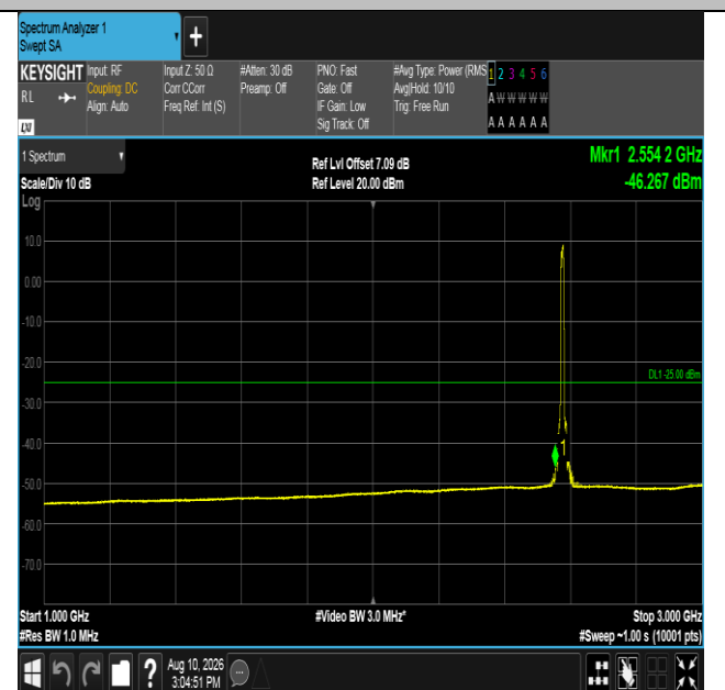
Band38-10MHz-QPSK-37800-50RB#0-1000~3000-PASS
