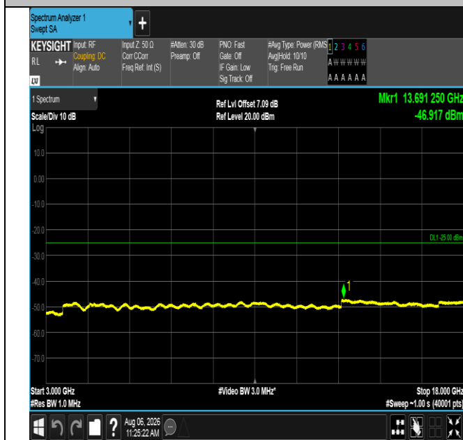
Band38-10MHz-16QAM-37800-1RB#0-3000~18000-PASS
