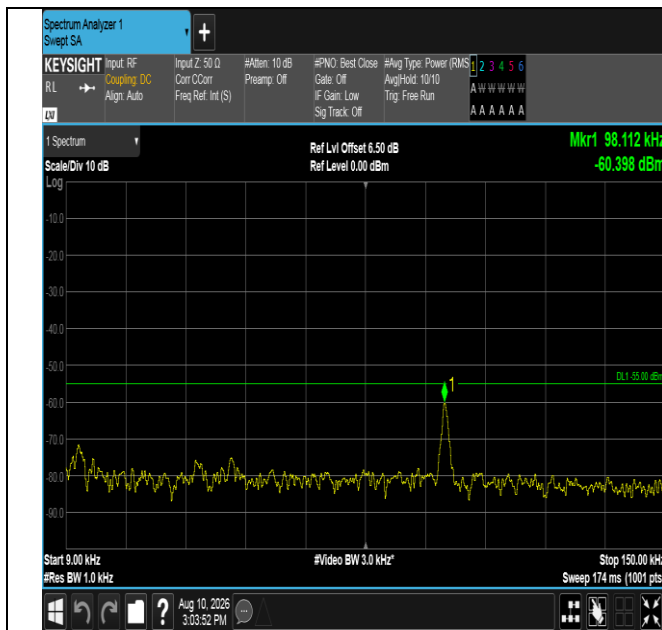
Band38-10MHz-QPSK-37800-50RB#0-0.009~0.15-PASS
