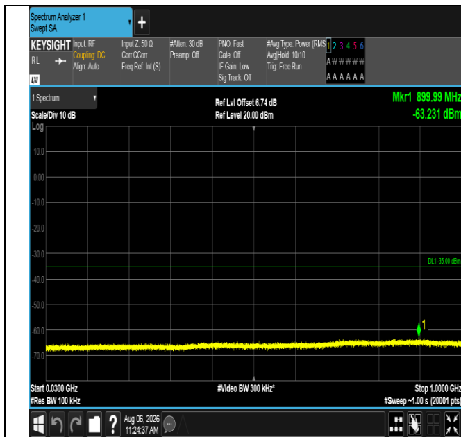
Band38-10MHz-16QAM-37800-1RB#0-30~1000-PASS
