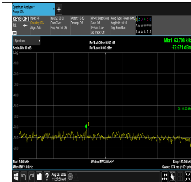
Band38-10MHz-16QAM-37800-1RB#49-0.009~0.15-PASS
