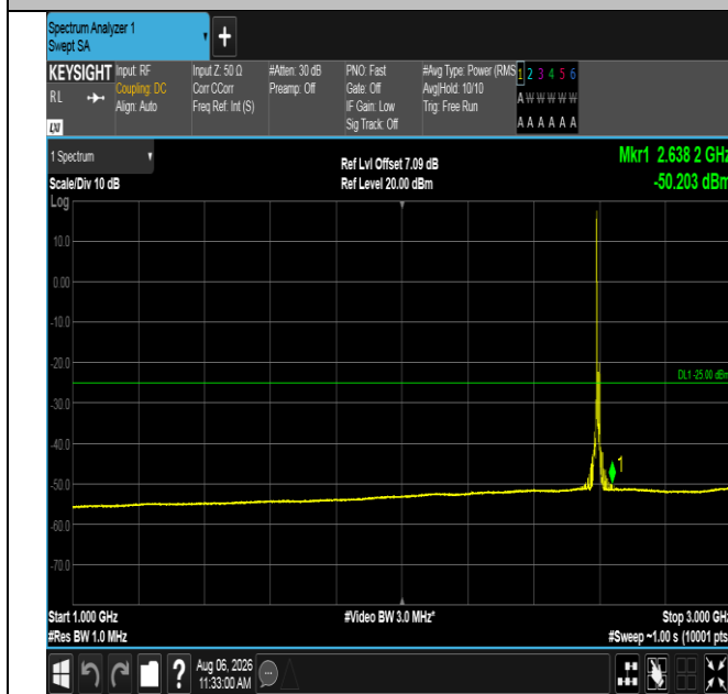
Band38-10MHz-16QAM-38000-1RB#0-1000~3000-PASS
