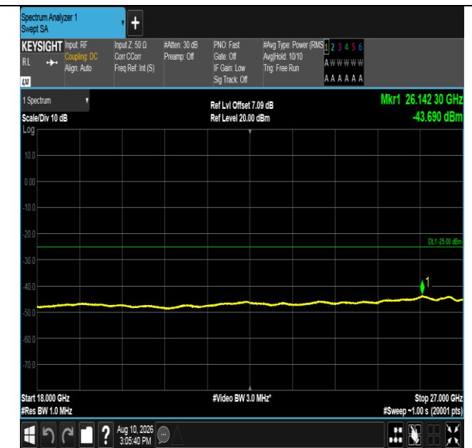
Band38-10MHz-QPSK-37800-50RB#0-18000~27000-PASS
