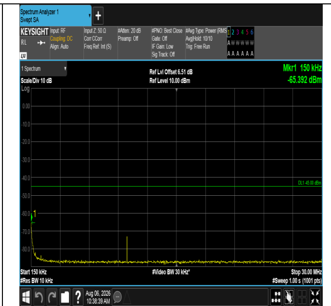
Band38-5MHz-16QAM-38225-1RB#24-0.15~30-PASS
