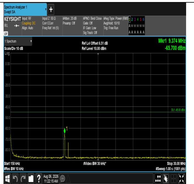
Band38-10MHz-QPSK-37800-1RB#0-0.15~30-PASS
