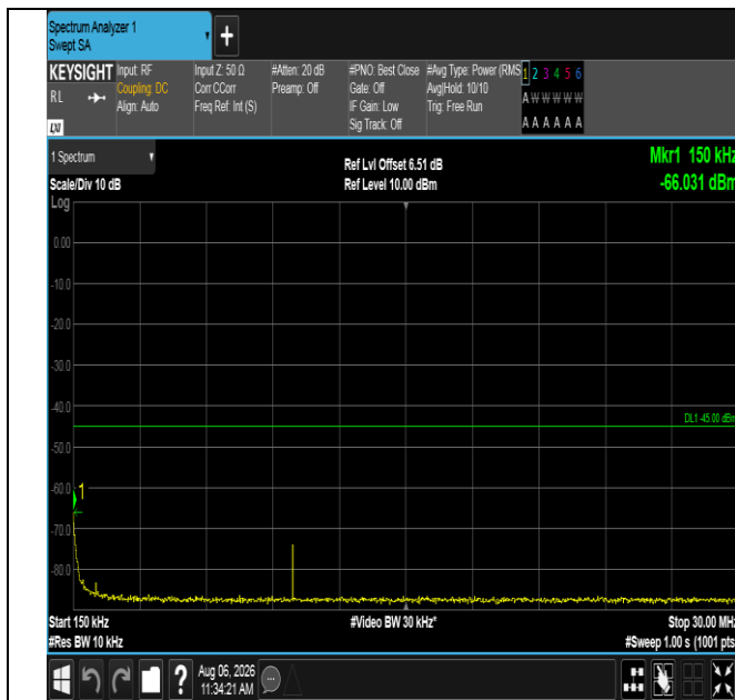
Band38-10MHz-QPSK-38000-1RB#49-0.15~30-PASS
