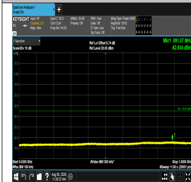
Band38-10MHz-16QAM-37800-1RB#49-30~1000-PASS
