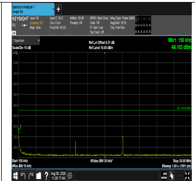
Band38-10MHz-16QAM-37800-1RB#49-0.15~30-PASS
