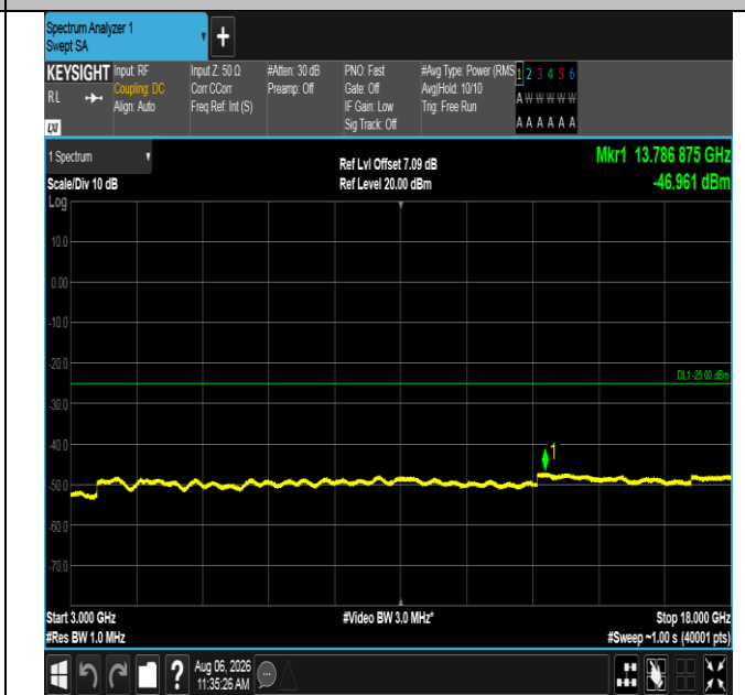
Band38-10MHz-QPSK-38000-1RB#49-3000~18000-PASS
