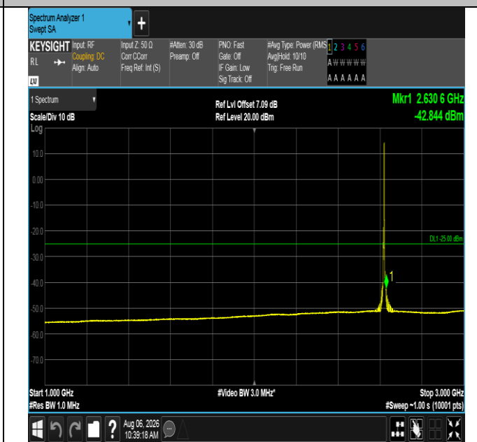
Band38-5MHz-16QAM-38225-1RB#24-1000~3000-PASS
