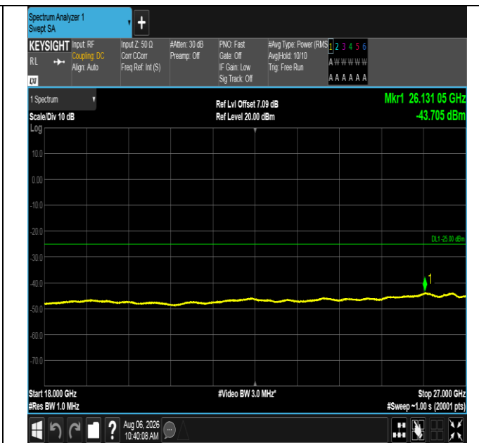
Band38-5MHz-16QAM-38225-1RB#24-18000~27000-PASS
