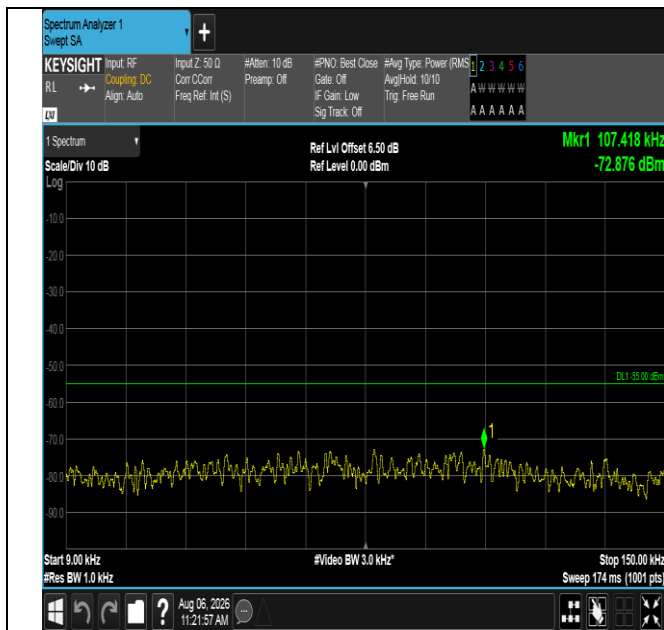
Band38-10MHz-QPSK-37800-1RB#0-0.009~0.15-PASS
