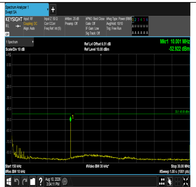
Band38-10MHz-QPSK-37800-50RB#0-0.15~30-PASS
