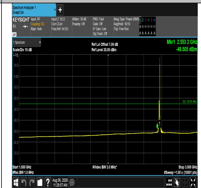
Band38-10MHz-16QAM-37800-1RB#49-1000~3000-PASS
