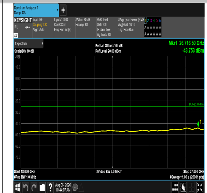
Band38-5MHz-16QAM-38225-25RB#0-18000~27000-PASS
