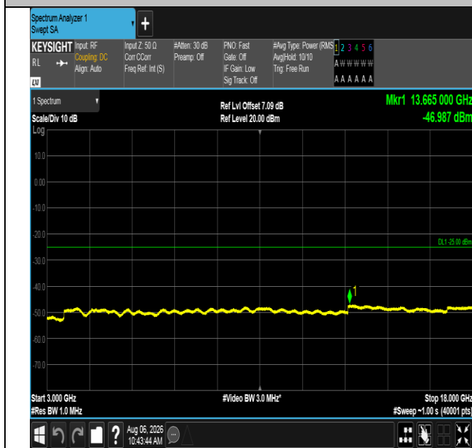
Band38-5MHz-16QAM-38225-25RB#0-3000~18000-PASS
