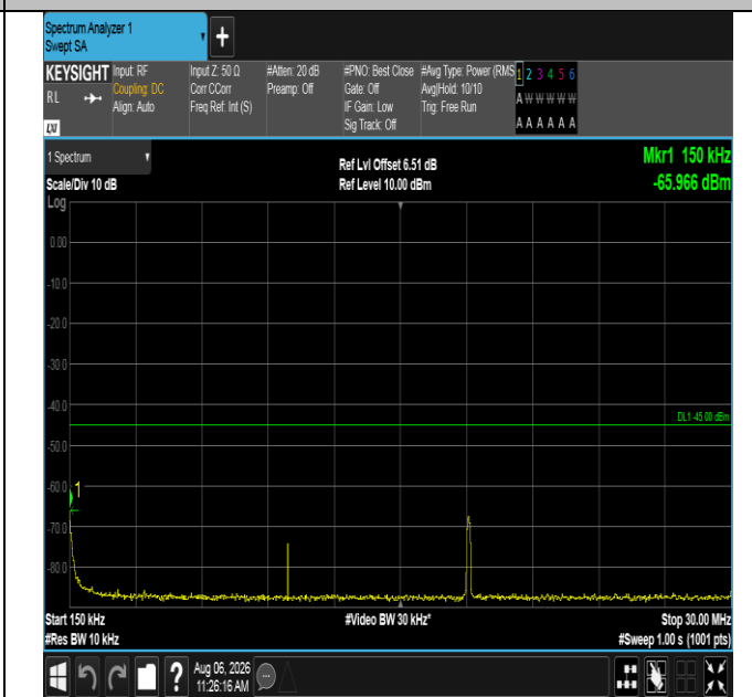
Band38-10MHz-QPSK-37800-1RB#49-0.15~30-PASS
