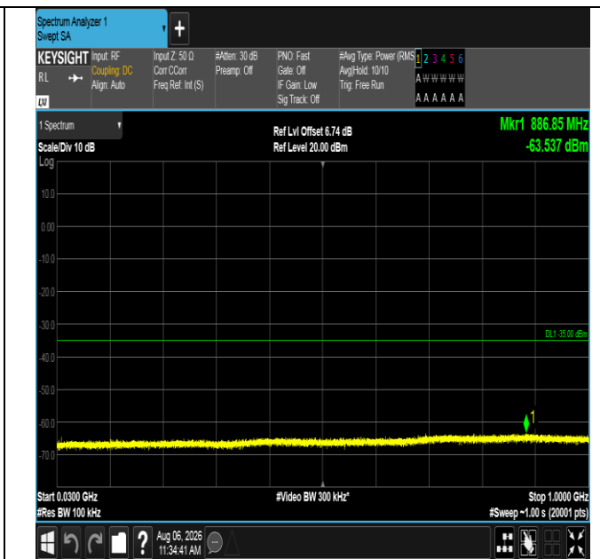
Band38-10MHz-QPSK-38000-1RB#49-30~1000-PASS
