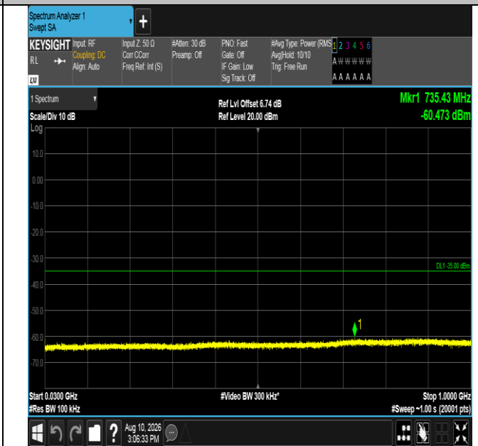
Band38-10MHz-QPSK-38000-50RB#0-30~1000-PASS
