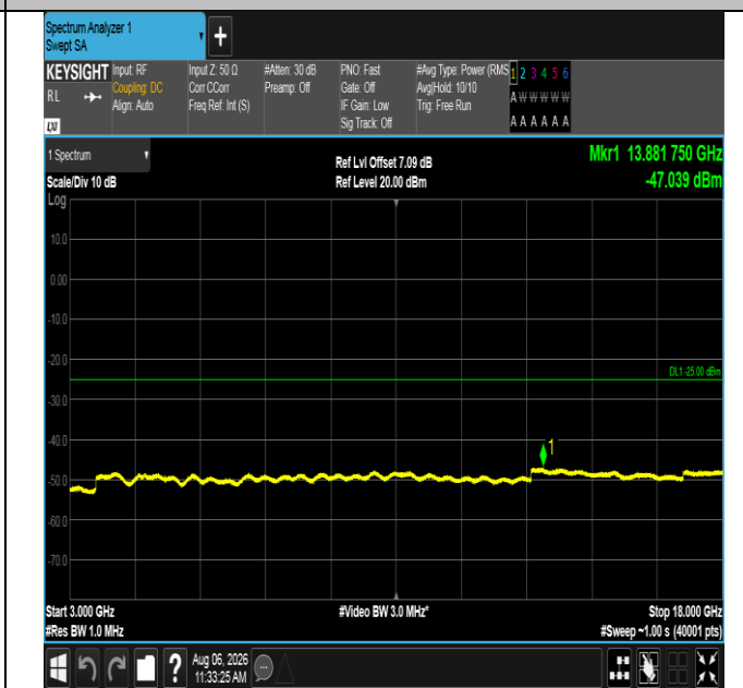
Band38-10MHz-16QAM-38000-1RB#0-3000~18000-PASS
