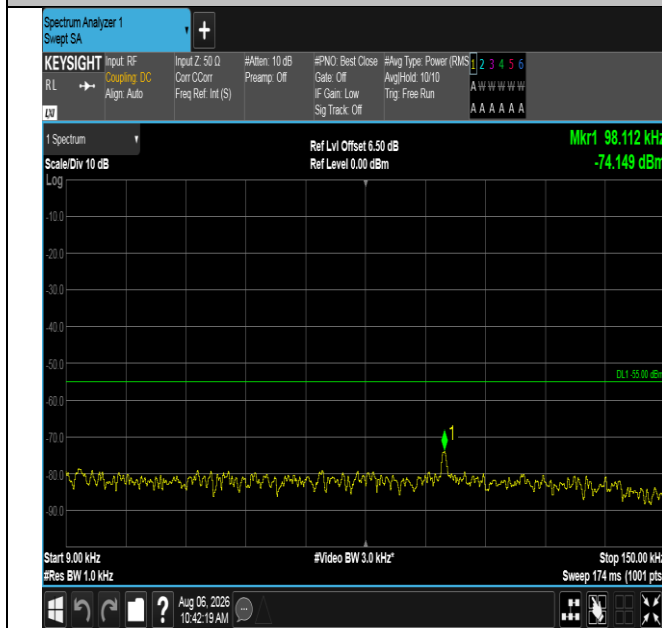
Band38-5MHz-16QAM-38225-25RB#0-0.009~0.15-PASS
