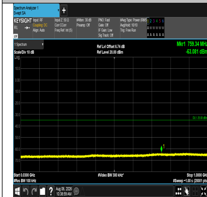
Band38-5MHz-16QAM-38225-1RB#24-30~1000-PASS
