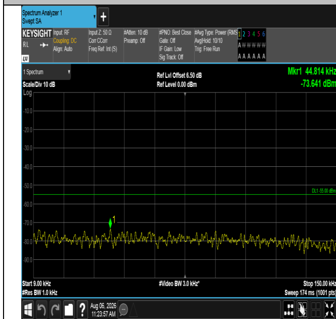
Band38-10MHz-16QAM-37800-1RB#0-0.009~0.15-PASS
