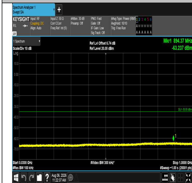
Band38-10MHz-QPSK-37800-1RB#0-30~1000-PASS
