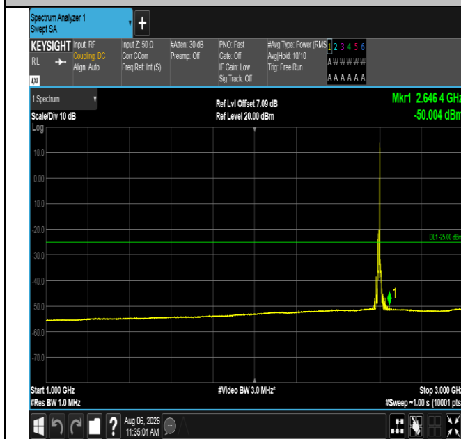
Band38-10MHz-QPSK-38000-1RB#49-1000~3000-PASS
