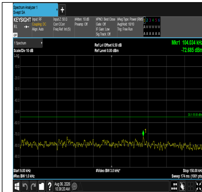
Band38-5MHz-16QAM-38225-1RB#24-0.009~0.15-PASS
