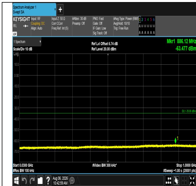
Band38-5MHz-16QAM-38225-25RB#0-30~1000-PASS
