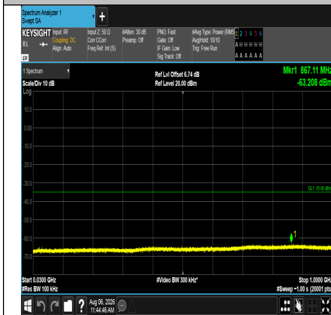
Band38-10MHz-16QAM-38200-1RB#49-30~1000-PASS
