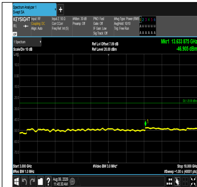
Band38-10MHz-16QAM-38200-1RB#49-3000~18000-PASS
