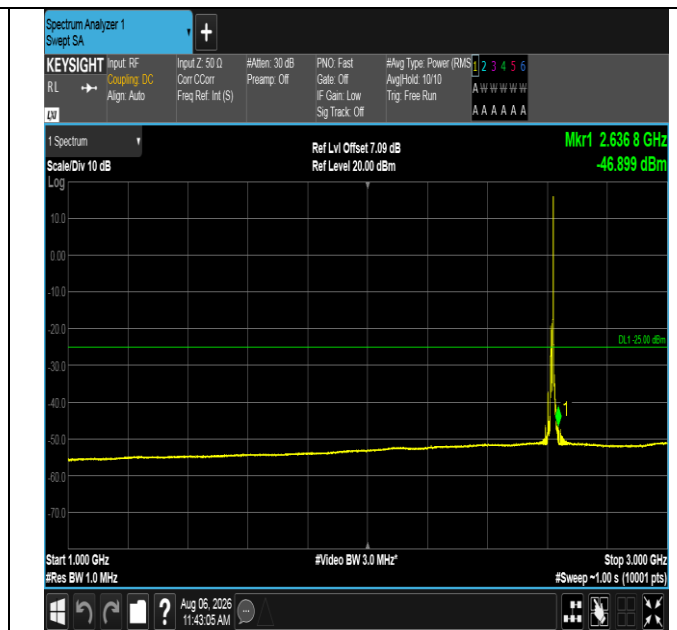
Band38-10MHz-QPSK-38200-1RB#49-1000~3000-PASS
