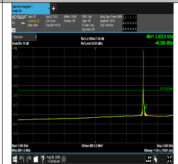
Band38-10MHz-16QAM-38200-1RB#49-1000~3000-PASS
