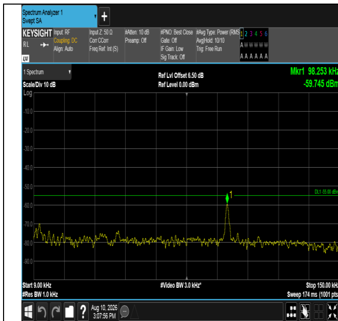
Band38-10MHz-QPSK-38200-50RB#0-0.009~0.15-PASS
