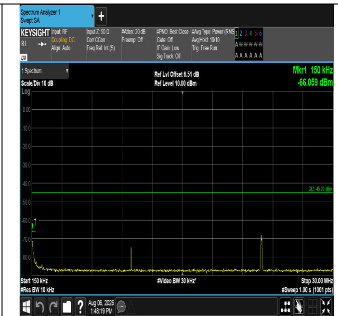
Band38-15MHz-16QAM-37825-1RB#74-0.15~30-PASS
