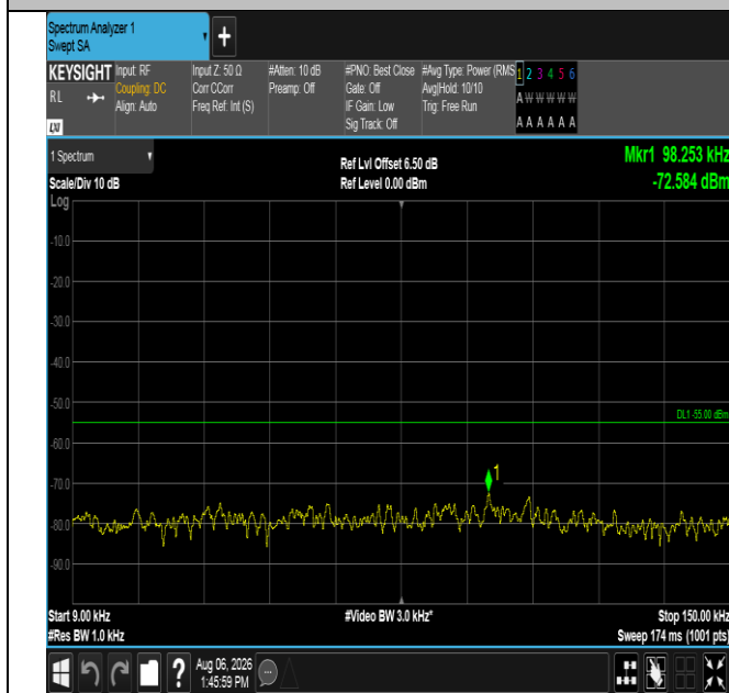
Band38-15MHz-QPSK-37825-1RB#74-0.009~0.15-PASS
