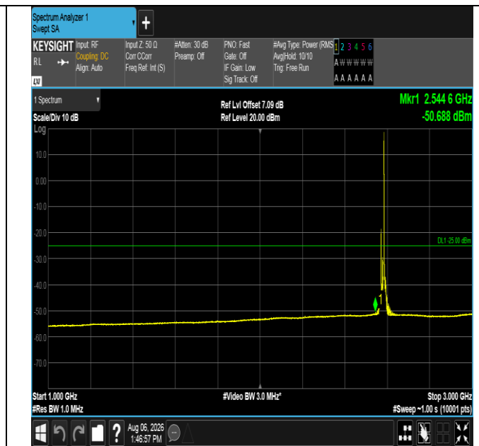
Band38-15MHz-QPSK-37825-1RB#74-1000~3000-PASS
