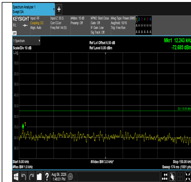
Band38-15MHz-16QAM-37825-1RB#74-0.009~0.15-PASS
