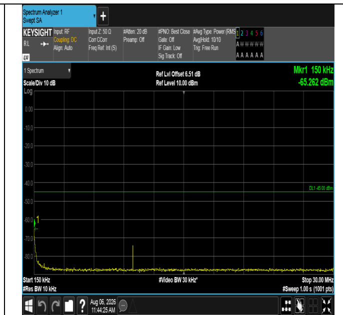
Band38-10MHz-16QAM-38200-1RB#49-0.15~30-PASS
