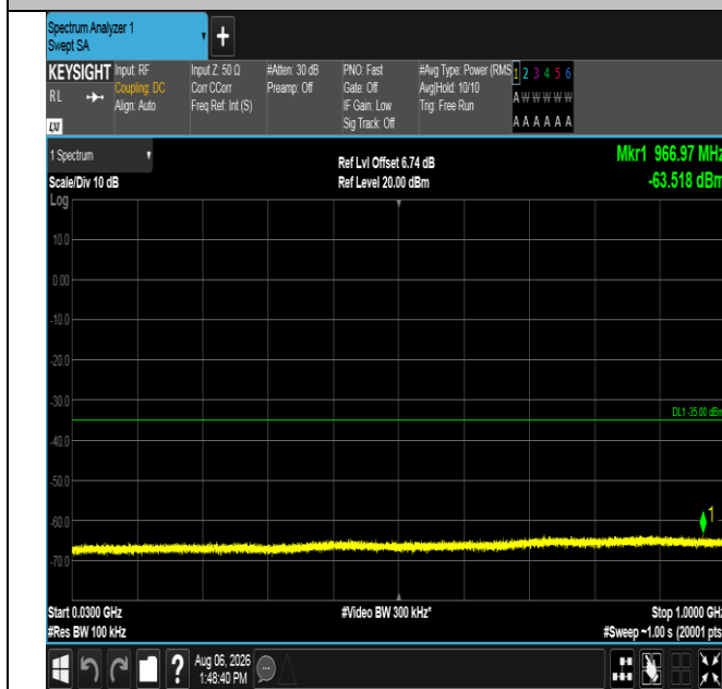
Band38-15MHz-16QAM-37825-1RB#74-30~1000-PASS
