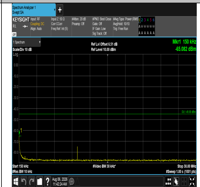
Band38-10MHz-QPSK-38200-1RB#49-0.15~30-PASS
