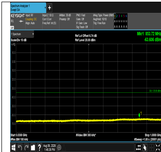
Band38-15MHz-QPSK-37825-1RB#74-30~1000-PASS
