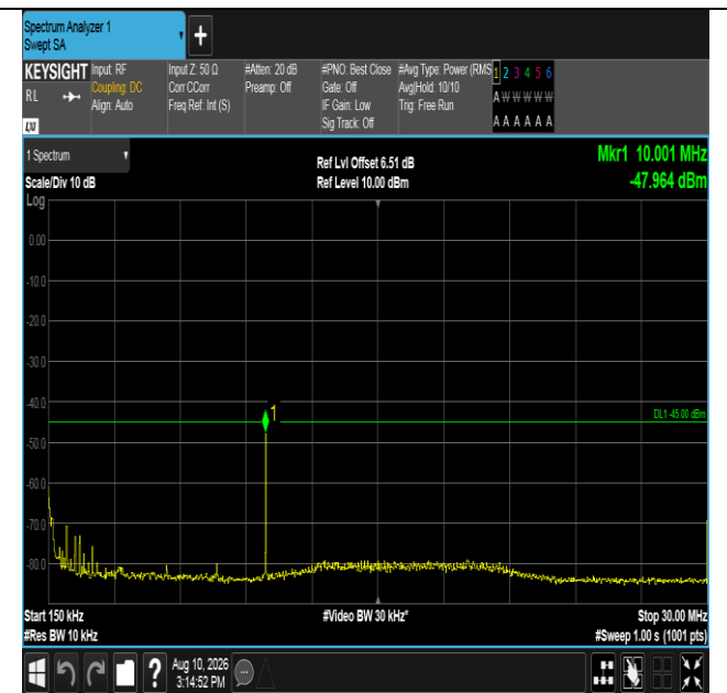
Band38-15MHz-QPSK-37825-75RB#0-0.15~30-PASS
