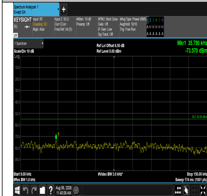
Band38-10MHz-16QAM-38200-1RB#0-0.009~0.15-PASS
