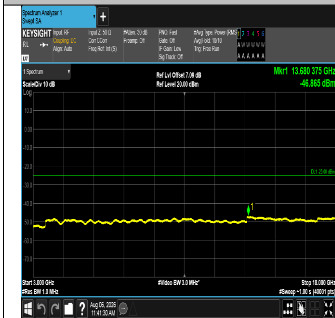
Band38-10MHz-16QAM-38200-1RB#0-3000~18000-PASS
