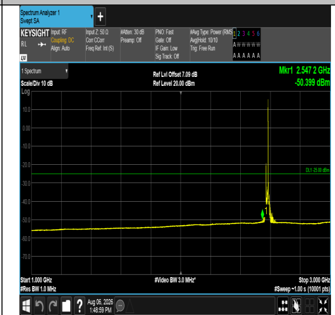
Band38-15MHz-16QAM-37825-1RB#74-1000~3000-PASS
