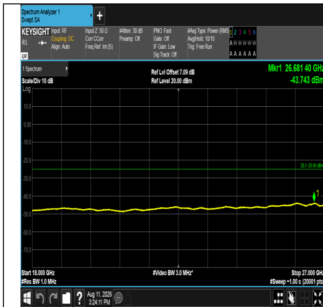
Band38-15MHz-16QAM-37825-75RB#0-18000~27000-PASS
