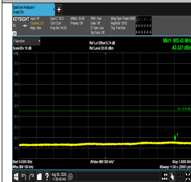
Band38-10MHz-QPSK-38200-1RB#0-30~1000-PASS
