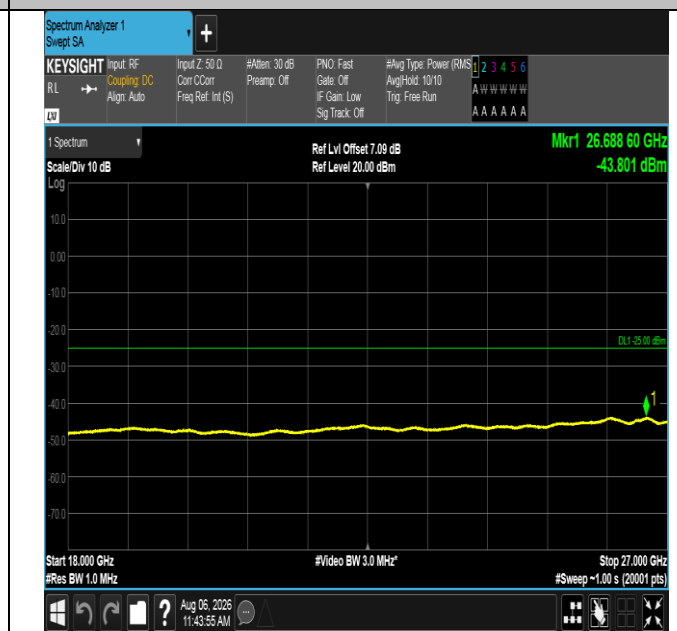
Band38-10MHz-QPSK-38200-1RB#49-18000~27000-PASS
