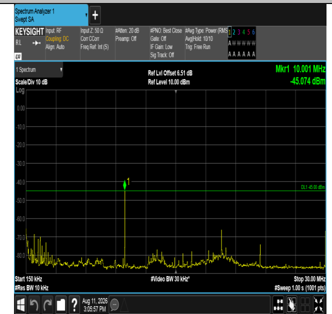
Band38-10MHz-16QAM-38200-50RB#0-0.15~30-PASS
