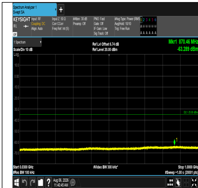
Band38-10MHz-16QAM-38200-1RB#0-30~1000-PASS
