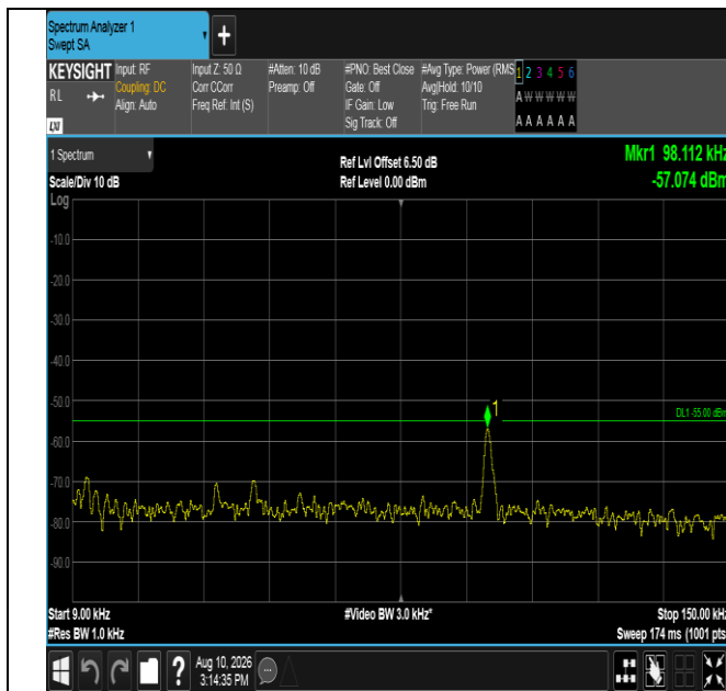
Band38-15MHz-QPSK-37825-75RB#0-0.009~0.15-PASS
