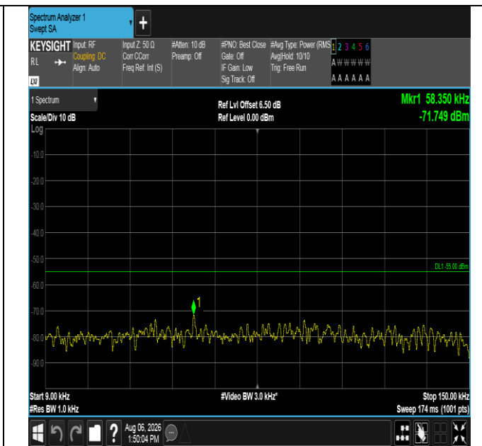
Band38-15MHz-QPSK-38000-1RB#0-0.009~0.15-PASS
