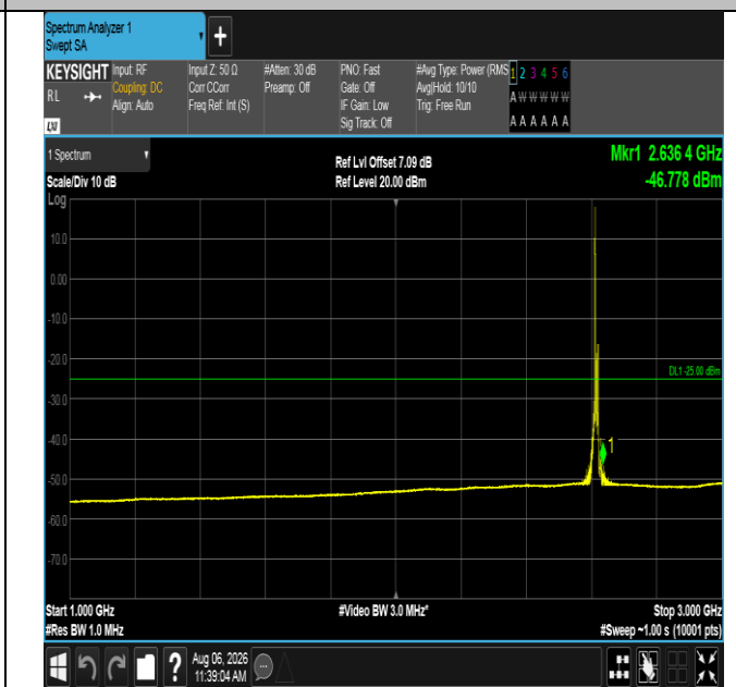
Band38-10MHz-QPSK-38200-1RB#0-1000~3000-PASS
