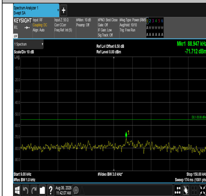
Band38-10MHz-QPSK-38200-1RB#49-0.009~0.15-PASS
