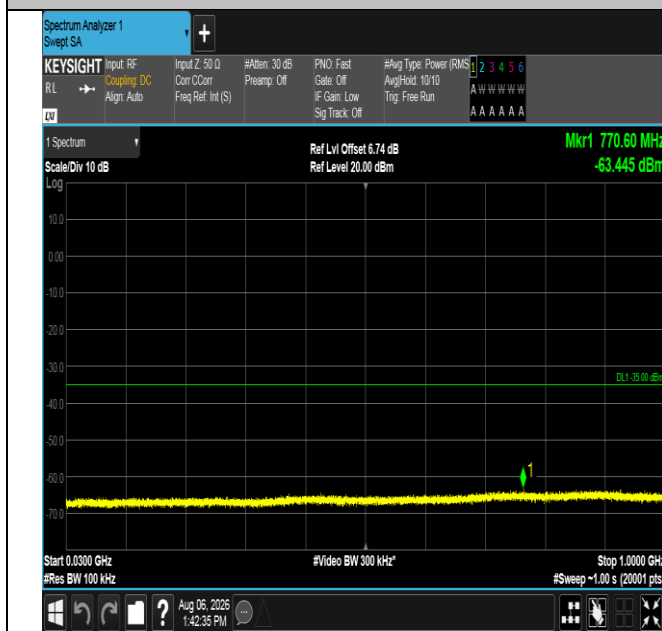
Band38-15MHz-QPSK-37825-1RB#0-30~1000-PASS
