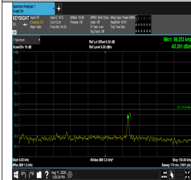
Band38-10MHz-16QAM-38200-50RB#0-0.009~0.15-PASS
