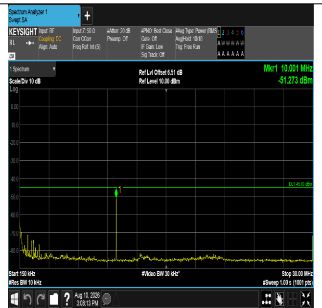
Band38-10MHz-QPSK-38200-50RB#0-0.15~30-PASS
