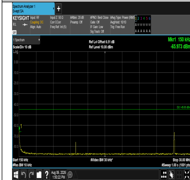
Band38-15MHz-QPSK-38000-1RB#0-0.15~30-PASS
