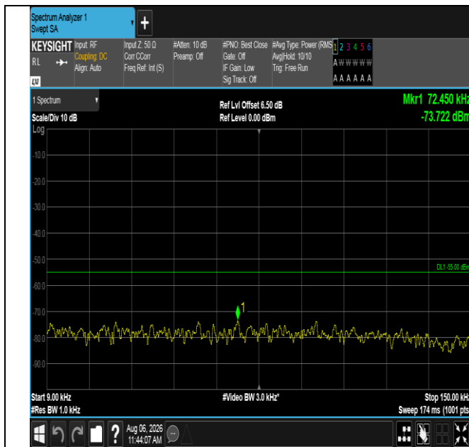
Band38-10MHz-16QAM-38200-1RB#49-0.009~0.15-PASS
