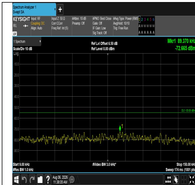
Band38-10MHz-QPSK-38200-1RB#0-0.009~0.15-PASS
