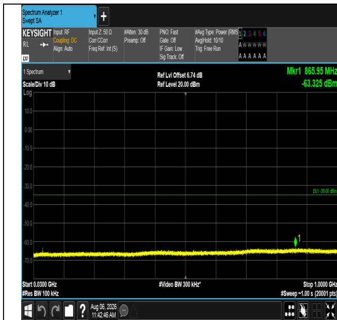
Band38-10MHz-QPSK-38200-1RB#49-30~1000-PASS
