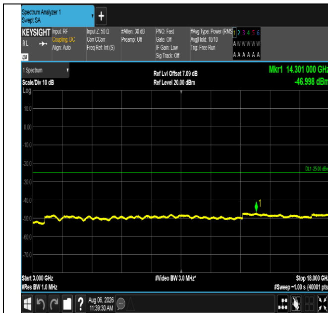
Band38-10MHz-QPSK-38200-1RB#0-3000~18000-PASS
