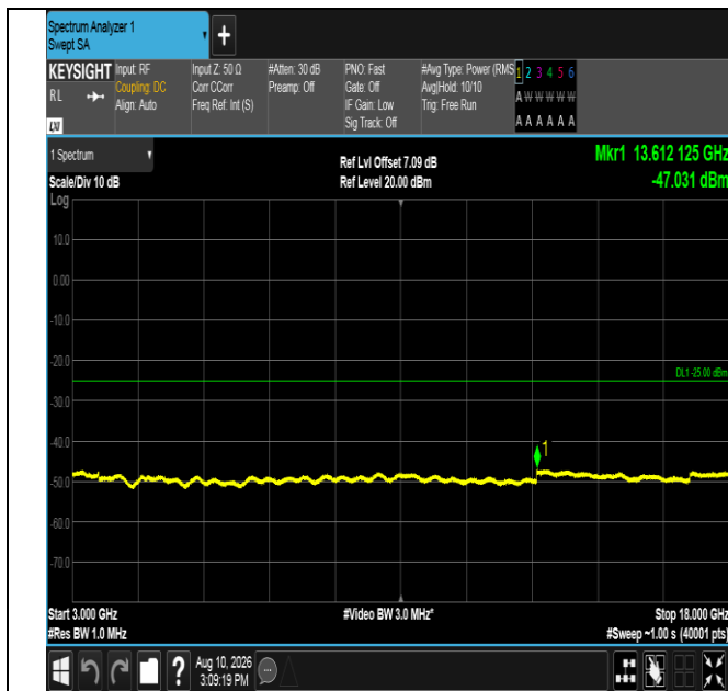
Band38-10MHz-QPSK-38200-50RB#0-3000~18000-PASS
