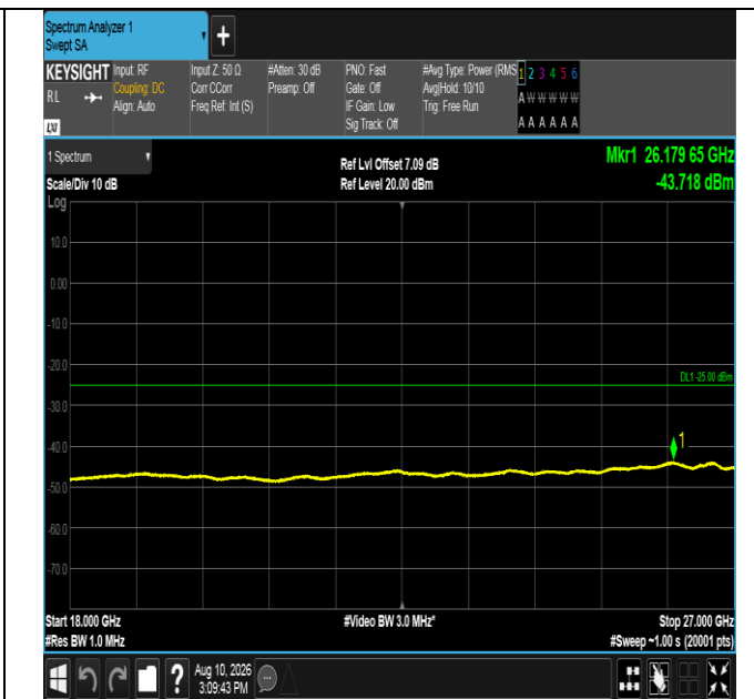
Band38-10MHz-QPSK-38200-50RB#0-18000~27000-PASS
