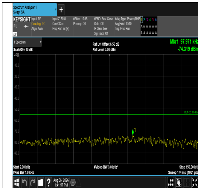
Band38-15MHz-QPSK-37825-1RB#0-0.009~0.15-PASS
