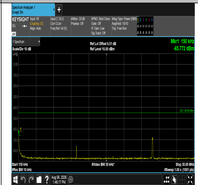
Band38-15MHz-QPSK-37825-1RB#74-0.15~30-PASS
