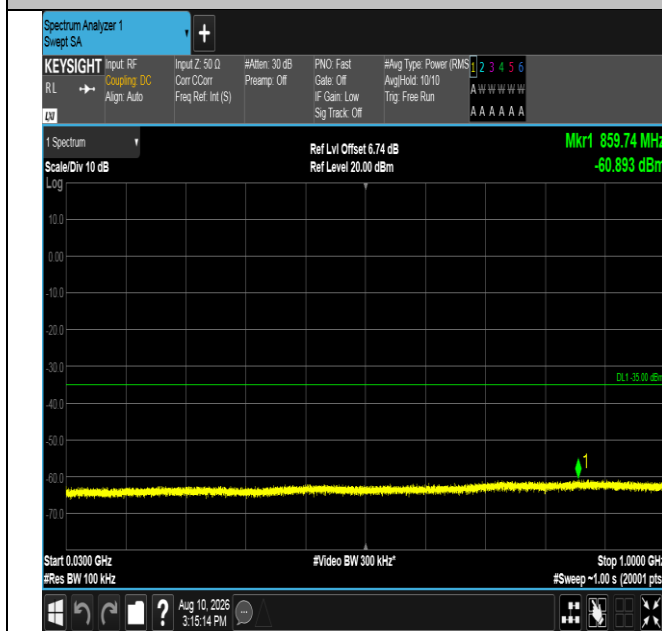
Band38-15MHz-QPSK-37825-75RB#0-30~1000-PASS
