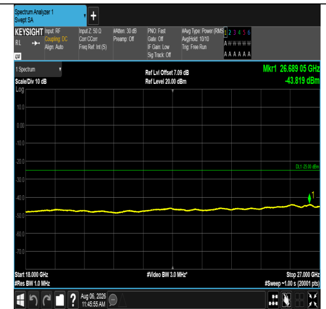
Band38-10MHz-16QAM-38200-1RB#49-18000~27000-PASS
