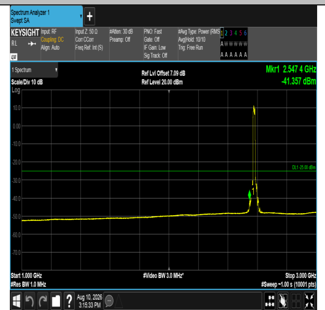
Band38-15MHz-QPSK-37825-75RB#0-1000~3000-PASS
