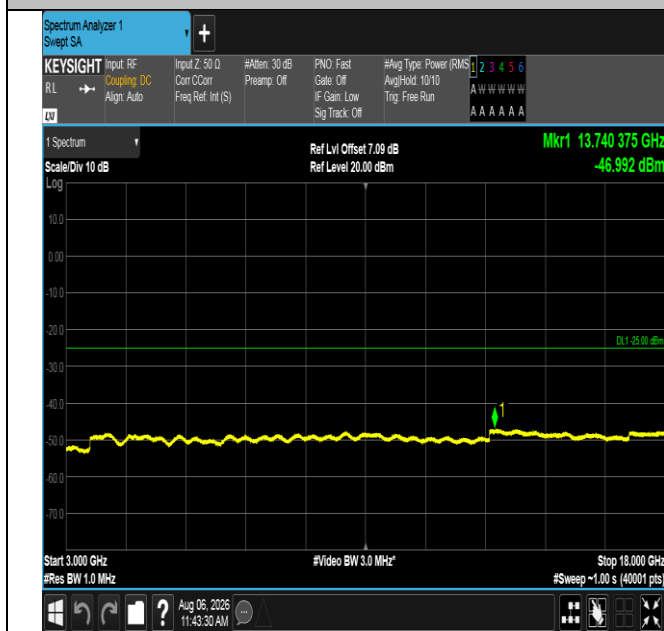
Band38-10MHz-QPSK-38200-1RB#49-3000~18000-PASS
