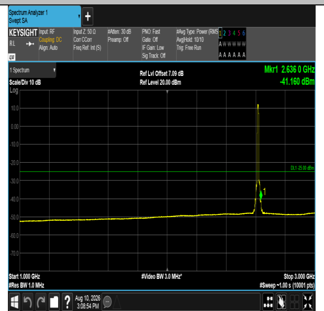
Band38-10MHz-QPSK-38200-50RB#0-1000~3000-PASS
