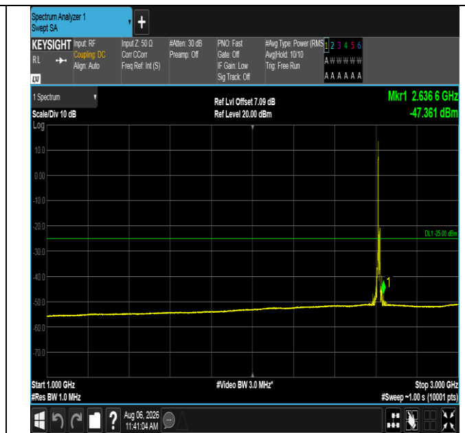
Band38-10MHz-16QAM-38200-1RB#0-1000~3000-PASS
