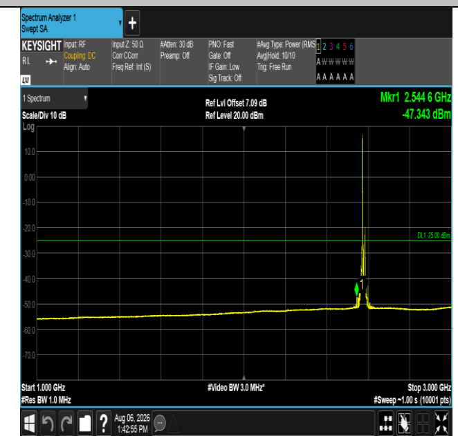
Band38-15MHz-QPSK-37825-1RB#0-1000~3000-PASS
