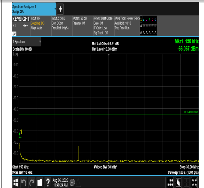
Band38-10MHz-16QAM-38200-1RB#0-0.15~30-PASS
