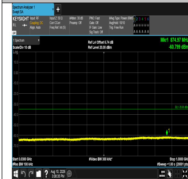
Band38-10MHz-QPSK-38200-50RB#0-30~1000-PASS
