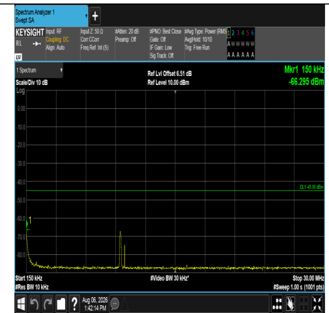
Band38-15MHz-QPSK-37825-1RB#0-0.15~30-PASS
