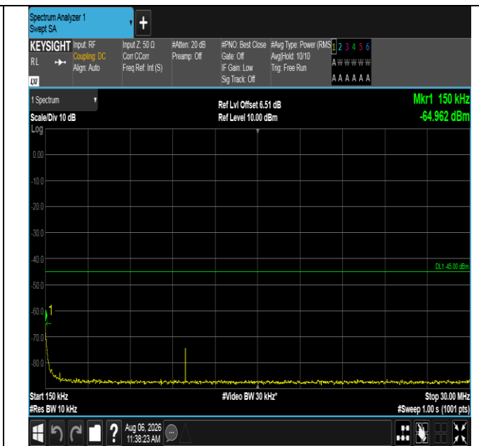
Band38-10MHz-QPSK-38200-1RB#0-0.15~30-PASS
