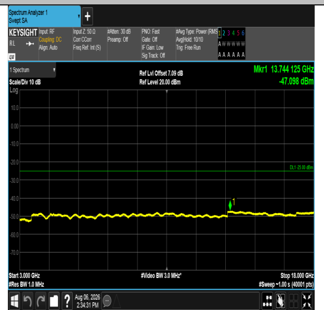
Band38-20MHz-16QAM-37850-1RB#0-3000~18000-PASS
