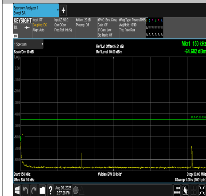
Band38-20MHz-16QAM-37850-1RB#99-0.15~30-PASS
