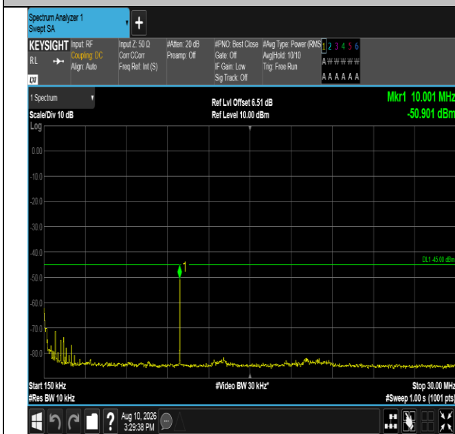
Band38-20MHz-QPSK-38150-100RB#0-0.15~30-PASS
