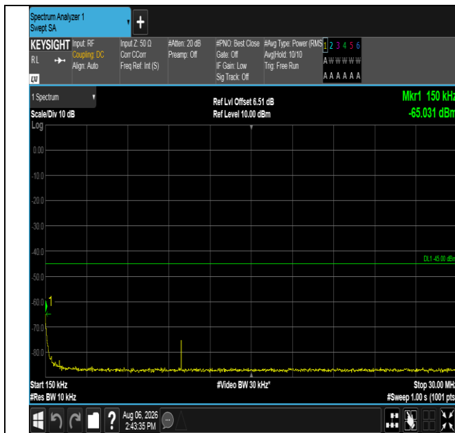
Band38-20MHz-QPSK-38000-1RB#99-0.15~30-PASS
