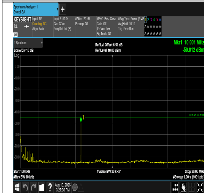
Band38-20MHz-QPSK-38000-100RB#0-0.15~30-PASS
