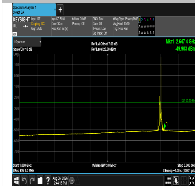
Band38-20MHz-QPSK-38000-1RB#99-1000~3000-PASS
