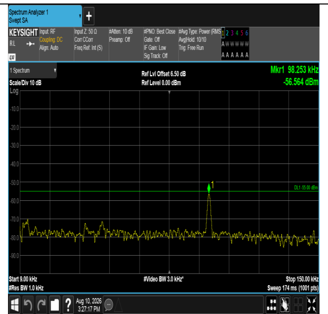
Band38-20MHz-QPSK-38000-100RB#0-0.009~0.15-PASS
