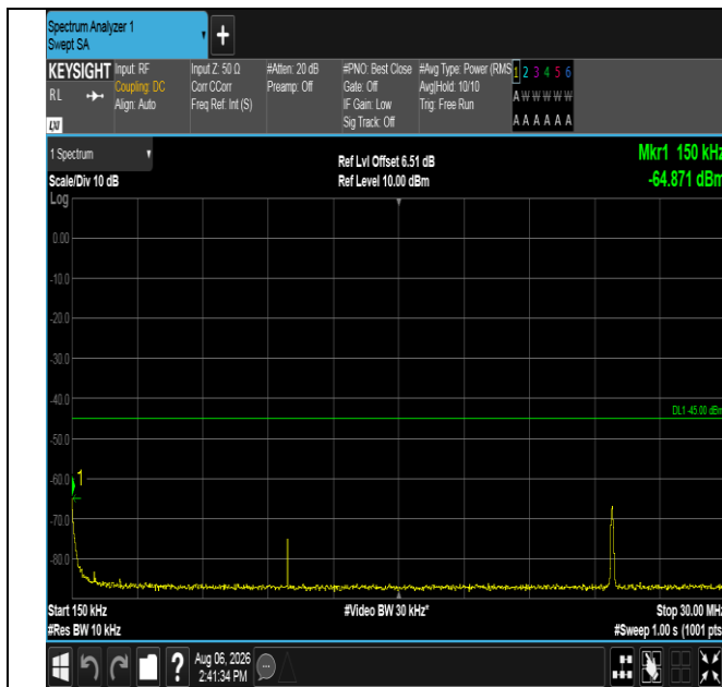
Band38-20MHz-16QAM-38000-1RB#0-0.15~30-PASS
