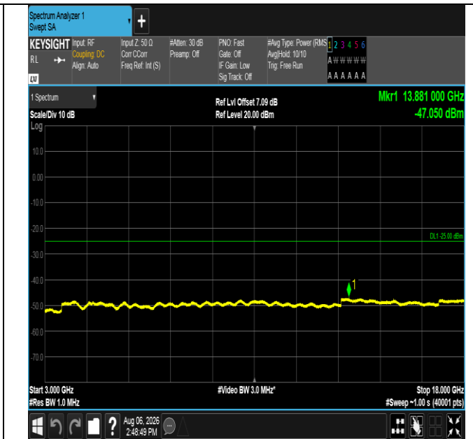
Band38-20MHz-QPSK-38150-1RB#0-3000~18000-PASS
