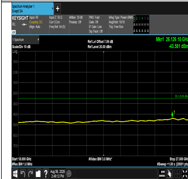
Band38-20MHz-QPSK-38150-1RB#0-18000~27000-PASS
