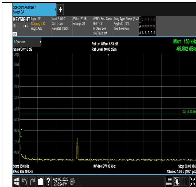
Band38-20MHz-16QAM-37850-1RB#0-0.15~30-PASS
