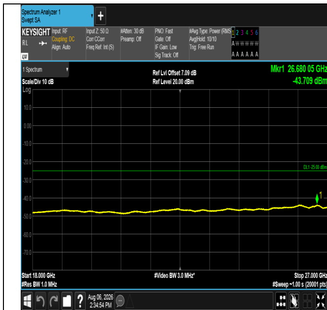
Band38-20MHz-16QAM-37850-1RB#0-18000~27000-PASS
