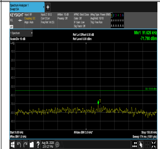
Band38-20MHz-QPSK-38150-1RB#99-0.009~0.15-PASS
