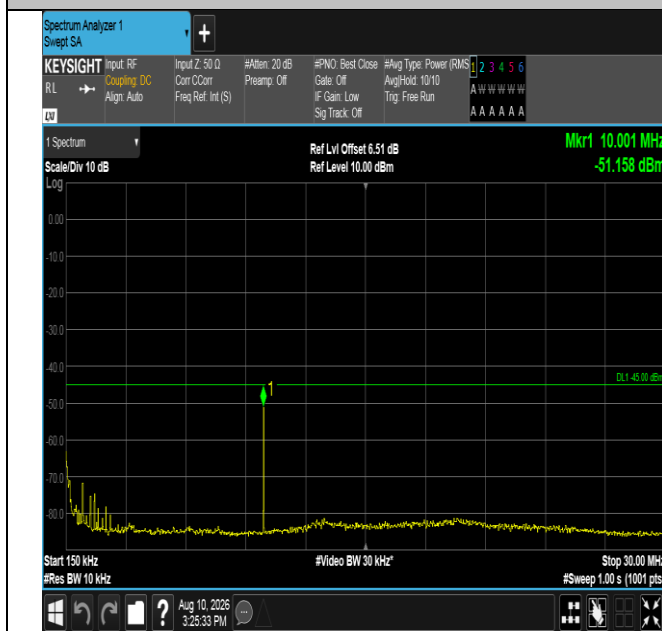
Band38-20MHz-QPSK-37850-100RB#0-0.15~30-PASS
