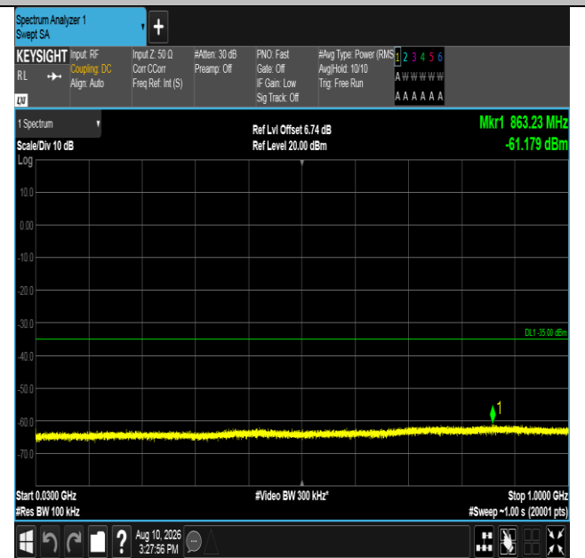
Band38-20MHz-QPSK-38000-100RB#0-30~1000-PASS
