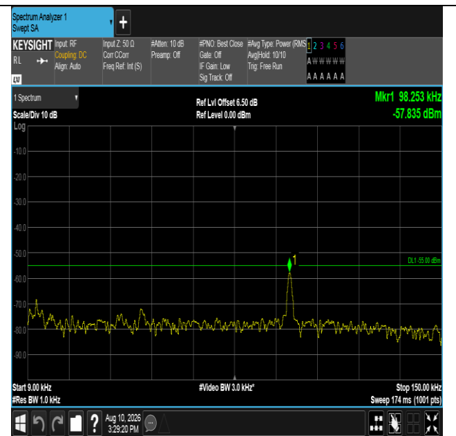
Band38-20MHz-QPSK-38150-100RB#0-0.009~0.15-PASS
