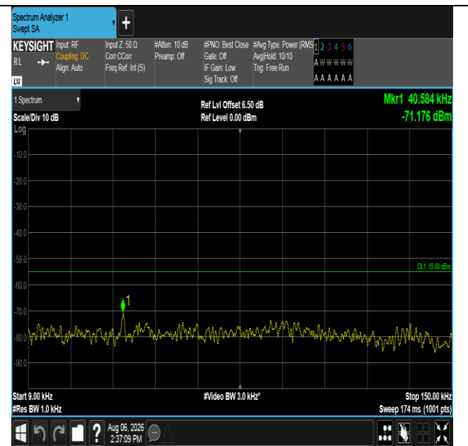
Band38-20MHz-16QAM-37850-1RB#99-0.009~0.15-PASS
