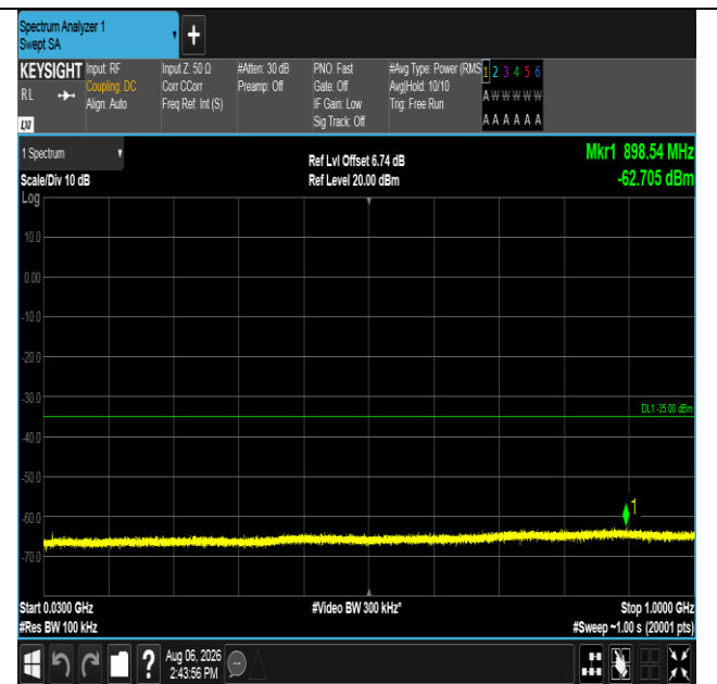
Band38-20MHz-QPSK-38000-1RB#99-30~1000-PASS
