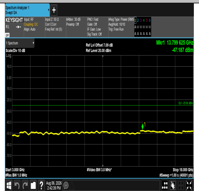
Band38-20MHz-16QAM-38000-1RB#0-3000~18000-PASS
