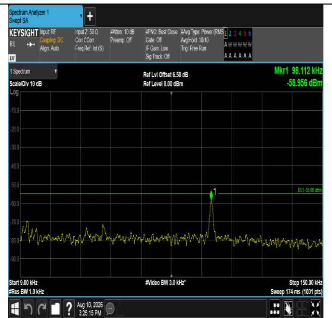
Band38-20MHz-QPSK-37850-100RB#0-0.009~0.15-PASS
