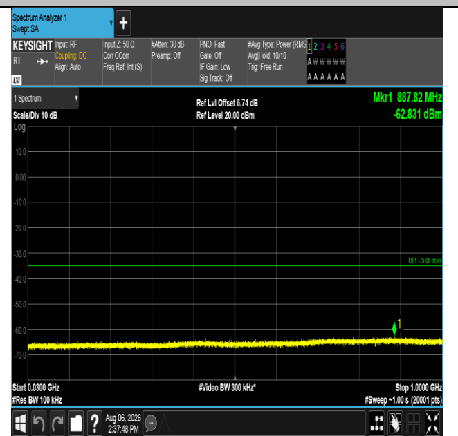
Band38-20MHz-16QAM-37850-1RB#99-30~1000-PASS
