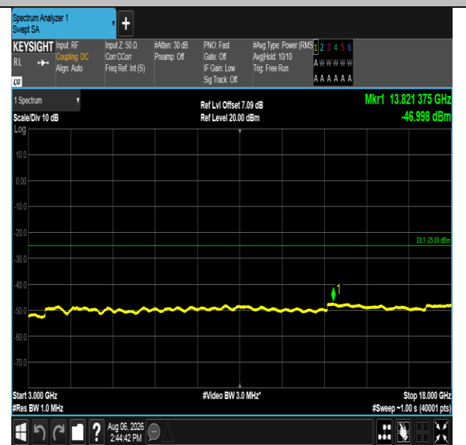
Band38-20MHz-QPSK-38000-1RB#99-3000~18000-PASS
