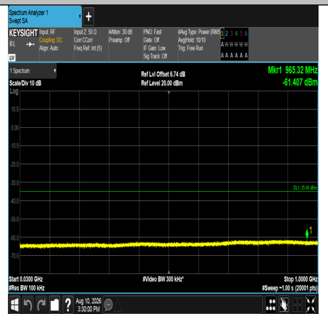
Band38-20MHz-QPSK-38150-100RB#0-30~1000-PASS
