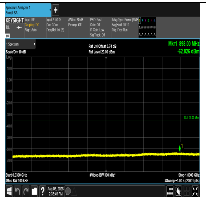
Band38-20MHz-16QAM-37850-1RB#0-30~1000-PASS
