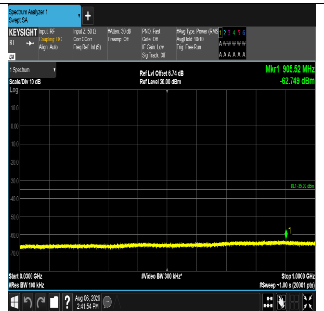
Band38-20MHz-16QAM-38000-1RB#0-30~1000-PASS
