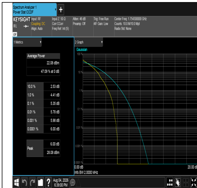
Band4-1.4MHz-QPSK-20393-1RB#0-PASS
