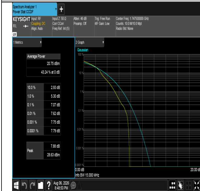
Band4-15MHz-16QAM-20325-1RB#0-PASS
