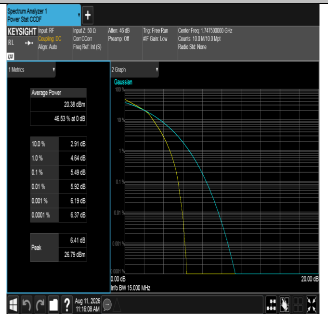
Band4-15MHz-16QAM-20325-75RB#0-PASS
