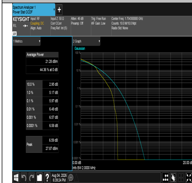
Band4-1.4MHz-16QAM-20393-1RB#0-PASS
