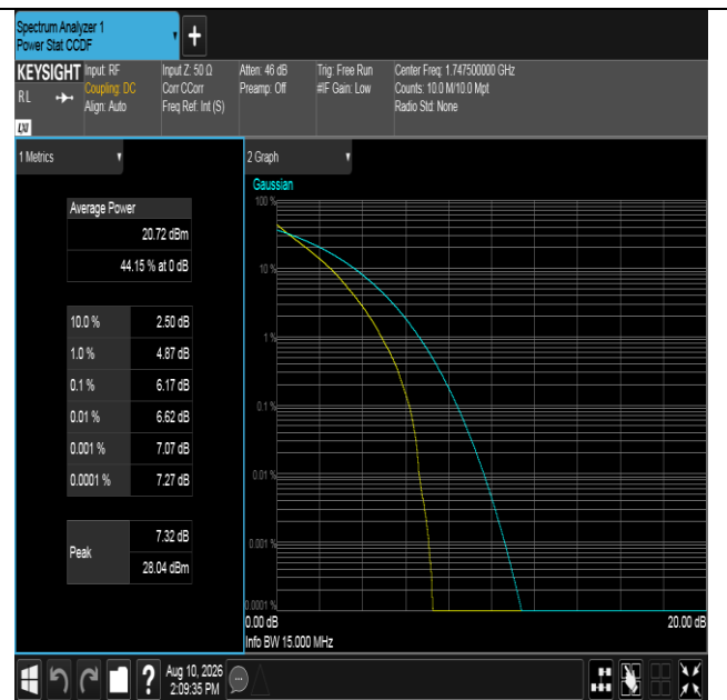
Band4-15MHz-QPSK-20325-75RB#0-PASS
