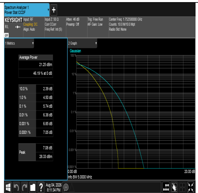
Band4-5MHz-QPSK-20375-25RB#0-PASS
