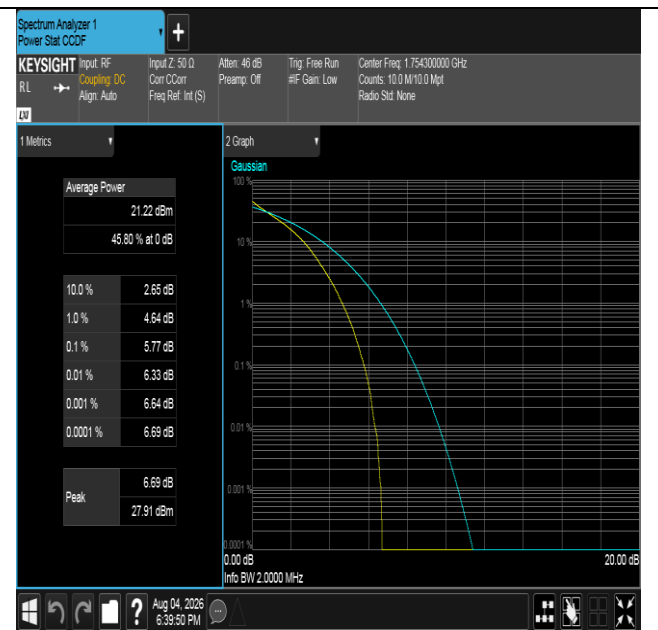
Band4-1.4MHz-QPSK-20393-6RB#0-PASS
