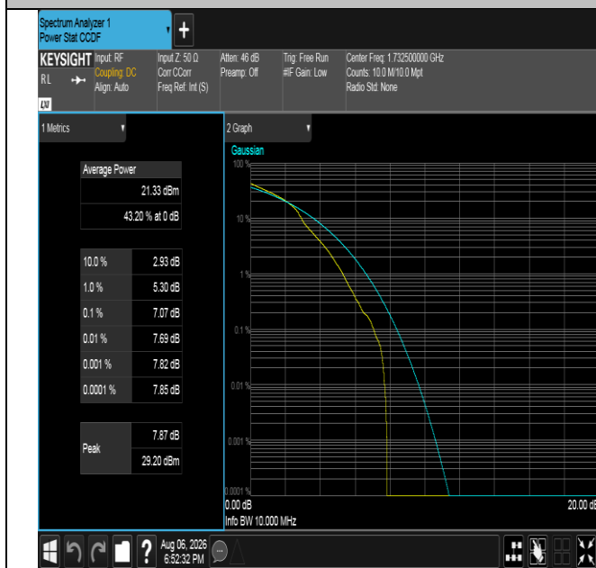
Band4-10MHz-16QAM-20175-1RB#0-PASS
