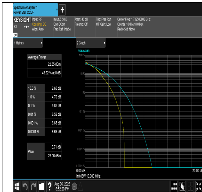
Band4-10MHz-QPSK-20175-1RB#0-PASS
