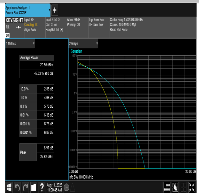
Band4-10MHz-16QAM-20175-50RB#0-PASS
