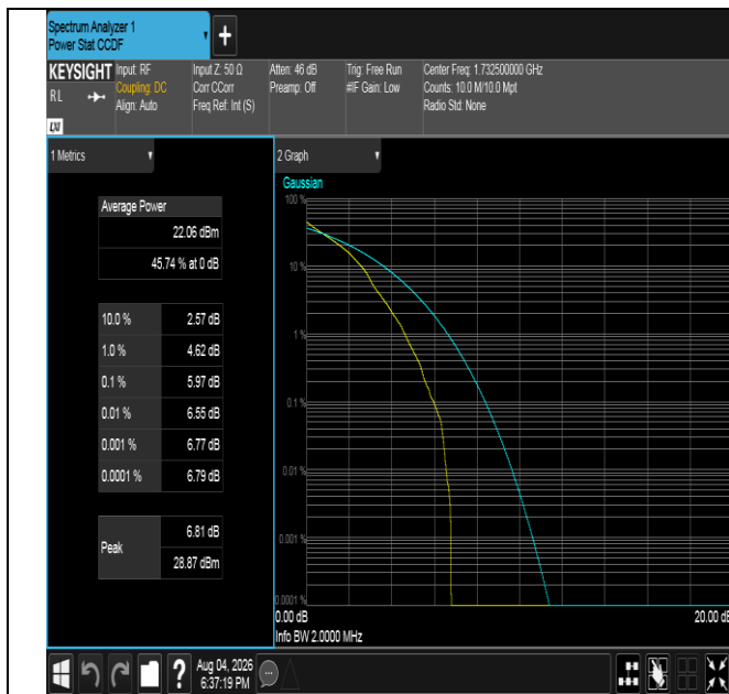
Band4-1.4MHz-QPSK-20175-1RB#0-PASS
