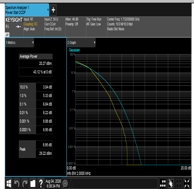
Band4-1.4MHz-16QAM-20175-6RB#0-PASS
