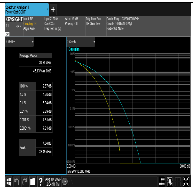
Band4-10MHz-QPSK-20175-50RB#0-PASS
