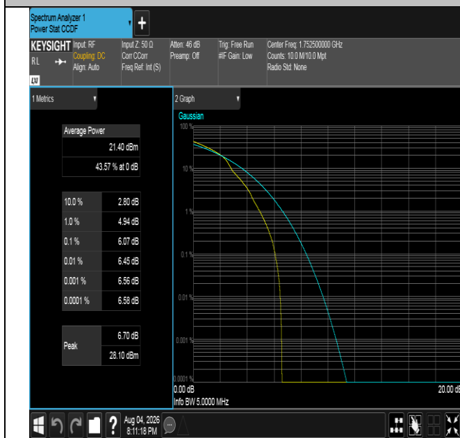
Band4-5MHz-16QAM-20375-1RB#0-PASS
