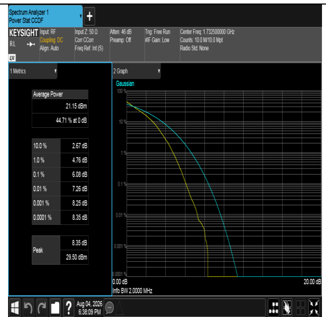
Band4-1.4MHz-QPSK-20175-6RB#0-PASS
