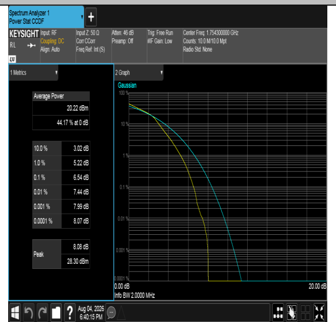
Band4-1.4MHz-16QAM-20393-6RB#0-PASS
