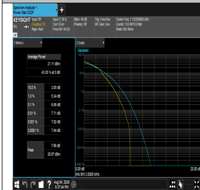
Band4-1.4MHz-16QAM-20175-1RB#0-PASS
