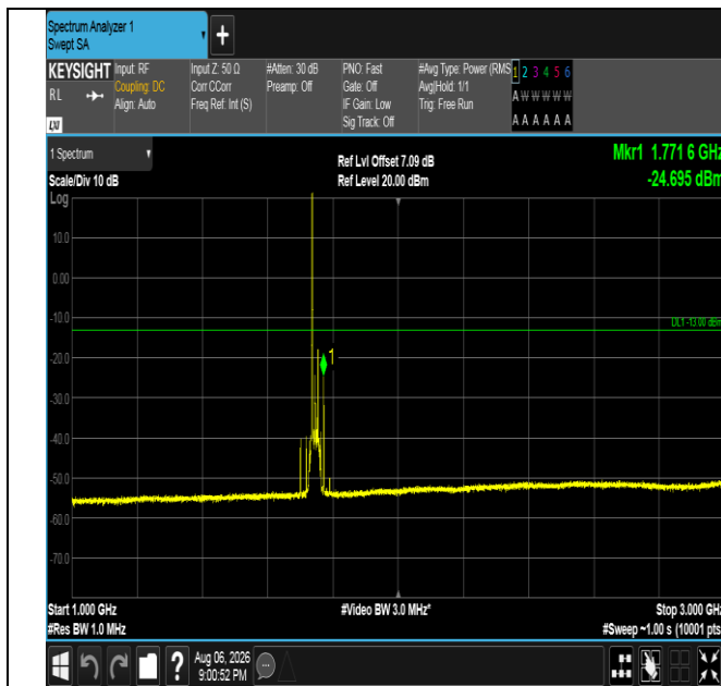
Band4-20MHz-16QAM-20300-1RB#0-1000~3000-PASS
