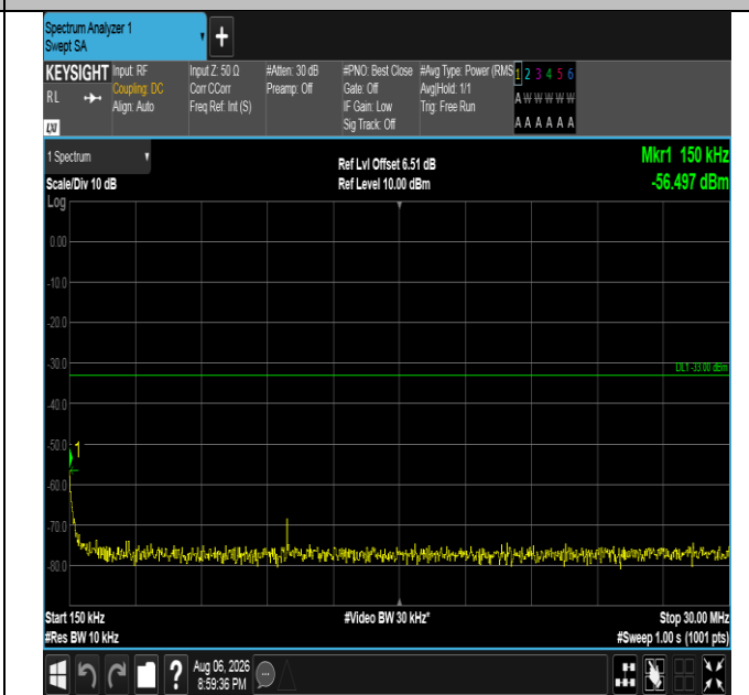
Band4-20MHz-QPSK-20300-1RB#0-0.15~30-PASS
