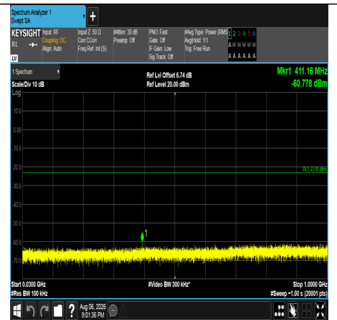
Band4-20MHz-QPSK-20300-1RB#99-30~1000-PASS
