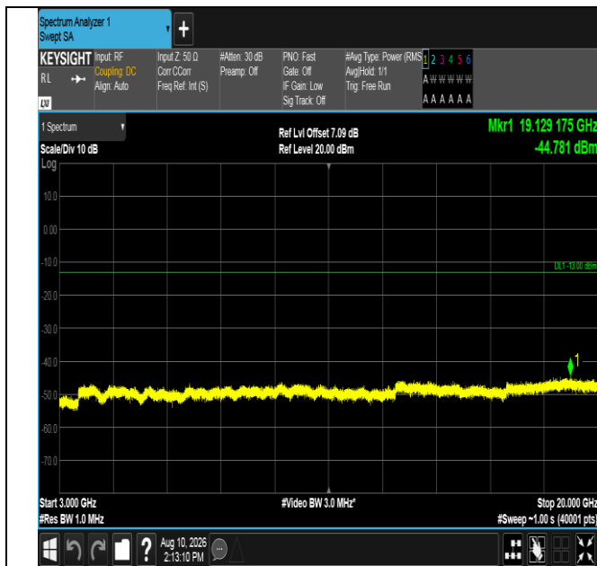
Band4-20MHz-QPSK-20300-100RB#0-3000~20000-PASS
