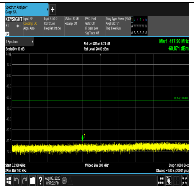
Band4-20MHz-16QAM-20175-1RB#0-30~1000-PASS
