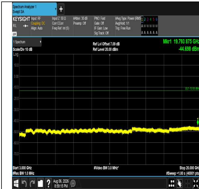
Band4-20MHz-16QAM-20175-1RB#99-3000~20000-PASS
