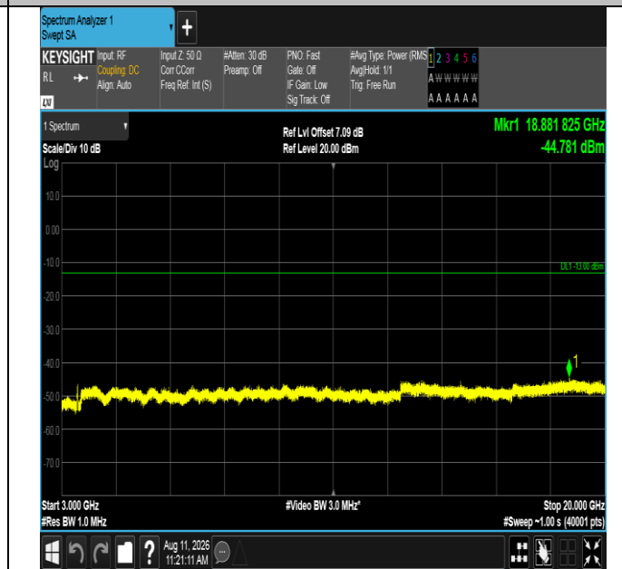
Band4-20MHz-16QAM-20300-100RB#0-3000~20000-PASS
