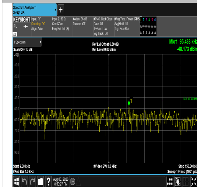
Band4-20MHz-QPSK-20300-1RB#0-0.009~0.15-PASS
