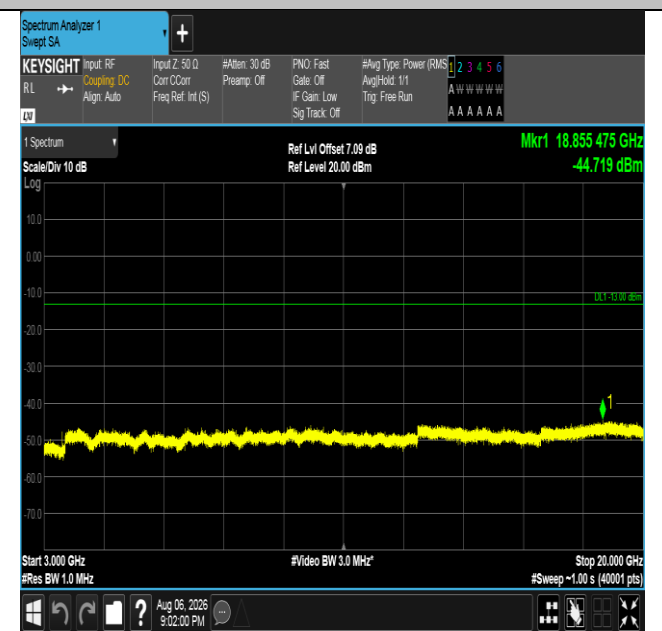
Band4-20MHz-QPSK-20300-1RB#99-3000~20000-PASS
