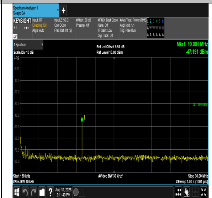
Band4-20MHz-QPSK-20175-100RB#0-0.15~30-PASS
