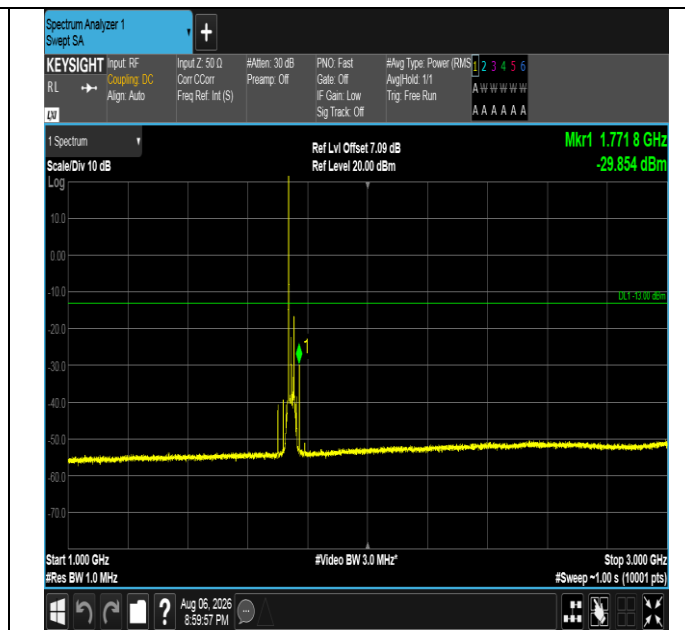
Band4-20MHz-QPSK-20300-1RB#0-1000~3000-PASS
