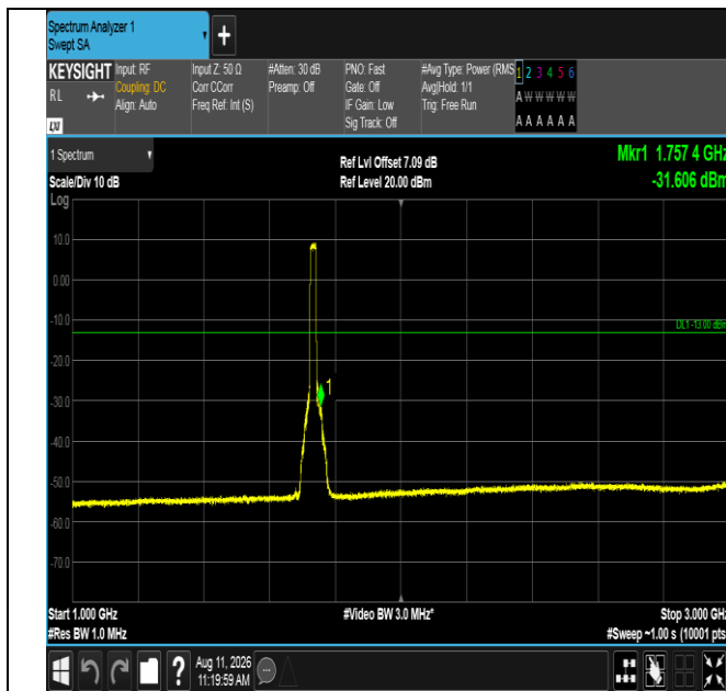
Band4-20MHz-16QAM-20175-100RB#0-1000~3000-PASS
