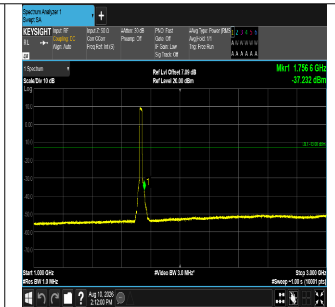
Band4-20MHz-QPSK-20175-100RB#0-1000~3000-PASS
