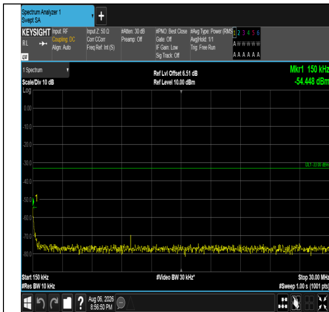
Band4-20MHz-16QAM-20175-1RB#0-0.15~30-PASS
