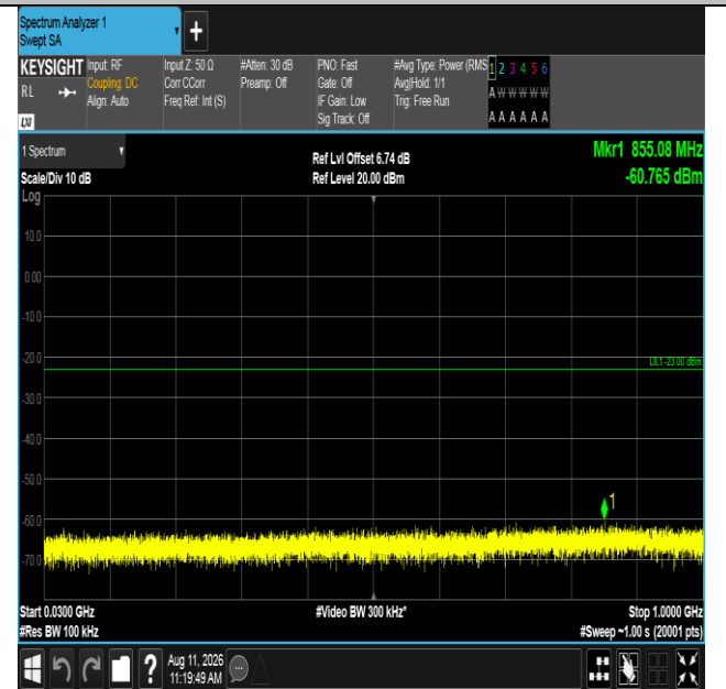
Band4-20MHz-16QAM-20175-100RB#0-30~1000-PASS
