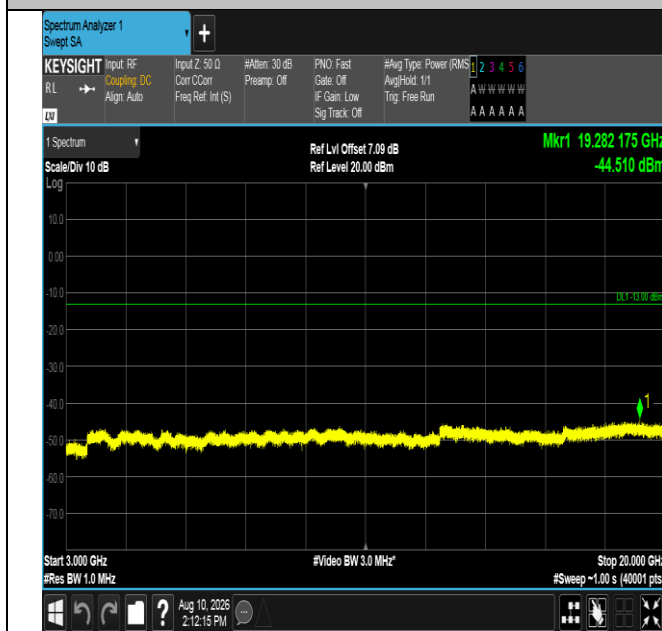
Band4-20MHz-QPSK-20175-100RB#0-3000~20000-PASS
