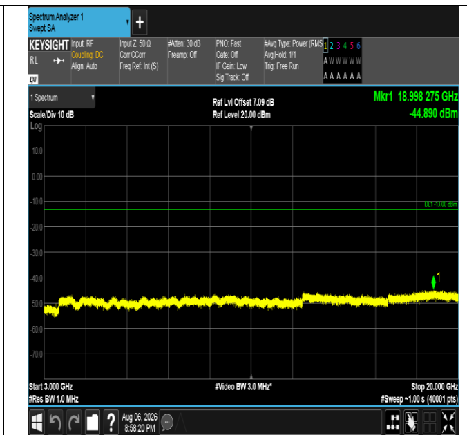
Band4-20MHz-QPSK-20175-1RB#99-3000~20000-PASS
