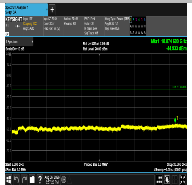
Band4-20MHz-16QAM-20175-1RB#0-3000~20000-PASS
