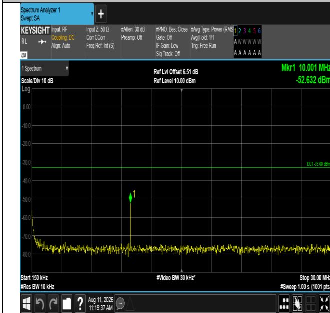
Band4-20MHz-16QAM-20175-100RB#0-0.15~30-PASS
