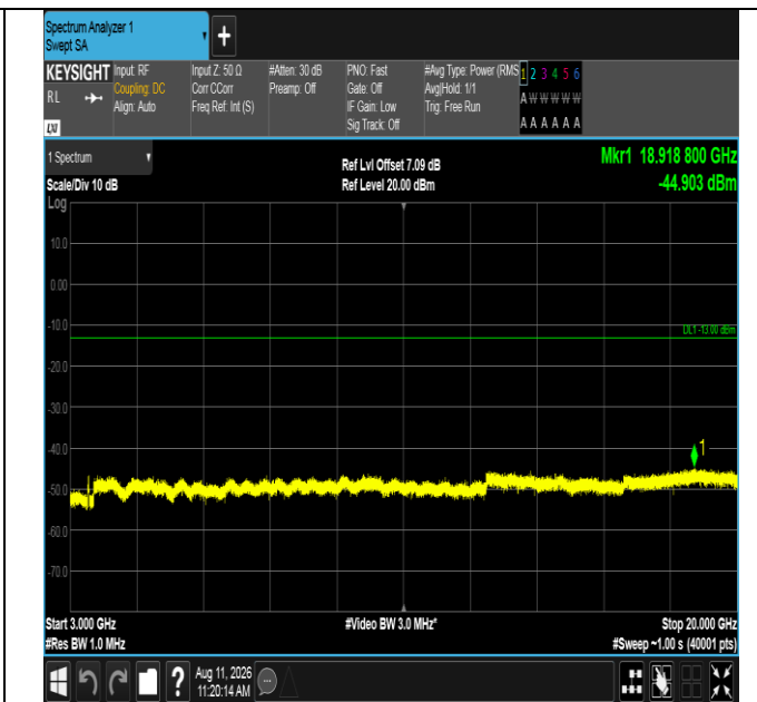
Band4-20MHz-16QAM-20175-100RB#0-3000~20000-PASS
