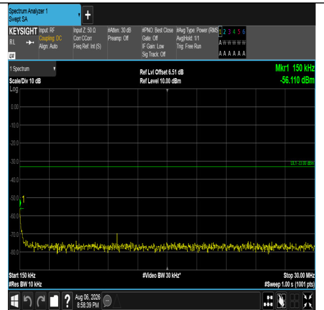
Band4-20MHz-16QAM-20175-1RB#99-0.15~30-PASS
