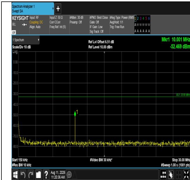
Band4-20MHz-16QAM-20300-100RB#0-0.15~30-PASS
