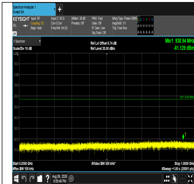
Band4-20MHz-QPSK-20300-1RB#0-30~1000-PASS
