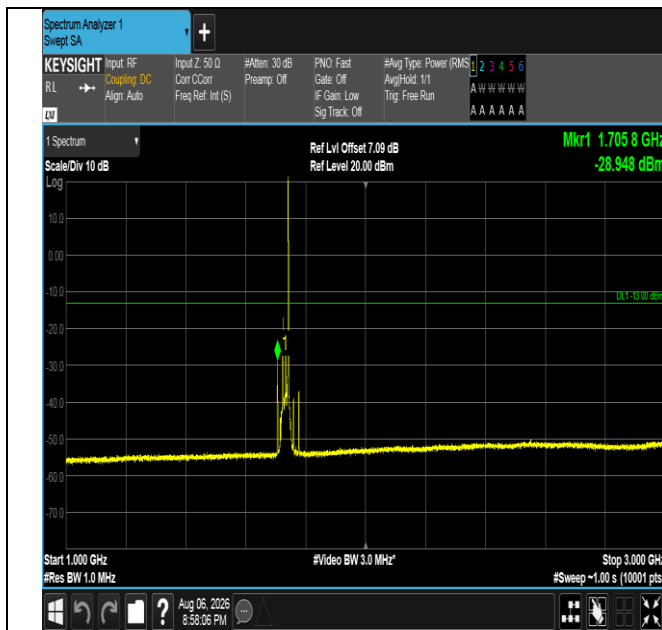
Band4-20MHz-QPSK-20175-1RB#99-1000~3000-PASS
