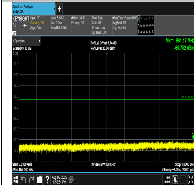
Band4-20MHz-16QAM-20175-1RB#99-30~1000-PASS
