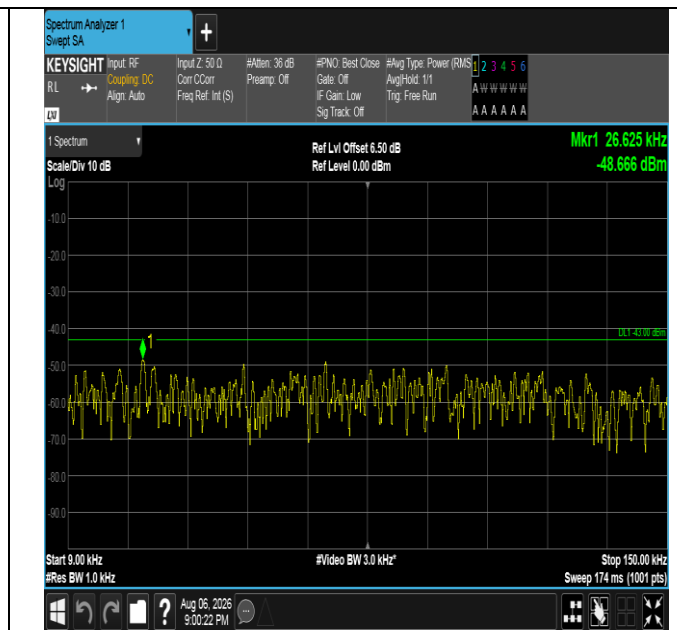
Band4-20MHz-16QAM-20300-1RB#0-0.009~0.15-PASS
