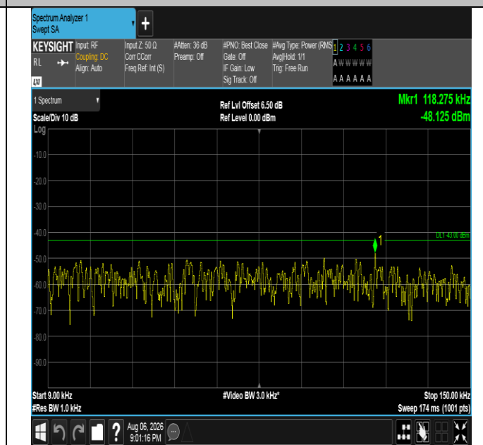
Band4-20MHz-QPSK-20300-1RB#99-0.009~0.15-PASS
