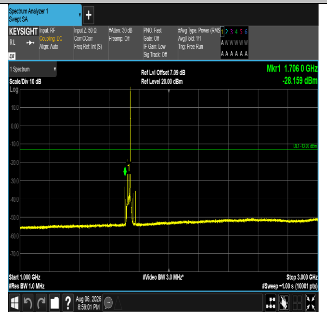
Band4-20MHz-16QAM-20175-1RB#99-1000~3000-PASS
