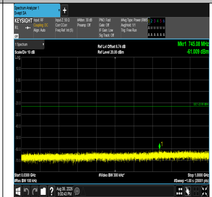
Band4-20MHz-16QAM-20300-1RB#0-30~1000-PASS
