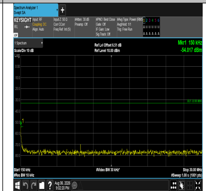
Band4-20MHz-16QAM-20300-1RB#99-0.15~30-PASS
