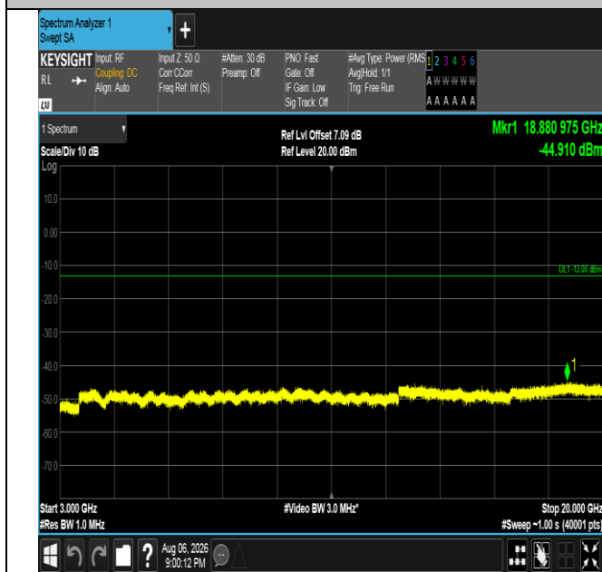
Band4-20MHz-QPSK-20300-1RB#0-3000~20000-PASS
