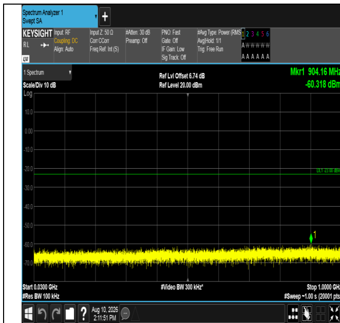
Band4-20MHz-QPSK-20175-100RB#0-30~1000-PASS
