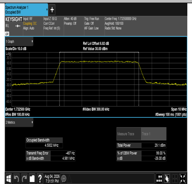
Band4-5MHz-16QAM-20175-25RB#0-PASS
