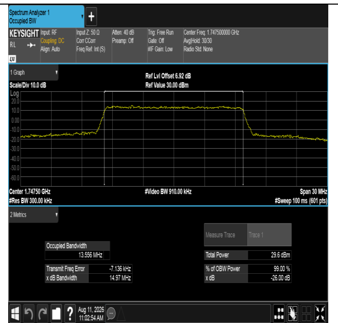
Band4-15MHz-16QAM-20325-75RB#0-PASS
