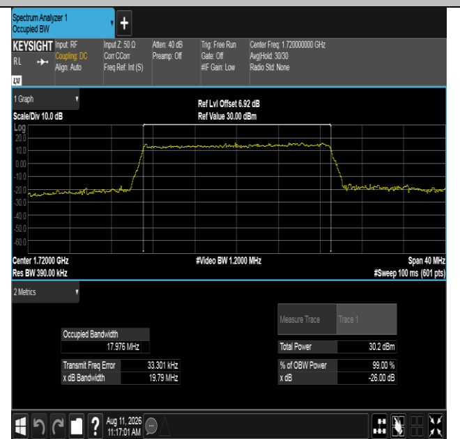
Band4-20MHz-16QAM-20050-100RB#0-PASS
