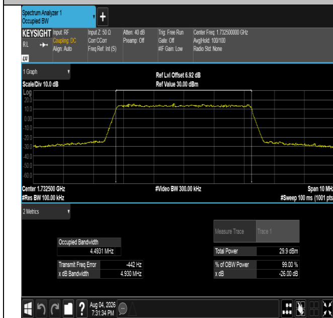
Band4-5MHz-QPSK-20175-25RB#0-PASS
