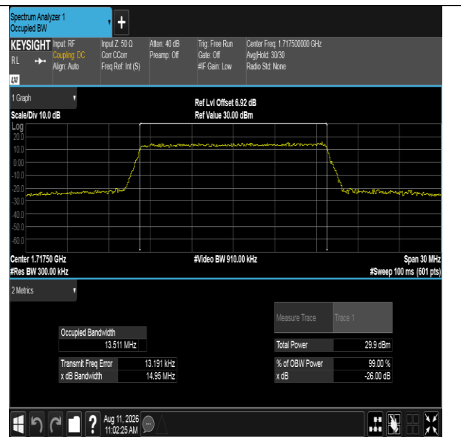
Band4-15MHz-16QAM-20025-75RB#0-PASS
