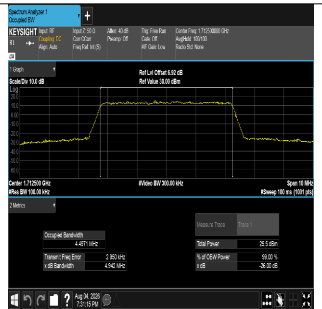
Band4-5MHz-16QAM-19975-25RB#0-PASS
