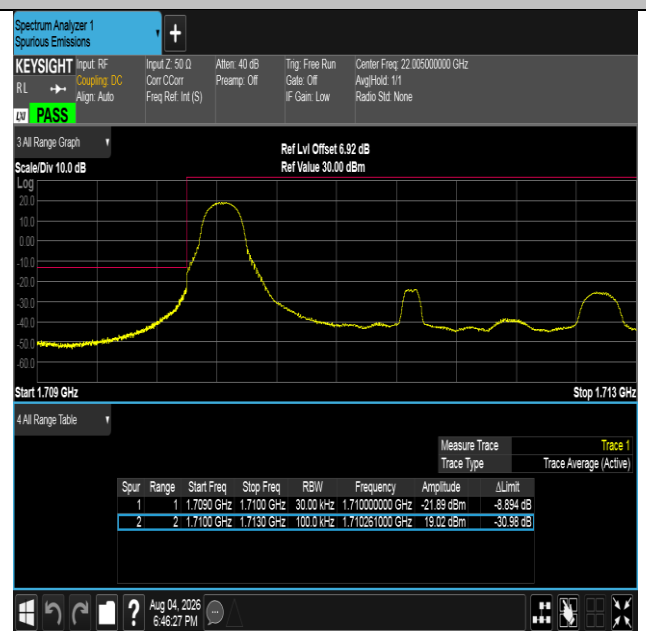
Band4-3MHz-16QAM-19965-1RB#0-PASS
