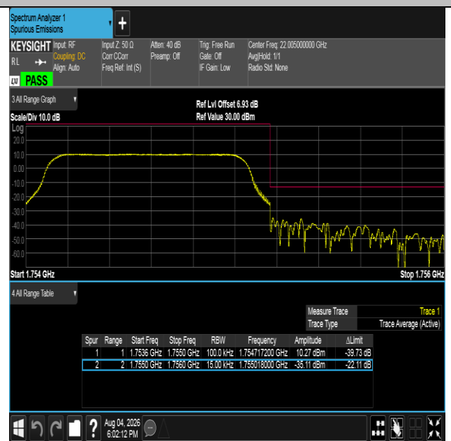
Band4-1.4MHz-16QAM-20393-6RB#0-PASS
