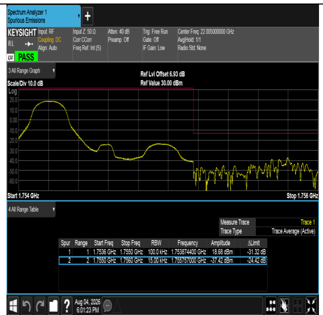
Band4-1.4MHz-16QAM-20393-1RB#0-PASS
