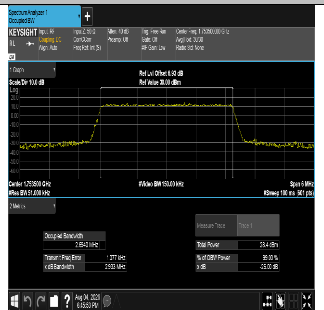
Band4-3MHz-16QAM-20385-15RB#0-PASS
