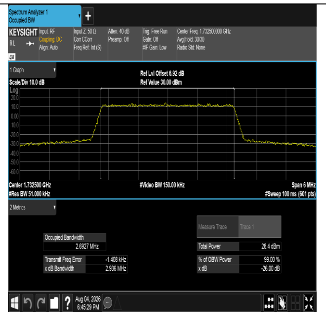
Band4-3MHz-16QAM-20175-15RB#0-PASS
