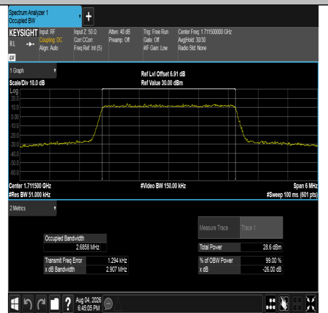
Band4-3MHz-16QAM-19965-15RB#0-PASS
