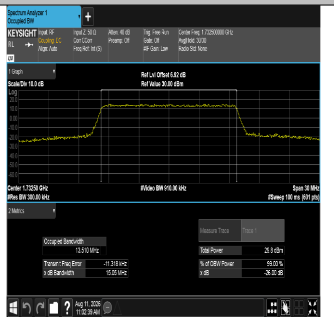
Band4-15MHz-16QAM-20175-75RB#0-PASS
