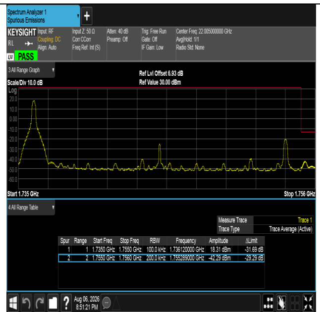
Band4-20MHz-16QAM-20300-1RB#0-PASS
