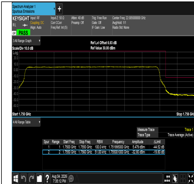
Band4-5MHz-QPSK-20375-25RB#0-PASS
