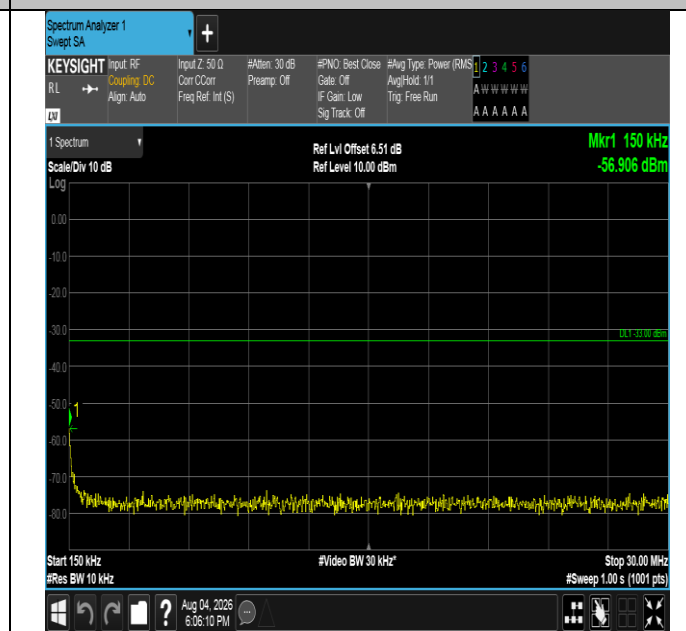
Band4-1.4MHz-QPSK-19957-6RB#0-0.15~30-PASS
