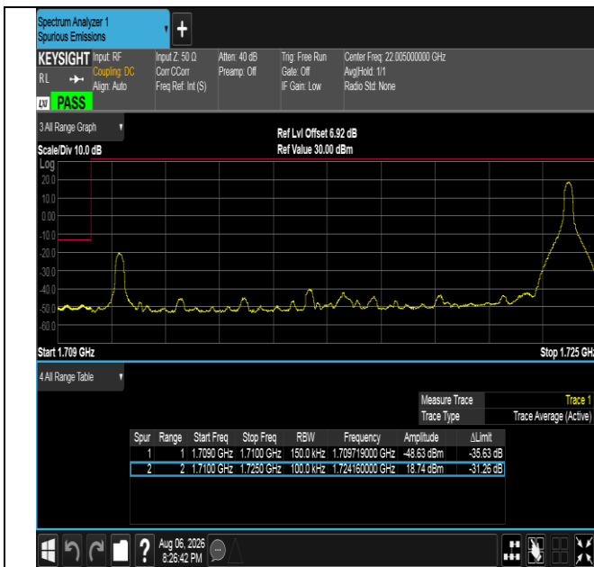
Band4-15MHz-16QAM-20025-1RB#74-PASS
