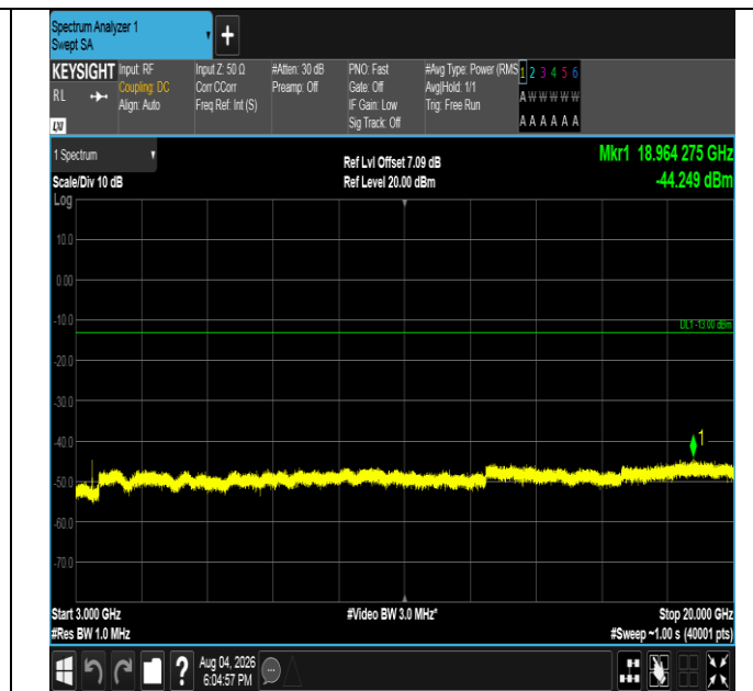
Band4-1.4MHz-QPSK-19957-1RB#5-3000~20000-PASS
