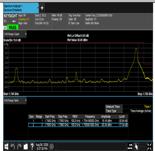
Band4-15MHz-QPSK-20325-1RB#74-PASS
