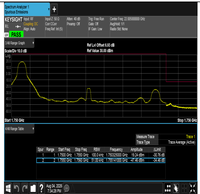
Band4-5MHz-16QAM-20375-1RB#0-PASS
