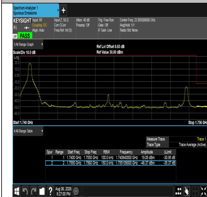
Band4-15MHz-QPSK-20325-1RB#0-PASS
