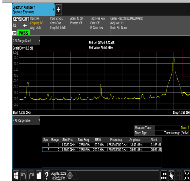
Band4-20MHz-16QAM-20300-1RB#99-PASS
