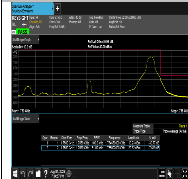
Band4-5MHz-16QAM-20375-1RB#24-PASS
