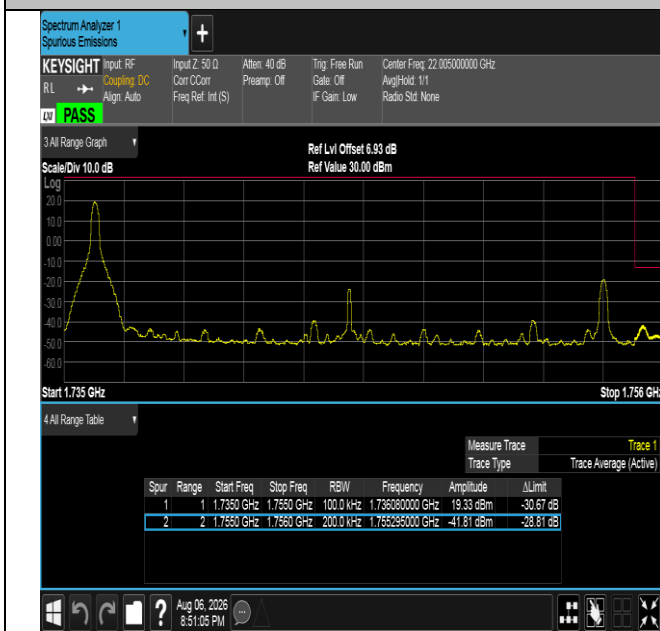
Band4-20MHz-QPSK-20300-1RB#0-PASS
