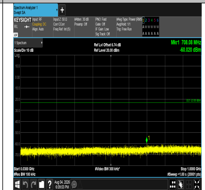
Band4-1.4MHz-16QAM-20175-1RB#0-30~1000-PASS
