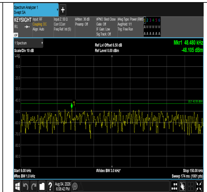
Band4-1.4MHz-16QAM-20175-1RB#0-0.009~0.15-PASS
