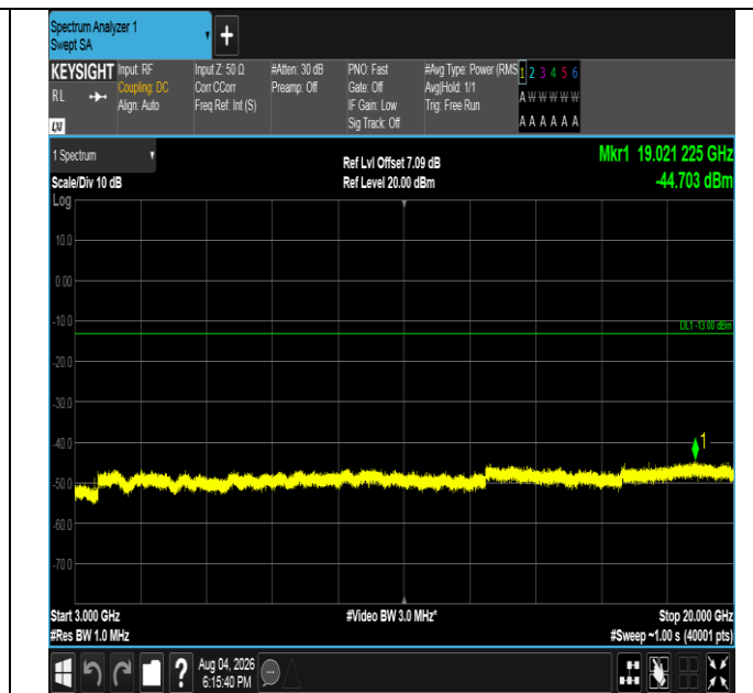
Band4-1.4MHz-QPSK-20393-1RB#5-3000~20000-PASS
