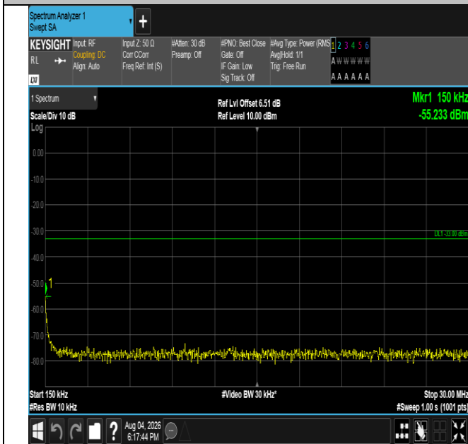
Band4-1.4MHz-16QAM-20393-6RB#0-0.15~30-PASS
