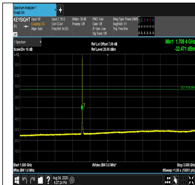
Band4-1.4MHz-16QAM-19957-6RB#0-1000~3000-PASS
