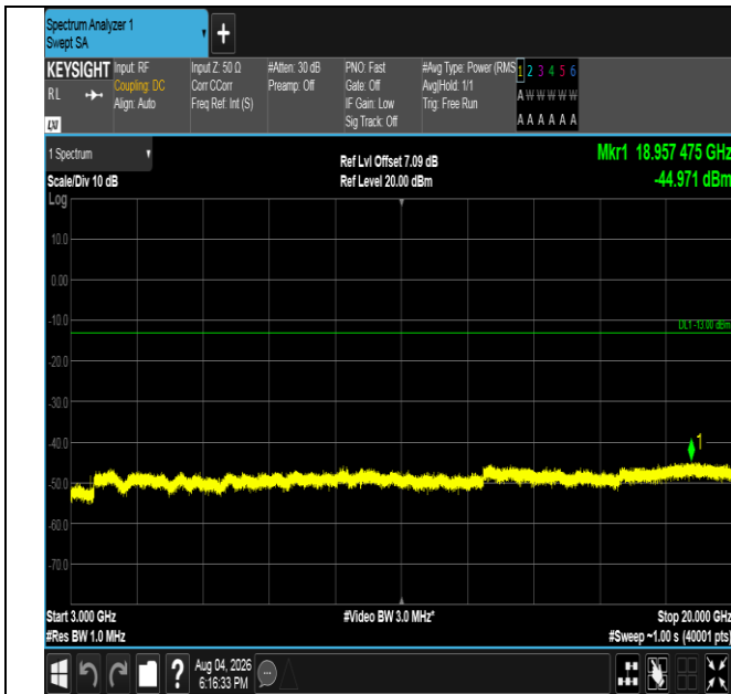
Band4-1.4MHz-16QAM-20393-1RB#5-3000~20000-PASS
