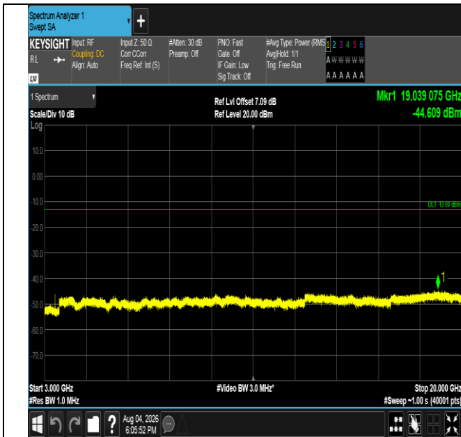
Band4-1.4MHz-16QAM-19957-1RB#5-3000~20000-PASS
