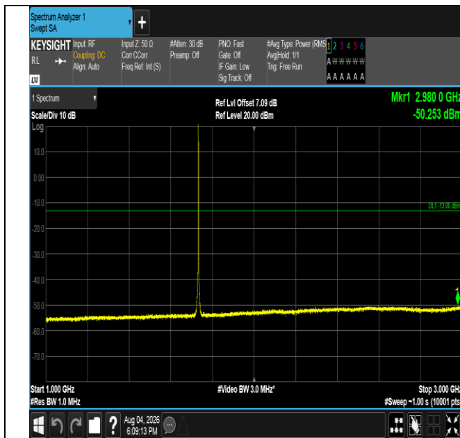
Band4-1.4MHz-16QAM-20175-1RB#0-1000~3000-PASS
