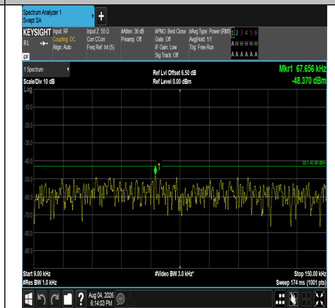
Band4-1.4MHz-16QAM-20393-1RB#0-0.009~0.15-PASS
