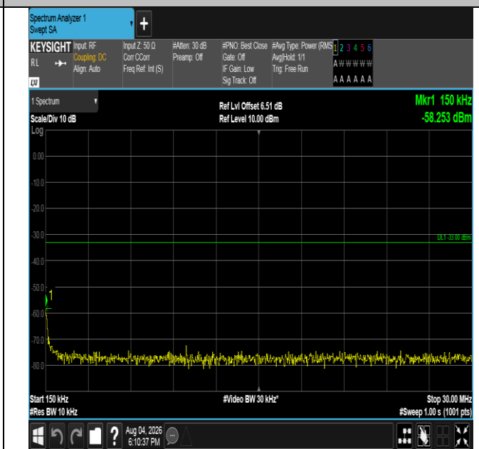
Band4-1.4MHz-16QAM-20175-1RB#5-0.15~30-PASS
