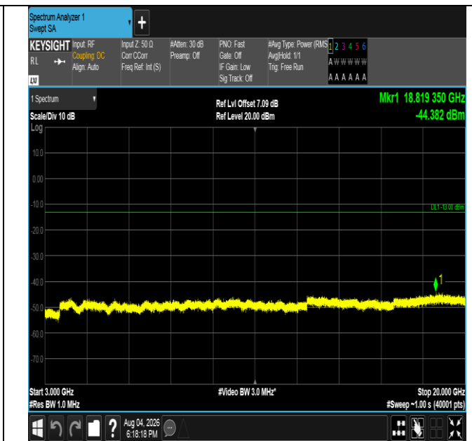
Band4-1.4MHz-16QAM-20393-6RB#0-3000~20000-PASS
