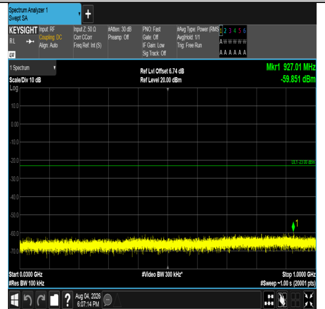
Band4-1.4MHz-16QAM-19957-6RB#0-30~1000-PASS
