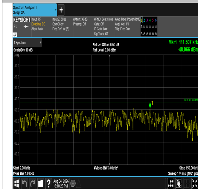
Band4-1.4MHz-16QAM-20175-1RB#5-0.009~0.15-PASS
