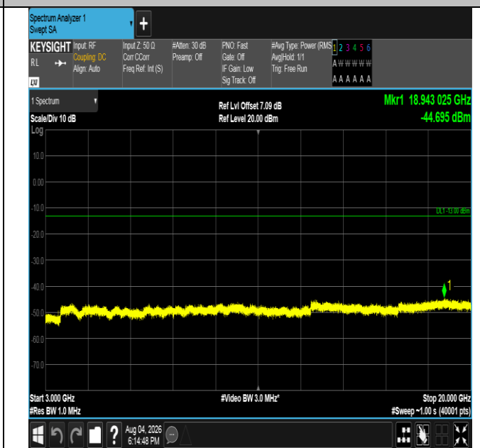
Band4-1.4MHz-16QAM-20393-1RB#0-3000~20000-PASS
