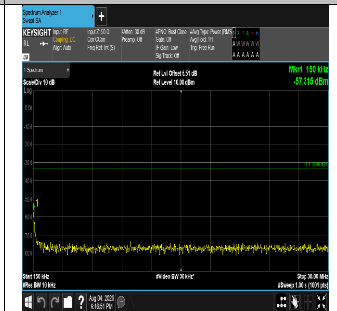
Band4-1.4MHz-QPSK-20393-6RB#0-0.15~30-PASS
