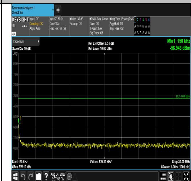
Band4-1.4MHz-QPSK-20175-1RB#0-0.15~30-PASS
