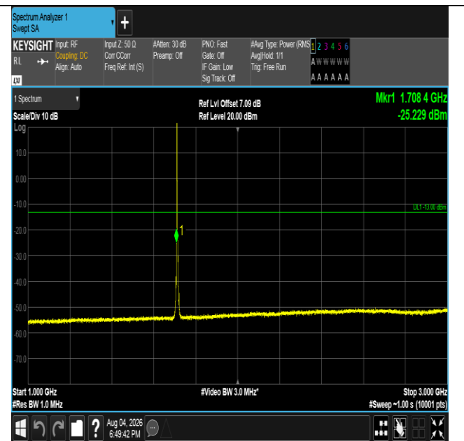
Band4-3MHz-QPSK-19965-1RB#0-1000~3000-PASS
