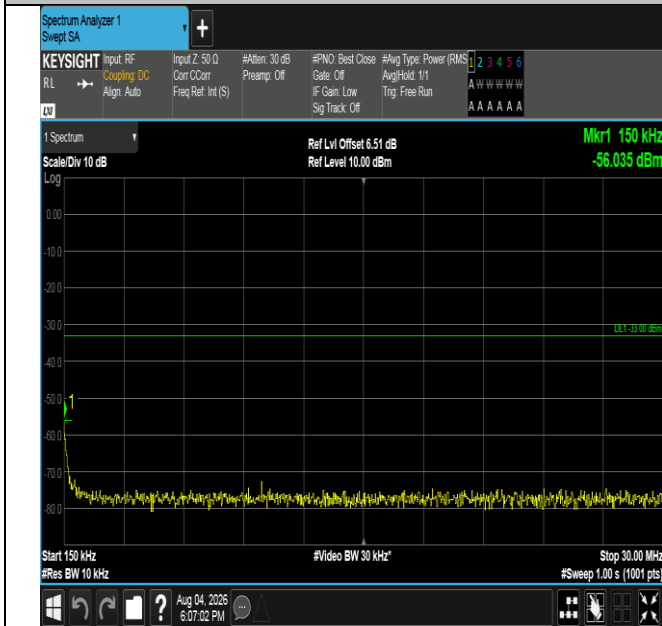
Band4-1.4MHz-16QAM-19957-6RB#0-0.15~30-PASS
