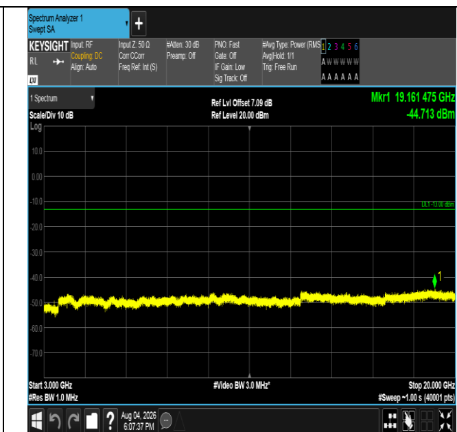
Band4-1.4MHz-16QAM-19957-6RB#0-3000~20000-PASS
