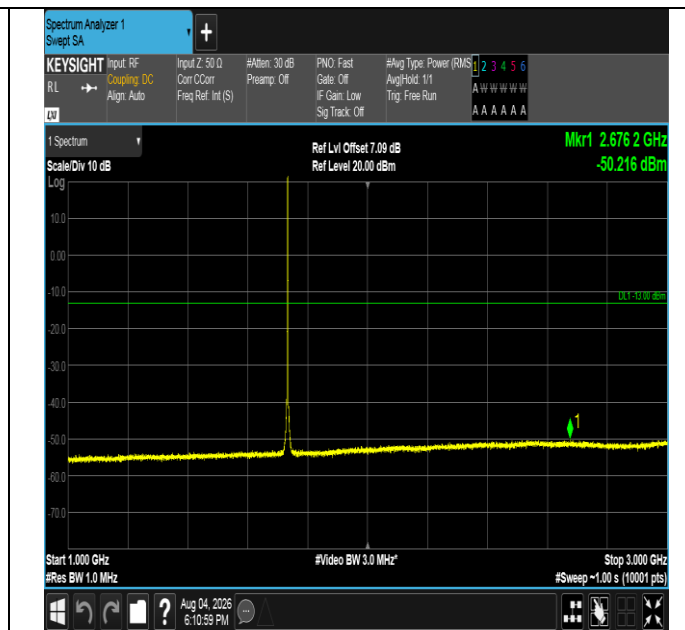
Band4-1.4MHz-16QAM-20175-1RB#5-1000~3000-PASS
