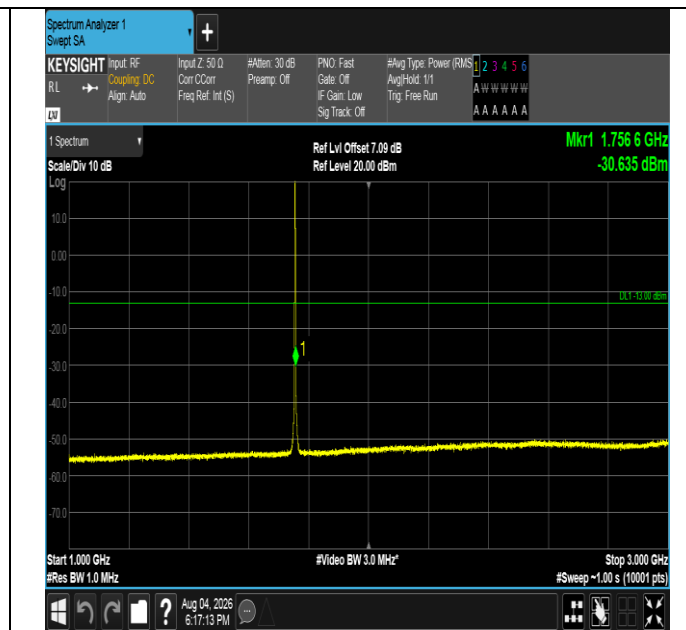
Band4-1.4MHz-QPSK-20393-6RB#0-1000~3000-PASS
