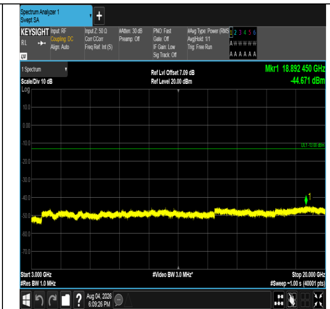
Band4-1.4MHz-16QAM-20175-1RB#0-3000~20000-PASS
