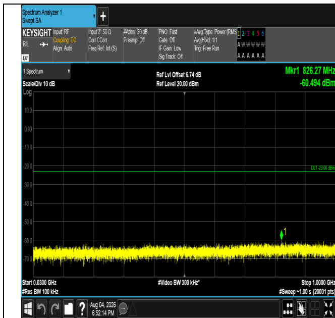
Band4-3MHz-16QAM-19965-1RB#14-30~1000-PASS
