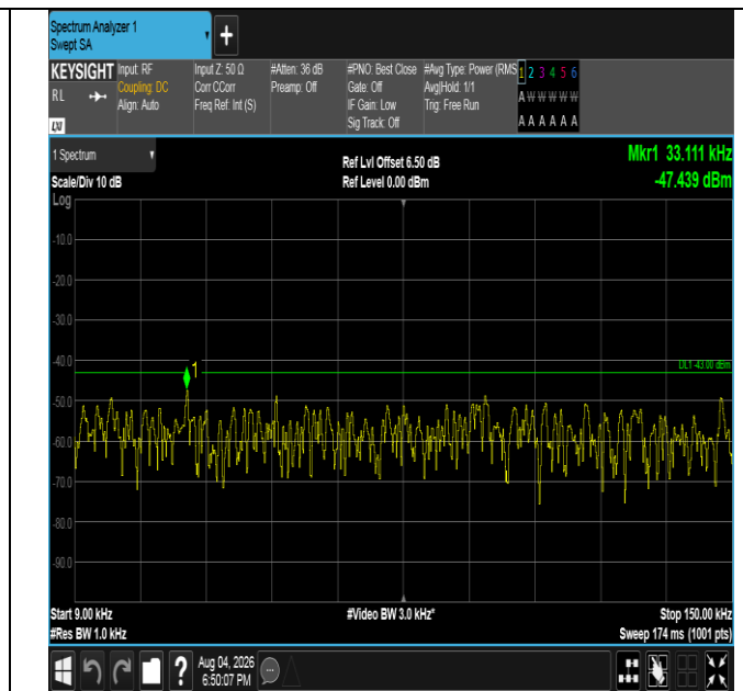
Band4-3MHz-16QAM-19965-1RB#0-0.009~0.15-PASS
