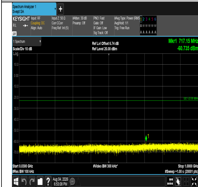
Band4-3MHz-QPSK-19965-15RB#0-30~1000-PASS
