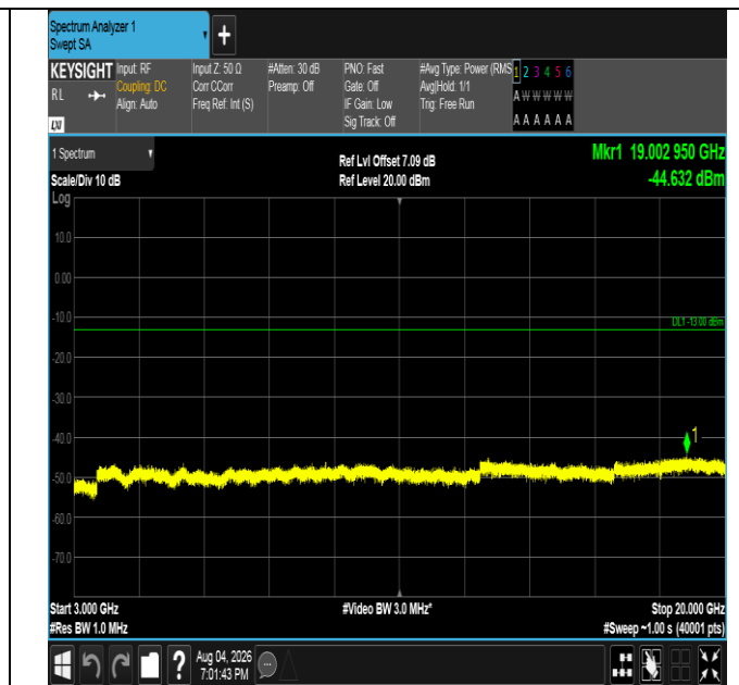
Band4-3MHz-16QAM-20385-1RB#0-3000~20000-PASS
