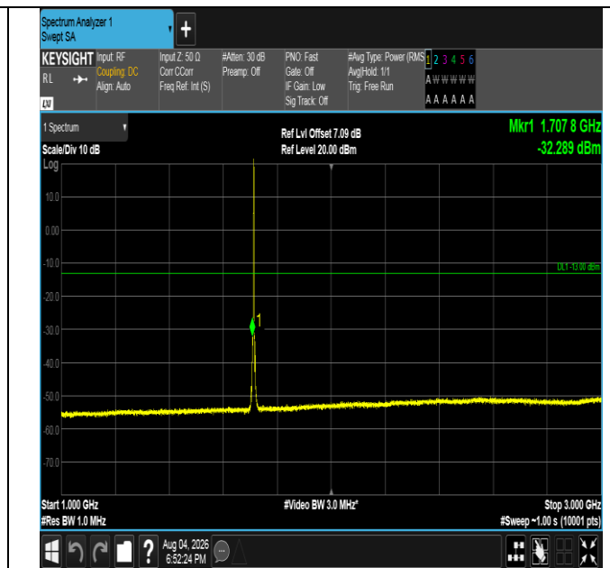
Band4-3MHz-16QAM-19965-1RB#14-1000~3000-PASS
