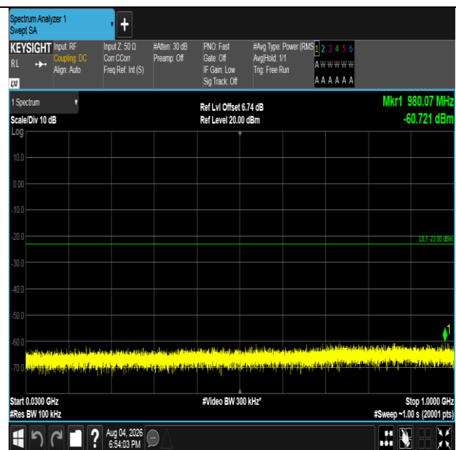
Band4-3MHz-16QAM-19965-15RB#0-30~1000-PASS
