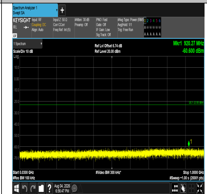
Band4-3MHz-QPSK-20175-1RB#14-30~1000-PASS
