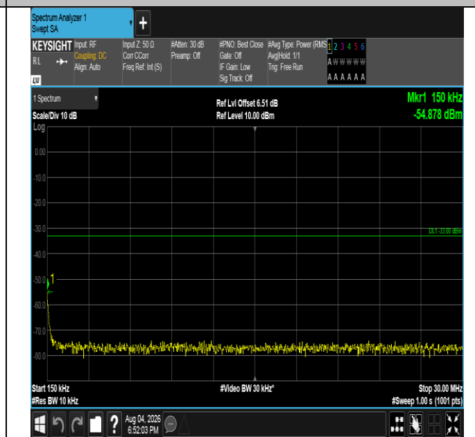
Band4-3MHz-16QAM-19965-1RB#14-0.15~30-PASS
