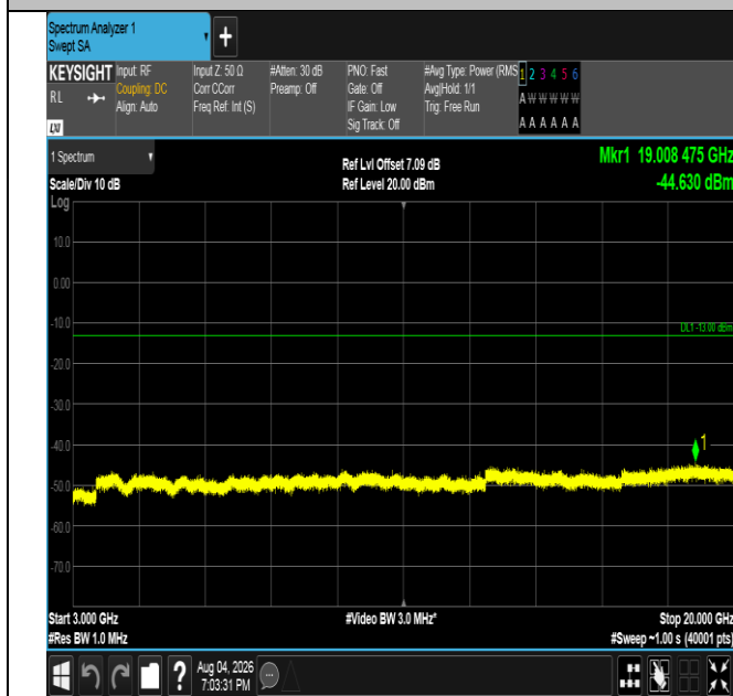
Band4-3MHz-16QAM-20385-1RB#14-3000~20000-PASS
