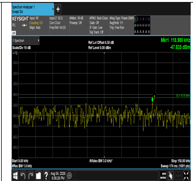
Band4-3MHz-QPSK-20175-1RB#14-0.009~0.15-PASS
