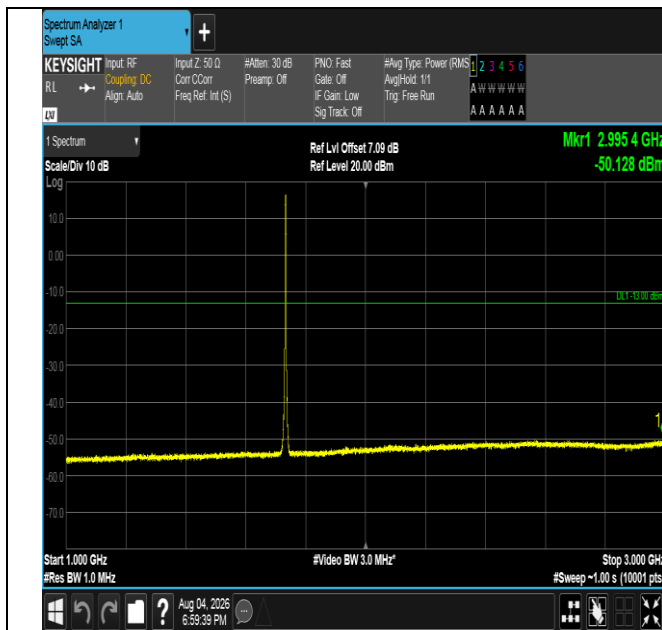
Band4-3MHz-16QAM-20175-15RB#0-1000~3000-PASS
