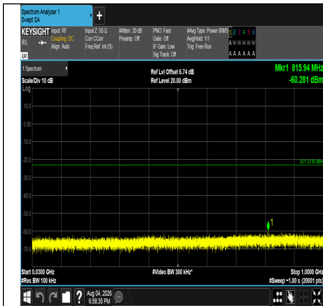
Band4-3MHz-QPSK-20175-15RB#0-30~1000-PASS
