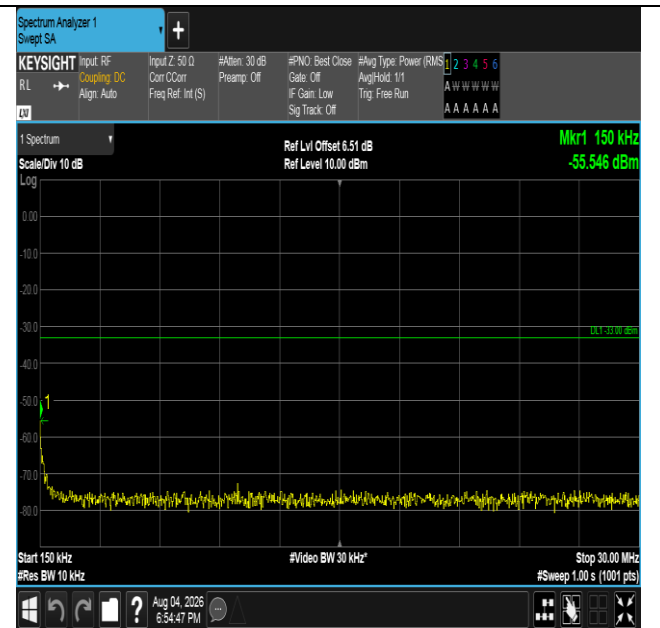
Band4-3MHz-QPSK-20175-1RB#0-0.15~30-PASS
