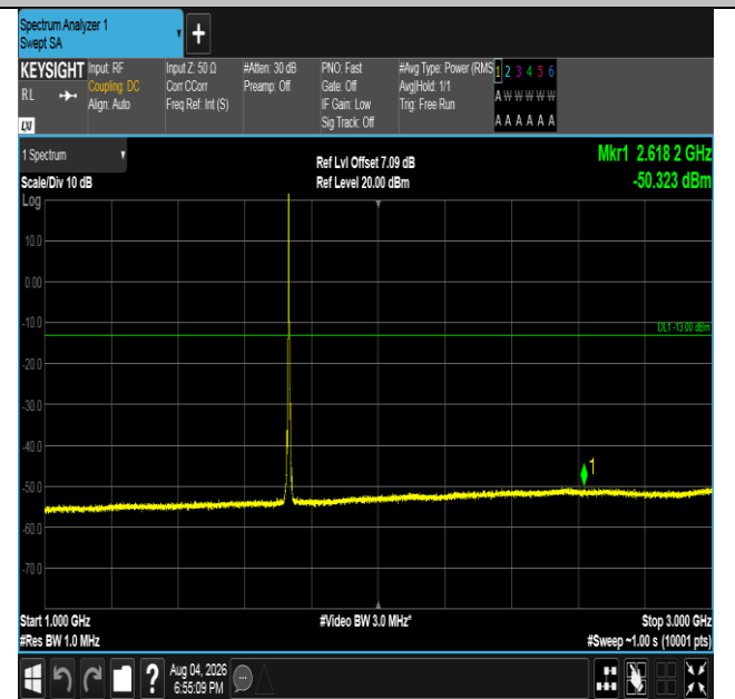
Band4-3MHz-QPSK-20175-1RB#0-1000~3000-PASS
