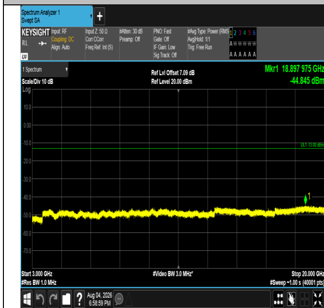
Band4-3MHz-QPSK-20175-15RB#0-3000~20000-PASS
