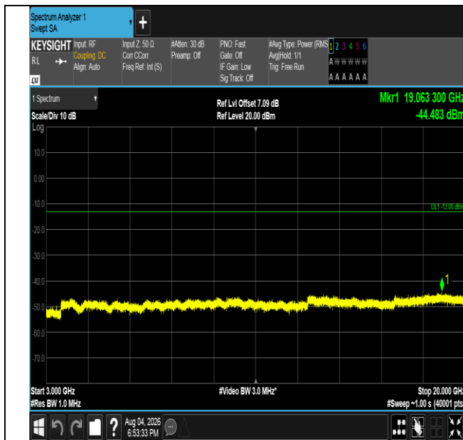
Band4-3MHz-QPSK-19965-15RB#0-3000~20000-PASS
