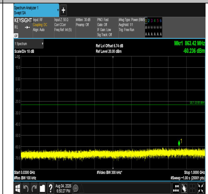
Band4-3MHz-16QAM-19965-1RB#0-30~1000-PASS
