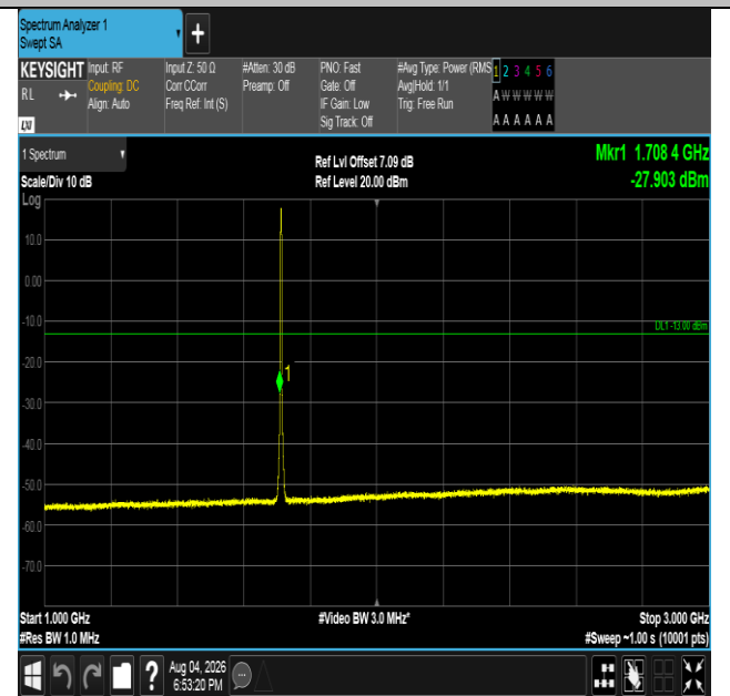
Band4-3MHz-QPSK-19965-15RB#0-1000~3000-PASS
