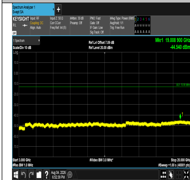
Band4-3MHz-16QAM-19965-1RB#14-3000~20000-PASS
