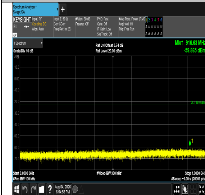
Band4-3MHz-QPSK-20175-1RB#0-30~1000-PASS
