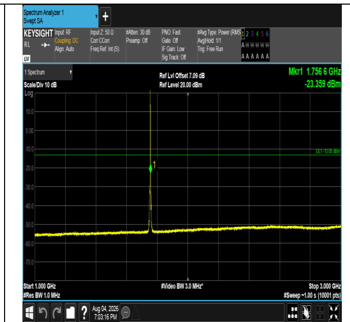
Band4-3MHz-16QAM-20385-1RB#14-1000~3000-PASS
