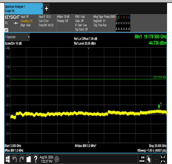
Band4-3MHz-QPSK-20385-1RB#14-3000~20000-PASS
