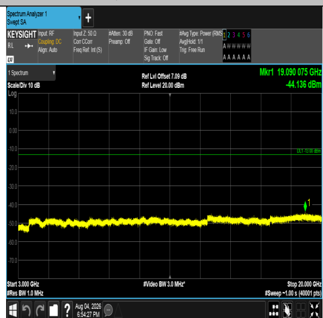
Band4-3MHz-16QAM-19965-15RB#0-3000~20000-PASS
