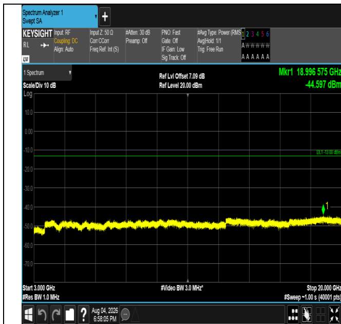
Band4-3MHz-16QAM-20175-1RB#14-3000~20000-PASS
