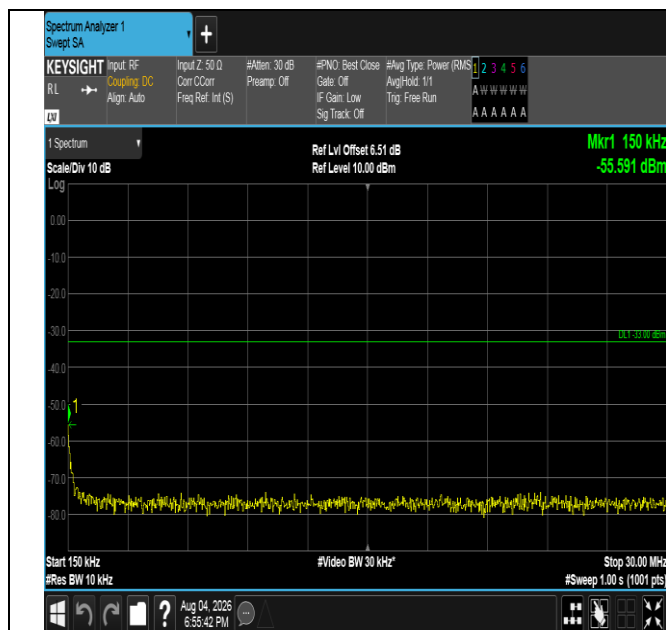
Band4-3MHz-16QAM-20175-1RB#0-0.15~30-PASS
