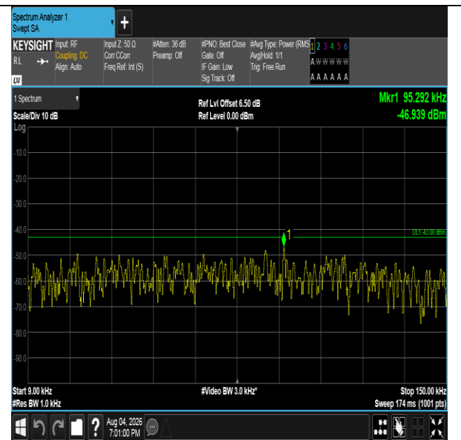
Band4-3MHz-16QAM-20385-1RB#0-0.009~0.15-PASS
