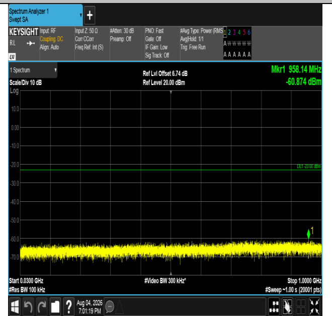
Band4-3MHz-16QAM-20385-1RB#0-30~1000-PASS
