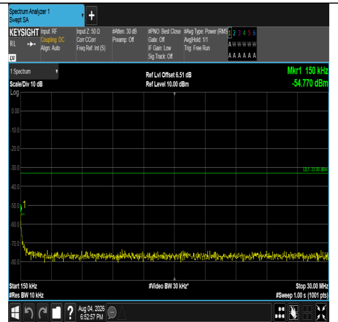
Band4-3MHz-QPSK-19965-15RB#0-0.15~30-PASS
