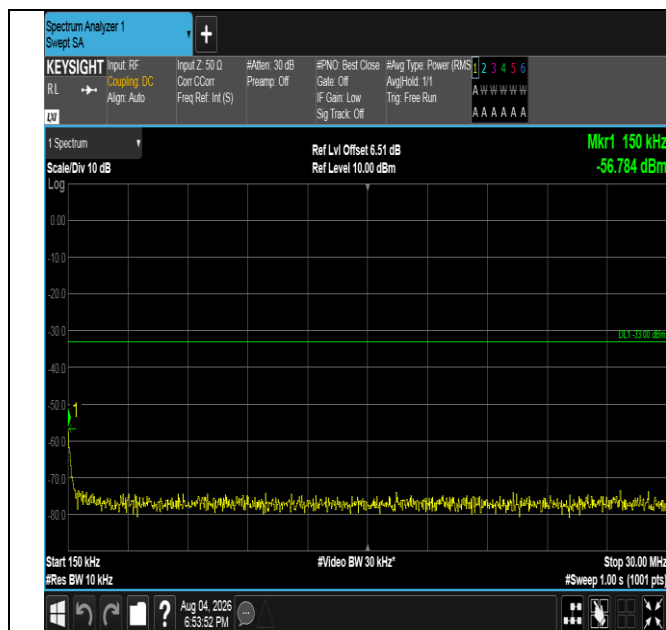
Band4-3MHz-16QAM-19965-15RB#0-0.15~30-PASS
