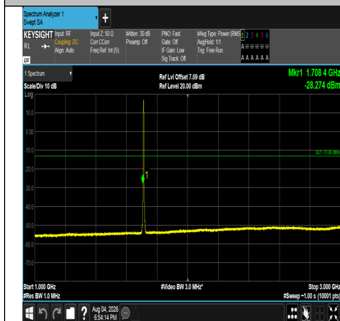
Band4-3MHz-16QAM-19965-15RB#0-1000~3000-PASS
