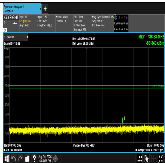
Band4-3MHz-16QAM-20175-1RB#0-30~1000-PASS
