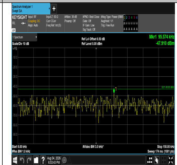
Band4-3MHz-16QAM-19965-15RB#0-0.009~0.15-PASS
