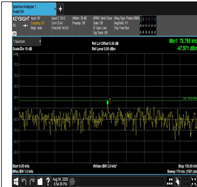
Band4-3MHz-QPSK-20175-1RB#0-0.009~0.15-PASS
