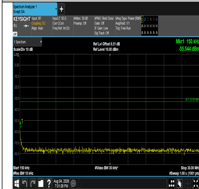
Band4-3MHz-16QAM-20385-1RB#0-0.15~30-PASS
