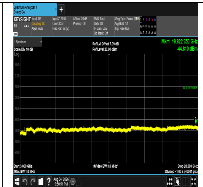
Band4-3MHz-16QAM-19965-1RB#0-3000~20000-PASS
