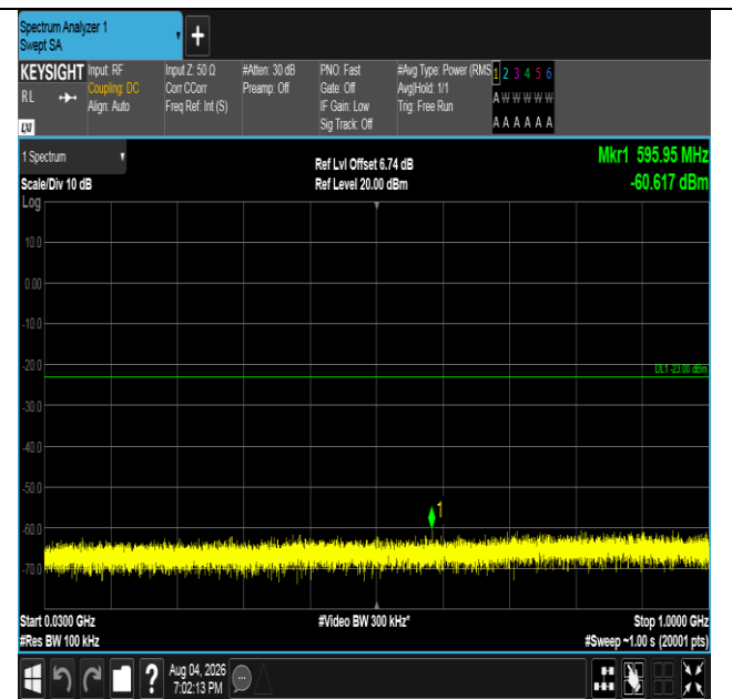
Band4-3MHz-QPSK-20385-1RB#14-30~1000-PASS
