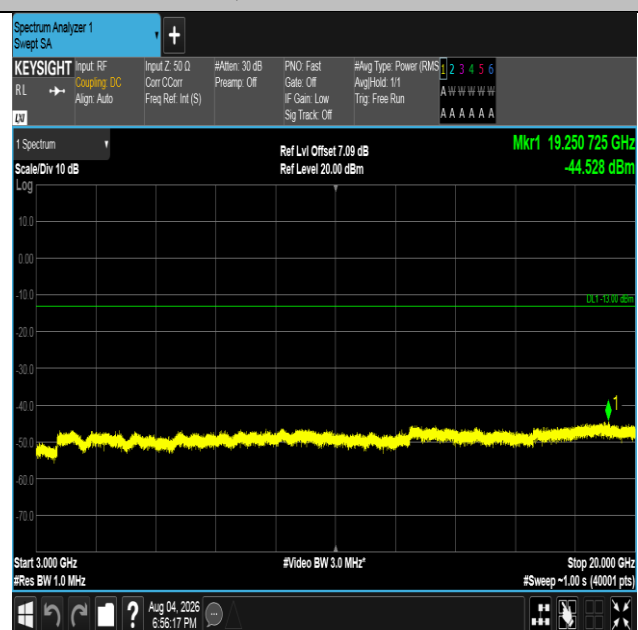
Band4-3MHz-16QAM-20175-1RB#0-3000~20000-PASS
