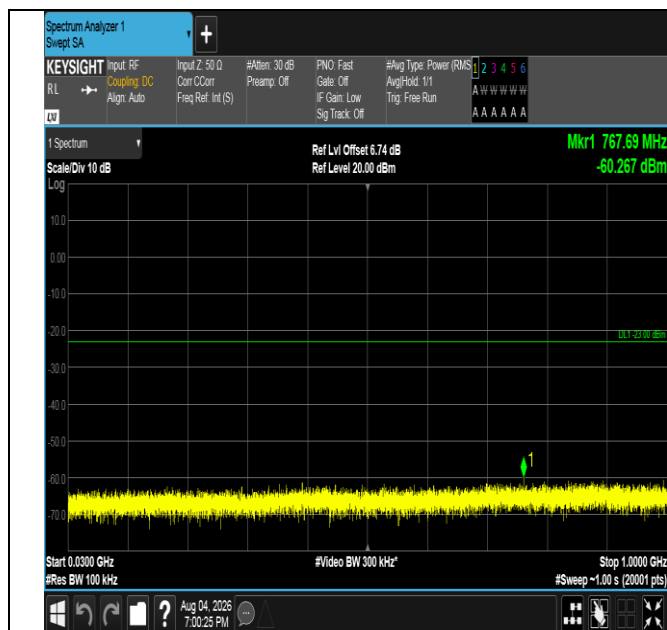
Band4-3MHz-QPSK-20385-1RB#0-30~1000-PASS
