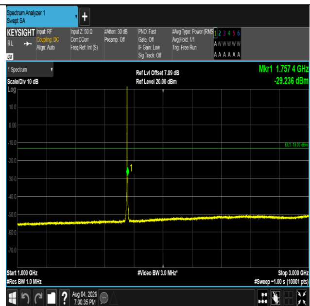
Band4-3MHz-QPSK-20385-1RB#0-1000~3000-PASS
