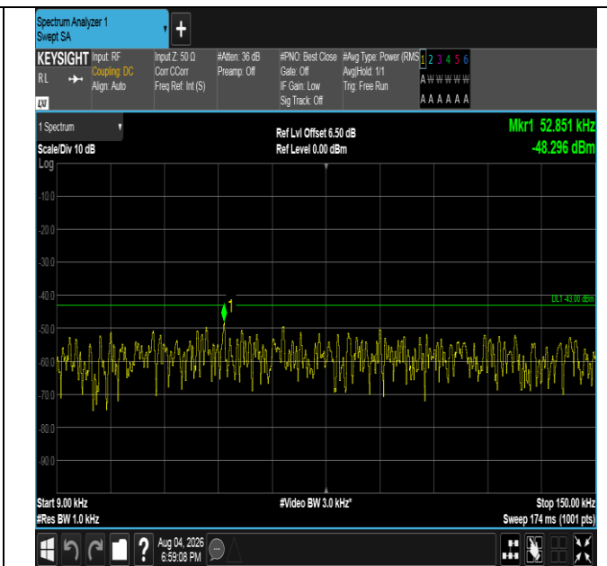
Band4-3MHz-16QAM-20175-15RB#0-0.009~0.15-PASS
