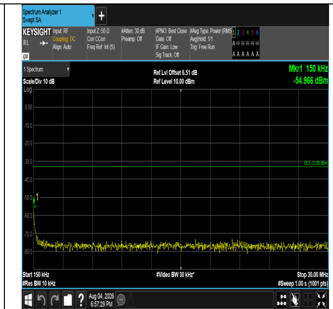
Band4-3MHz-16QAM-20175-1RB#14-0.15~30-PASS
