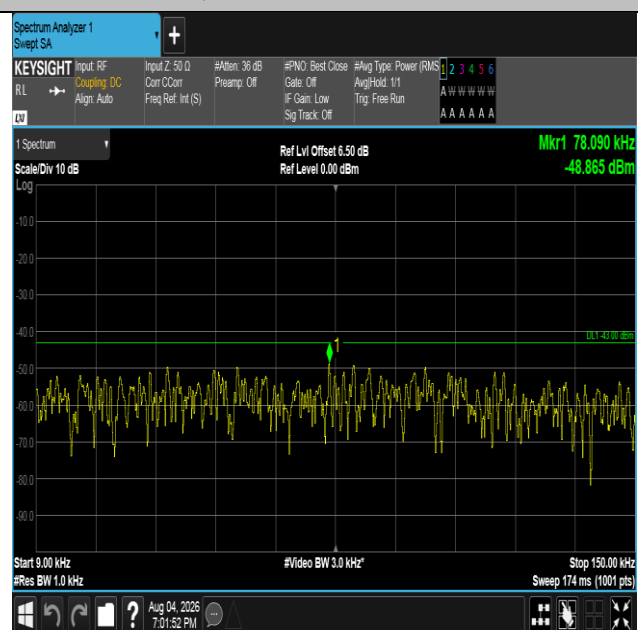
Band4-3MHz-QPSK-20385-1RB#14-0.009~0.15-PASS
