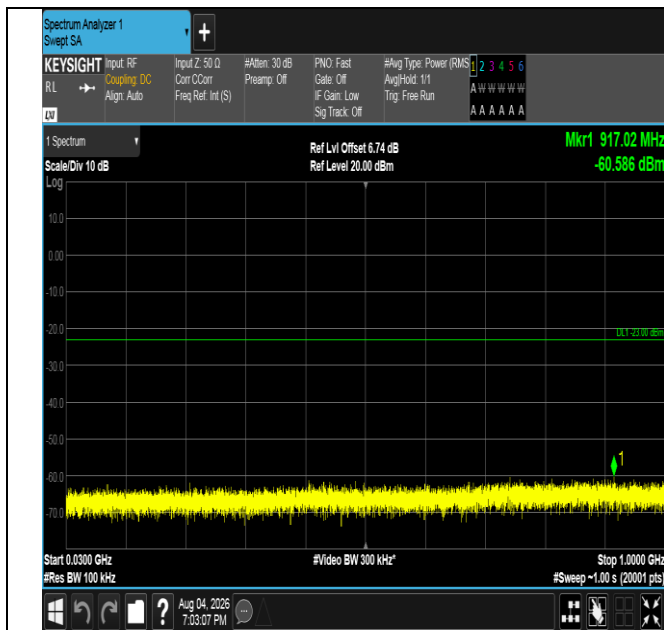
Band4-3MHz-16QAM-20385-1RB#14-30~1000-PASS
