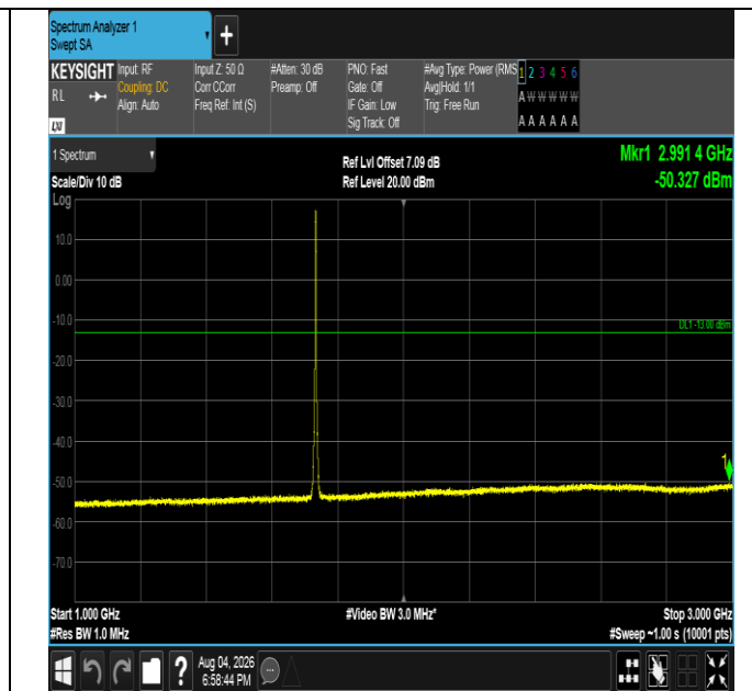
Band4-3MHz-QPSK-20175-15RB#0-1000~3000-PASS
