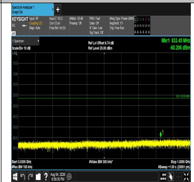
Band4-3MHz-16QAM-20175-15RB#0-30~1000-PASS
