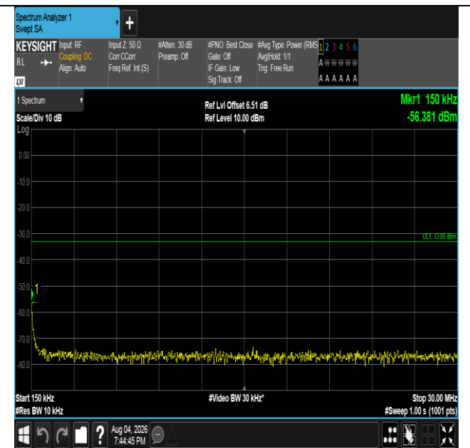
Band4-5MHz-QPSK-20175-25RB#0-0.15~30-PASS
