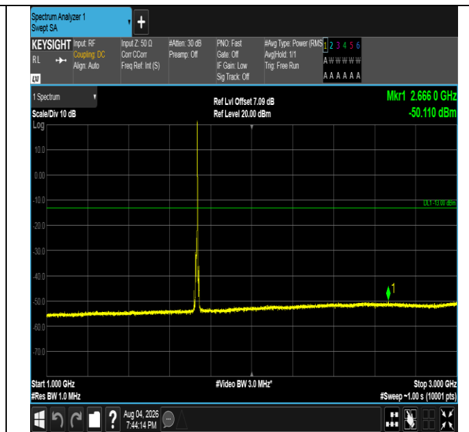
Band4-5MHz-16QAM-20175-1RB#24-1000~3000-PASS
