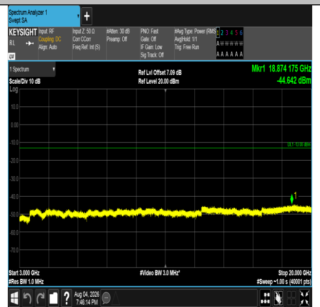
Band4-5MHz-16QAM-20175-25RB#0-3000~20000-PASS
