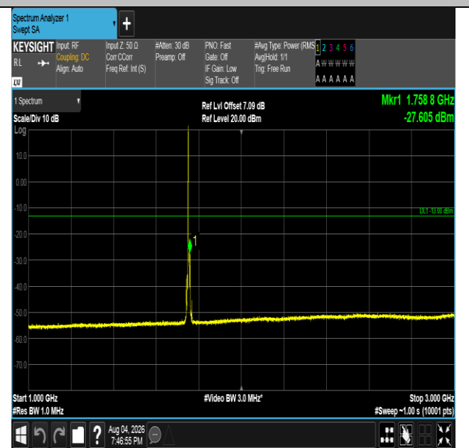
Band4-5MHz-QPSK-20375-1RB#0-1000~3000-PASS
