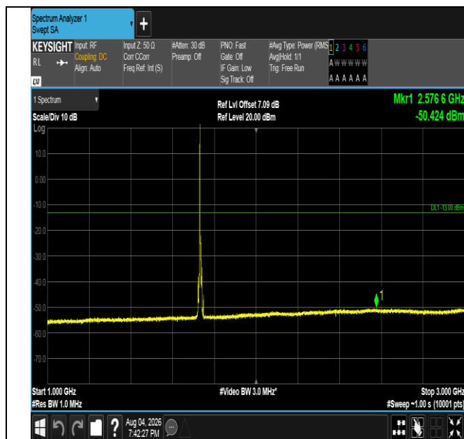
Band4-5MHz-16QAM-20175-1RB#0-1000~3000-PASS
