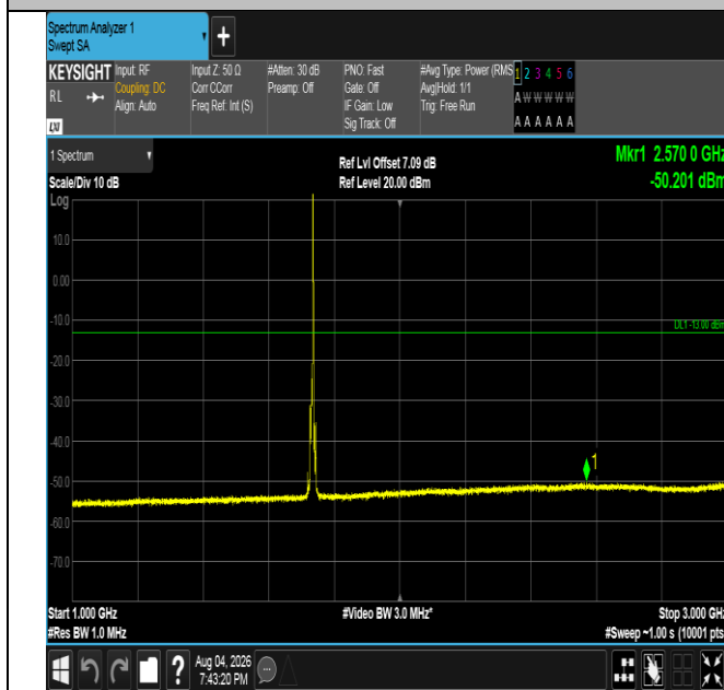
Band4-5MHz-QPSK-20175-1RB#24-1000~3000-PASS
