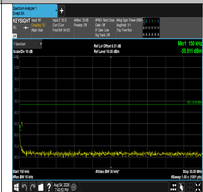
Band4-5MHz-16QAM-20175-1RB#24-0.15~30-PASS
