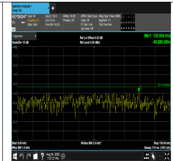
Band4-5MHz-QPSK-19975-1RB#24-0.009~0.15-PASS
