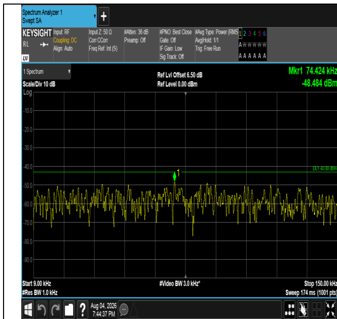
Band4-5MHz-QPSK-20175-25RB#0-0.009~0.15-PASS
