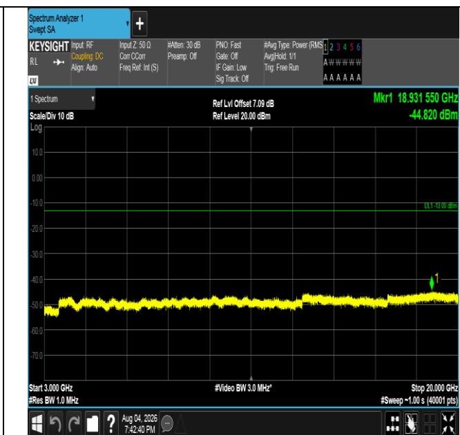
Band4-5MHz-16QAM-20175-1RB#0-3000~20000-PASS
