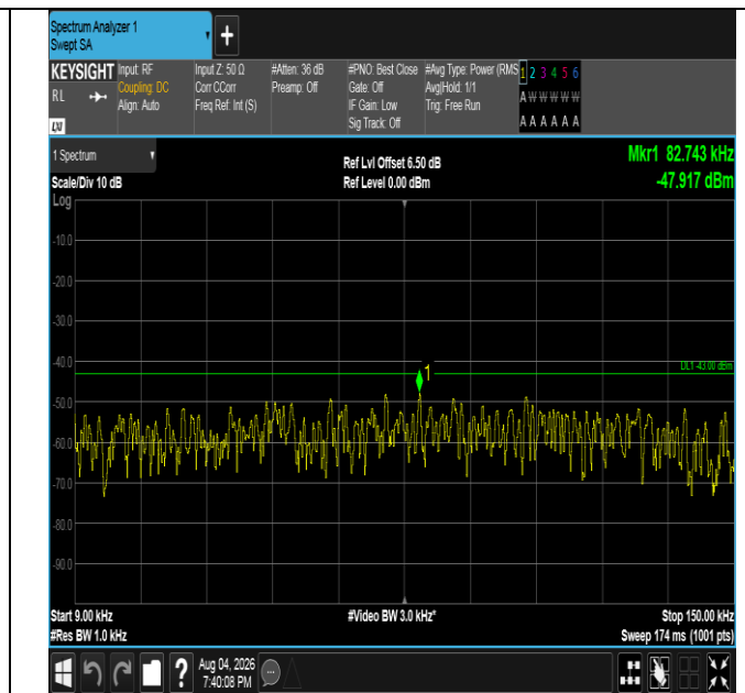
Band4-5MHz-16QAM-19975-25RB#0-0.009~0.15-PASS
