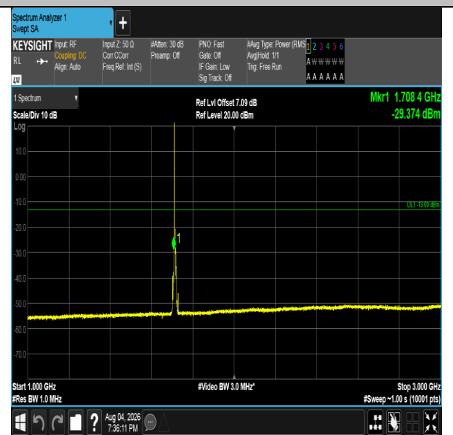
Band4-5MHz-QPSK-19975-1RB#0-1000~3000-PASS
