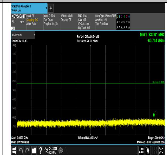
Band4-5MHz-16QAM-19975-25RB#0-30~1000-PASS
