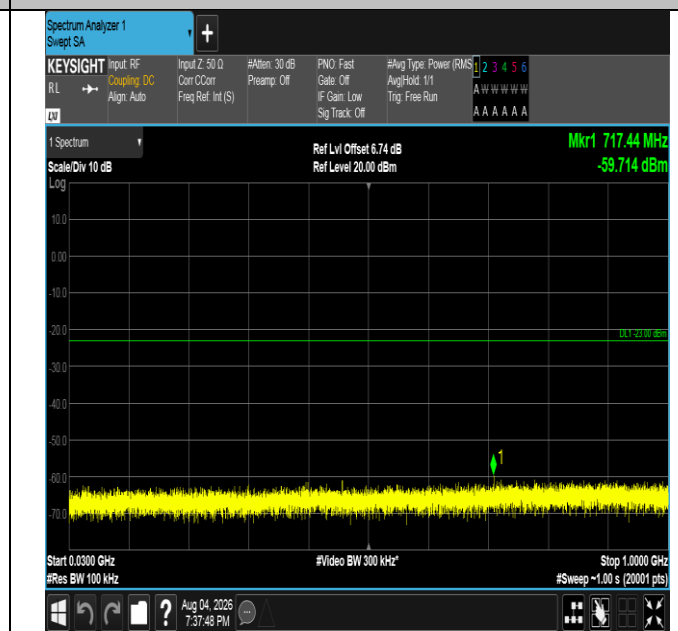
Band4-5MHz-QPSK-19975-1RB#24-30~1000-PASS
