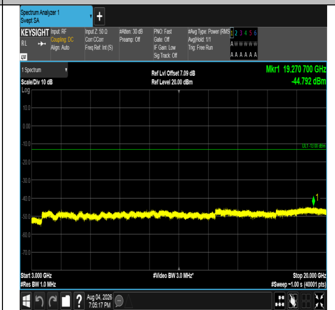
Band4-3MHz-16QAM-20385-15RB#0-3000~20000-PASS
