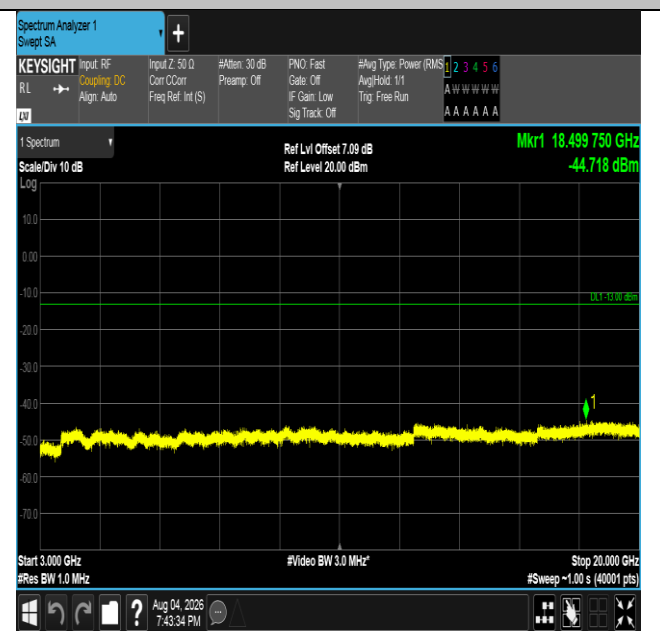
Band4-5MHz-QPSK-20175-1RB#24-3000~20000-PASS
