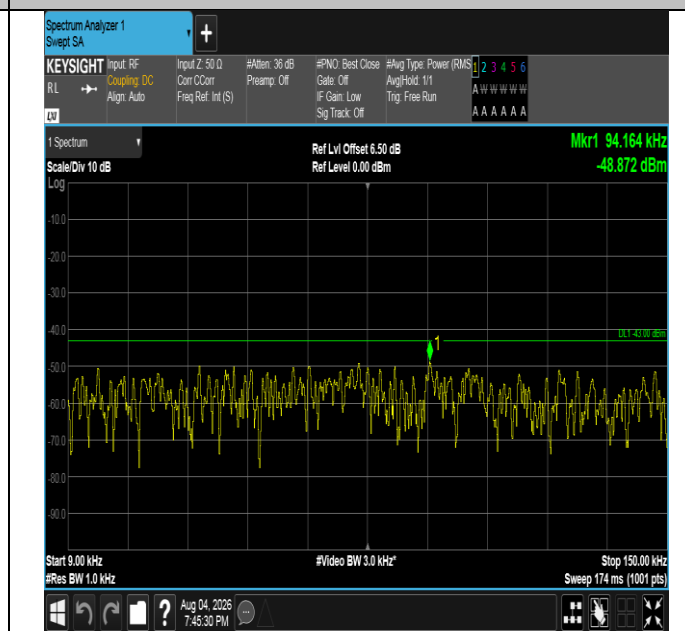
Band4-5MHz-16QAM-20175-25RB#0-0.009~0.15-PASS
