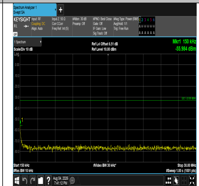
Band4-5MHz-QPSK-20175-1RB#0-0.15~30-PASS
