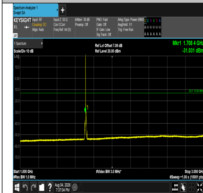
Band4-5MHz-16QAM-19975-1RB#0-1000~3000-PASS
