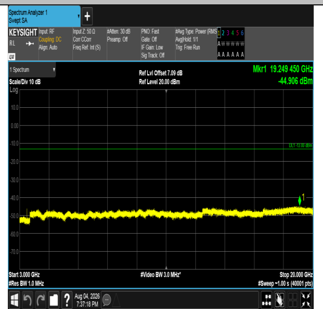
Band4-5MHz-16QAM-19975-1RB#0-3000~20000-PASS
