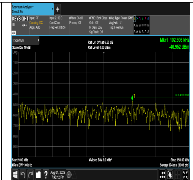
Band4-5MHz-QPSK-20375-1RB#24-0.009~0.15-PASS
