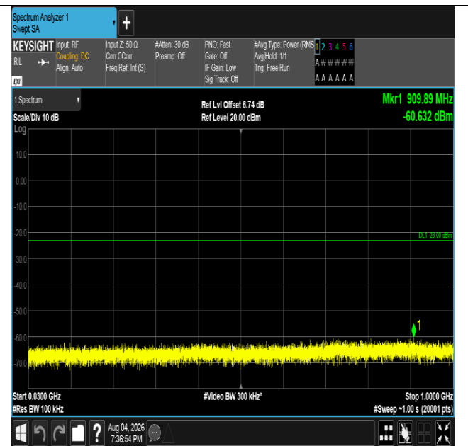
Band4-5MHz-16QAM-19975-1RB#0-30~1000-PASS
