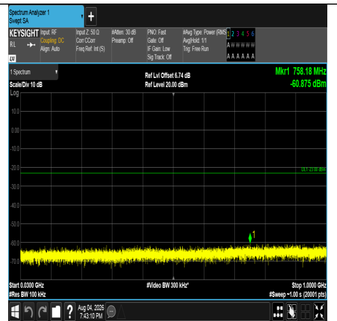
Band4-5MHz-QPSK-20175-1RB#24-30~1000-PASS
