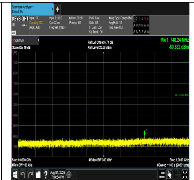
Band4-3MHz-16QAM-20385-15RB#0-30~1000-PASS
