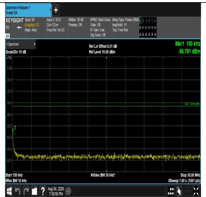
Band4-5MHz-QPSK-19975-1RB#0-0.15~30-PASS
