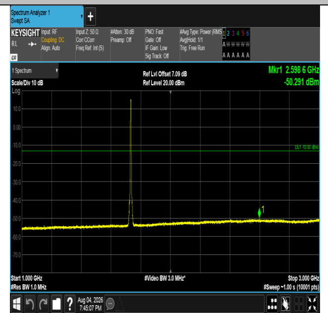
Band4-5MHz-QPSK-20175-25RB#0-1000~3000-PASS
