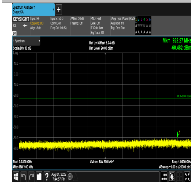
Band4-5MHz-QPSK-20175-25RB#0-30~1000-PASS
