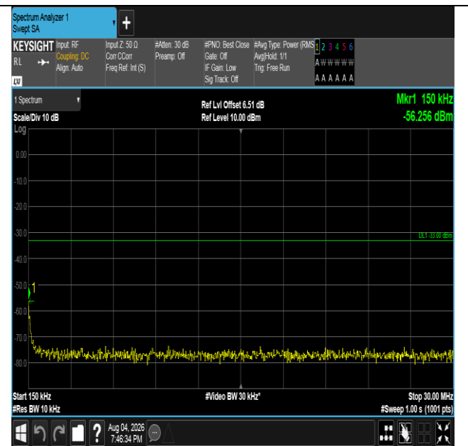
Band4-5MHz-QPSK-20375-1RB#0-0.15~30-PASS
