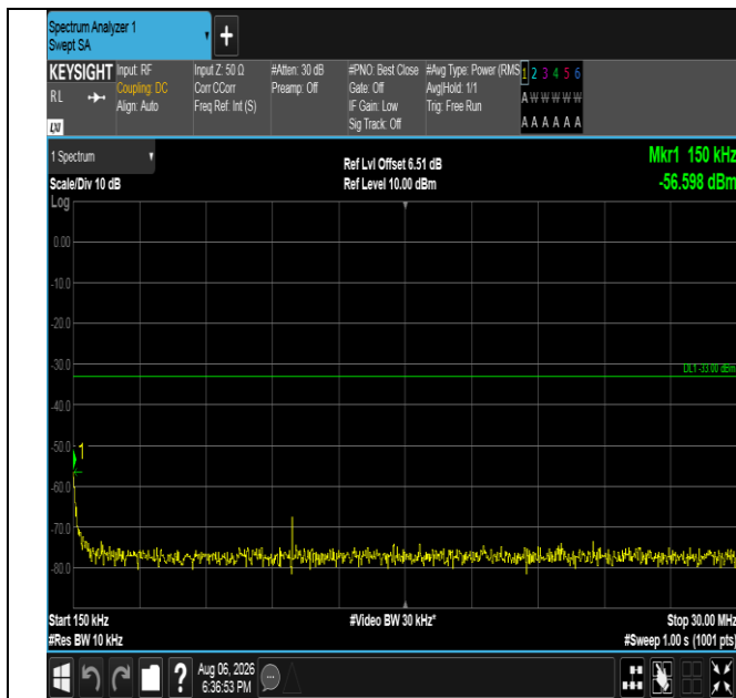
Band4-10MHz-16QAM-20175-1RB#0-0.15~30-PASS
