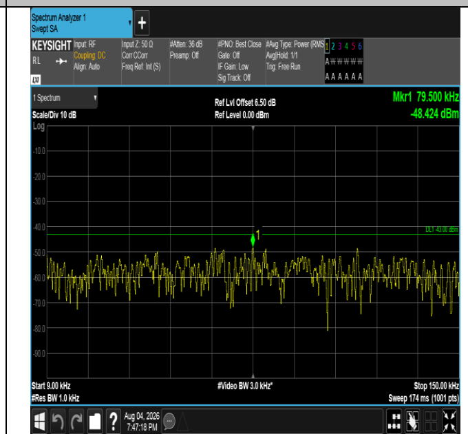
Band4-5MHz-16QAM-20375-1RB#0-0.009~0.15-PASS
