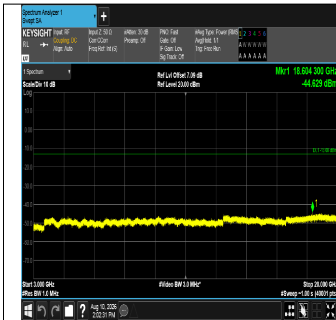
Band4-10MHz-QPSK-20000-50RB#0-3000~20000-PASS
