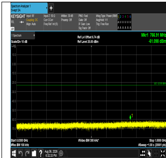
Band4-10MHz-QPSK-20000-1RB#0-30~1000-PASS
