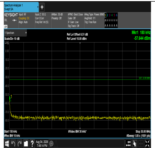
Band4-5MHz-16QAM-20375-1RB#24-0.15~30-PASS
