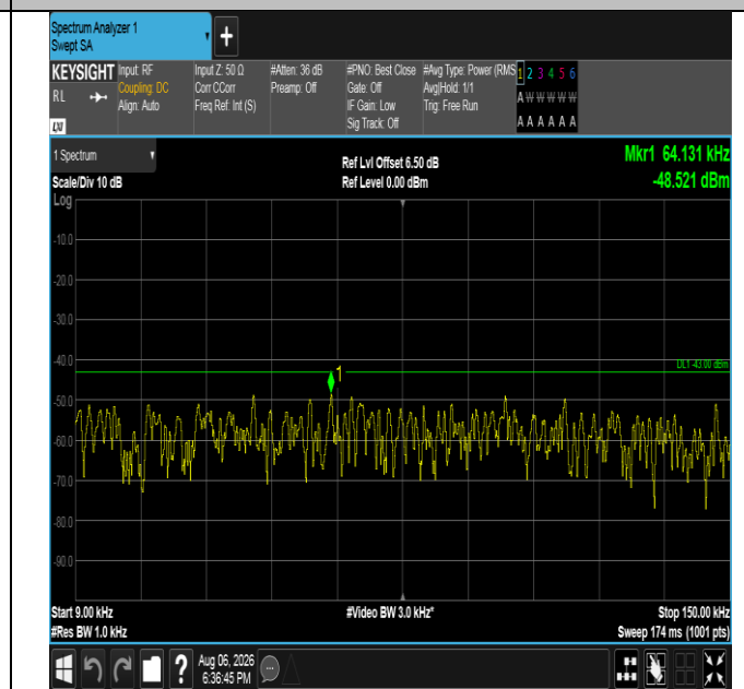
Band4-10MHz-16QAM-20175-1RB#0-0.009~0.15-PASS
