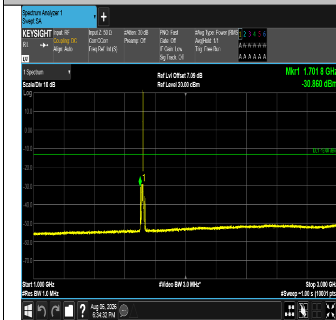
Band4-10MHz-QPSK-20000-1RB#49-1000~3000-PASS
