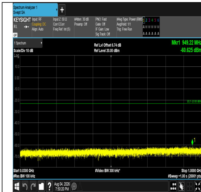
Band4-5MHz-QPSK-20375-25RB#0-30~1000-PASS
