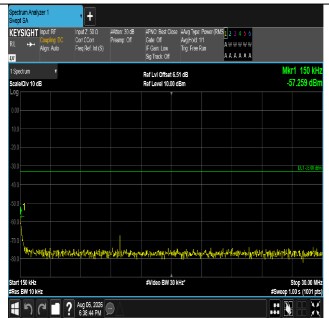
Band4-10MHz-16QAM-20175-1RB#49-0.15~30-PASS
