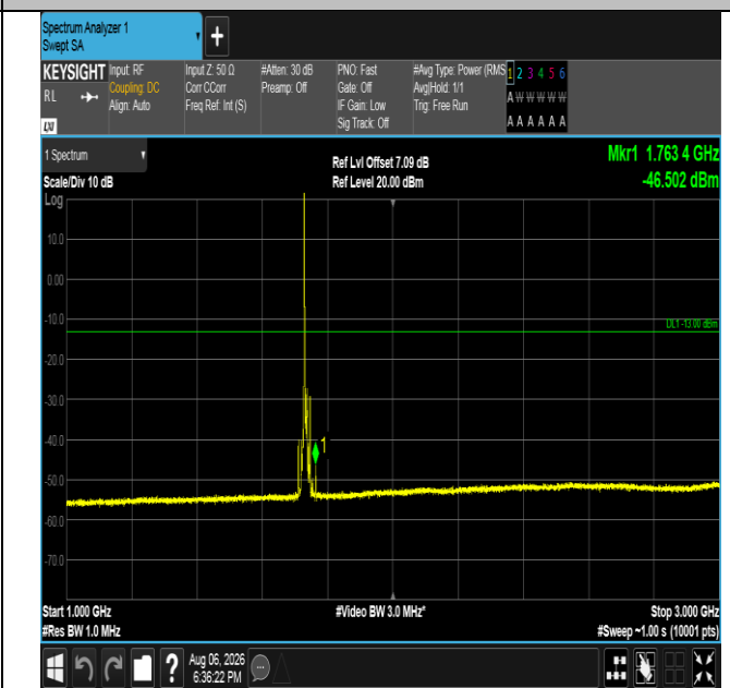
Band4-10MHz-QPSK-20175-1RB#0-1000~3000-PASS
