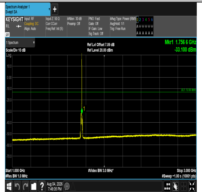
Band4-5MHz-16QAM-20375-1RB#24-1000~3000-PASS
