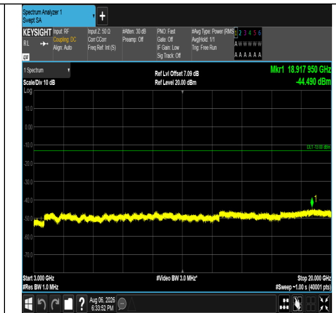
Band4-10MHz-16QAM-20000-1RB#0-3000~20000-PASS
