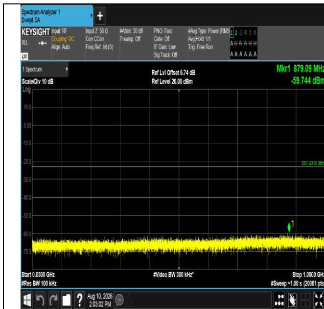
Band4-10MHz-QPSK-20175-50RB#0-30~1000-PASS
