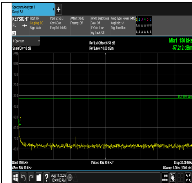
Band4-10MHz-16QAM-20000-50RB#0-0.15~30-PASS
