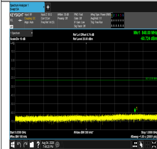
Band4-5MHz-16QAM-20375-1RB#24-30~1000-PASS
