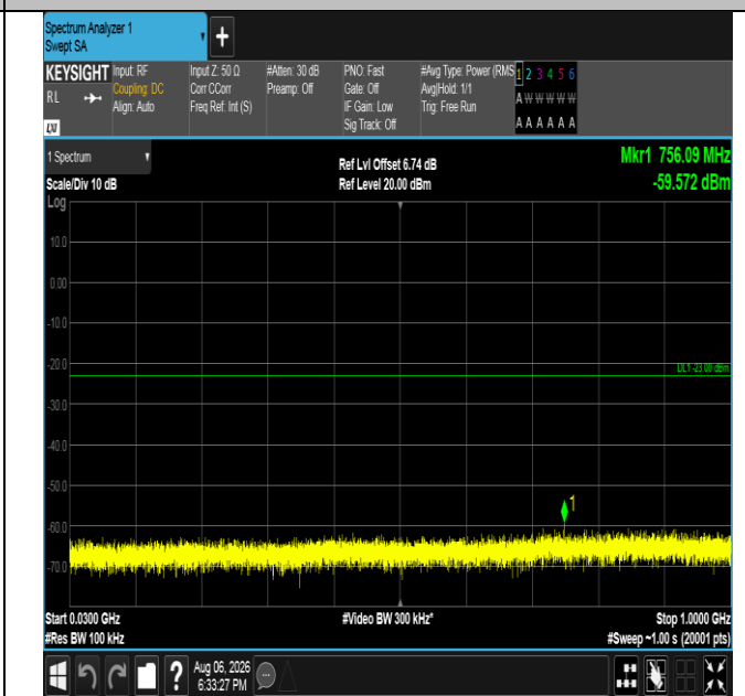
Band4-10MHz-16QAM-20000-1RB#0-30~1000-PASS
