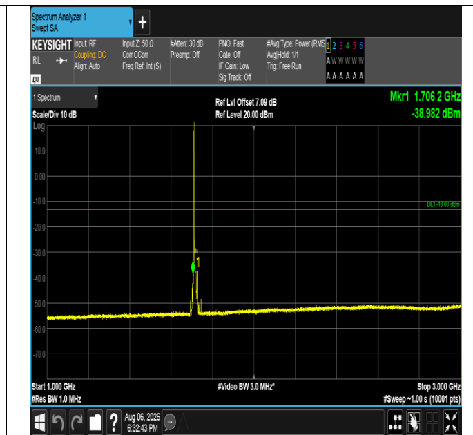
Band4-10MHz-QPSK-20000-1RB#0-1000~3000-PASS
