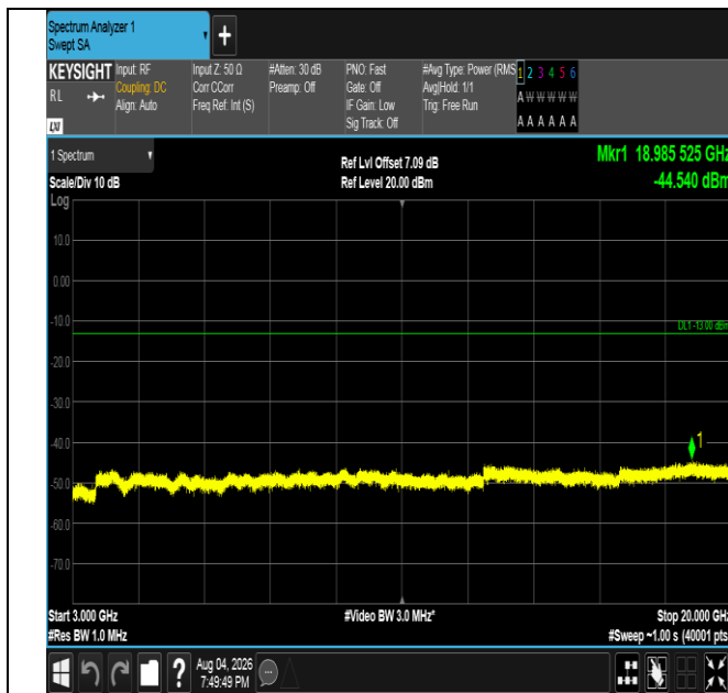
Band4-5MHz-16QAM-20375-1RB#24-3000~20000-PASS
