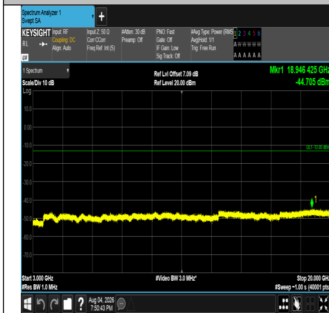
Band4-5MHz-QPSK-20375-25RB#0-3000~20000-PASS
