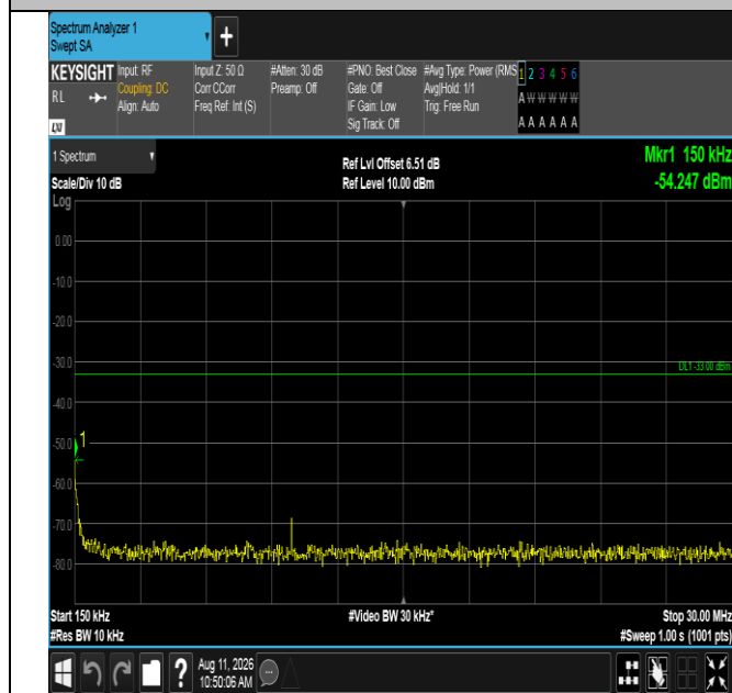
Band4-10MHz-16QAM-20175-50RB#0-0.15~30-PASS
