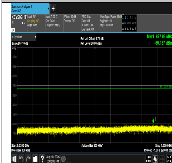
Band4-10MHz-QPSK-20000-50RB#0-30~1000-PASS
