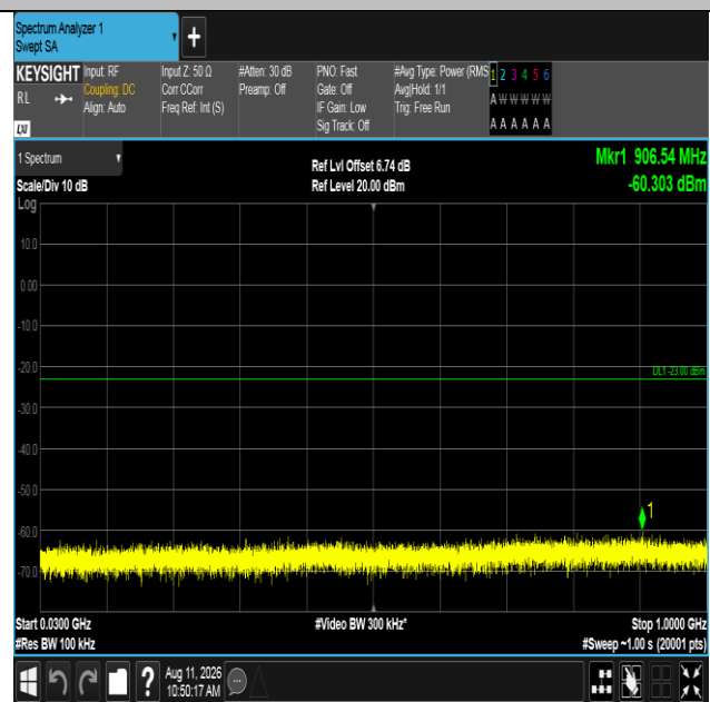
Band4-10MHz-16QAM-20175-50RB#0-30~1000-PASS
