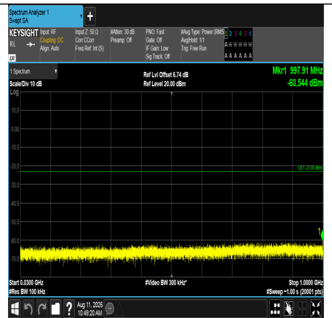
Band4-10MHz-16QAM-20000-50RB#0-30~1000-PASS
