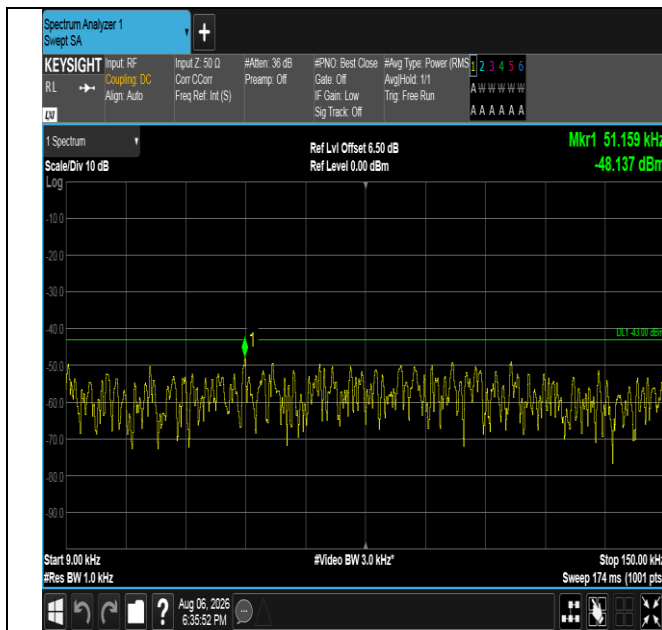
Band4-10MHz-QPSK-20175-1RB#0-0.009~0.15-PASS
