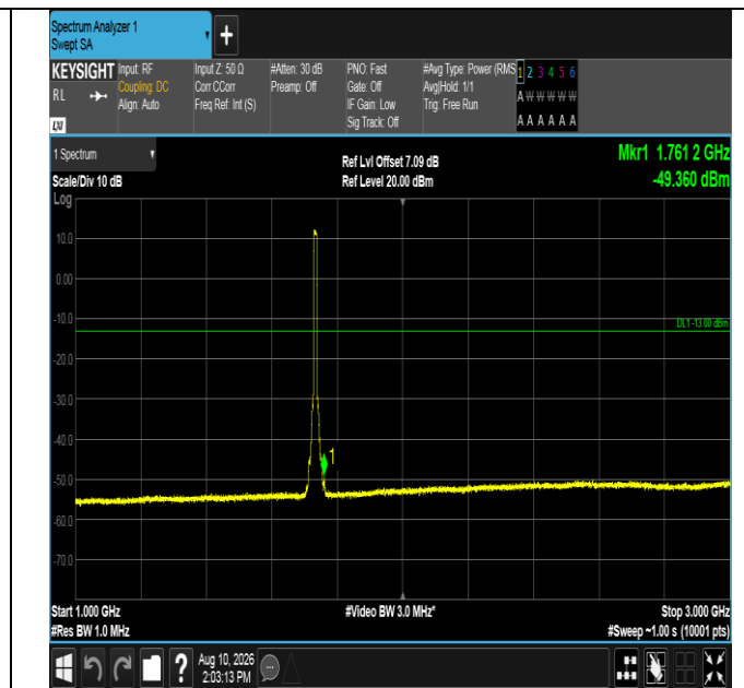
Band4-10MHz-QPSK-20175-50RB#0-1000~3000-PASS
