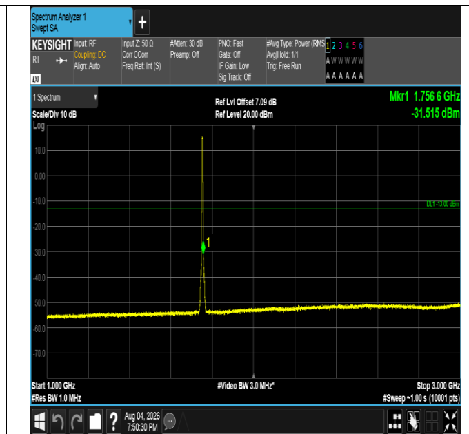
Band4-5MHz-QPSK-20375-25RB#0-1000~3000-PASS
