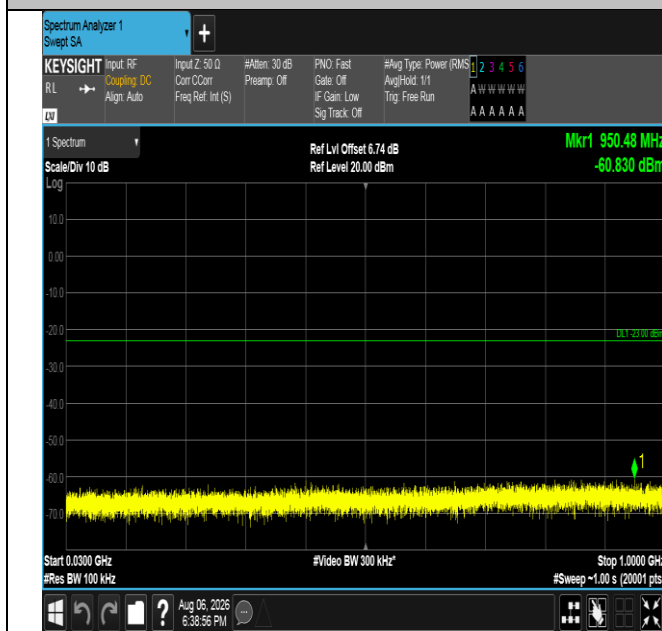
Band4-10MHz-16QAM-20175-1RB#49-30~1000-PASS
