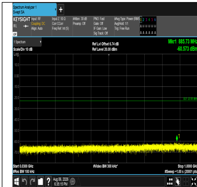
Band4-10MHz-16QAM-20000-1RB#49-30~1000-PASS
