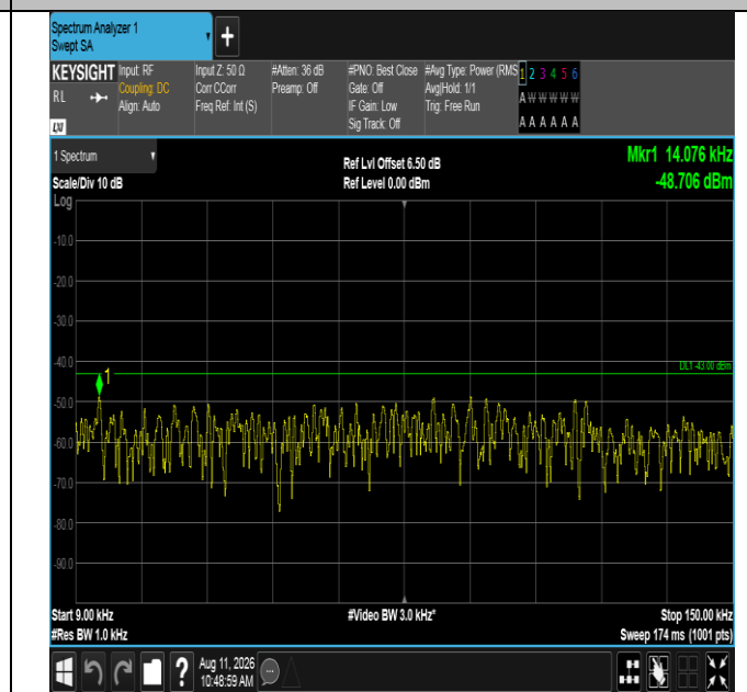
Band4-10MHz-16QAM-20000-50RB#0-0.009~0.15-PASS
