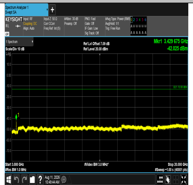
Band4-10MHz-16QAM-20000-50RB#0-3000~20000-PASS
