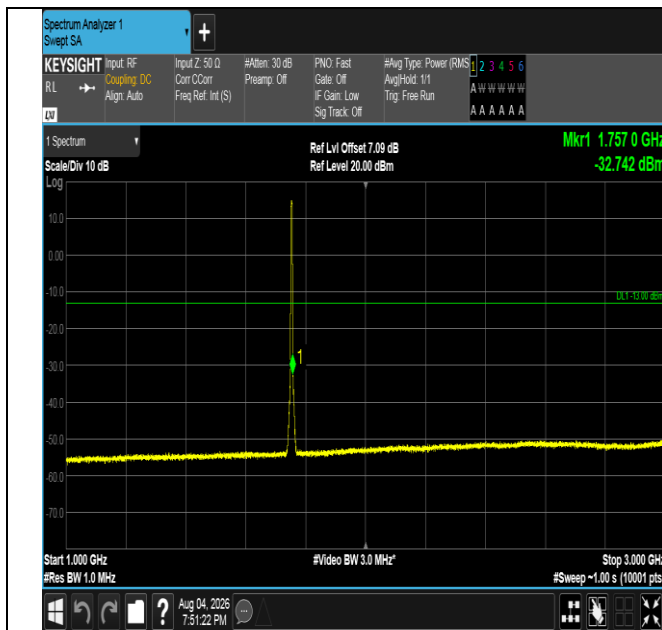
Band4-5MHz-16QAM-20375-25RB#0-1000~3000-PASS
