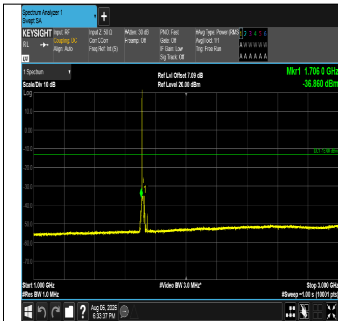
Band4-10MHz-16QAM-20000-1RB#0-1000~3000-PASS
