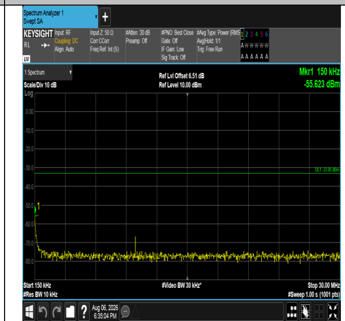
Band4-10MHz-16QAM-20000-1RB#49-0.15~30-PASS
