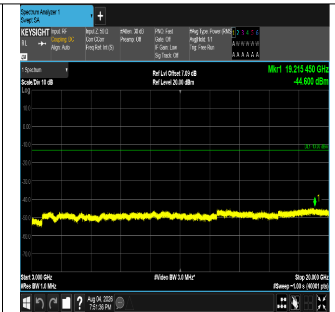
Band4-5MHz-16QAM-20375-25RB#0-3000~20000-PASS
