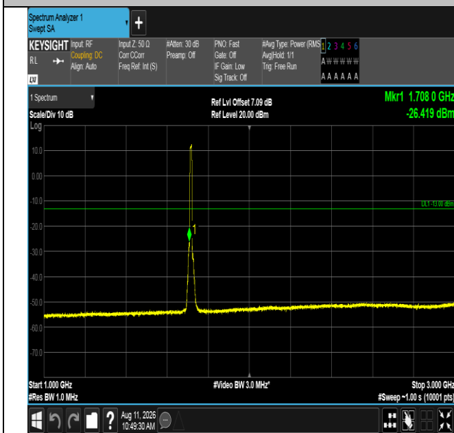
Band4-10MHz-16QAM-20000-50RB#0-1000~3000-PASS
