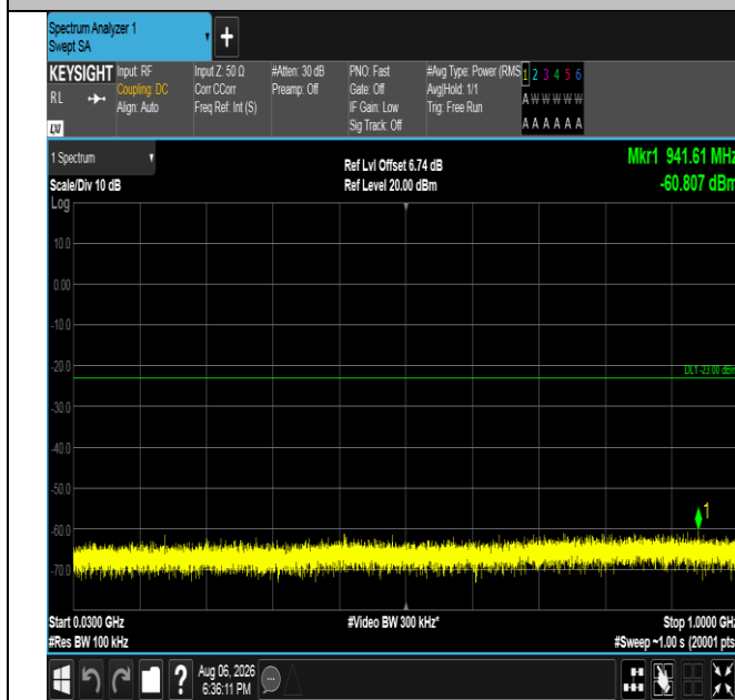
Band4-10MHz-QPSK-20175-1RB#0-30~1000-PASS
