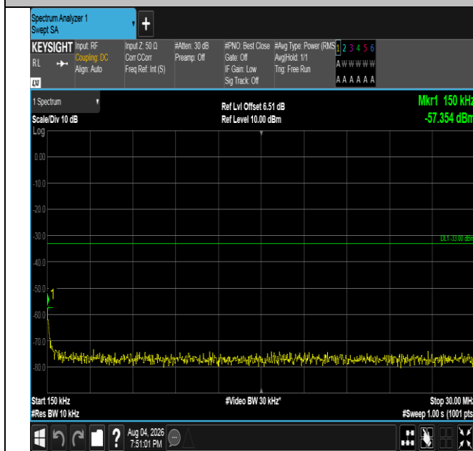
Band4-5MHz-16QAM-20375-25RB#0-0.15~30-PASS
