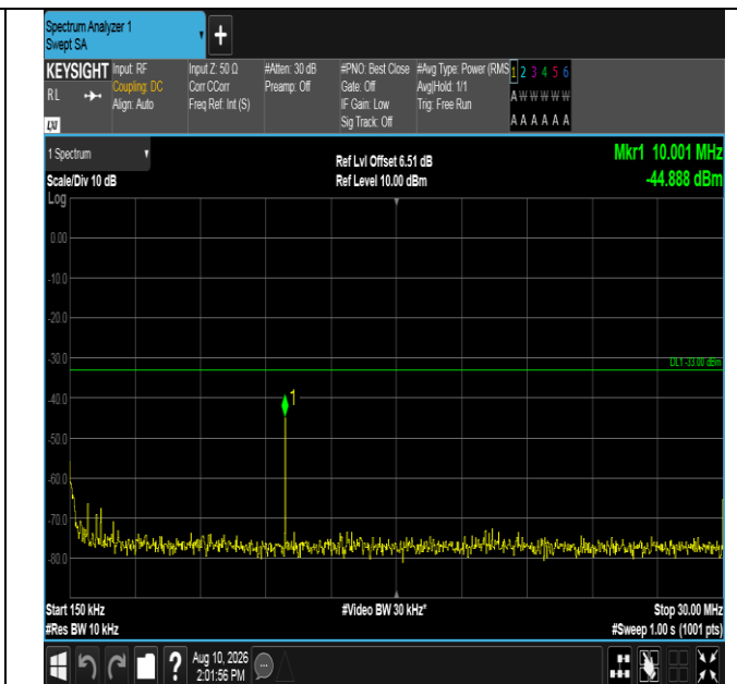
Band4-10MHz-QPSK-20000-50RB#0-0.15~30-PASS
