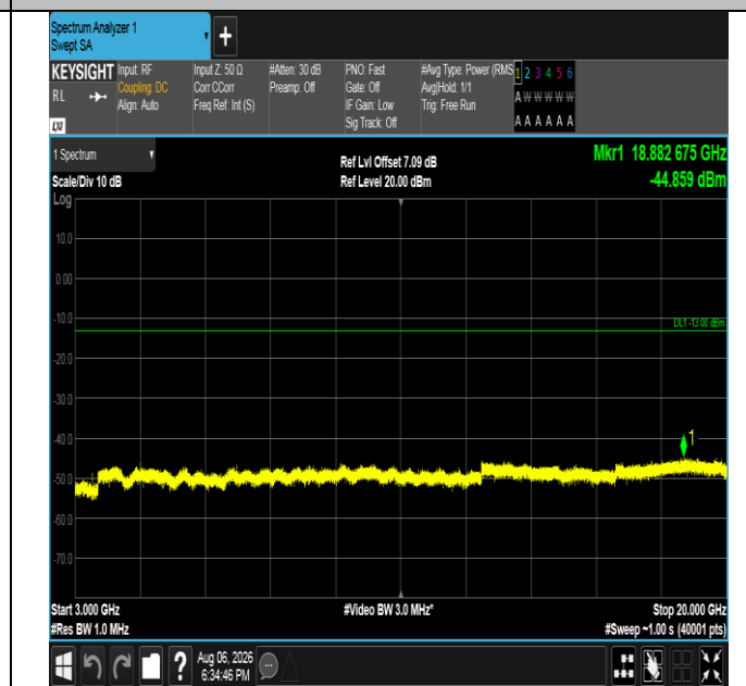
Band4-10MHz-QPSK-20000-1RB#49-3000~20000-PASS
