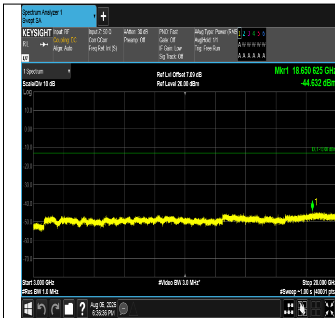
Band4-10MHz-QPSK-20175-1RB#0-3000~20000-PASS
