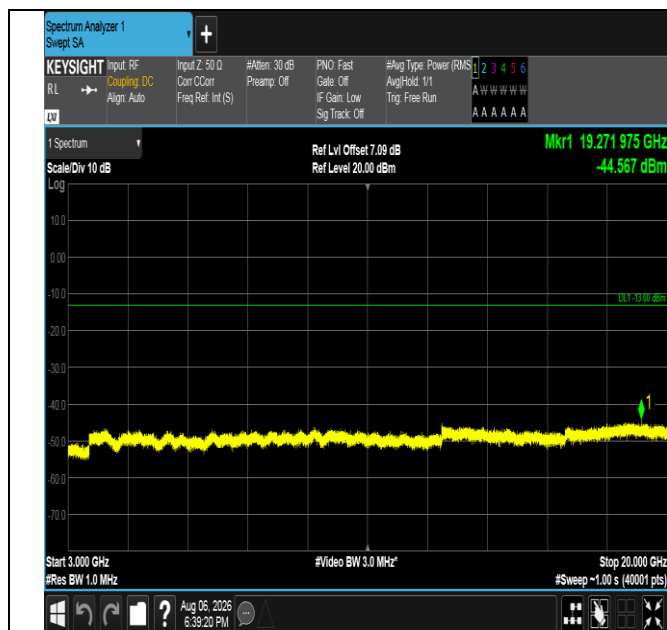
Band4-10MHz-16QAM-20175-1RB#49-3000~20000-PASS
