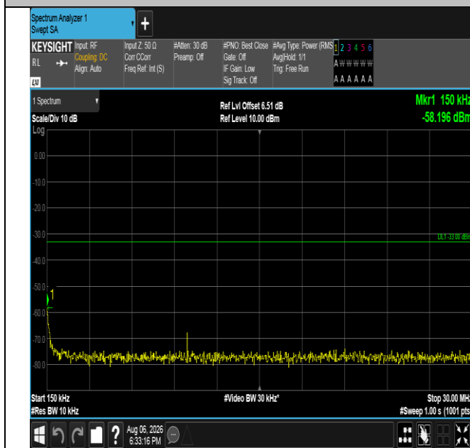
Band4-10MHz-16QAM-20000-1RB#0-0.15~30-PASS
