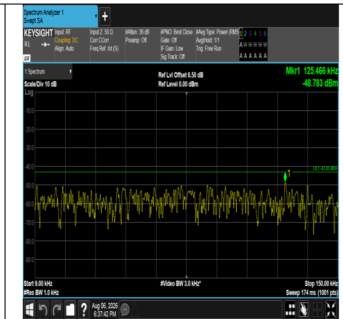
Band4-10MHz-QPSK-20175-1RB#49-0.009~0.15-PASS
