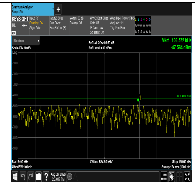
Band4-10MHz-16QAM-20000-1RB#0-0.009~0.15-PASS
