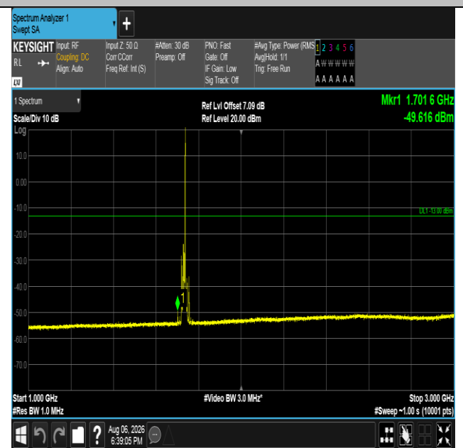
Band4-10MHz-16QAM-20175-1RB#49-1000~3000-PASS
