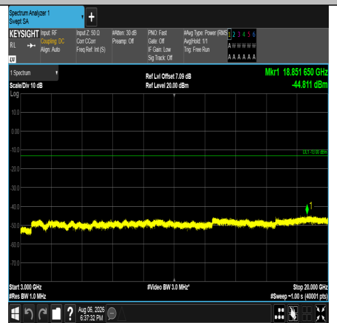
Band4-10MHz-16QAM-20175-1RB#0-3000~20000-PASS
