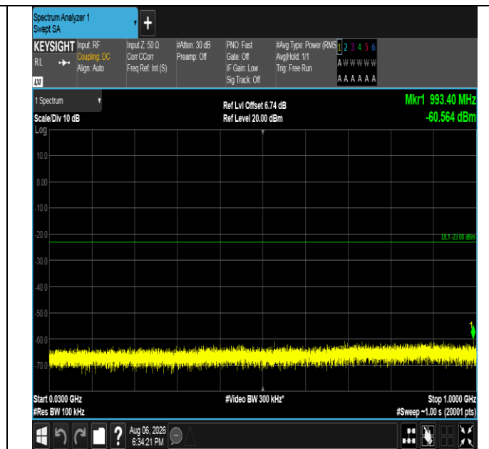
Band4-10MHz-QPSK-20000-1RB#49-30~1000-PASS
