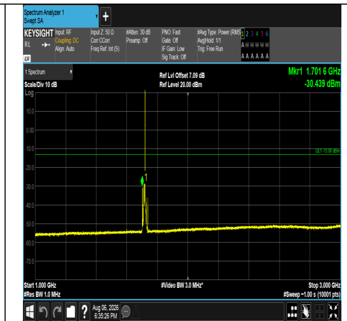
Band4-10MHz-16QAM-20000-1RB#49-1000~3000-PASS
