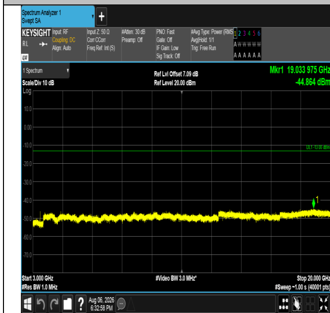
Band4-10MHz-QPSK-20000-1RB#0-3000~20000-PASS
