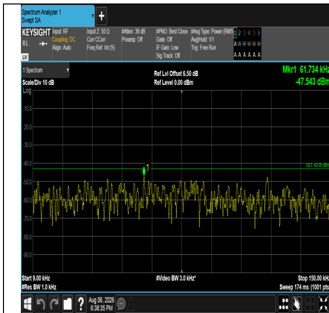
Band4-10MHz-16QAM-20175-1RB#49-0.009~0.15-PASS
