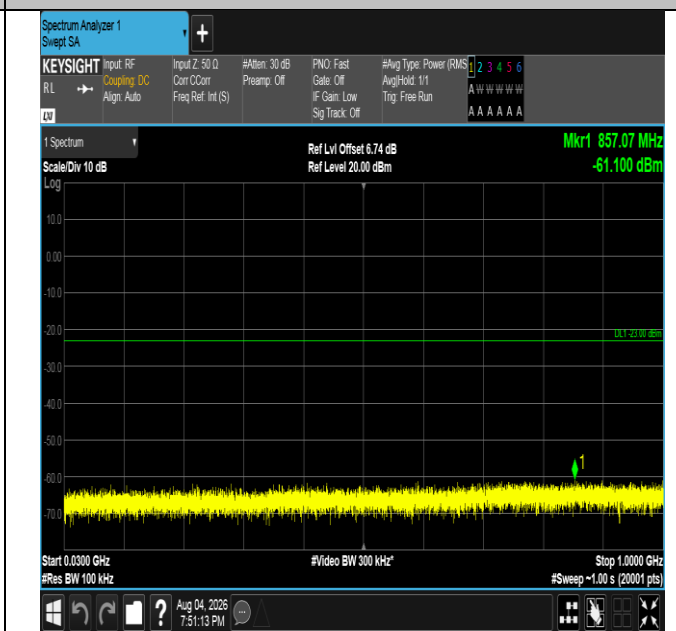
Band4-5MHz-16QAM-20375-25RB#0-30~1000-PASS
