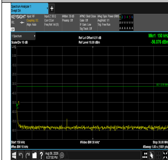
Band4-10MHz-QPSK-20175-1RB#49-0.15~30-PASS
