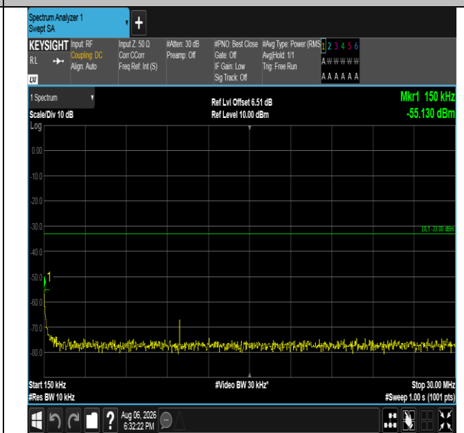
Band4-10MHz-QPSK-20000-1RB#0-0.15~30-PASS
