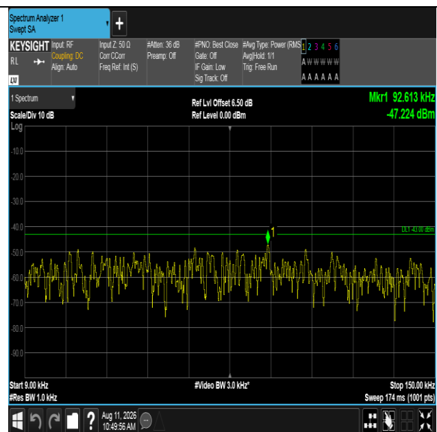
Band4-10MHz-16QAM-20175-50RB#0-0.009~0.15-PASS
