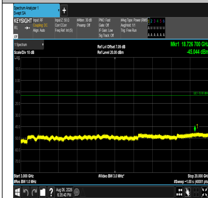
Band4-10MHz-16QAM-20000-1RB#49-3000~20000-PASS
