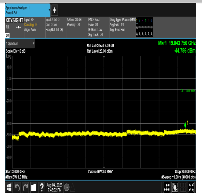
Band4-5MHz-16QAM-20375-1RB#0-3000~20000-PASS
