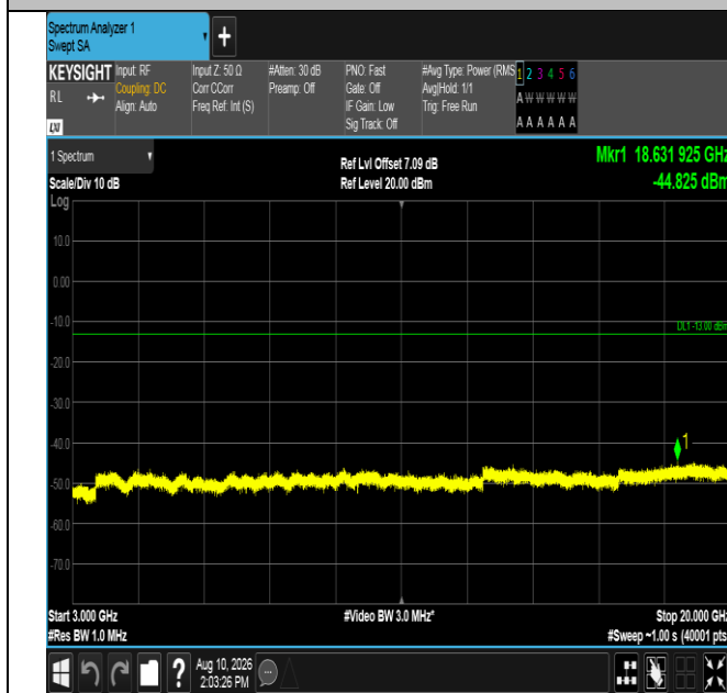
Band4-10MHz-QPSK-20175-50RB#0-3000~20000-PASS
