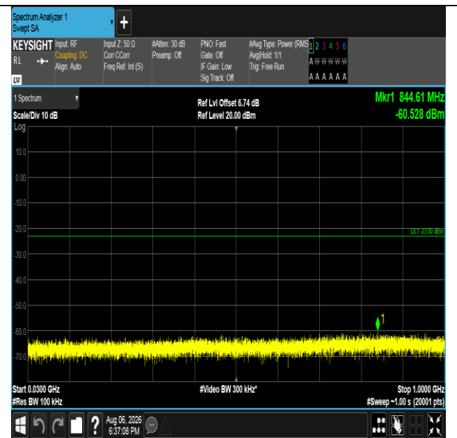
Band4-10MHz-16QAM-20175-1RB#0-30~1000-PASS
