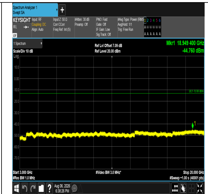
Band4-10MHz-QPSK-20175-1RB#49-3000~20000-PASS
