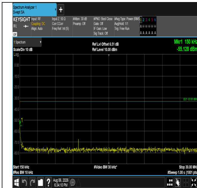
Band4-10MHz-QPSK-20000-1RB#49-0.15~30-PASS
