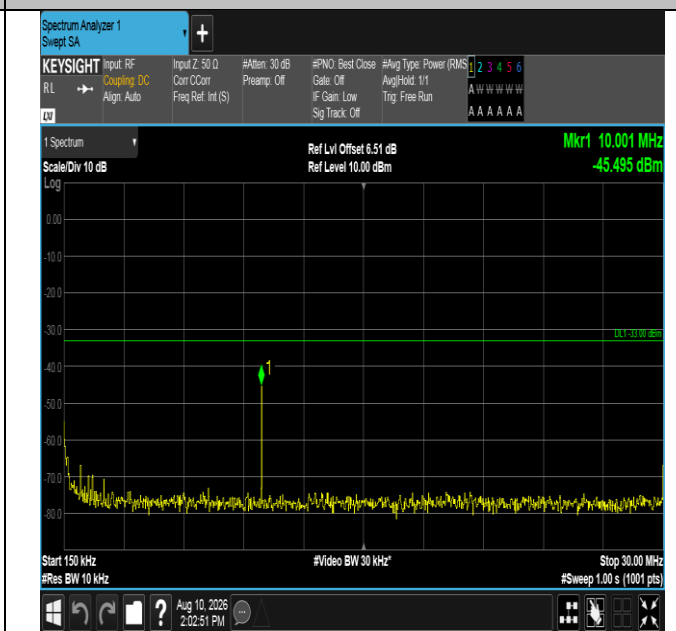
Band4-10MHz-QPSK-20175-50RB#0-0.15~30-PASS
