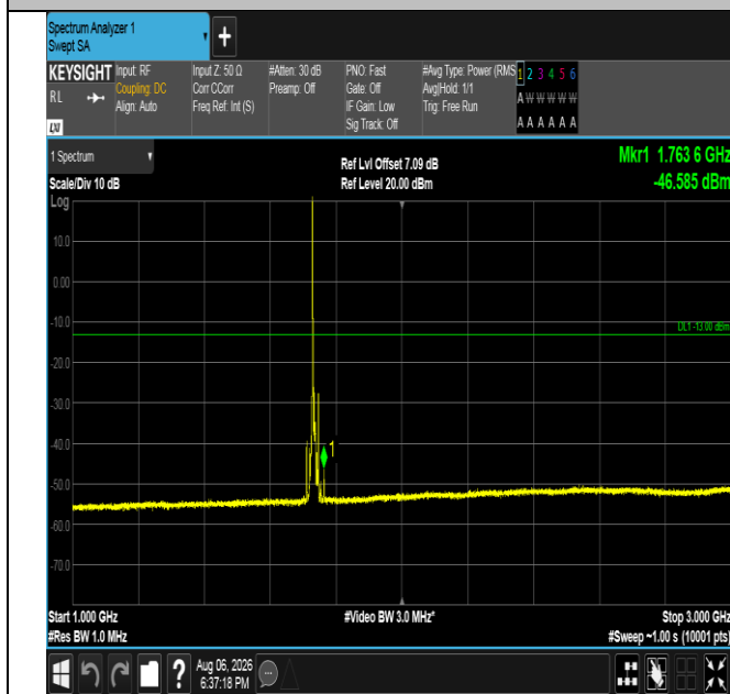
Band4-10MHz-16QAM-20175-1RB#0-1000~3000-PASS
