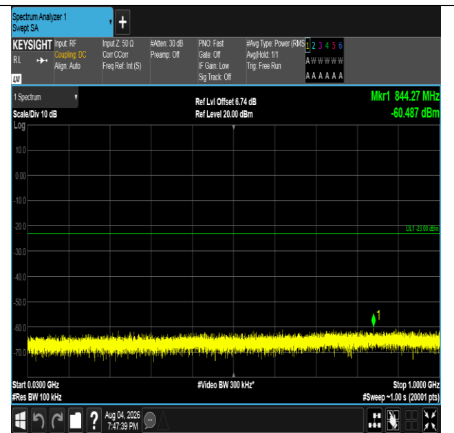
Band4-5MHz-16QAM-20375-1RB#0-30~1000-PASS
