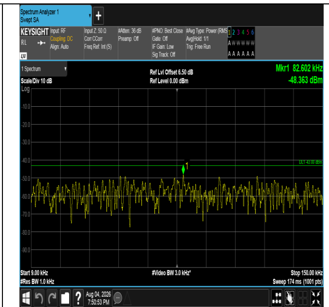
Band4-5MHz-16QAM-20375-25RB#0-0.009~0.15-PASS
