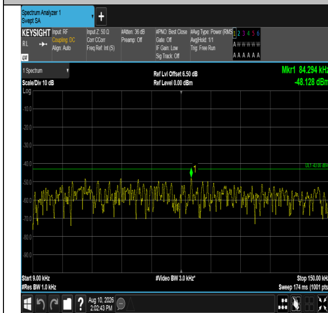
Band4-10MHz-QPSK-20175-50RB#0-0.009~0.15-PASS
