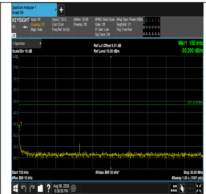
Band4-10MHz-QPSK-20175-1RB#0-0.15~30-PASS
