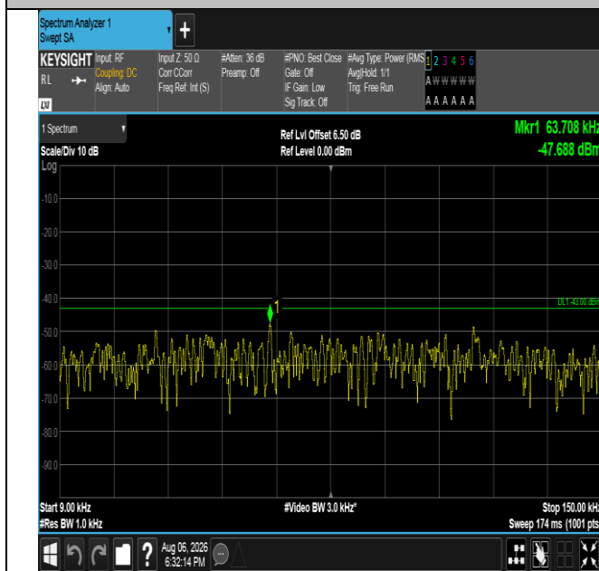
Band4-10MHz-QPSK-20000-1RB#0-0.009~0.15-PASS
