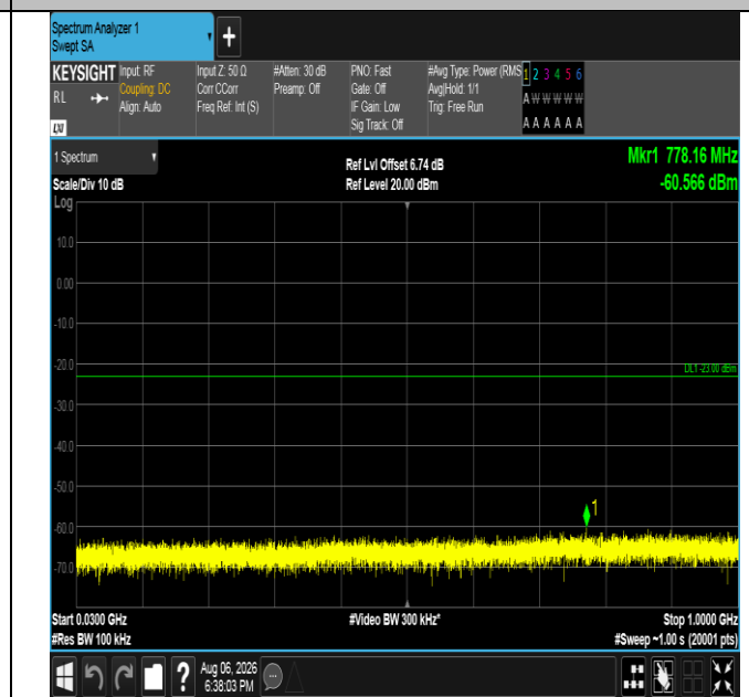
Band4-10MHz-QPSK-20175-1RB#49-30~1000-PASS
