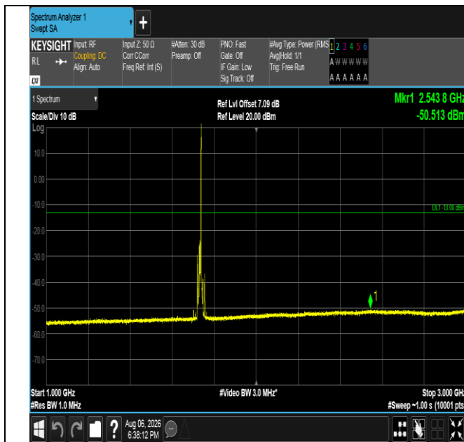
Band4-10MHz-QPSK-20175-1RB#49-1000~3000-PASS
