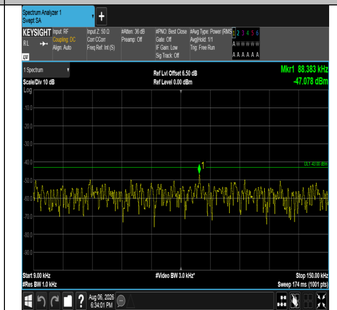
Band4-10MHz-QPSK-20000-1RB#49-0.009~0.15-PASS
