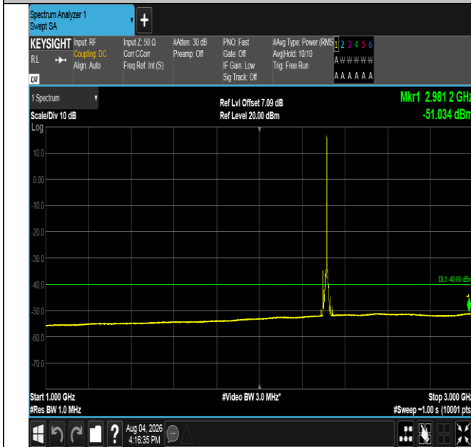
Band40(2305-2315)-10MHz-16QAM-38750-1RB#49-1000~30 00-PASS
