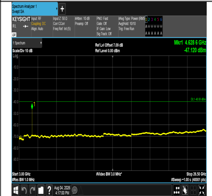
Band40(2305-2315)-10MHz-16QAM-38750-1RB#49-3000~26 500-PASS
