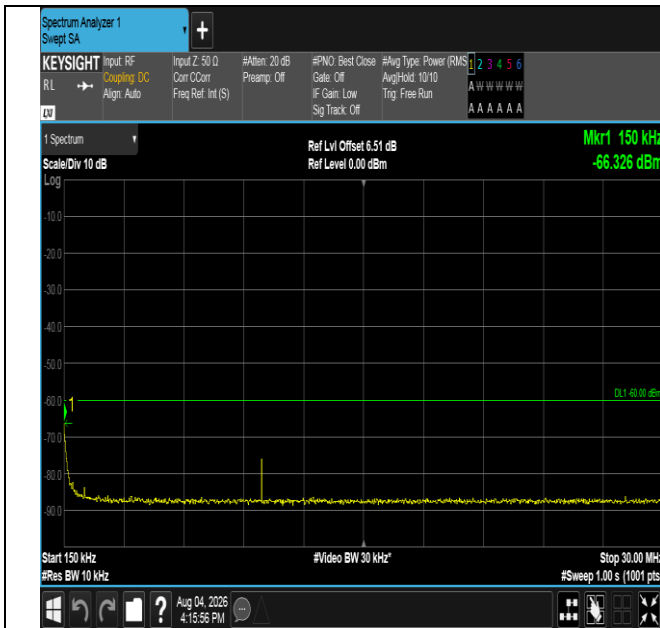
Band40(2305-2315)-10MHz-16QAM-38750-1RB#49-0.15~30- PASS
