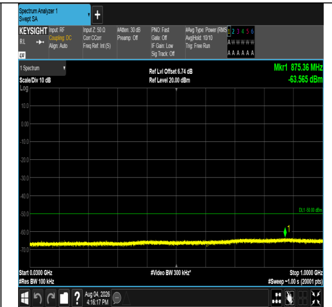
Band40(2305-2315)-10MHz-16QAM-38750-1RB#49-30~1000 -PASS
