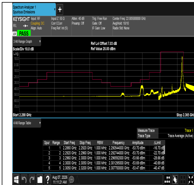
Band40(2350-2360)-10MHz-16QAM-39200-1RB#49-PASS
