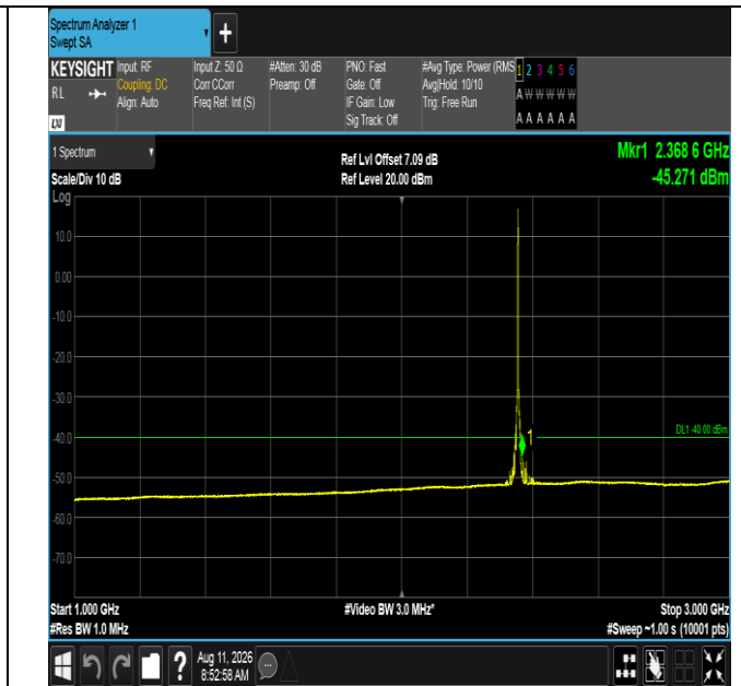
Band40(2350-2360)-5MHz-16QAM-39175-1RB#24-1000~3000-PASS
