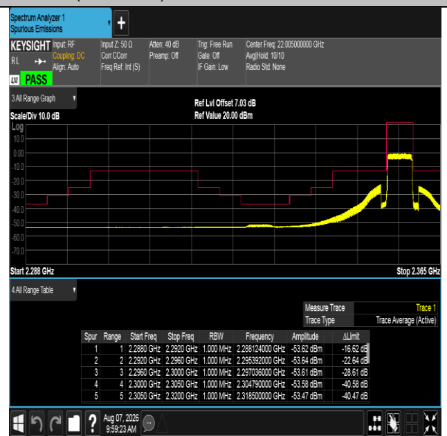
Band40(2350-2360)-5MHz-16QAM-39225-25RB#0-PASS
