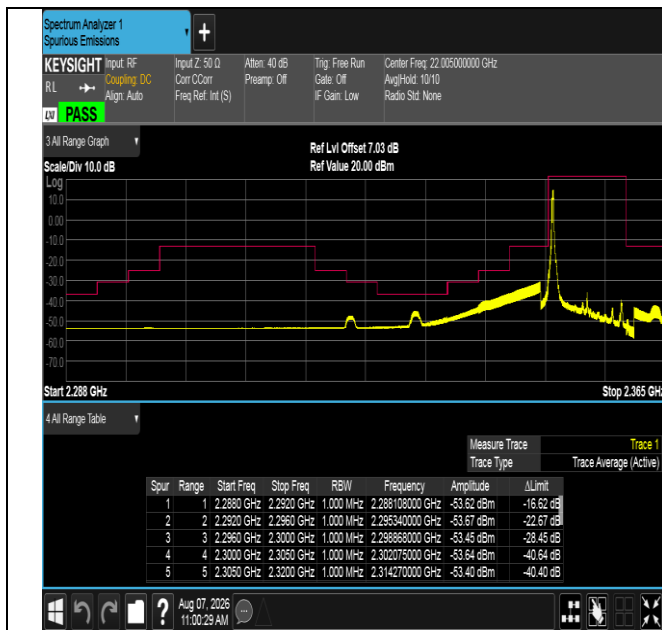
Band40(2350-2360)-10MHz-QPSK-39200-1RB#0-PASS
