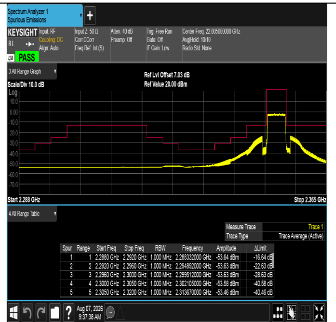
Band40(2350-2360)-5MHz-16QAM-39175-25RB#0-PASS
