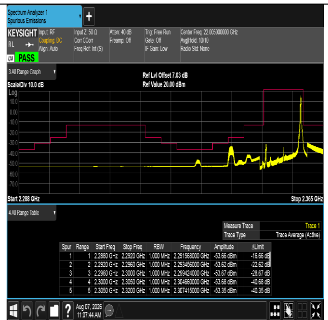
Band40(2350-2360)-10MHz-QPSK-39200-1RB#49-PASS
