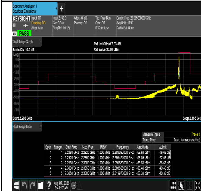
Band40(2350-2360)-5MHz-QPSK-39225-1RB#0-PASS
