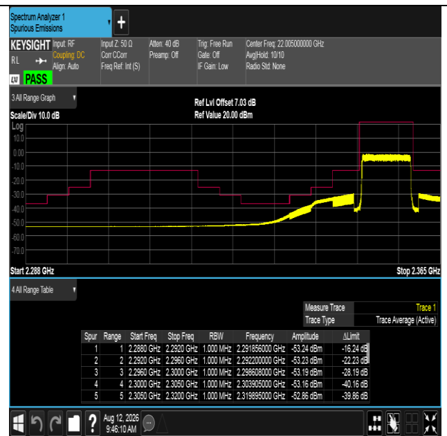
Band40(2350-2360)-10MHz-16QAM-39200-50RB#0-PASS
