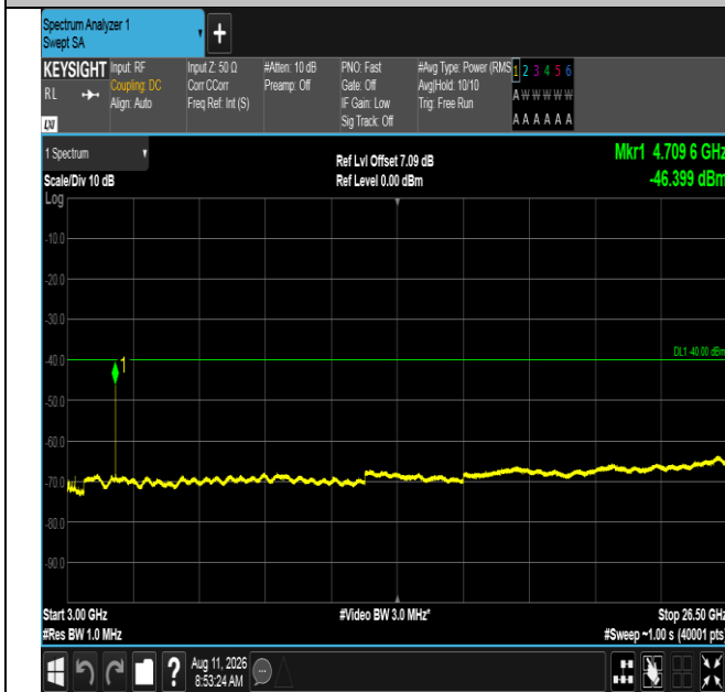
Band40(2350-2360)-5MHz-16QAM-39175-1RB#24-3000~26500-PASS
