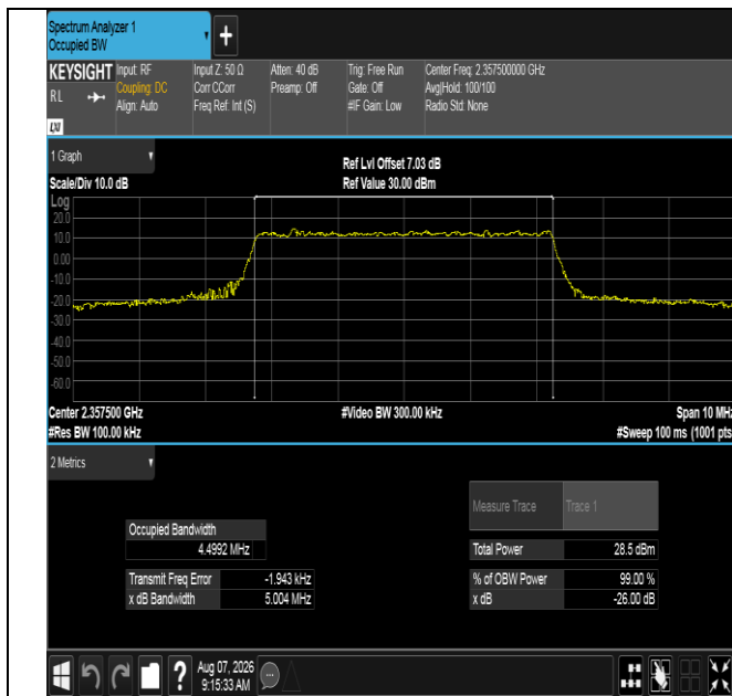
Band40(2350-2360)-5MHz-QPSK-39225-25RB#0-PASS
