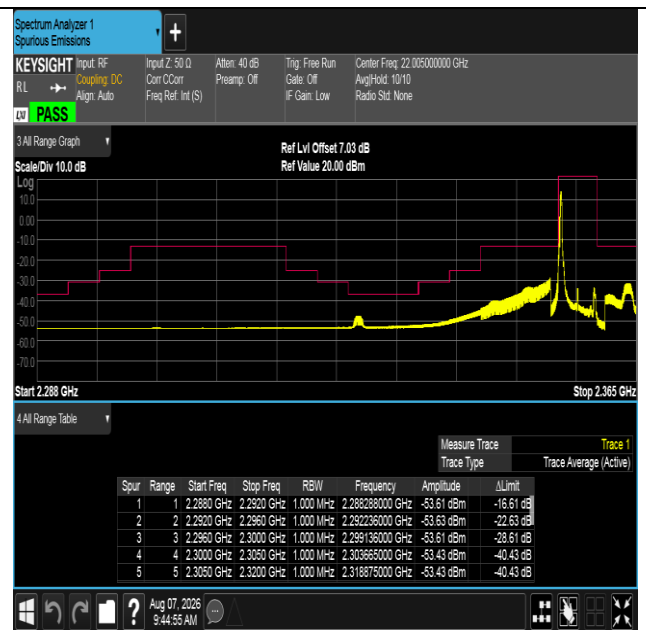
Band40(2350-2360)-5MHz-16QAM-39225-1RB#0-PASS
