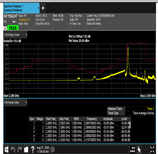
Band40(2350-2360)-10MHz-16QAM-39200-1RB#0-PASS
