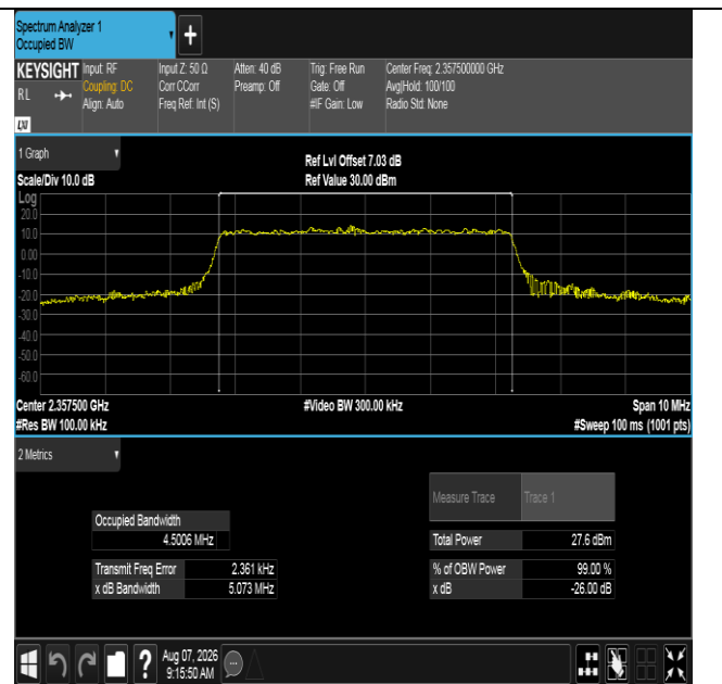
Band40(2350-2360)-5MHz-16QAM-39225-25RB#0-PASS
