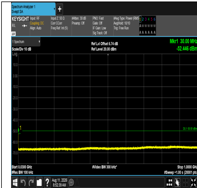
Band40(2350-2360)-5MHz-16QAM-39175-1RB#24-30~1000-PASS
