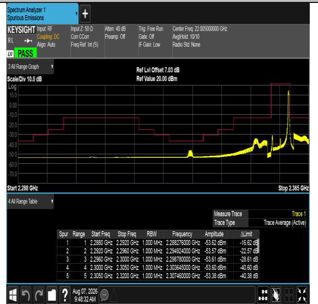
Band40(2350-2360)-5MHz-QPSK-39225-1RB#24-PASS
