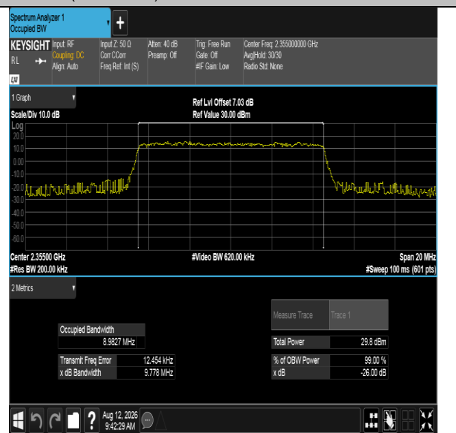
Band40(2350-2360)-10MHz-16QAM-39200-50RB#0-PASS
