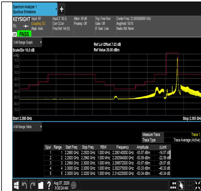
Band40(2350-2360)-5MHz-16QAM-39175-1RB#24-PASS
