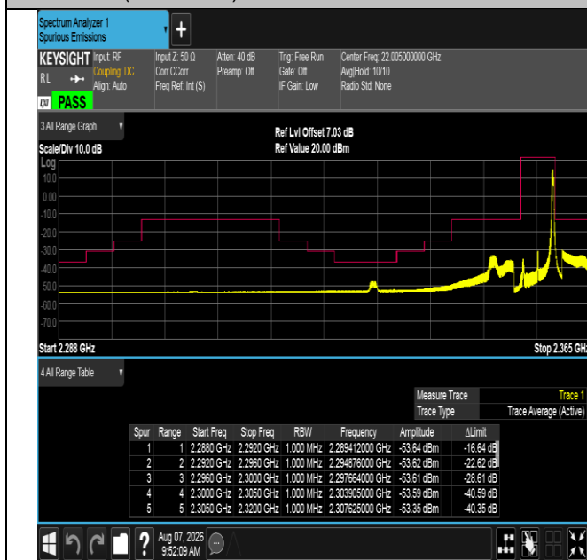
Band40(2350-2360)-5MHz-16QAM-39225-1RB#24-PASS
