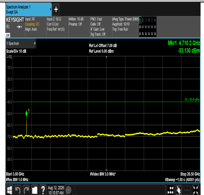
Band40(2350-2360)-10MHz-16QAM-39200-50RB#0-3000~26500-PASS
