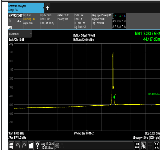
Band40(2350-2360)-10MHz-16QAM-39200-50RB#0-1000~3000- PASS
