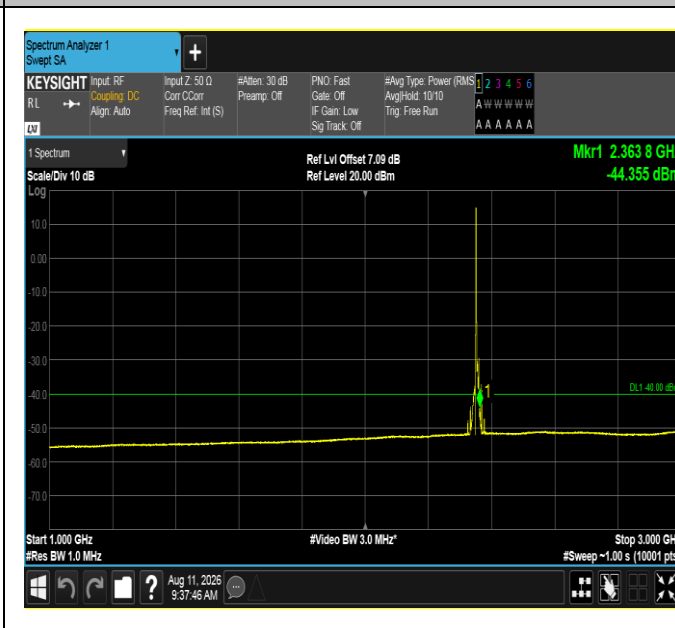
Band40(2350-2360)-10MHz-QPSK-39200-50RB#0-1000~3000-PASS
