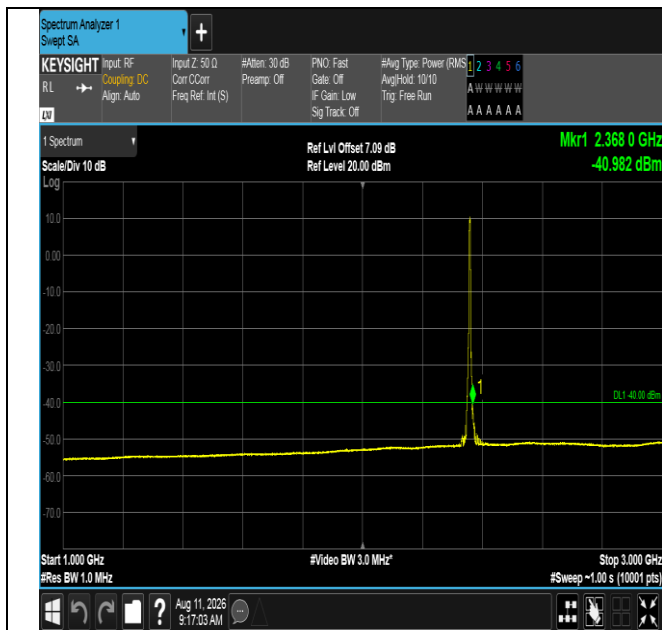
Band40(2350-2360)-5MHz-QPSK-39225-25RB#0-1000~3000-PASS
