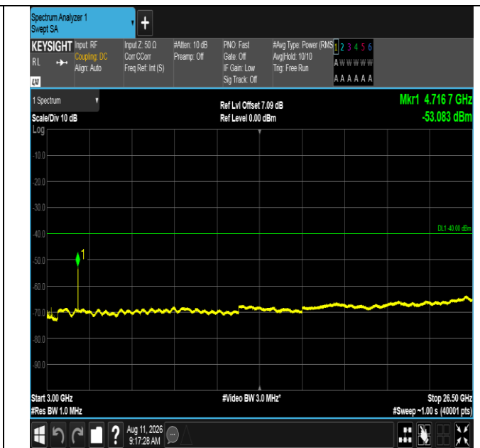
Band40(2350-2360)-5MHz-QPSK-39225-25RB#0-3000~26500-PASS
