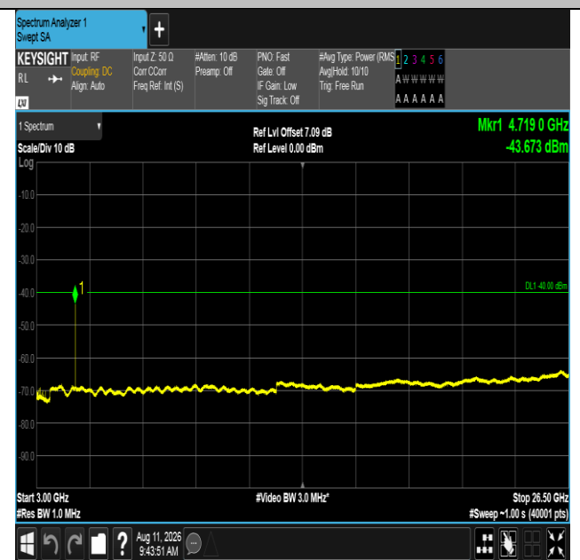
Band40(2350-2360)-10MHz-16QAM-39200-1RB#49-3000~26500-PASS
