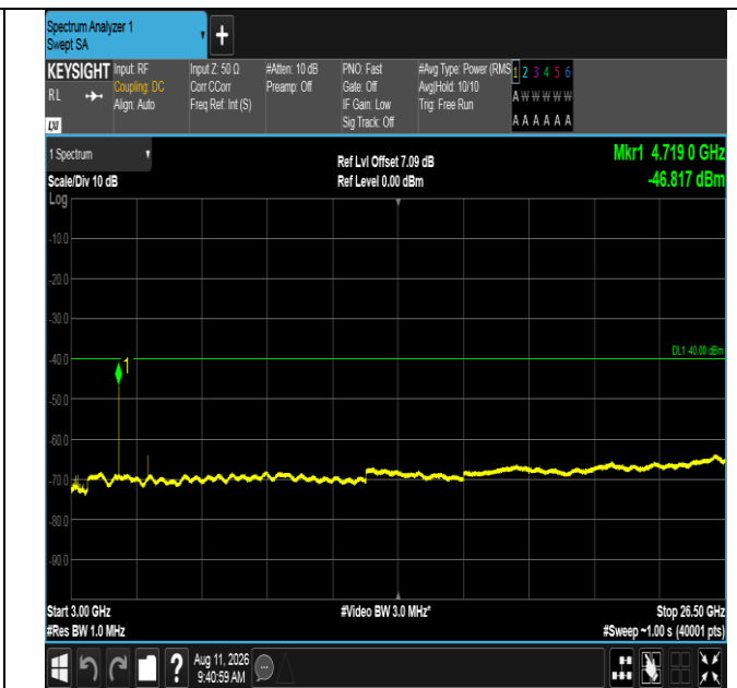
Band40(2350-2360)-10MHz-QPSK-39200-1RB#49-3000~26500-PASS
