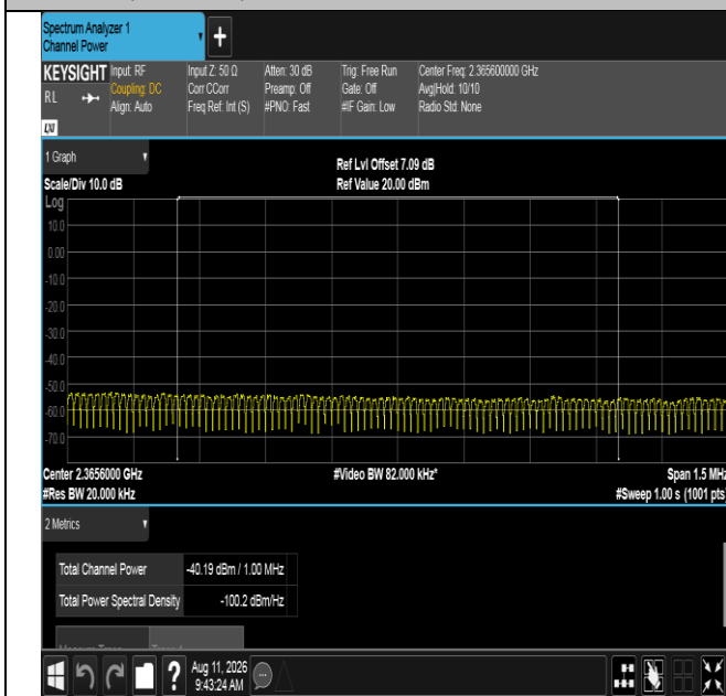
Band40(2350-2360)-10MHz-16QAM-39200-1RB#49-1000~3000-PASS
