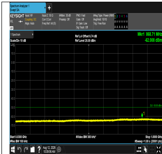
Band40(2350-2360)-10MHz-16QAM-39200-50RB#0-30~1000-PASS
