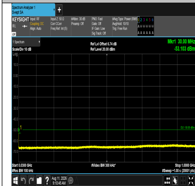
Band40(2350-2360)-5MHz-16QAM-39225-1RB#0-30~1000-PASS
