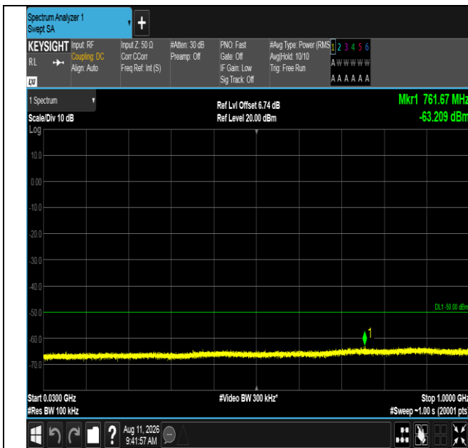
Band40(2350-2360)-10MHz-16QAM-39200-1RB#49-30~1000-PASS
