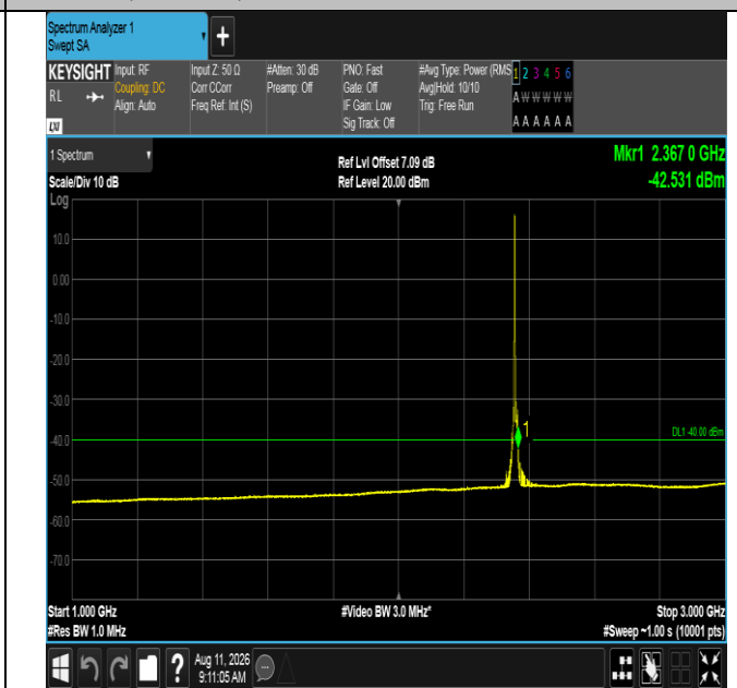
Band40(2350-2360)-5MHz-16QAM-39225-1RB#0-1000~3000-PASS
