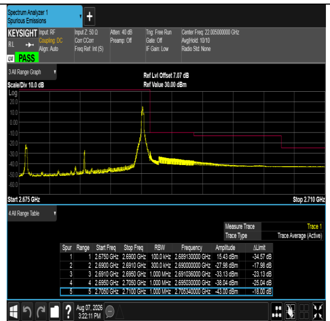
Band41-15MHz-QPSK-41515-1RB#74-PASS
