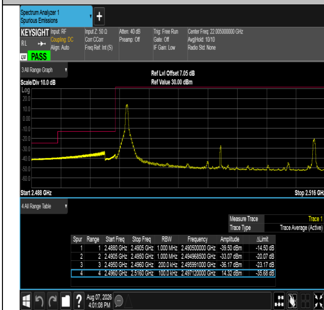
Band41-20MHz-QPSK-39750-1RB#0-PASS
