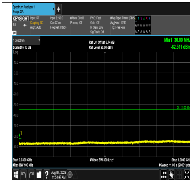
Band41-5MHz-QPSK-39675-1RB#24-30~1000-PASS
