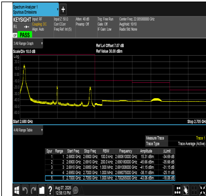
Band41-10MHz-QPSK-41540-1RB#0-PASS
