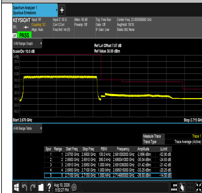
Band41-20MHz-QPSK-41490-100RB#0-PASS
