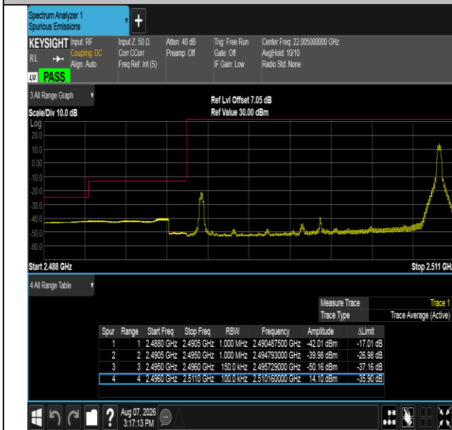
Band41-15MHz-16QAM-39725-1RB#74-PASS
