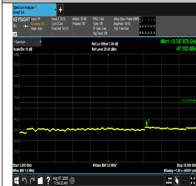
Band41-5MHz-QPSK-39675-1RB#24-3000~18000-PASS
