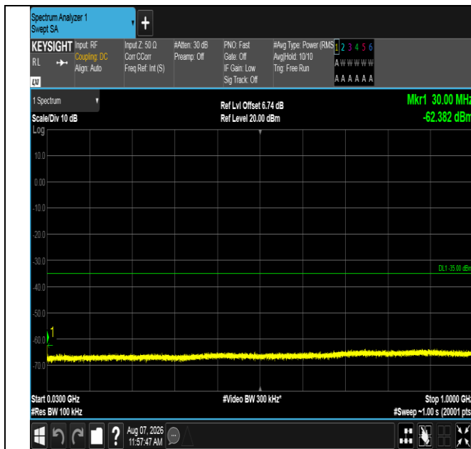
Band41-5MHz-QPSK-39675-25RB#0-30~1000-PASS
