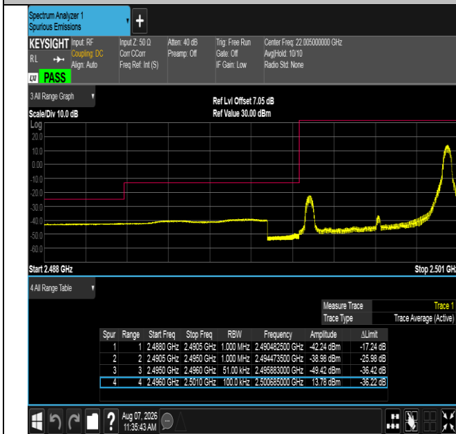
Band41-5MHz-16QAM-39675-1RB#24-PASS
