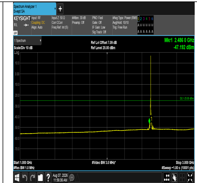
Band41-5MHz-16QAM-39675-1RB#24-1000~3000-PASS
