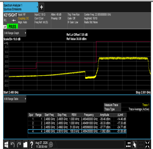
Band41-5MHz-16QAM-39675-25RB#0-PASS
