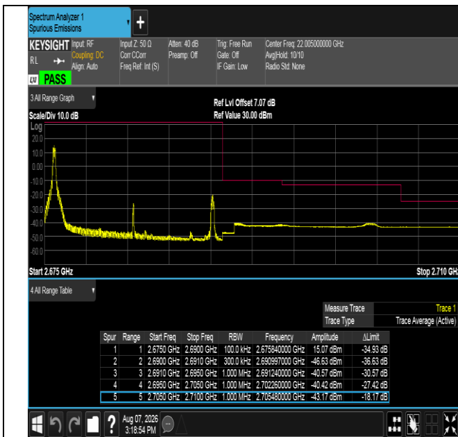
Band41-15MHz-QPSK-41515-1RB#0-PASS
