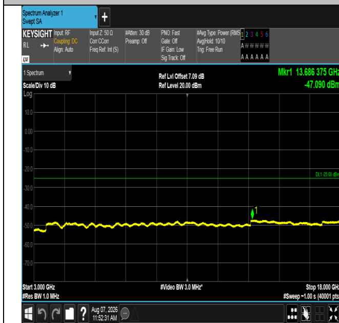
Band41-5MHz-16QAM-39675-1RB#0-3000~18000-PASS
