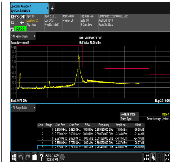
Band41-15MHz-16QAM-41515-1RB#74-PASS
