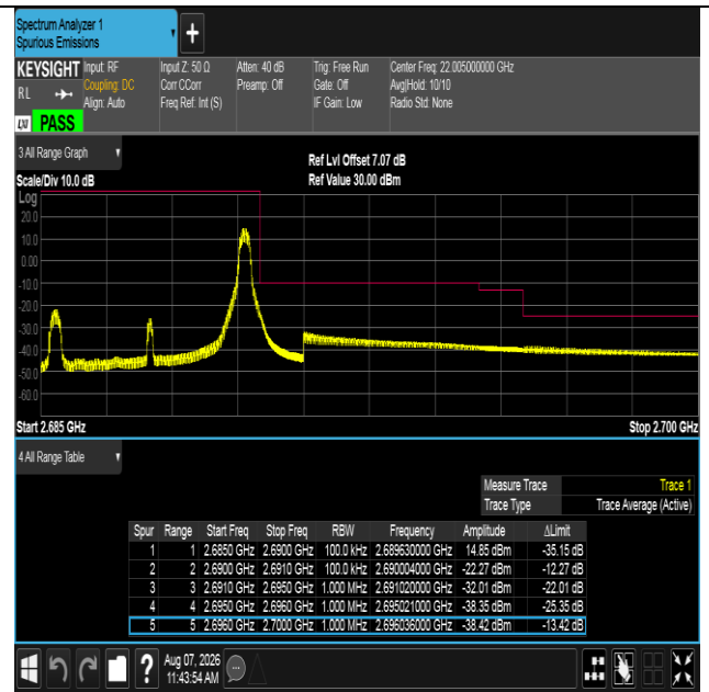
Band41-5MHz-QPSK-41565-1RB#24-PASS
