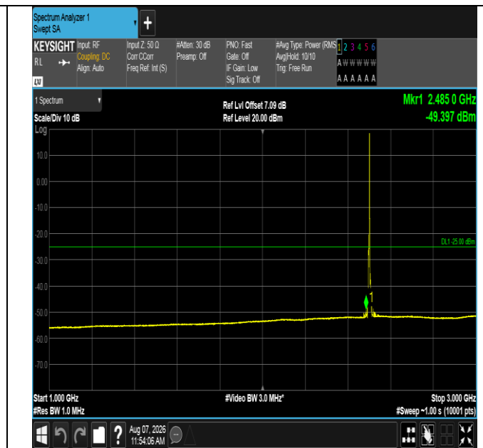
Band41-5MHz-QPSK-39675-1RB#24-1000~3000-PASS
