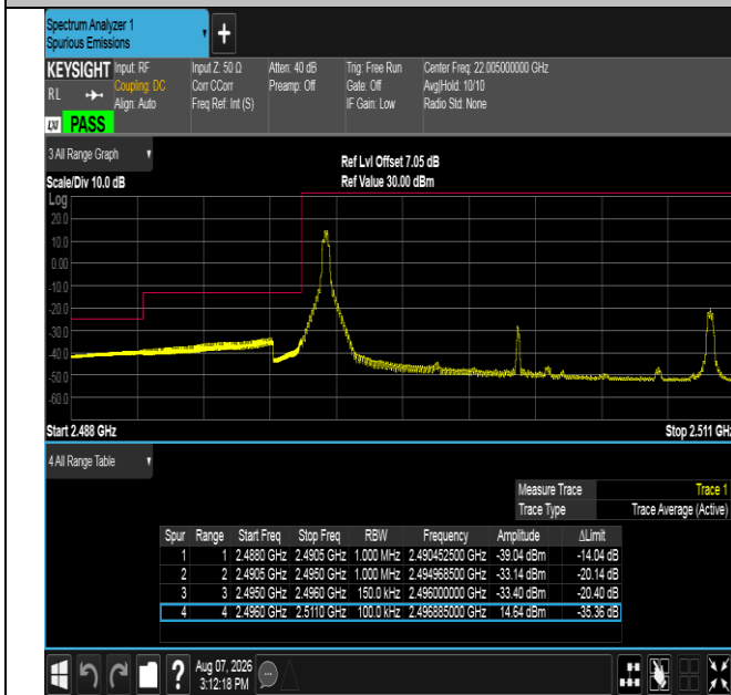
Band41-15MHz-QPSK-39725-1RB#0-PASS
