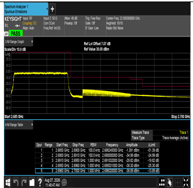
Band41-5MHz-16QAM-41565-25RB#0-PASS
