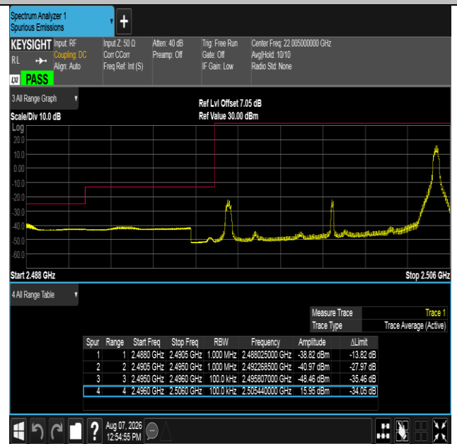
Band41-10MHz-QPSK-39700-1RB#49-PASS
