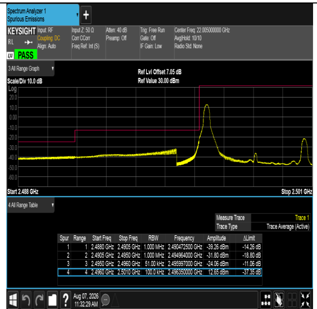
Band41-5MHz-16QAM-39675-1RB#0-PASS
