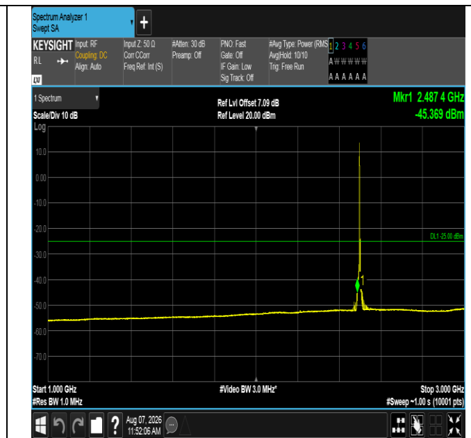
Band41-5MHz-16QAM-39675-1RB#0-1000~3000-PASS
