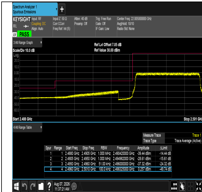
Band41-5MHz-QPSK-39675-25RB#0-PASS
