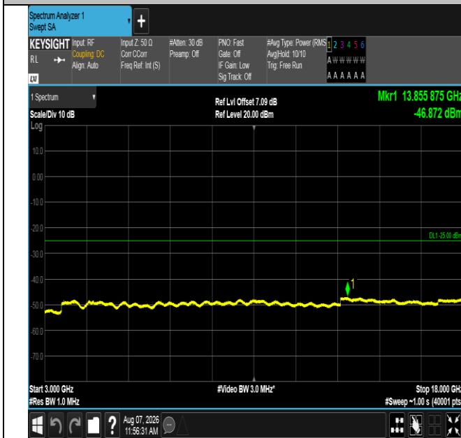
Band41-5MHz-16QAM-39675-1RB#24-3000~18000-PASS
