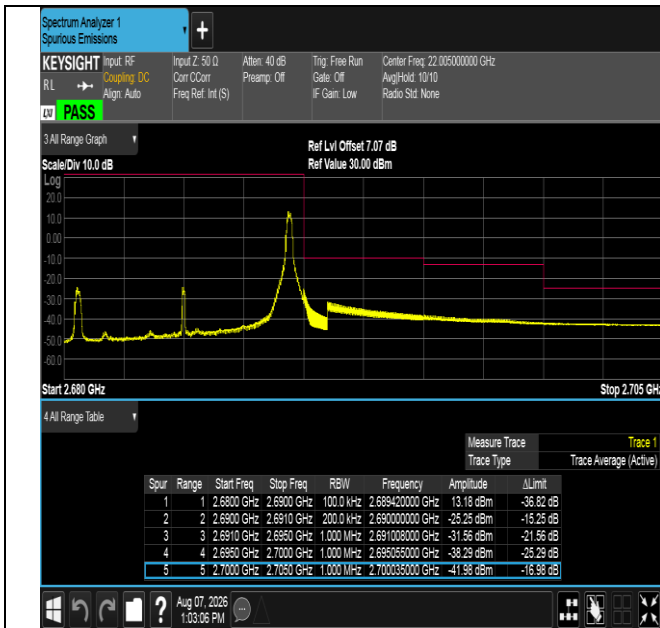
Band41-10MHz-16QAM-41540-1RB#49-PASS
