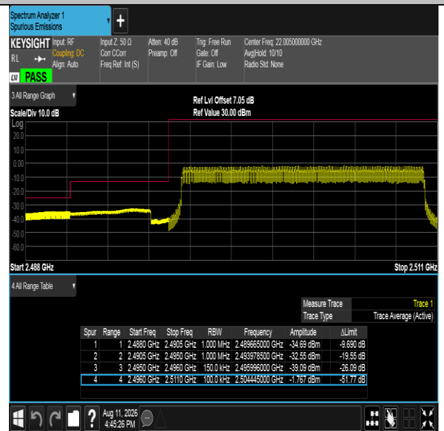
Band41-15MHz-16QAM-39725-75RB#0-PASS
