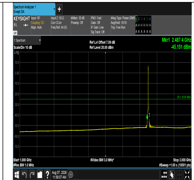
Band41-5MHz-QPSK-39675-25RB#0-1000~3000-PASS
