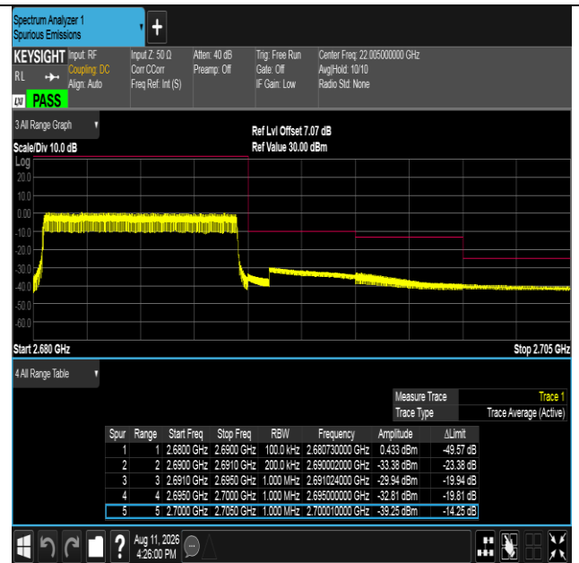
Band41-10MHz-16QAM-41540-50RB#0-PASS
