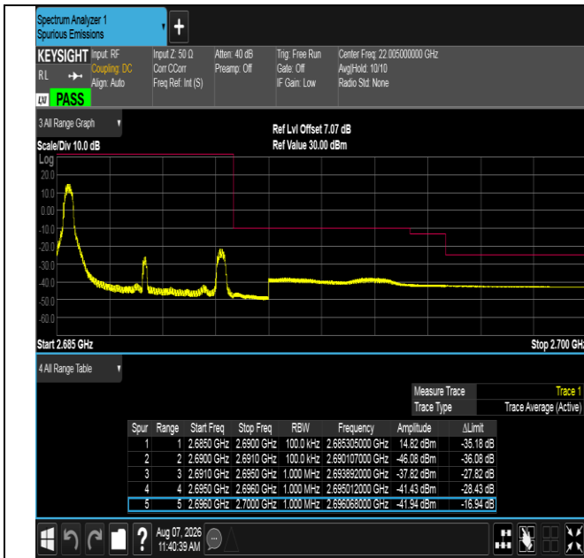
Band41-5MHz-QPSK-41565-1RB#0-PASS
