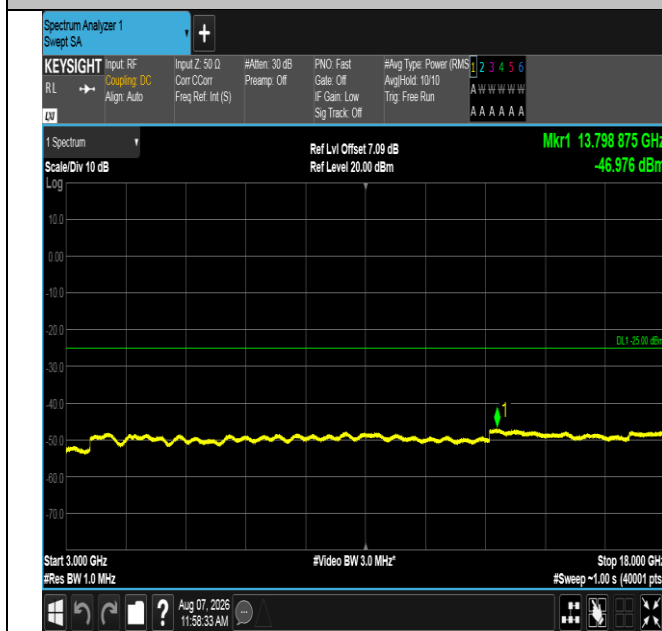
Band41-5MHz-QPSK-39675-25RB#0-3000~18000-PASS
