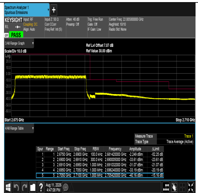
Band41-15MHz-16QAM-41515-75RB#0-PASS
