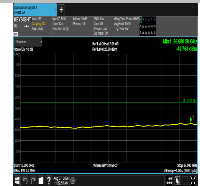
Band41-5MHz-16QAM-39675-1RB#0-18000~27000-PASS
