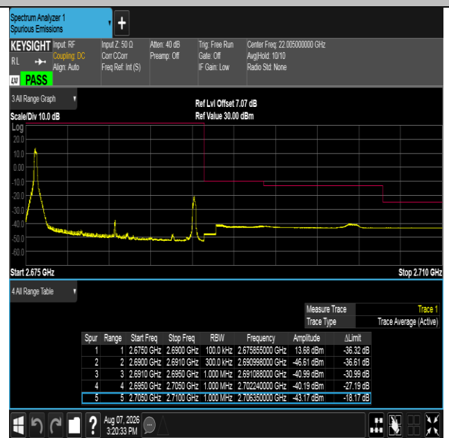
Band41-15MHz-16QAM-41515-1RB#0-PASS
