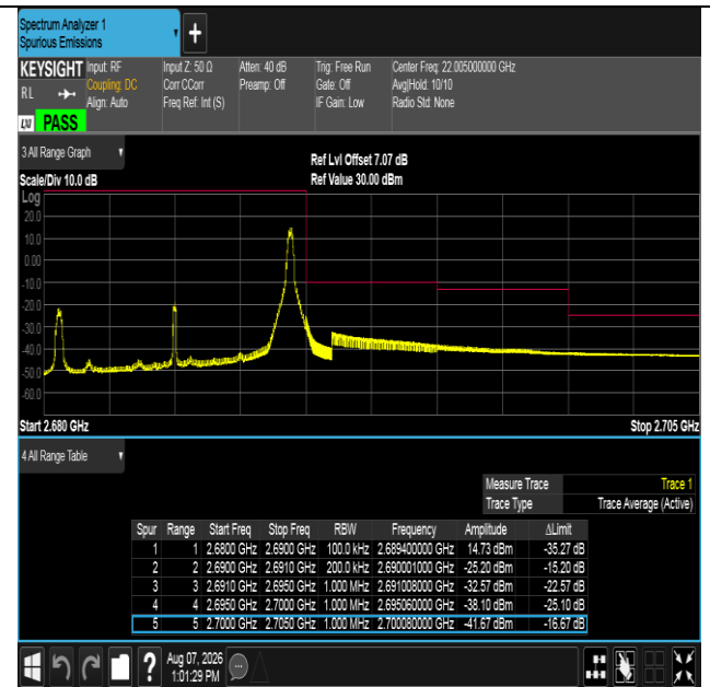
Band41-10MHz-QPSK-41540-1RB#49-PASS
