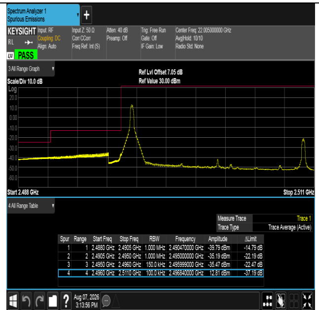
Band41-15MHz-16QAM-39725-1RB#0-PASS
