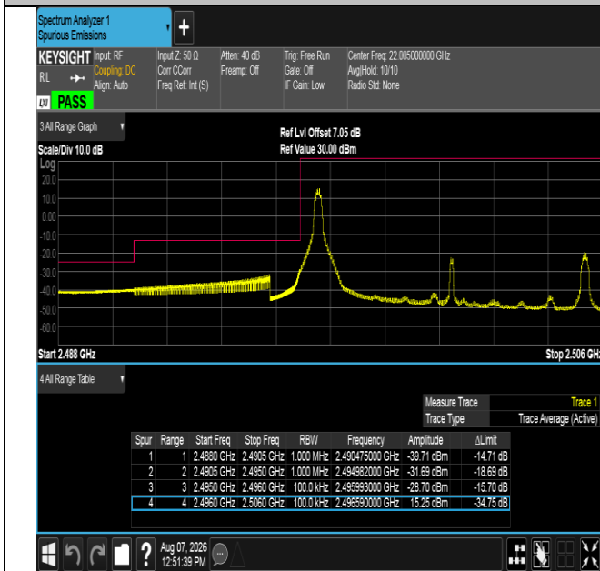
Band41-10MHz-QPSK-39700-1RB#0-PASS
