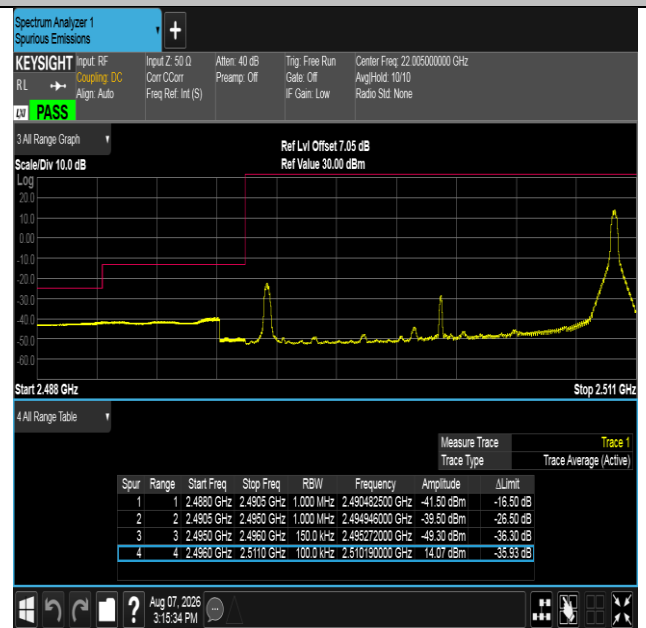
Band41-15MHz-QPSK-39725-1RB#74-PASS
