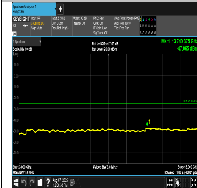
Band41-5MHz-16QAM-40620-1RB#24-3000~18000-PASS
