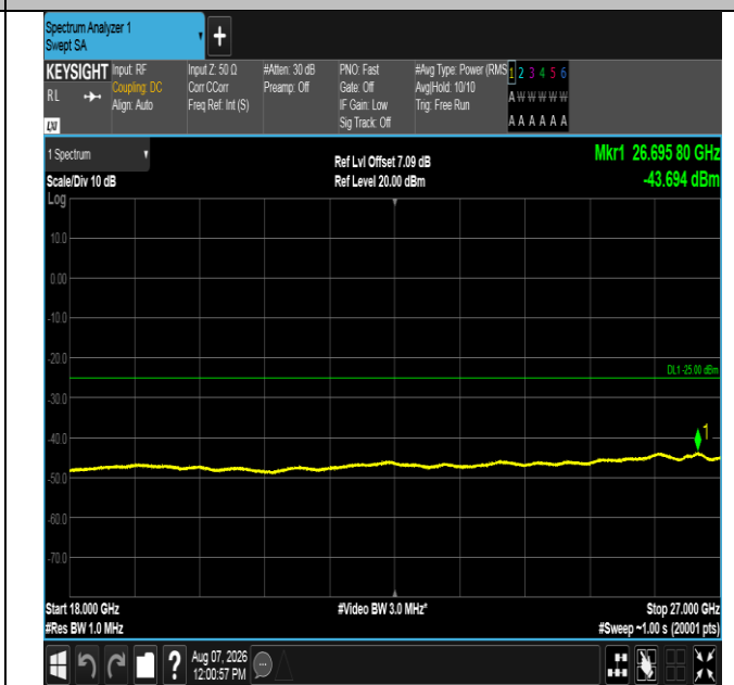
Band41-5MHz-16QAM-39675-25RB#0-18000~27000-PASS
