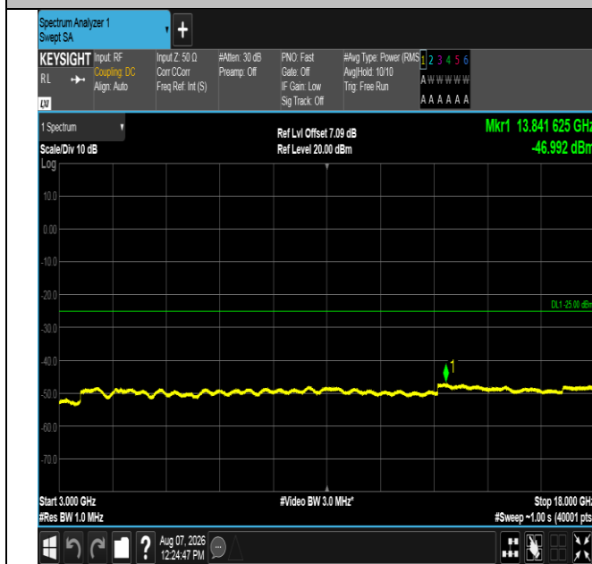
Band41-5MHz-16QAM-41565-25RB#0-3000~18000-PASS
