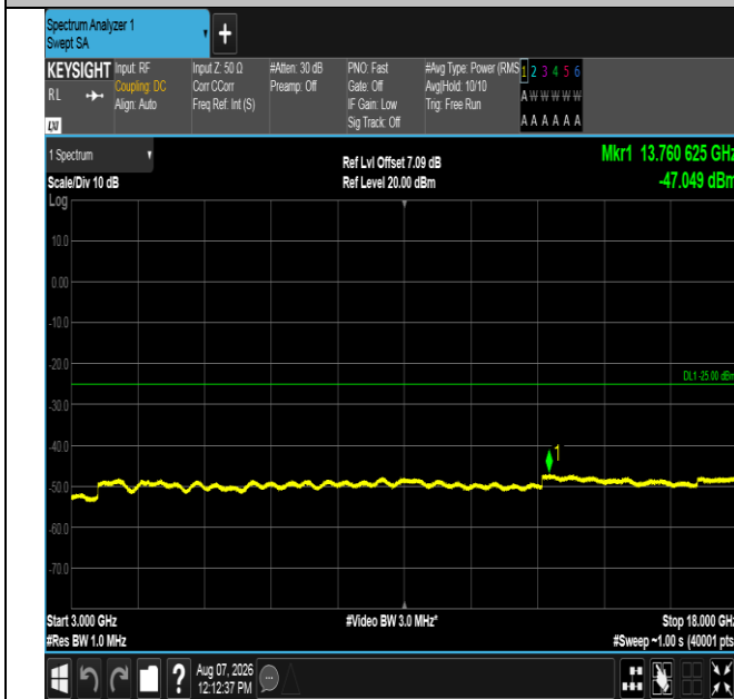
Band41-5MHz-16QAM-40620-25RB#0-3000~18000-PASS
