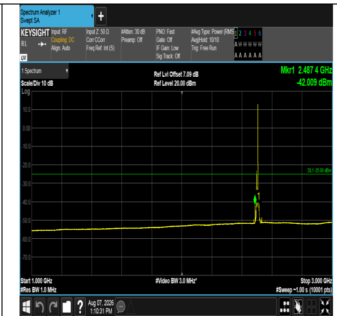
Band41-10MHz-16QAM-39700-1RB#49-1000~3000-PASS
