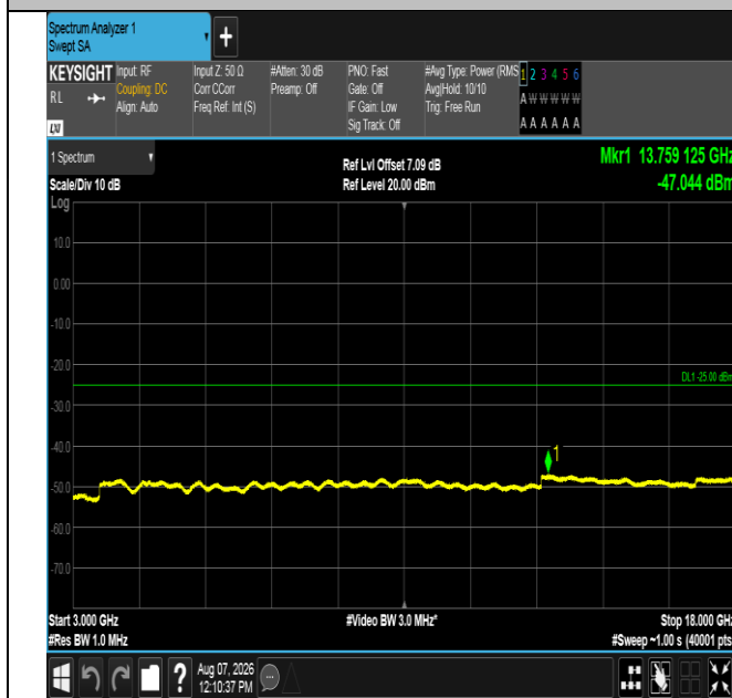
Band41-5MHz-QPSK-40620-25RB#0-3000~18000-PASS
