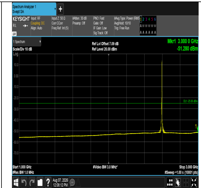
Band41-5MHz-16QAM-40620-1RB#24-1000~3000-PASS
