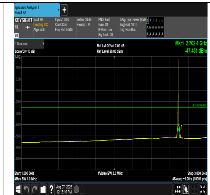
Band41-5MHz-QPSK-41565-1RB#24-1000~3000-PASS
