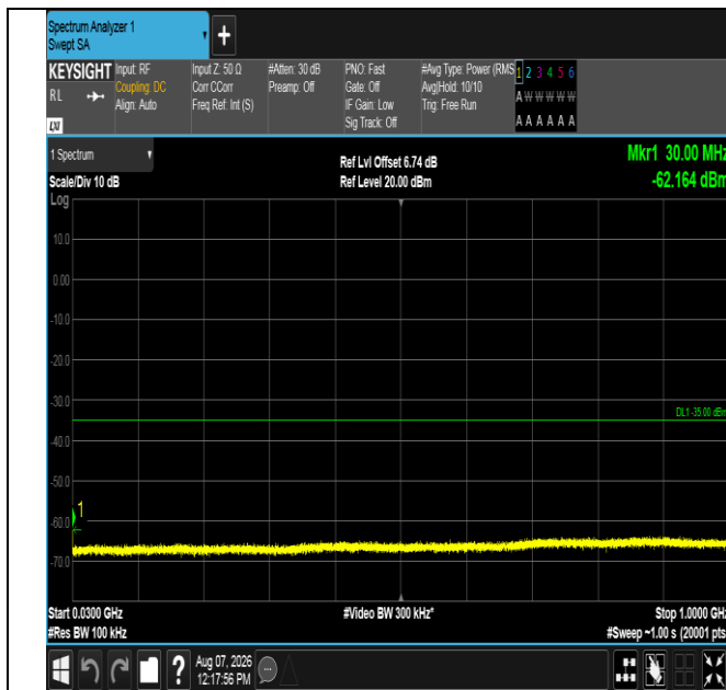
Band41-5MHz-QPSK-41565-1RB#24-30~1000-PASS
