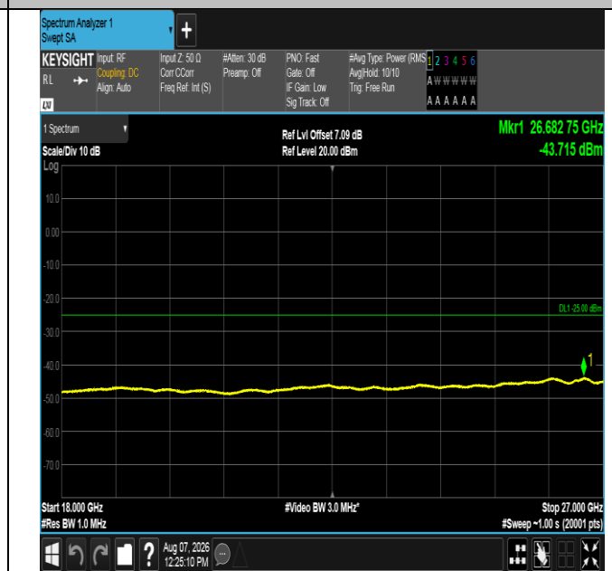
Band41-5MHz-16QAM-41565-25RB#0-18000~27000-PASS
