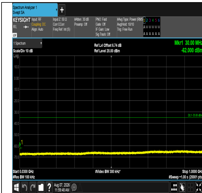
Band41-5MHz-16QAM-39675-25RB#0-30~1000-PASS
