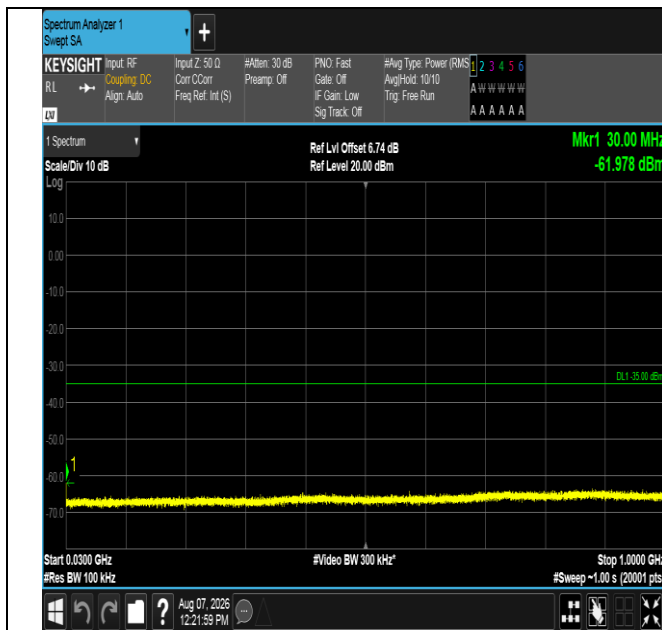
Band41-5MHz-QPSK-41565-25RB#0-30~1000-PASS
