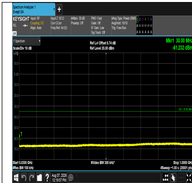
Band41-5MHz-16QAM-41565-1RB#24-30~1000-PASS
