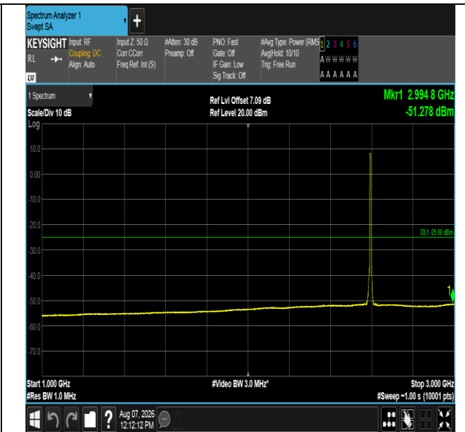
Band41-5MHz-16QAM-40620-25RB#0-1000~3000-PASS
