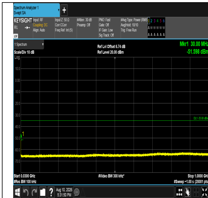
Band41-10MHz-QPSK-39700-50RB#0-30~1000-PASS
