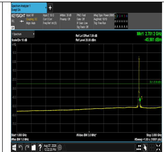
Band41-5MHz-QPSK-41565-25RB#0-1000~3000-PASS
