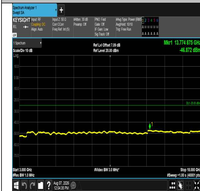
Band41-5MHz-16QAM-40620-1RB#0-3000~18000-PASS
