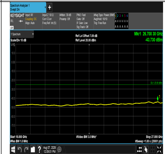
Band41-5MHz-16QAM-40620-1RB#24-18000~27000-PASS
