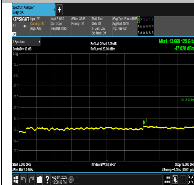
Band41-5MHz-16QAM-39675-25RB#0-3000~18000-PASS
