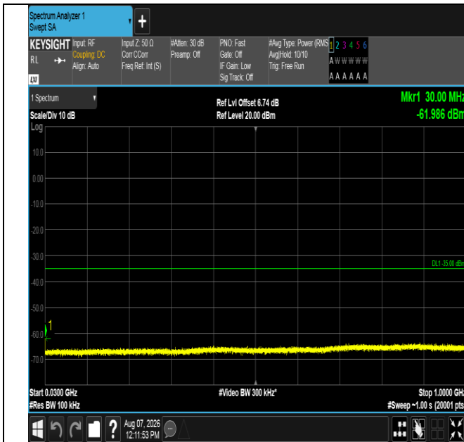
Band41-5MHz-16QAM-40620-25RB#0-30~1000-PASS
