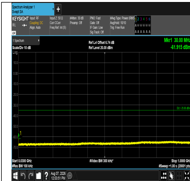
Band41-5MHz-16QAM-40620-1RB#0-30~1000-PASS
