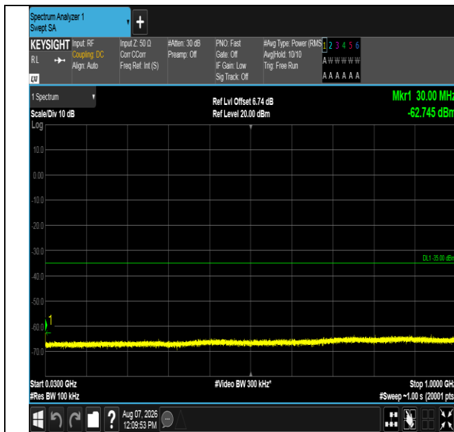
Band41-5MHz-QPSK-40620-25RB#0-30~1000-PASS
