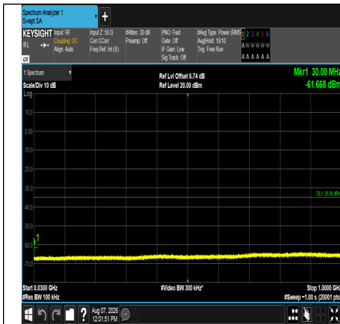
Band41-5MHz-QPSK-40620-1RB#0-30~1000-PASS
