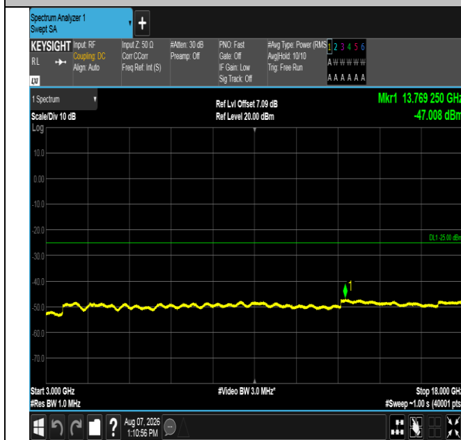
Band41-10MHz-16QAM-39700-1RB#49-3000~18000-PASS
