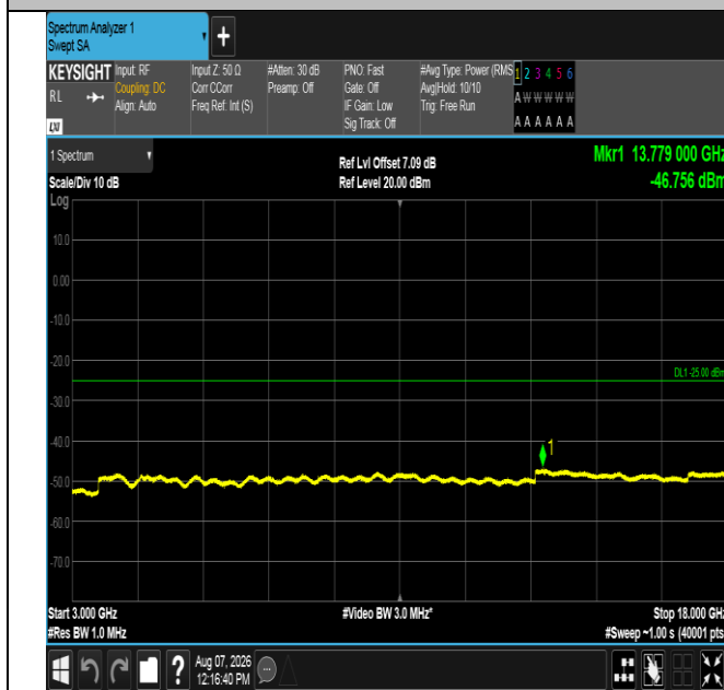
Band41-5MHz-16QAM-41565-1RB#0-3000~18000-PASS
