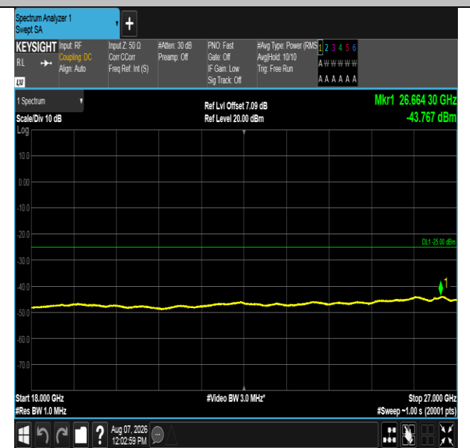
Band41-5MHz-QPSK-40620-1RB#0-18000~27000-PASS
