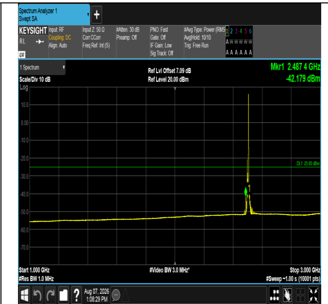
Band41-10MHz-QPSK-39700-1RB#49-1000~3000-PASS
