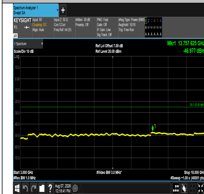
Band41-5MHz-QPSK-41565-1RB#24-3000~18000-PASS
