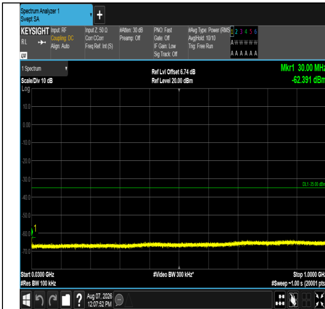
Band41-5MHz-16QAM-40620-1RB#24-30~1000-PASS
