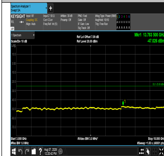
Band41-5MHz-16QAM-41565-1RB#24-3000~18000-PASS
