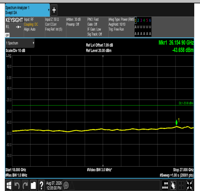
Band41-5MHz-16QAM-40620-1RB#0-18000~27000-PASS
