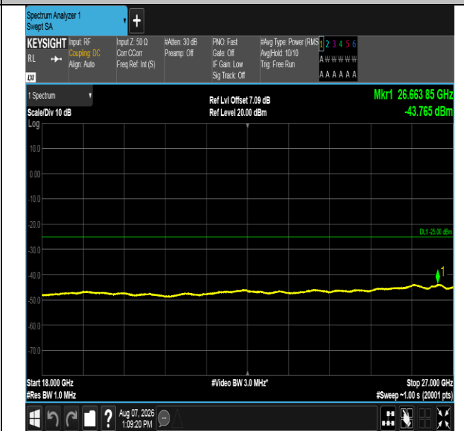
Band41-10MHz-QPSK-39700-1RB#49-18000~27000-PASS
