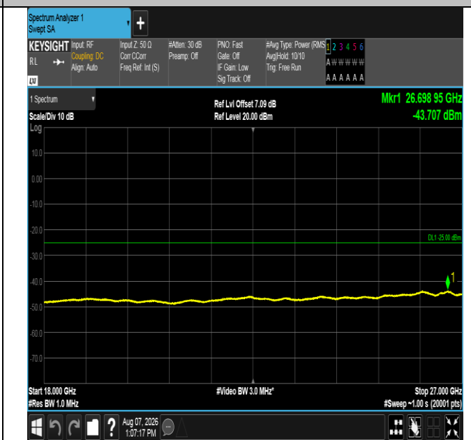
Band41-10MHz-16QAM-39700-1RB#0-18000~27000-PASS
