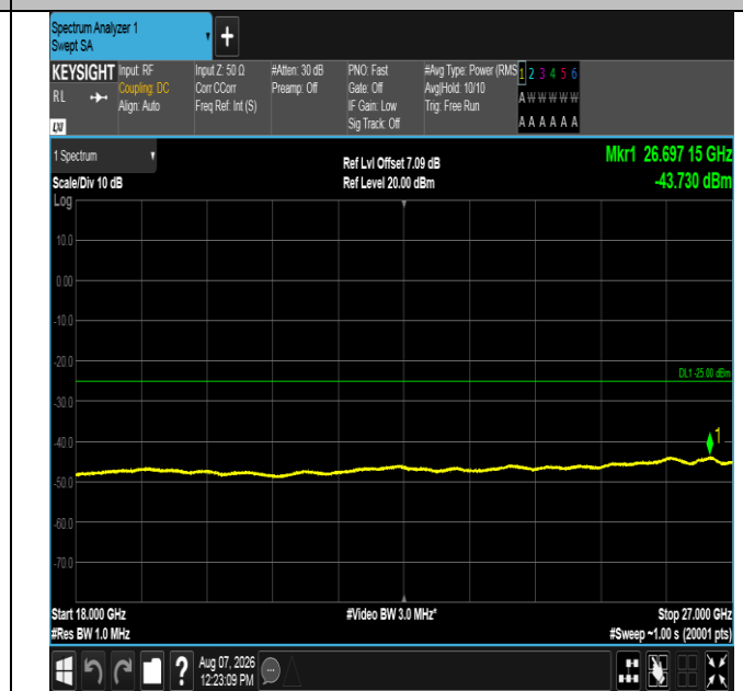
Band41-5MHz-QPSK-41565-25RB#0-18000~27000-PASS
