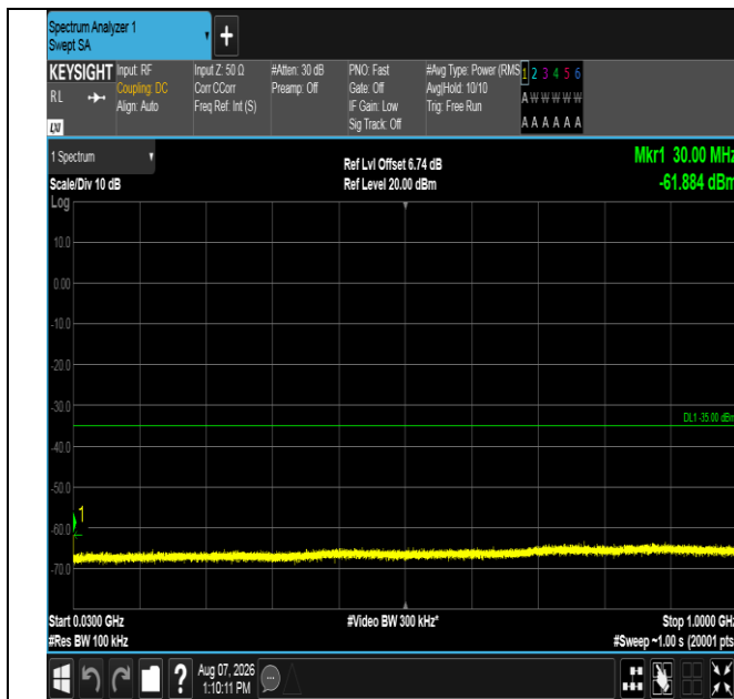
Band41-10MHz-16QAM-39700-1RB#49-30~1000-PASS
