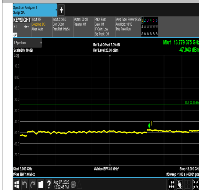
Band41-5MHz-QPSK-41565-25RB#0-3000~18000-PASS
