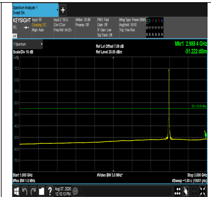
Band41-5MHz-QPSK-40620-25RB#0-1000~3000-PASS
