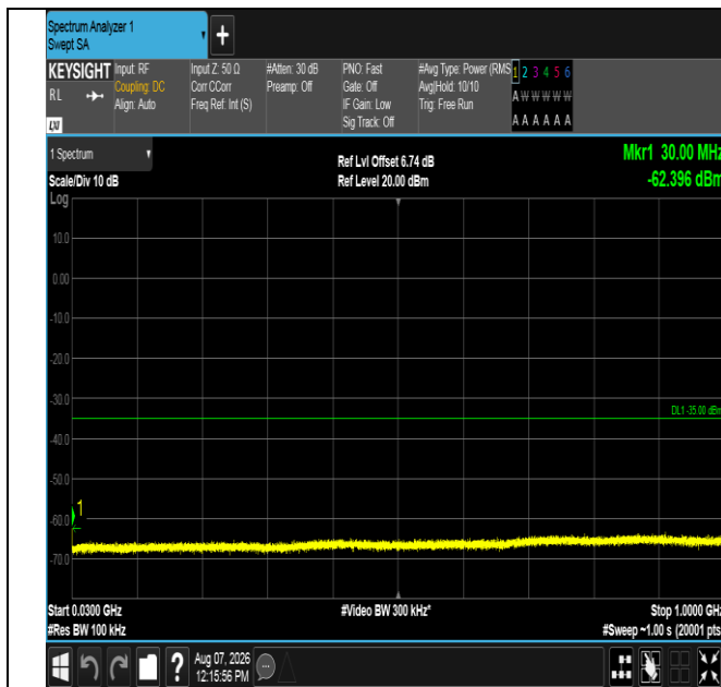
Band41-5MHz-16QAM-41565-1RB#0-30~1000-PASS
