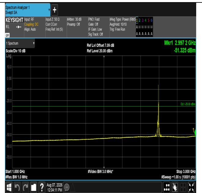
Band41-5MHz-16QAM-40620-1RB#0-1000~3000-PASS
