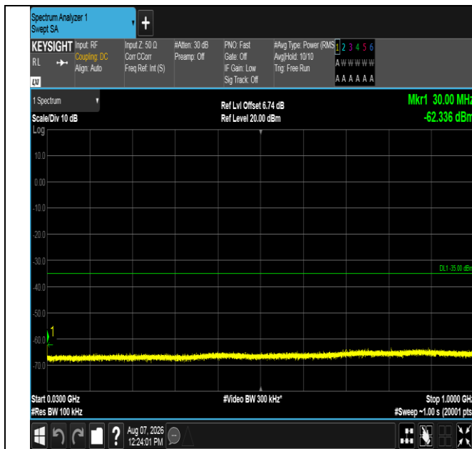
Band41-5MHz-16QAM-41565-25RB#0-30~1000-PASS
