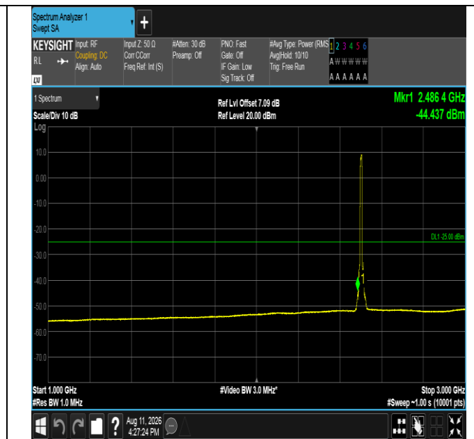
Band41-10MHz-16QAM-39700-50RB#0-1000~3000-PASS
