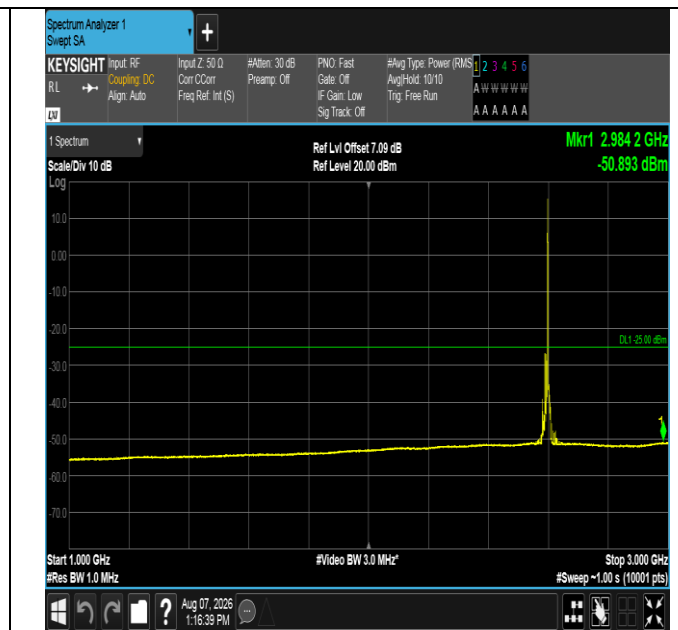
Band41-10MHz-QPSK-40620-1RB#49-1000~3000-PASS
