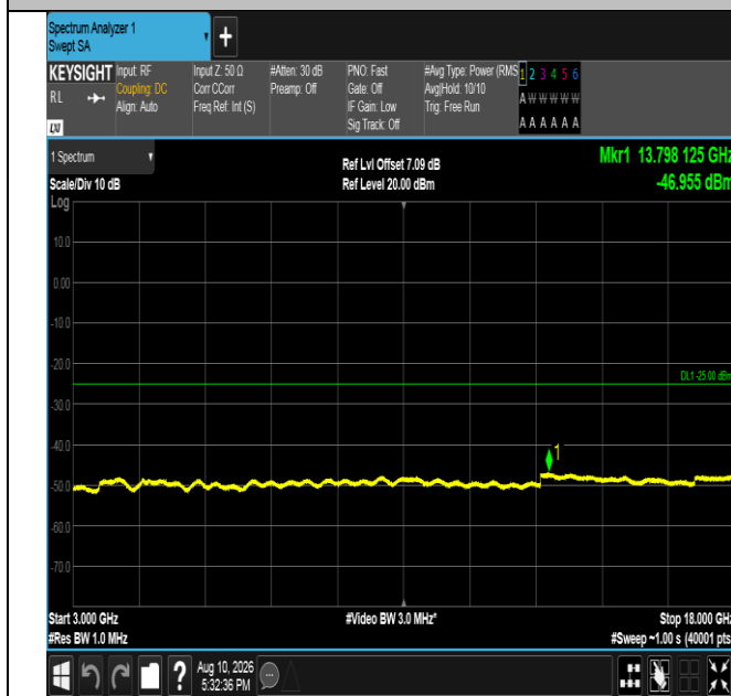
Band41-10MHz-QPSK-39700-50RB#0-3000~18000-PASS
