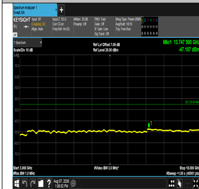
Band41-10MHz-16QAM-39700-1RB#0-3000~18000-PASS
