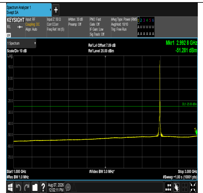
Band41-5MHz-QPSK-40620-1RB#0-1000~3000-PASS
