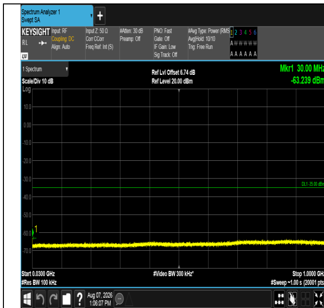
Band41-10MHz-16QAM-39700-1RB#0-30~1000-PASS
