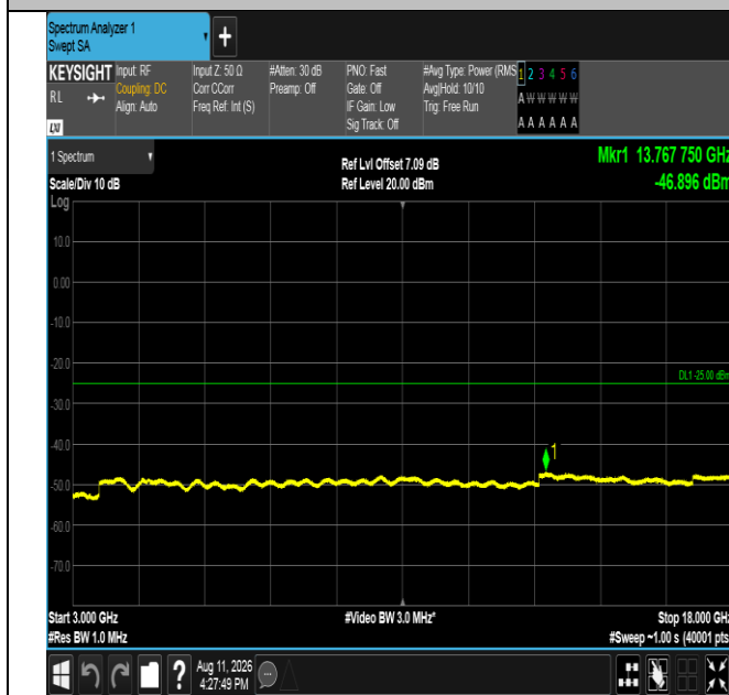
Band41-10MHz-16QAM-39700-50RB#0-3000~18000-PASS
