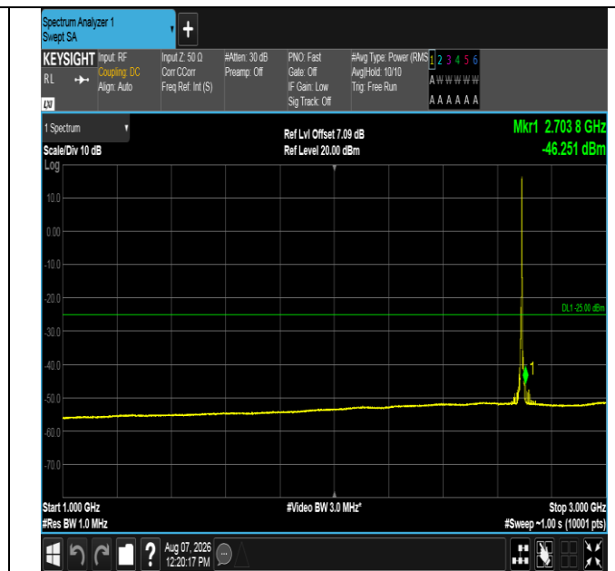
Band41-5MHz-16QAM-41565-1RB#24-1000~3000-PASS
