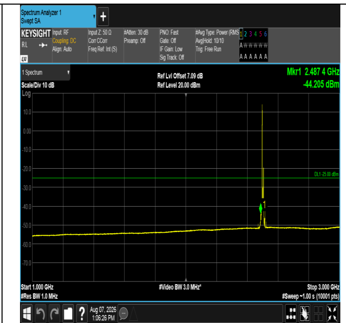
Band41-10MHz-16QAM-39700-1RB#0-1000~3000-PASS
