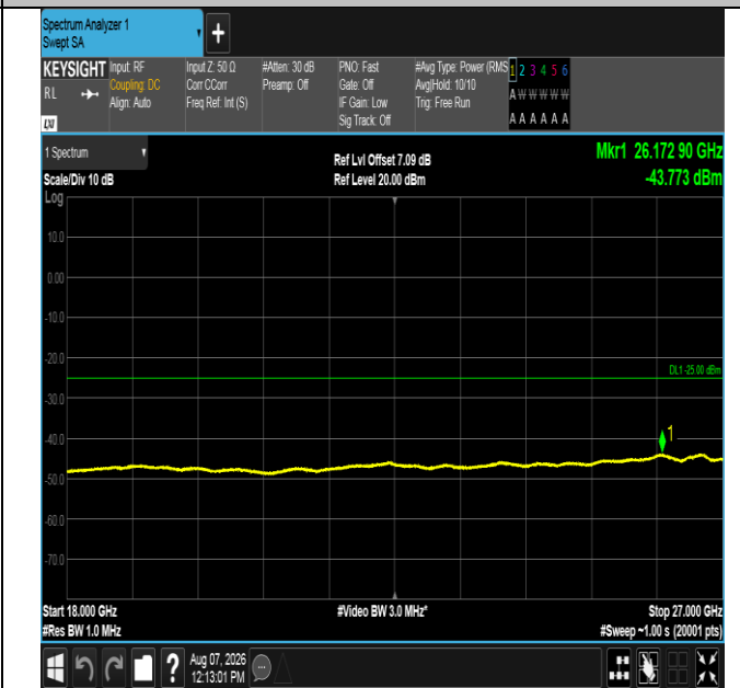
Band41-5MHz-16QAM-40620-25RB#0-18000~27000-PASS
