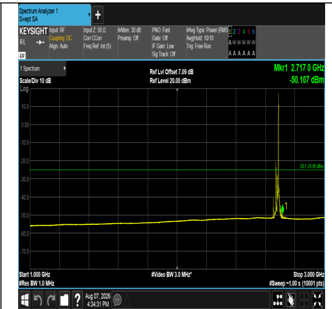
Band41-20MHz-QPSK-41490-1RB#99-1000~3000-PASS
