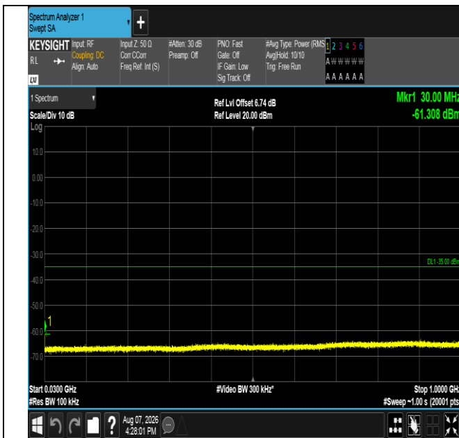
Band41-20MHz-16QAM-40620-1RB#99-30~1000-PASS
