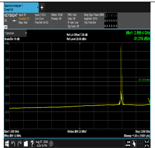
Band41-20MHz-16QAM-40620-1RB#0-1000~3000-PASS
