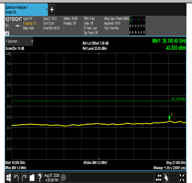
Band41-20MHz-16QAM-40620-1RB#0-18000~27000-PASS
