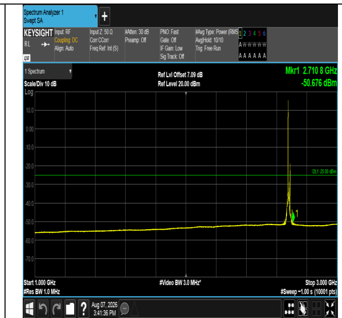
Band41-15MHz-QPSK-41515-1RB#0-1000~3000-PASS
