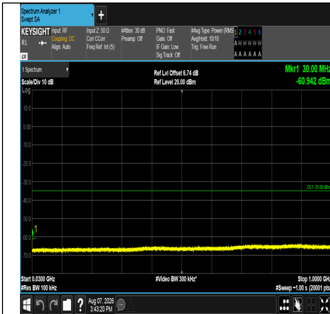
Band41-15MHz-16QAM-41515-1RB#0-30~1000-PASS
