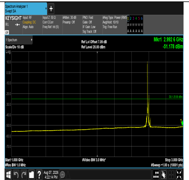
Band41-20MHz-QPSK-40620-1RB#0-1000~3000-PASS
