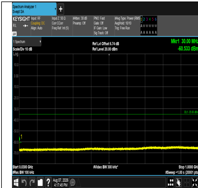
Band41-20MHz-QPSK-39750-1RB#99-30~1000-PASS
