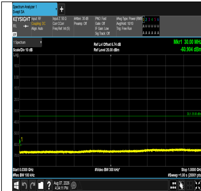
Band41-20MHz-QPSK-41490-1RB#99-30~1000-PASS
