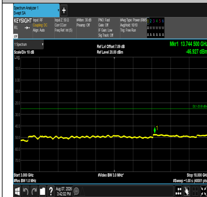
Band41-15MHz-QPSK-41515-1RB#0-3000~18000-PASS
