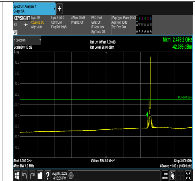
Band41-20MHz-QPSK-39750-1RB#99-1000~3000-PASS
