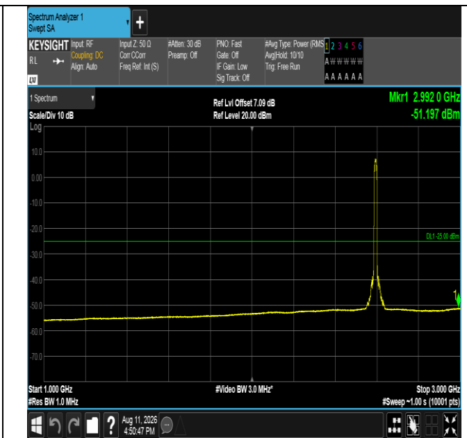
Band41-15MHz-16QAM-40620-75RB#0-1000~3000-PASS
