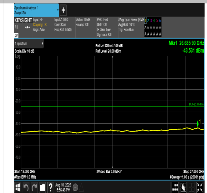
Band41-20MHz-QPSK-40620-100RB#0-18000~27000-PASS
