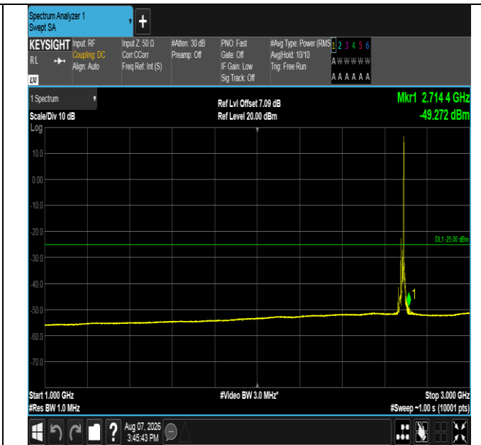
Band41-15MHz-QPSK-41515-1RB#74-1000~3000-PASS
