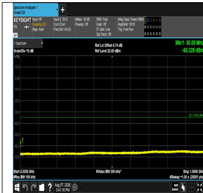
Band41-15MHz-QPSK-41515-1RB#0-30~1000-PASS
