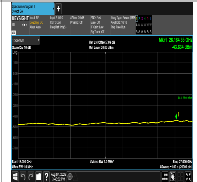
Band41-15MHz-QPSK-41515-1RB#74-18000~27000-PASS
