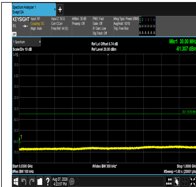
Band41-20MHz-16QAM-40620-1RB#0-30~1000-PASS
