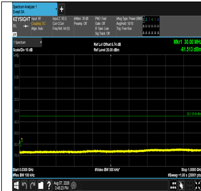
Band41-15MHz-QPSK-41515-1RB#74-30~1000-PASS
