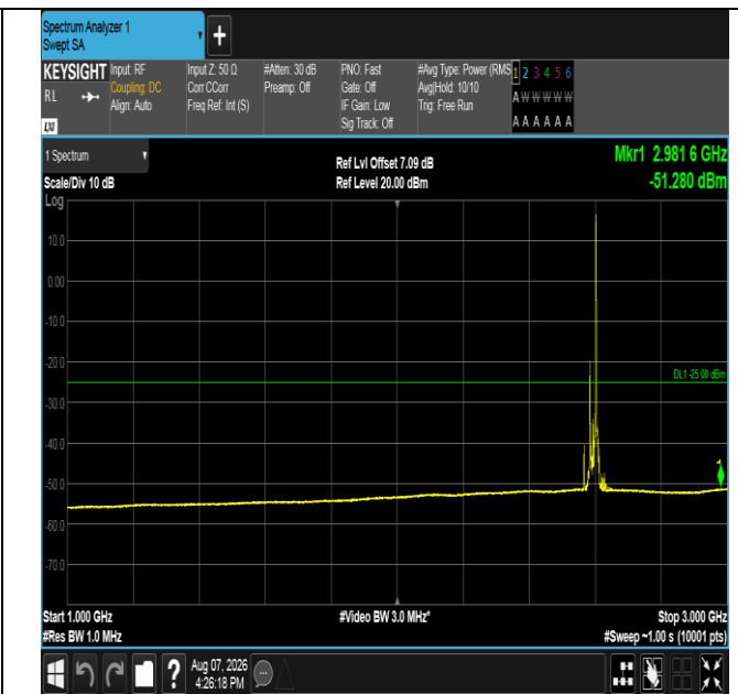
Band41-20MHz-QPSK-40620-1RB#99-1000~3000-PASS
