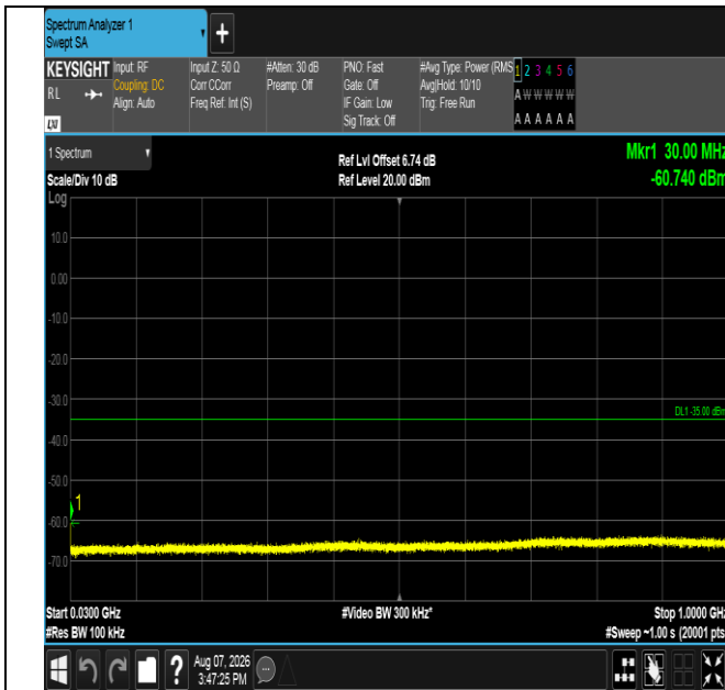
Band41-15MHz-16QAM-41515-1RB#74-30~1000-PASS
