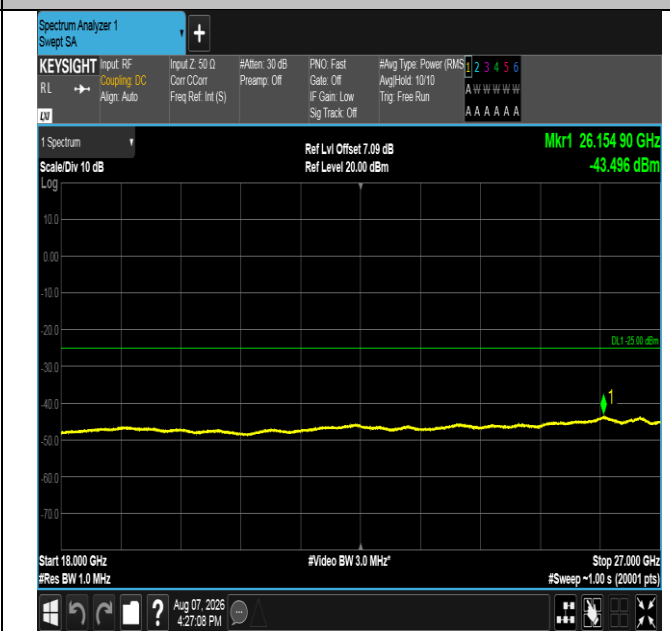
Band41-20MHz-QPSK-40620-1RB#99-18000~27000-PASS
