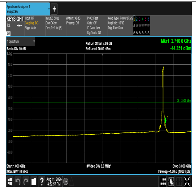
Band41-15MHz-16QAM-41515-75RB#0-1000~3000-PASS
