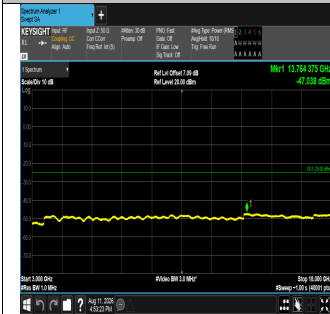
Band41-15MHz-16QAM-41515-75RB#0-3000~18000-PASS
