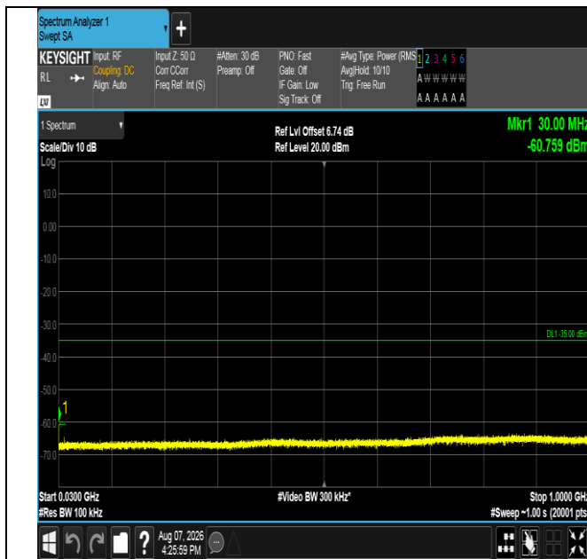
Band41-20MHz-QPSK-40620-1RB#99-30~1000-PASS
