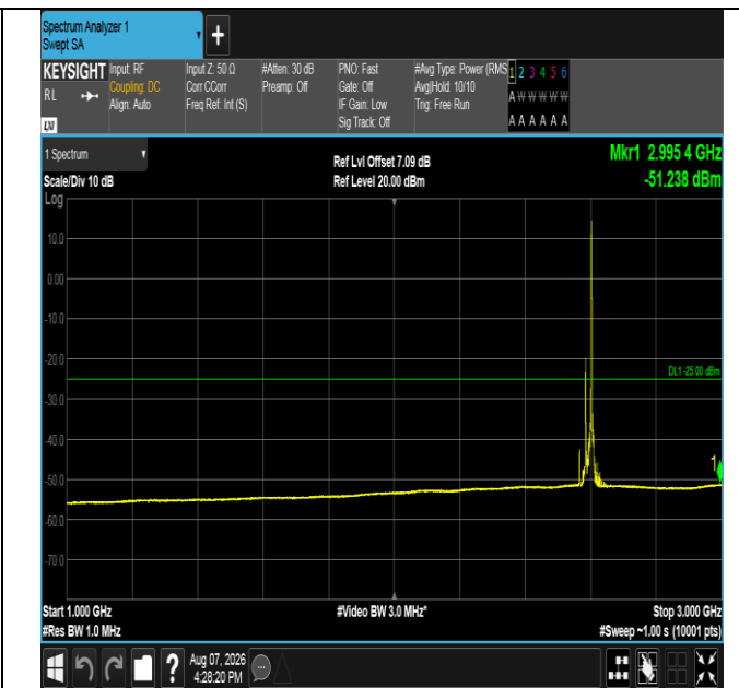
Band41-20MHz-16QAM-40620-1RB#99-1000~3000-PASS
