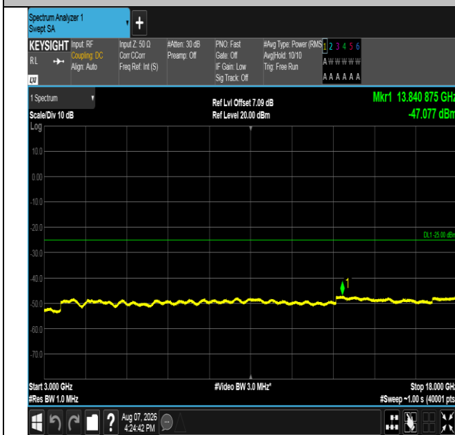
Band41-20MHz-16QAM-40620-1RB#0-3000~18000-PASS
