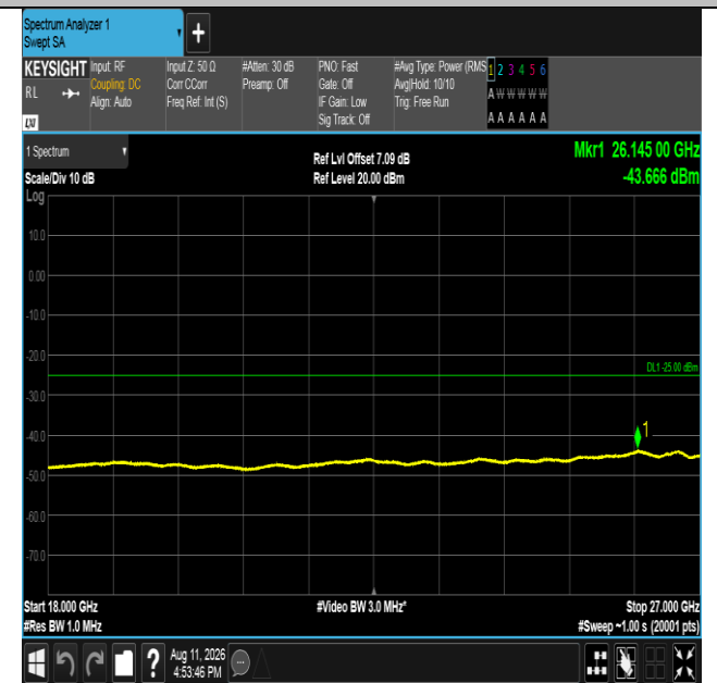
Band41-15MHz-16QAM-41515-75RB#0-18000~27000-PASS
