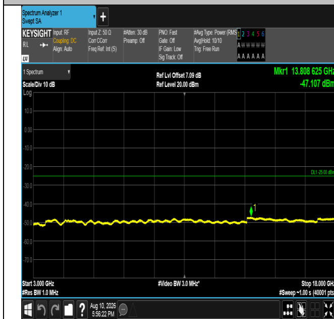
Band41-20MHz-QPSK-40620-100RB#0-3000~18000-PASS
