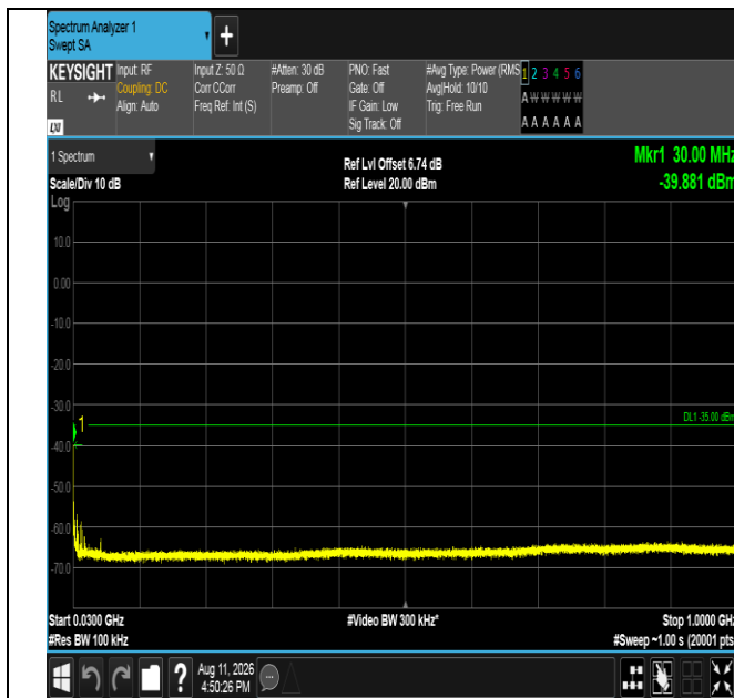
Band41-15MHz-16QAM-40620-75RB#0-30~1000-PASS
