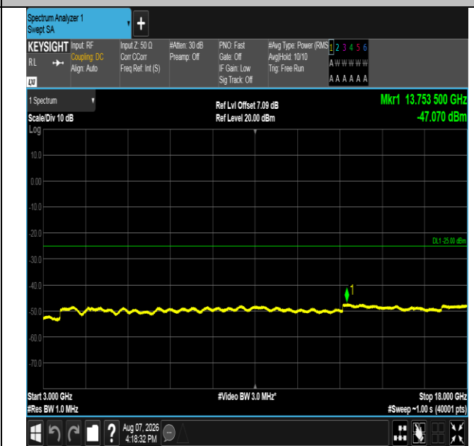
Band41-20MHz-QPSK-39750-1RB#99-3000~18000-PASS
