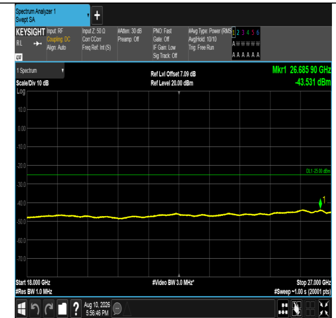
Band41-20MHz-QPSK-40620-100RB#0-18000~27000-PASS
