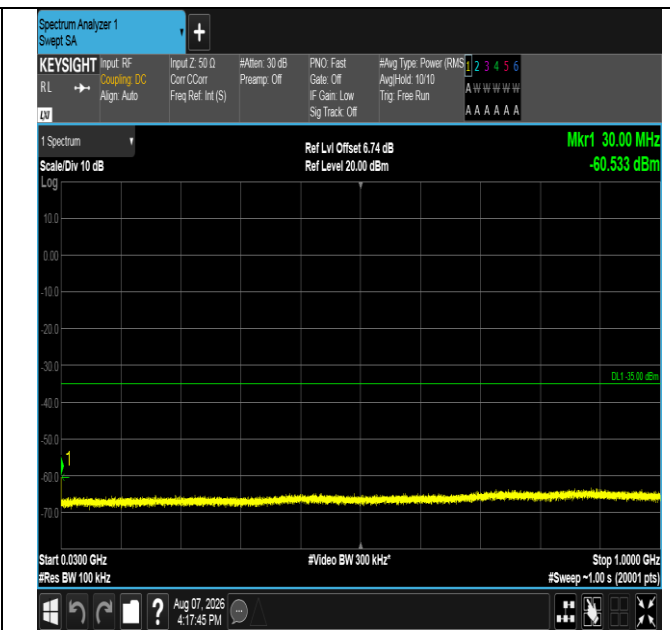
Band41-20MHz-QPSK-39750-1RB#99-30~1000-PASS
