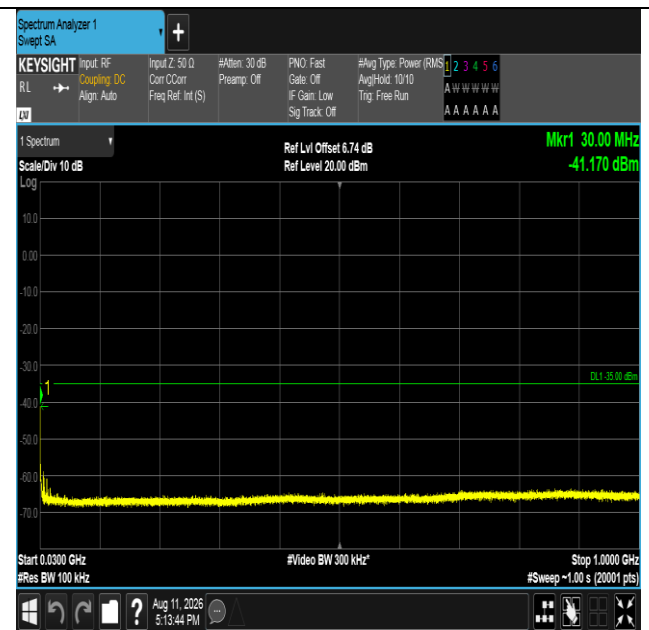
Band41-20MHz-16QAM-40620-100RB#0-30~1000-PASS
