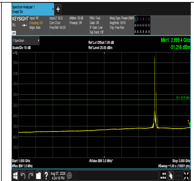
Band41-20MHz-16QAM-40620-1RB#0-1000~3000-PASS
