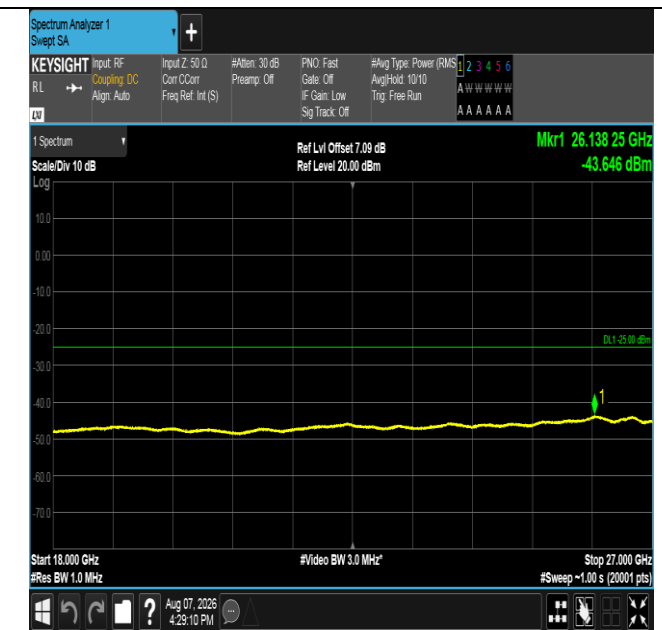
Band41-20MHz-16QAM-40620-1RB#99-18000~27000-PASS
