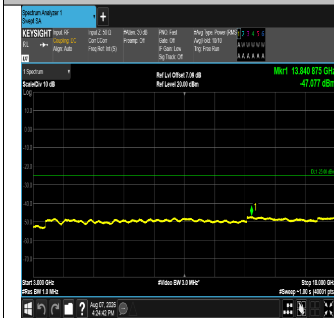
Band41-20MHz-16QAM-40620-1RB#0-3000~18000-PASS
