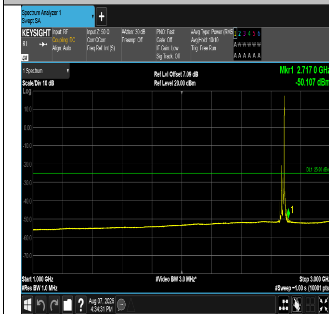
Band41-20MHz-QPSK-41490-1RB#99-1000~3000-PASS
