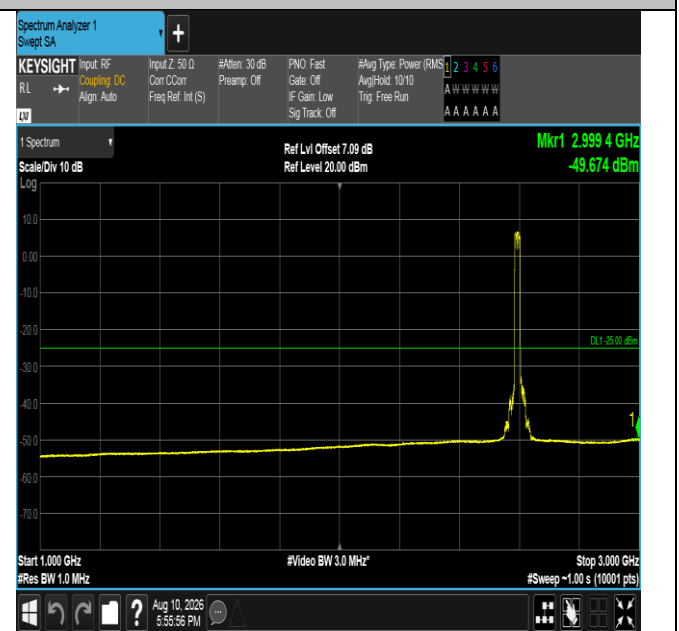
Band41-20MHz-QPSK-40620-100RB#0-1000~3000-PASS
