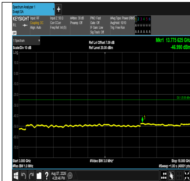
Band41-20MHz-16QAM-40620-1RB#99-3000~18000-PASS
