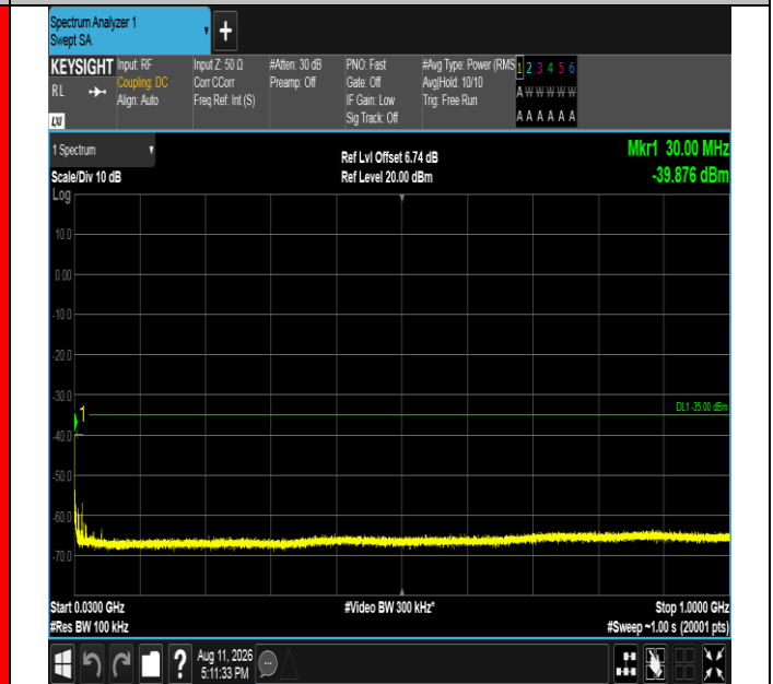
Band41-20MHz-16QAM-39750-100RB#0-30~1000-PASS
