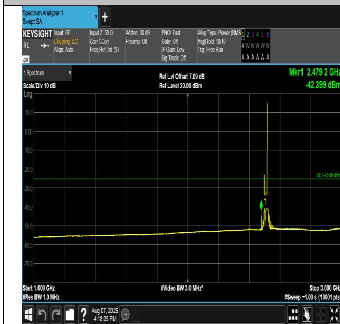
Band41-20MHz-QPSK-39750-1RB#99-1000~3000-PASS
