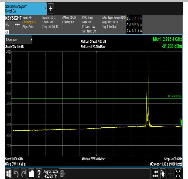
Band41-20MHz-16QAM-40620-1RB#99-1000~3000-PASS
