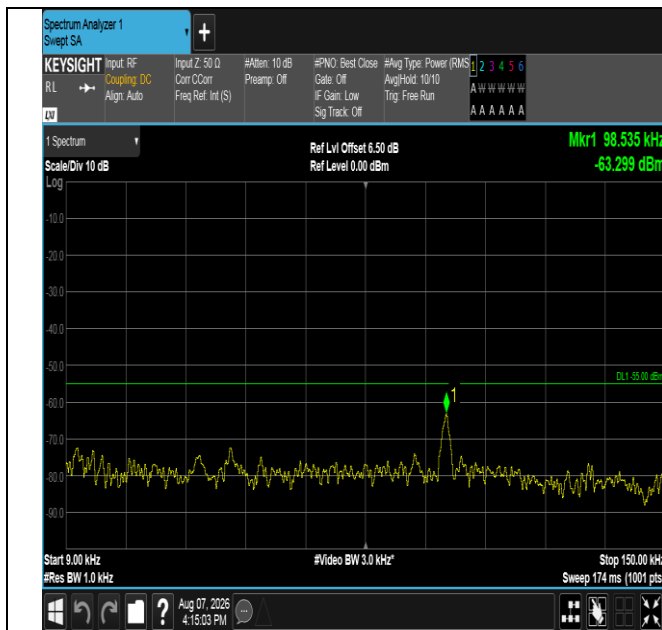
Band41-20MHz-16QAM-39750-1RB#0-0.009~0.15-PASS
