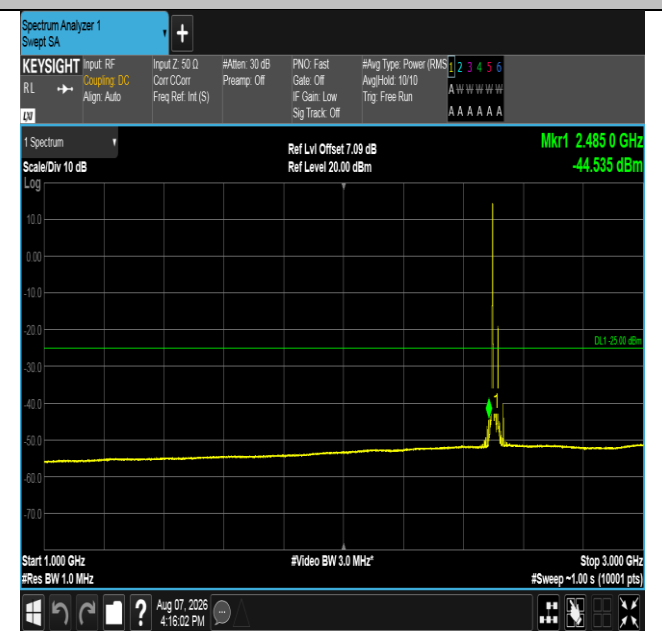
Band41-20MHz-16QAM-39750-1RB#0-1000~3000-PASS
