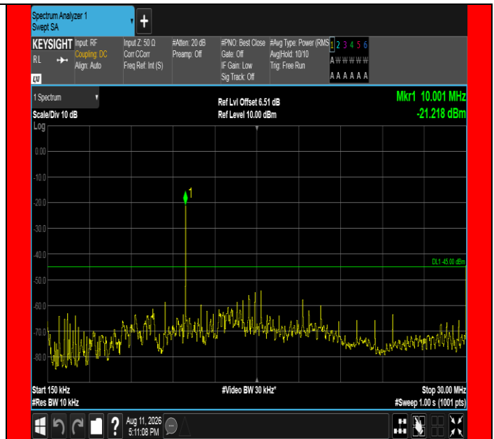
Band41-20MHz-16QAM-39750-100RB#0-0.15~30-FAIL
