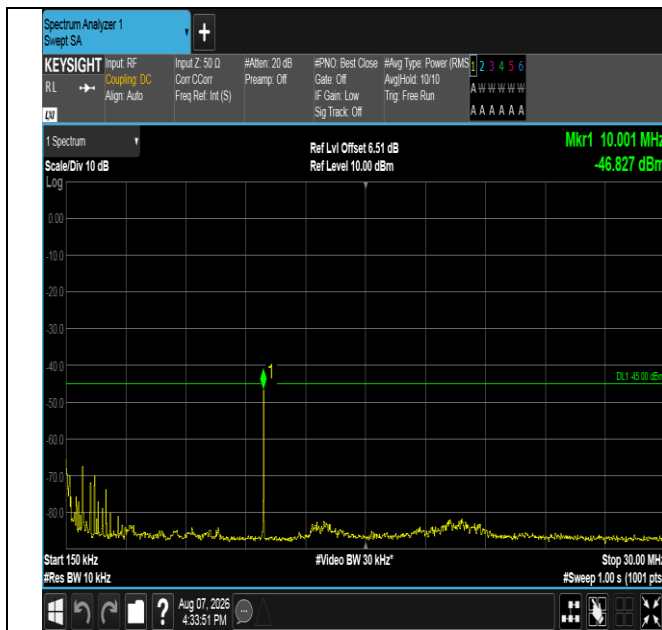
Band41-20MHz-QPSK-41490-1RB#99-0.15~30-PASS
