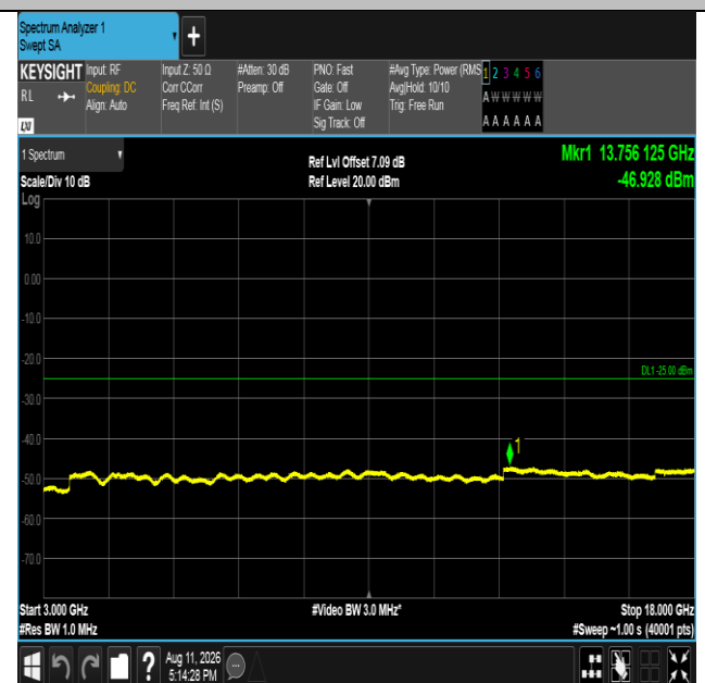
Band41-20MHz-16QAM-40620-100RB#0-3000~18000-PASS
