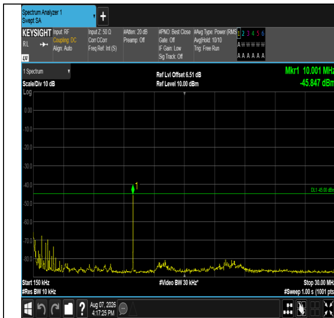
Band41-20MHz-QPSK-39750-1RB#99-0.15~30-PASS
