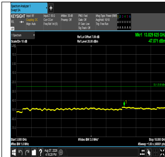
Band41-20MHz-16QAM-39750-1RB#0-3000~18000-PASS
