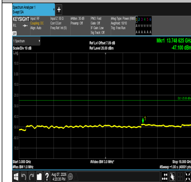
Band41-20MHz-16QAM-39750-1RB#99-3000~18000-PASS
