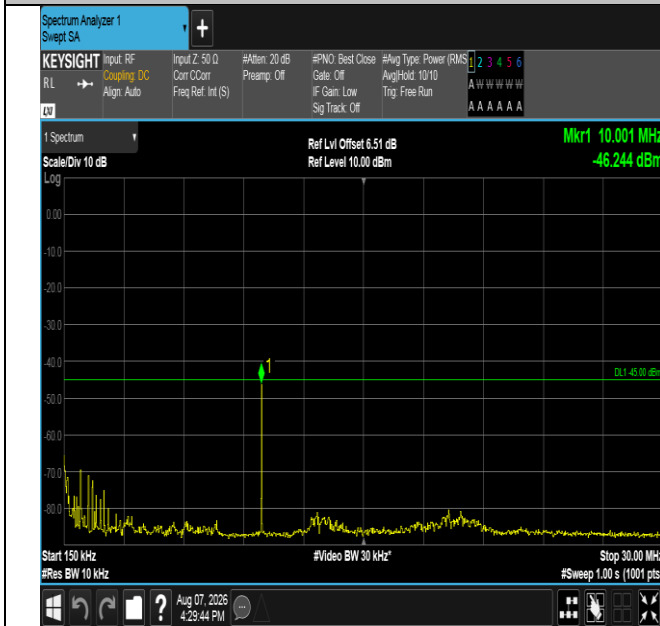
Band41-20MHz-QPSK-41490-1RB#0-0.15~30-PASS
