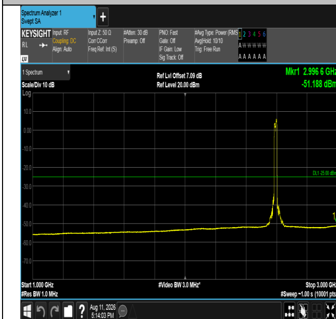
Band41-20MHz-16QAM-40620-100RB#0-1000~3000-PASS
