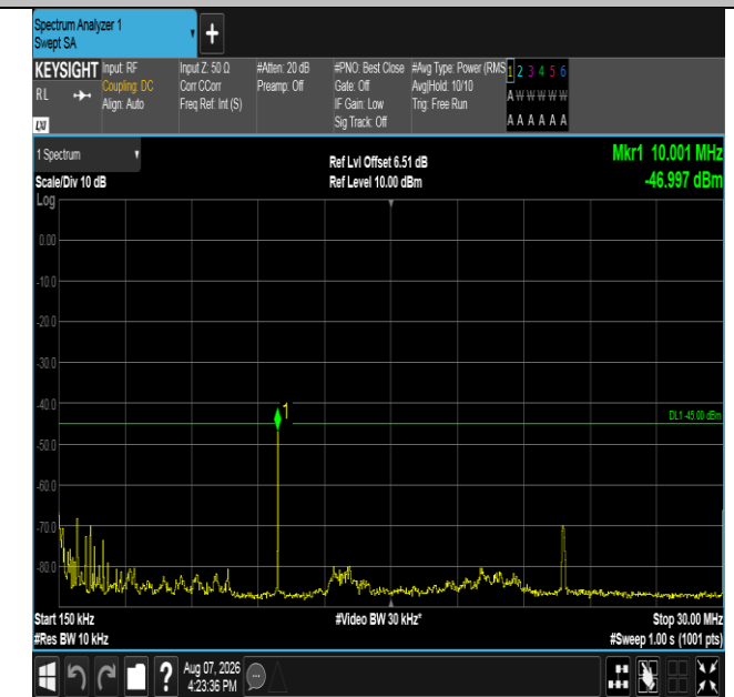
Band41-20MHz-16QAM-40620-1RB#0-0.15~30-PASS
