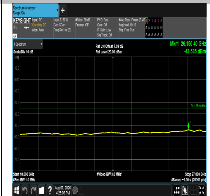
Band41-20MHz-16QAM-40620-1RB#0-18000~27000-PASS
