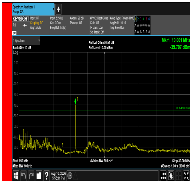
Band41-20MHz-QPSK-40620-100RB#0-0.15~30-FAIL
