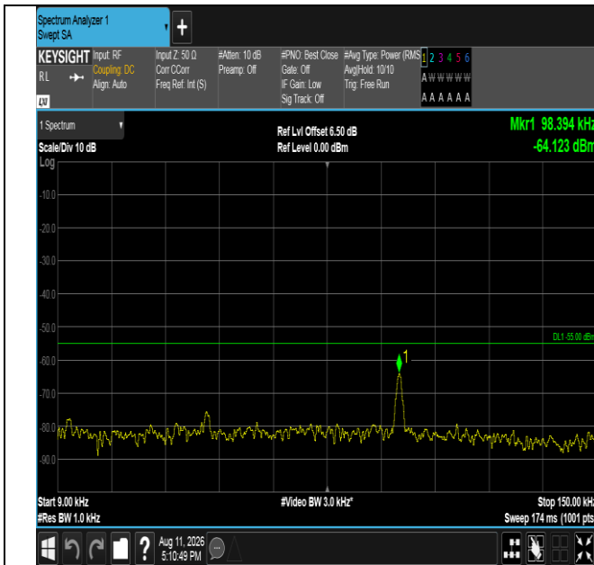
Band41-20MHz-16QAM-39750-100RB#0-0.009~0.15-PASS
