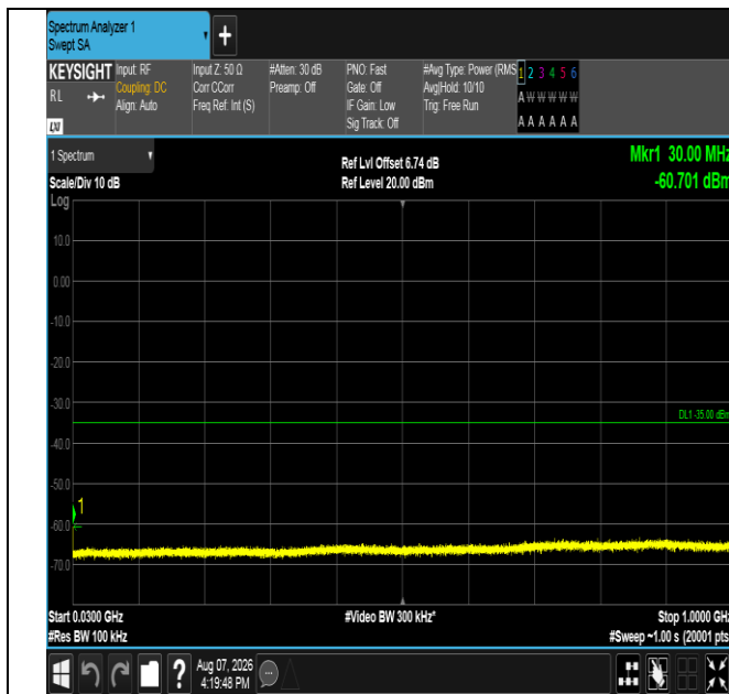
Band41-20MHz-16QAM-39750-1RB#99-30~1000-PASS
