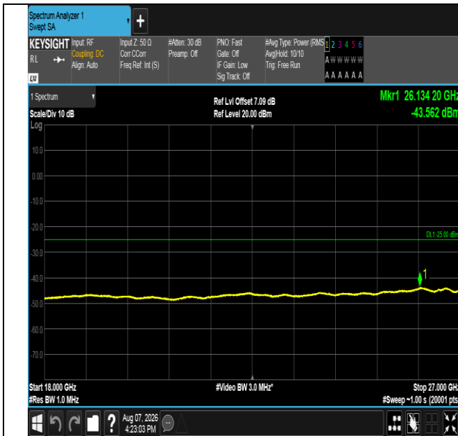
Band41-20MHz-QPSK-40620-1RB#0-18000~27000-PASS
