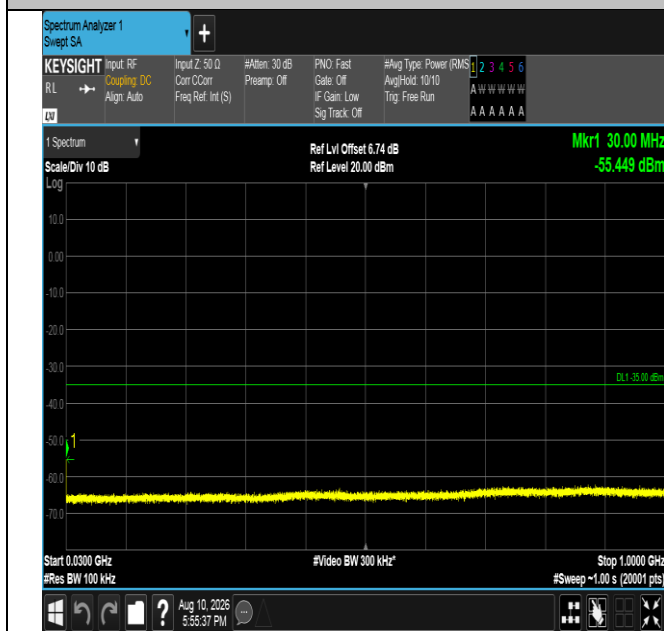
Band41-20MHz-QPSK-40620-100RB#0-30~1000-PASS
