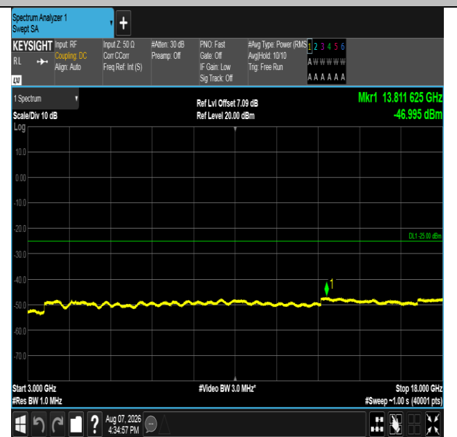
Band41-20MHz-QPSK-41490-1RB#99-3000~18000-PASS
