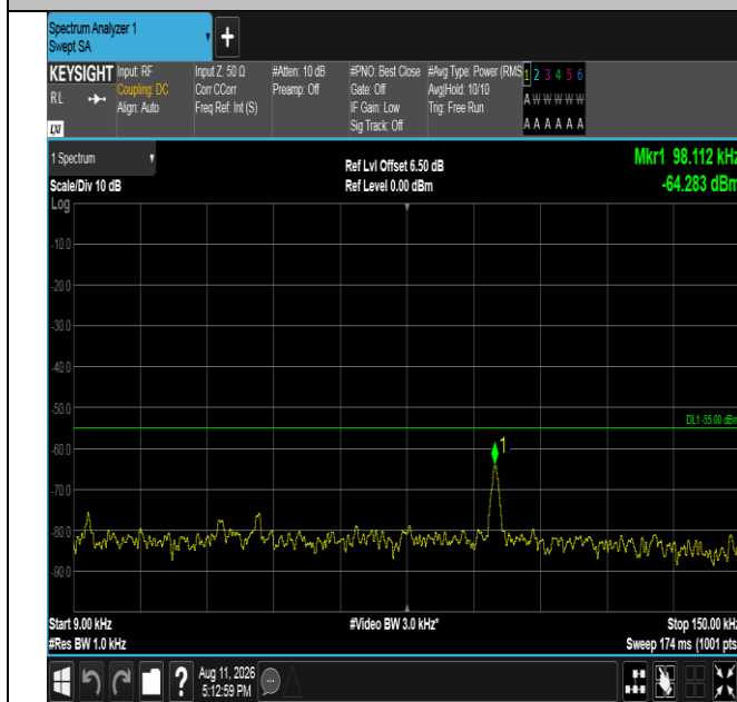
Band41-20MHz-16QAM-40620-100RB#0-0.009~0.15-PASS
