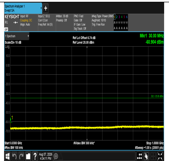
Band41-20MHz-QPSK-41490-1RB#99-30~1000-PASS
