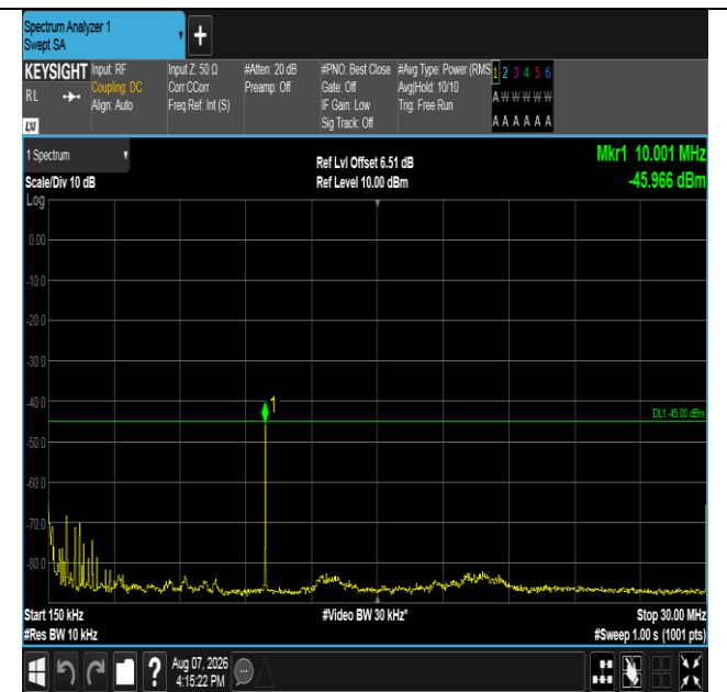
Band41-20MHz-16QAM-39750-1RB#0-0.15~30-PASS
