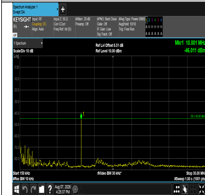
Band41-20MHz-QPSK-40620-1RB#99-0.15~30-PASS
