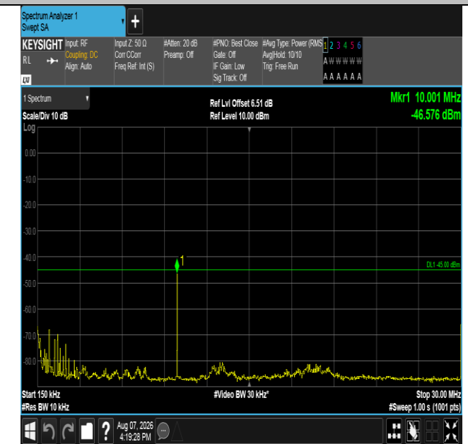
Band41-20MHz-16QAM-39750-1RB#99-0.15~30-PASS
