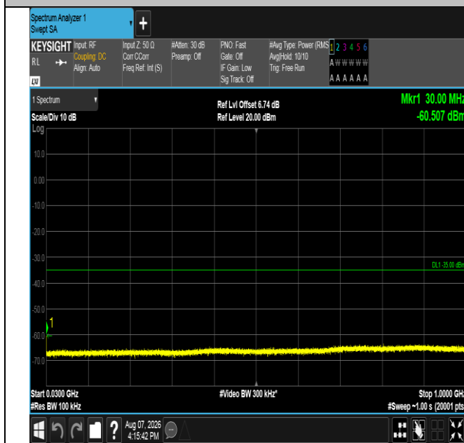
Band41-20MHz-16QAM-39750-1RB#0-30~1000-PASS
