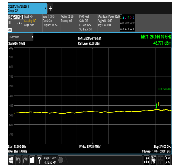
Band41-20MHz-16QAM-39750-1RB#0-18000~27000-PASS
