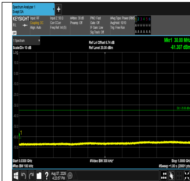
Band41-20MHz-16QAM-40620-1RB#0-30~1000-PASS
