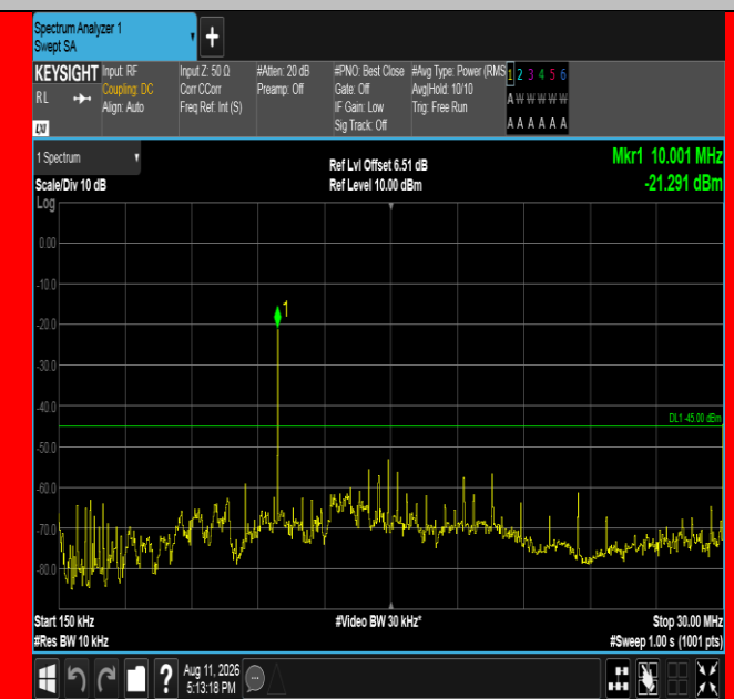
Band41-20MHz-16QAM-40620-100RB#0-0.15~30-FAIL
