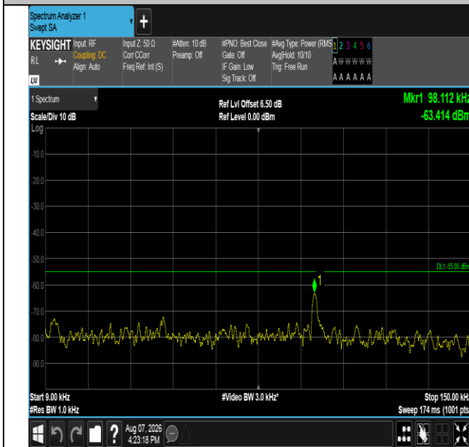
Band41-20MHz-16QAM-40620-1RB#0-0.009~0.15-PASS
