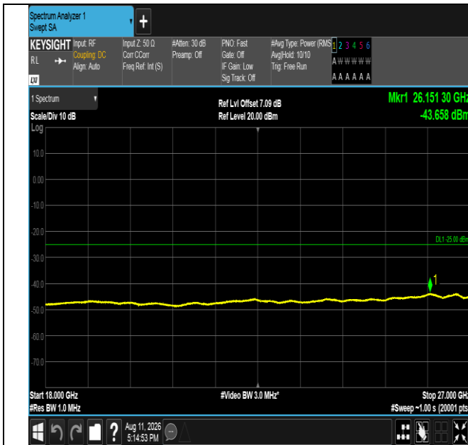
Band41-20MHz-16QAM-40620-100RB#0-18000~27000-PASS
