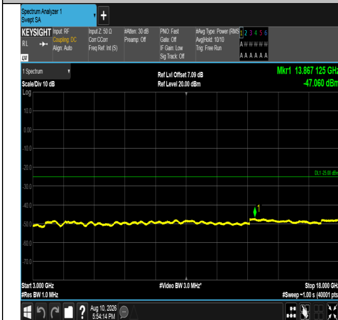
Band41-20MHz-QPSK-39750-100RB#0-3000~18000-PASS
