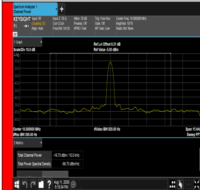
Band41-20MHz-16QAM-41490-100RB#0-0.15~30-FAIL
