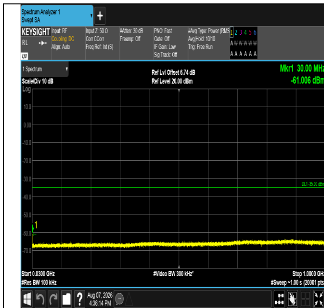
Band41-20MHz-16QAM-41490-1RB#99-30~1000-PASS
