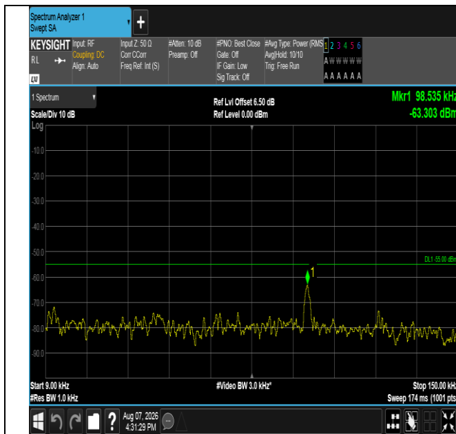
Band41-20MHz-16QAM-41490-1RB#0-0.009~0.15-PASS
