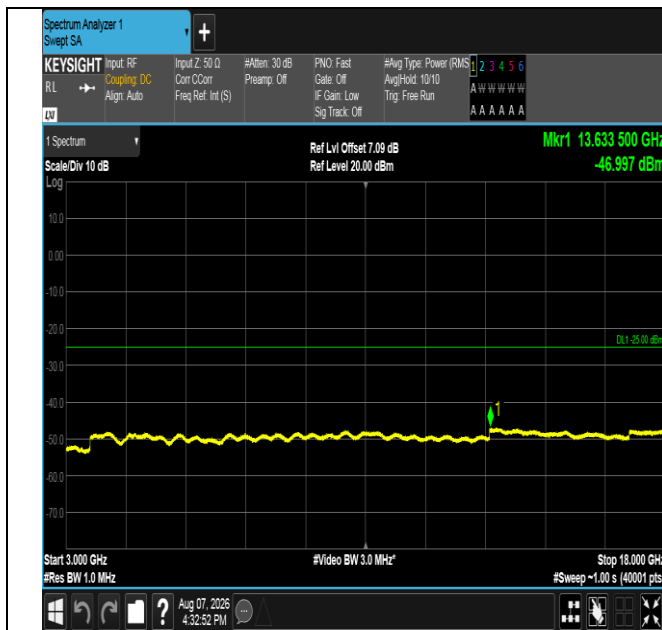
Band41-20MHz-16QAM-41490-1RB#0-3000~18000-PASS
