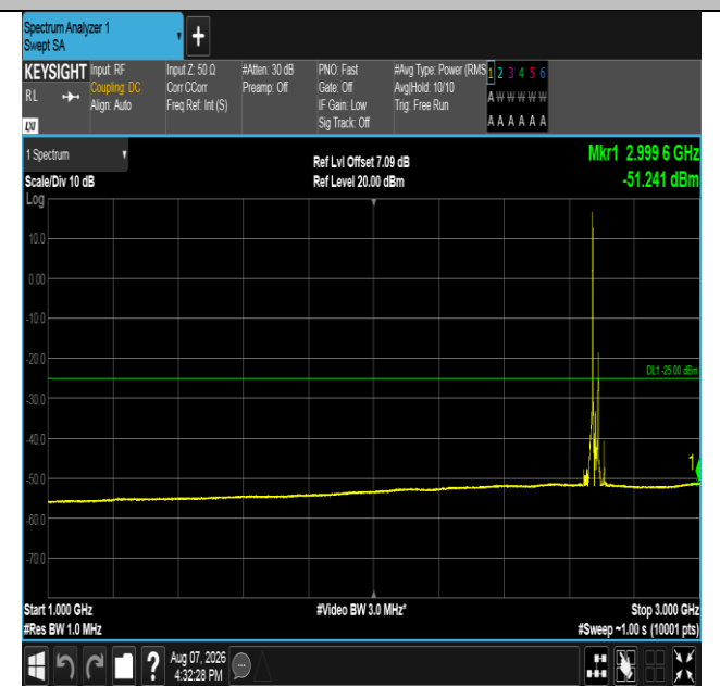
Band41-20MHz-16QAM-41490-1RB#0-1000~3000-PASS
