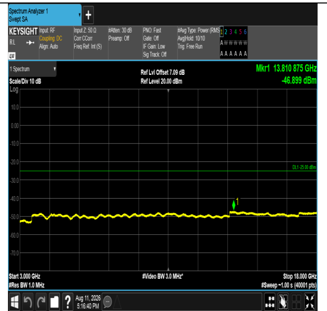
Band41-20MHz-16QAM-41490-100RB#0-3000~18000-PASS
