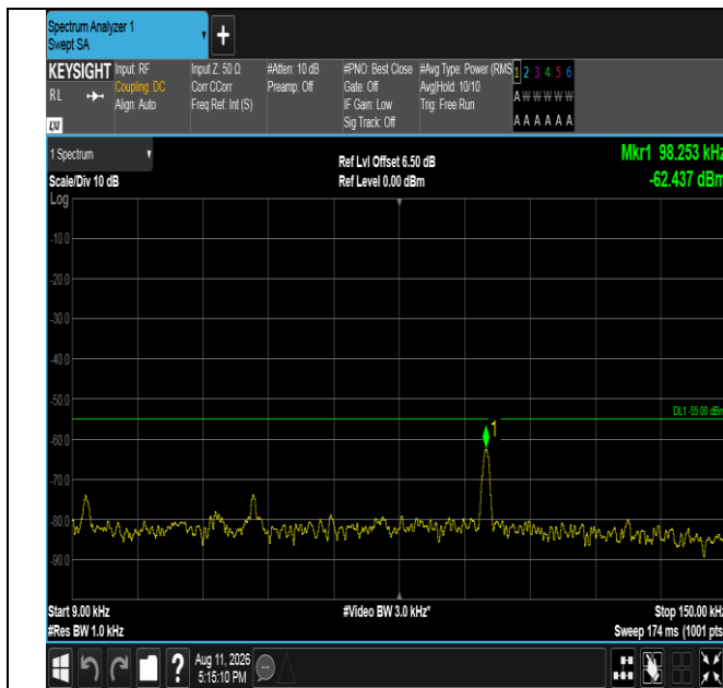
Band41-20MHz-16QAM-41490-100RB#0-0.009~0.15-PASS
