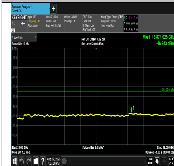
Band41-20MHz-16QAM-41490-1RB#99-3000~18000-PASS
