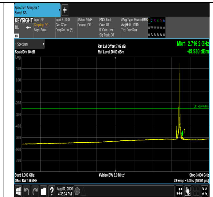
Band41-20MHz-16QAM-41490-1RB#99-1000~3000-PASS
