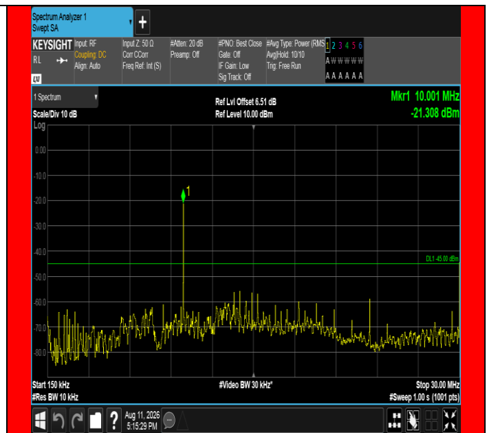
Band41-20MHz-16QAM-41490-100RB#0-0.15~30-FAIL
