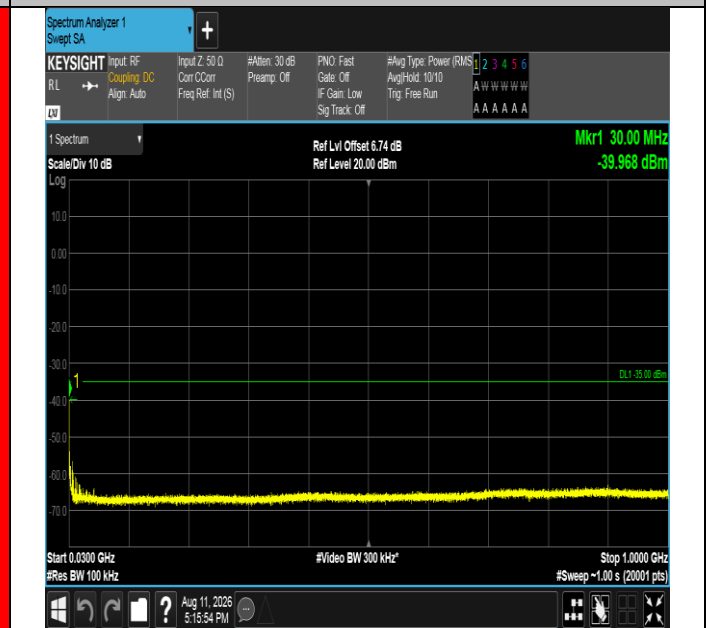
Band41-20MHz-16QAM-41490-100RB#0-30~1000-PASS
