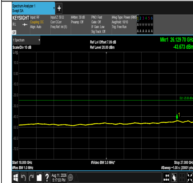
Band41-20MHz-16QAM-41490-100RB#0-18000~27000-PASS
