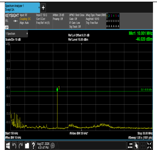
Band41-20MHz-16QAM-41490-1RB#0-0.15~30-PASS
