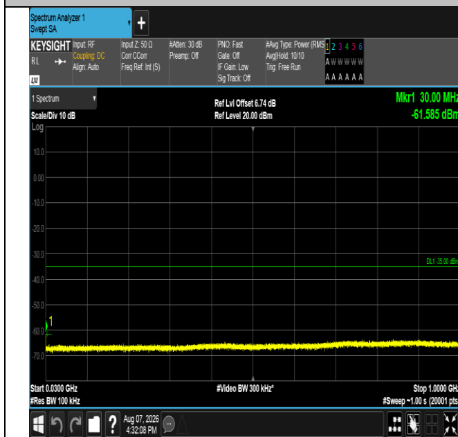
Band41-20MHz-16QAM-41490-1RB#0-30~1000-PASS
