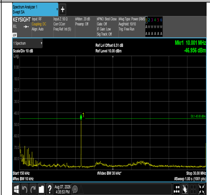
Band41-20MHz-16QAM-41490-1RB#99-0.15~30-PASS
