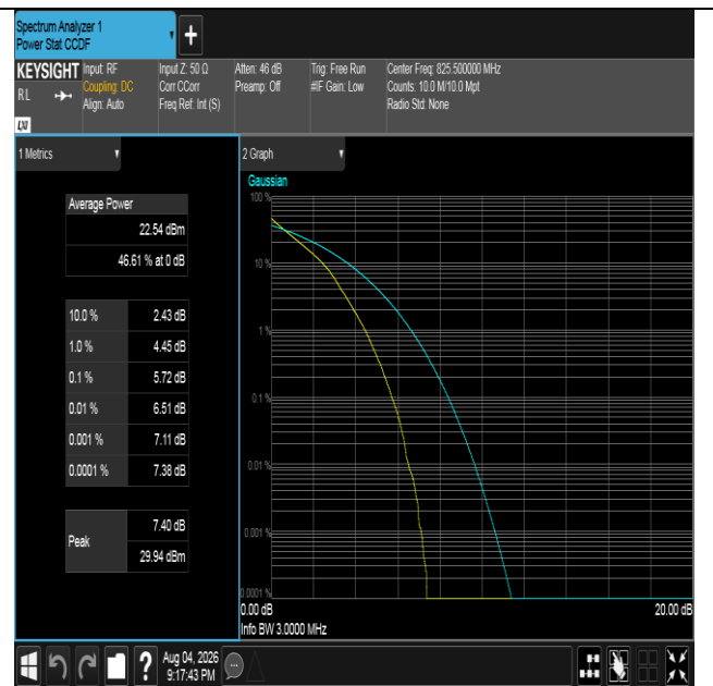
Band5-3MHz-QPSK-20415-15RB#0-PASS
