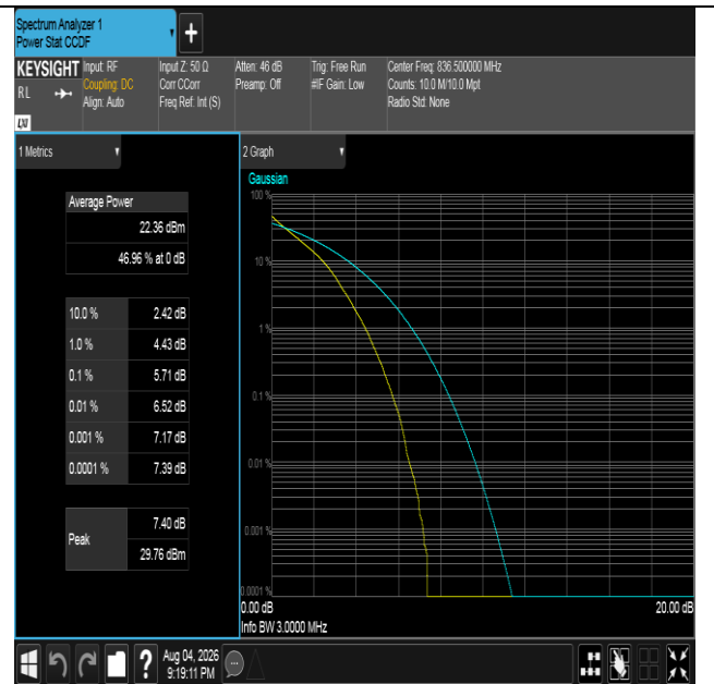
Band5-3MHz-QPSK-20525-15RB#0-PASS
