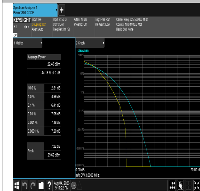
Band5-3MHz-16QAM-20415-1RB#0-PASS
