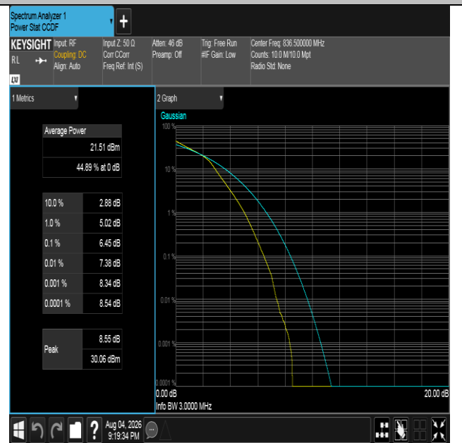
Band5-3MHz-16QAM-20525-15RB#0-PASS
