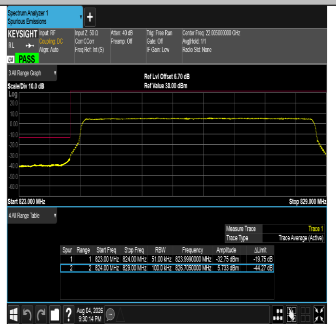
Band5-5MHz-16QAM-20425-25RB#0-PASS
