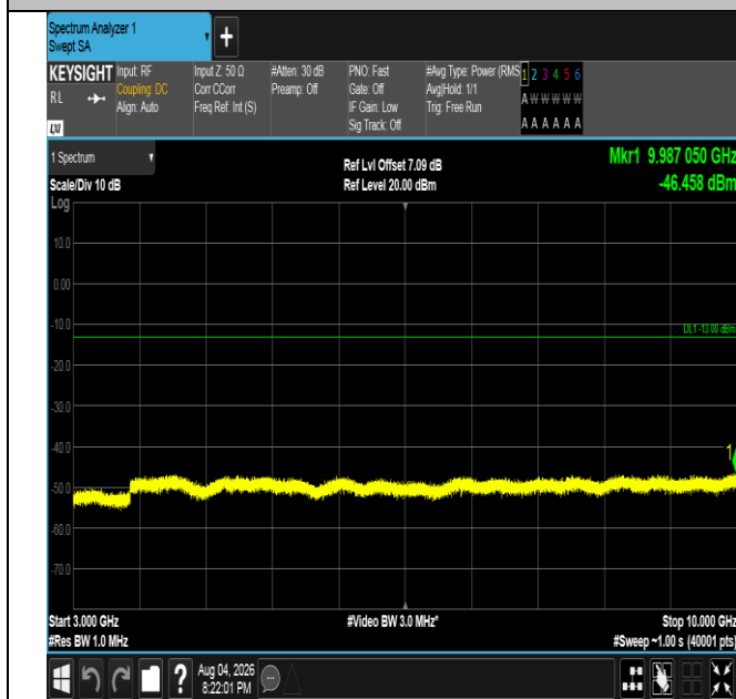
Band5-1.4MHz-QPSK-20407-1RB#0-3000~10000-PASS
