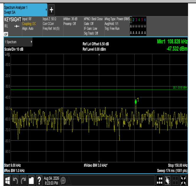
Band5-1.4MHz-QPSK-20407-1RB#5-0.009~0.15-PASS
