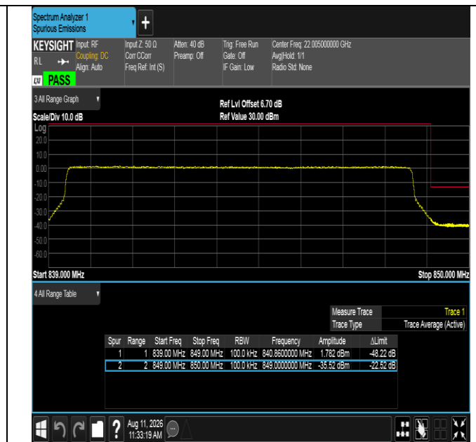
Band5-10MHz-16QAM-20600-50RB#0-PASS
