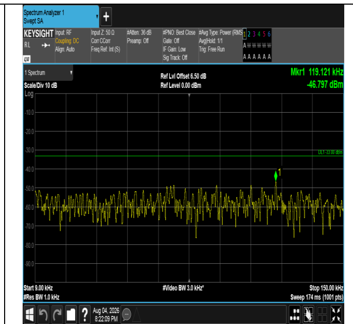
Band5-1.4MHz-16QAM-20407-1RB#0-0.009~0.15-PASS
