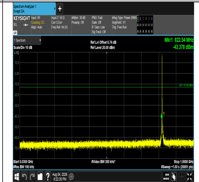
Band5-1.4MHz-16QAM-20407-1RB#0-30~1000-PASS
