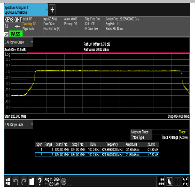
Band5-10MHz-16QAM-20450-50RB#0-PASS
