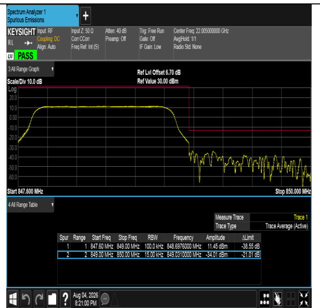
Band5-1.4MHz-16QAM-20643-6RB#0-PASS
