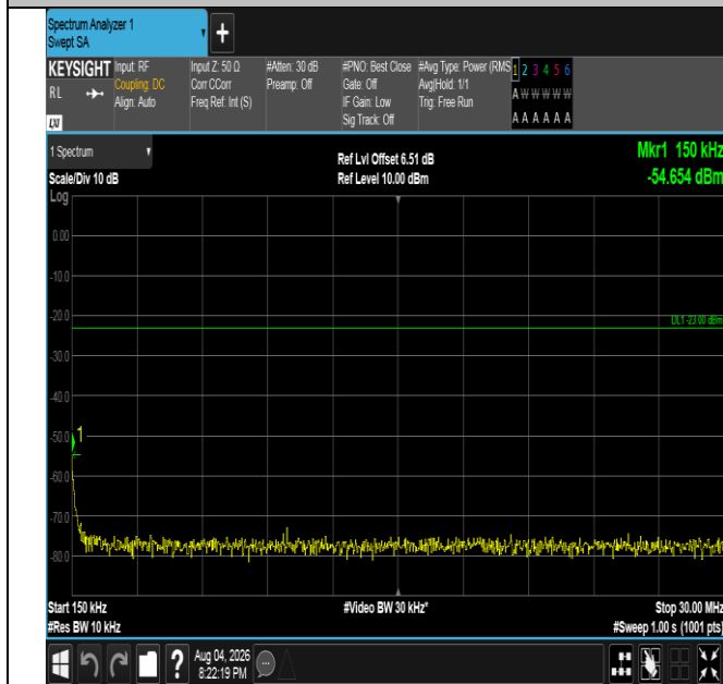
Band5-1.4MHz-16QAM-20407-1RB#0-0.15~30-PASS
