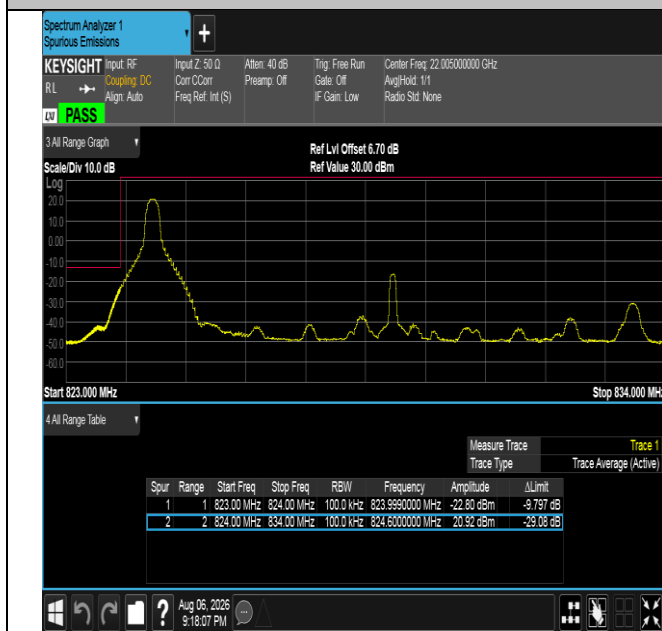
Band5-10MHz-QPSK-20450-1RB#0-PASS
