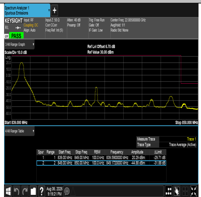
Band5-10MHz-16QAM-20600-1RB#0-PASS
