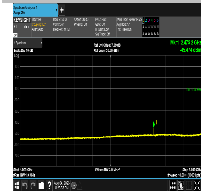
Band5-1.4MHz-QPSK-20407-1RB#5-1000~3000-PASS
