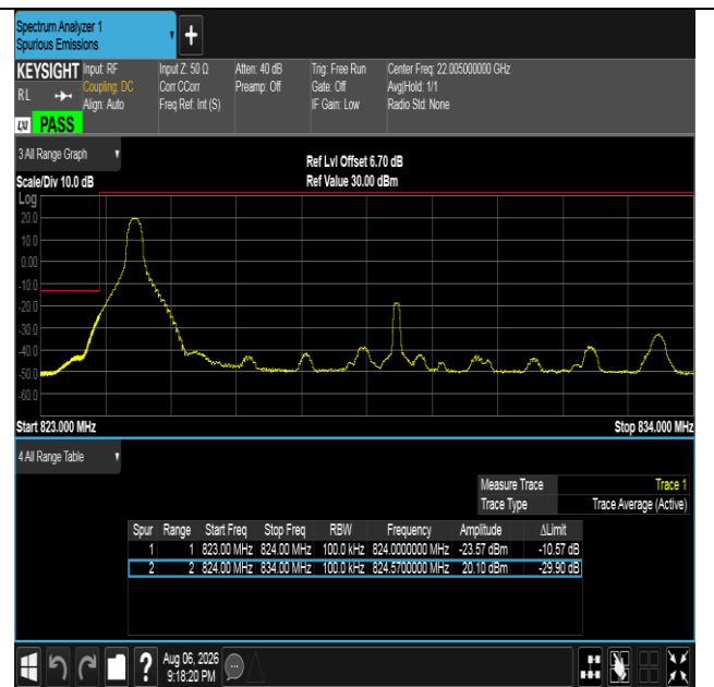
Band5-10MHz-16QAM-20450-1RB#0-PASS
