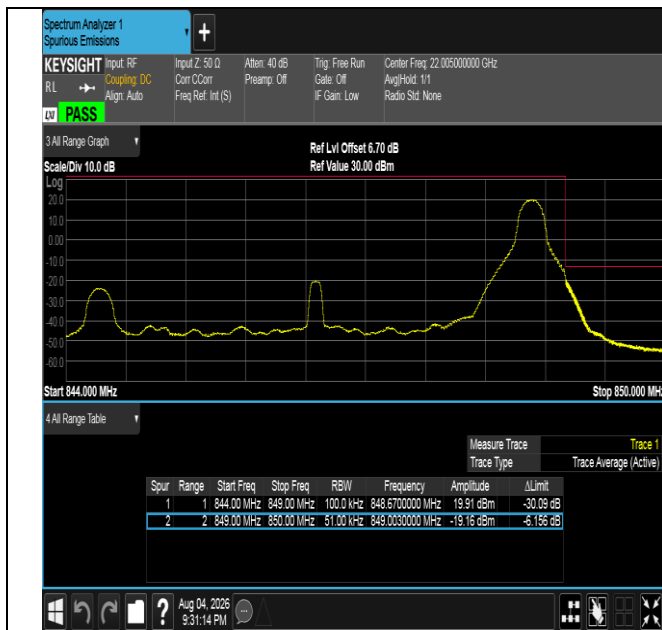
Band5-5MHz-16QAM-20625-1RB#24-PASS
