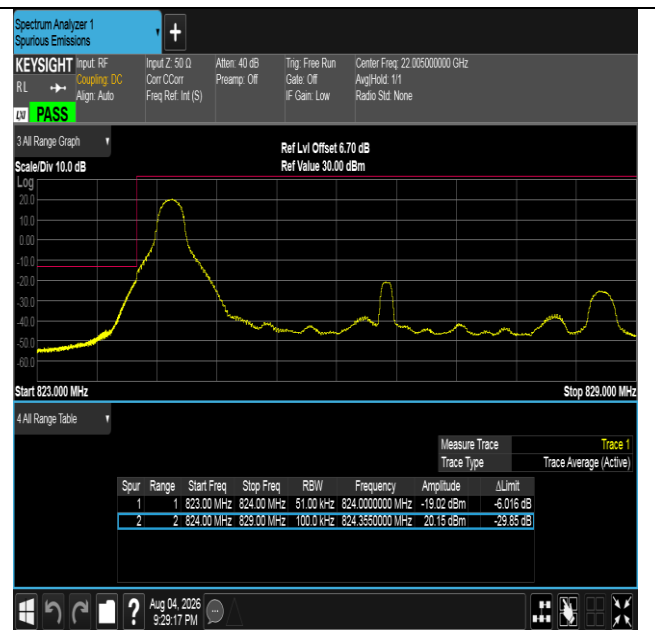
Band5-5MHz-16QAM-20425-1RB#0-PASS
