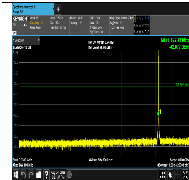
Band5-1.4MHz-QPSK-20407-1RB#0-30~1000-PASS
