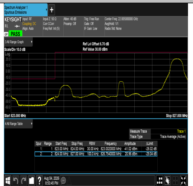
Band5-3MHz-QPSK-20415-1RB#14-PASS
