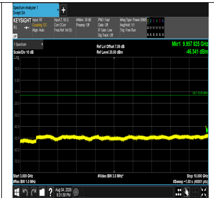
Band5-1.4MHz-16QAM-20525-6RB#0-3000~10000-PASS
