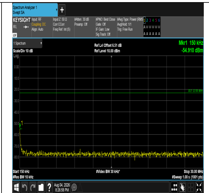
Band5-1.4MHz-QPSK-20525-1RB#0-0.15~30-PASS
