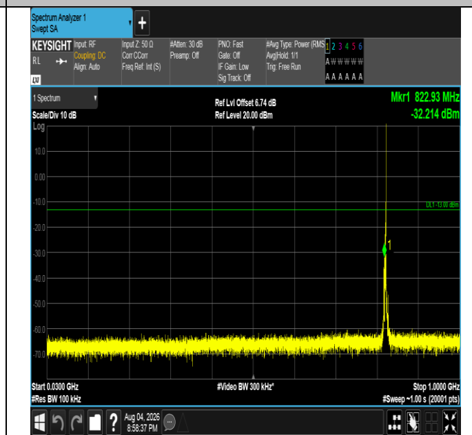
Band5-3MHz-QPSK-20415-1RB#14-30~1000-PASS
