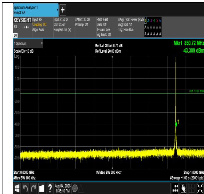
Band5-1.4MHz-16QAM-20643-1RB#5-30~1000-PASS
