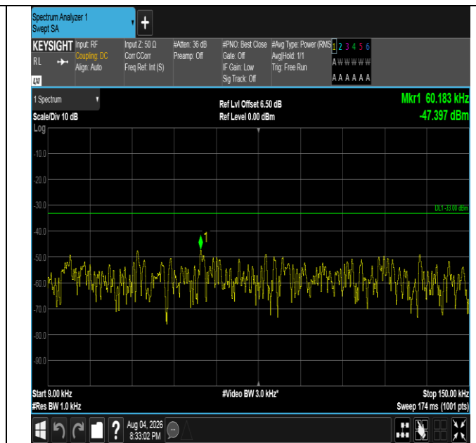
Band5-1.4MHz-16QAM-20643-1RB#0-0.009~0.15-PASS
