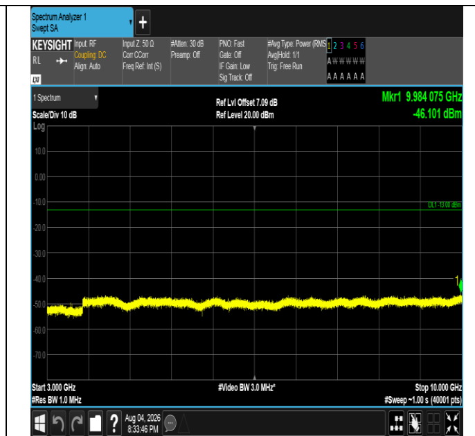
Band5-1.4MHz-16QAM-20643-1RB#0-3000~10000-PASS
