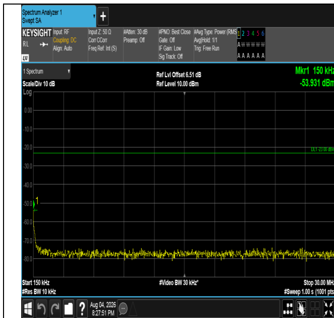
Band5-1.4MHz-16QAM-20525-1RB#0-0.15~30-PASS
