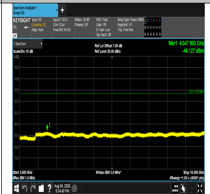
Band5-1.4MHz-QPSK-20643-1RB#5-3000~10000-PASS
