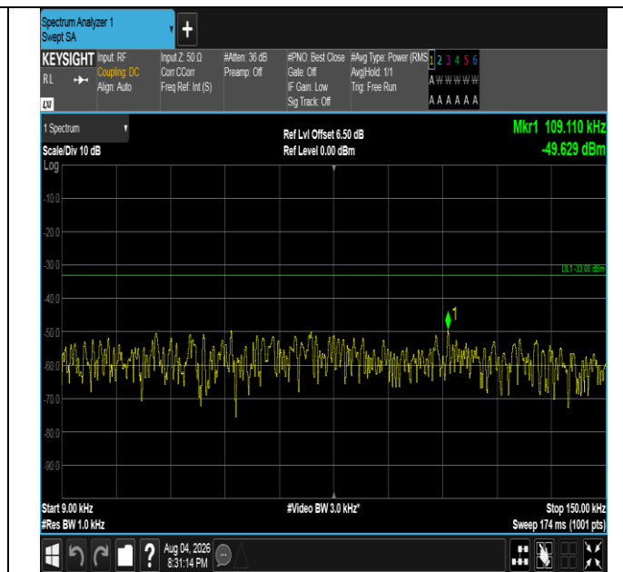
Band5-1.4MHz-16QAM-20525-6RB#0-0.009~0.15-PASS
