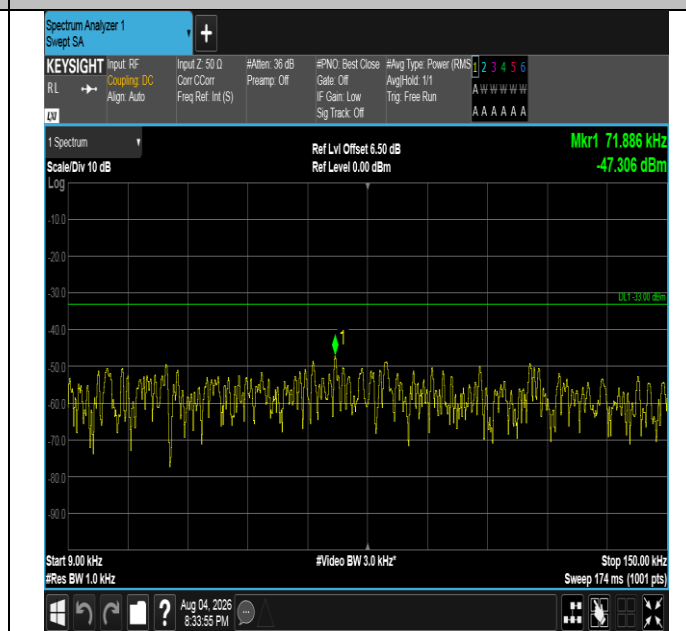
Band5-1.4MHz-QPSK-20643-1RB#5-0.009~0.15-PASS
