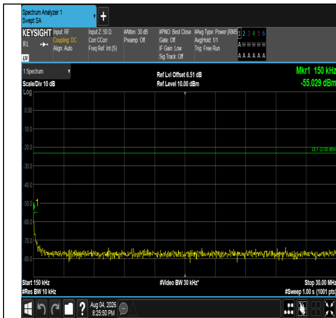
Band5-1.4MHz-16QAM-20407-6RB#0-0.15~30-PASS
