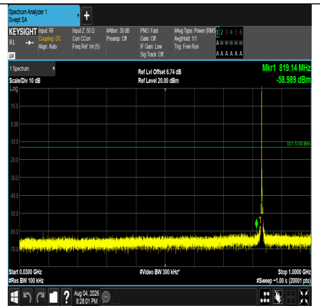
Band5-1.4MHz-16QAM-20525-1RB#0-30~1000-PASS
