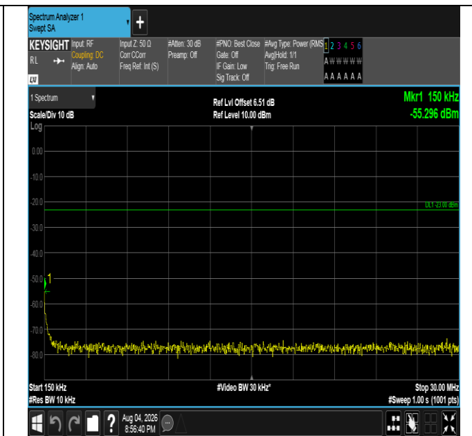
Band5-3MHz-QPSK-20415-1RB#0-0.15~30-PASS
