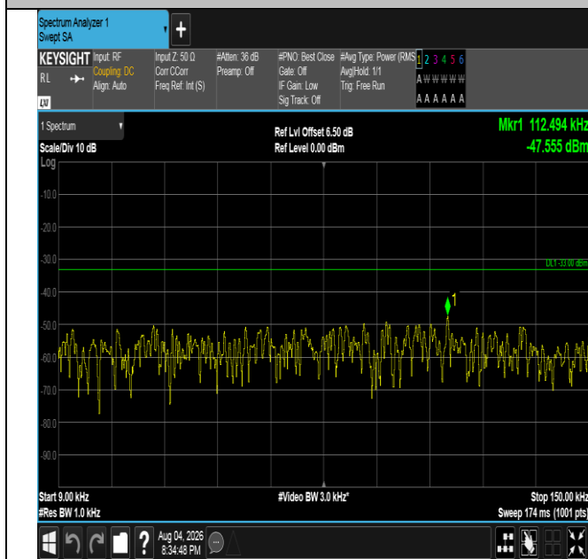
Band5-1.4MHz-16QAM-20643-1RB#5-0.009~0.15-PASS
