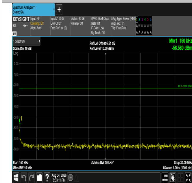
Band5-1.4MHz-16QAM-20643-1RB#0-0.15~30-PASS
