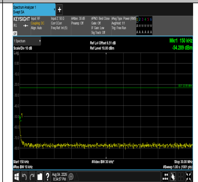
Band5-1.4MHz-16QAM-20643-1RB#5-0.15~30-PASS
