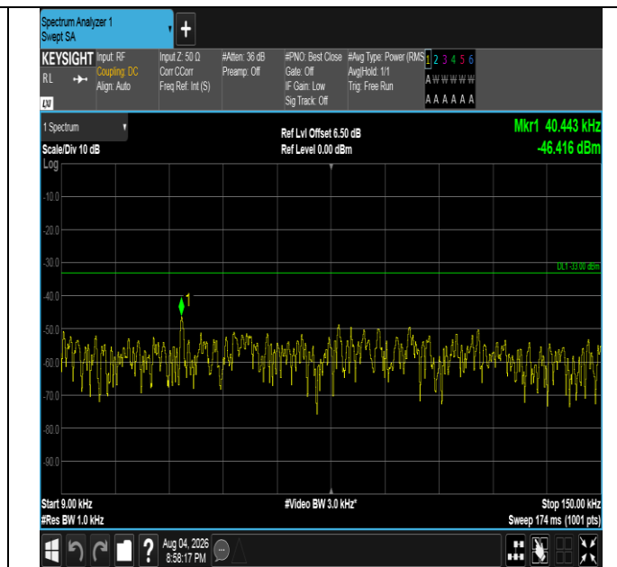
Band5-3MHz-QPSK-20415-1RB#14-0.009~0.15-PASS
