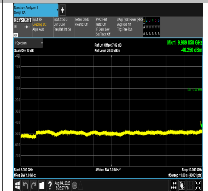
Band5-1.4MHz-16QAM-20407-6RB#0-3000~10000-PASS
