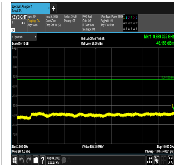
Band5-1.4MHz-QPSK-20643-6RB#0-3000~10000-PASS
