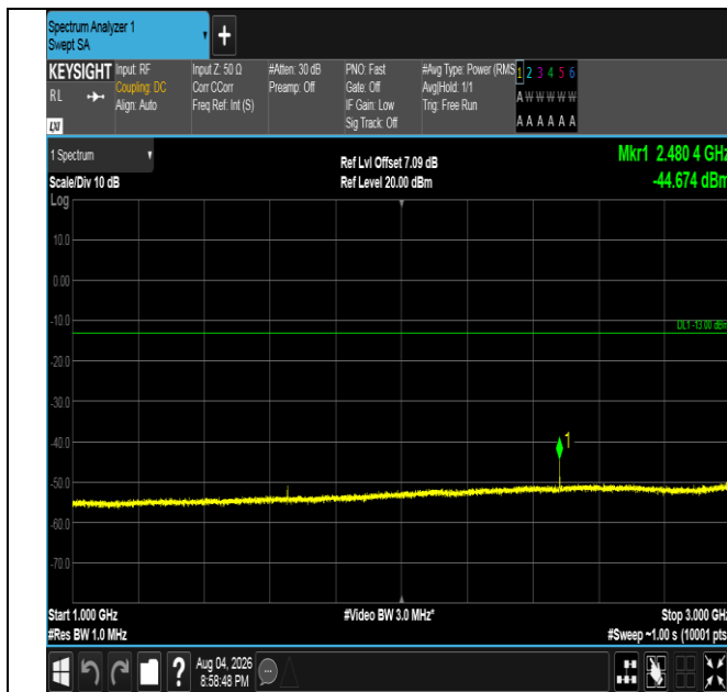
Band5-3MHz-QPSK-20415-1RB#14-1000~3000-PASS
