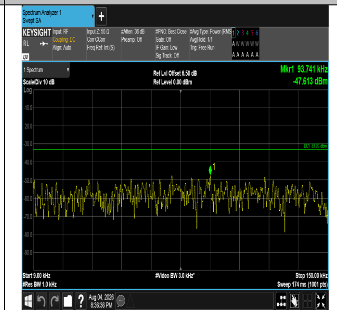
Band5-1.4MHz-16QAM-20643-6RB#0-0.009~0.15-PASS
