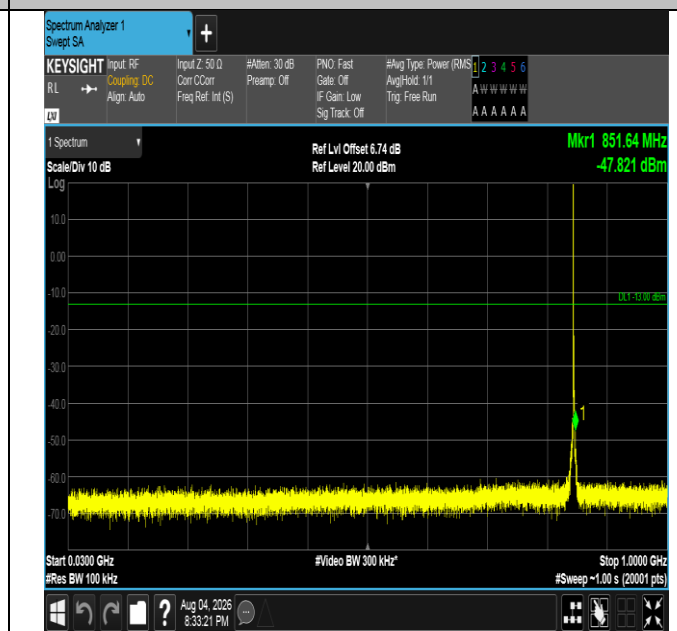
Band5-1.4MHz-16QAM-20643-1RB#0-30~1000-PASS
