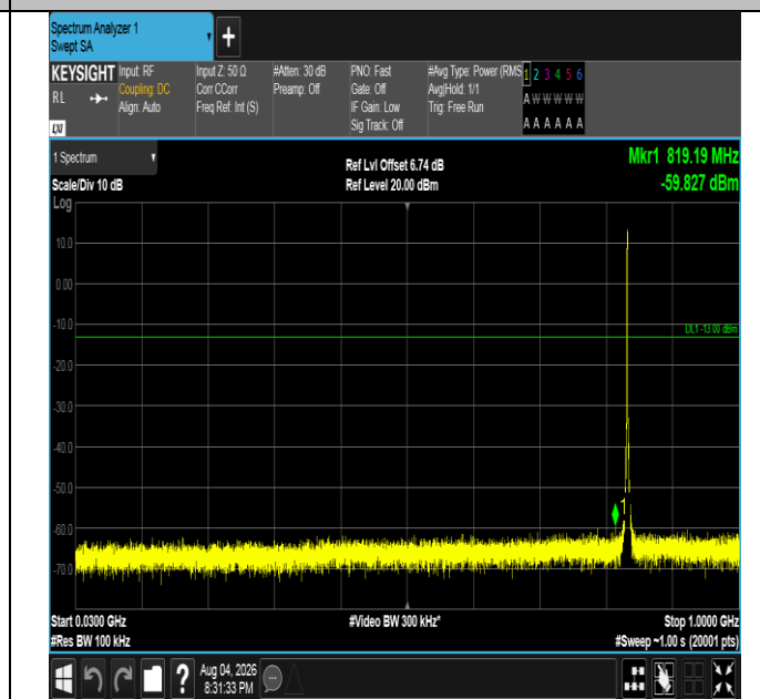
Band5-1.4MHz-16QAM-20525-6RB#0-30~1000-PASS
