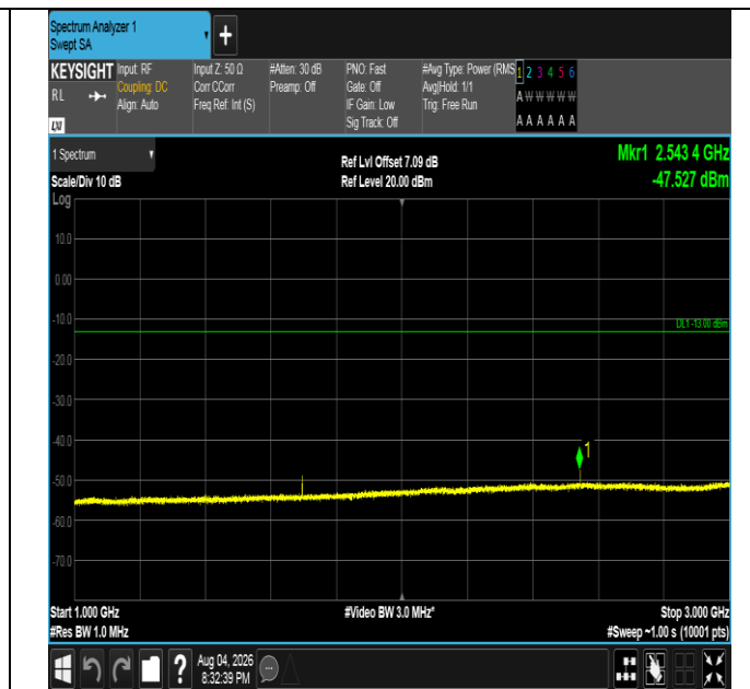
Band5-1.4MHz-QPSK-20643-1RB#0-1000~3000-PASS
