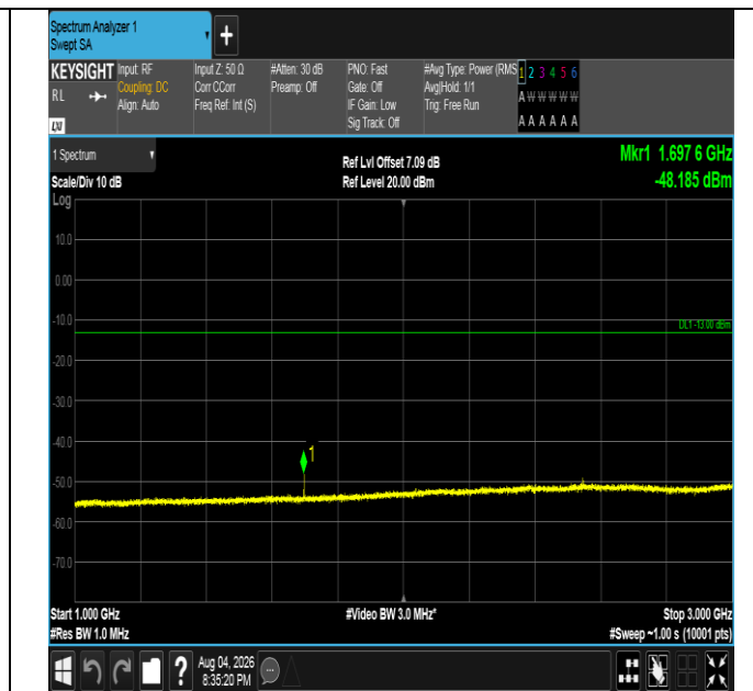
Band5-1.4MHz-16QAM-20643-1RB#5-1000~3000-PASS
