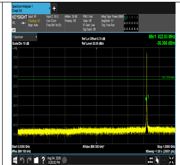
Band5-1.4MHz-16QAM-20407-6RB#0-30~1000-PASS
