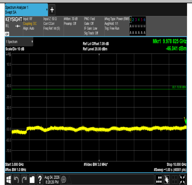
Band5-1.4MHz-16QAM-20525-1RB#0-3000~10000-PASS
