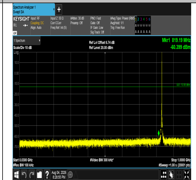
Band5-1.4MHz-QPSK-20525-1RB#5-30~1000-PASS
