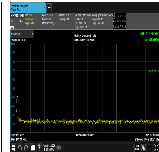
Band5-1.4MHz-QPSK-20643-1RB#5-0.15~30-PASS
