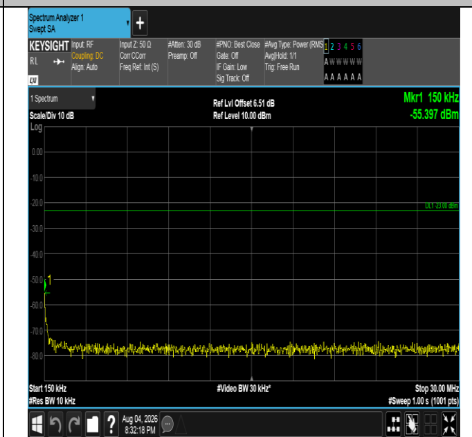
Band5-1.4MHz-QPSK-20643-1RB#0-0.15~30-PASS
