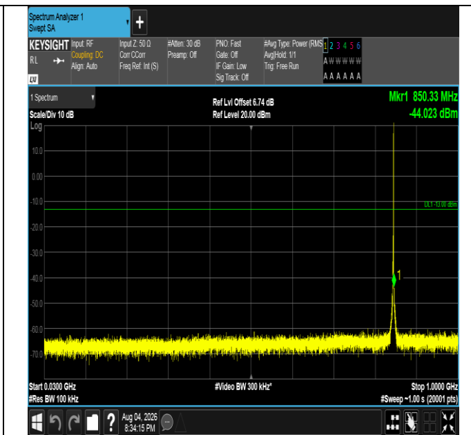
Band5-1.4MHz-QPSK-20643-1RB#5-30~1000-PASS
