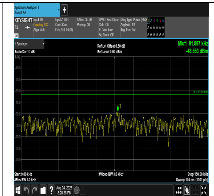
Band5-1.4MHz-QPSK-20525-1RB#5-0.009~0.15-PASS
