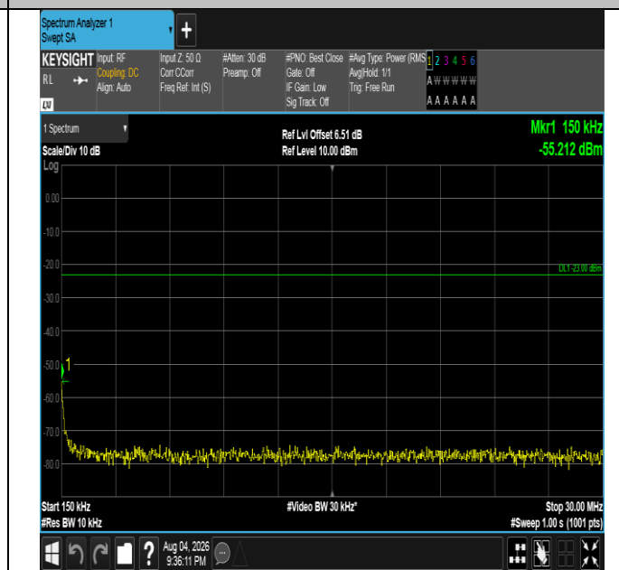
Band5-5MHz-16QAM-20425-1RB#24-0.15~30-PASS
