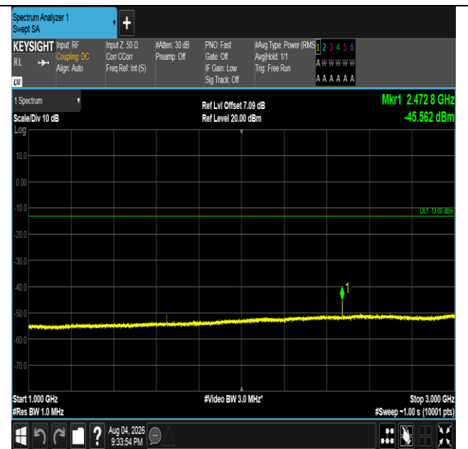
Band5-5MHz-QPSK-20425-1RB#0-1000~3000-PASS
