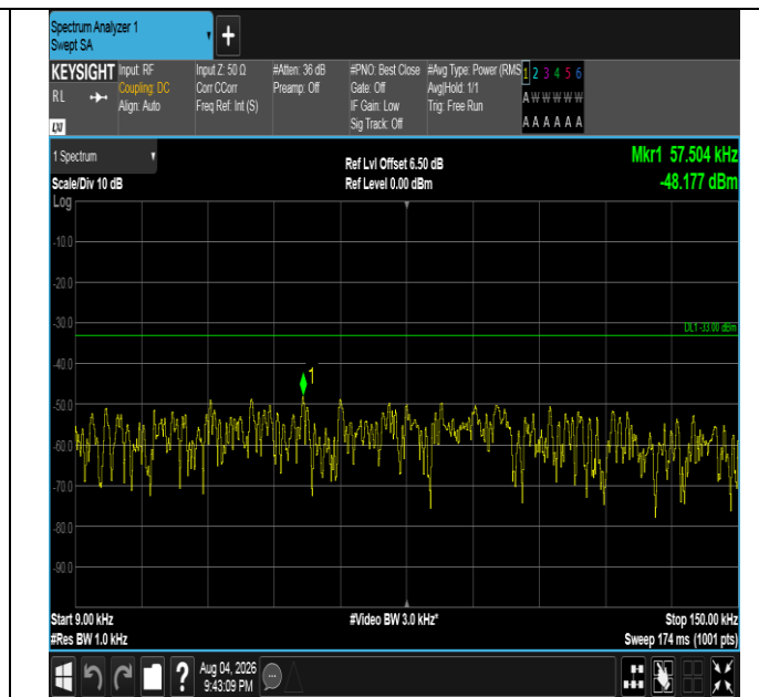
Band5-5MHz-16QAM-20525-25RB#0-0.009~0.15-PASS
