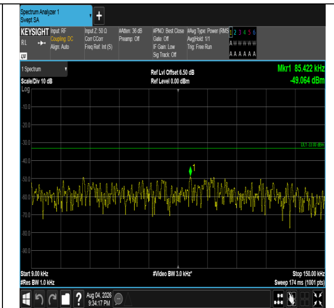
Band5-5MHz-16QAM-20425-1RB#0-0.009~0.15-PASS
