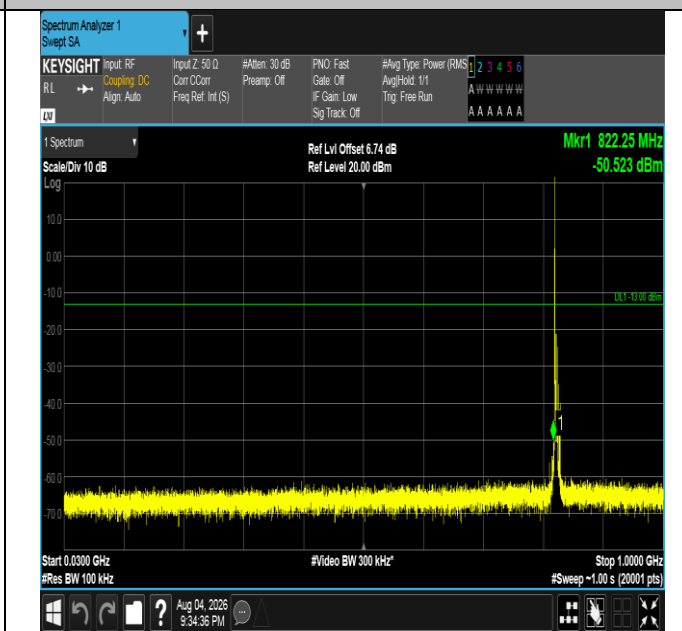
Band5-5MHz-16QAM-20425-1RB#0-30~1000-PASS
