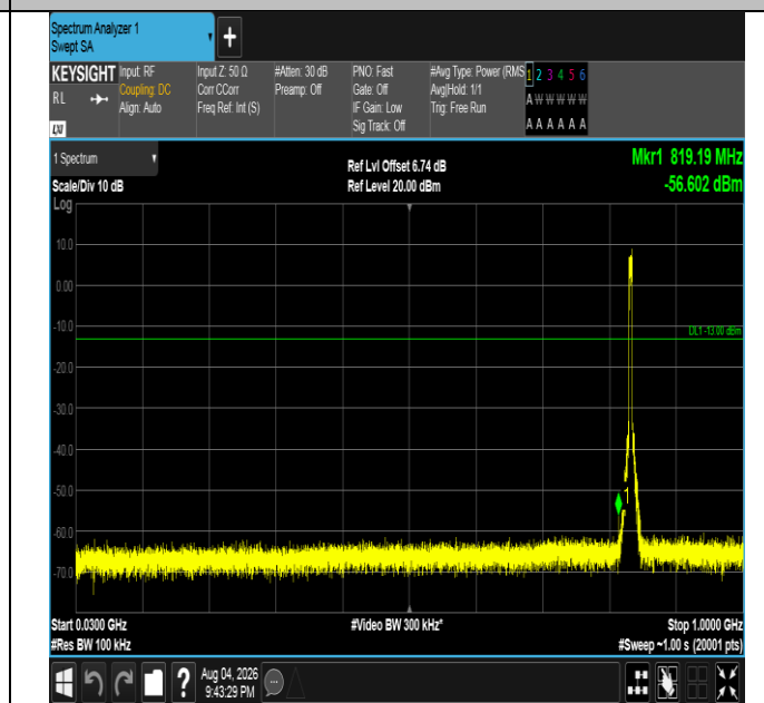
Band5-5MHz-16QAM-20525-25RB#0-30~1000-PASS
