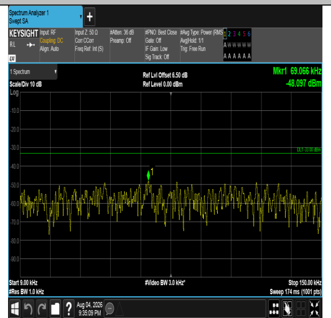
Band5-5MHz-QPSK-20425-1RB#24-0.009~0.15-PASS
