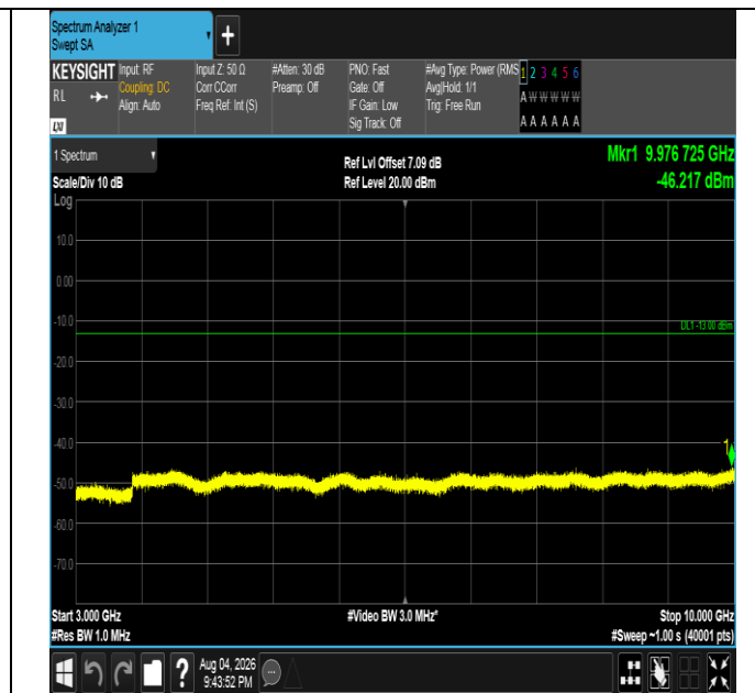
Band5-5MHz-16QAM-20525-25RB#0-3000~10000-PASS
