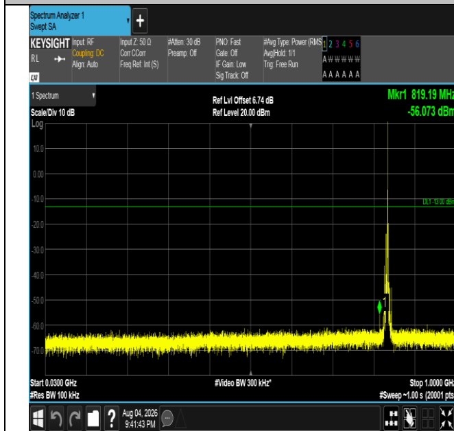
Band5-5MHz-16QAM-20525-1RB#24-30~1000-PASS
