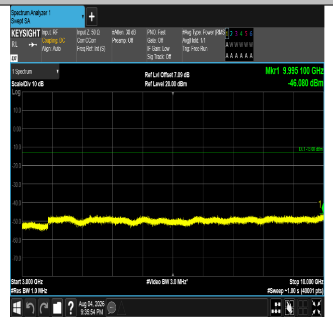
Band5-5MHz-QPSK-20425-1RB#24-3000~10000-PASS
