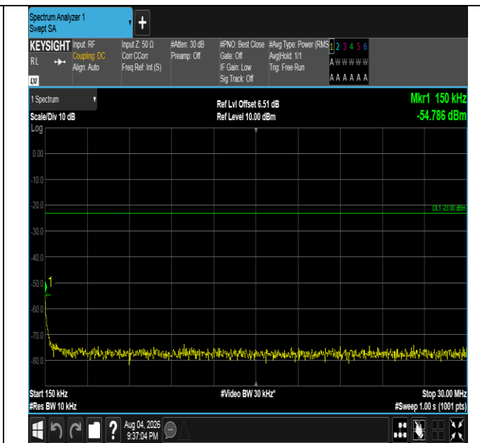
Band5-5MHz-QPSK-20425-25RB#0-0.15~30-PASS
