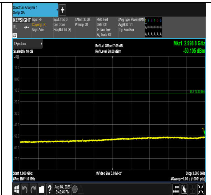
Band5-5MHz-QPSK-20525-25RB#0-1000~3000-PASS
