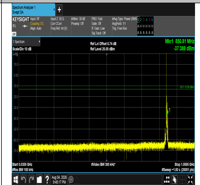
Band5-5MHz-16QAM-20625-1RB#0-30~1000-PASS
