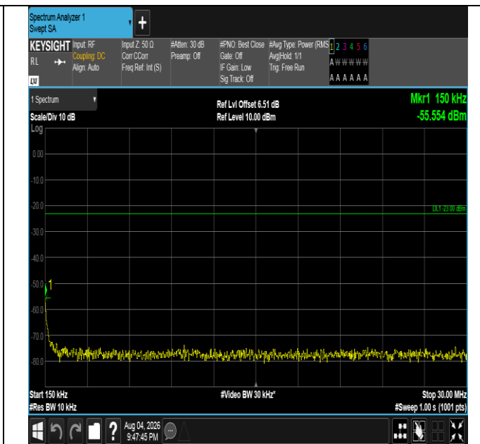
Band5-5MHz-QPSK-20625-25RB#0-0.15~30-PASS
