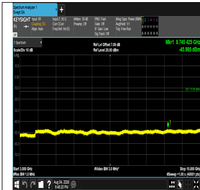
Band5-5MHz-QPSK-20625-25RB#0-3000~10000-PASS
