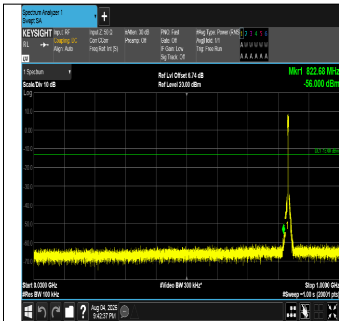
Band5-5MHz-QPSK-20525-25RB#0-30~1000-PASS
