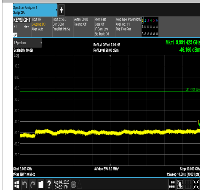
Band5-5MHz-QPSK-20525-25RB#0-3000~10000-PASS
