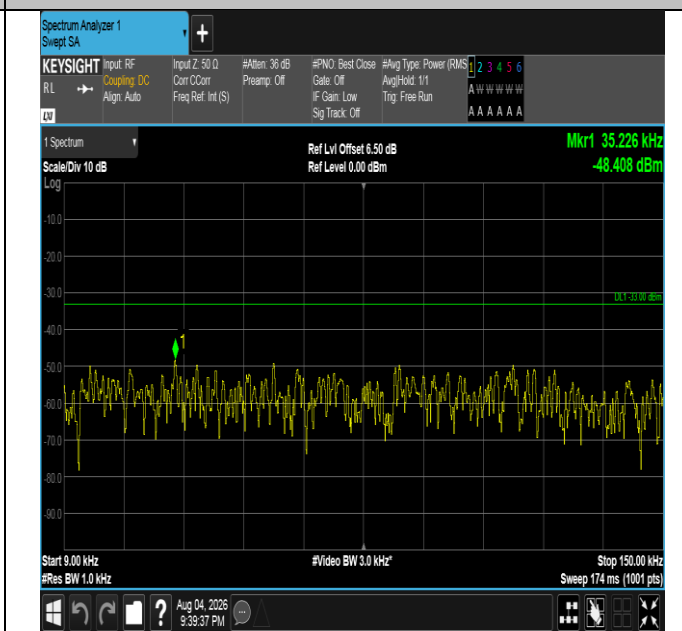
Band5-5MHz-16QAM-20525-1RB#0-0.009~0.15-PASS
