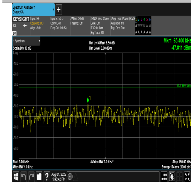
Band5-5MHz-16QAM-20625-1RB#24-0.009~0.15-PASS
