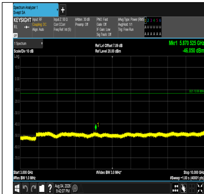
Band5-5MHz-16QAM-20525-1RB#24-3000~10000-PASS
