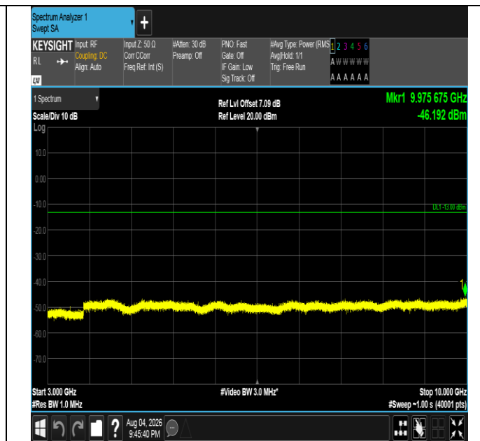
Band5-5MHz-16QAM-20625-1RB#0-3000~10000-PASS
