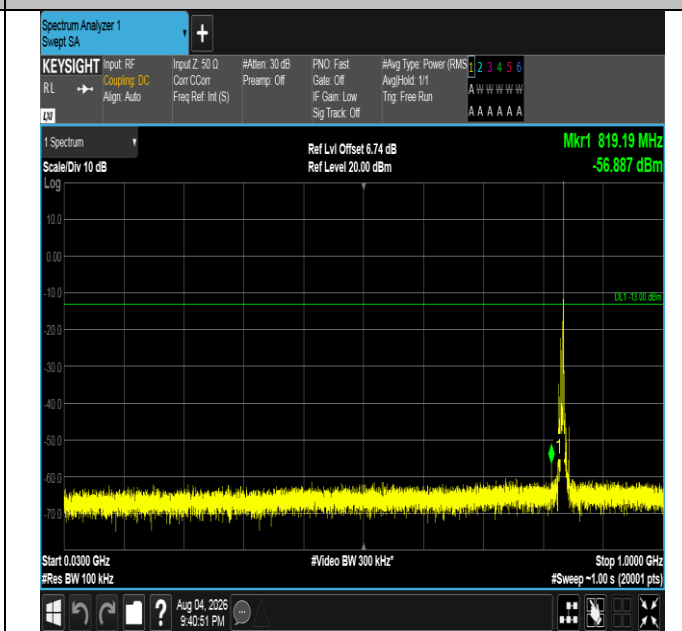
Band5-5MHz-QPSK-20525-1RB#24-30~1000-PASS
