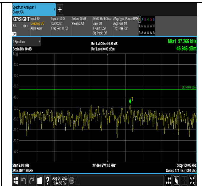
Band5-5MHz-16QAM-20625-1RB#0-0.009~0.15-PASS
