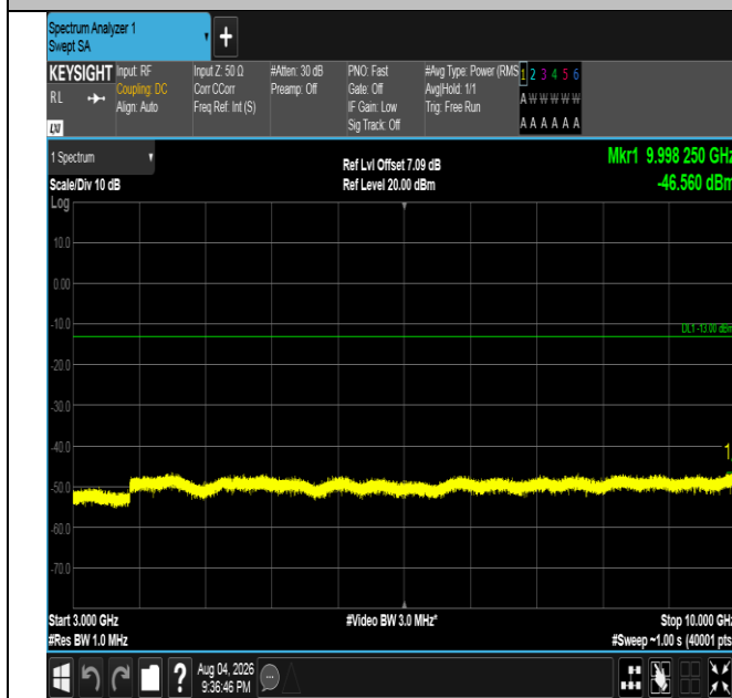
Band5-5MHz-16QAM-20425-1RB#24-3000~10000-PASS
