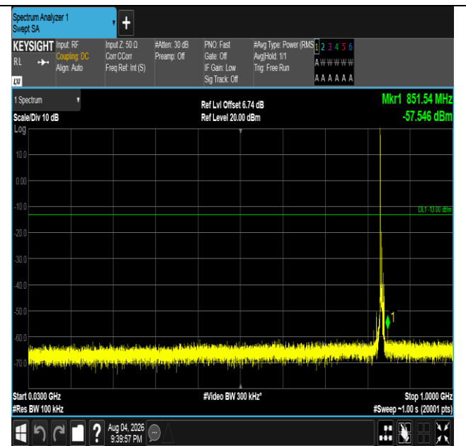
Band5-5MHz-16QAM-20525-1RB#0-30~1000-PASS
