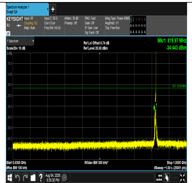
Band5-5MHz-QPSK-20425-1RB#24-30~1000-PASS
