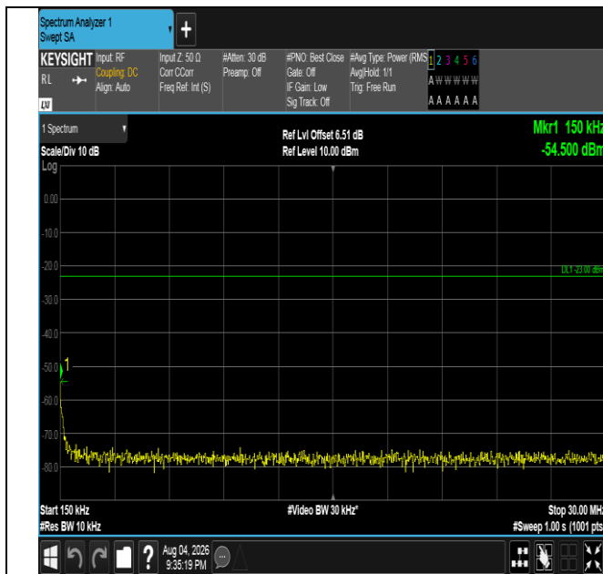
Band5-5MHz-QPSK-20425-1RB#24-0.15~30-PASS
