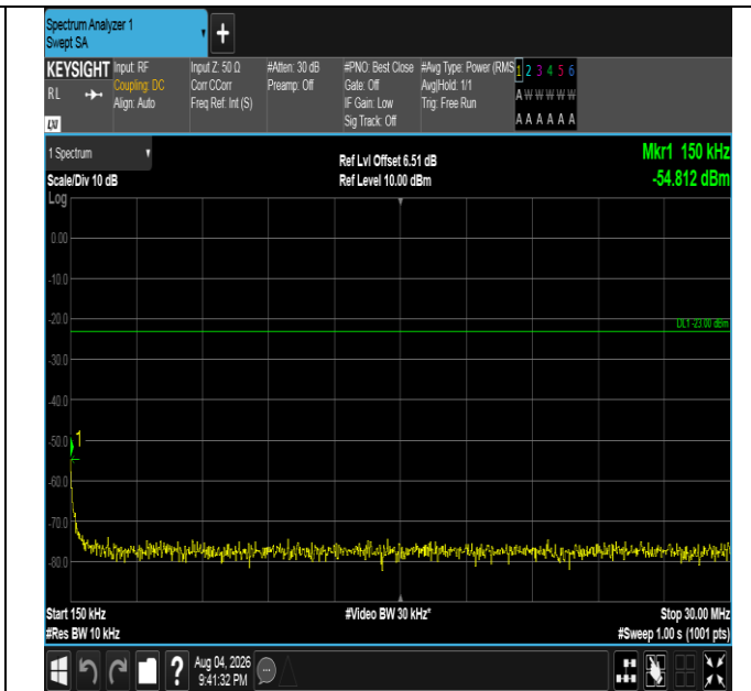
Band5-5MHz-16QAM-20525-1RB#24-0.15~30-PASS
