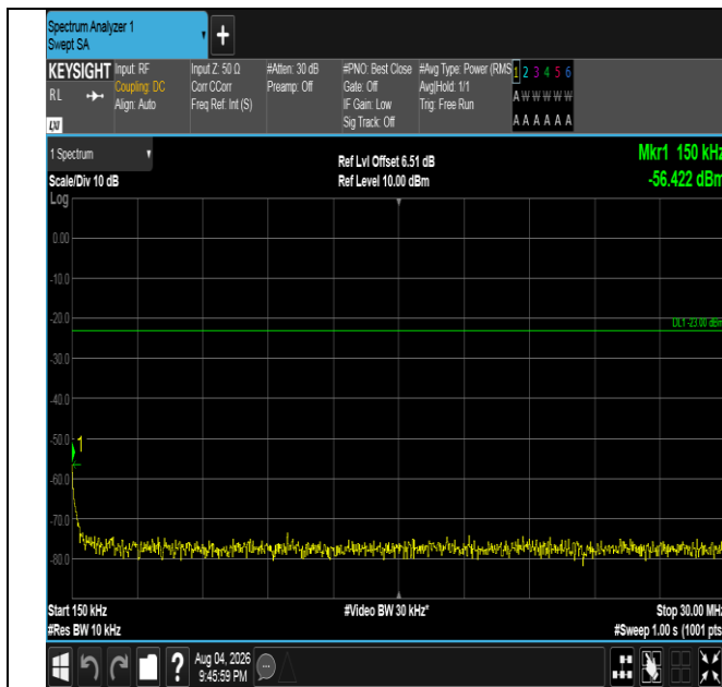
Band5-5MHz-QPSK-20625-1RB#24-0.15~30-PASS
