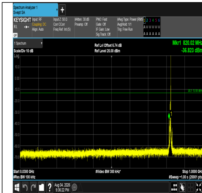
Band5-5MHz-16QAM-20425-1RB#24-30~1000-PASS
