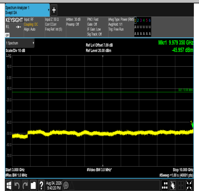
Band5-5MHz-16QAM-20525-1RB#0-3000~10000-PASS
