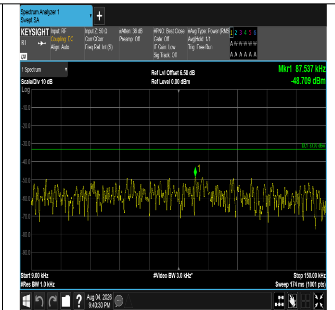
Band5-5MHz-QPSK-20525-1RB#24-0.009~0.15-PASS
