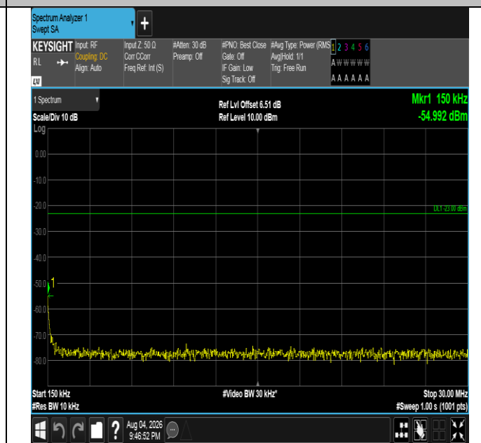
Band5-5MHz-16QAM-20625-1RB#24-0.15~30-PASS
