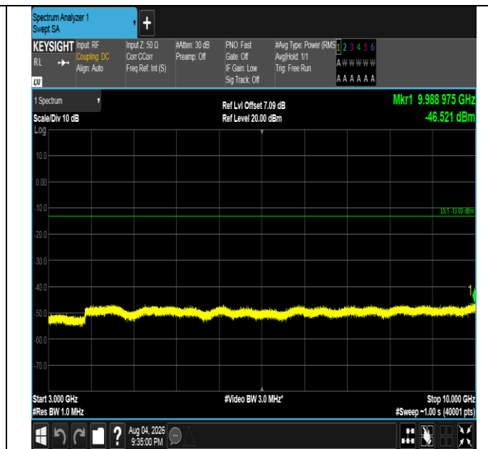
Band5-5MHz-16QAM-20425-1RB#0-3000~10000-PASS
