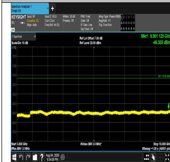
Band5-5MHz-QPSK-20425-1RB#0-3000~10000-PASS
