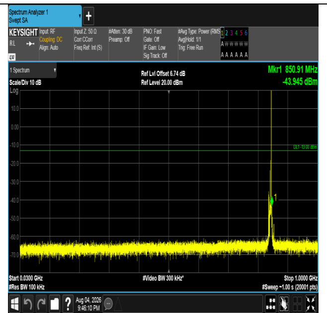
Band5-5MHz-QPSK-20625-1RB#24-30~1000-PASS
