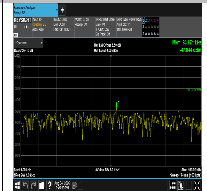
Band5-5MHz-QPSK-20625-1RB#24-0.009~0.15-PASS
