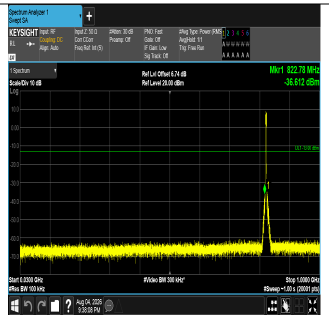
Band5-5MHz-16QAM-20425-25RB#0-30~1000-PASS
