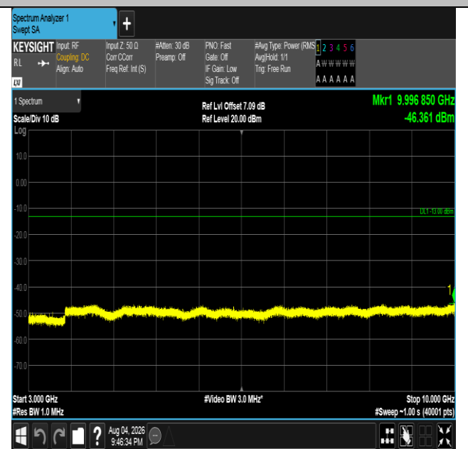
Band5-5MHz-QPSK-20625-1RB#24-3000~10000-PASS
