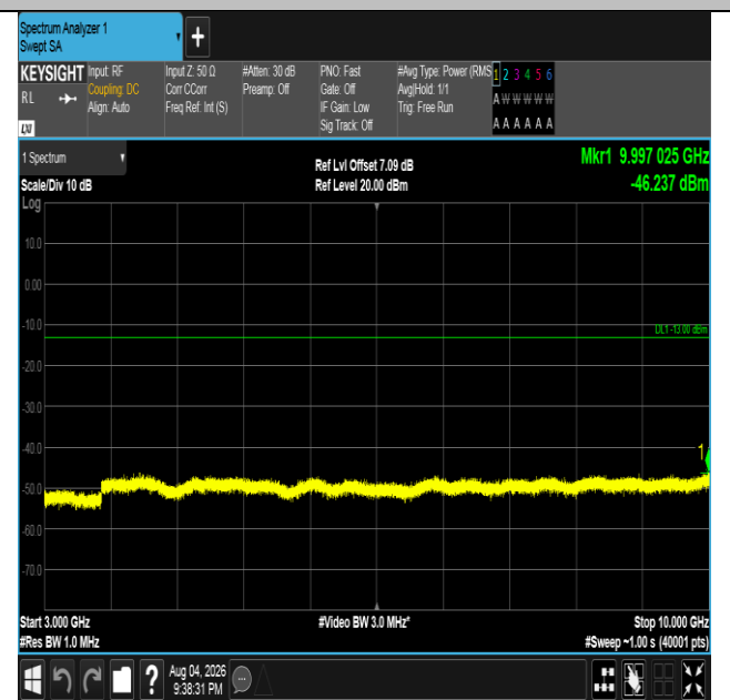
Band5-5MHz-16QAM-20425-25RB#0-3000~10000-PASS
