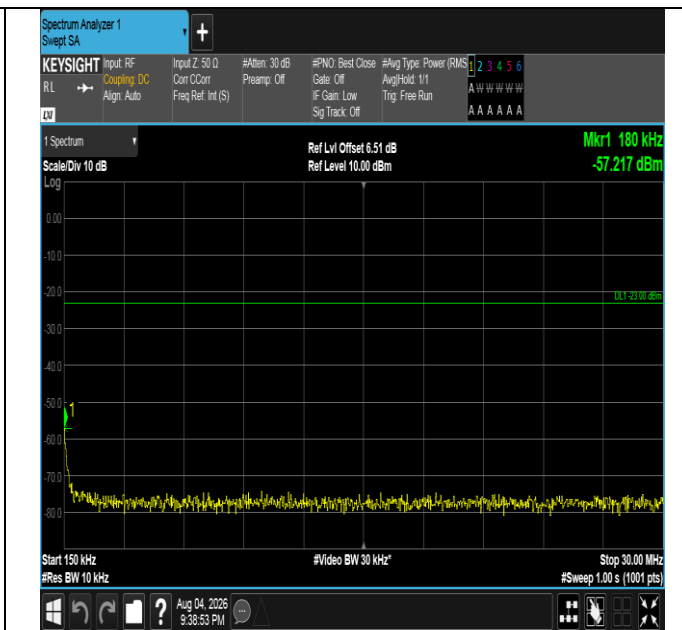
Band5-5MHz-QPSK-20525-1RB#0-0.15~30-PASS
