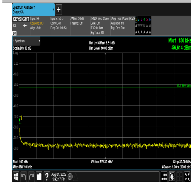
Band5-5MHz-16QAM-20525-25RB#0-0.15~30-PASS
