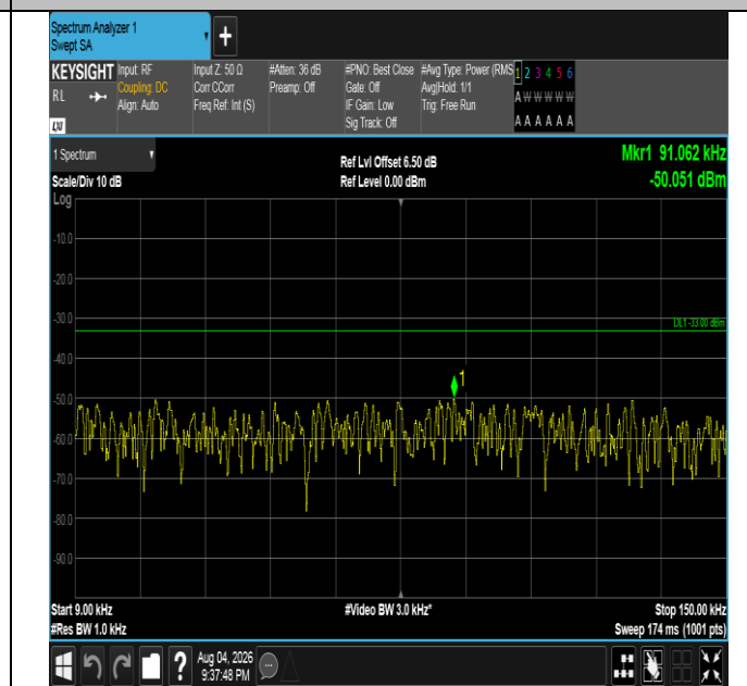
Band5-5MHz-16QAM-20425-25RB#0-0.009~0.15-PASS
