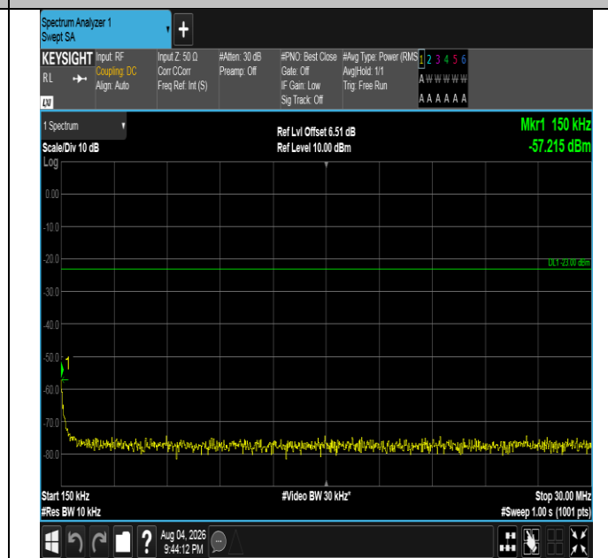
Band5-5MHz-QPSK-20625-1RB#0-0.15~30-PASS
