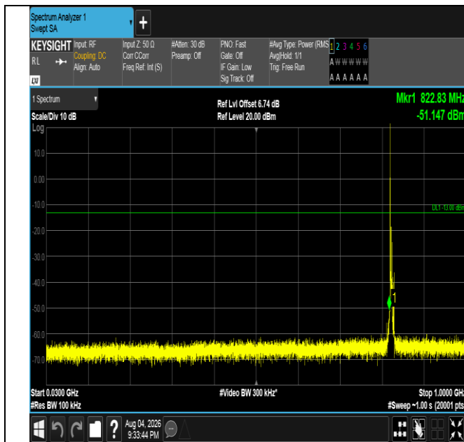
Band5-5MHz-QPSK-20425-1RB#0-30~1000-PASS
