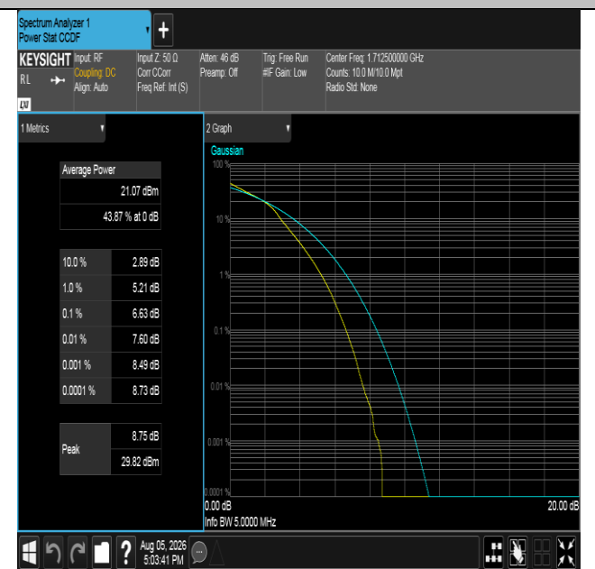
Band66-5MHz-16QAM-131997-25RB#0-PASS
