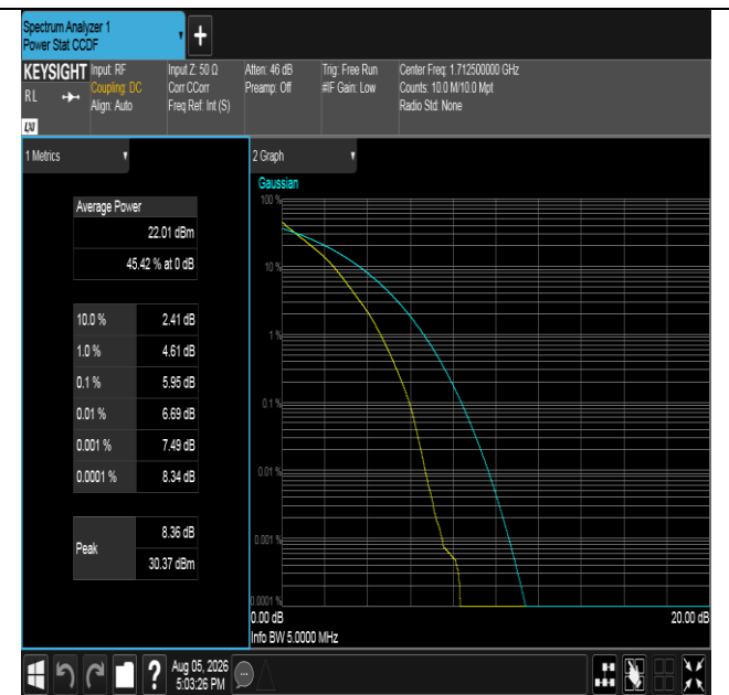
Band66-5MHz-QPSK-131997-25RB#0-PASS
