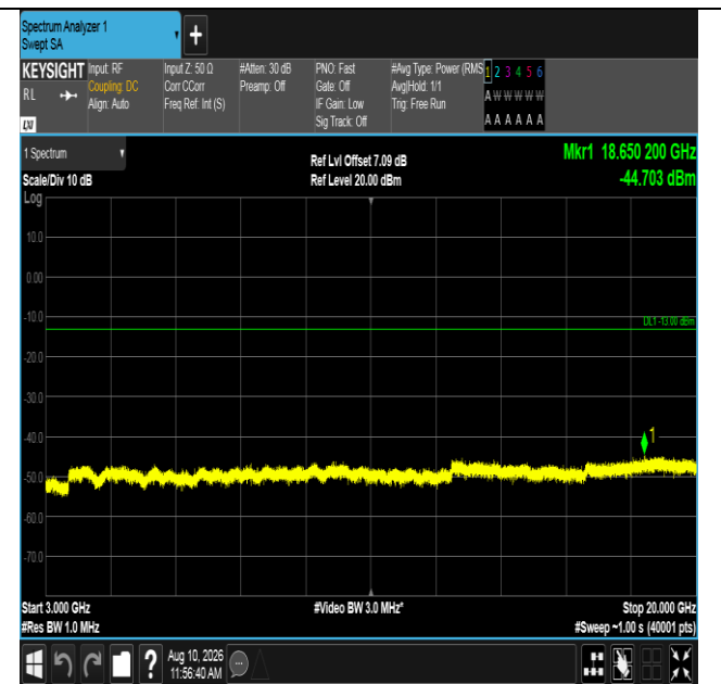
Band66-20MHz-16QAM-132572-1RB#0-3000~20000-PASS
