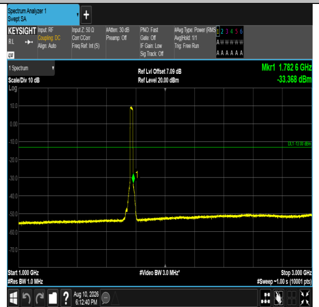
Band66-20MHz-QPSK-132572-100RB#0-1000~3000-PASS
