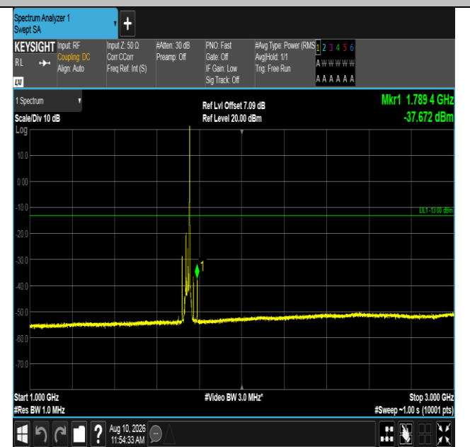
Band66-20MHz-16QAM-132322-1RB#99-1000~3000-PASS
