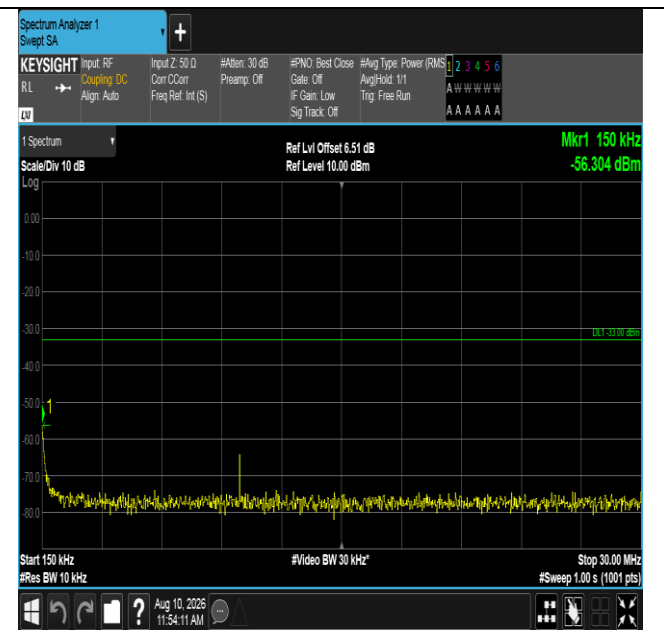
Band66-20MHz-16QAM-132322-1RB#99-0.15~30-PASS
