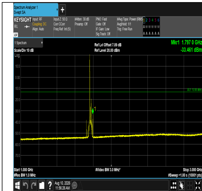
Band66-20MHz-16QAM-132572-1RB#0-1000~3000-PASS
