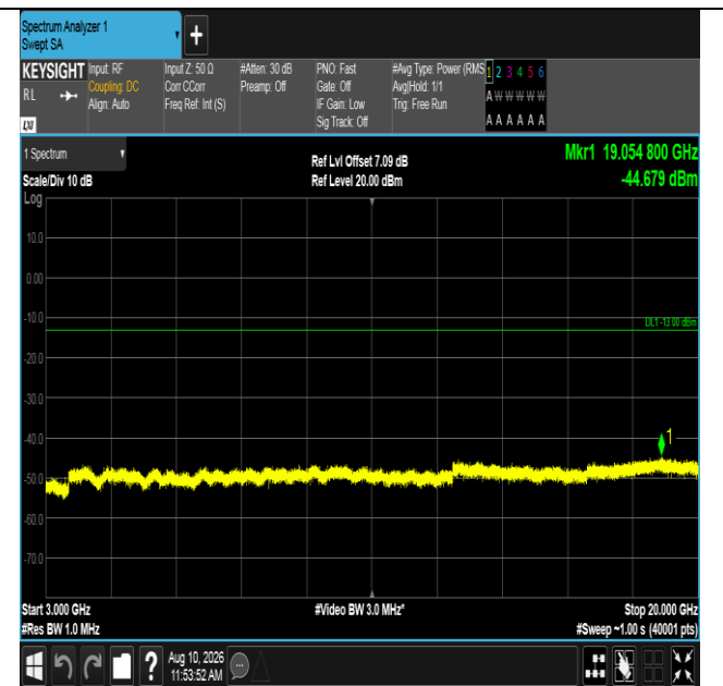
Band66-20MHz-QPSK-132322-1RB#99-3000~20000-PASS
