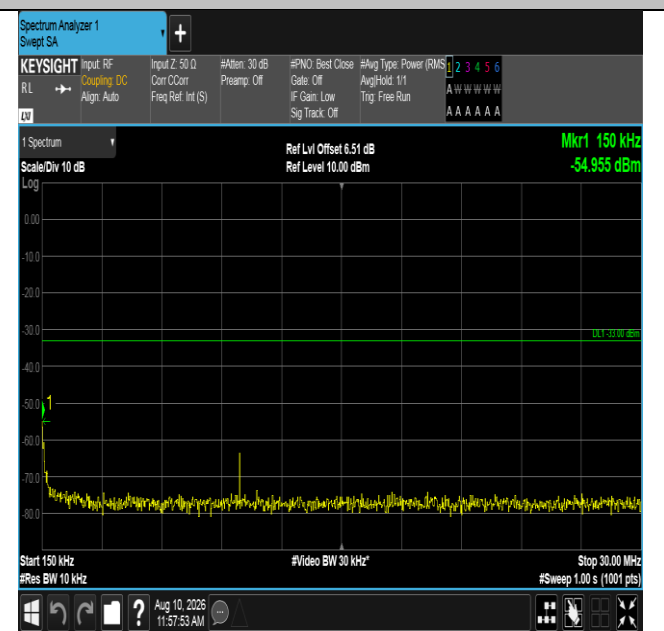
Band66-20MHz-16QAM-132572-1RB#99-0.15~30-PASS
