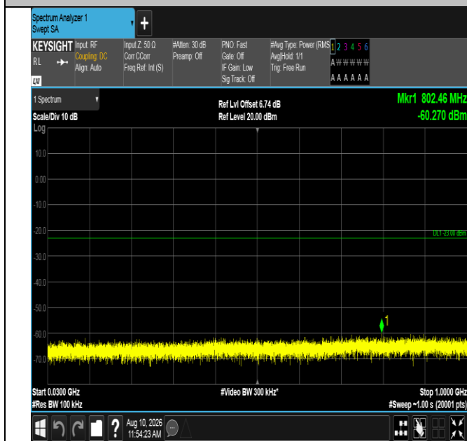
Band66-20MHz-16QAM-132322-1RB#99-30~1000-PASS
