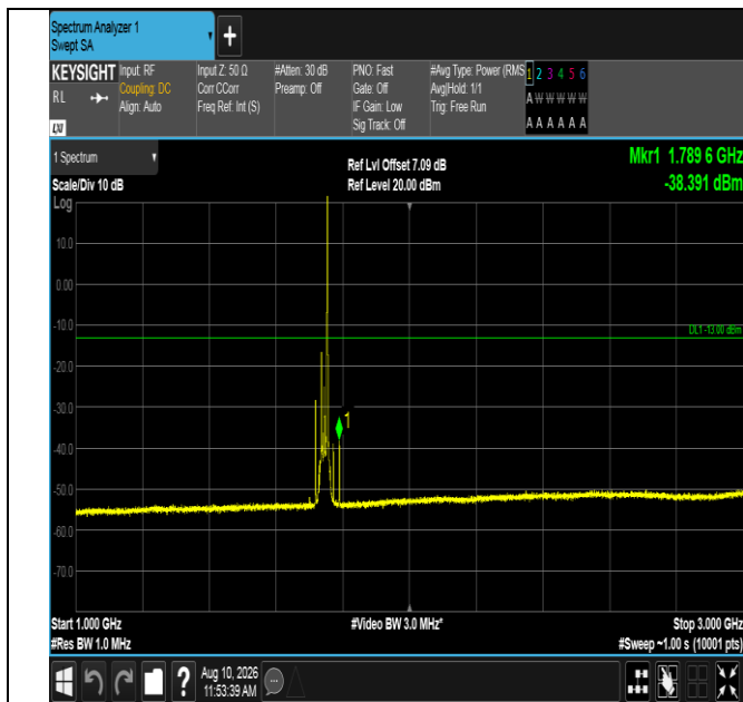
Band66-20MHz-QPSK-132322-1RB#99-1000~3000-PASS
