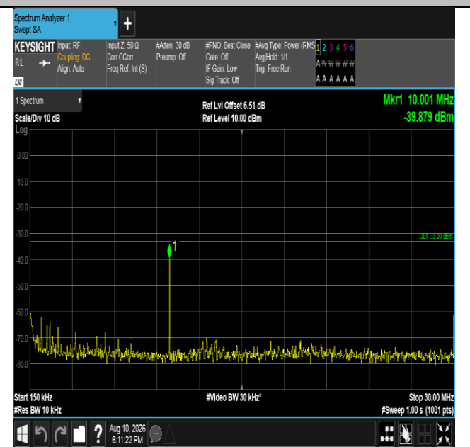
Band66-20MHz-QPSK-132322-100RB#0-0.15~30-PASS
