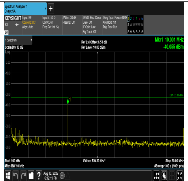
Band66-20MHz-QPSK-132572-100RB#0-0.15~30-PASS
