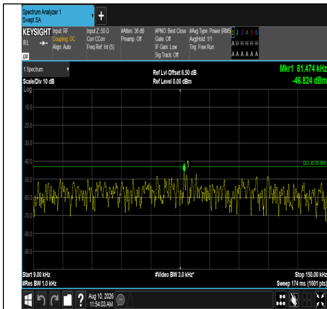
Band66-20MHz-16QAM-132322-1RB#99-0.009~0.15-PASS
