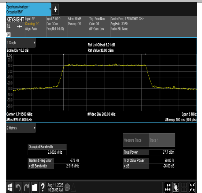
Band66-3MHz-16QAM-131987-15RB#0-PASS
