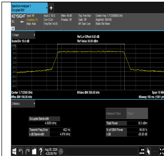
Band66-5MHz-QPSK-131997-25RB#0-PASS
