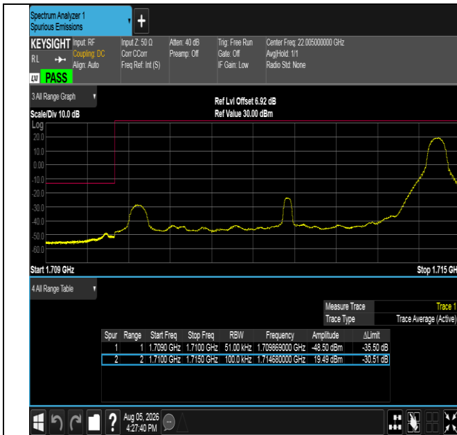
Band66-5MHz-16QAM-131997-1RB#24-PASS
