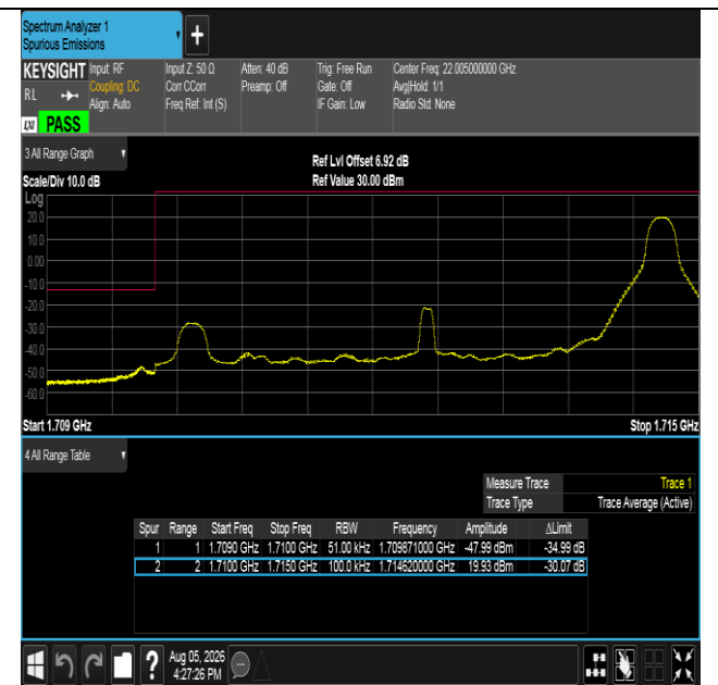
Band66-5MHz-QPSK-131997-1RB#24-PASS
