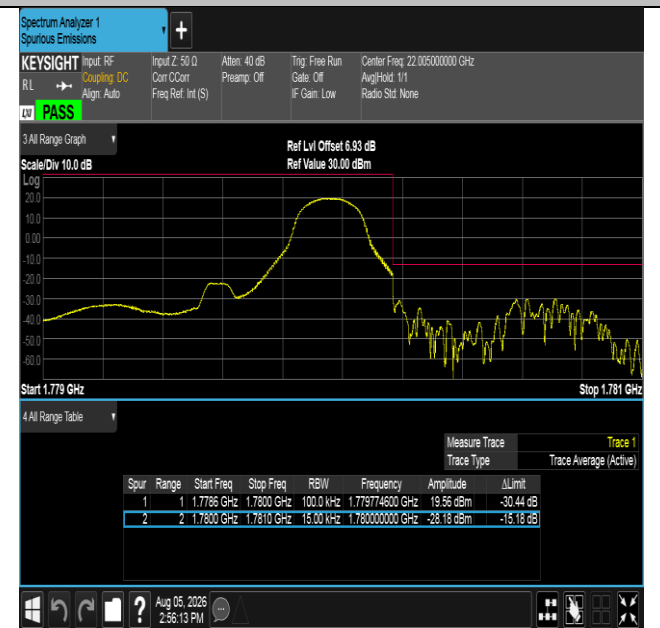
Band66-1.4MHz-QPSK-132665-1RB#5-PASS
