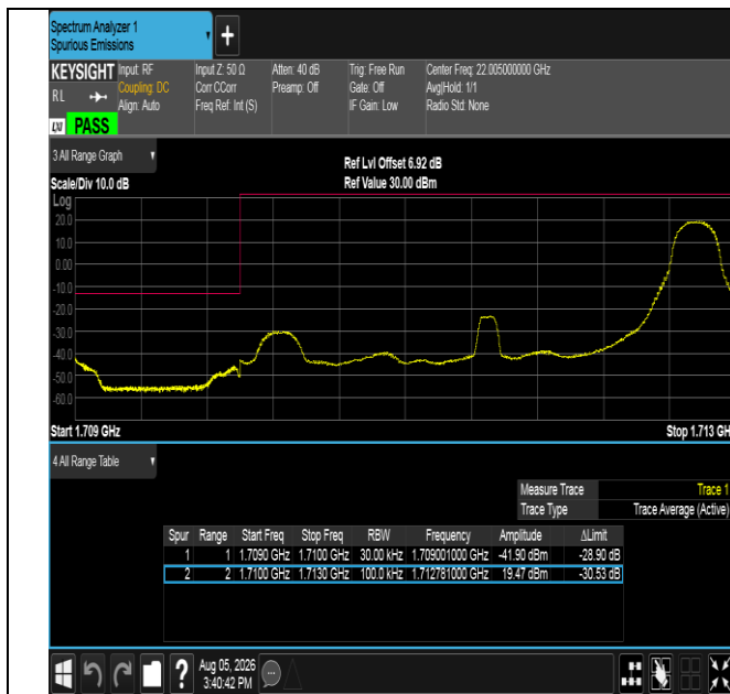
Band66-3MHz-16QAM-131987-1RB#14-PASS
