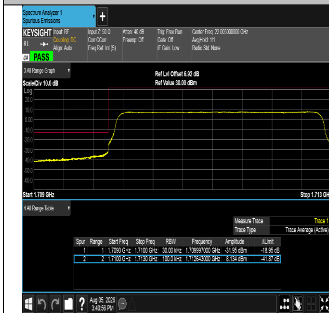
Band66-3MHz-QPSK-131987-15RB#0-PASS
