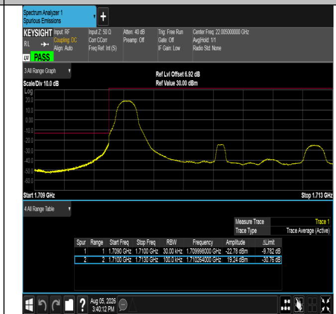
Band66-3MHz-16QAM-131987-1RB#0-PASS
