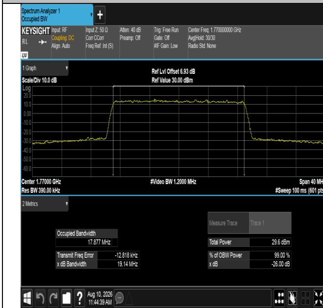
Band66-20MHz-QPSK-132572-100RB#0-PASS
