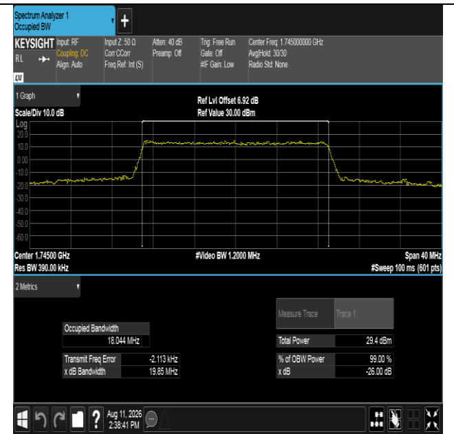
Band66-20MHz-16QAM-132322-100RB#0-PASS
