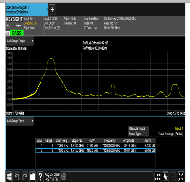
Band66-5MHz-16QAM-131997-1RB#0-PASS
