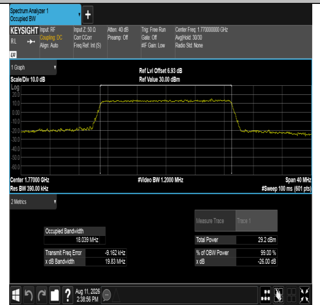
Band66-20MHz-16QAM-132572-100RB#0-PASS
