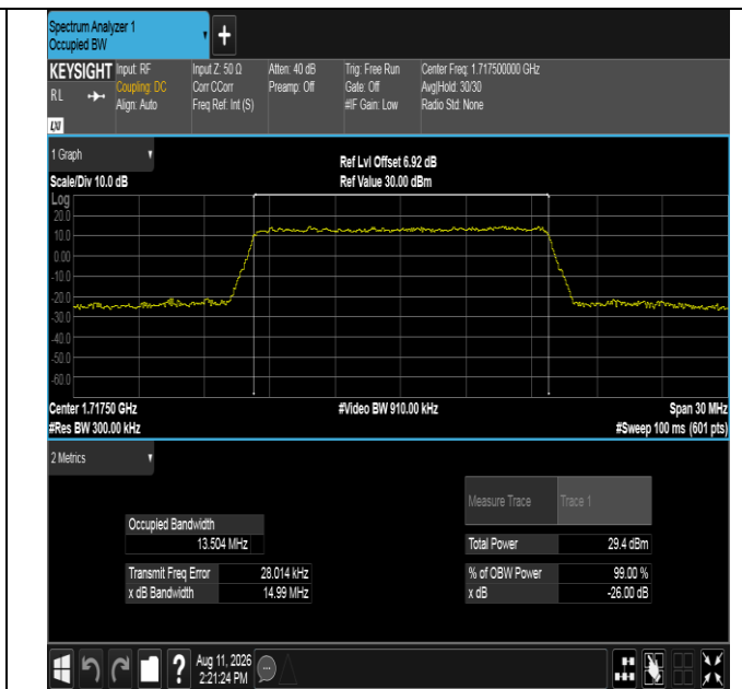
Band66-15MHz-16QAM-132047-75RB#0-PASS
