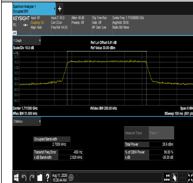
Band66-3MHz-QPSK-131987-15RB#0-PASS
