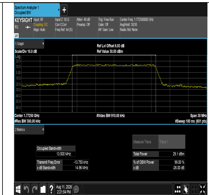
Band66-15MHz-16QAM-132597-75RB#0-PASS
