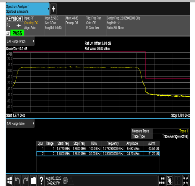
Band66-3MHz-16QAM-132657-15RB#0-PASS
