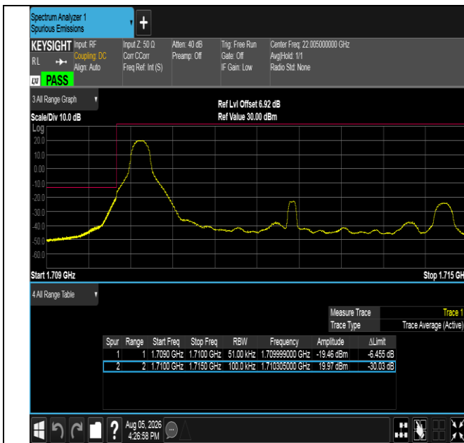
Band66-5MHz-QPSK-131997-1RB#0-PASS
