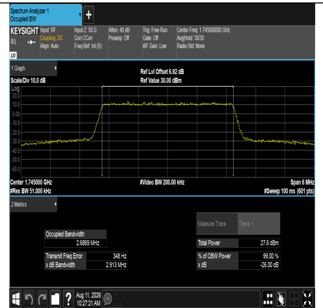
Band66-3MHz-16QAM-132322-15RB#0-PASS
