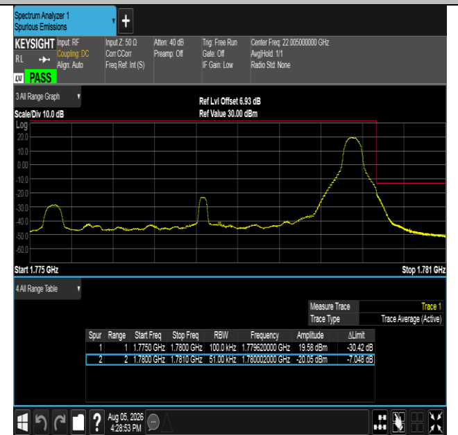
Band66-5MHz-QPSK-132647-1RB#24-PASS
