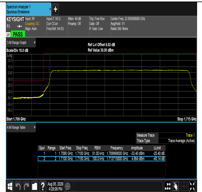
Band66-5MHz-16QAM-131997-25RB#0-PASS
