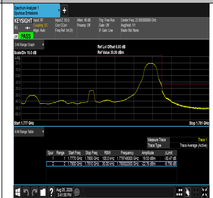
Band66-3MHz-QPSK-132657-1RB#14-PASS
