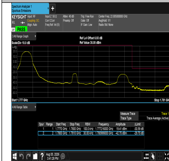
Band66-3MHz-QPSK-132657-1RB#0-PASS
