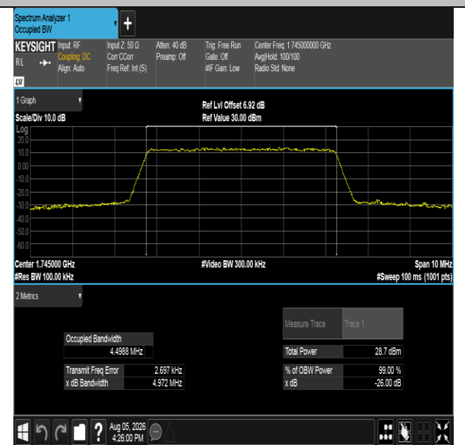
Band66-5MHz-16QAM-132322-25RB#0-PASS
