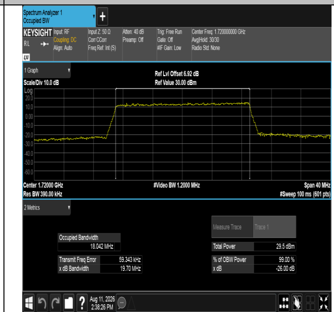
Band66-20MHz-16QAM-132072-100RB#0-PASS
