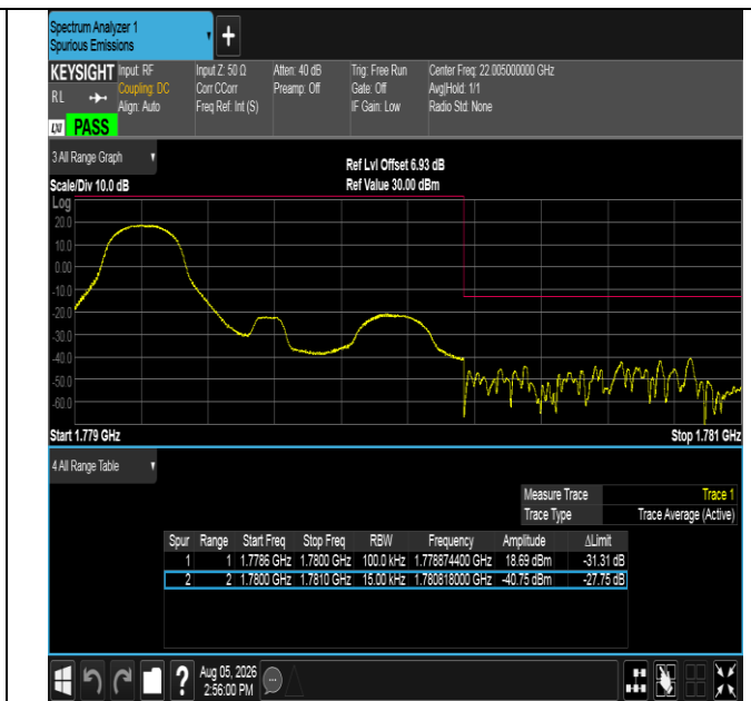
Band66-1.4MHz-16QAM-132665-1RB#0-PASS
