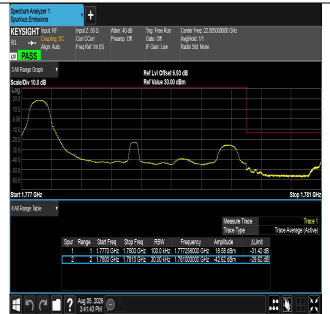
Band66-3MHz-16QAM-132657-1RB#0-PASS
