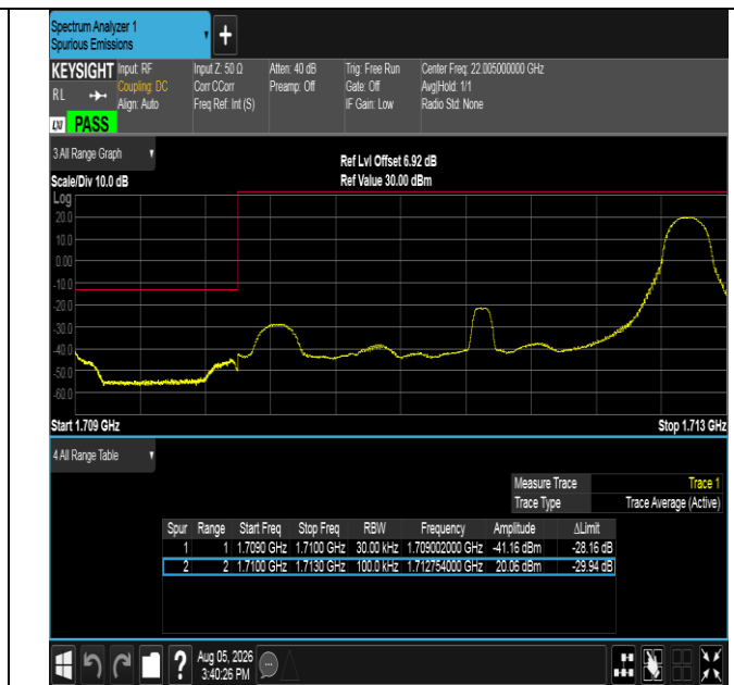
Band66-3MHz-QPSK-131987-1RB#14-PASS
