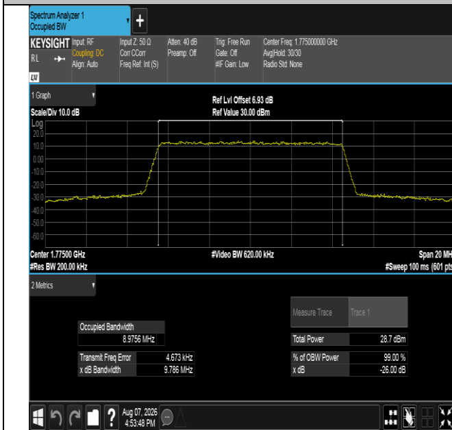
Band66-10MHz-QPSK-132622-50RB#0-PASS
