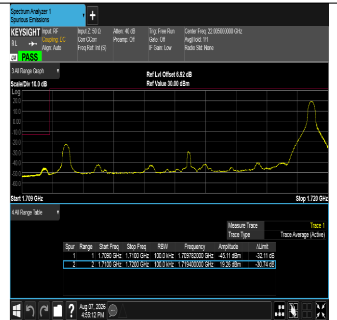
Band66-10MHz-QPSK-132022-1RB#49-PASS
