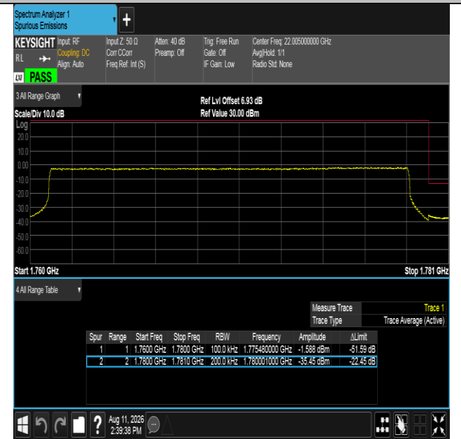
Band66-20MHz-16QAM-132572-100RB#0-PASS
