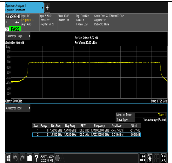
Band66-15MHz-16QAM-132047-75RB#0-PASS
