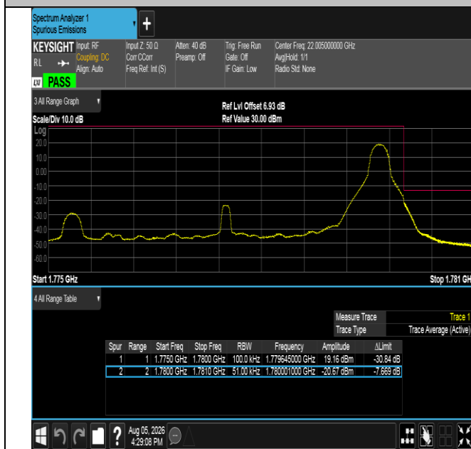
Band66-5MHz-16QAM-132647-1RB#24-PASS
