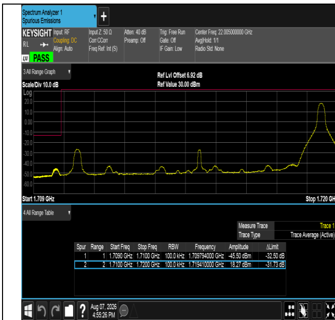
Band66-10MHz-16QAM-132022-1RB#49-PASS
