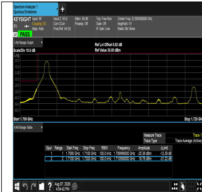
Band66-10MHz-QPSK-132022-1RB#0-PASS
