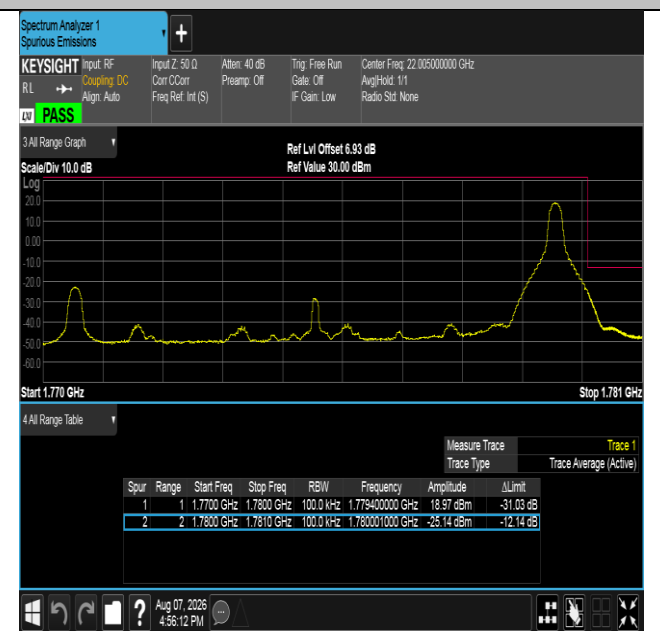
Band66-10MHz-QPSK-132622-1RB#49-PASS
