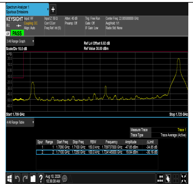
Band66-15MHz-QPSK-132047-1RB#74-PASS
