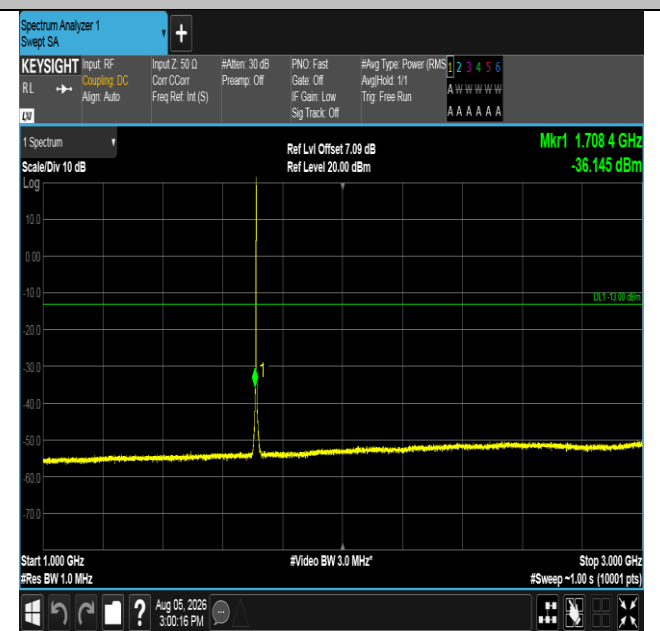
Band66-1.4MHz-16QAM-131979-1RB#5-1000~3000-PASS
