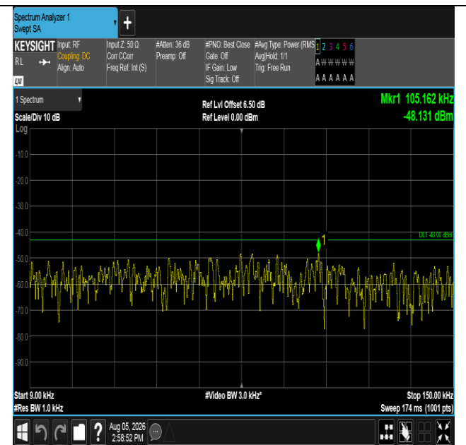
Band66-1.4MHz-QPSK-131979-1RB#5-0.009~0.15-PASS
