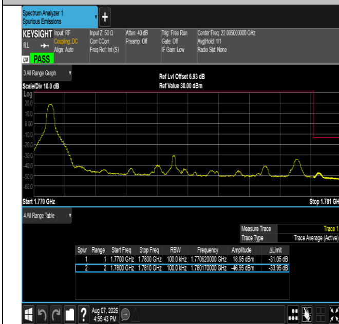
Band66-10MHz-QPSK-132622-1RB#0-PASS
