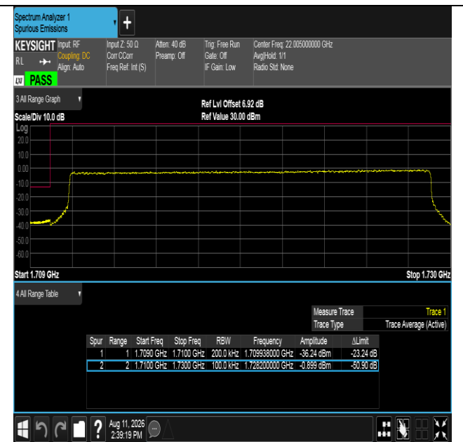
Band66-20MHz-16QAM-132072-100RB#0-PASS
