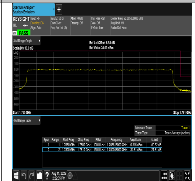
Band66-15MHz-16QAM-132597-75RB#0-PASS
