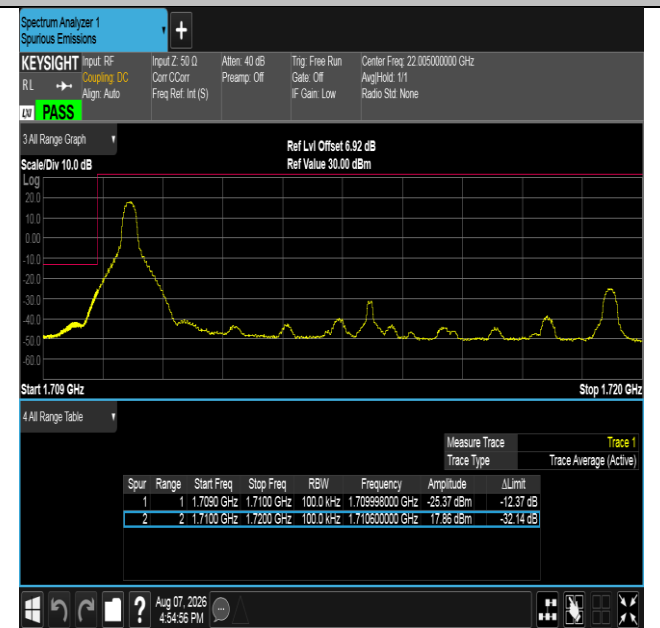
Band66-10MHz-16QAM-132022-1RB#0-PASS
