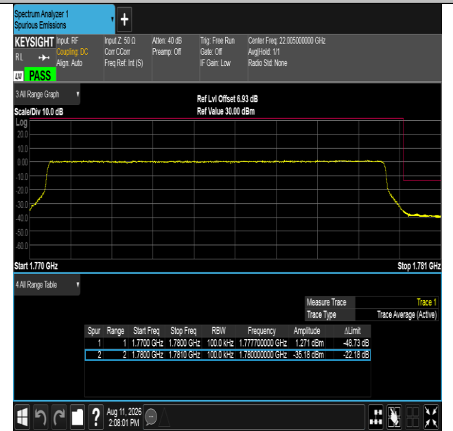
Band66-10MHz-16QAM-132622-50RB#0-PASS
