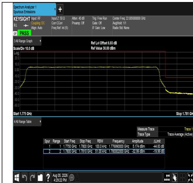
Band66-5MHz-QPSK-132647-25RB#0-PASS
