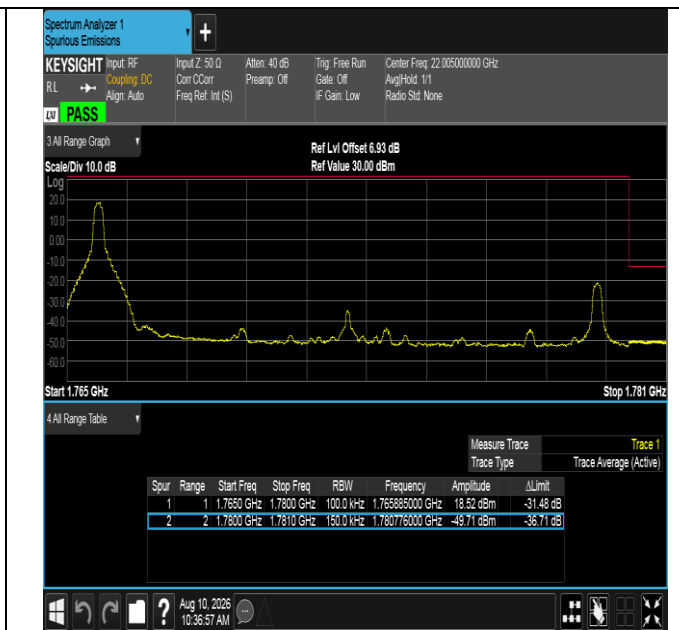
Band66-15MHz-16QAM-132597-1RB#0-PASS
