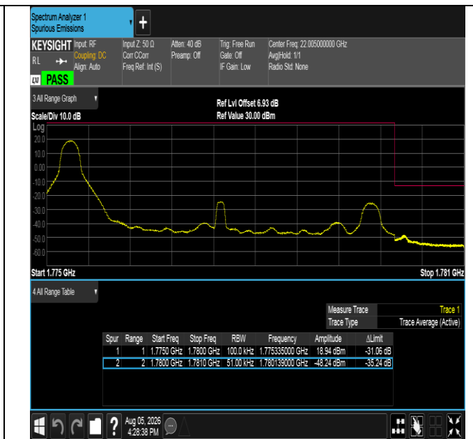
Band66-5MHz-16QAM-132647-1RB#0-PASS
