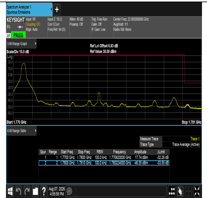
Band66-10MHz-16QAM-132622-1RB#0-PASS
