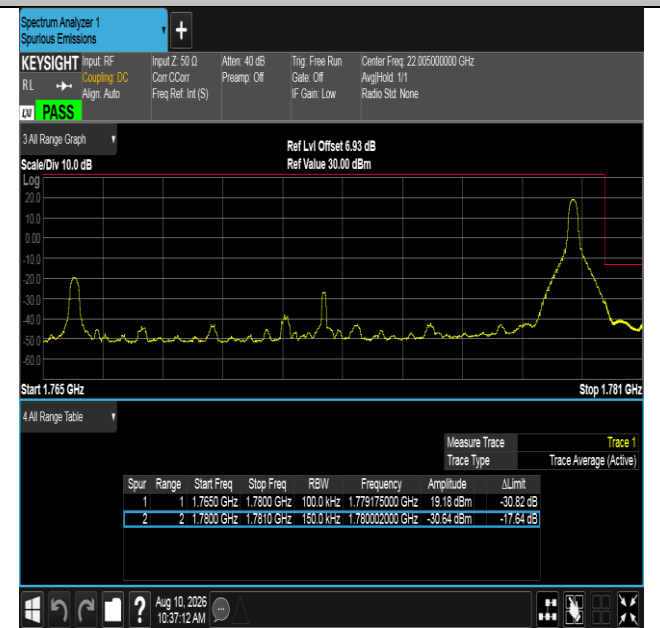
Band66-15MHz-QPSK-132597-1RB#74-PASS
