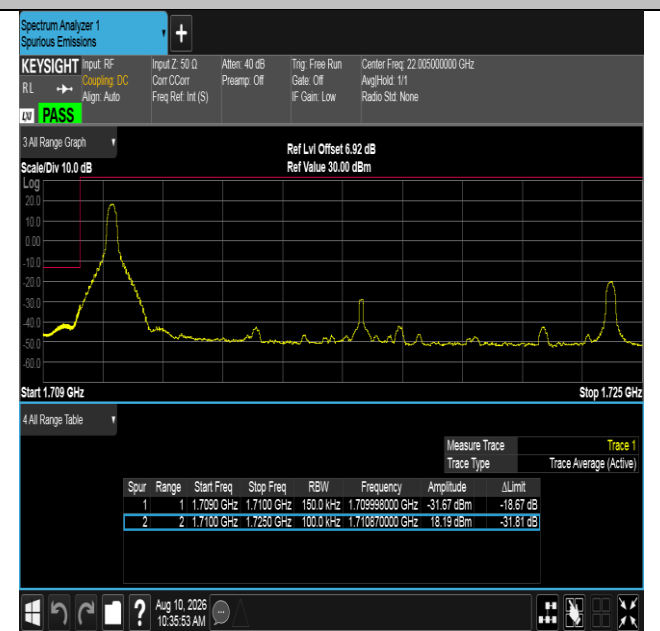
Band66-15MHz-16QAM-132047-1RB#0-PASS
