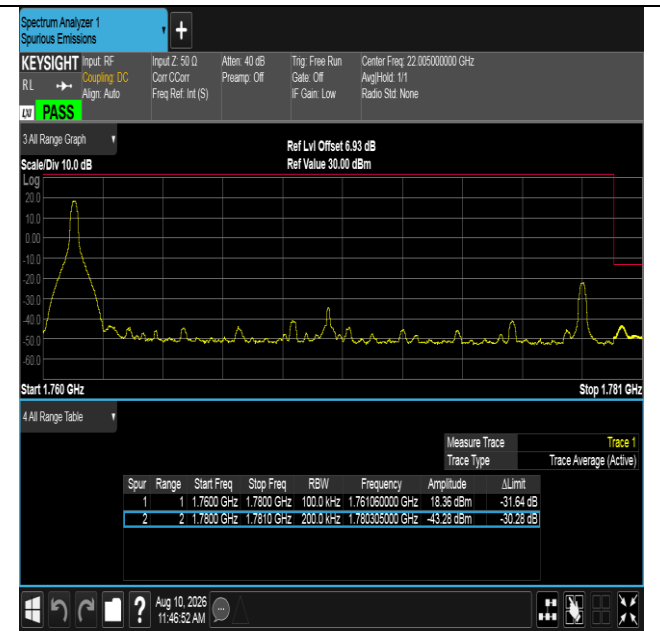
Band66-20MHz-16QAM-132572-1RB#0-PASS
