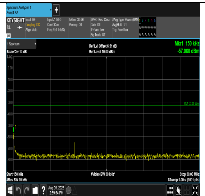
Band66-1.4MHz-16QAM-131979-1RB#5-0.15~30-PASS
