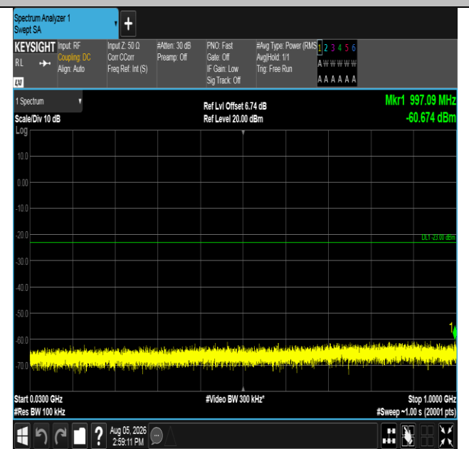
Band66-1.4MHz-QPSK-131979-1RB#5-30~1000-PASS
