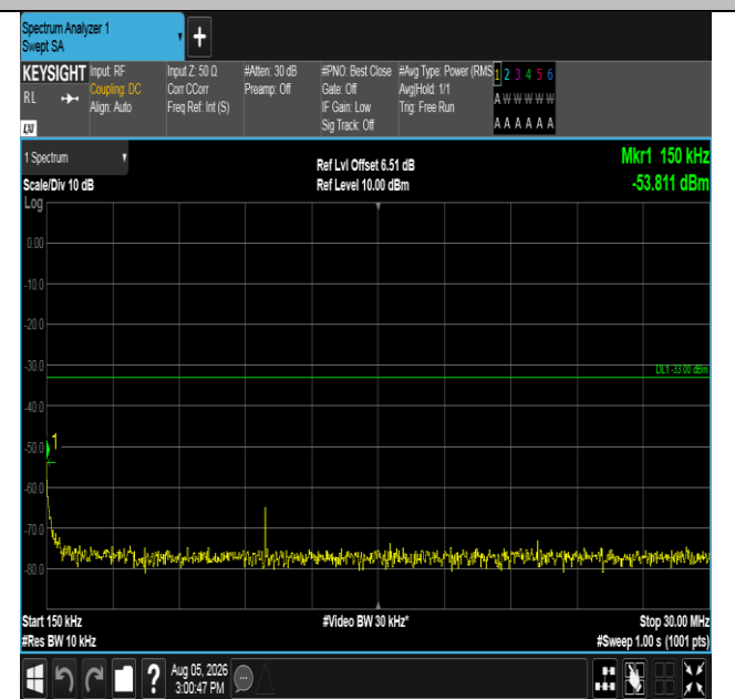
Band66-1.4MHz-QPSK-131979-6RB#0-0.15~30-PASS
