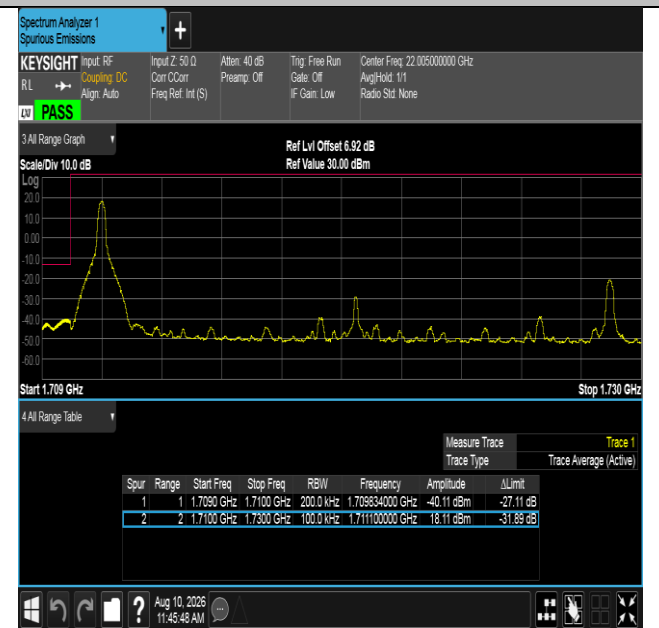
Band66-20MHz-16QAM-132072-1RB#0-PASS
