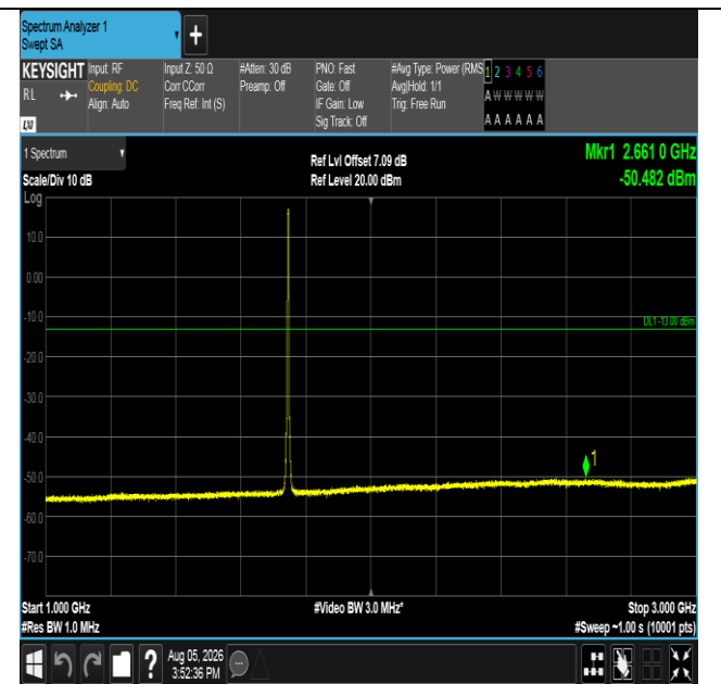
Band66-3MHz-QPSK-132322-15RB#0-1000~3000-PASS
