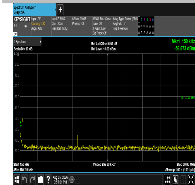
Band66-3MHz-16QAM-132657-1RB#0-0.15~30-PASS
