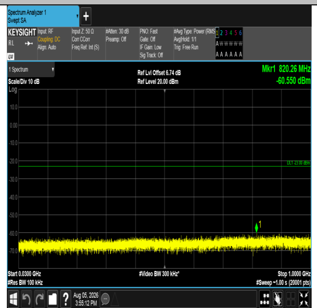
Band66-3MHz-16QAM-132657-1RB#0-30~1000-PASS
