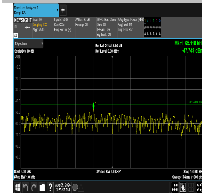
Band66-3MHz-QPSK-132657-1RB#0-0.009~0.15-PASS
