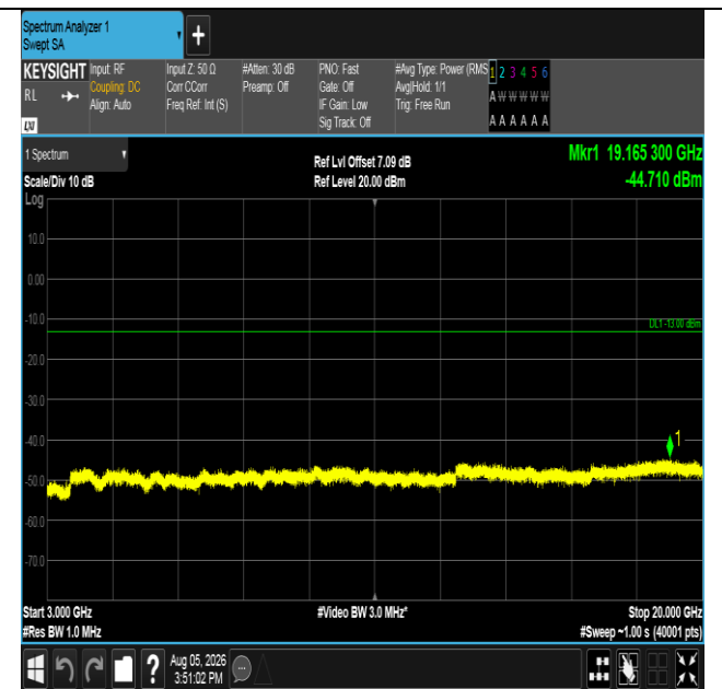
Band66-3MHz-QPSK-132322-1RB#14-3000~20000-PASS
