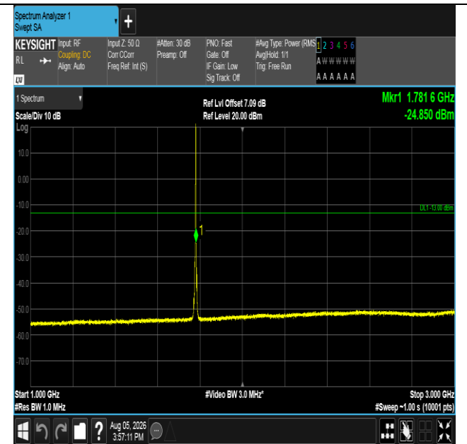
Band66-3MHz-16QAM-132657-1RB#14-1000~3000-PASS
