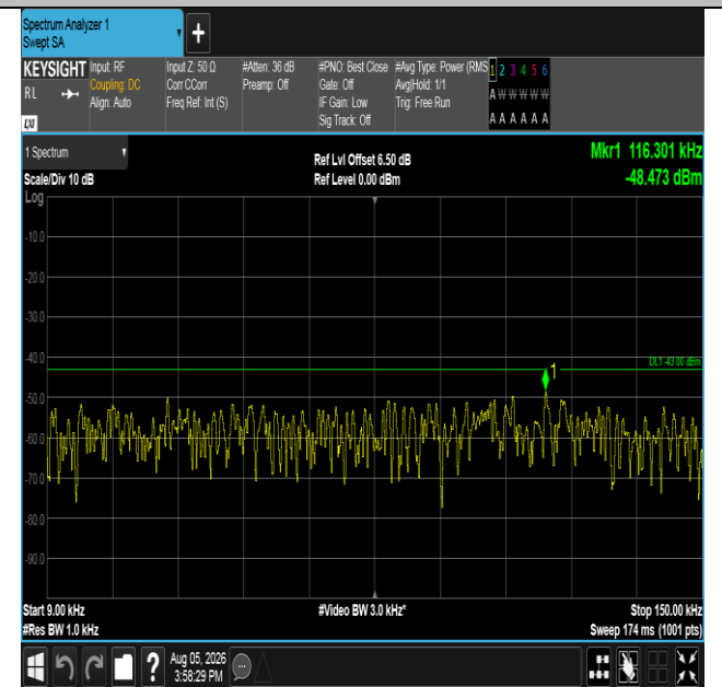
Band66-3MHz-16QAM-132657-15RB#0-0.009~0.15-PASS
