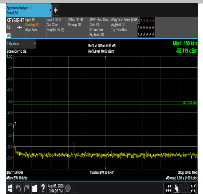
Band66-3MHz-QPSK-132657-1RB#0-0.15~30-PASS
