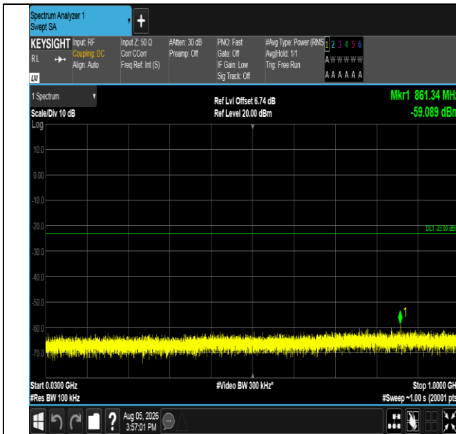
Band66-3MHz-16QAM-132657-1RB#14-30~1000-PASS
