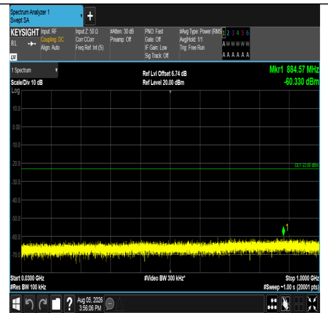
Band66-3MHz-QPSK-132657-1RB#14-30~1000-PASS
