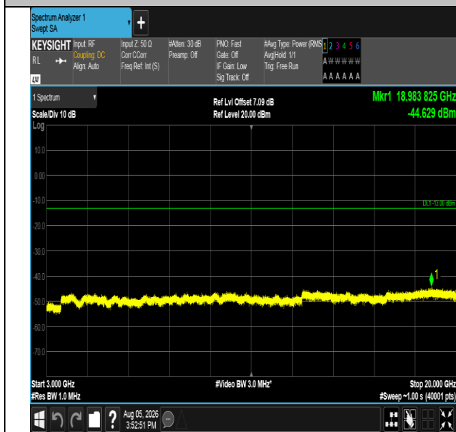
Band66-3MHz-QPSK-132322-15RB#0-3000~20000-PASS
