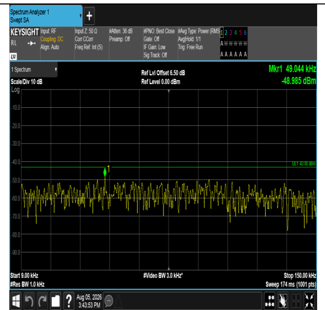
Band66-3MHz-16QAM-131987-1RB#0-0.009~0.15-PASS
