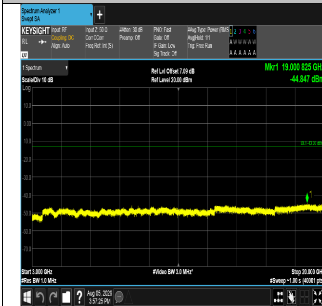
Band66-3MHz-16QAM-132657-1RB#14-3000~20000-PASS
