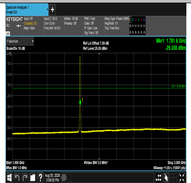
Band66-3MHz-QPSK-132657-15RB#0-1000~3000-PASS
