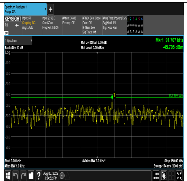
Band66-3MHz-16QAM-132657-1RB#0-0.009~0.15-PASS
