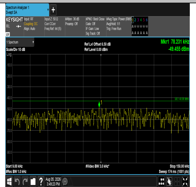
Band66-3MHz-16QAM-132322-1RB#0-0.009~0.15-PASS
