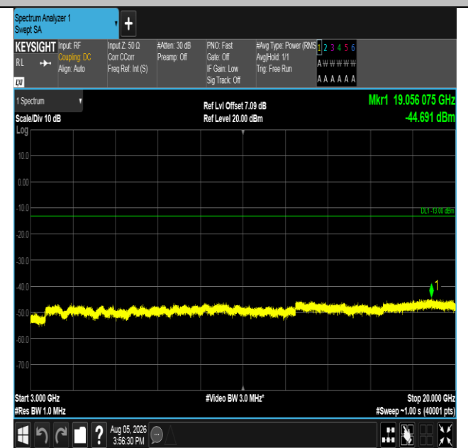
Band66-3MHz-QPSK-132657-1RB#14-3000~20000-PASS
