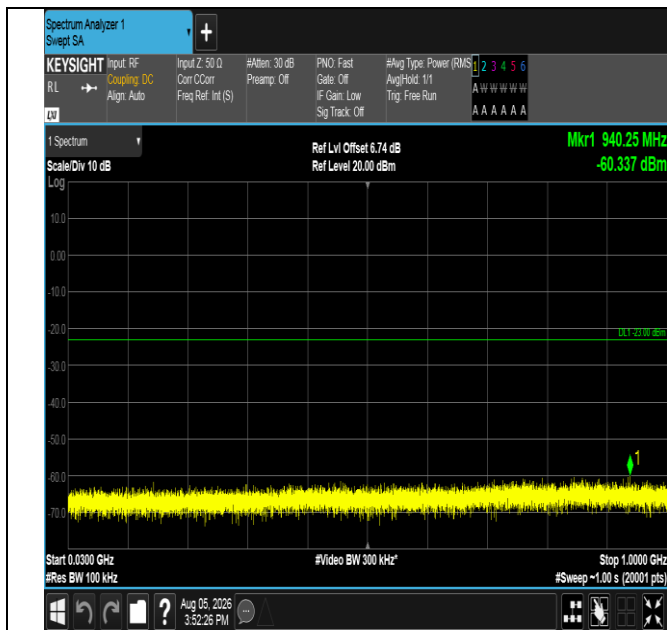
Band66-3MHz-QPSK-132322-15RB#0-30~1000-PASS
