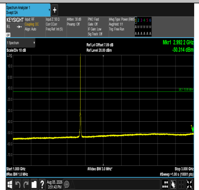
Band66-3MHz-16QAM-132322-1RB#14-1000~3000-PASS
