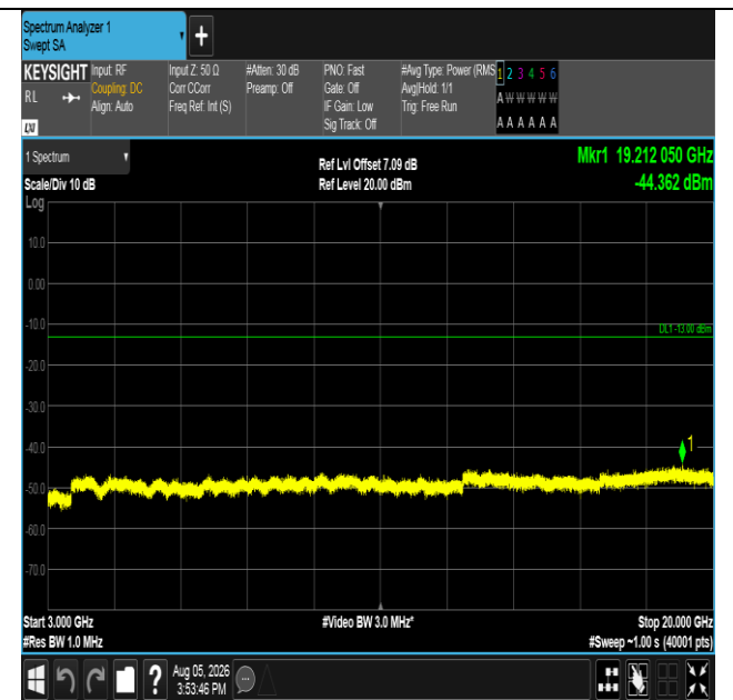
Band66-3MHz-16QAM-132322-15RB#0-3000~20000-PASS
