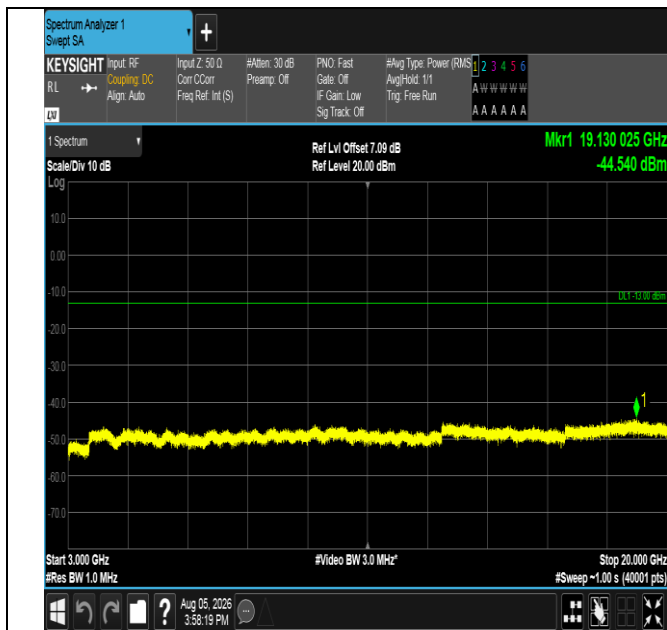
Band66-3MHz-QPSK-132657-15RB#0-3000~20000-PASS
