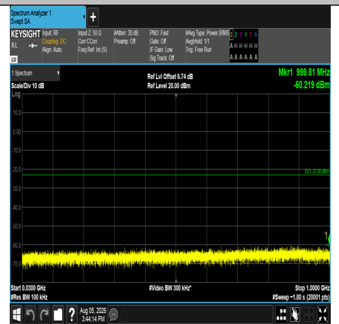
Band66-3MHz-16QAM-131987-1RB#0-30~1000-PASS
