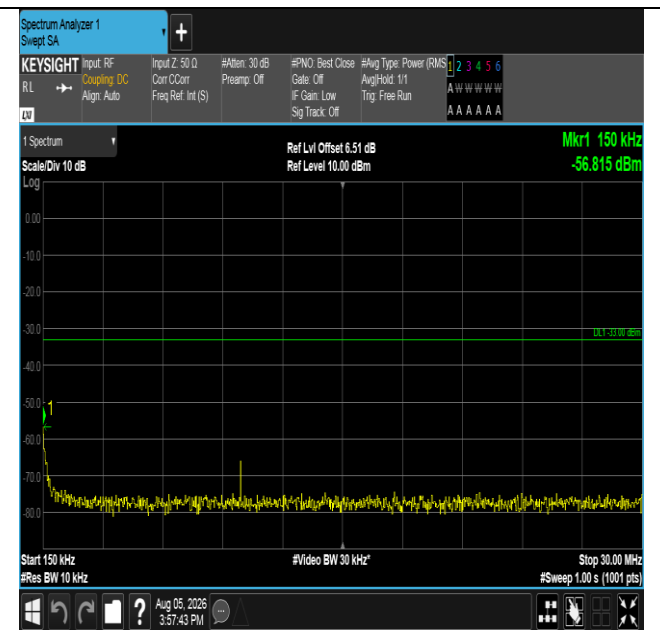
Band66-3MHz-QPSK-132657-15RB#0-0.15~30-PASS
