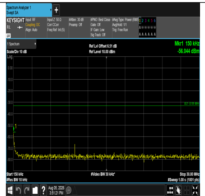
Band66-3MHz-16QAM-132322-1RB#14-0.15~30-PASS
