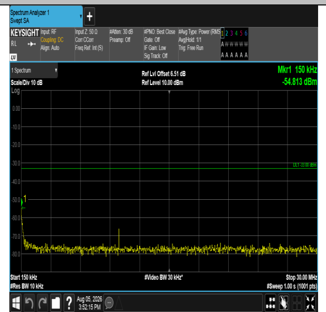
Band66-3MHz-QPSK-132322-15RB#0-0.15~30-PASS
