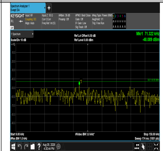
Band66-5MHz-16QAM-131997-1RB#0-0.009~0.15-PASS
