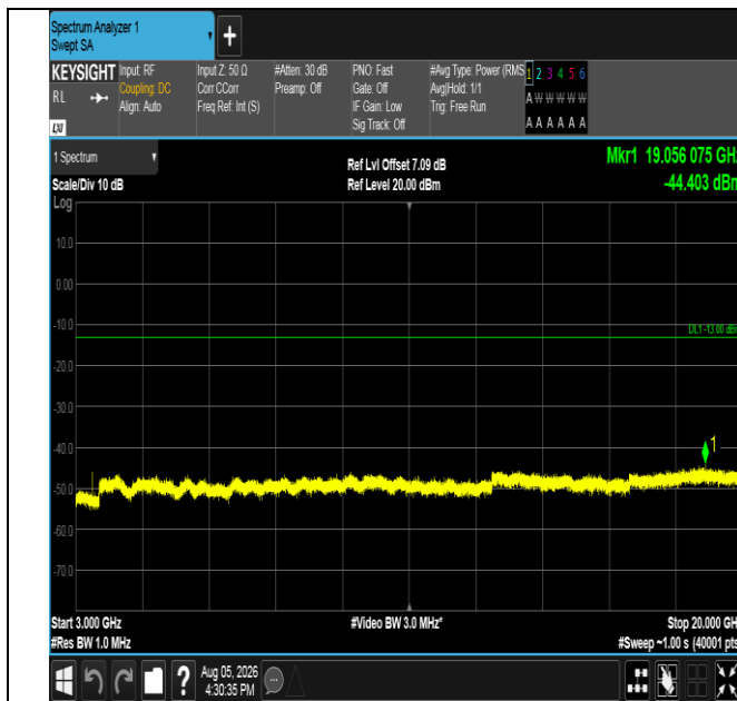
Band66-5MHz-QPSK-131997-1RB#0-3000~20000-PASS
