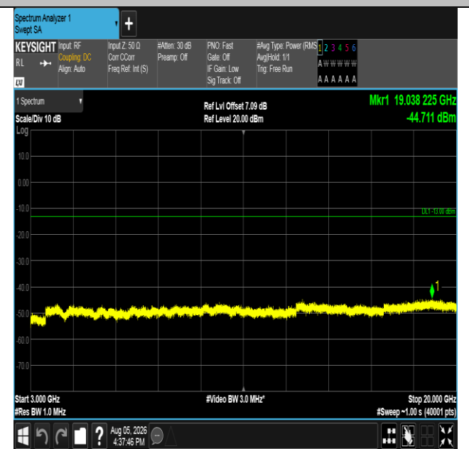
Band66-5MHz-QPSK-132322-1RB#24-3000~20000-PASS
