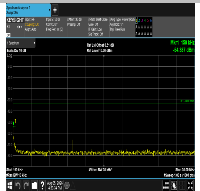
Band66-5MHz-QPSK-131997-25RB#0-0.15~30-PASS
