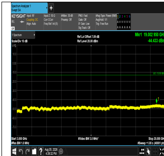
Band66-5MHz-QPSK-132322-25RB#0-3000~20000-PASS
