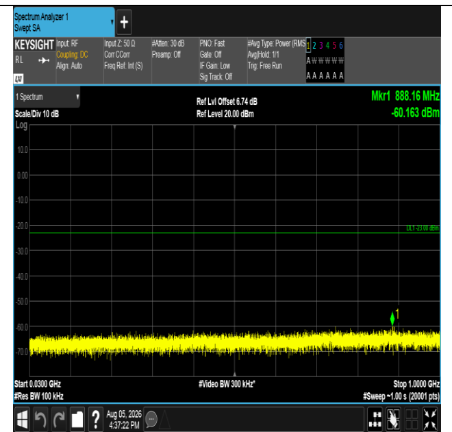
Band66-5MHz-QPSK-132322-1RB#24-30~1000-PASS
