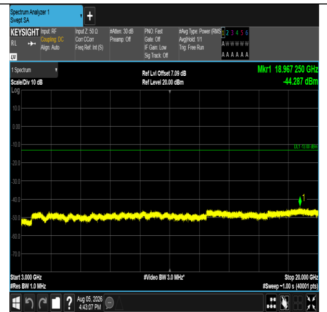
Band66-5MHz-QPSK-132647-1RB#24-3000~20000-PASS
