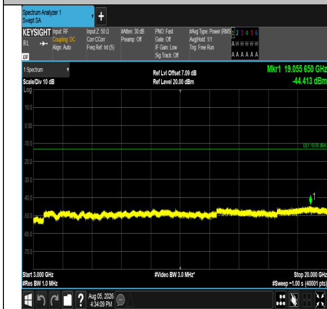
Band66-5MHz-QPSK-131997-25RB#0-3000~20000-PASS
