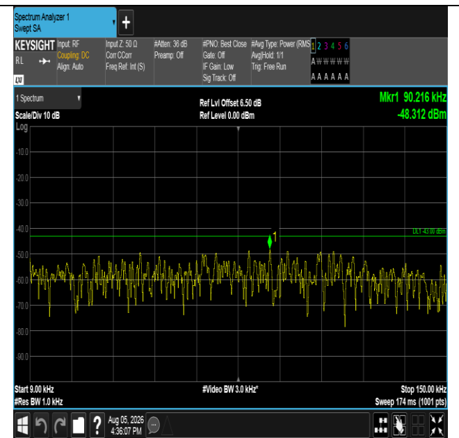
Band66-5MHz-16QAM-132322-1RB#0-0.009~0.15-PASS
