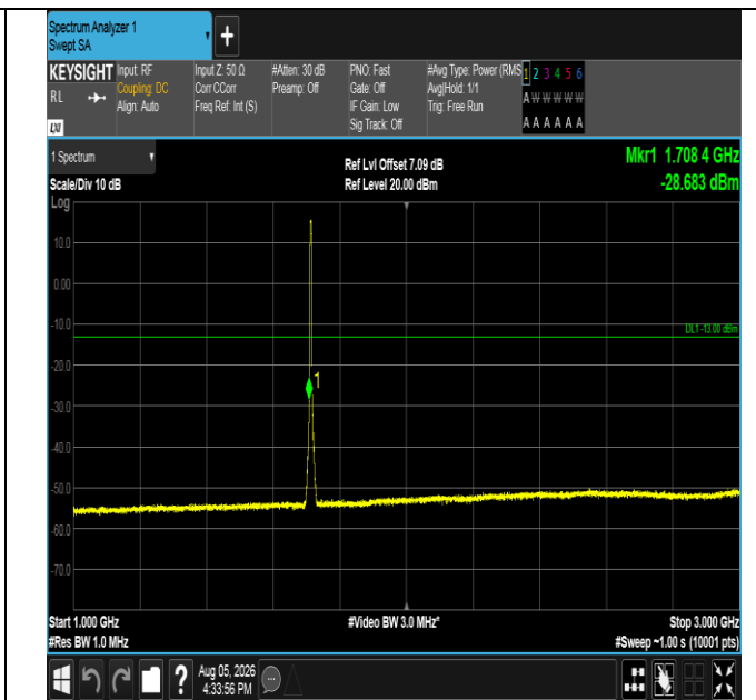
Band66-5MHz-QPSK-131997-25RB#0-1000~3000-PASS
