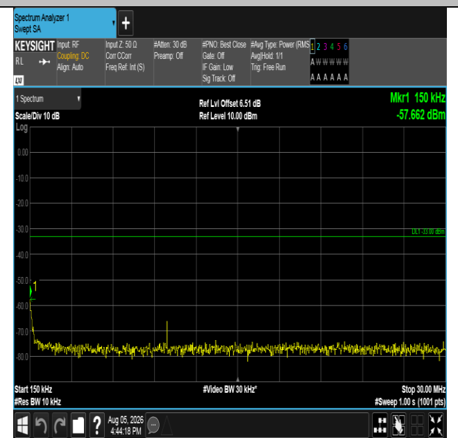
Band66-5MHz-QPSK-132647-25RB#0-0.15~30-PASS
