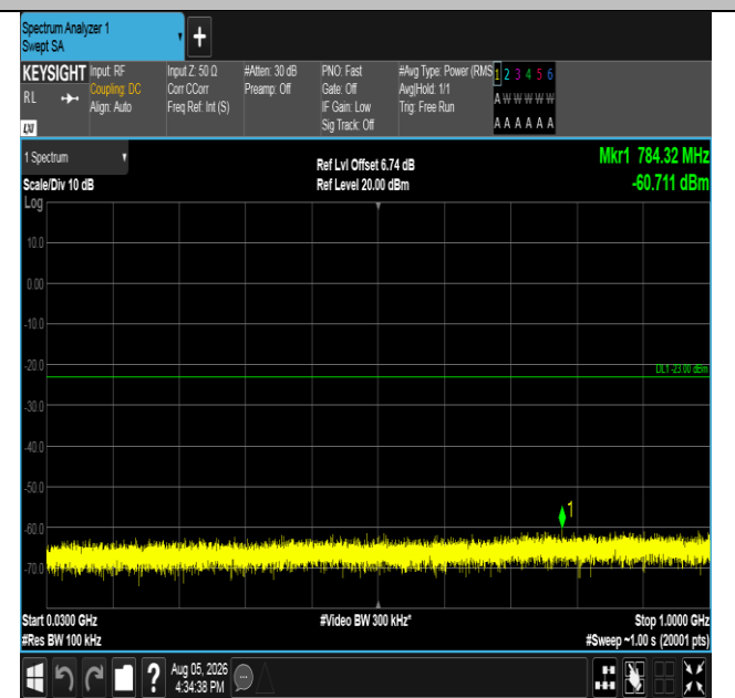
Band66-5MHz-16QAM-131997-25RB#0-30~1000-PASS
