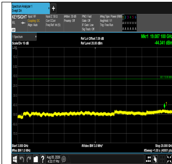
Band66-5MHz-16QAM-131997-1RB#24-3000~20000-PASS
