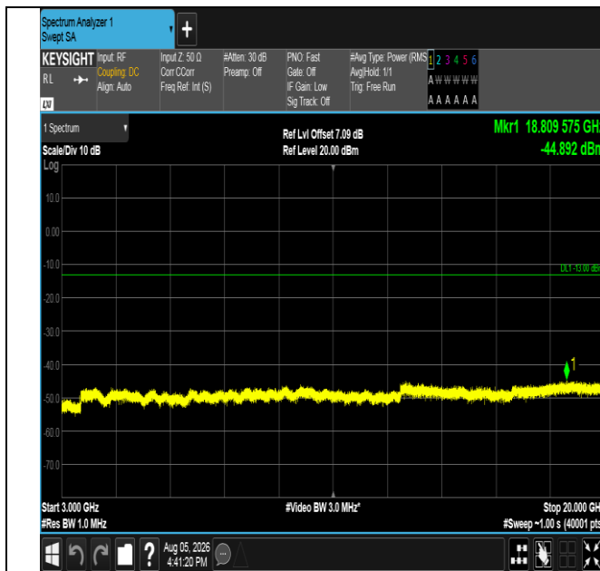
Band66-5MHz-QPSK-132647-1RB#0-3000~20000-PASS
