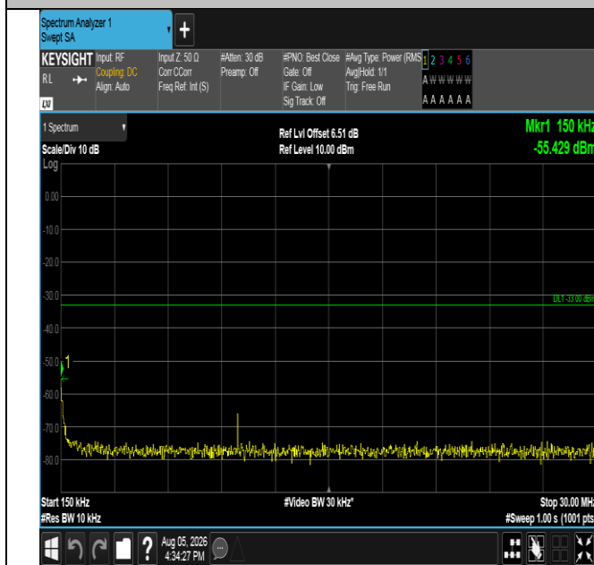
Band66-5MHz-16QAM-131997-25RB#0-0.15~30-PASS
