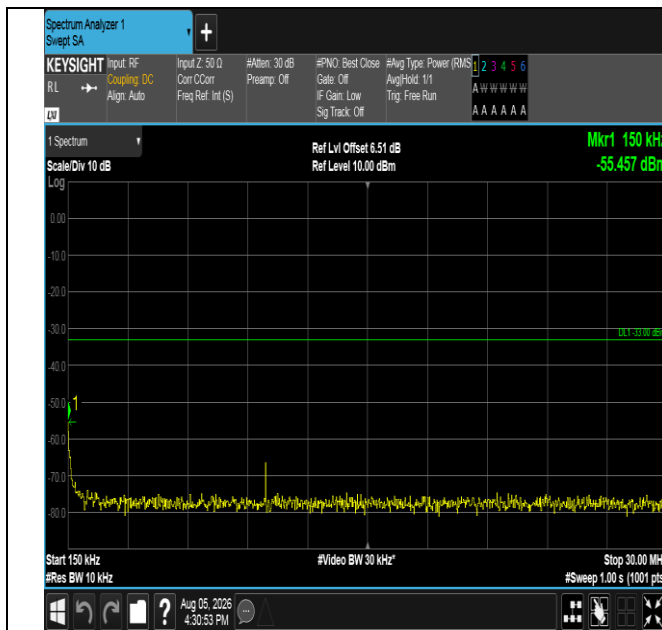
Band66-5MHz-16QAM-131997-1RB#0-0.15~30-PASS
