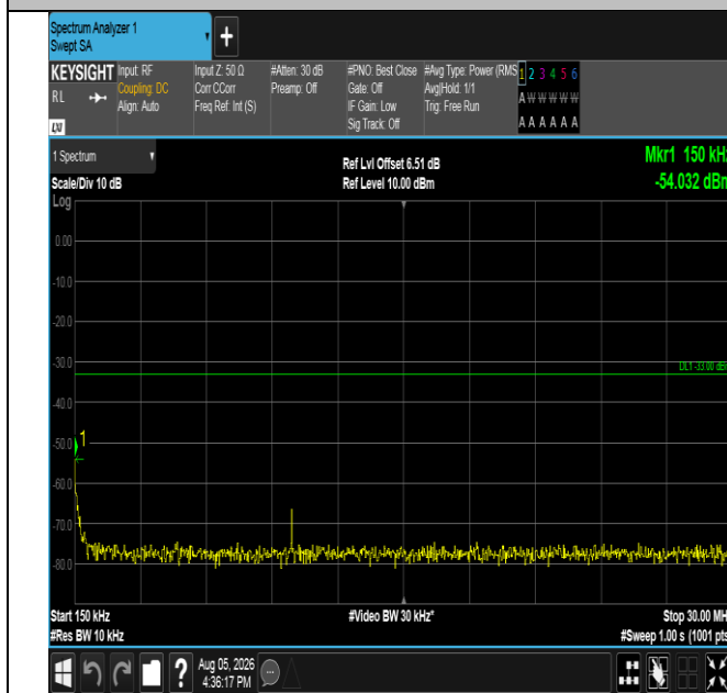
Band66-5MHz-16QAM-132322-1RB#0-0.15~30-PASS
