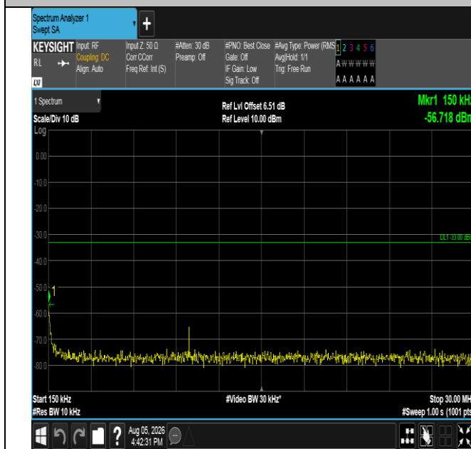
Band66-5MHz-QPSK-132647-1RB#24-0.15~30-PASS
