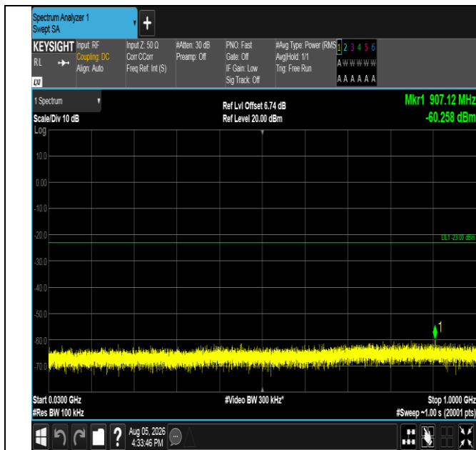
Band66-5MHz-QPSK-131997-25RB#0-30~1000-PASS
