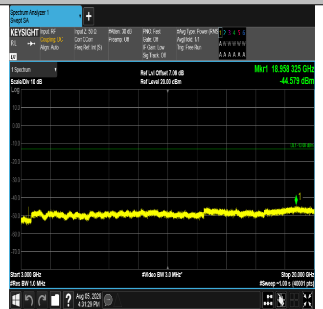
Band66-5MHz-16QAM-131997-1RB#0-3000~20000-PASS
