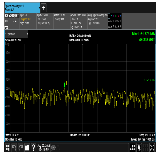
Band66-5MHz-16QAM-131997-25RB#0-0.009~0.15-PASS
