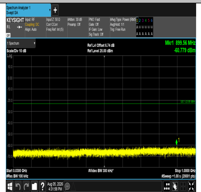
Band66-5MHz-QPSK-131997-1RB#24-30~1000-PASS
