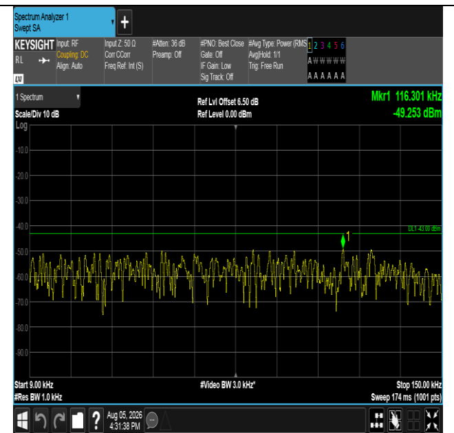
Band66-5MHz-QPSK-131997-1RB#24-0.009~0.15-PASS
