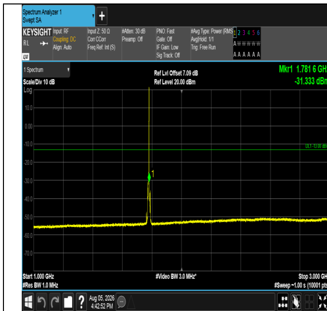
Band66-5MHz-QPSK-132647-1RB#24-1000~3000-PASS
