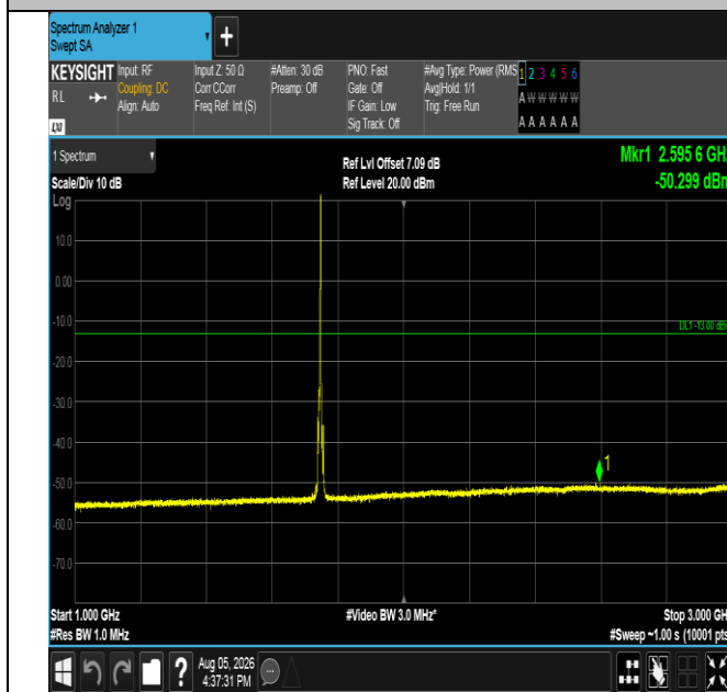
Band66-5MHz-QPSK-132322-1RB#24-1000~3000-PASS
