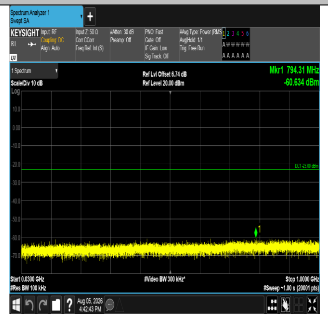
Band66-5MHz-QPSK-132647-1RB#24-30~1000-PASS
