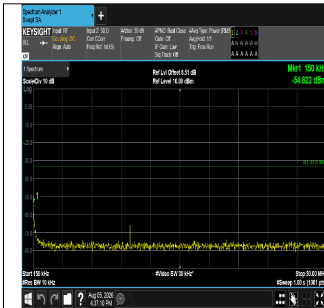
Band66-5MHz-QPSK-132322-1RB#24-0.15~30-PASS
