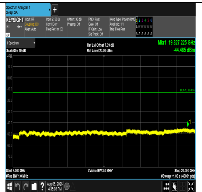
Band66-5MHz-16QAM-131997-25RB#0-3000~20000-PASS
