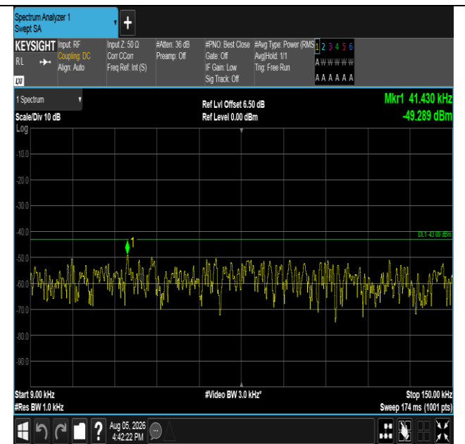
Band66-5MHz-QPSK-132647-1RB#24-0.009~0.15-PASS
