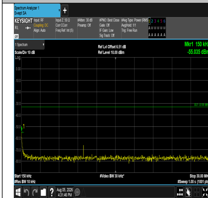
Band66-5MHz-QPSK-131997-1RB#24-0.15~30-PASS
