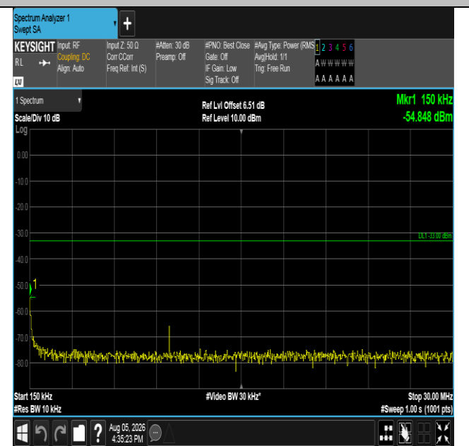
Band66-5MHz-QPSK-132322-1RB#0-0.15~30-PASS
