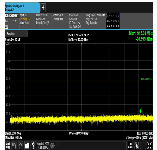
Band66-5MHz-16QAM-131997-1RB#0-30~1000-PASS
