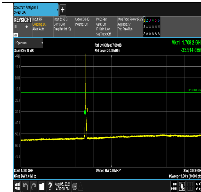
Band66-5MHz-QPSK-131997-1RB#24-1000~3000-PASS
