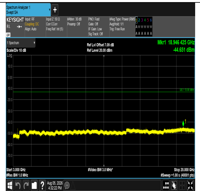
Band66-5MHz-QPSK-131997-1RB#24-3000~20000-PASS
