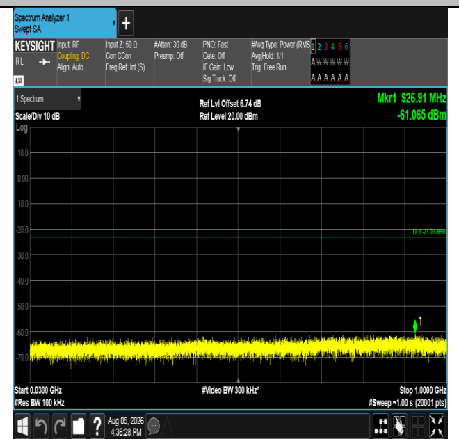
Band66-5MHz-16QAM-132322-1RB#0-30~1000-PASS
