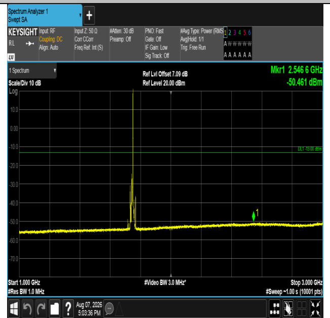
Band66-10MHz-16QAM-132322-1RB#49-1000~3000-PASS
