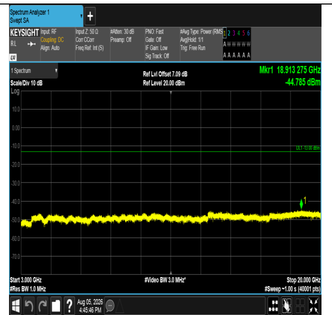
Band66-5MHz-16QAM-132647-25RB#0-3000~20000-PASS
