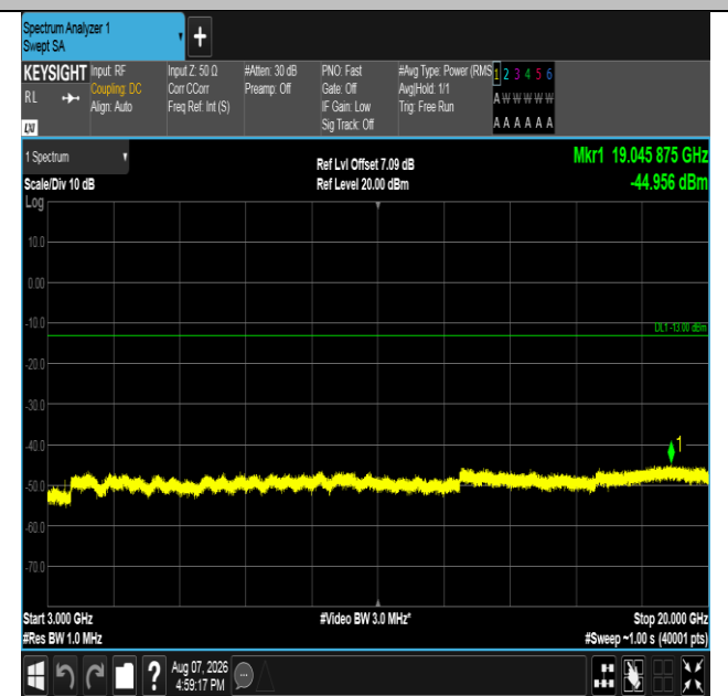
Band66-10MHz-QPSK-132022-1RB#49-3000~20000-PASS
