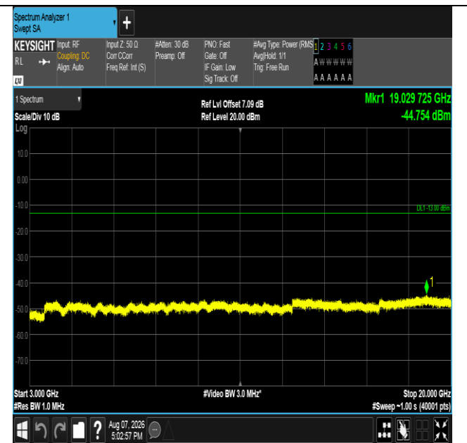
Band66-10MHz-QPSK-132322-1RB#49-3000~20000-PASS
