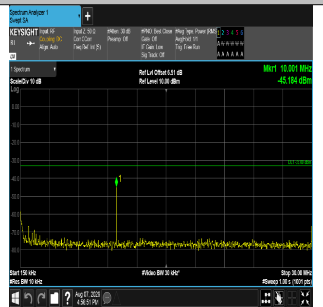
Band66-10MHz-QPSK-132022-1RB#0-0.15~30-PASS
