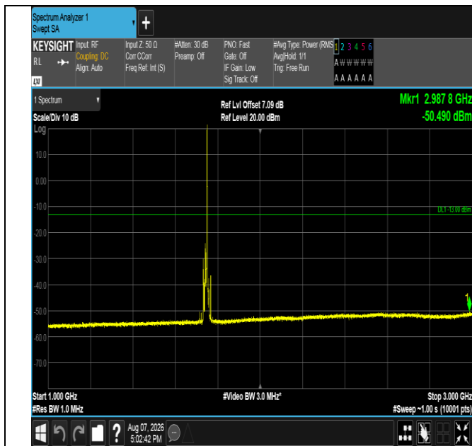
Band66-10MHz-QPSK-132322-1RB#49-1000~3000-PASS
