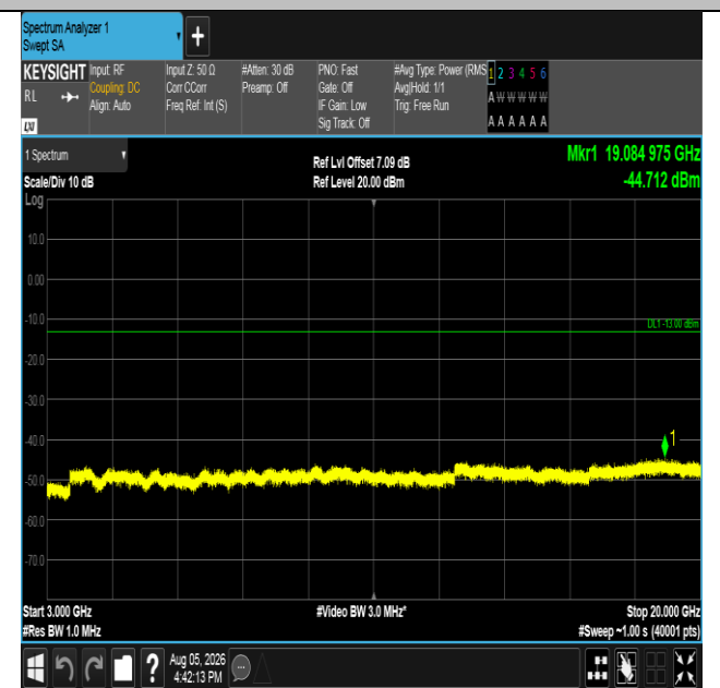
Band66-5MHz-16QAM-132647-1RB#0-3000~20000-PASS
