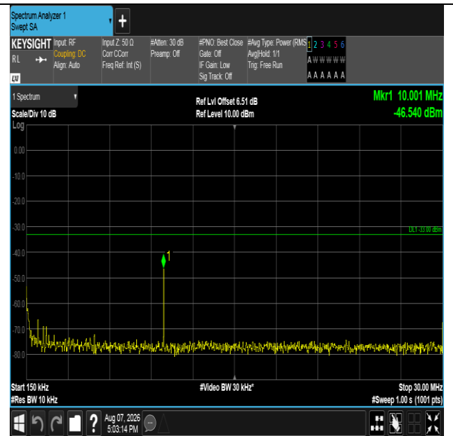
Band66-10MHz-16QAM-132322-1RB#49-0.15~30-PASS
