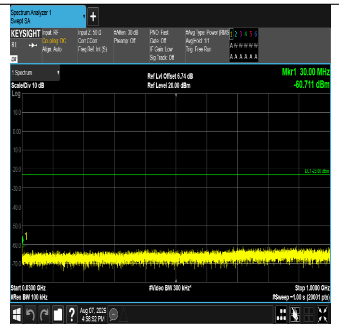
Band66-10MHz-QPSK-132022-1RB#49-30~1000-PASS
