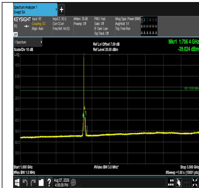
Band66-10MHz-16QAM-132022-1RB#0-1000~3000-PASS
