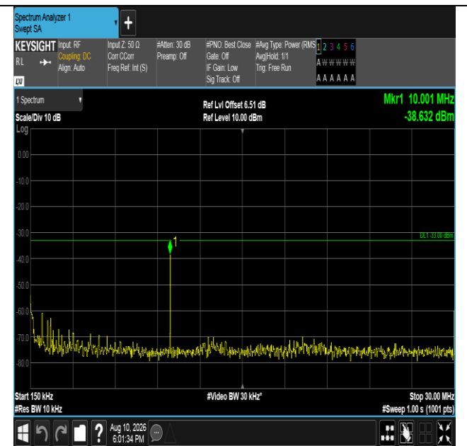
Band66-10MHz-QPSK-132022-50RB#0-0.15~30-PASS
