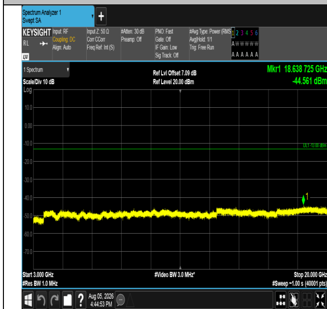
Band66-5MHz-QPSK-132647-25RB#0-3000~20000-PASS
