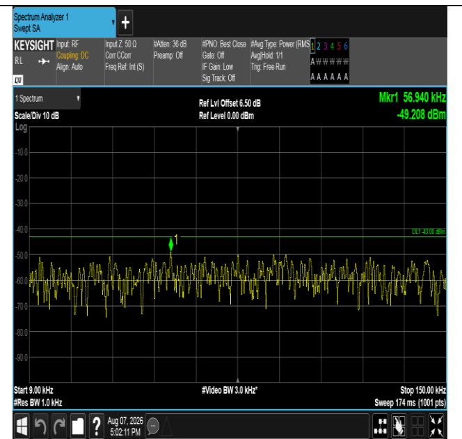
Band66-10MHz-QPSK-132322-1RB#49-0.009~0.15-PASS
