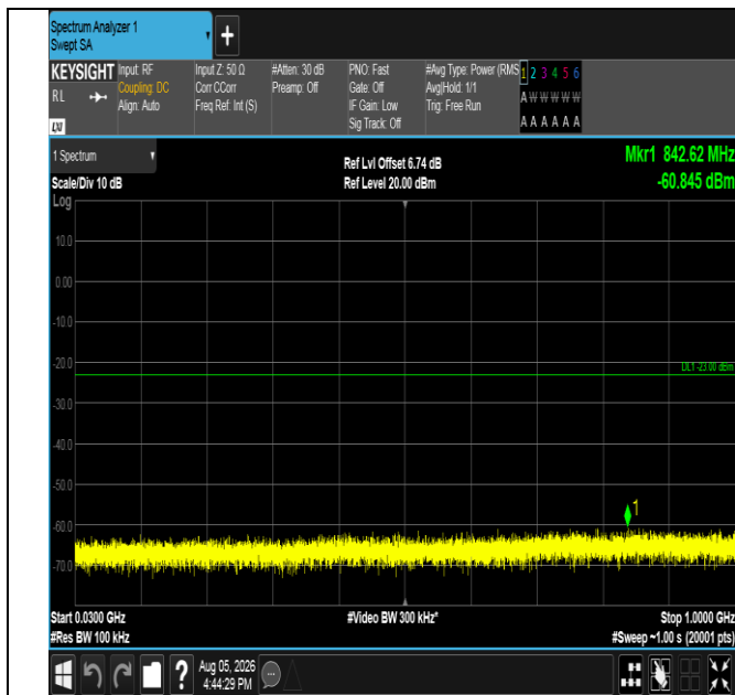
Band66-5MHz-QPSK-132647-25RB#0-30~1000-PASS
