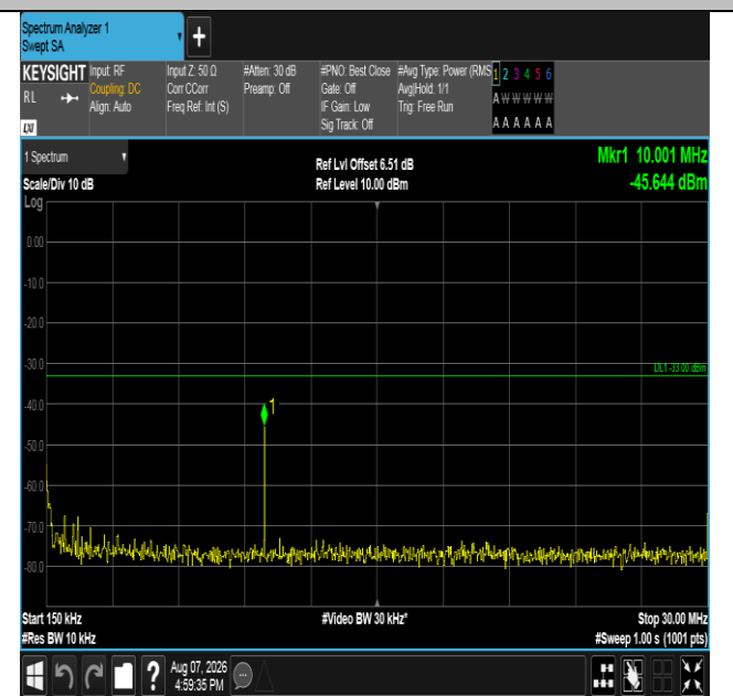
Band66-10MHz-16QAM-132022-1RB#49-0.15~30-PASS
