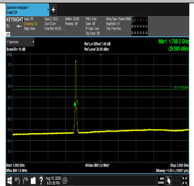
Band66-10MHz-QPSK-132022-50RB#0-1000~3000-PASS
