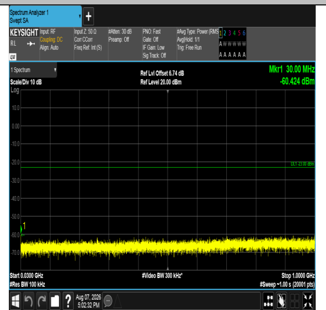
Band66-10MHz-QPSK-132322-1RB#49-30~1000-PASS
