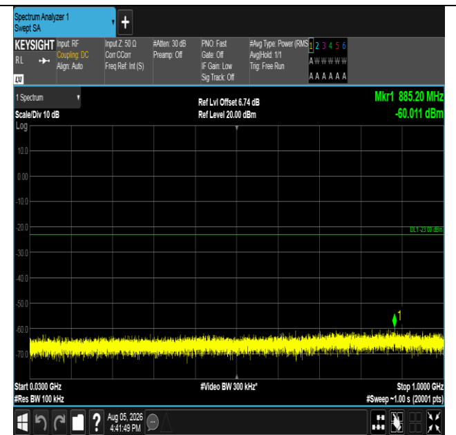
Band66-5MHz-16QAM-132647-1RB#0-30~1000-PASS
