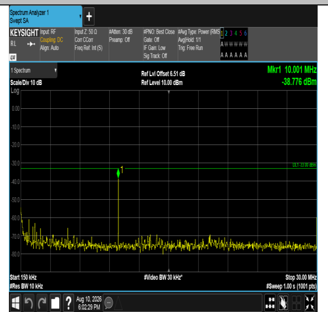
Band66-10MHz-QPSK-132322-50RB#0-0.15~30-PASS
