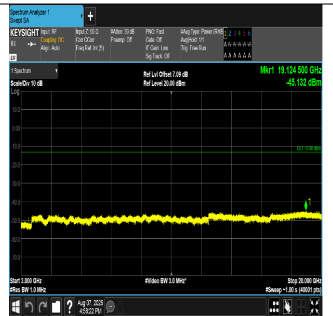
Band66-10MHz-16QAM-132022-1RB#0-3000~20000-PASS
