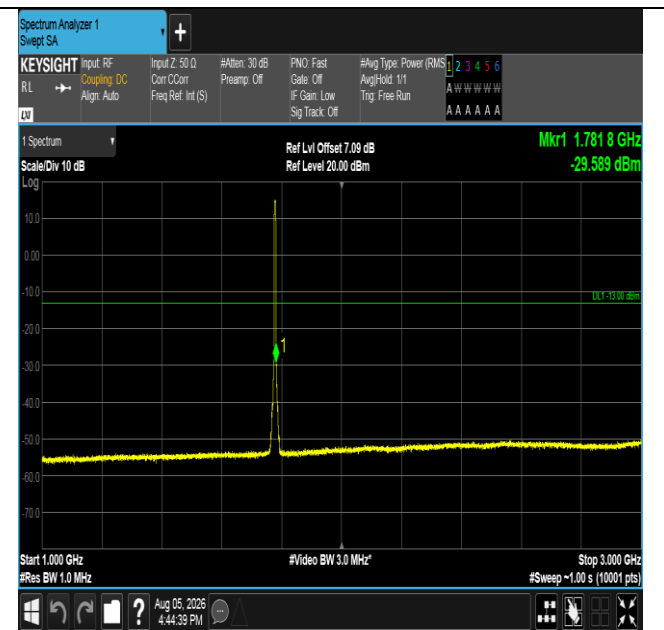
Band66-5MHz-QPSK-132647-25RB#0-1000~3000-PASS
