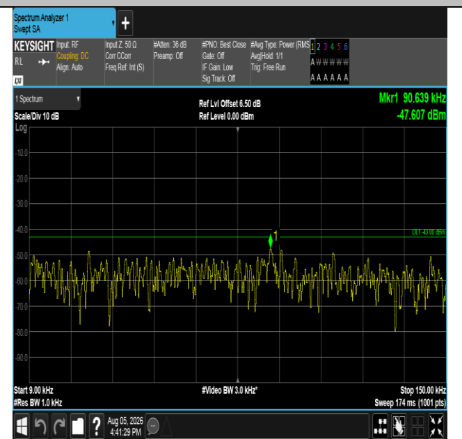
Band66-5MHz-16QAM-132647-1RB#0-0.009~0.15-PASS
