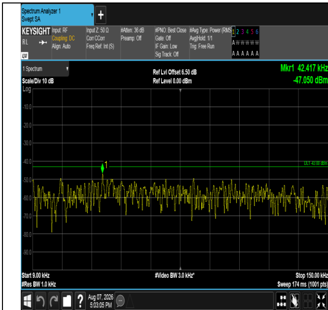
Band66-10MHz-16QAM-132322-1RB#49-0.009~0.15-PASS
