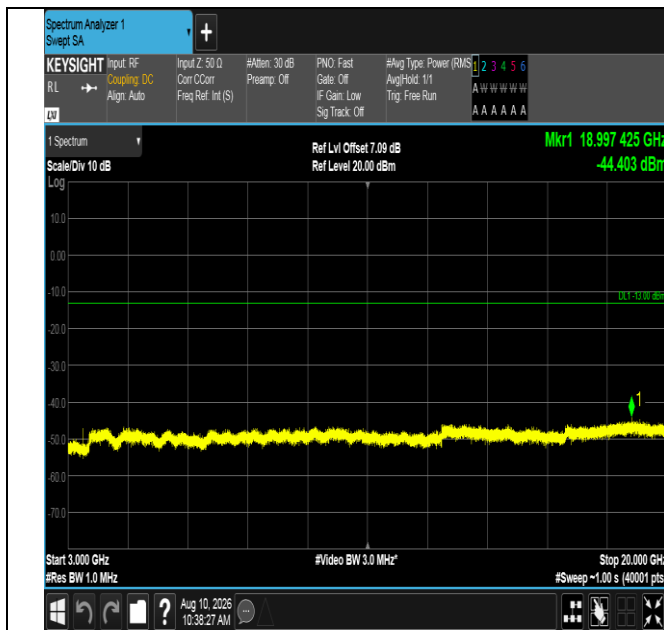
Band66-15MHz-QPSK-132047-1RB#0-3000~20000-PASS
