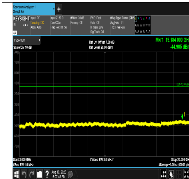
Band66-15MHz-QPSK-132322-75RB#0-3000~20000-PASS
