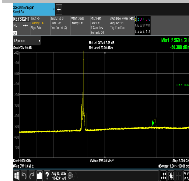
Band66-15MHz-QPSK-132322-1RB#74-1000~3000-PASS
