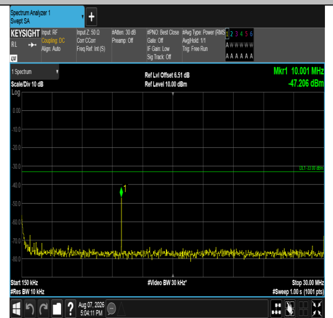
Band66-10MHz-QPSK-132622-1RB#0-0.15~30-PASS
