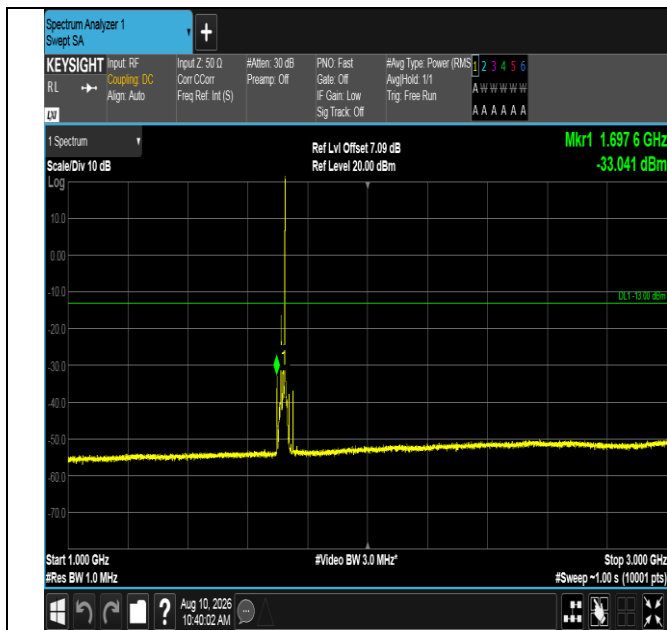
Band66-15MHz-QPSK-132047-1RB#74-1000~3000-PASS
