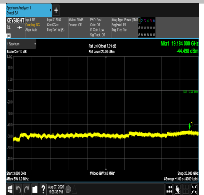
Band66-10MHz-QPSK-132622-1RB#49-3000~20000-PASS
