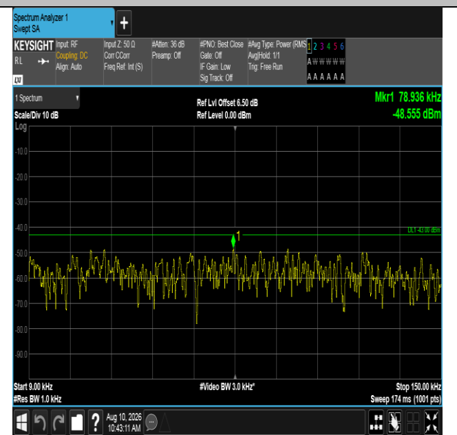
Band66-15MHz-QPSK-132322-1RB#74-0.009~0.15-PASS
