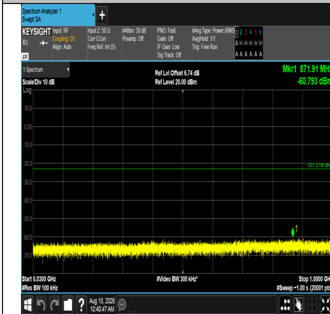
Band66-15MHz-16QAM-132047-1RB#74-30~1000-PASS
