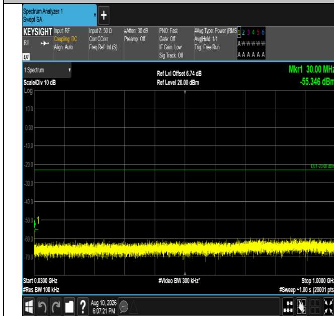
Band66-15MHz-QPSK-132322-75RB#0-30~1000-PASS
