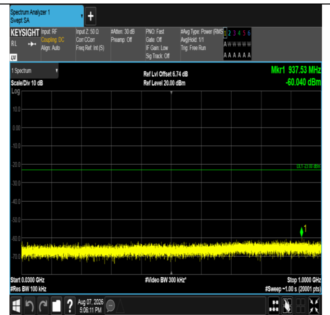
Band66-10MHz-QPSK-132622-1RB#49-30~1000-PASS
