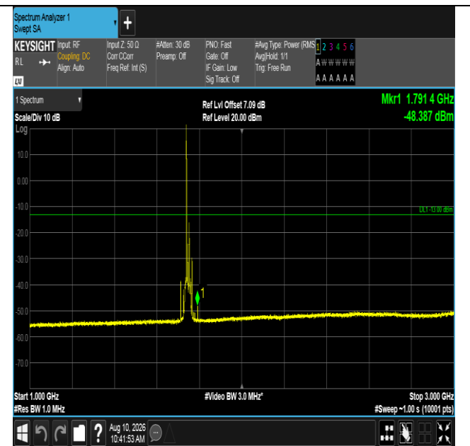
Band66-15MHz-QPSK-132322-1RB#0-1000~3000-PASS
