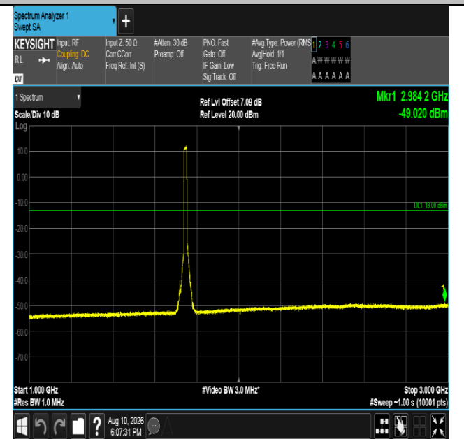
Band66-15MHz-QPSK-132322-75RB#0-1000~3000-PASS
