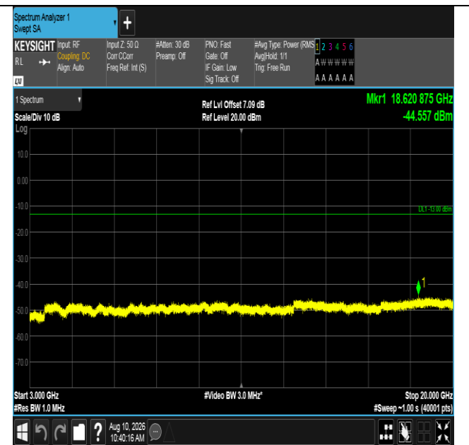
Band66-15MHz-QPSK-132047-1RB#74-3000~20000-PASS
