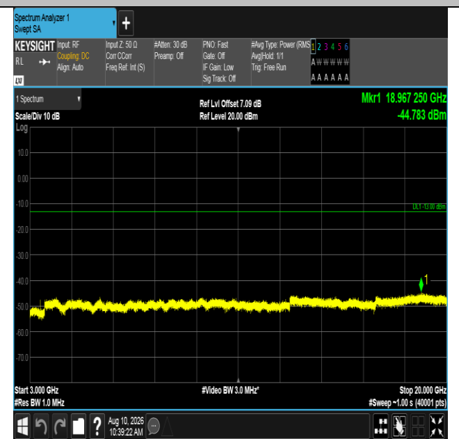
Band66-15MHz-16QAM-132047-1RB#0-3000~20000-PASS
