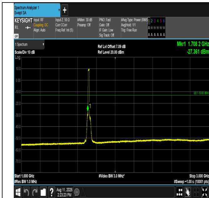
Band66-15MHz-16QAM-132047-75RB#0-1000~3000-PASS
