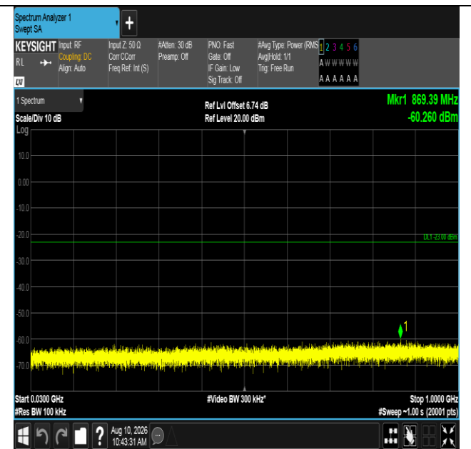
Band66-15MHz-QPSK-132322-1RB#74-30~1000-PASS
