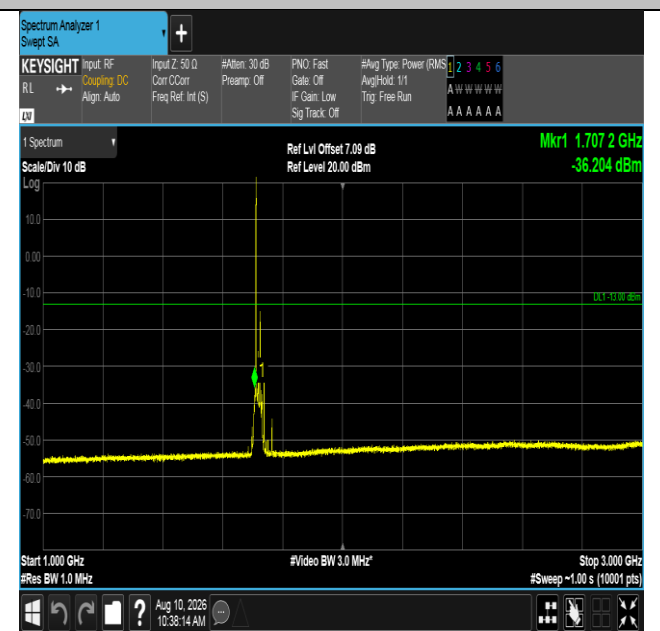
Band66-15MHz-QPSK-132047-1RB#0-1000~3000-PASS
