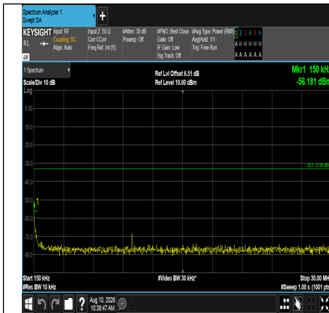
Band66-15MHz-16QAM-132047-1RB#0-0.15~30-PASS
