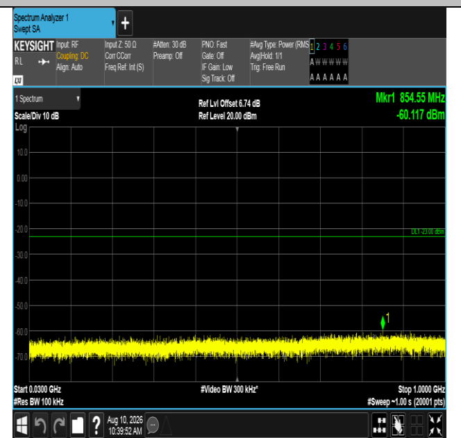
Band66-15MHz-QPSK-132047-1RB#74-30~1000-PASS
