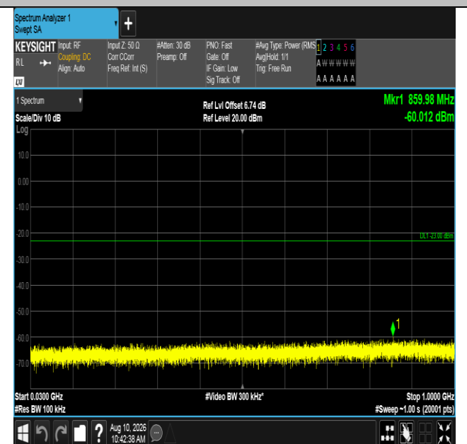
Band66-15MHz-16QAM-132322-1RB#0-30~1000-PASS
