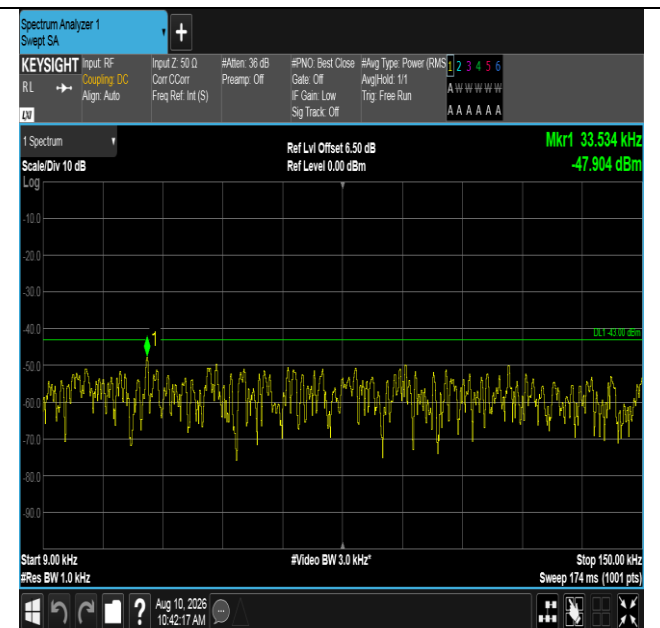
Band66-15MHz-16QAM-132322-1RB#0-0.009~0.15-PASS
