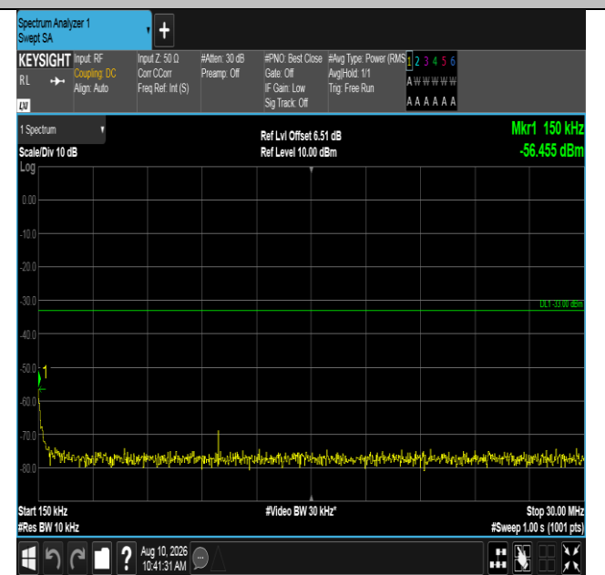
Band66-15MHz-QPSK-132322-1RB#0-0.15~30-PASS
