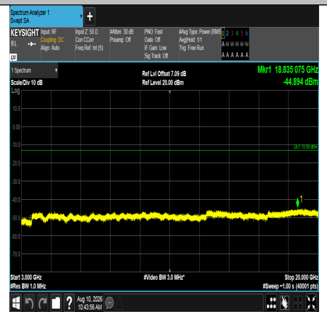
Band66-15MHz-QPSK-132322-1RB#74-3000~20000-PASS
