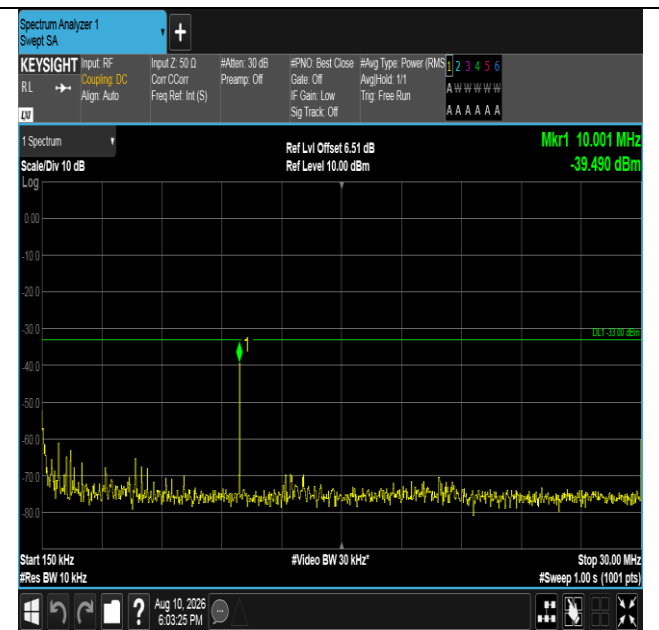
Band66-10MHz-QPSK-132622-50RB#0-0.15~30-PASS
