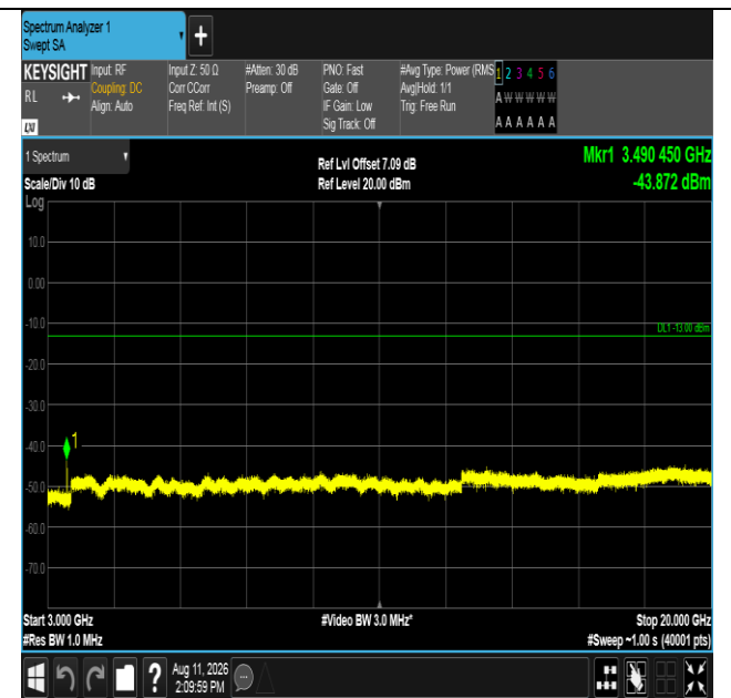
Band66-10MHz-16QAM-132322-50RB#0-3000~20000-PASS
