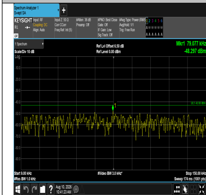
Band66-15MHz-QPSK-132322-1RB#0-0.009~0.15-PASS
