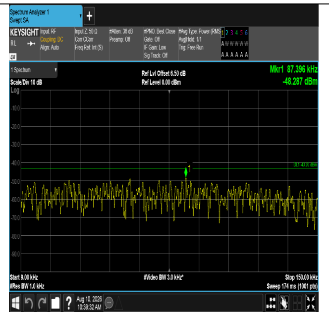
Band66-15MHz-QPSK-132047-1RB#74-0.009~0.15-PASS
