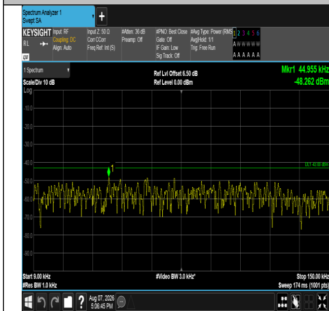
Band66-10MHz-16QAM-132622-1RB#49-0.009~0.15-PASS
