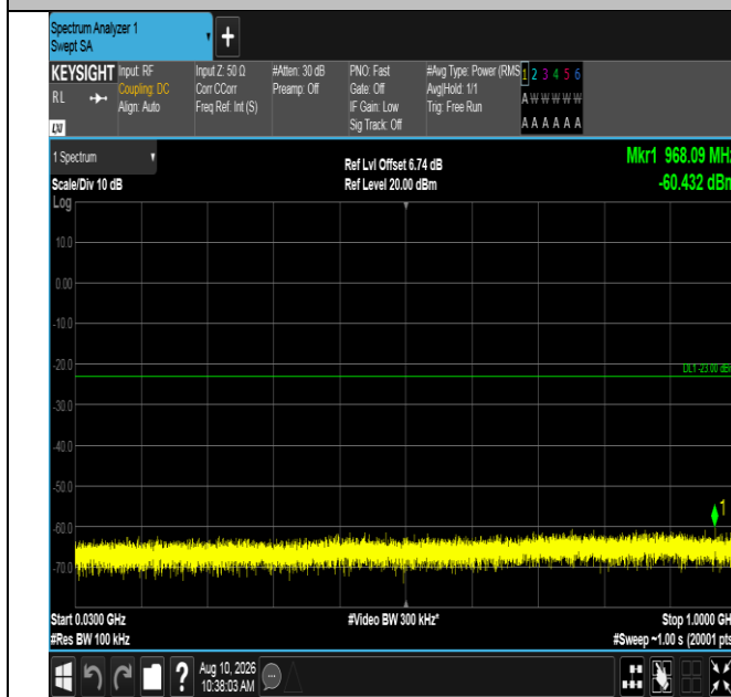
Band66-15MHz-QPSK-132047-1RB#0-30~1000-PASS
