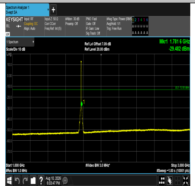
Band66-10MHz-QPSK-132622-50RB#0-1000~3000-PASS
