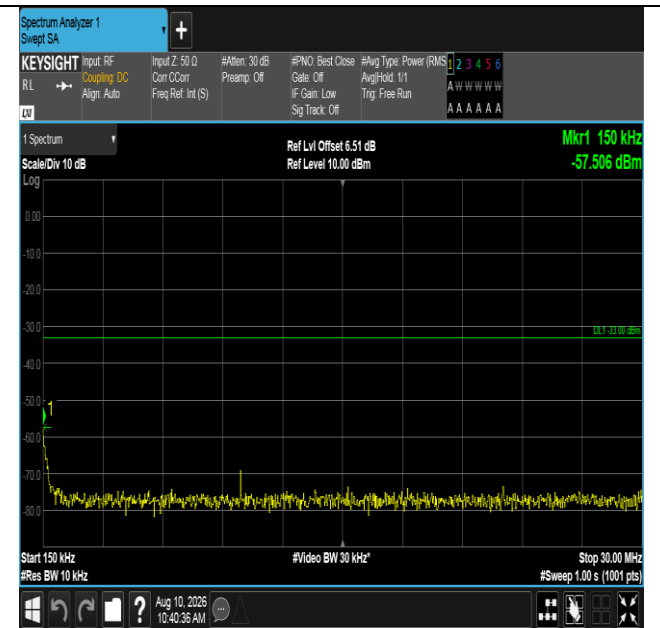
Band66-15MHz-16QAM-132047-1RB#74-0.15~30-PASS
