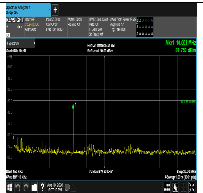
Band66-15MHz-QPSK-132322-75RB#0-0.15~30-PASS
