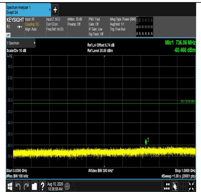
Band66-15MHz-16QAM-132047-1RB#0-30~1000-PASS
