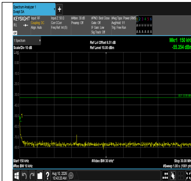
Band66-15MHz-QPSK-132322-1RB#74-0.15~30-PASS
