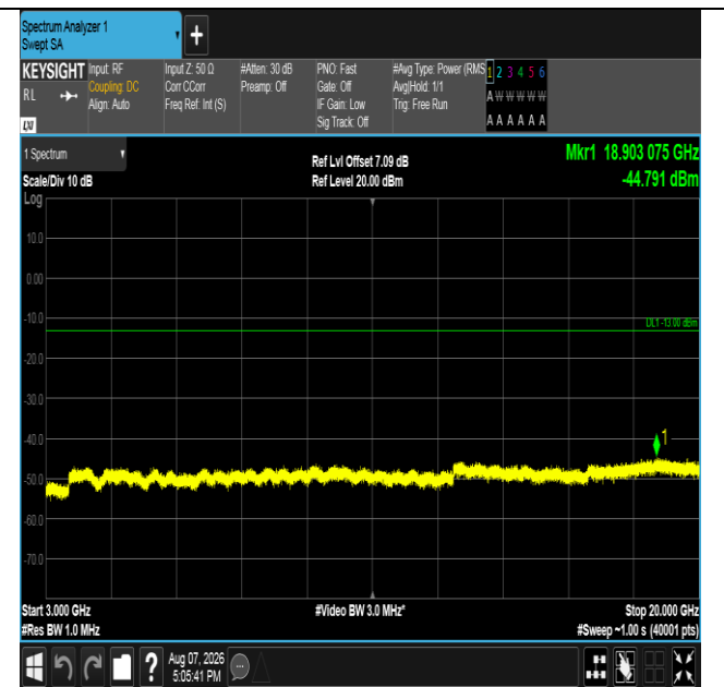
Band66-10MHz-16QAM-132622-1RB#0-3000~20000-PASS
