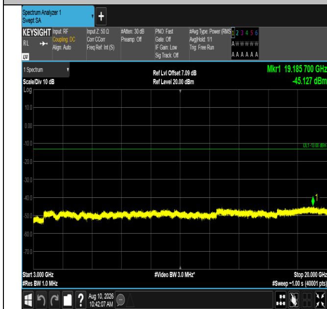
Band66-15MHz-QPSK-132322-1RB#0-3000~20000-PASS
