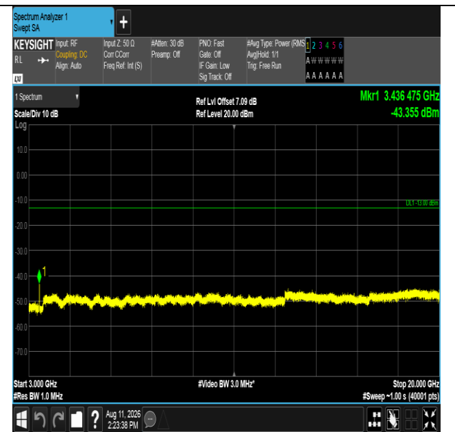
Band66-15MHz-16QAM-132047-75RB#0-3000~20000-PASS
