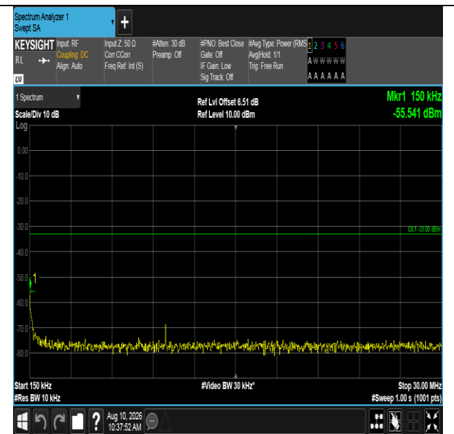
Band66-15MHz-QPSK-132047-1RB#0-0.15~30-PASS
