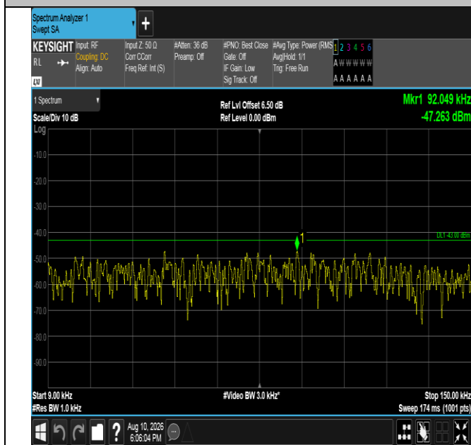
Band66-15MHz-QPSK-132047-75RB#0-0.009~0.15-PASS
