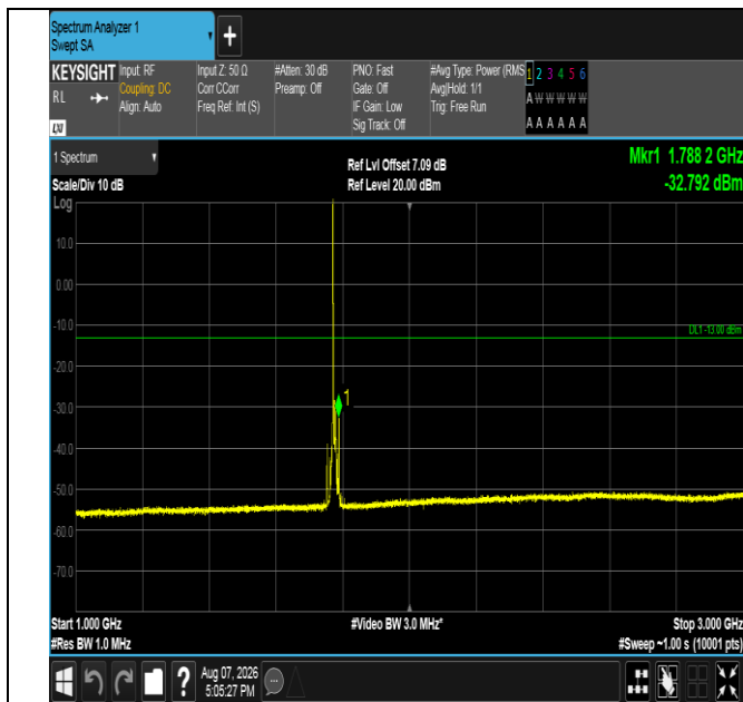
Band66-10MHz-16QAM-132622-1RB#0-1000~3000-PASS
