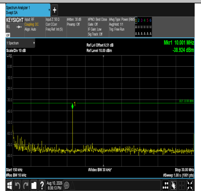
Band66-15MHz-QPSK-132047-75RB#0-0.15~30-PASS
