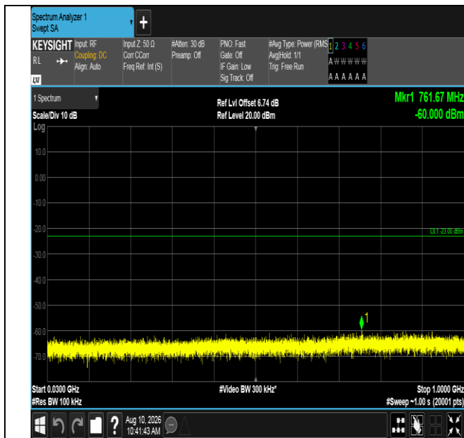
Band66-15MHz-QPSK-132322-1RB#0-30~1000-PASS
