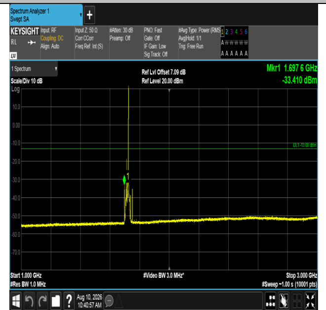
Band66-15MHz-16QAM-132047-1RB#74-1000~3000-PASS
