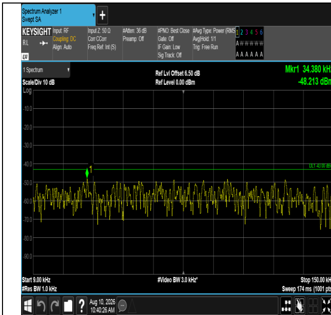
Band66-15MHz-16QAM-132047-1RB#74-0.009~0.15-PASS
