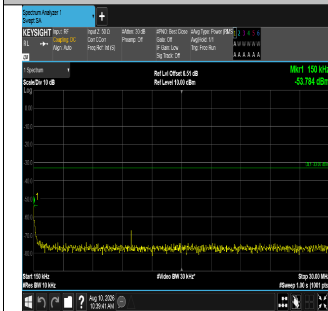
Band66-15MHz-QPSK-132047-1RB#74-0.15~30-PASS
