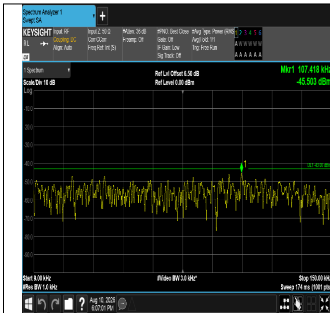
Band66-15MHz-QPSK-132322-75RB#0-0.009~0.15-PASS
