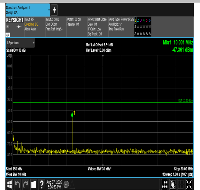
Band66-10MHz-16QAM-132622-1RB#49-0.15~30-PASS
