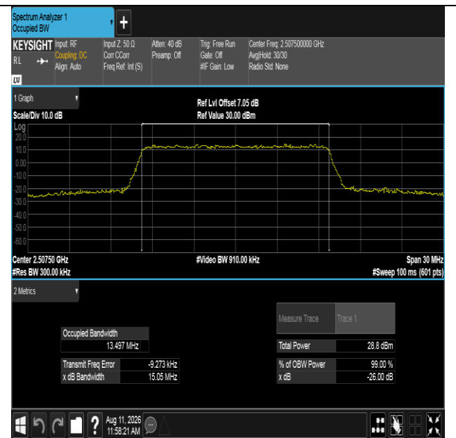
Band7-15MHz-16QAM-20825-75RB#0-PASS
