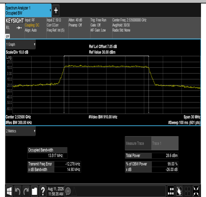
Band7-15MHz-16QAM-21100-75RB#0-PASS
