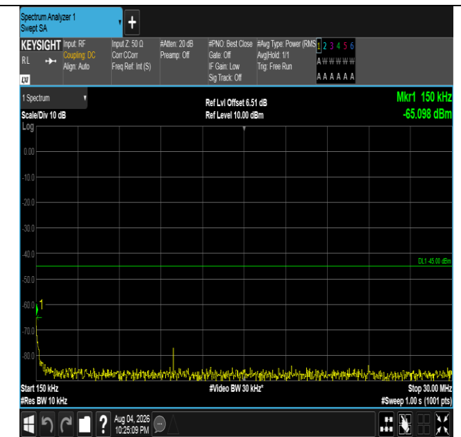
Band7-5MHz-QPSK-20775-1RB#24-0.15~30-PASS
