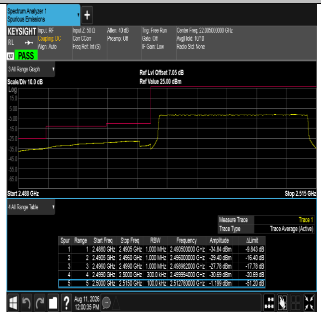
Band7-15MHz-16QAM-20825-75RB#0-PASS
