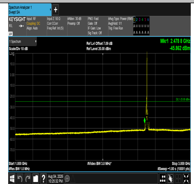
Band7-5MHz-QPSK-20775-1RB#24-1000~3000-PASS
