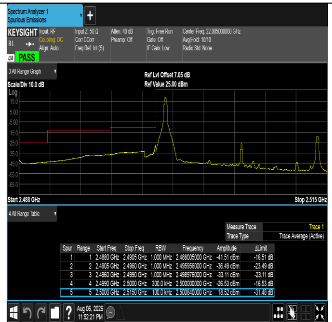
Band7-15MHz-16QAM-20825-1RB#0-PASS
