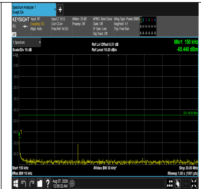
Band7-15MHz-QPSK-21100-1RB#74-0.15~30-PASS
