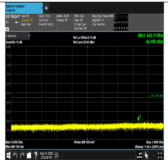
Band7-15MHz-QPSK-21100-75RB#0-30~1000-PASS
