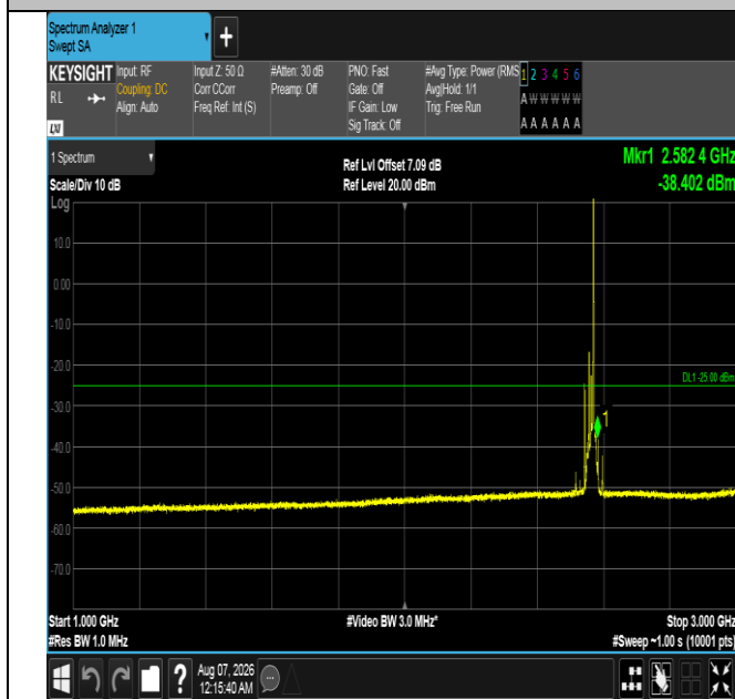
Band7-15MHz-16QAM-21375-1RB#74-1000~3000-PASS
