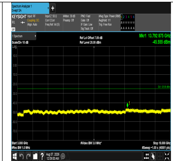
Band7-15MHz-16QAM-21100-1RB#0-3000~18000-PASS
