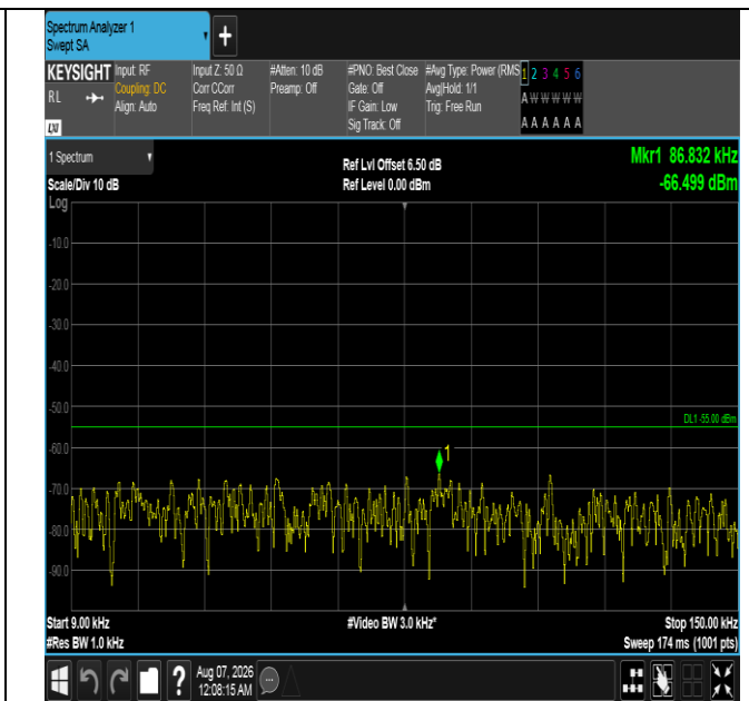
Band7-15MHz-16QAM-21100-1RB#0-0.009~0.15-PASS
