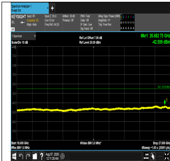
Band7-15MHz-16QAM-21100-1RB#74-18000~27000-PASS
