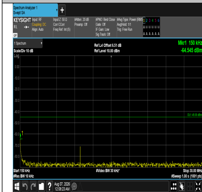
Band7-15MHz-16QAM-21100-1RB#0-0.15~30-PASS
