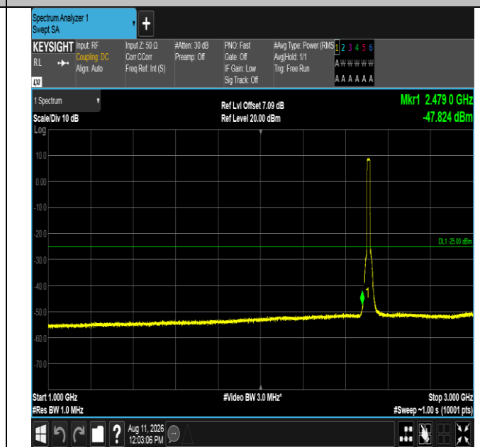
Band7-15MHz-16QAM-20825-75RB#0-1000~3000-PASS
