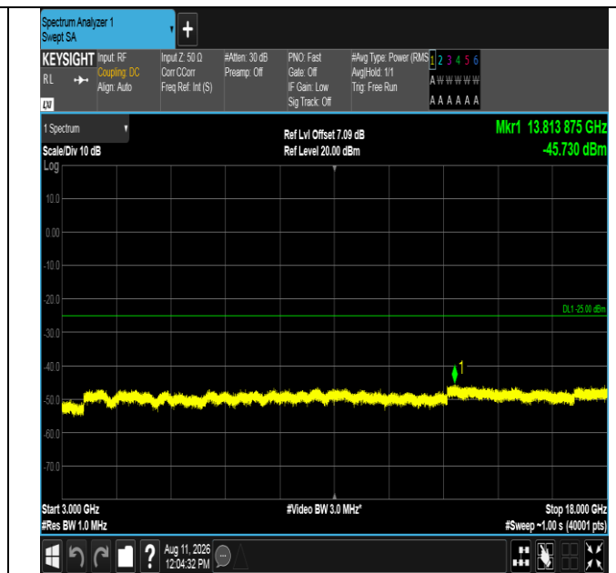
Band7-15MHz-16QAM-21100-75RB#0-3000~18000-PASS
