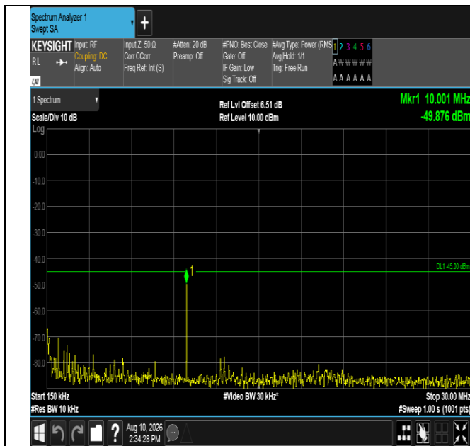
Band7-15MHz-QPSK-21100-75RB#0-0.15~30-PASS
