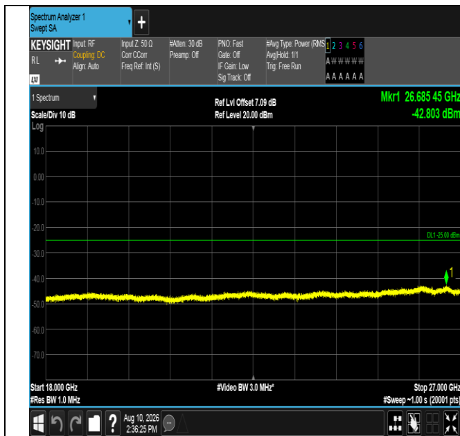
Band7-15MHz-QPSK-21375-75RB#0-18000~27000-PASS
