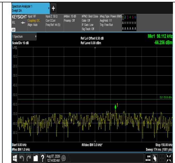
Band7-15MHz-QPSK-21375-1RB#74-0.009~0.15-PASS
