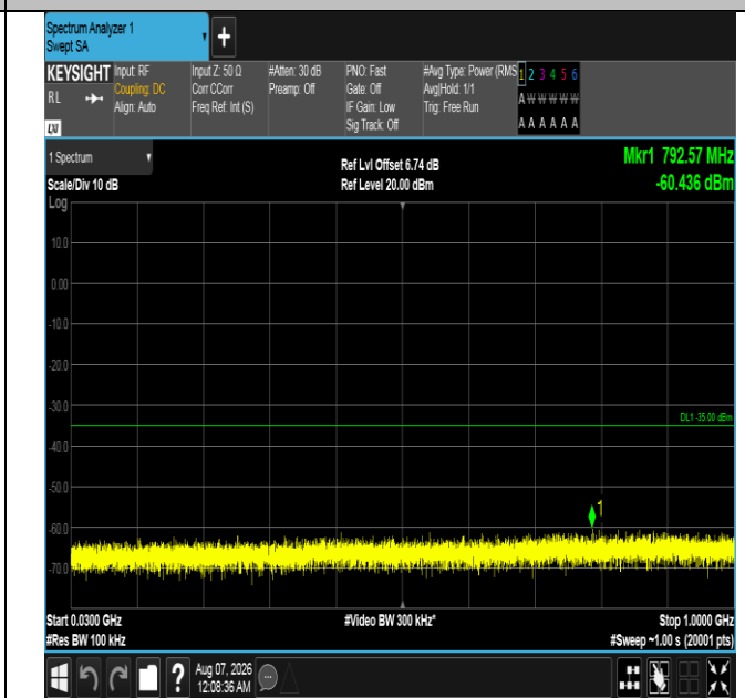
Band7-15MHz-16QAM-21100-1RB#0-30~1000-PASS
