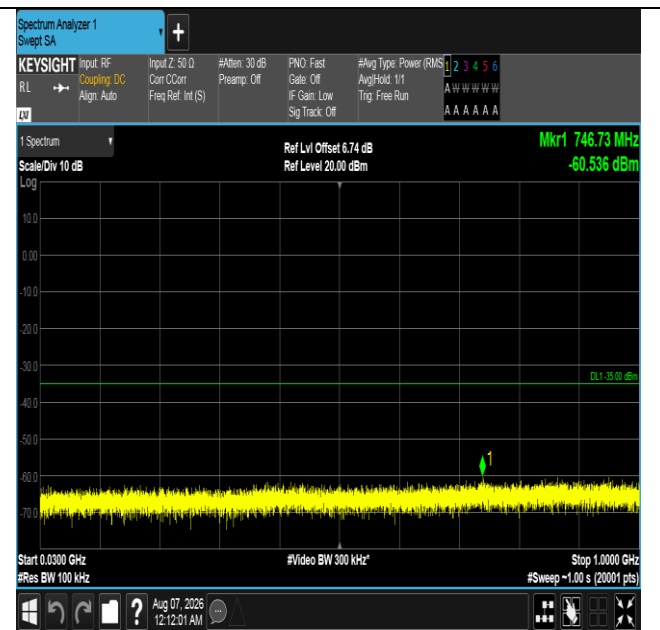
Band7-15MHz-QPSK-21375-1RB#0-30~1000-PASS
