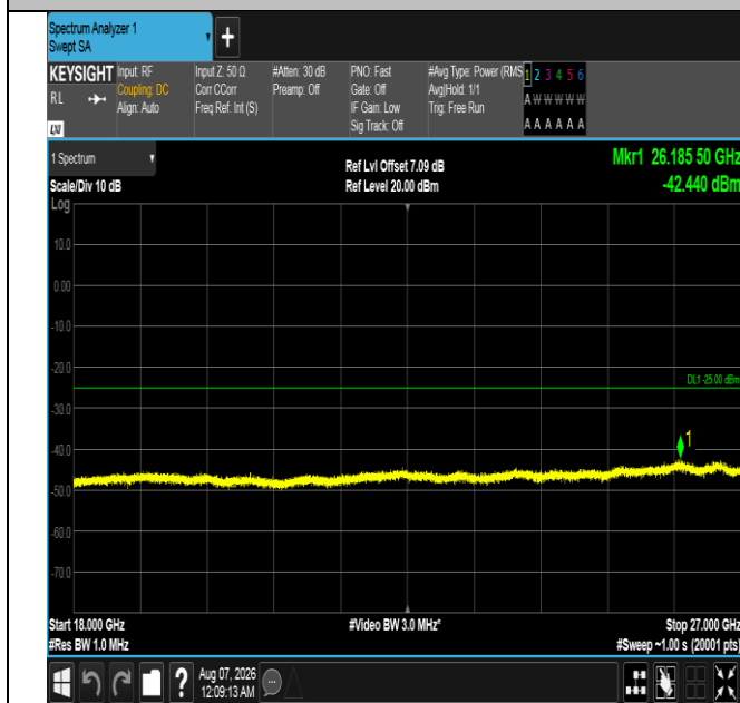
Band7-15MHz-16QAM-21100-1RB#0-18000~27000-PASS
