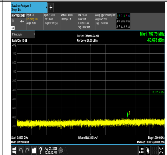
Band7-15MHz-16QAM-21375-1RB#0-30~1000-PASS
