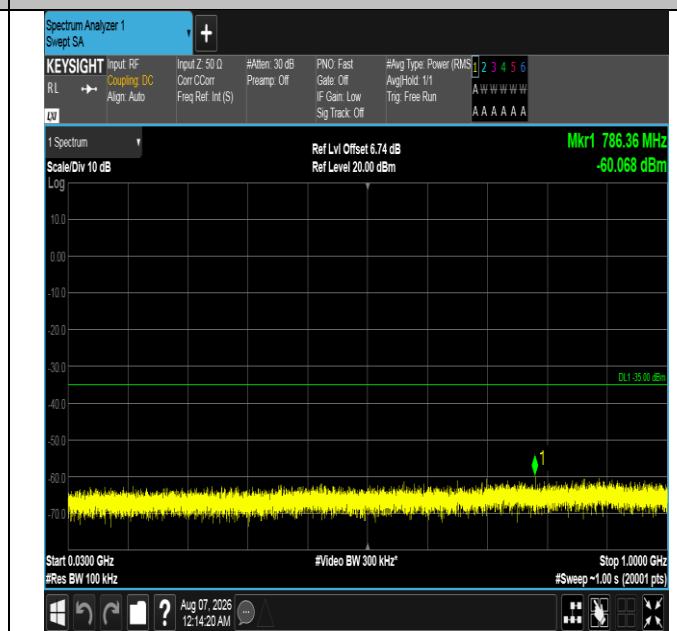
Band7-15MHz-QPSK-21375-1RB#74-30~1000-PASS
