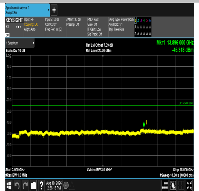
Band7-15MHz-QPSK-21375-75RB#0-3000~18000-PASS
