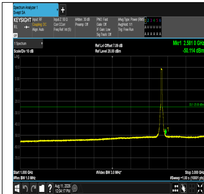
Band7-15MHz-16QAM-21100-75RB#0-1000~3000-PASS
