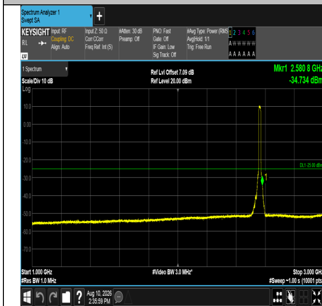
Band7-15MHz-QPSK-21375-75RB#0-1000~3000-PASS
