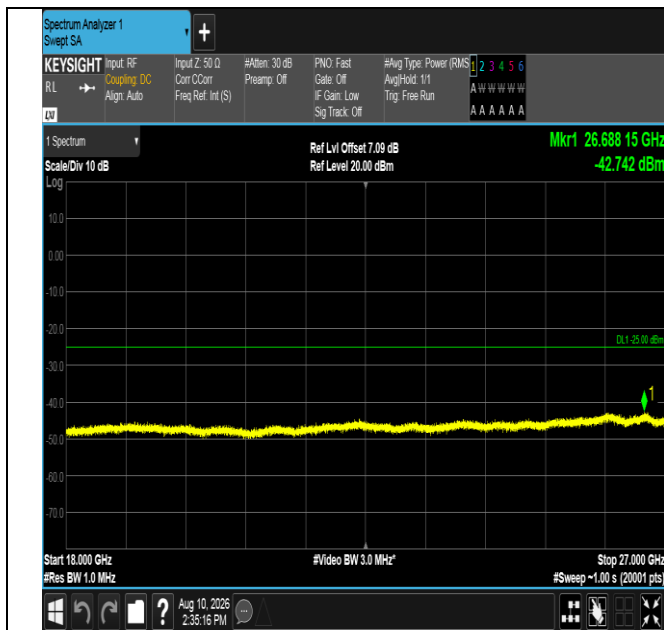
Band7-15MHz-QPSK-21100-75RB#0-18000~27000-PASS
