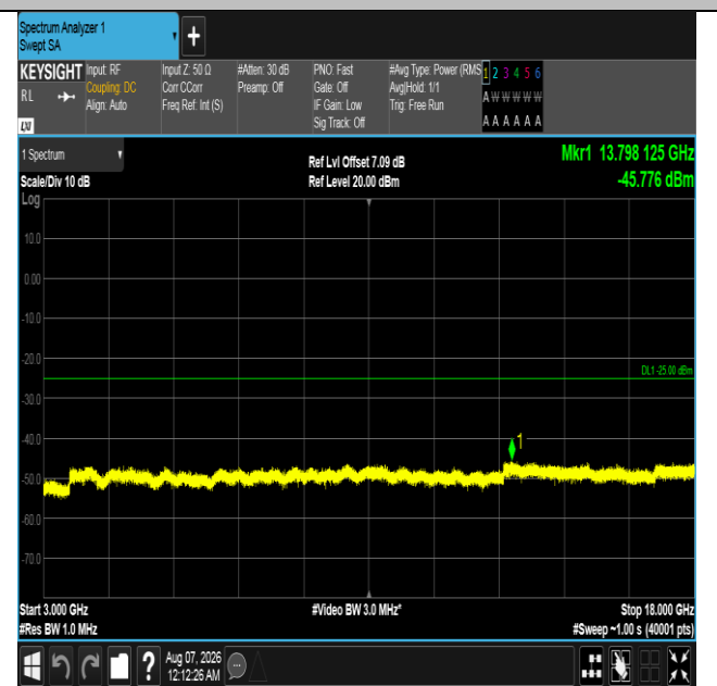
Band7-15MHz-QPSK-21375-1RB#0-3000~18000-PASS
