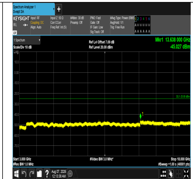
Band7-15MHz-16QAM-21375-1RB#0-3000~18000-PASS
