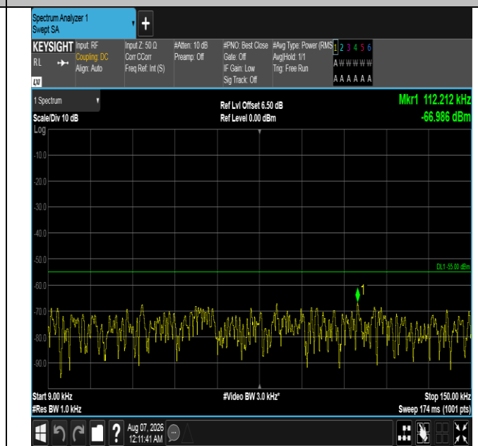
Band7-15MHz-QPSK-21375-1RB#0-0.009~0.15-PASS
