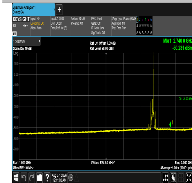
Band7-15MHz-16QAM-21100-1RB#74-1000~3000-PASS
