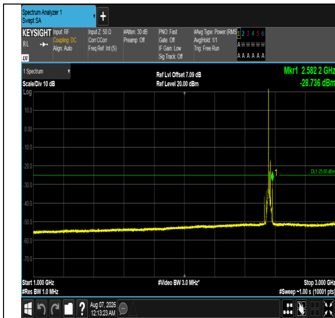
Band7-15MHz-16QAM-21375-1RB#0-1000~3000-PASS
