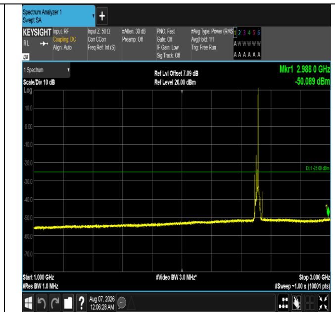
Band7-15MHz-16QAM-20825-1RB#74-1000~3000-PASS
