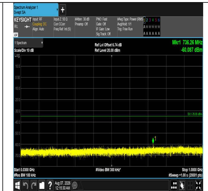
Band7-15MHz-16QAM-21375-1RB#74-30~1000-PASS
