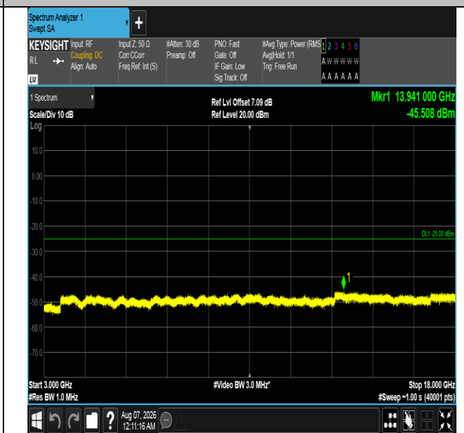
Band7-15MHz-16QAM-21100-1RB#74-3000~18000-PASS
