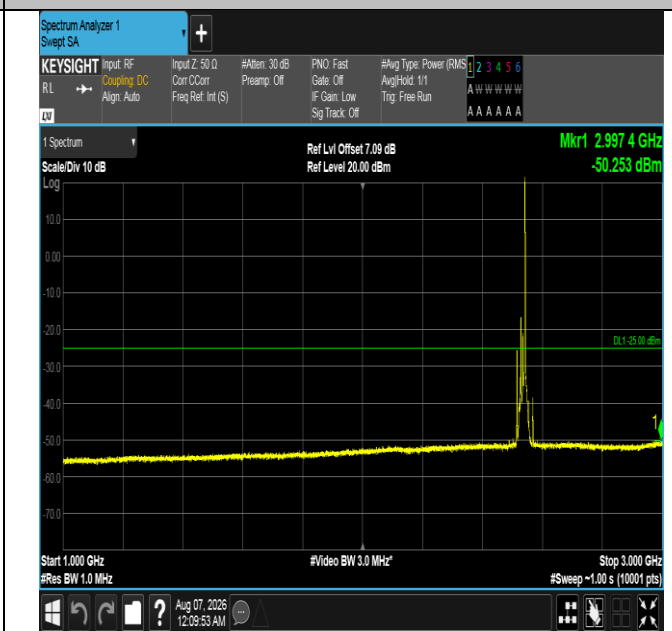
Band7-15MHz-QPSK-21100-1RB#74-1000~3000-PASS
