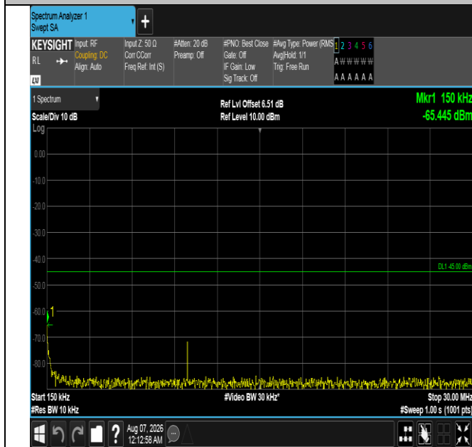
Band7-15MHz-16QAM-21375-1RB#0-0.15~30-PASS
