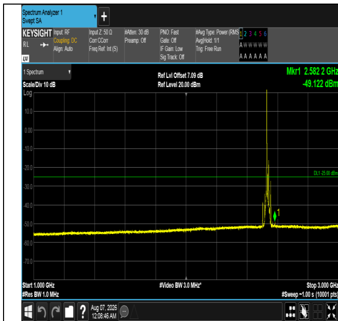
Band7-15MHz-16QAM-21100-1RB#0-1000~3000-PASS
