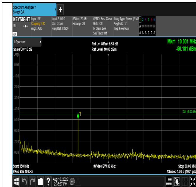
Band7-15MHz-QPSK-21375-75RB#0-0.15~30-PASS
