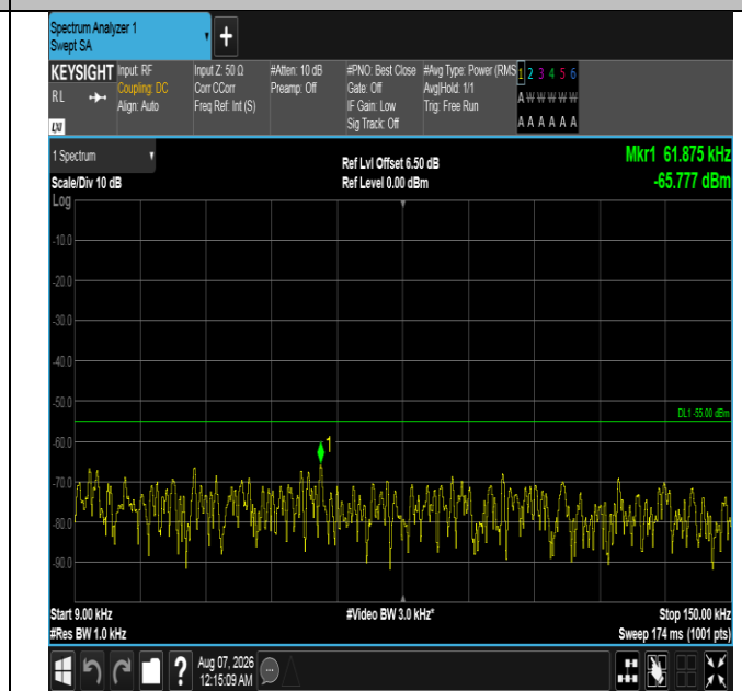
Band7-15MHz-16QAM-21375-1RB#74-0.009~0.15-PASS
