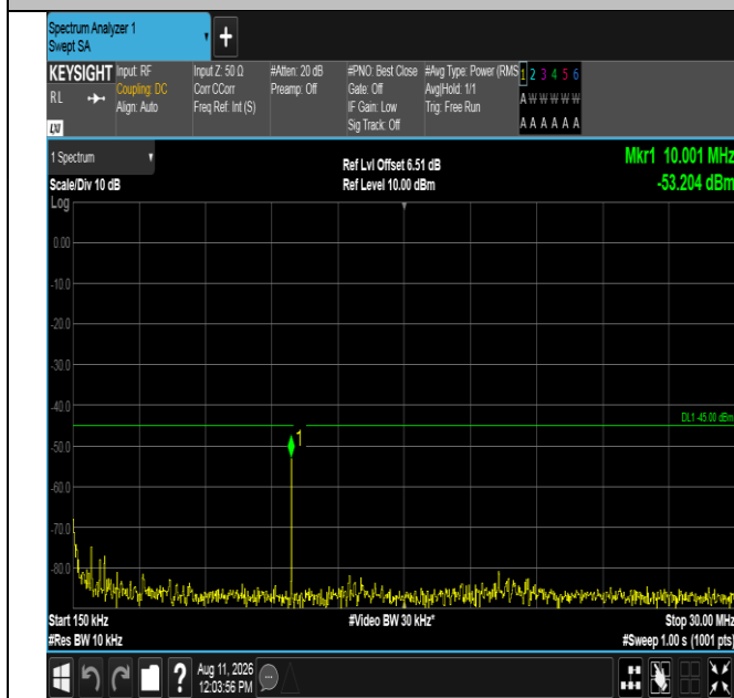
Band7-15MHz-16QAM-21100-75RB#0-0.15~30-PASS
