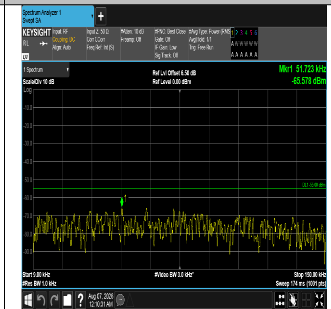
Band7-15MHz-16QAM-21100-1RB#74-0.009~0.15-PASS
