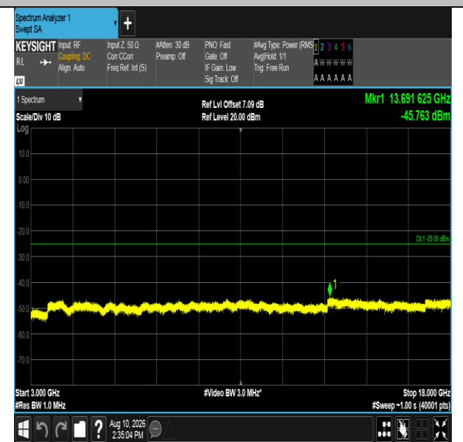
Band7-15MHz-QPSK-21100-75RB#0-3000~18000-PASS
