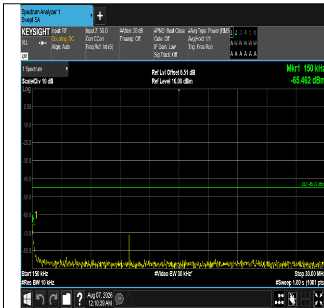
Band7-15MHz-16QAM-21100-1RB#74-0.15~30-PASS
