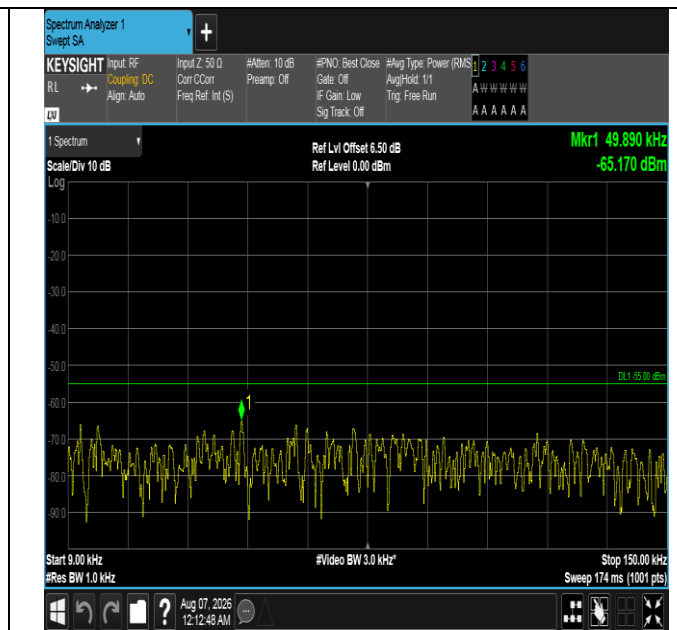
Band7-15MHz-16QAM-21375-1RB#0-0.009~0.15-PASS
