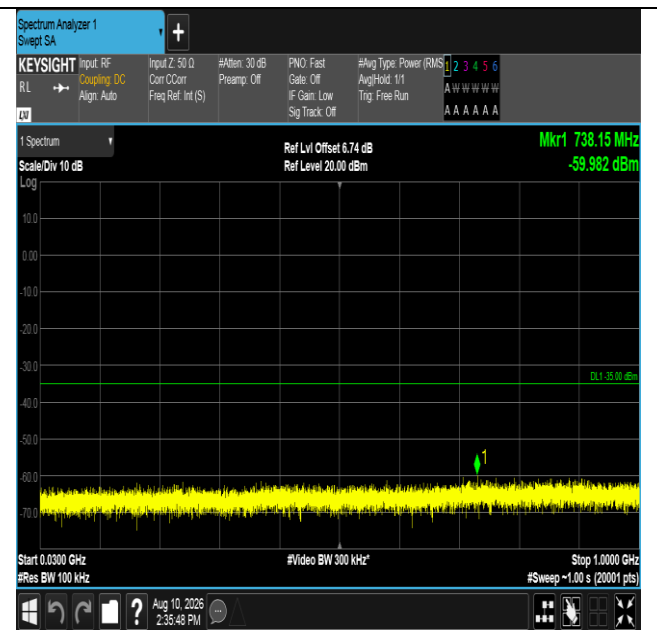
Band7-15MHz-QPSK-21375-75RB#0-30~1000-PASS
