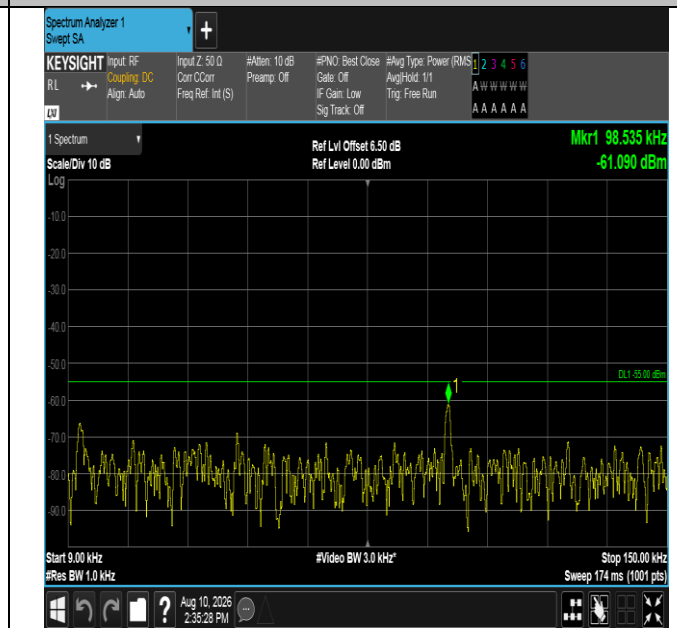
Band7-15MHz-QPSK-21375-75RB#0-0.009~0.15-PASS
