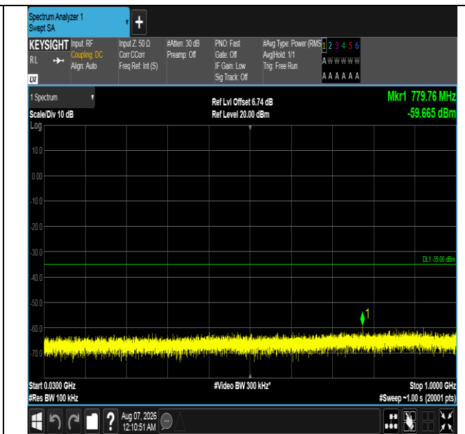
Band7-15MHz-16QAM-21100-1RB#74-30~1000-PASS
