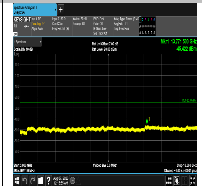
Band7-15MHz-16QAM-21375-1RB#74-3000~18000-PASS
