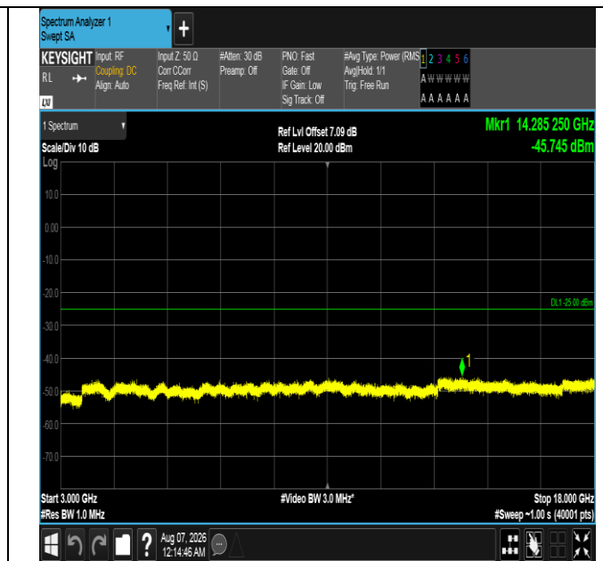
Band7-15MHz-QPSK-21375-1RB#74-3000~18000-PASS
