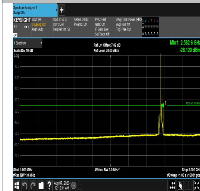
Band7-15MHz-QPSK-21375-1RB#0-1000~3000-PASS
