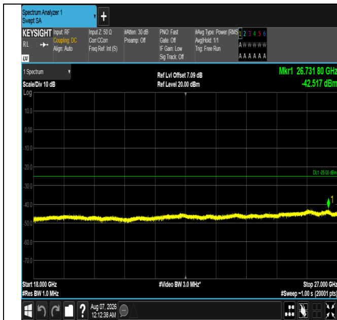
Band7-15MHz-QPSK-21375-1RB#0-18000~27000-PASS
