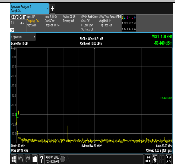
Band7-20MHz-16QAM-21100-1RB#0-0.15~30-PASS
