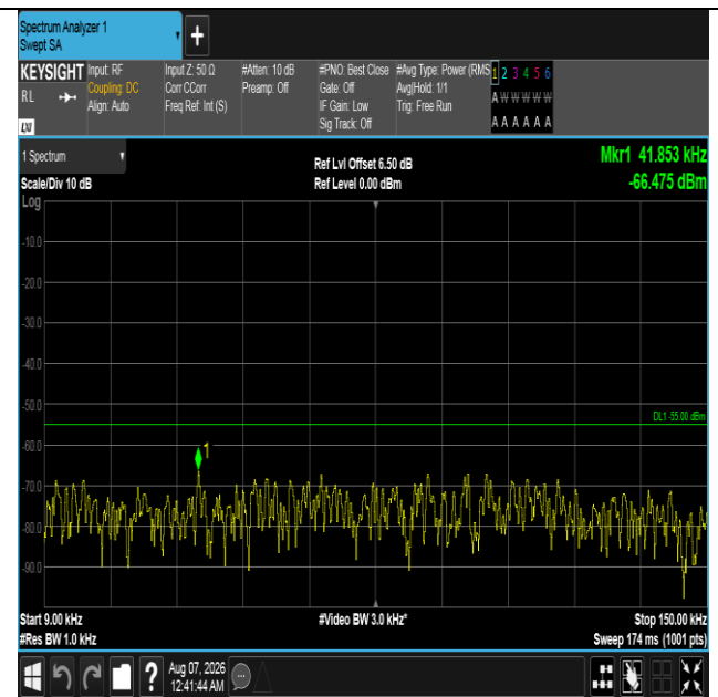
Band7-20MHz-16QAM-20850-1RB#0-0.009~0.15-PASS
