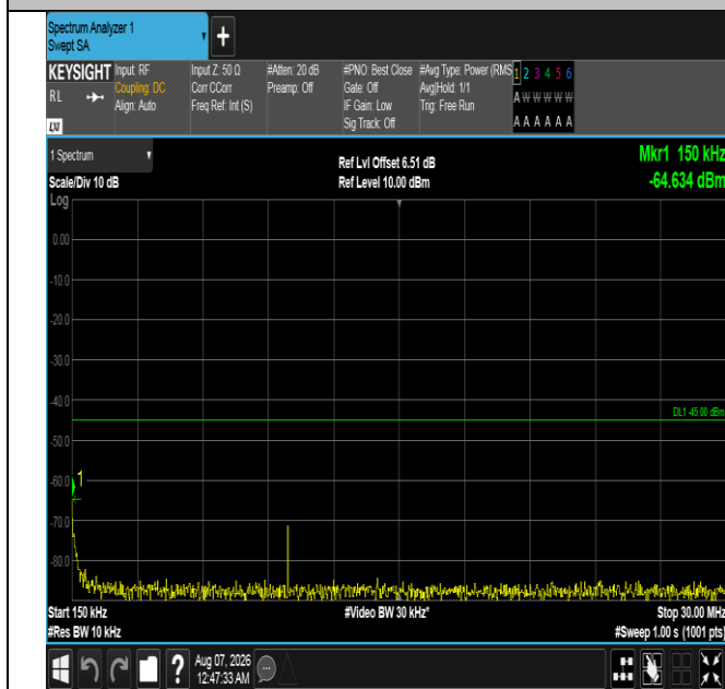
Band7-20MHz-QPSK-21100-1RB#99-0.15~30-PASS
