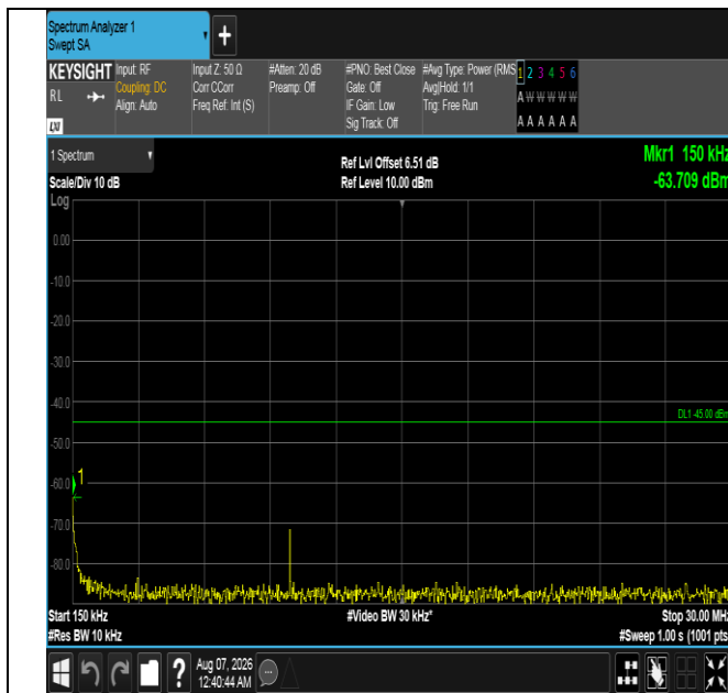
Band7-20MHz-QPSK-20850-1RB#0-0.15~30-PASS
