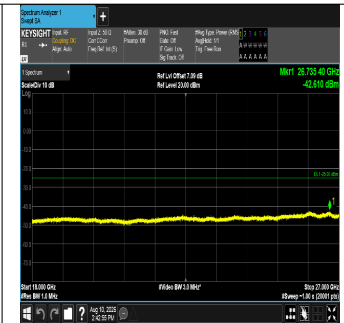
Band7-20MHz-QPSK-21100-100RB#0-18000~27000-PASS
