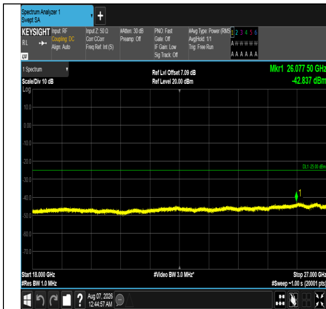
Band7-20MHz-16QAM-20850-1RB#99-18000~27000-PASS
