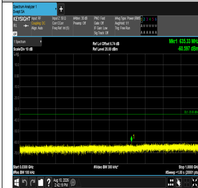
Band7-20MHz-QPSK-21100-100RB#0-30~1000-PASS
