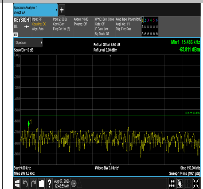
Band7-20MHz-16QAM-20850-1RB#99-0.009~0.15-PASS
