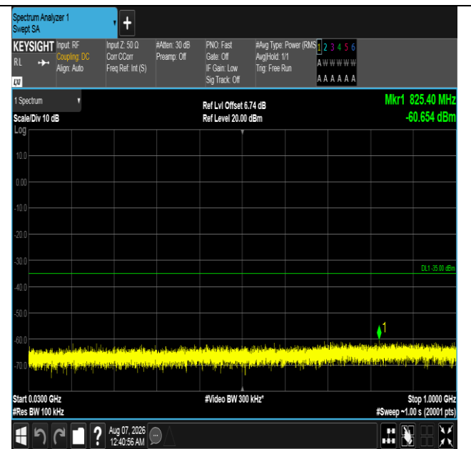
Band7-20MHz-QPSK-20850-1RB#0-30~1000-PASS
