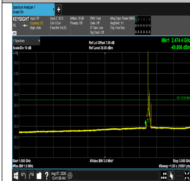
Band7-20MHz-QPSK-20850-1RB#0-1000~3000-PASS
