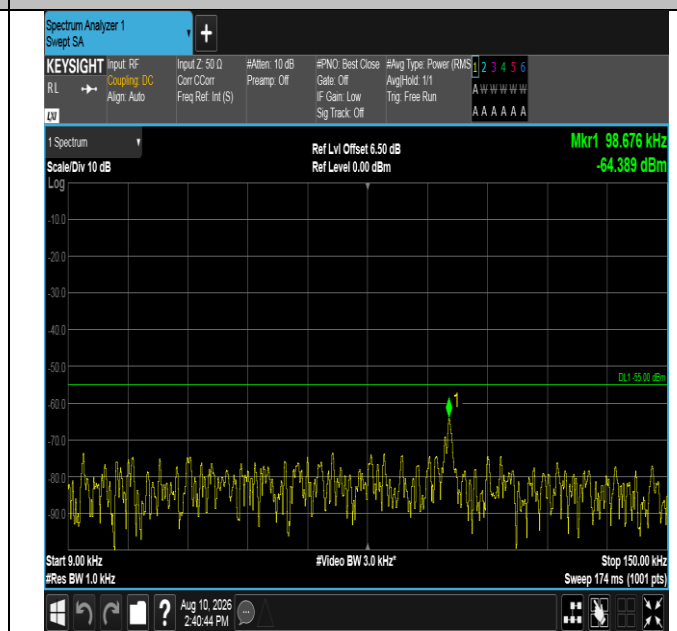
Band7-20MHz-QPSK-20850-100RB#0-0.009~0.15-PASS
