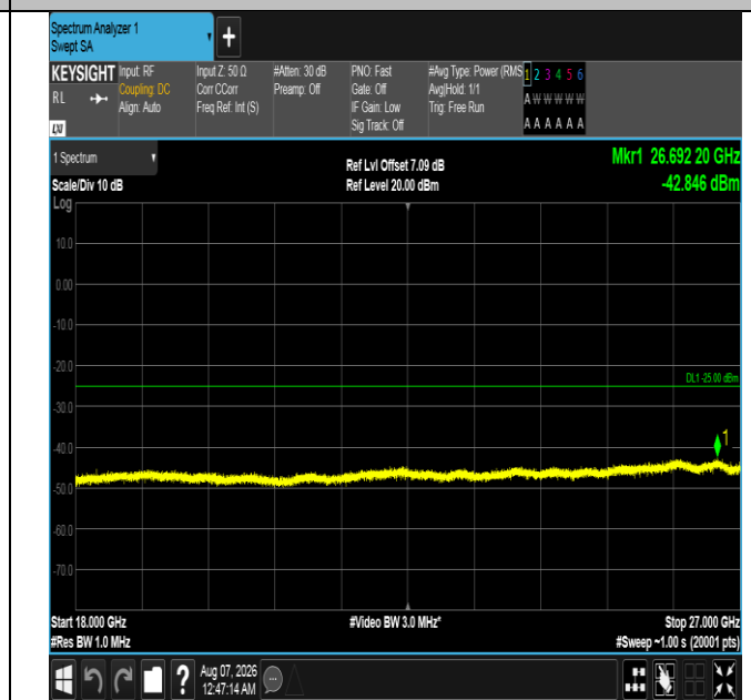
Band7-20MHz-16QAM-21100-1RB#0-18000~27000-PASS
