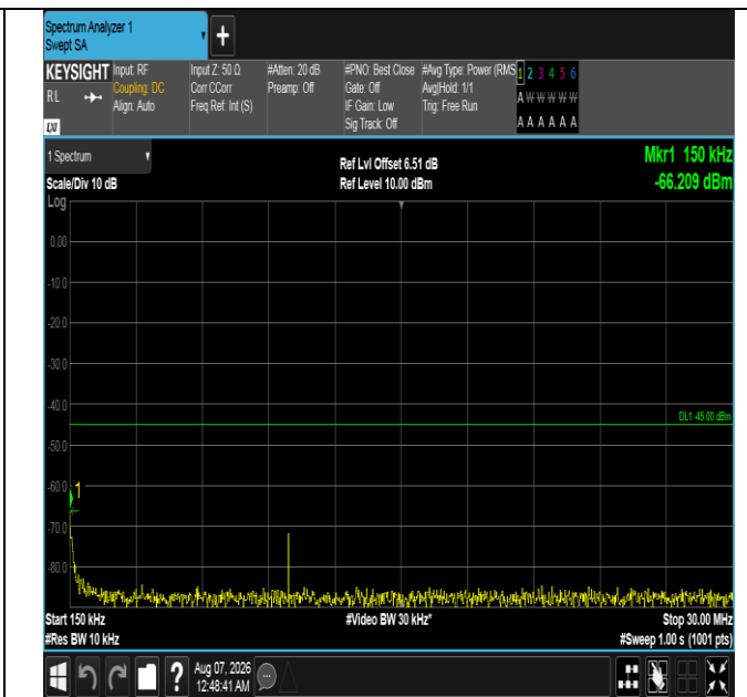
Band7-20MHz-16QAM-21100-1RB#99-0.15~30-PASS
