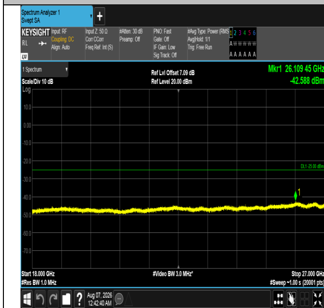
Band7-20MHz-16QAM-20850-1RB#0-18000~27000-PASS
