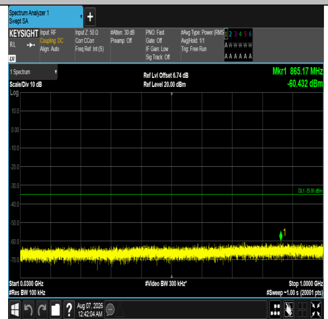
Band7-20MHz-16QAM-20850-1RB#0-30~1000-PASS
