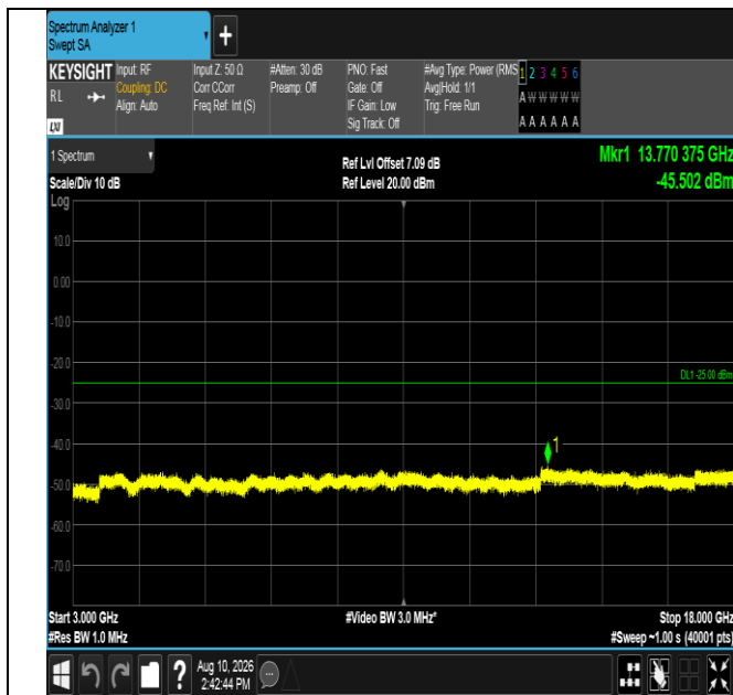
Band7-20MHz-QPSK-21100-100RB#0-3000~18000-PASS
