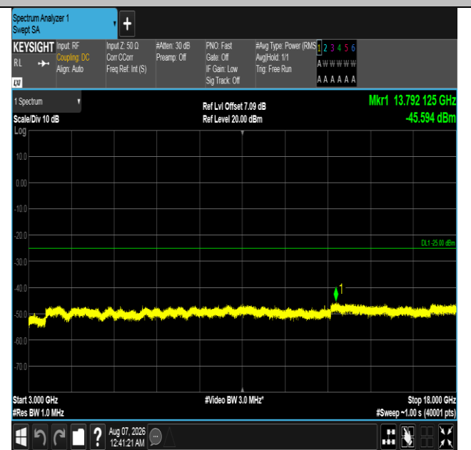
Band7-20MHz-QPSK-20850-1RB#0-3000~18000-PASS
