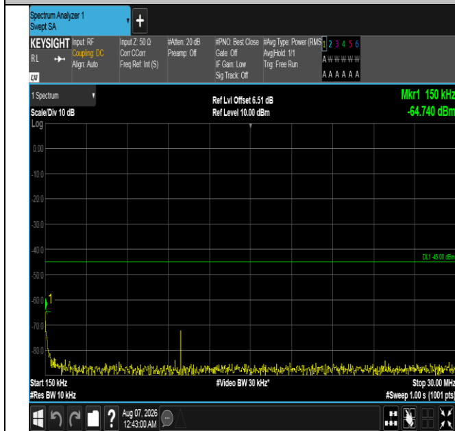
Band7-20MHz-QPSK-20850-1RB#99-0.15~30-PASS
