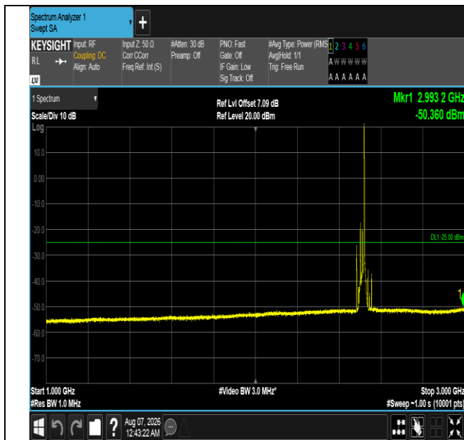
Band7-20MHz-QPSK-20850-1RB#99-1000~3000-PASS
