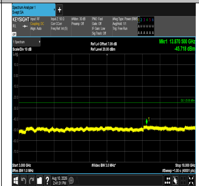
Band7-20MHz-QPSK-20850-100RB#0-3000~18000-PASS
