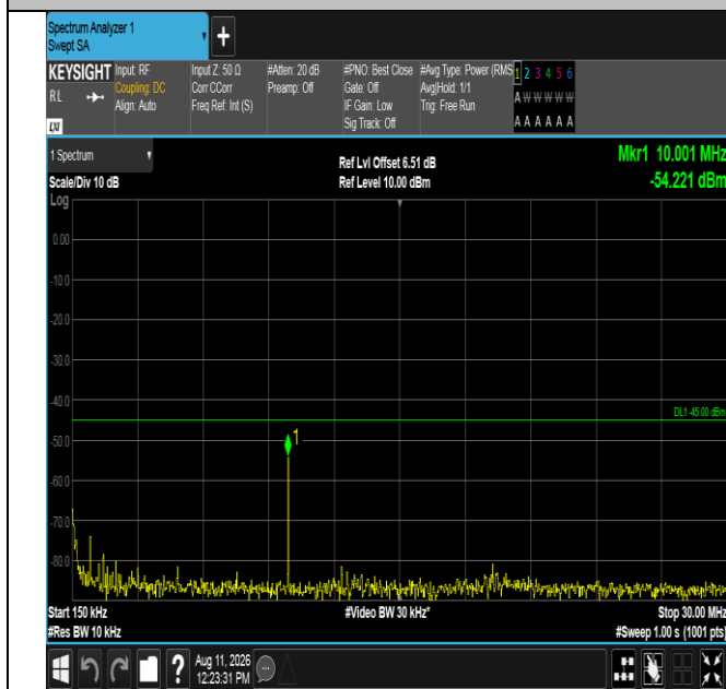
Band7-20MHz-16QAM-20850-100RB#0-0.15~30-PASS
