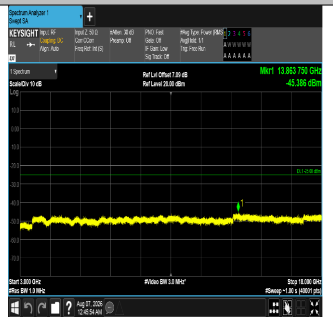
Band7-20MHz-QPSK-21100-1RB#0-3000~18000-PASS
