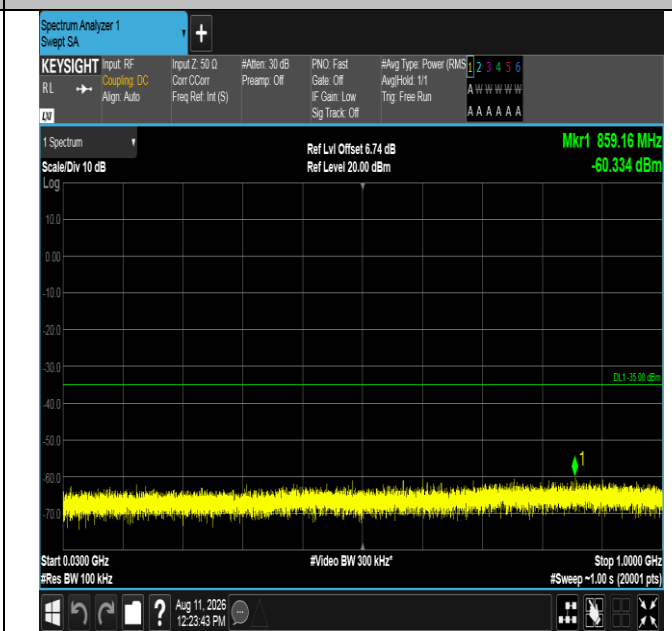
Band7-20MHz-16QAM-20850-100RB#0-30~1000-PASS
