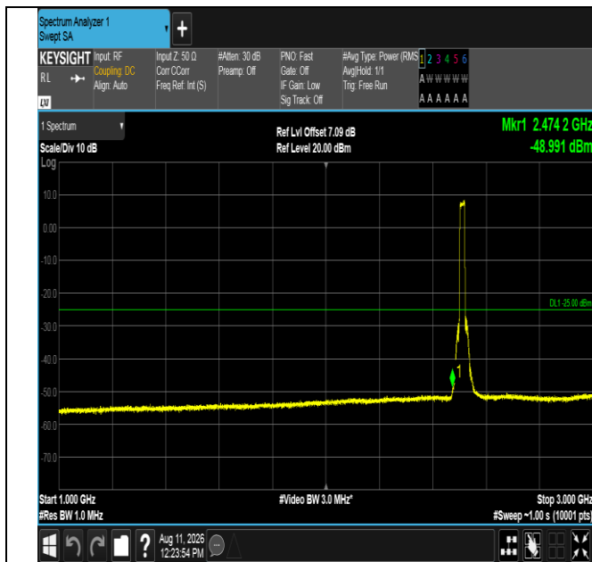
Band7-20MHz-16QAM-20850-100RB#0-1000~3000-PASS
