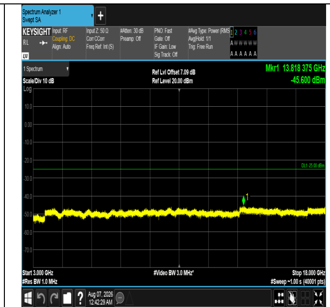
Band7-20MHz-16QAM-20850-1RB#0-3000~18000-PASS
