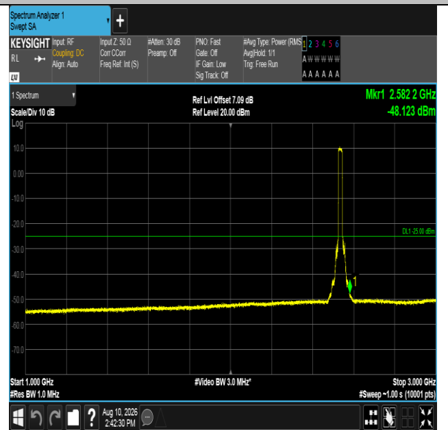
Band7-20MHz-QPSK-21100-100RB#0-1000~3000-PASS
