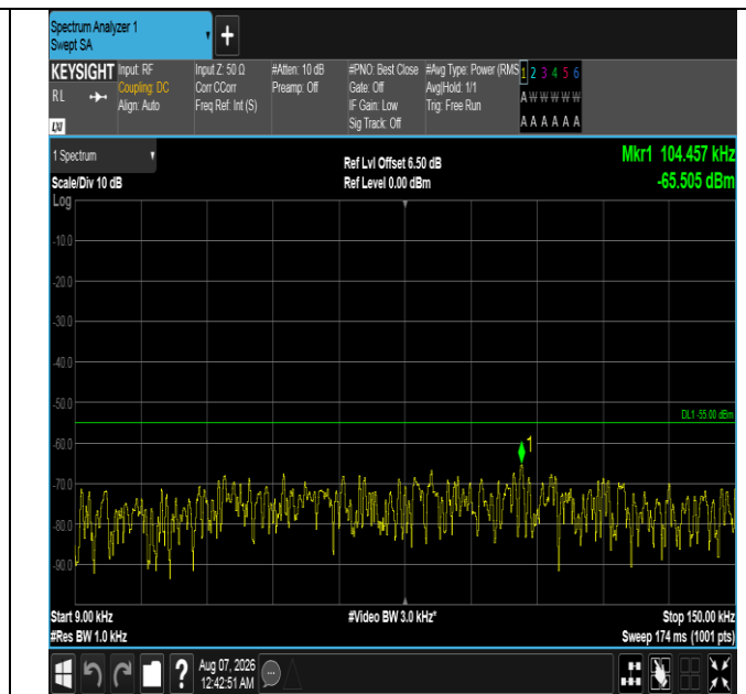
Band7-20MHz-QPSK-20850-1RB#99-0.009~0.15-PASS
