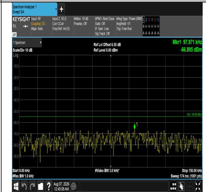
Band7-20MHz-QPSK-21100-1RB#0-0.009~0.15-PASS
