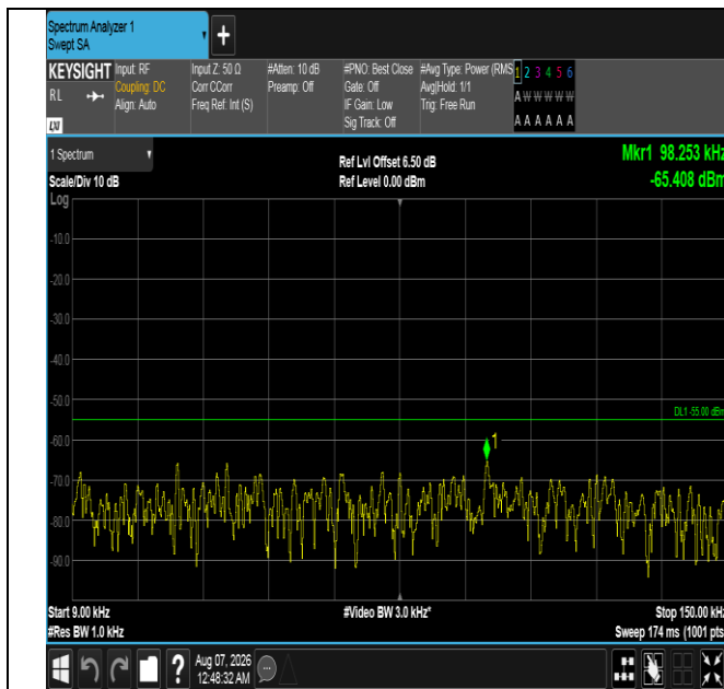
Band7-20MHz-16QAM-21100-1RB#99-0.009~0.15-PASS
