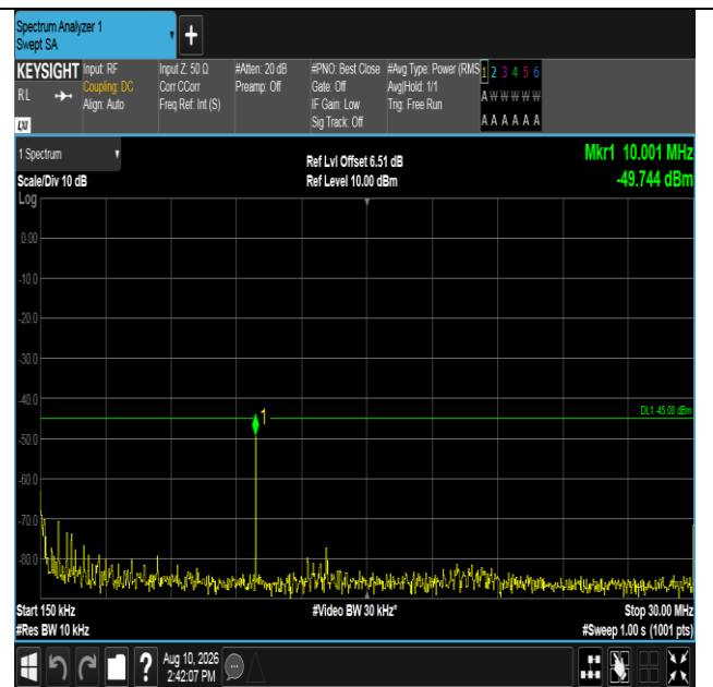
Band7-20MHz-QPSK-21100-100RB#0-0.15~30-PASS
