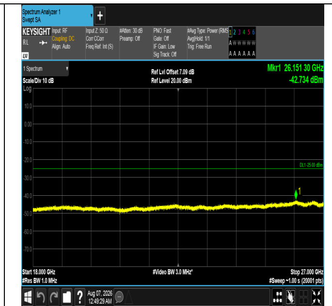
Band7-20MHz-16QAM-21100-1RB#99-18000~27000-PASS
