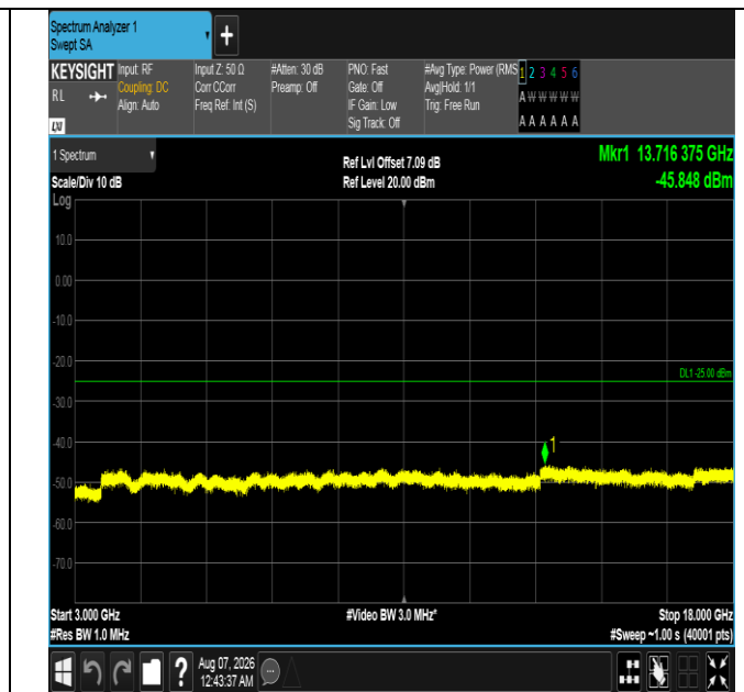
Band7-20MHz-QPSK-20850-1RB#99-3000~18000-PASS
