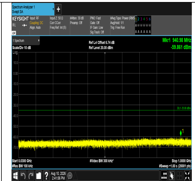
Band7-20MHz-QPSK-20850-100RB#0-30~1000-PASS
