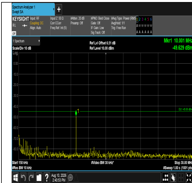
Band7-20MHz-QPSK-20850-100RB#0-0.15~30-PASS
