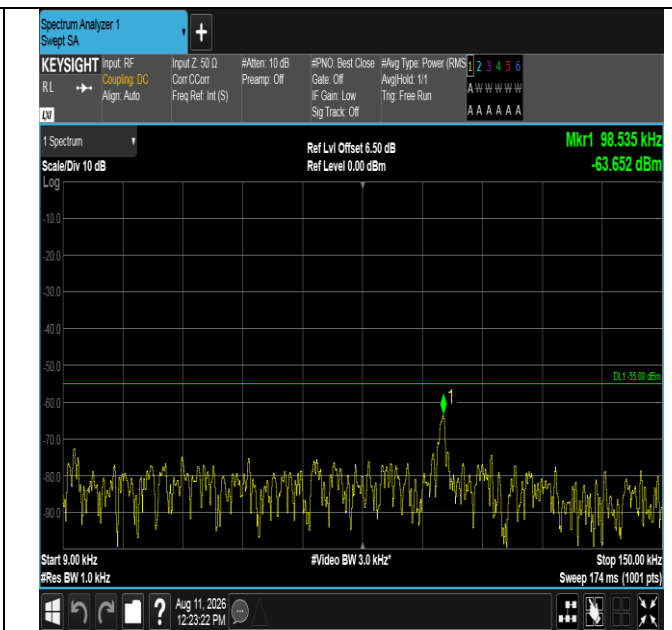
Band7-20MHz-16QAM-20850-100RB#0-0.009~0.15-PASS
