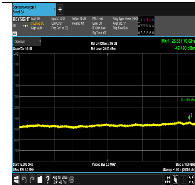
Band7-20MHz-QPSK-20850-100RB#0-18000~27000-PASS
