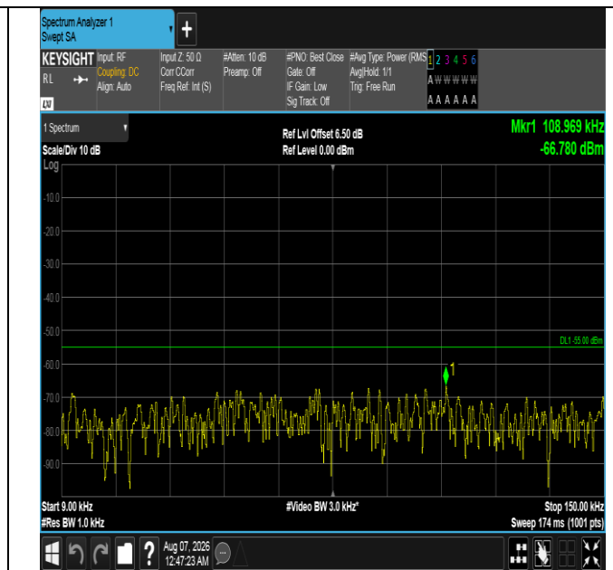
Band7-20MHz-QPSK-21100-1RB#99-0.009~0.15-PASS
