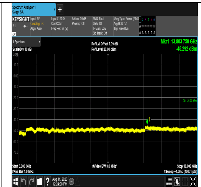
Band7-20MHz-16QAM-20850-100RB#0-3000~18000-PASS
