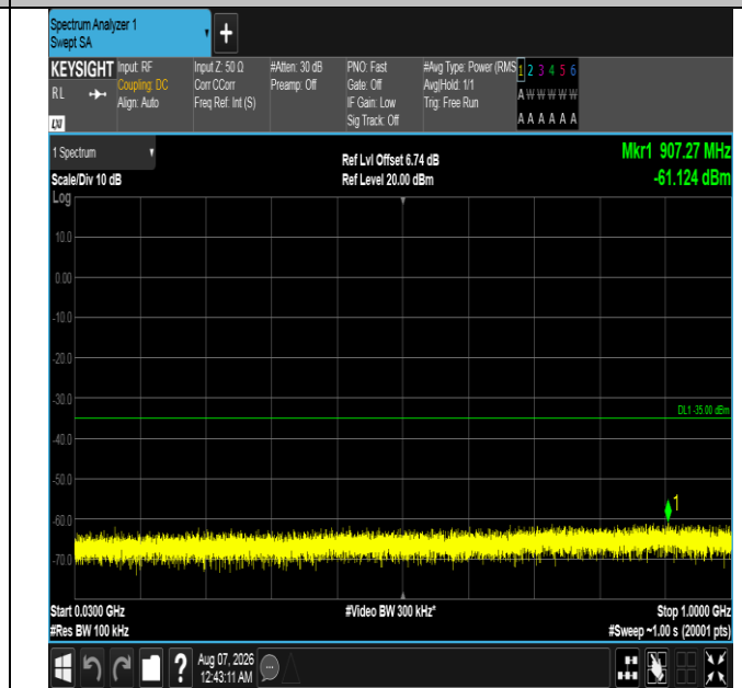
Band7-20MHz-QPSK-20850-1RB#99-30~1000-PASS
