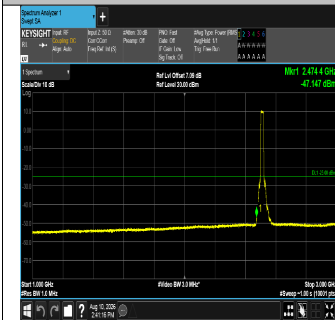
Band7-20MHz-QPSK-20850-100RB#0-1000~3000-PASS
