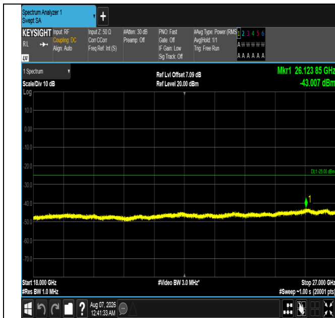
Band7-20MHz-QPSK-20850-1RB#0-18000~27000-PASS
