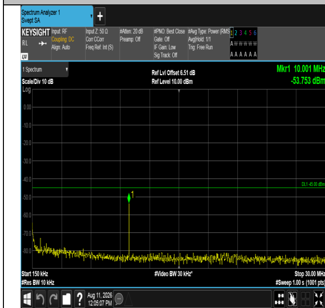
Band7-15MHz-16QAM-21375-75RB#0-0.15~30-PASS
