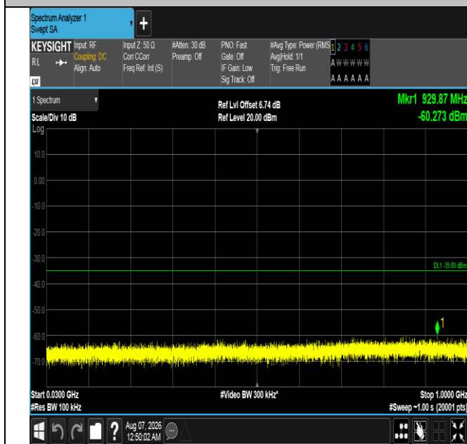
Band7-20MHz-QPSK-21350-1RB#0-30~1000-PASS
