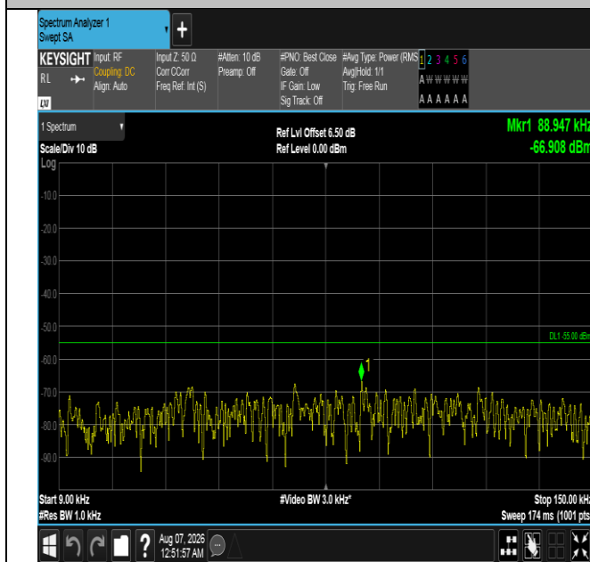
Band7-20MHz-QPSK-21350-1RB#99-0.009~0.15-PASS
