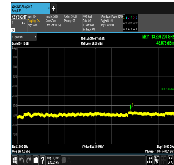
Band7-20MHz-QPSK-21350-100RB#0-3000~18000-PASS
