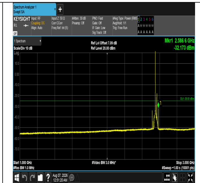
Band7-20MHz-16QAM-21350-1RB#0-1000~3000-PASS
