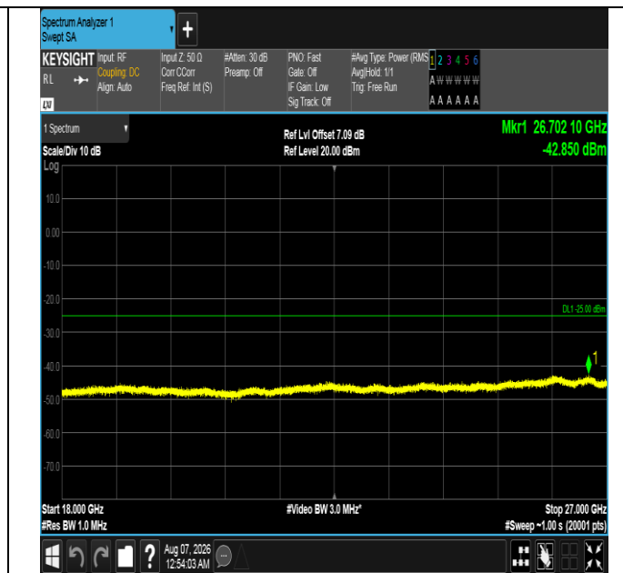
Band7-20MHz-16QAM-21350-1RB#99-18000~27000-PASS
