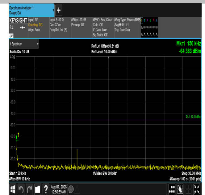
Band7-20MHz-16QAM-21350-1RB#0-0.15~30-PASS
