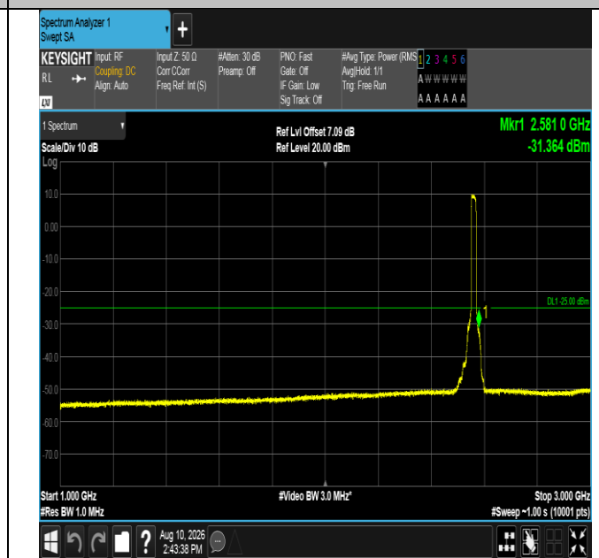
Band7-20MHz-QPSK-21350-100RB#0-1000~3000-PASS
