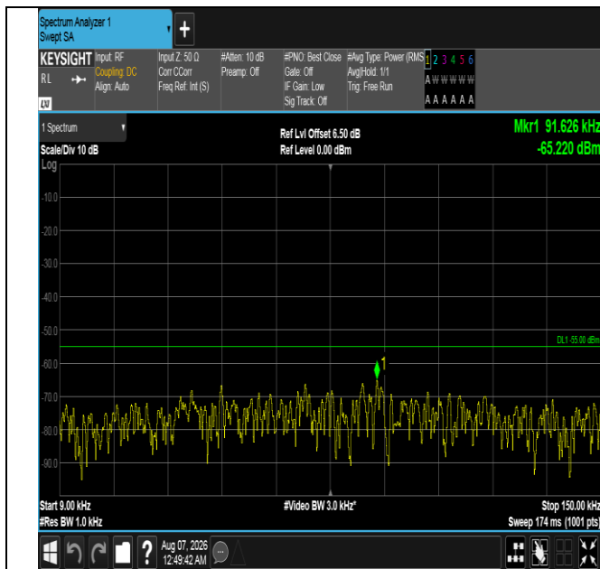
Band7-20MHz-QPSK-21350-1RB#0-0.009~0.15-PASS
