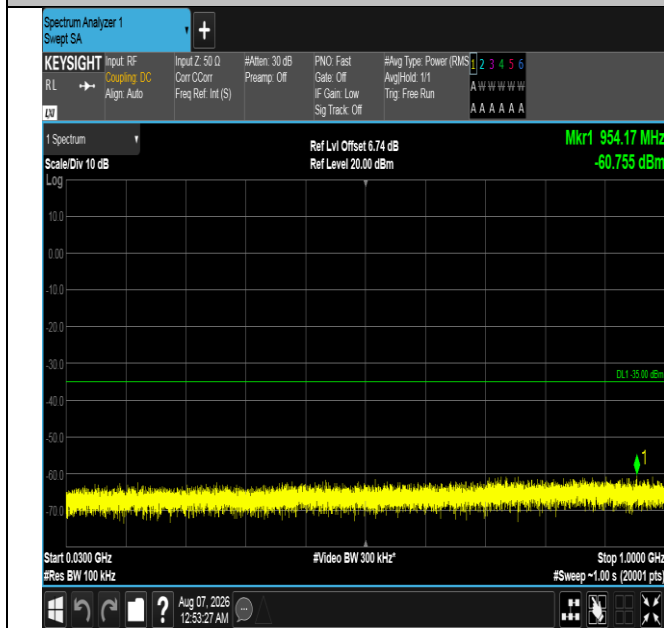
Band7-20MHz-16QAM-21350-1RB#99-30~1000-PASS
