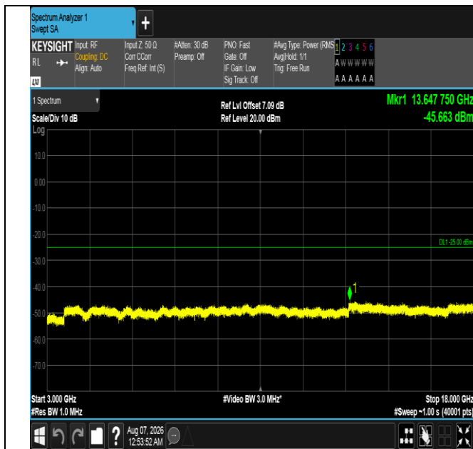
Band7-20MHz-16QAM-21350-1RB#99-3000~18000-PASS
