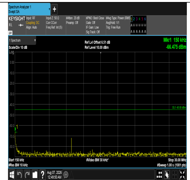
Band7-20MHz-QPSK-21350-1RB#0-0.15~30-PASS
