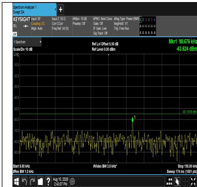
Band7-20MHz-QPSK-21350-100RB#0-0.009~0.15-PASS
