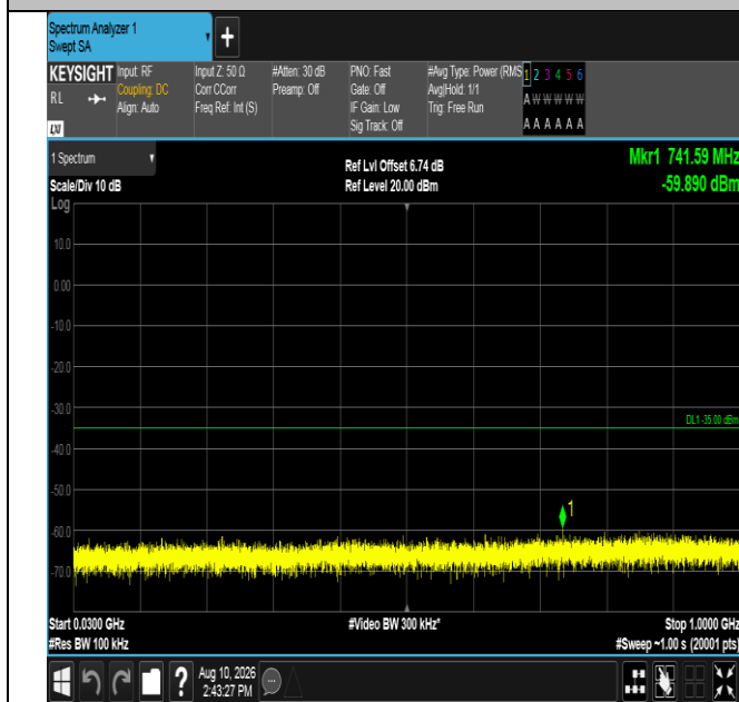
Band7-20MHz-QPSK-21350-100RB#0-30~1000-PASS
