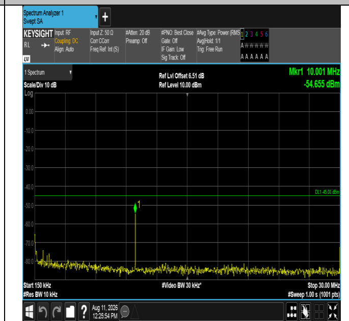
Band7-20MHz-16QAM-21350-100RB#0-0.15~30-PASS
