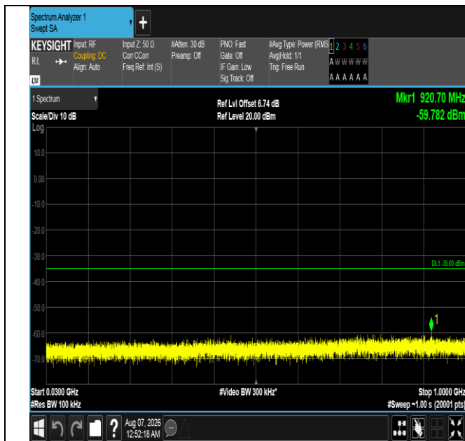
Band7-20MHz-QPSK-21350-1RB#99-30~1000-PASS
