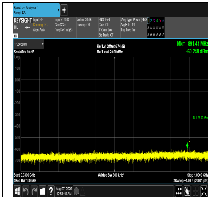
Band7-20MHz-16QAM-21350-1RB#0-30~1000-PASS
