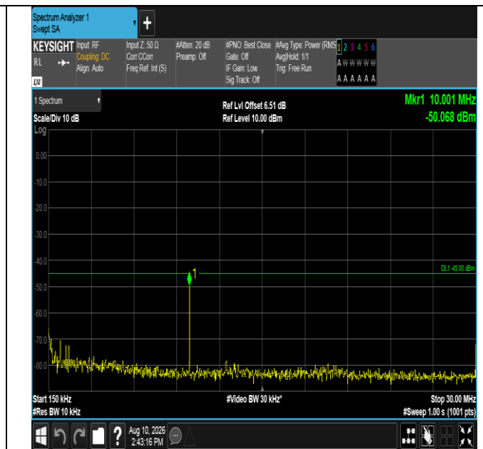
Band7-20MHz-QPSK-21350-100RB#0-0.15~30-PASS
