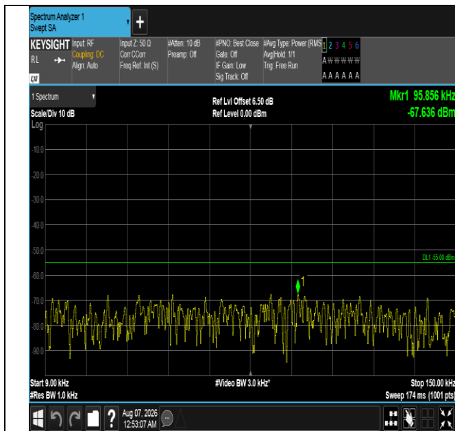
Band7-20MHz-16QAM-21350-1RB#99-0.009~0.15-PASS
