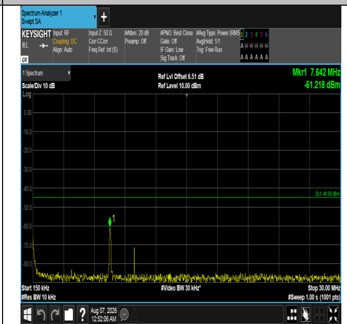
Band7-20MHz-QPSK-21350-1RB#99-0.15~30-PASS
