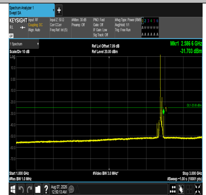
Band7-20MHz-QPSK-21350-1RB#0-1000~3000-PASS
