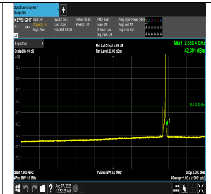
Band7-20MHz-QPSK-21350-1RB#99-1000~3000-PASS
