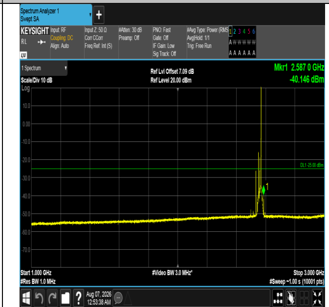
Band7-20MHz-16QAM-21350-1RB#99-1000~3000-PASS
