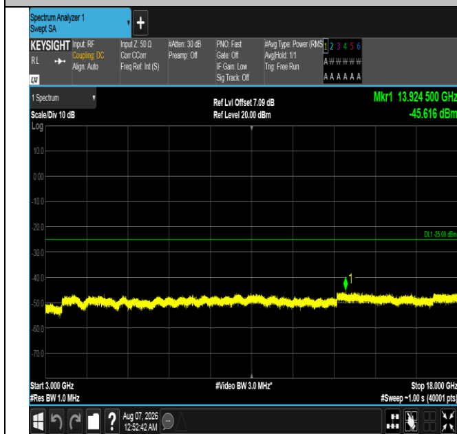
Band7-20MHz-QPSK-21350-1RB#99-3000~18000-PASS
