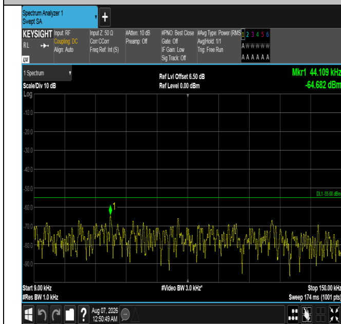
Band7-20MHz-16QAM-21350-1RB#0-0.009~0.15-PASS
