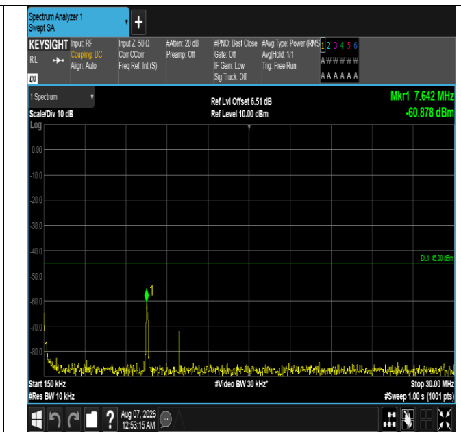
Band7-20MHz-16QAM-21350-1RB#99-0.15~30-PASS
