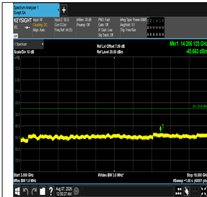
Band7-20MHz-QPSK-21350-1RB#0-3000~18000-PASS
