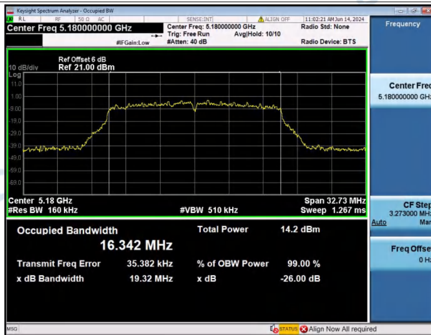
99%_OCB_NVNT_ANT1_802_11a_5180
