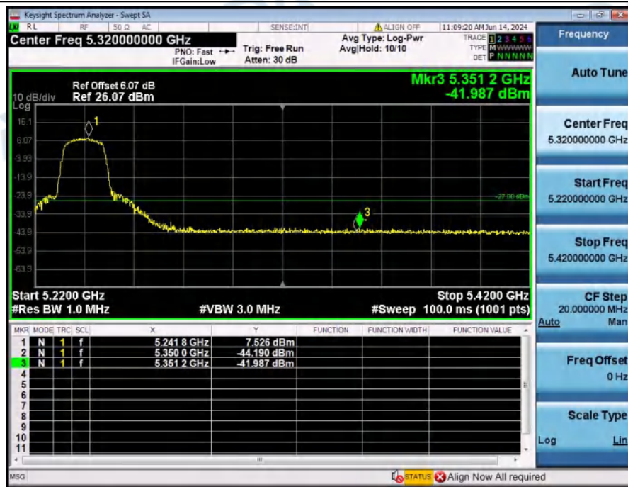
Bandedge_NVNT_ANT1_802_11a_5240
