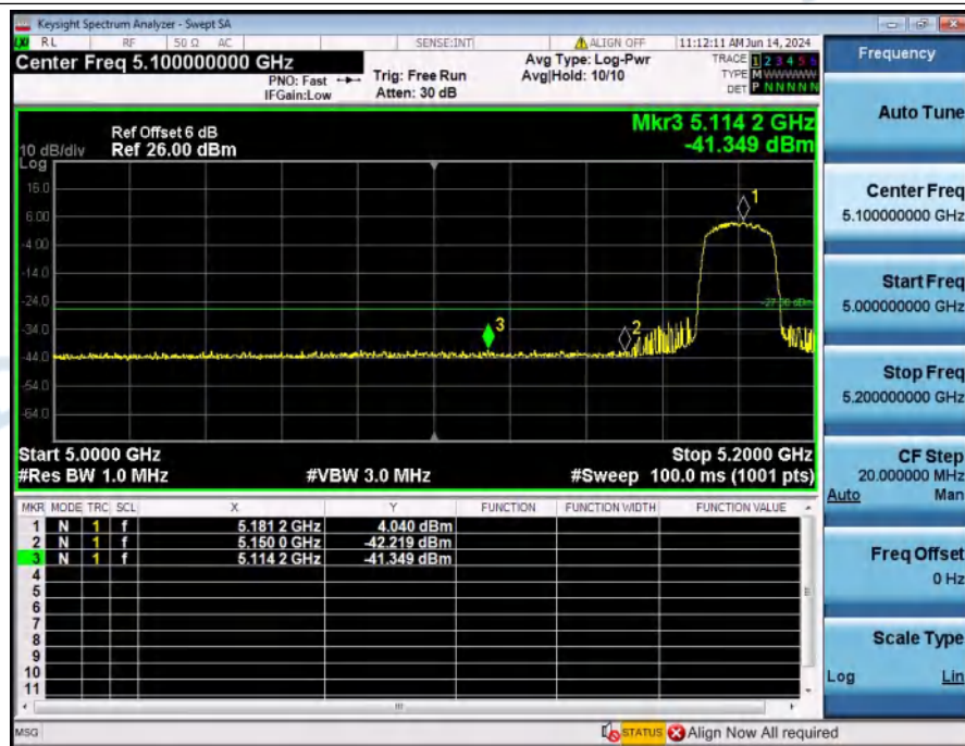
Bandedge_NVNT_ANT1_802_11n(HT20)_5180
