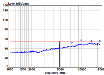
BT_3DH5_TX_CH_39_Horizontal
