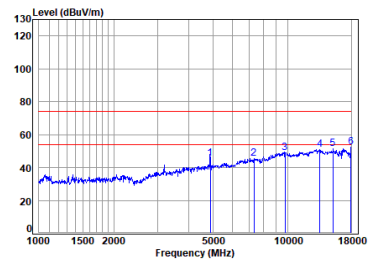
BT_3DH5_TX_CH_39_Vertical
