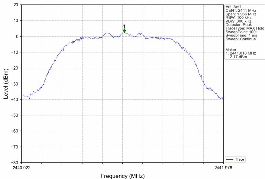
8DPSK_3DH5_MCH_2441MHz_Ant1_NTNV
