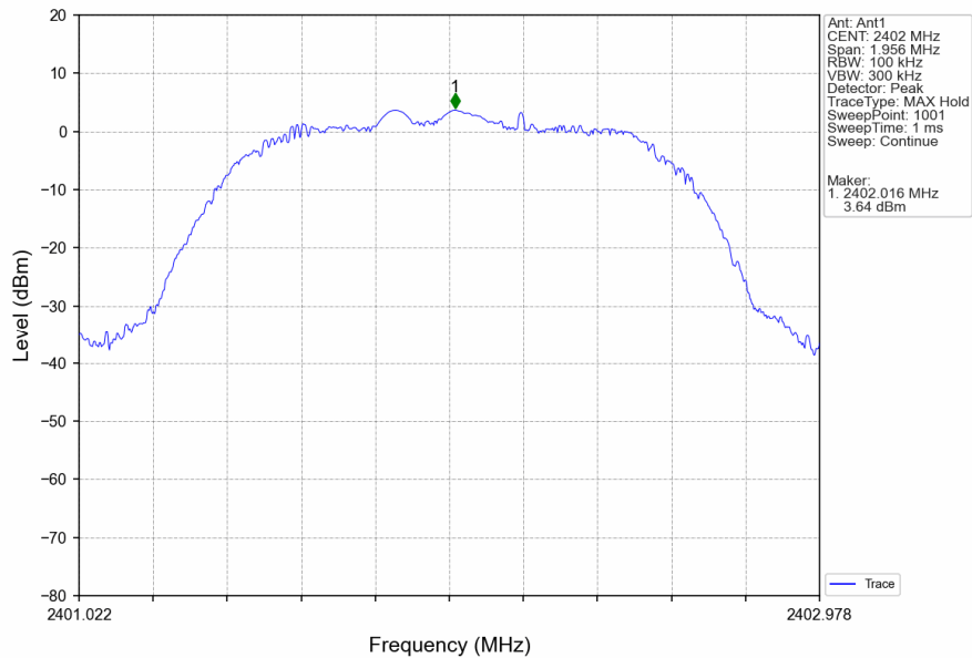
8DPSK_3DH5_LCH_2402MHz_Ant1_NTNV
