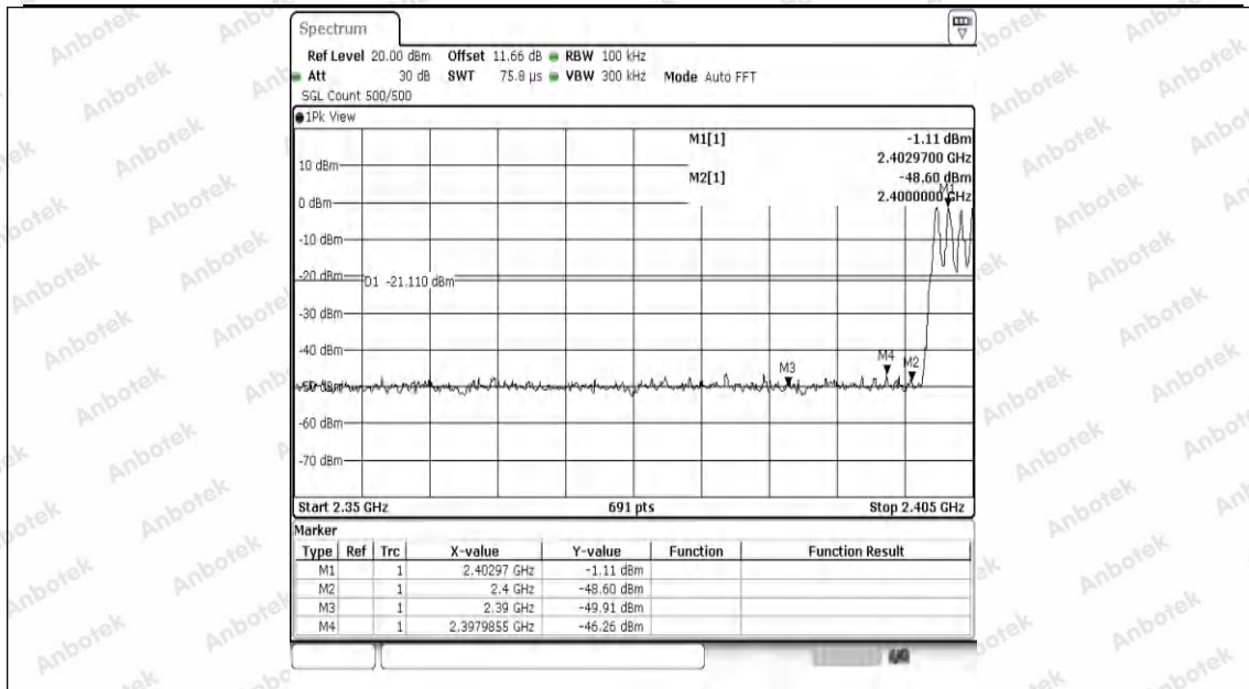
2.4G-Ant1-Hop_2402-PASS
