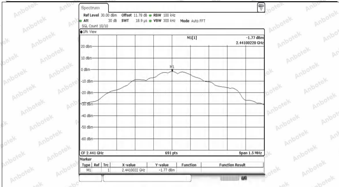
2.4G-Ant1-2441-0~Reference-PASS
