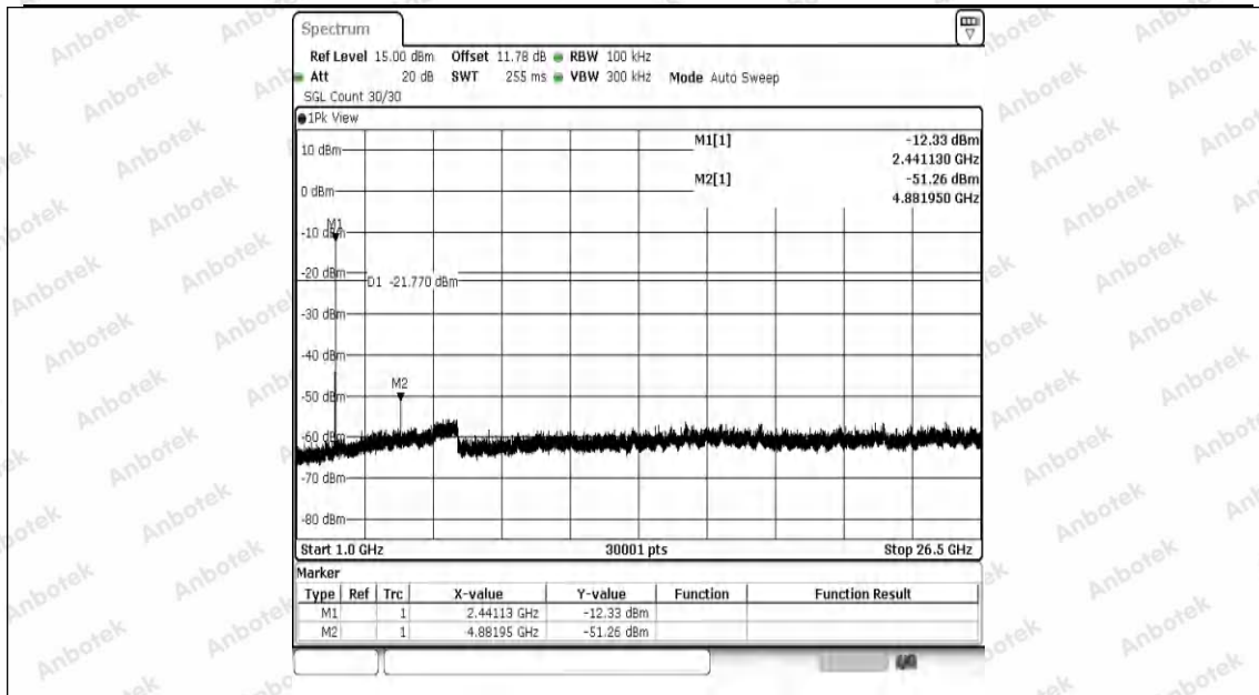
2.4G-Ant1-2441-1000~26500-PASS
