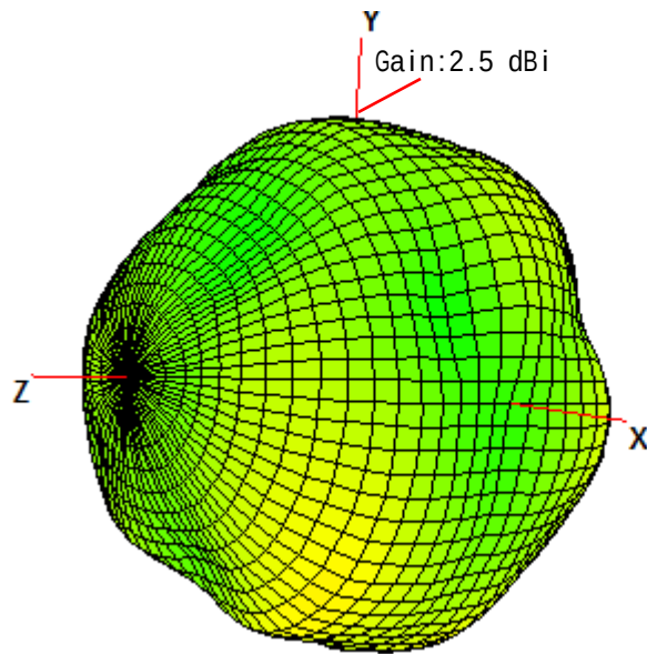
Figure 7. 3D Radiation Pattern at 2450 of the FXP75 Antenna.
