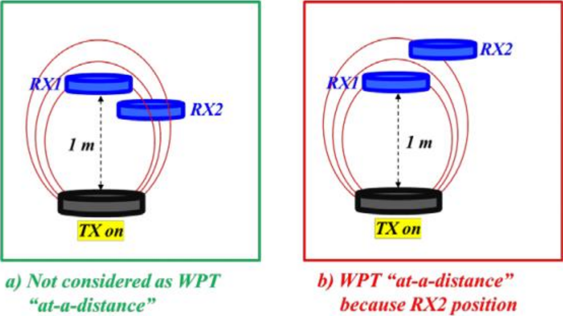
Figure 2-a) For multiple-receiver systems (here shown with two receivers, indicated with RX1 and RX2) the one-meter distance limit must apply for all the receivers that are engaged in the charging process. b) The WPT system is considered “at-a-distance” because it can function when the RX2 is further away than one meter from the transmitter.
