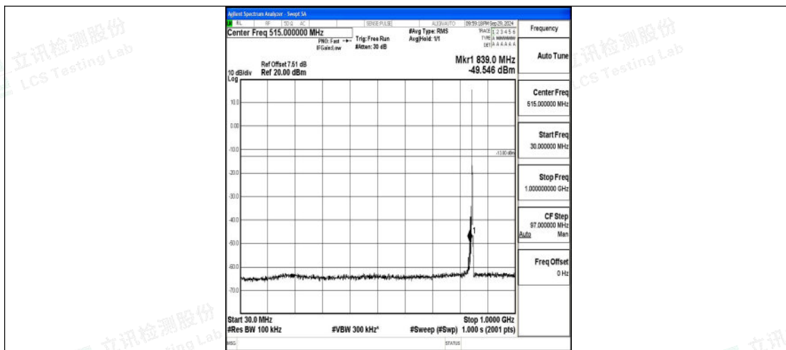
Band5_3MHz_16QAM_20635_1RB#0_30~1000_30~1000
